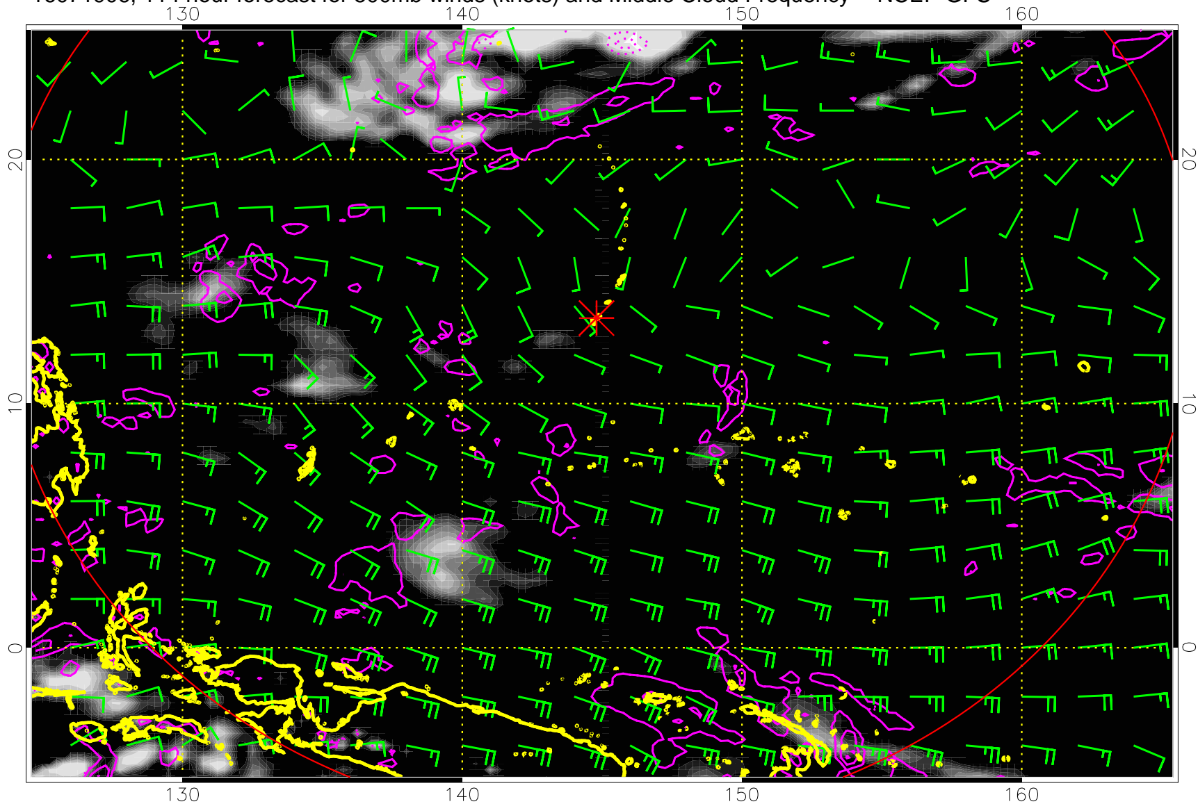
16071906, 114 hour forecast for 500mb winds (knots) and Middle Cloud Frequency -- NCEP GFS
