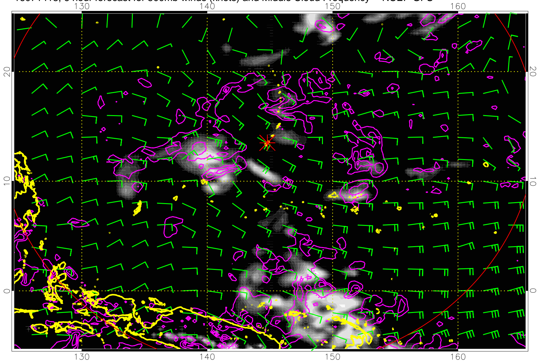
16071418, 6 hour forecast for 500mb winds (knots) and Middle Cloud Frequency -- NCEP GFS
