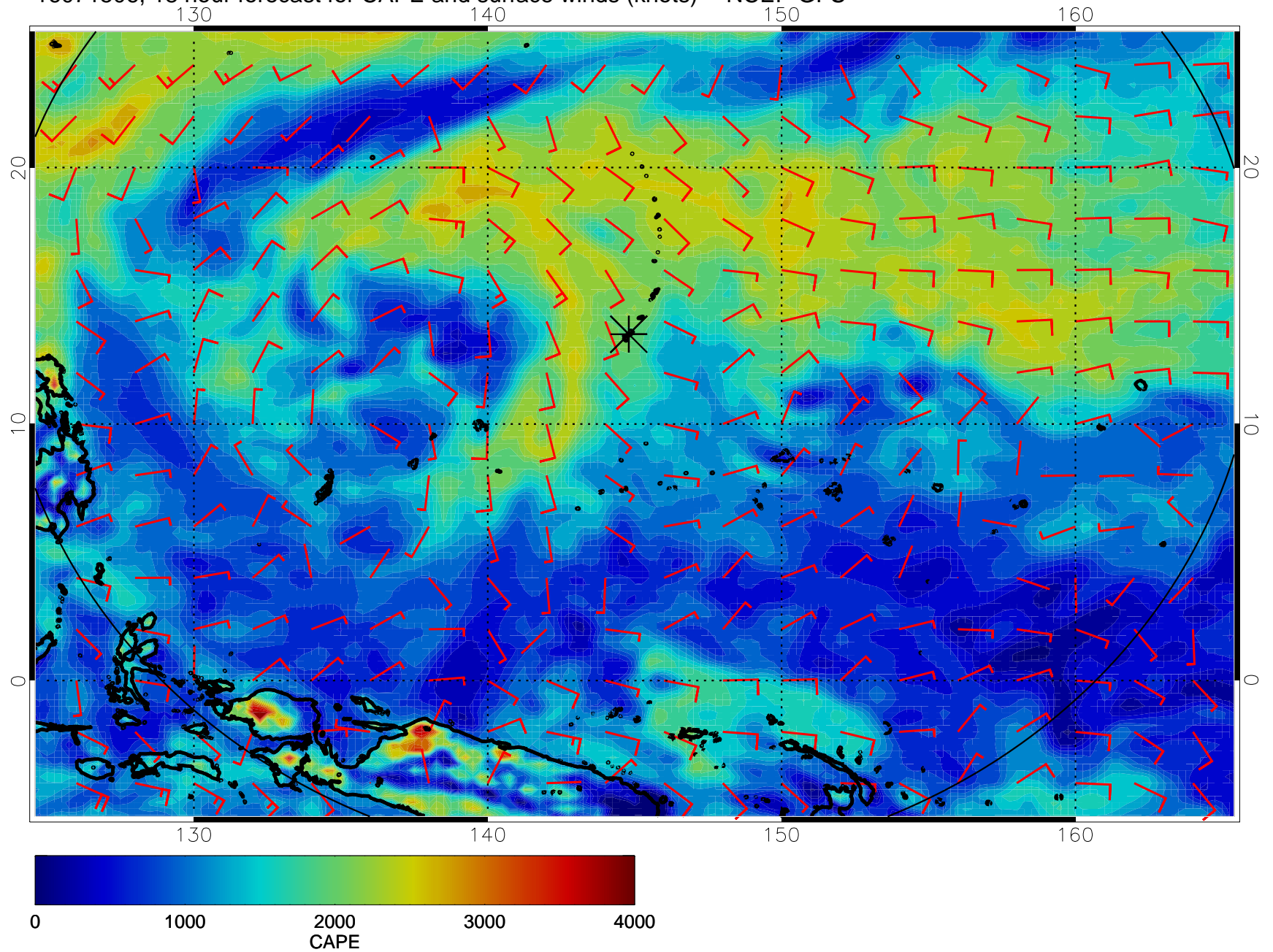
16071506, 18 hour forecast for CAPE and surface winds (knots) -- NCEP GFS
