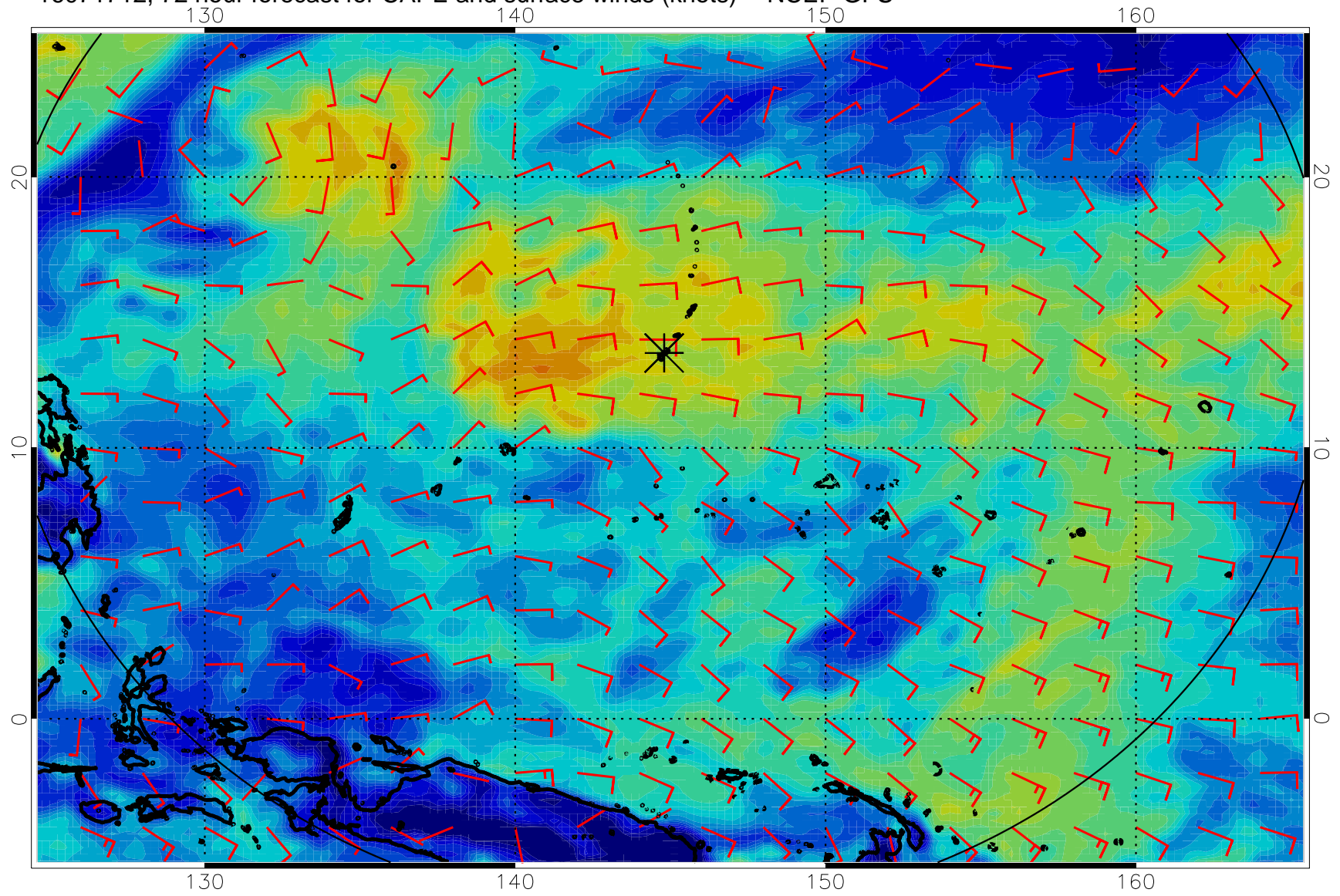
16071712, 72 hour forecast for CAPE and surface winds (knots) -- NCEP GFS
