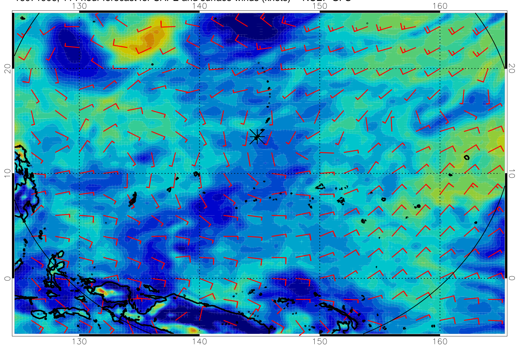
16071906, 114 hour forecast for CAPE and surface winds (knots) -- NCEP GFS
