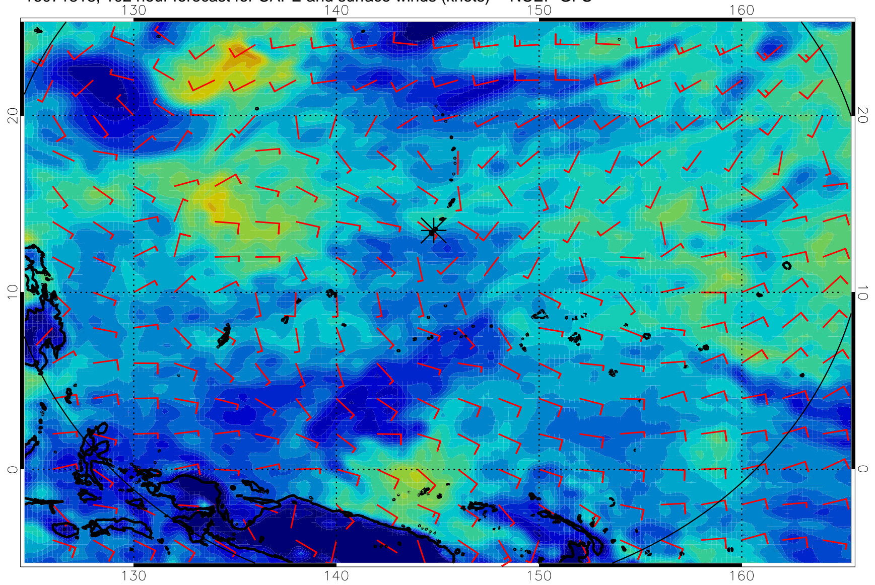
16071818, 102 hour forecast for CAPE and surface winds (knots) -- NCEP GFS
