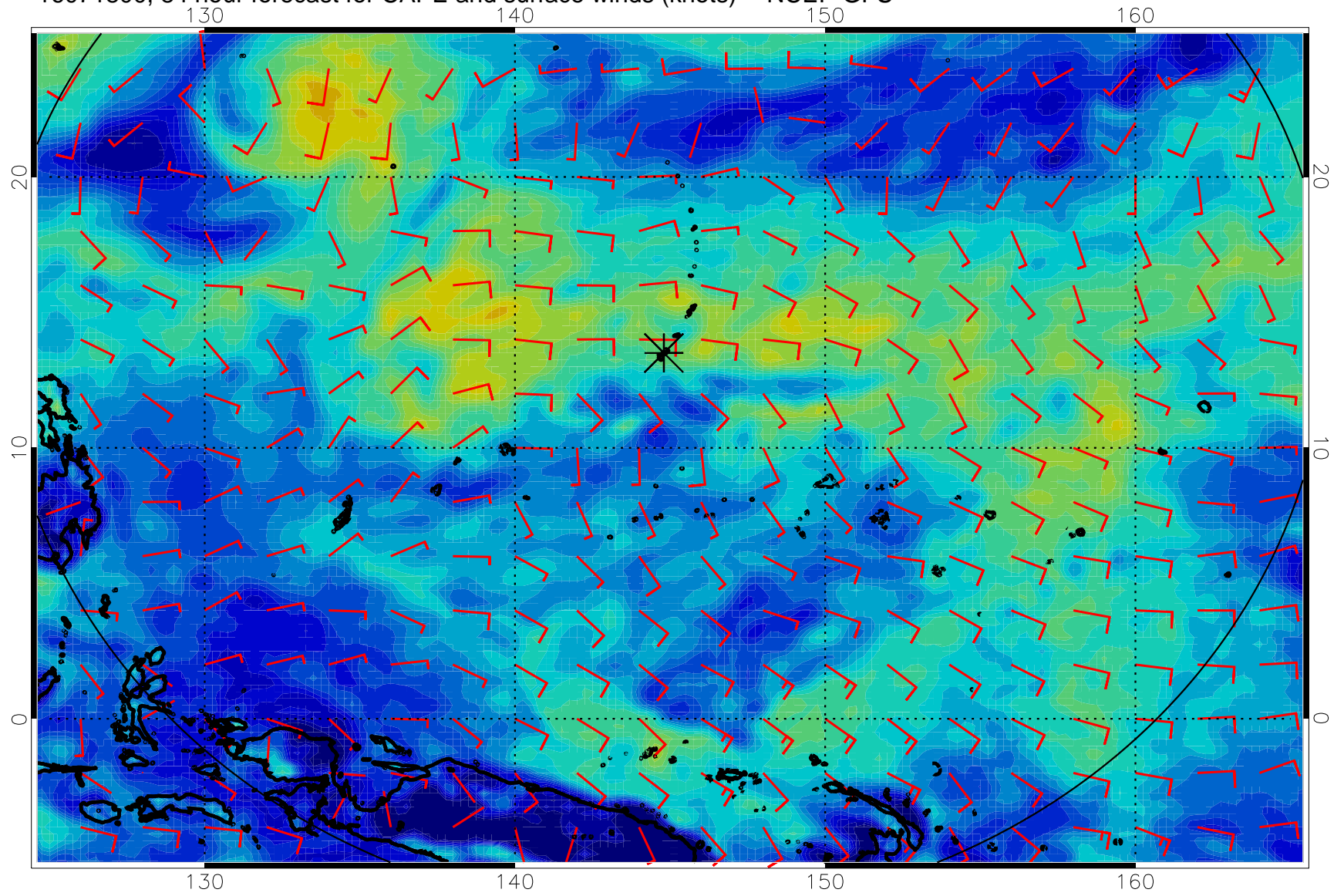
16071800, 84 hour forecast for CAPE and surface winds (knots) -- NCEP GFS
