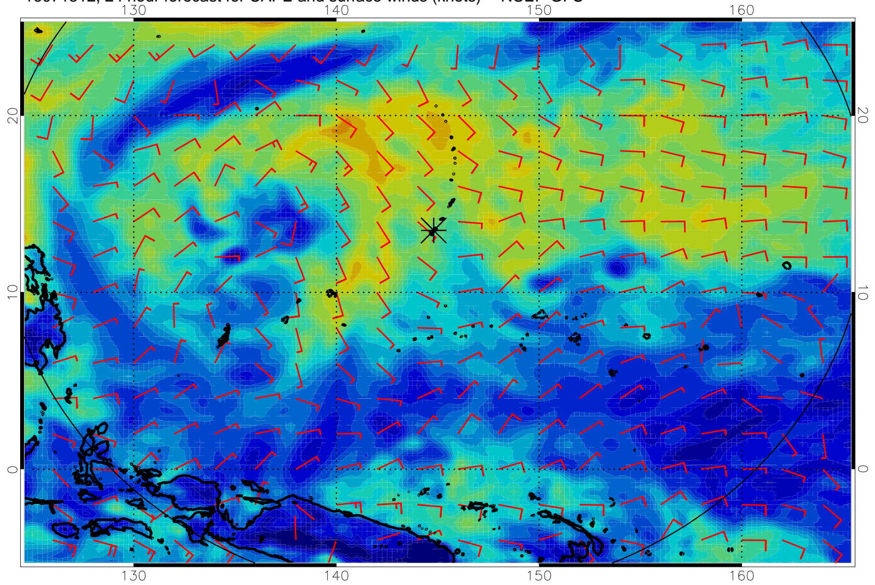
16071512, 24 hour forecast for CAPE and surface winds (knots) -- NCEP GFS
