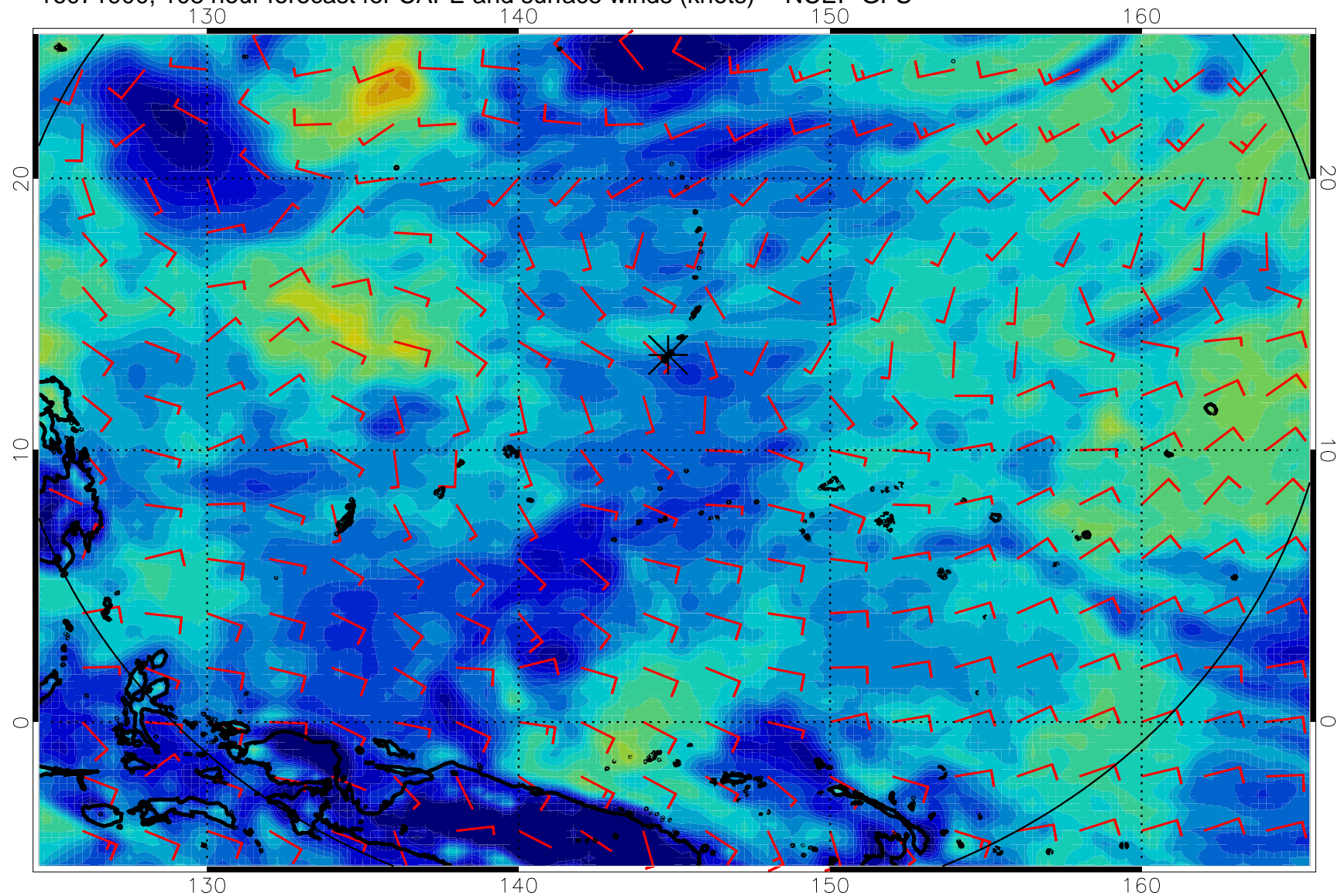
16071900, 108 hour forecast for CAPE and surface winds (knots) -- NCEP GFS
