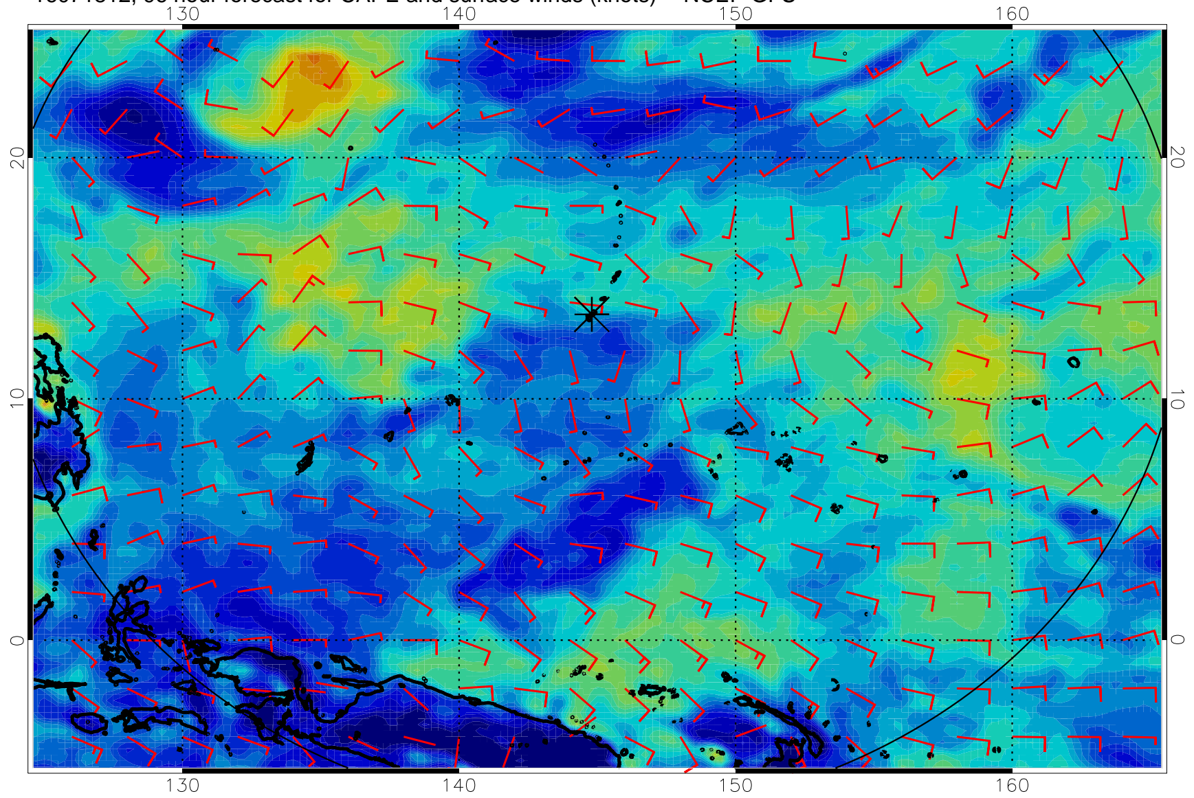
16071812, 96 hour forecast for CAPE and surface winds (knots) -- NCEP GFS
