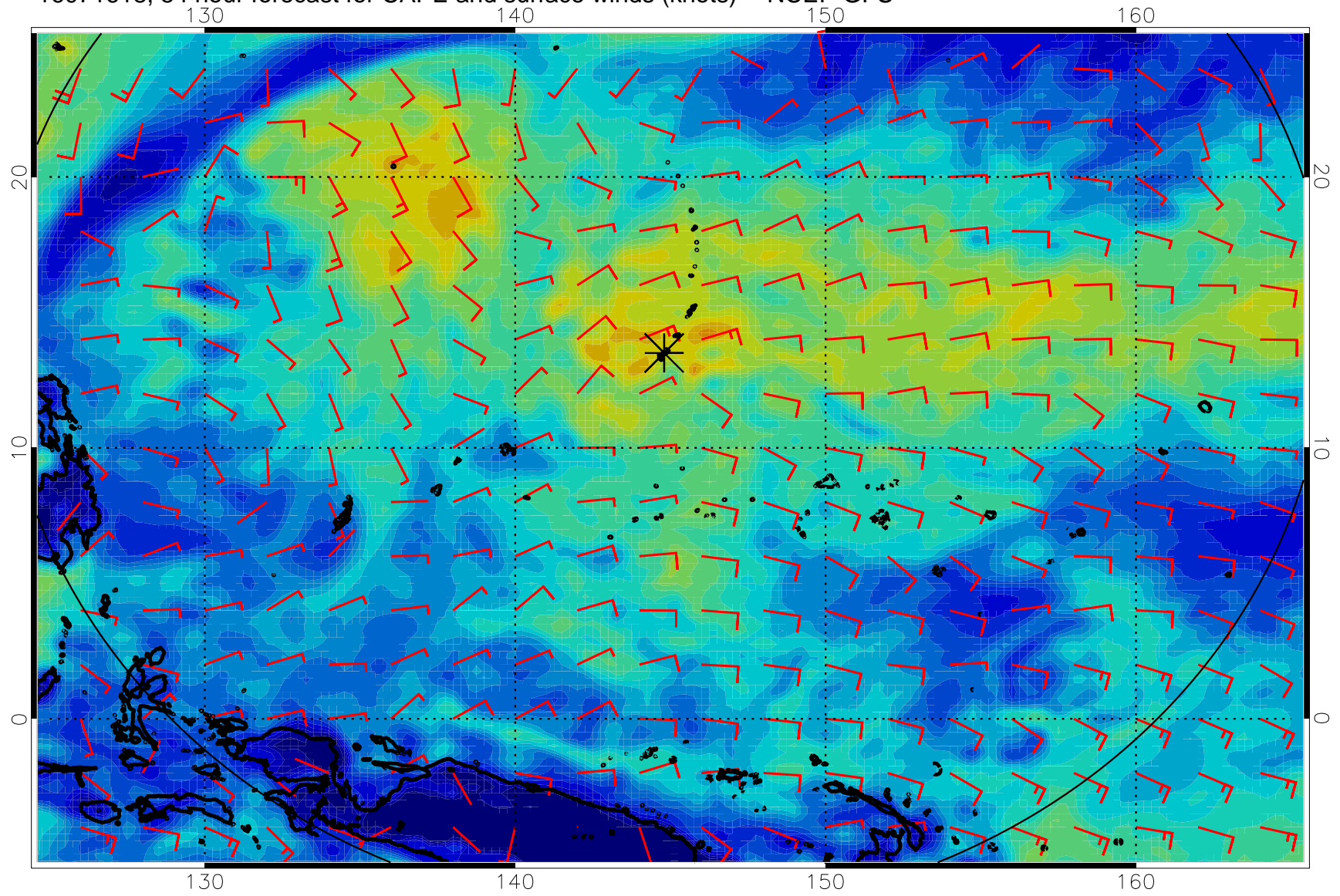
16071618, 54 hour forecast for CAPE and surface winds (knots) -- NCEP GFS
