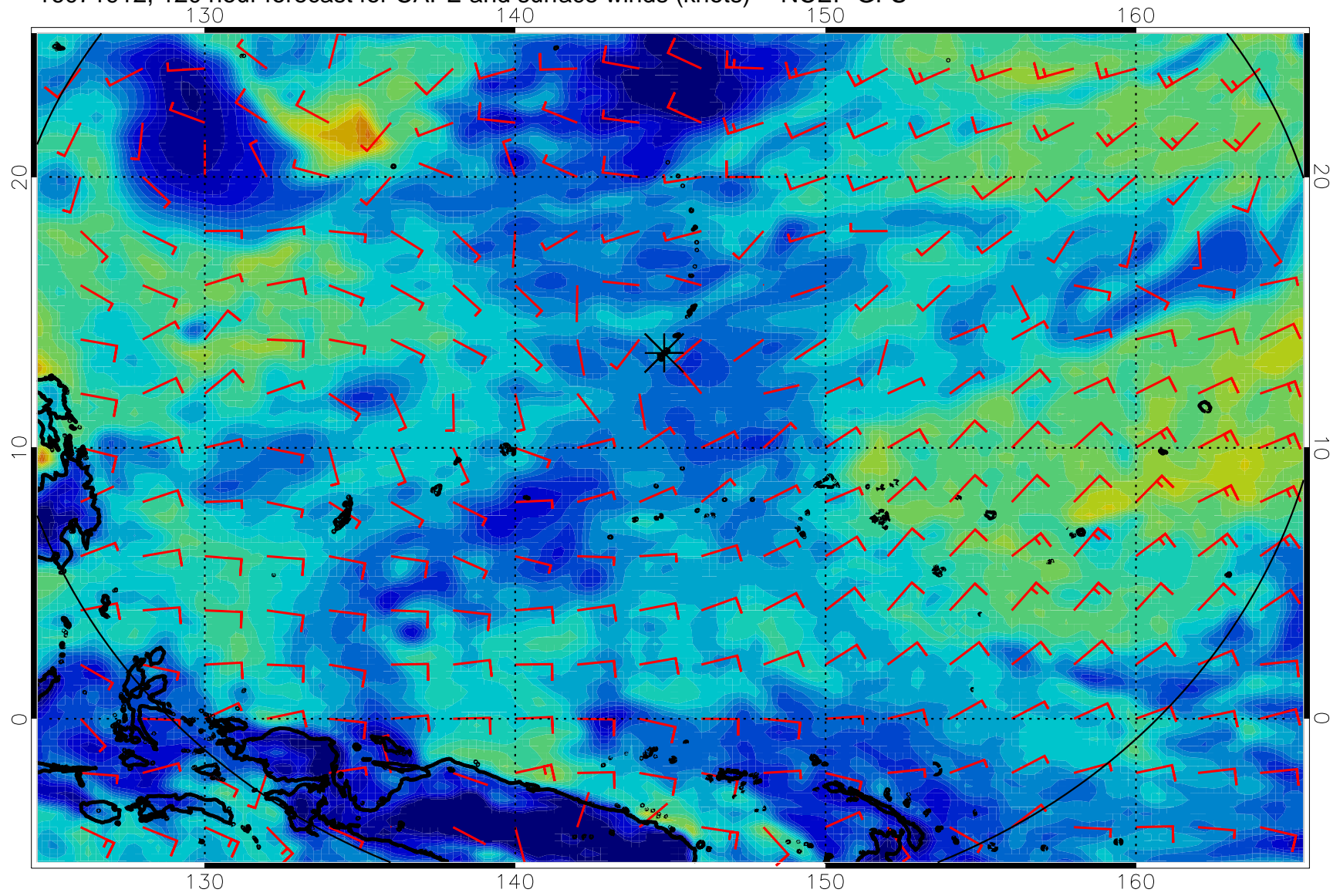
16071912, 120 hour forecast for CAPE and surface winds (knots) -- NCEP GFS
