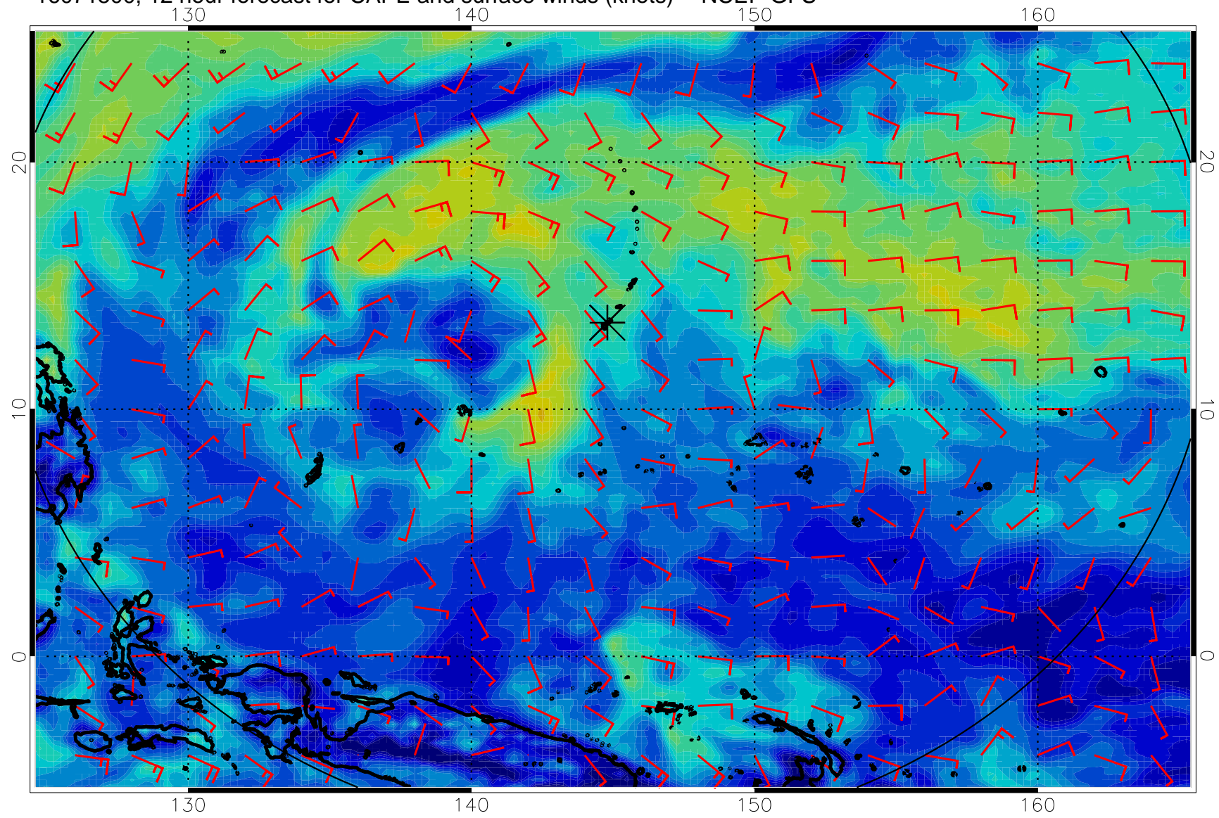
16071500, 12 hour forecast for CAPE and surface winds (knots) -- NCEP GFS
