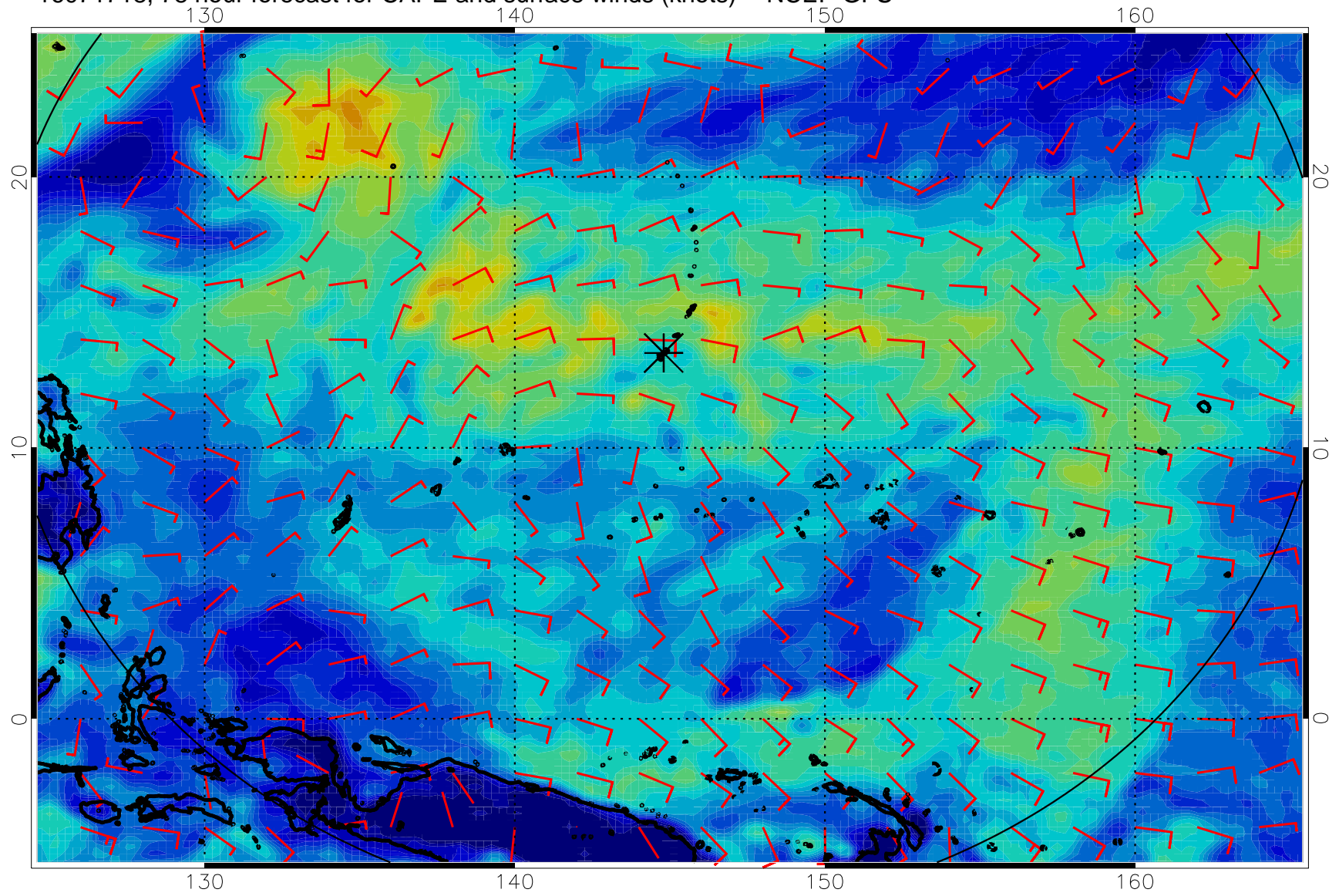
16071718, 78 hour forecast for CAPE and surface winds (knots) -- NCEP GFS
