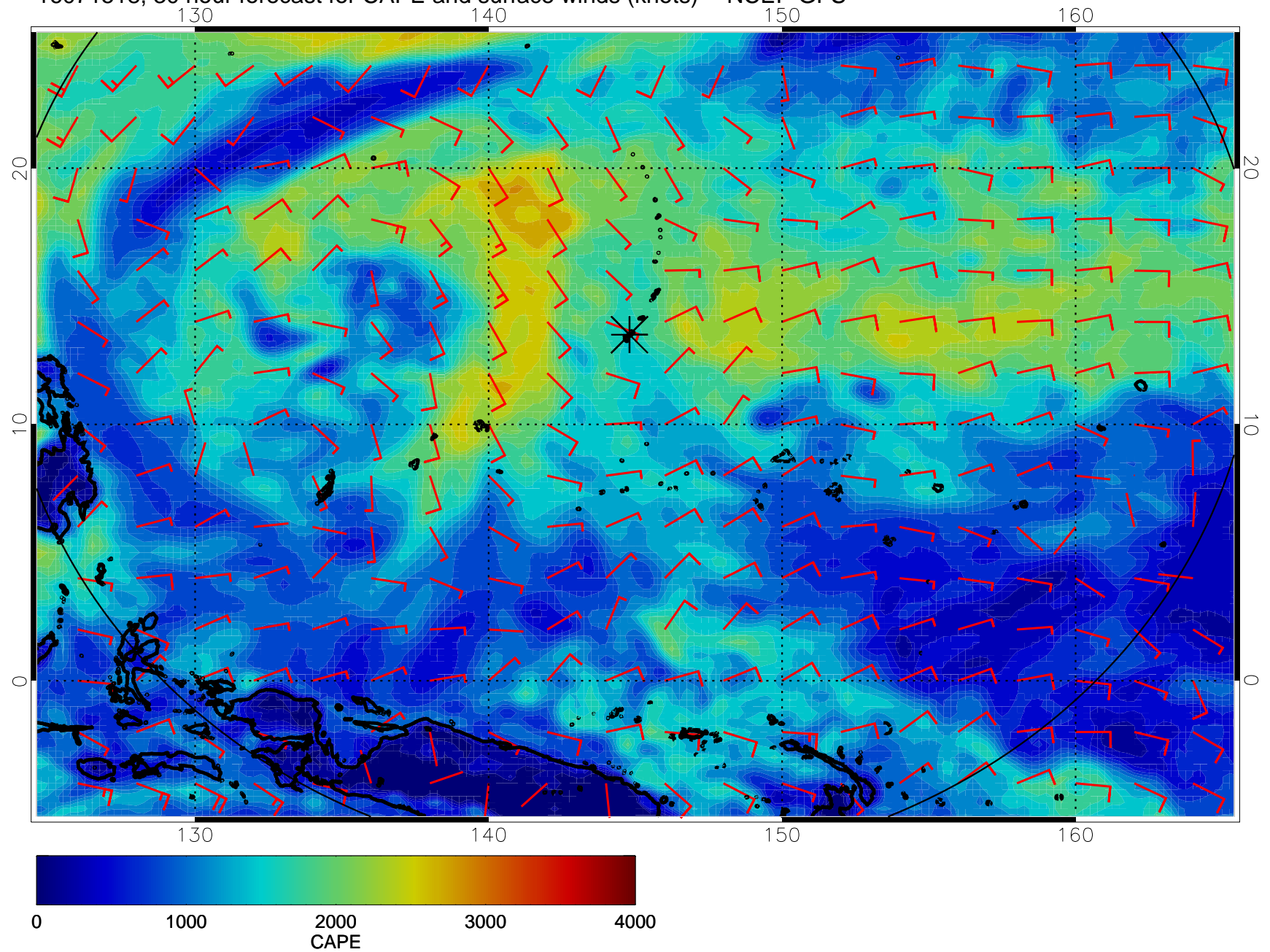
16071518, 30 hour forecast for CAPE and surface winds (knots) -- NCEP GFS
