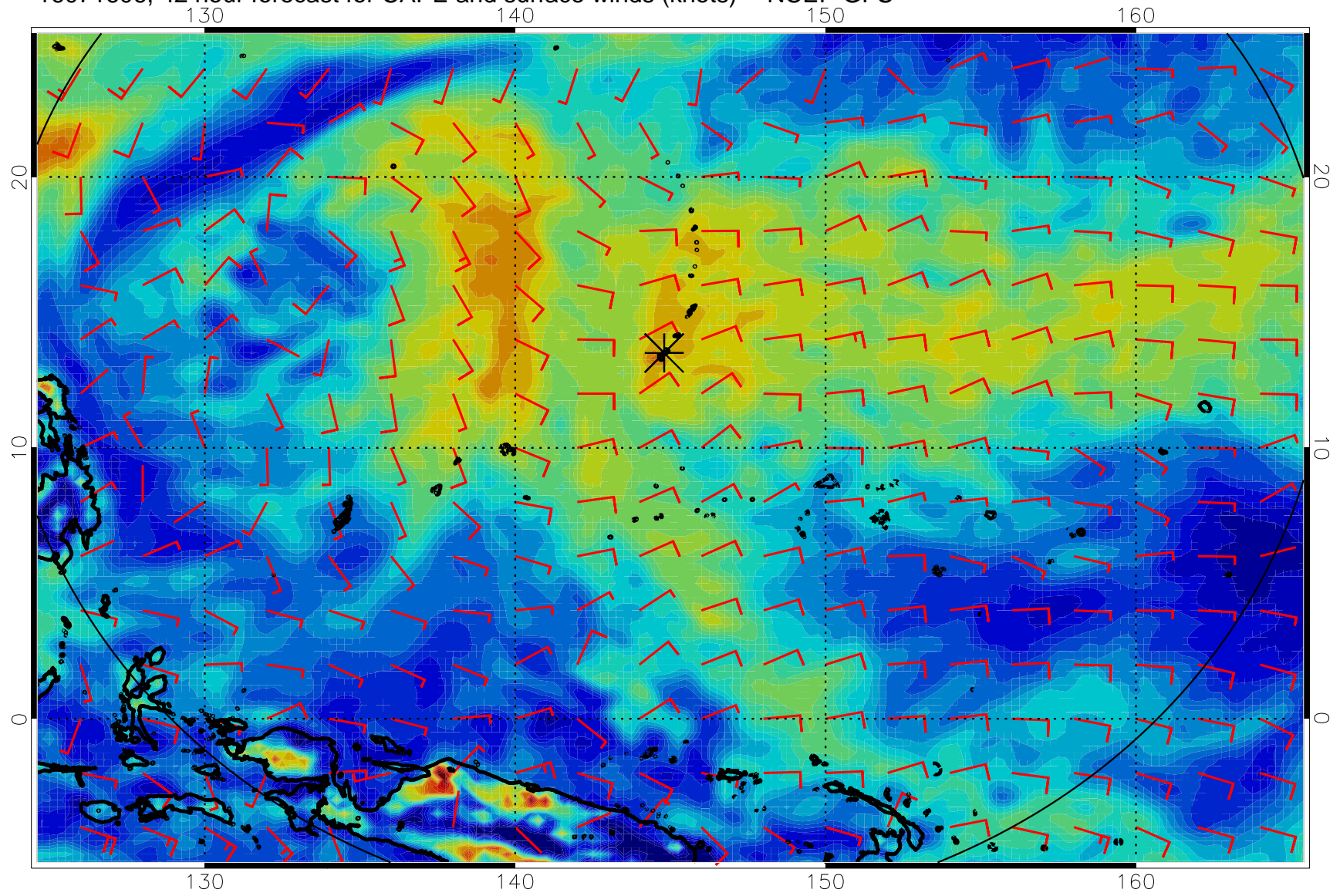
16071606, 42 hour forecast for CAPE and surface winds (knots) -- NCEP GFS
