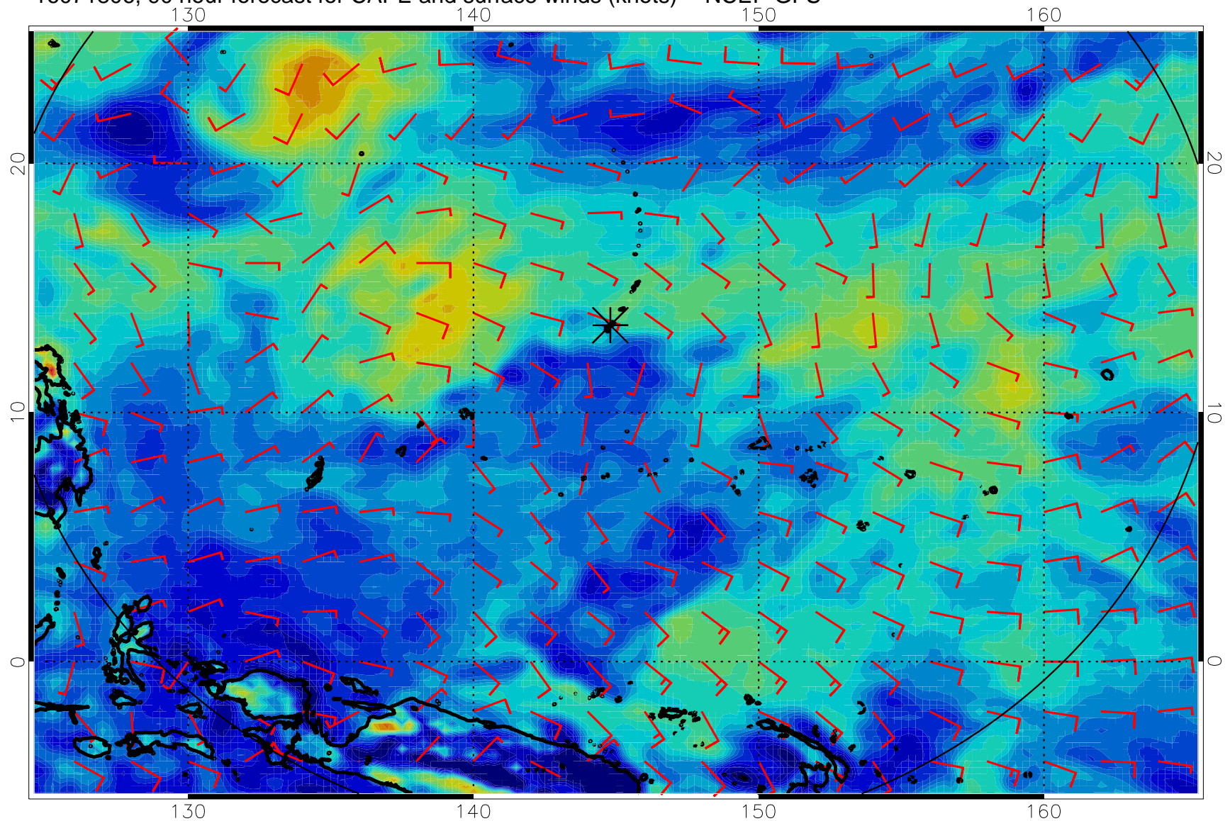
16071806, 90 hour forecast for CAPE and surface winds (knots) -- NCEP GFS
