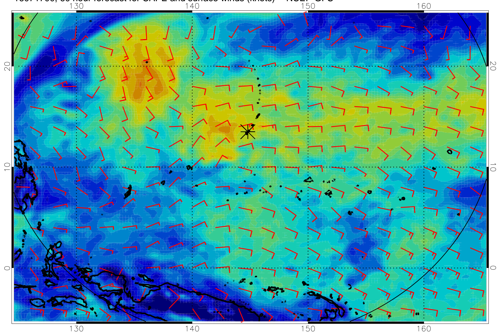
16071700, 60 hour forecast for CAPE and surface winds (knots) -- NCEP GFS
