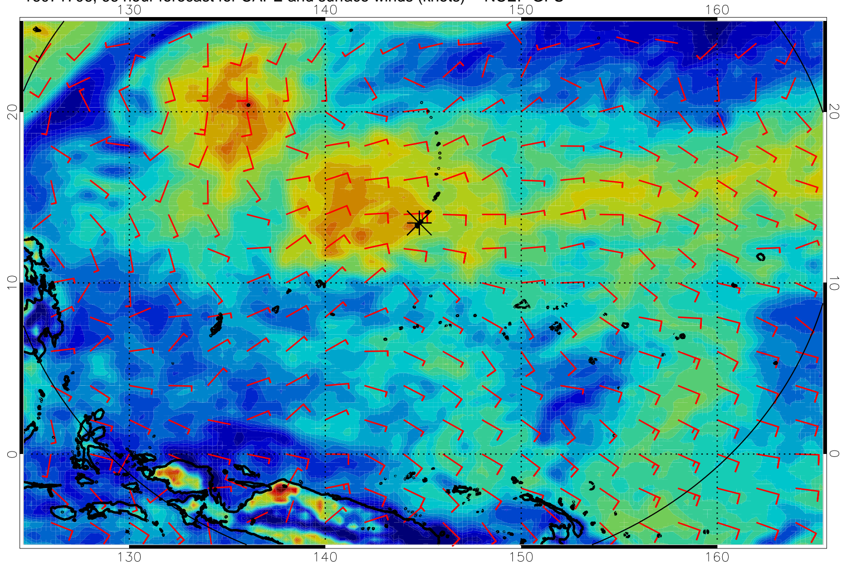
16071706, 66 hour forecast for CAPE and surface winds (knots) -- NCEP GFS
