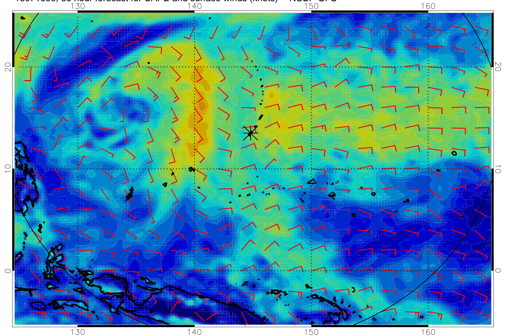
16071600, 36 hour forecast for CAPE and surface winds (knots) -- NCEP GFS
