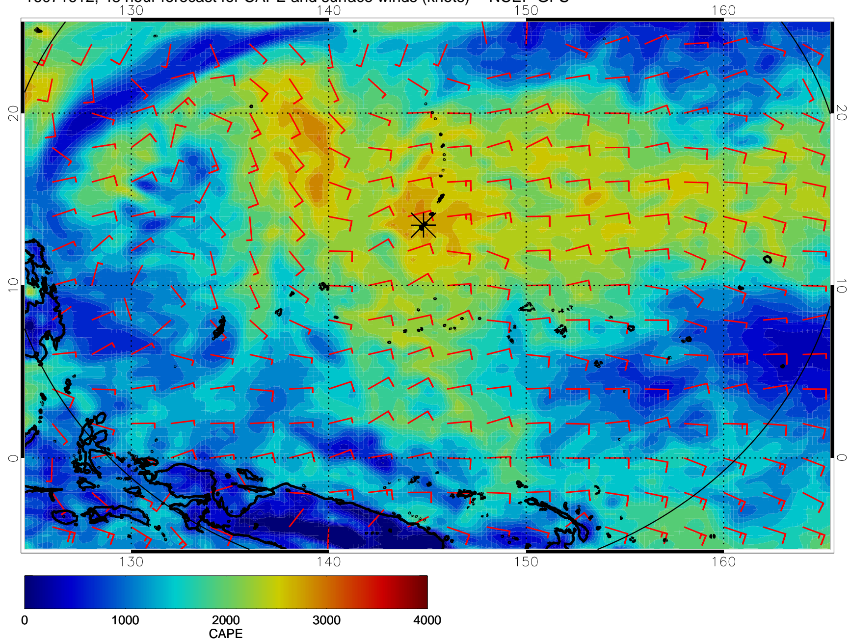
16071612, 48 hour forecast for CAPE and surface winds (knots) -- NCEP GFS
