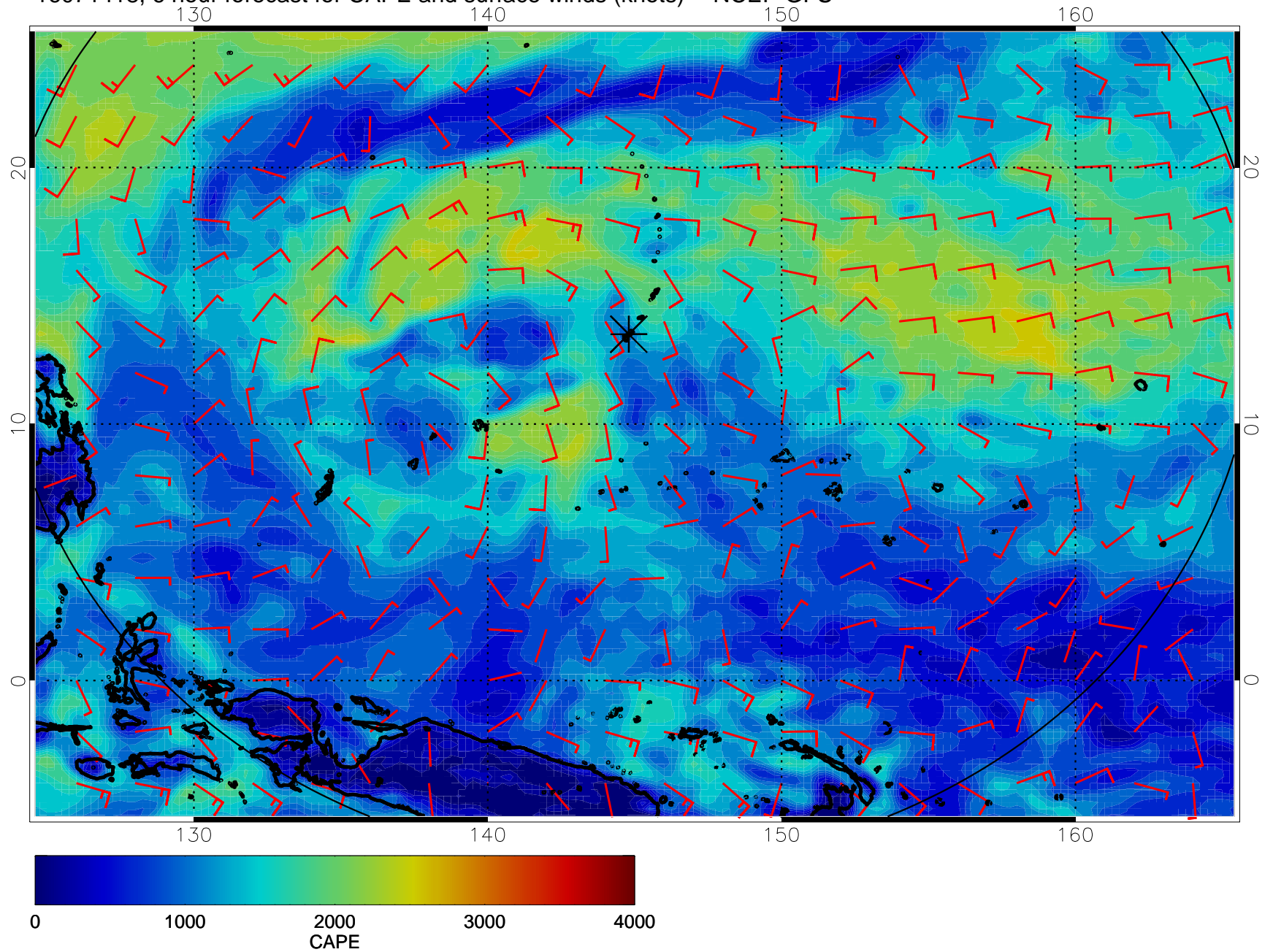
16071418, 6 hour forecast for CAPE and surface winds (knots) -- NCEP GFS
