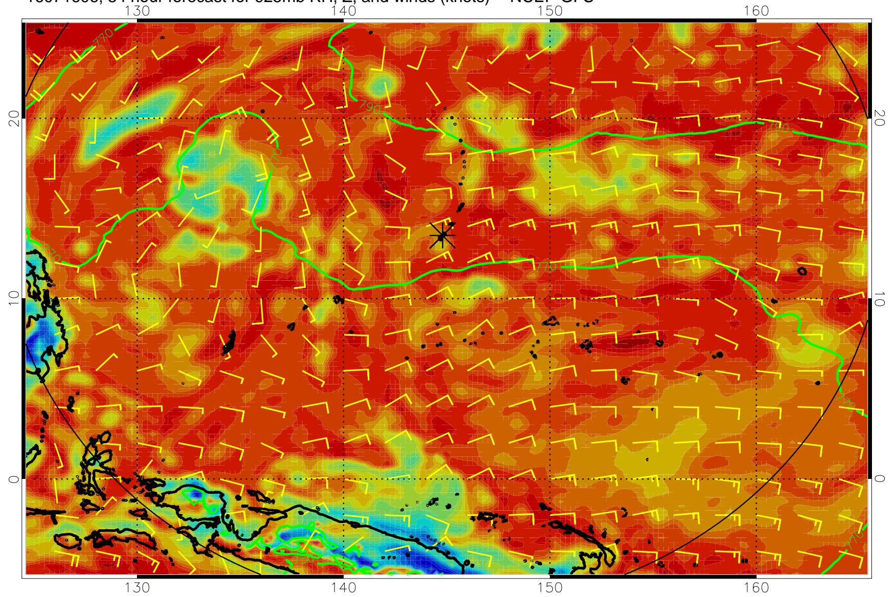
16071606, 54 hour forecast for 925mb RH, Z, and winds (knots) -- NCEP GFS
