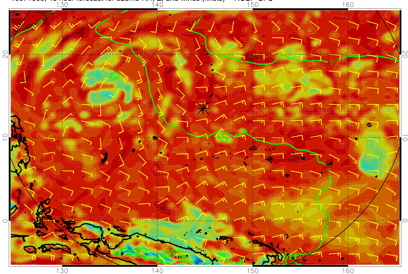
16071600, 48 hour forecast for 925mb RH, Z, and winds (knots) -- NCEP GFS
