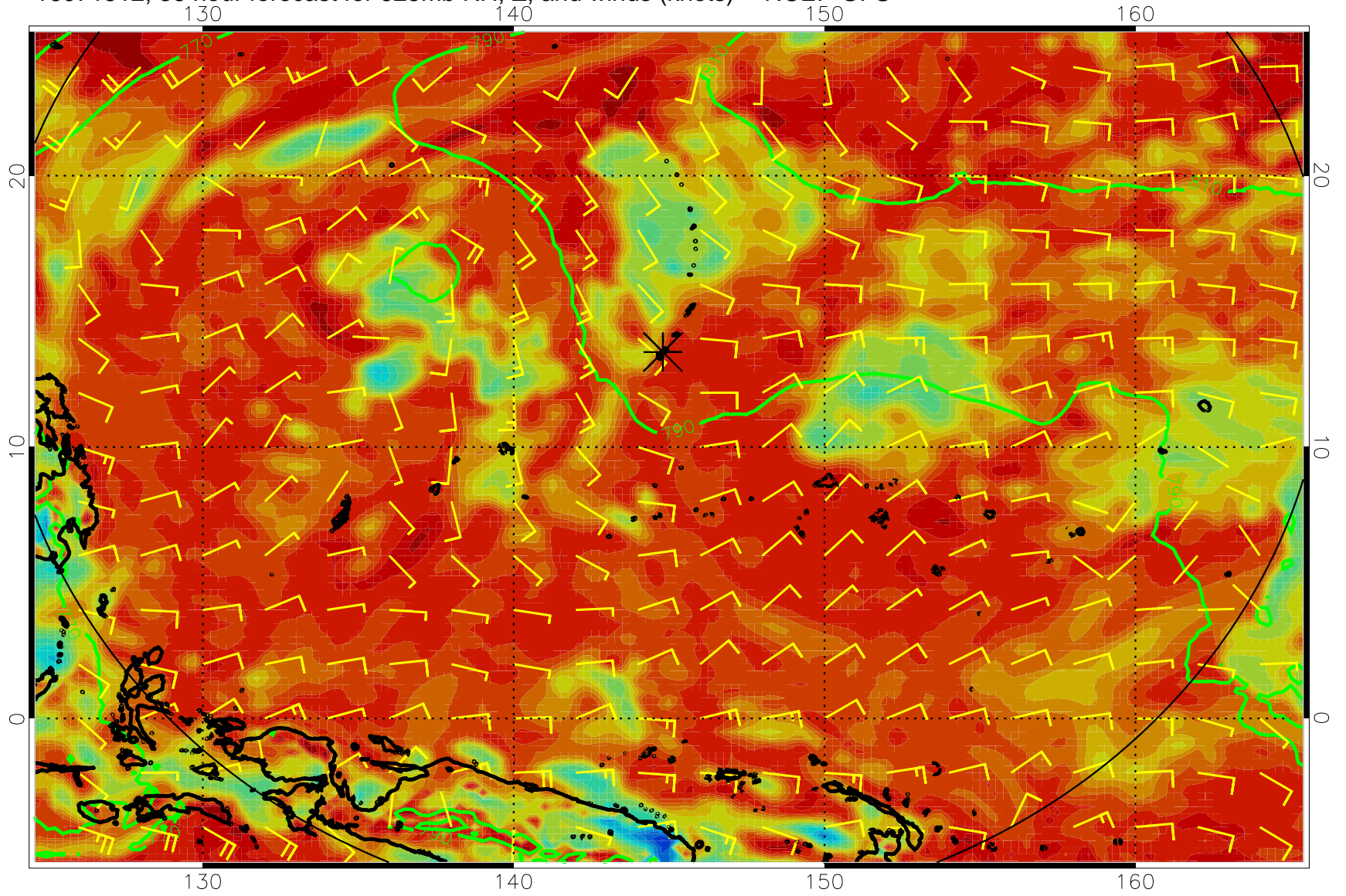
16071512, 36 hour forecast for 925mb RH, Z, and winds (knots) -- NCEP GFS
