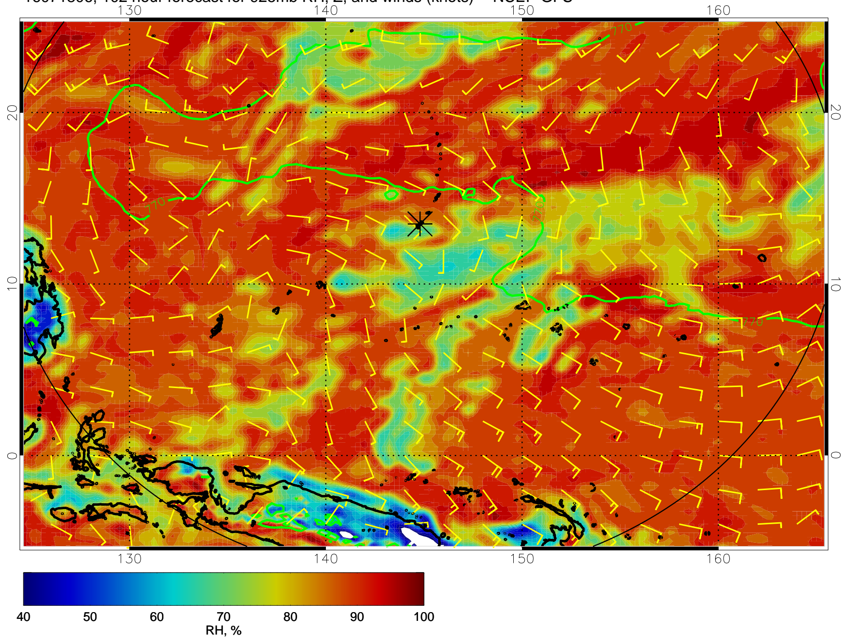
16071806, 102 hour forecast for 925mb RH, Z, and winds (knots) -- NCEP GFS
