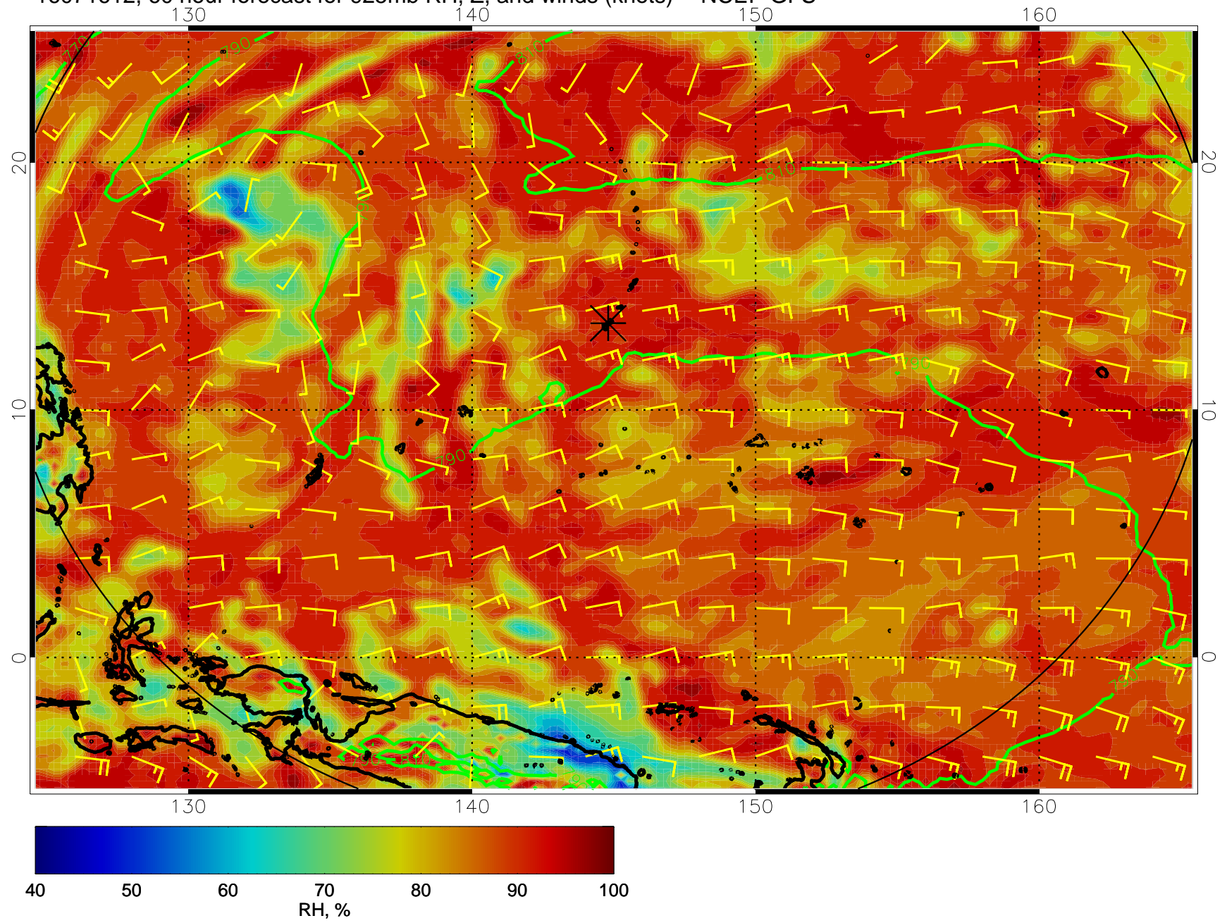
16071612, 60 hour forecast for 925mb RH, Z, and winds (knots) -- NCEP GFS
