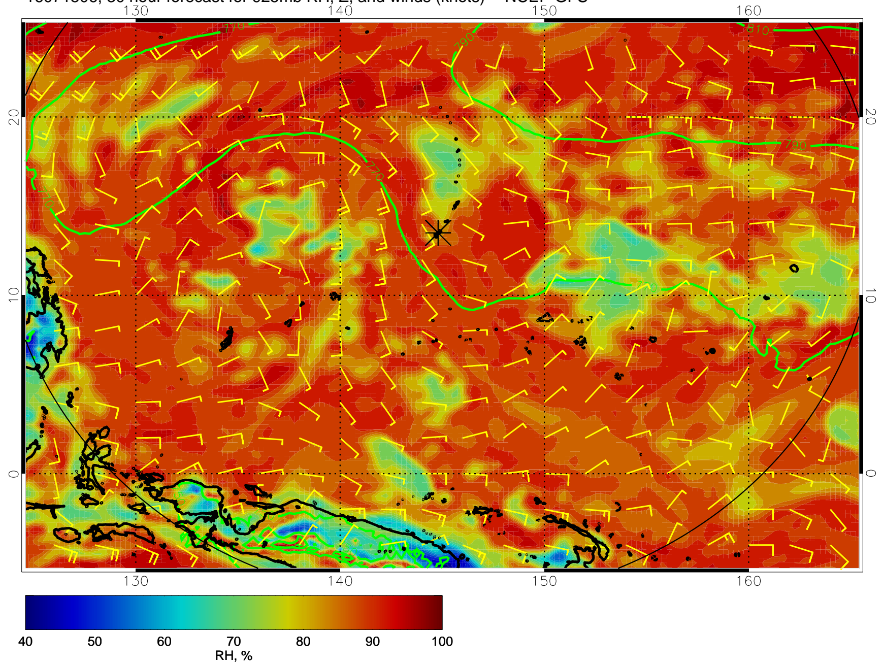
16071506, 30 hour forecast for 925mb RH, Z, and winds (knots) -- NCEP GFS
