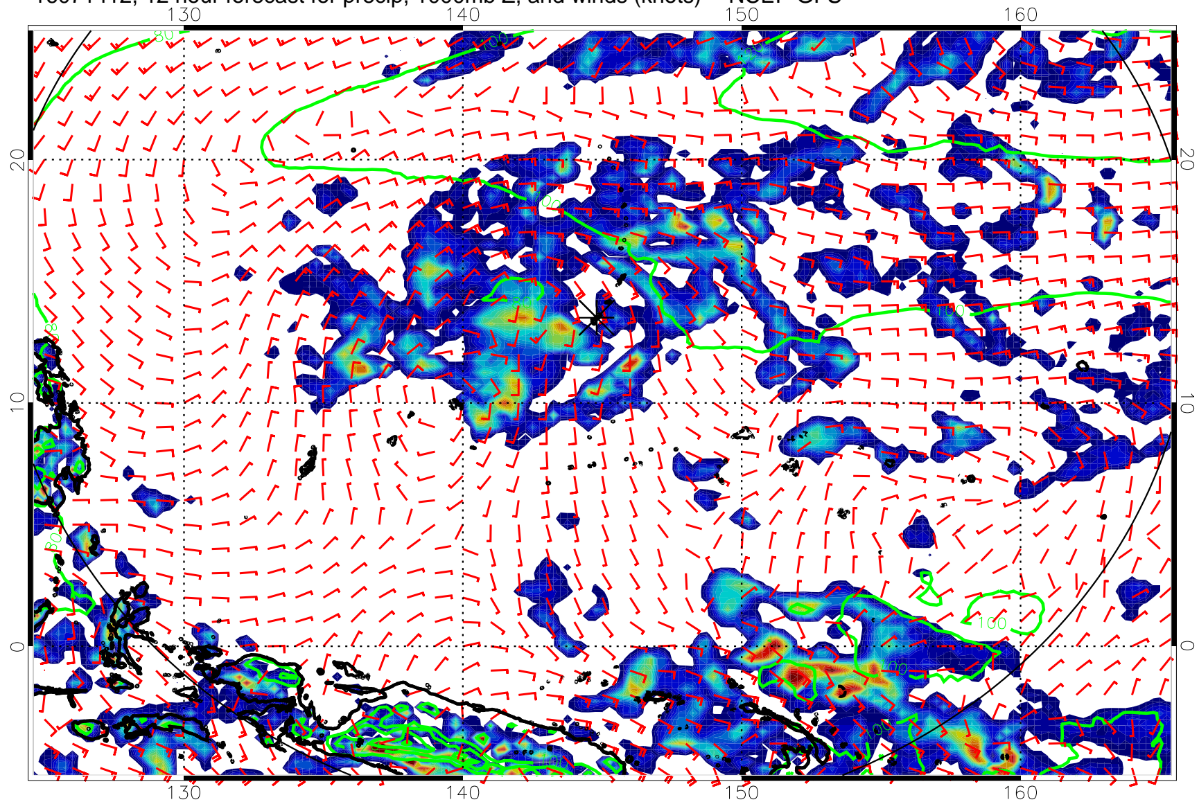
16071412, 12 hour forecast for precip, 1000mb Z, and winds (knots) -- NCEP GFS
