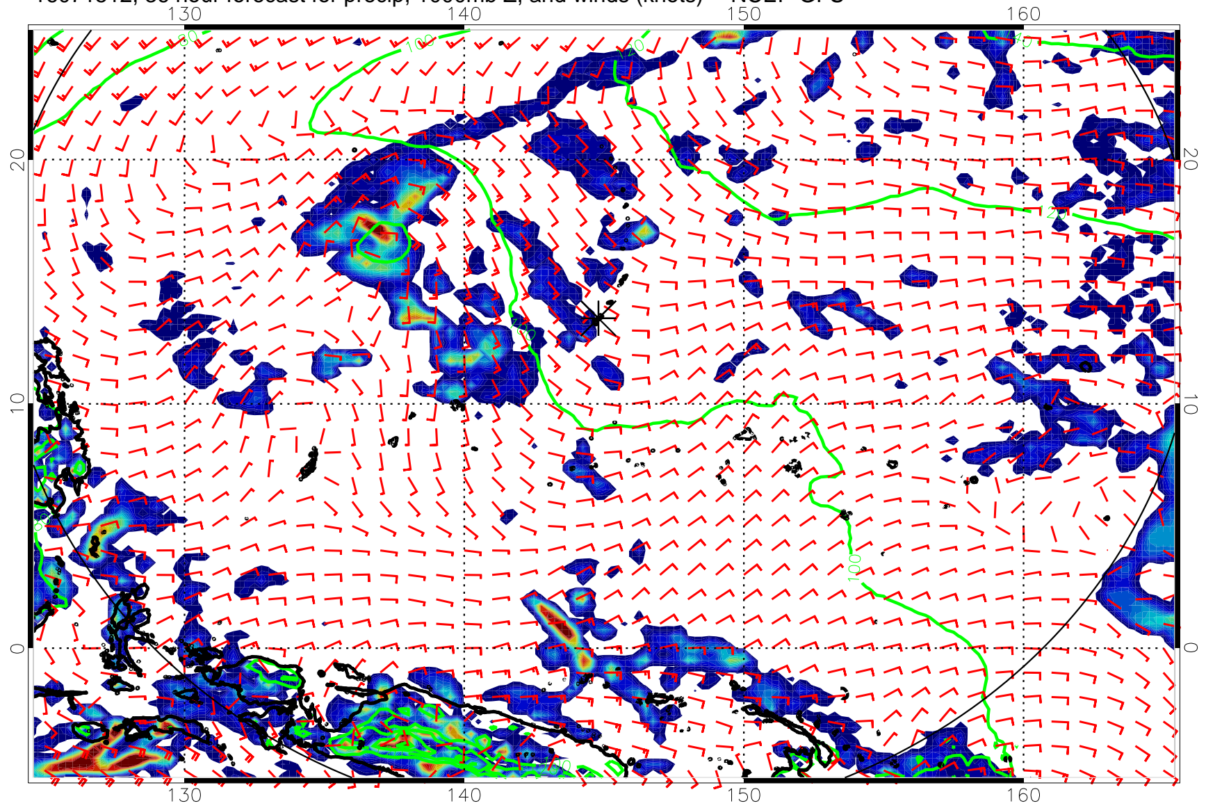
16071512, 36 hour forecast for precip, 1000mb Z, and winds (knots) -- NCEP GFS
