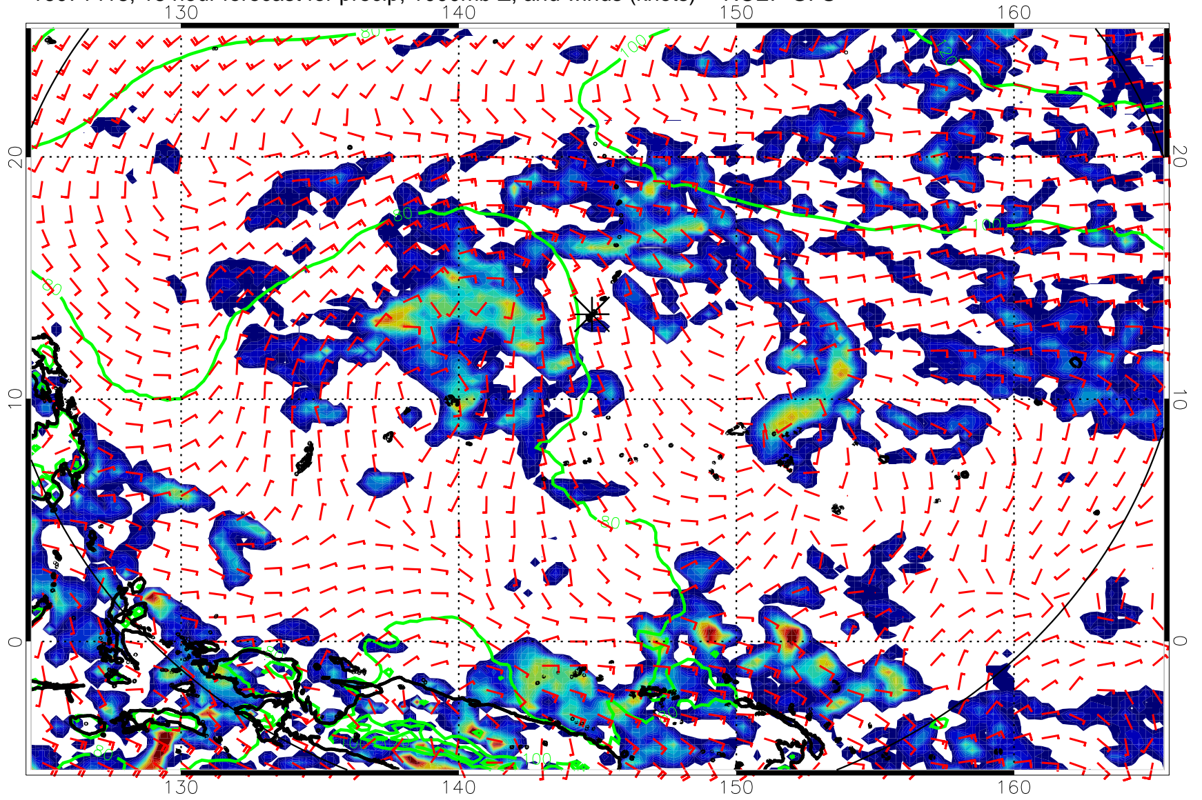
16071418, 18 hour forecast for precip, 1000mb Z, and winds (knots) -- NCEP GFS
