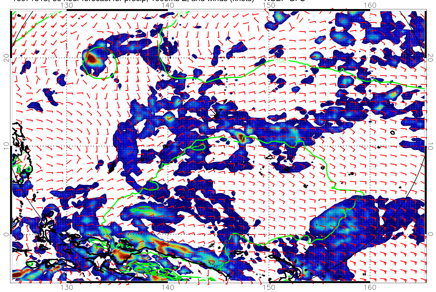
16071618, 66 hour forecast for precip, 1000mb Z, and winds (knots) -- NCEP GFS
