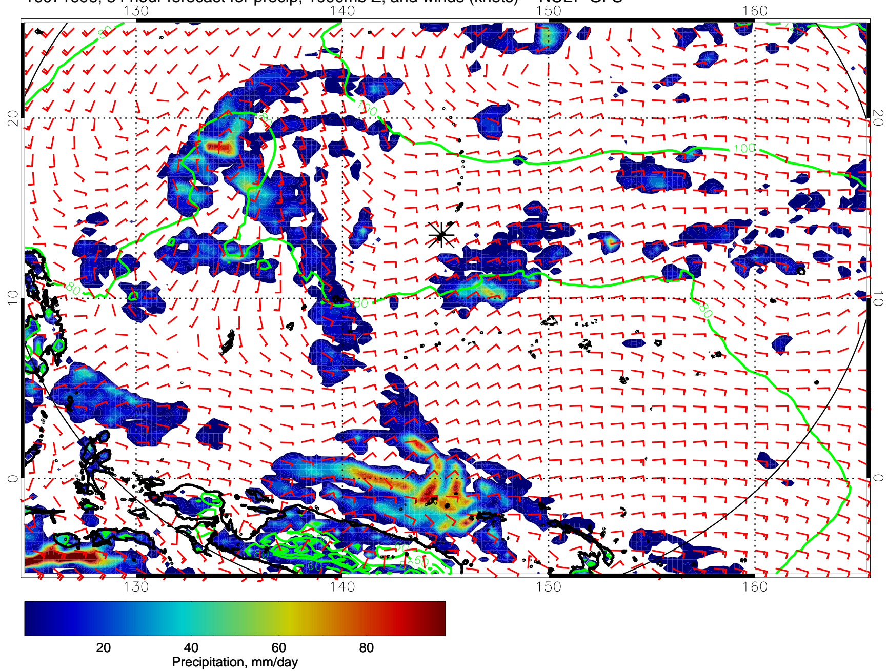
16071606, 54 hour forecast for precip, 1000mb Z, and winds (knots) -- NCEP GFS
