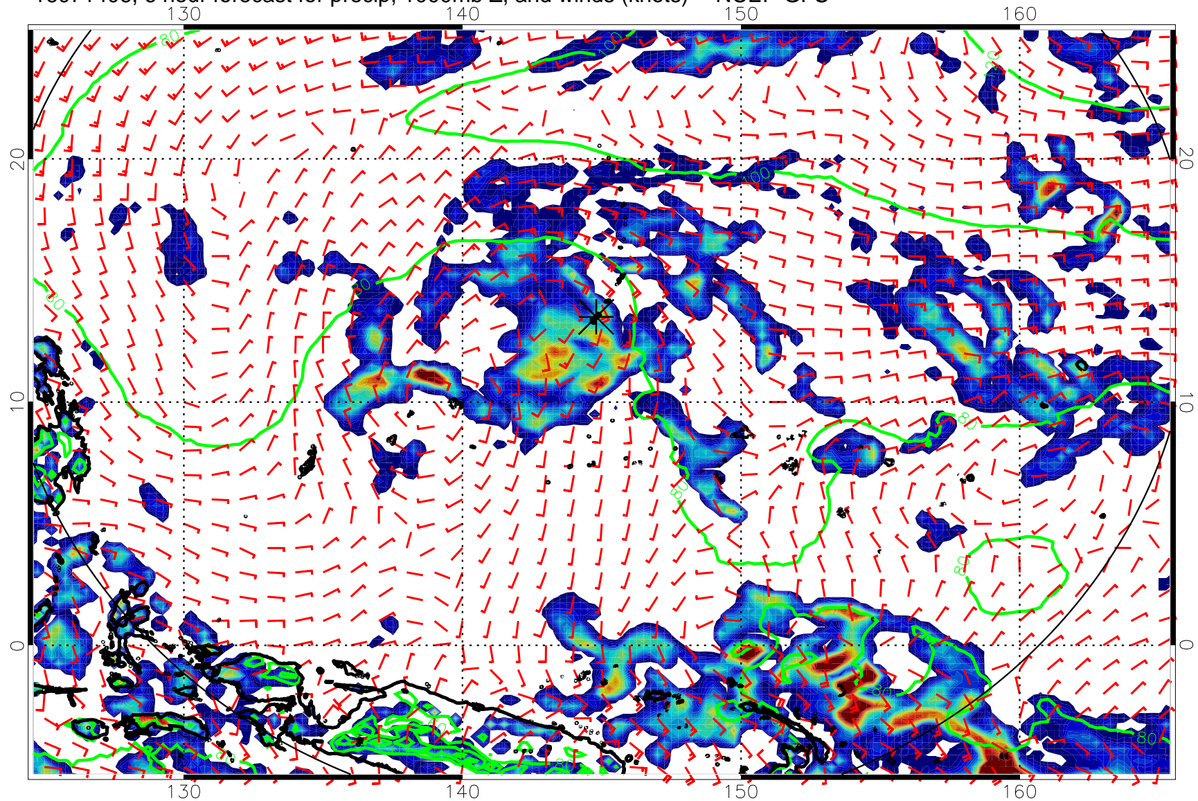
16071406, 6 hour forecast for precip, 1000mb Z, and winds (knots) -- NCEP GFS
