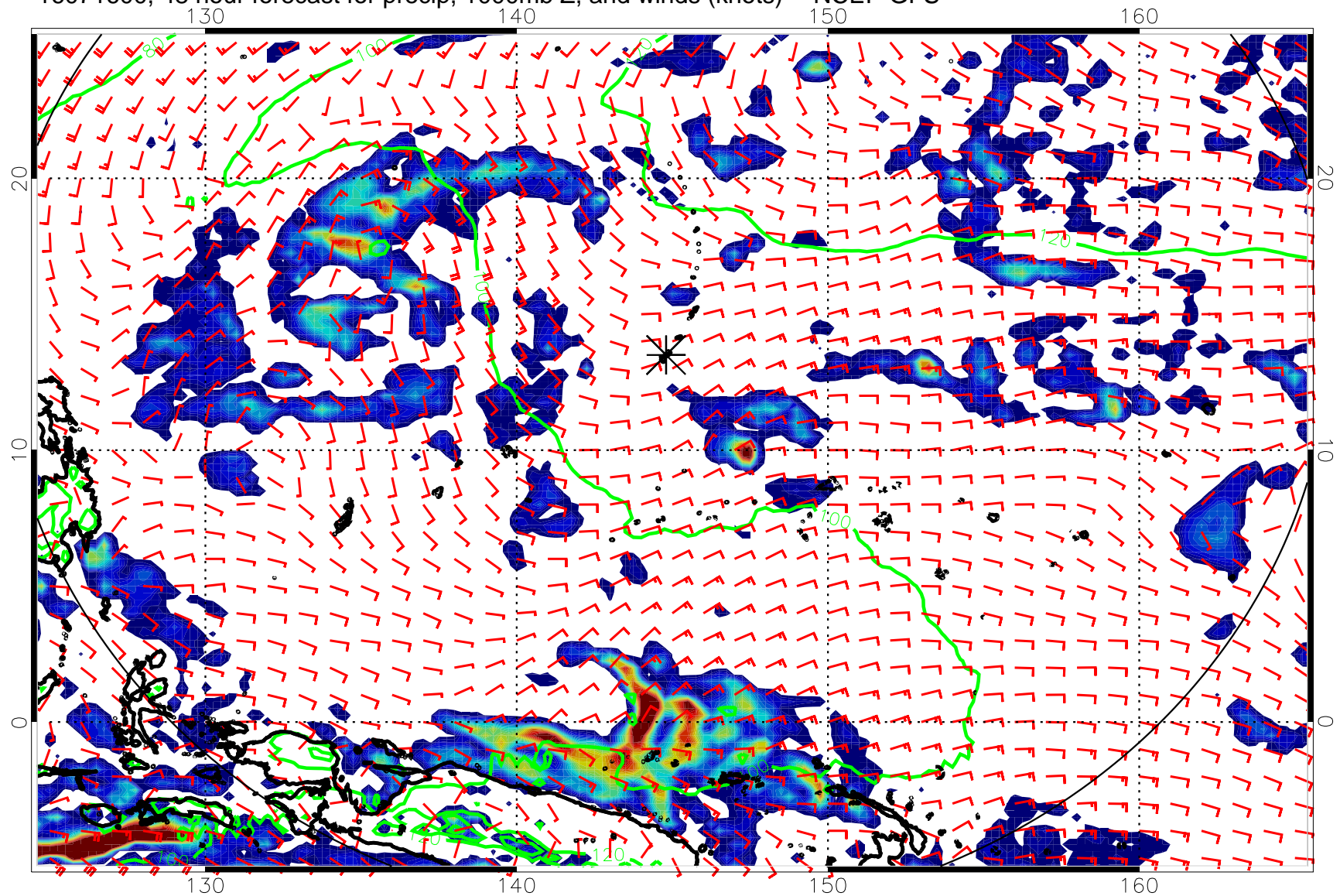
16071600, 48 hour forecast for precip, 1000mb Z, and winds (knots) -- NCEP GFS
