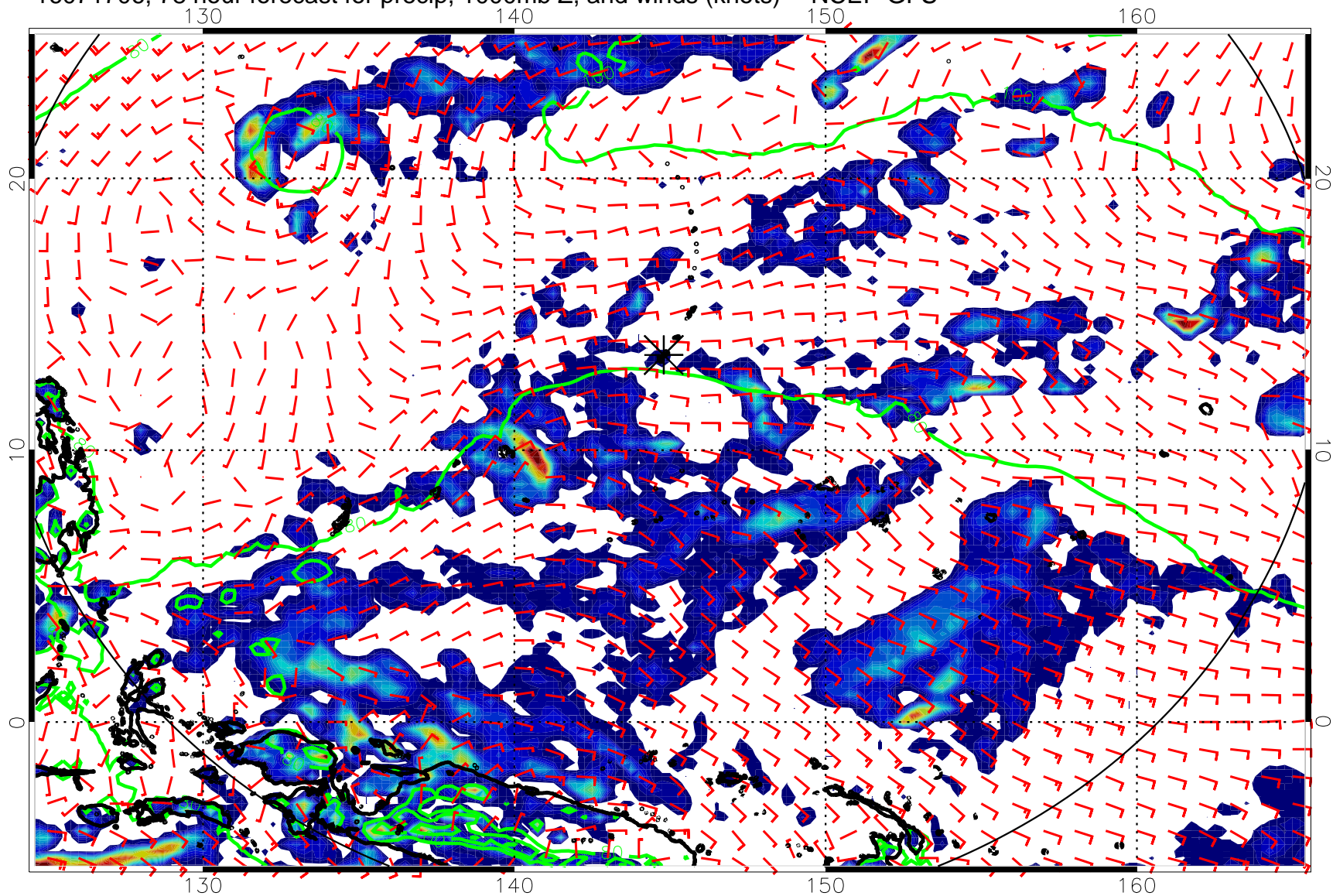
16071706, 78 hour forecast for precip, 1000mb Z, and winds (knots) -- NCEP GFS
