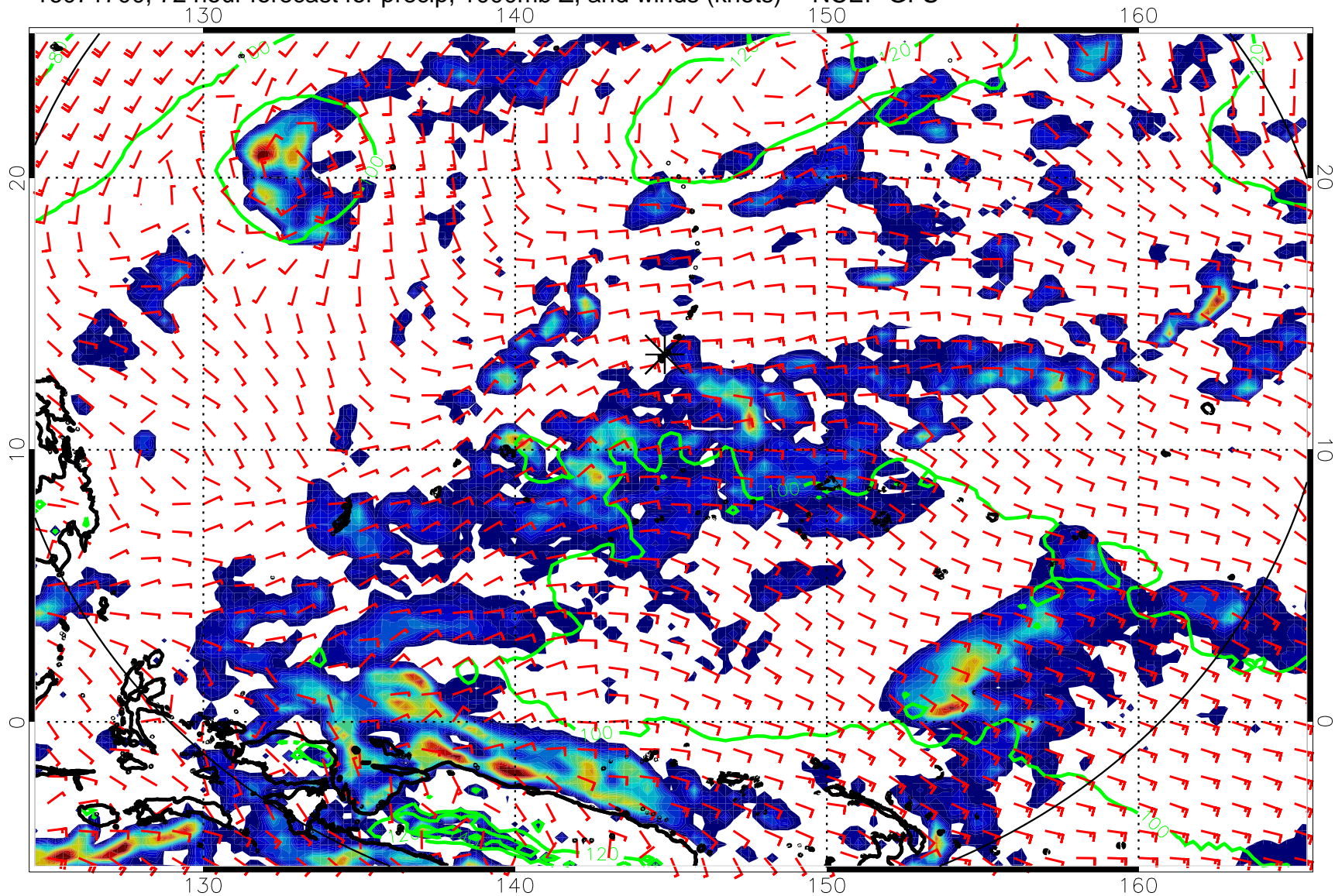
16071700, 72 hour forecast for precip, 1000mb Z, and winds (knots) -- NCEP GFS
