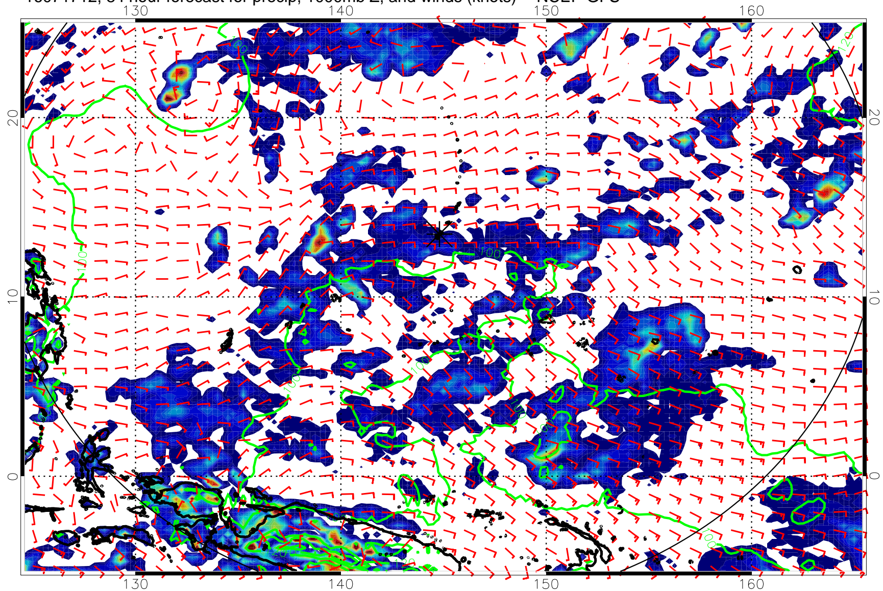
16071712, 84 hour forecast for precip, 1000mb Z, and winds (knots) -- NCEP GFS
