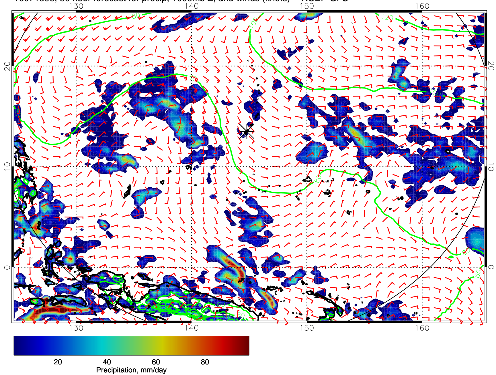
16071506, 30 hour forecast for precip, 1000mb Z, and winds (knots) -- NCEP GFS
