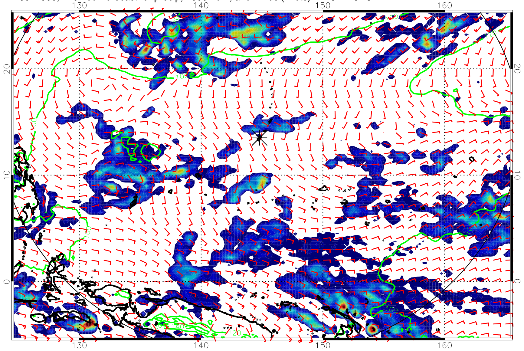
16071900, 120 hour forecast for precip, 1000mb Z, and winds (knots) -- NCEP GFS
