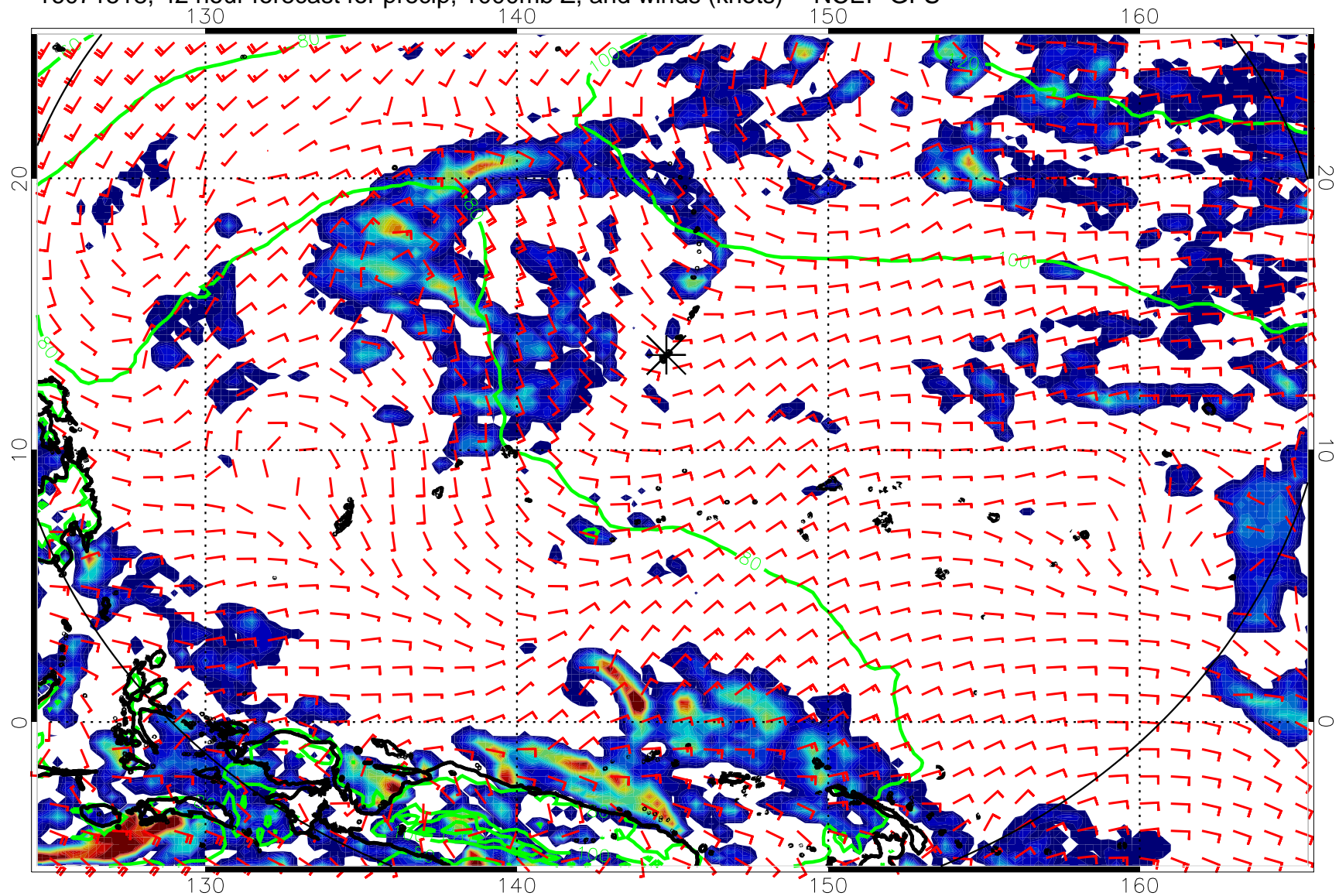
16071518, 42 hour forecast for precip, 1000mb Z, and winds (knots) -- NCEP GFS
