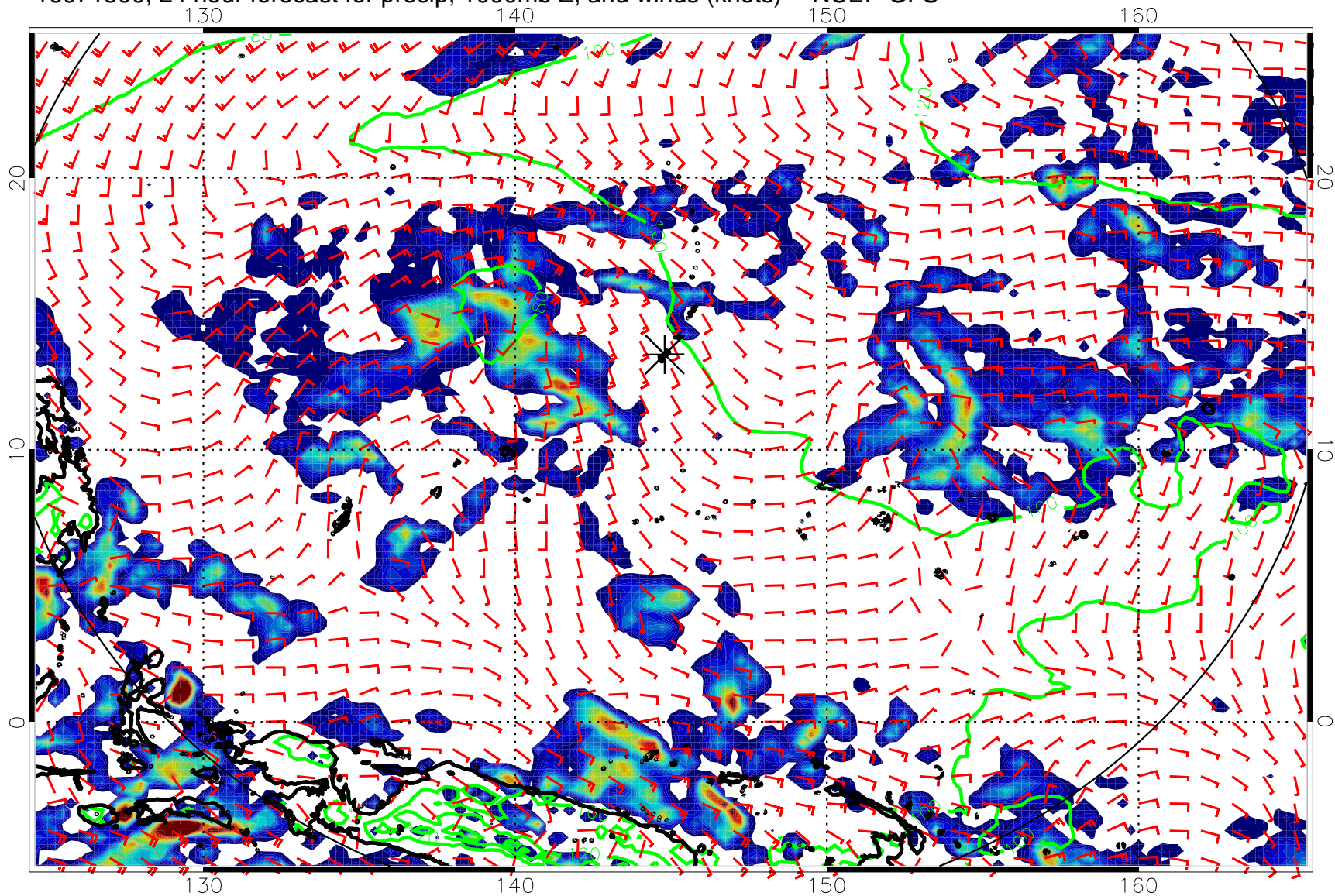
16071500, 24 hour forecast for precip, 1000mb Z, and winds (knots) -- NCEP GFS
