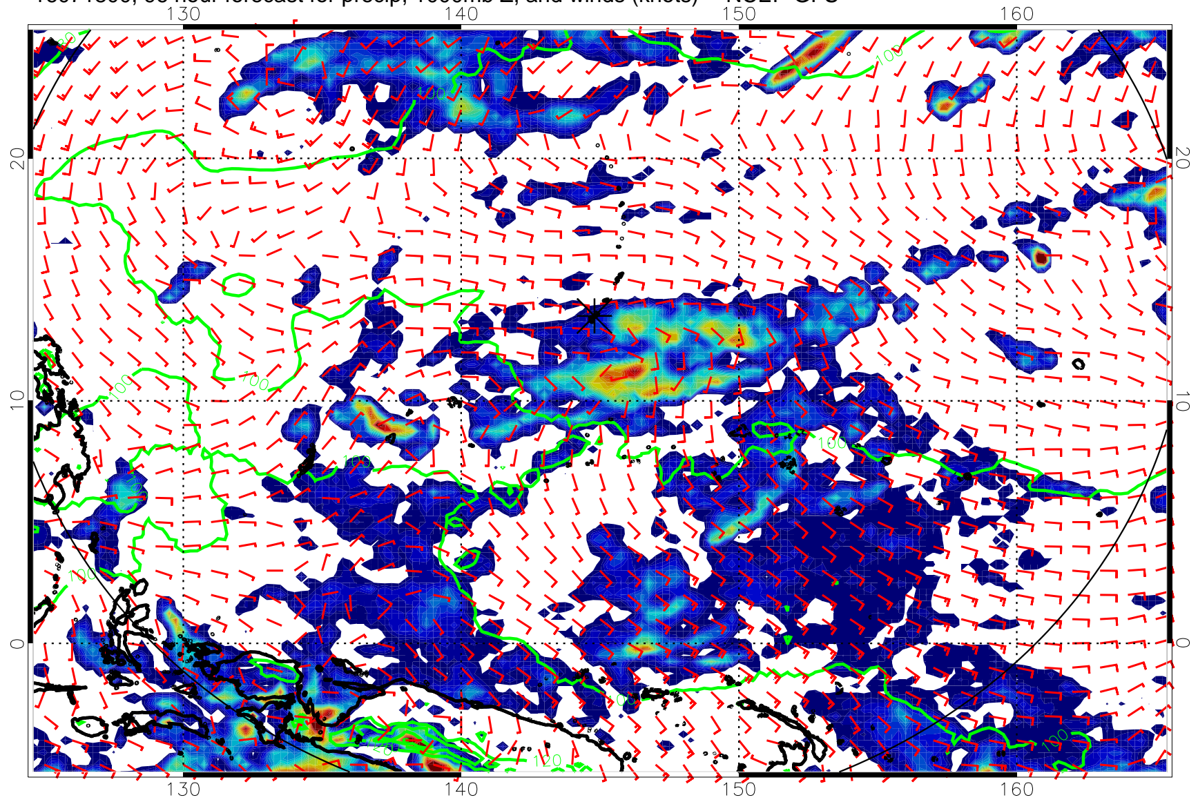
16071800, 96 hour forecast for precip, 1000mb Z, and winds (knots) -- NCEP GFS
