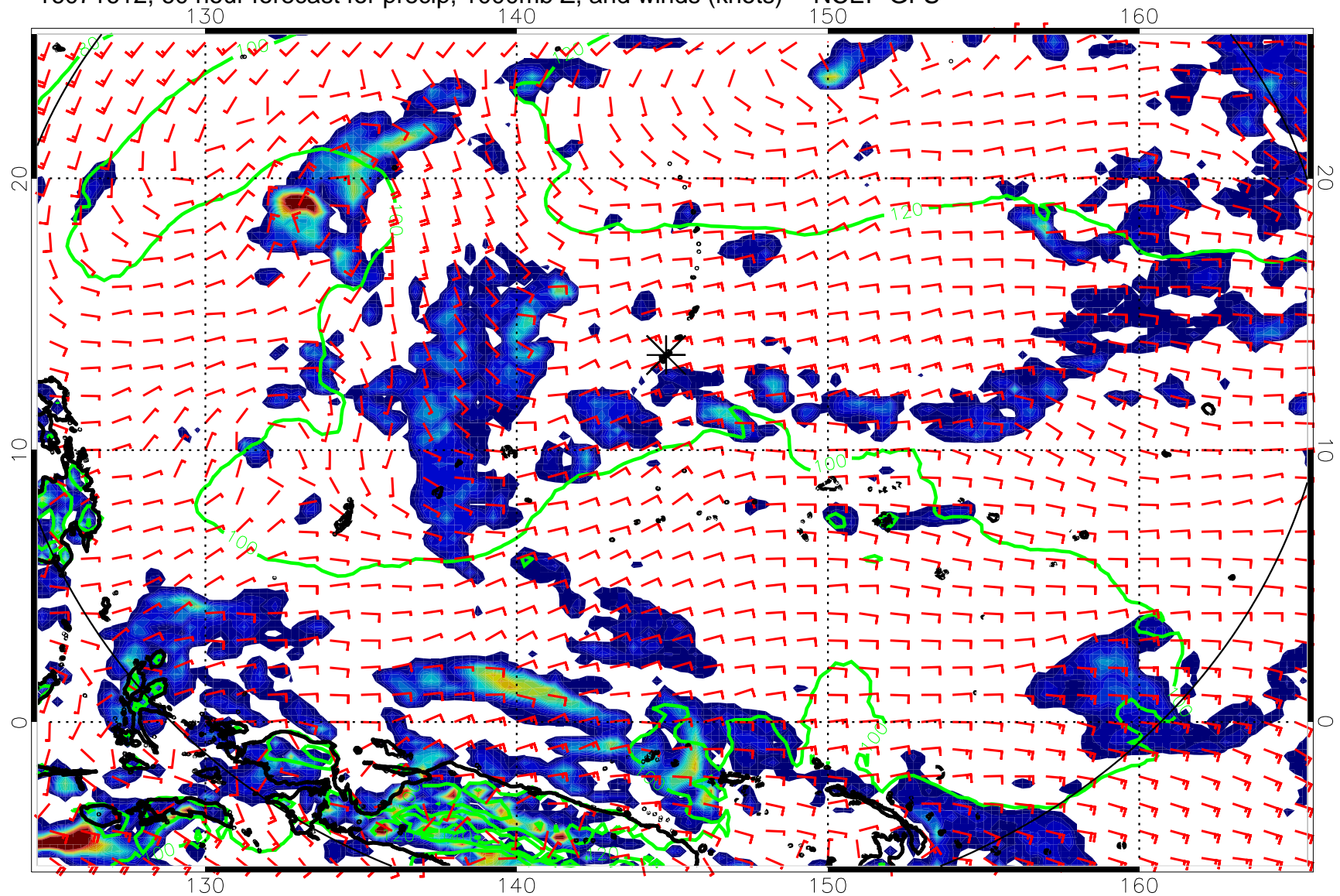
16071612, 60 hour forecast for precip, 1000mb Z, and winds (knots) -- NCEP GFS
