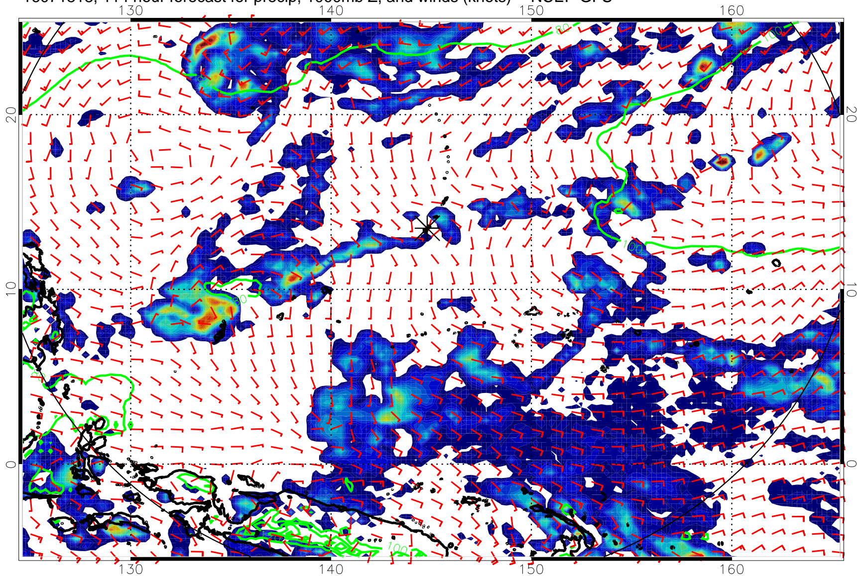
16071818, 114 hour forecast for precip, 1000mb Z, and winds (knots) -- NCEP GFS
