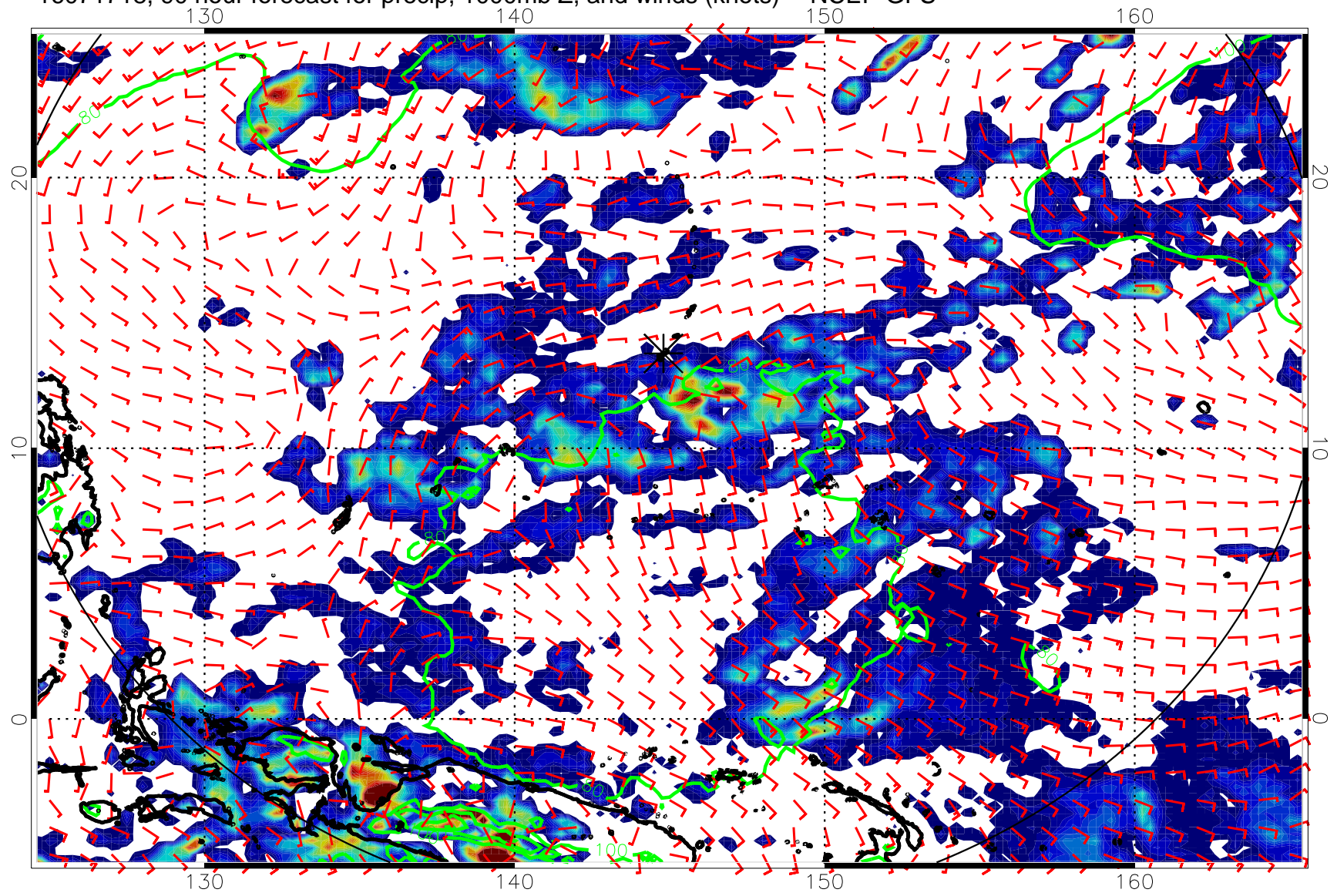
16071718, 90 hour forecast for precip, 1000mb Z, and winds (knots) -- NCEP GFS
