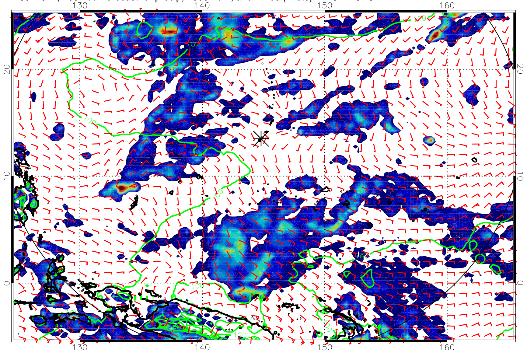
16071812, 108 hour forecast for precip, 1000mb Z, and winds (knots) -- NCEP GFS
