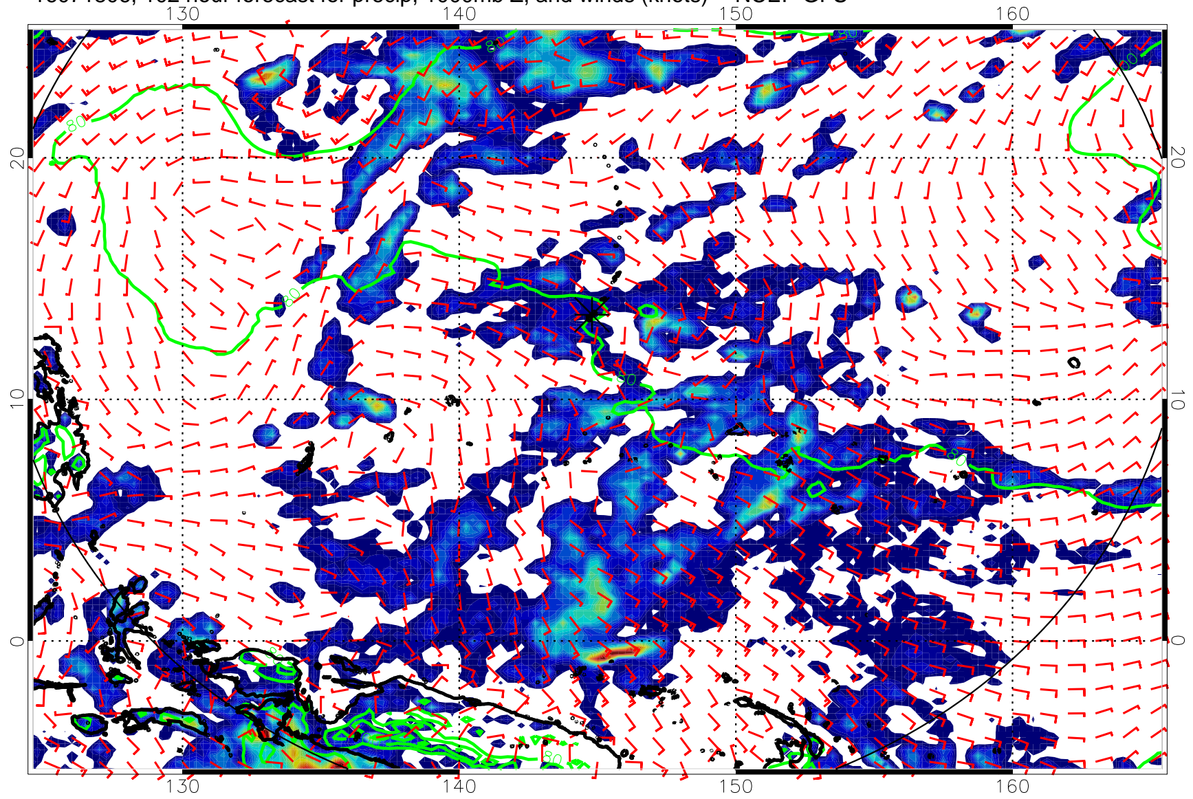
16071806, 102 hour forecast for precip, 1000mb Z, and winds (knots) -- NCEP GFS
