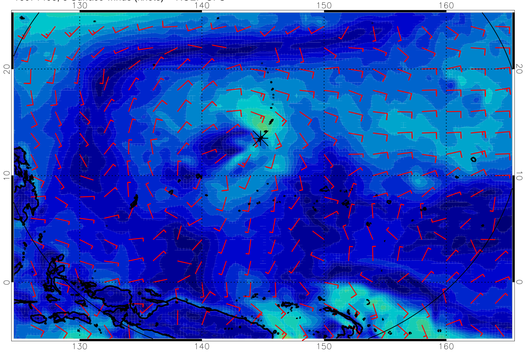
16071406, 6 Surface winds (knots) -- NCEP GFS
