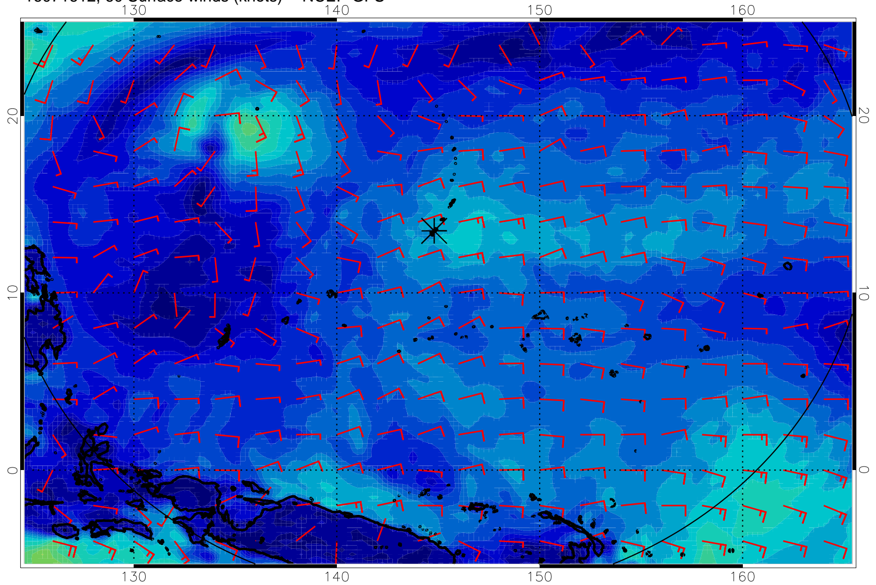
16071612, 60 Surface winds (knots) -- NCEP GFS
