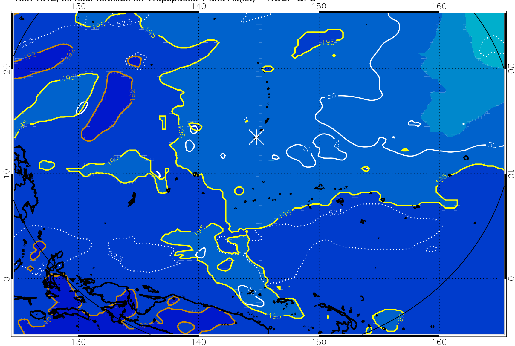
16071612, 60 hour forecast for Tropopause T and Alt(kft) -- NCEP GFS
