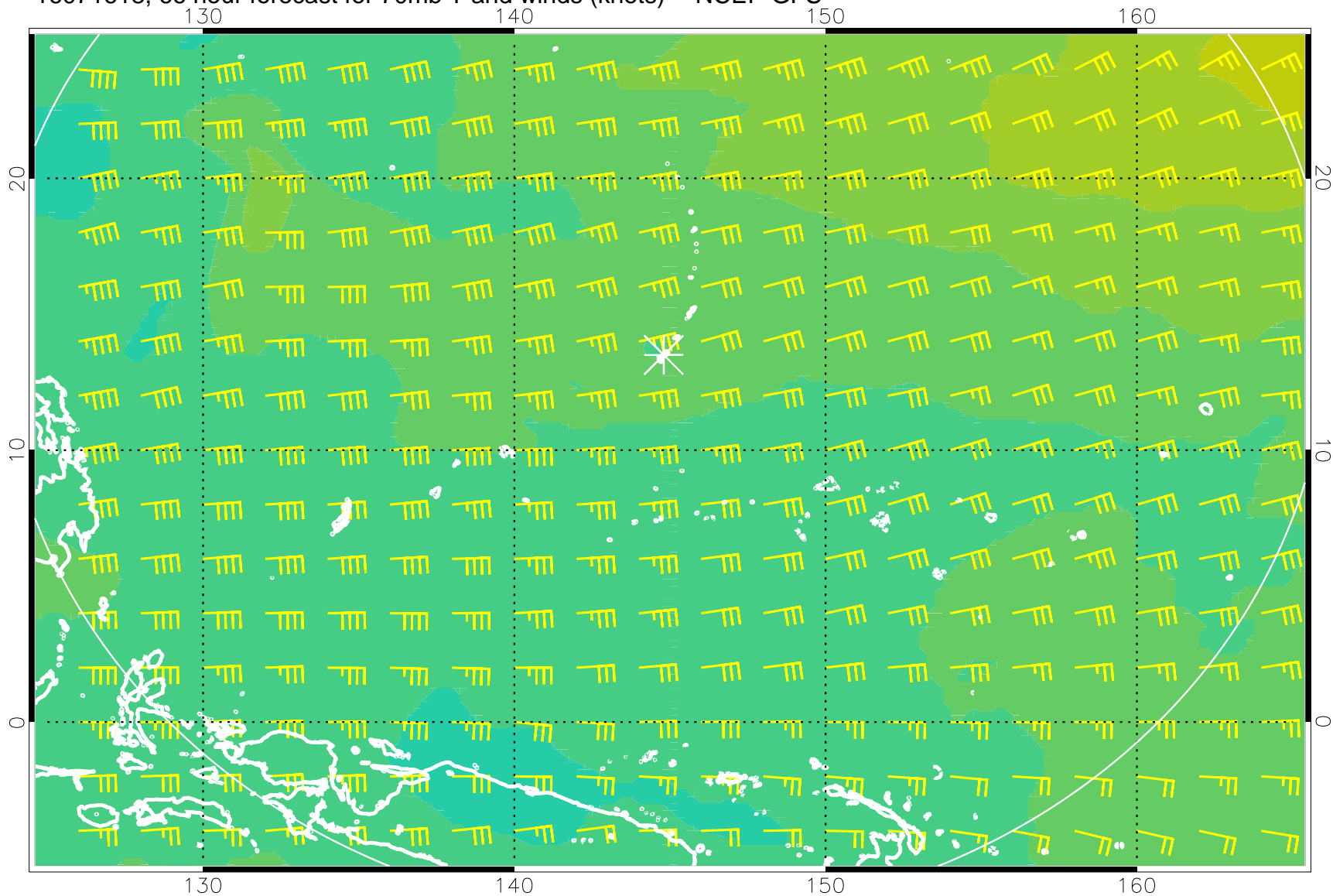
16071618, 66 hour forecast for 70mb T and winds (knots) -- NCEP GFS
