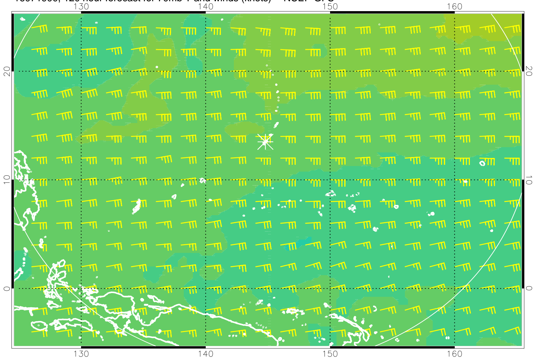
16071900, 120 hour forecast for 70mb T and winds (knots) -- NCEP GFS
