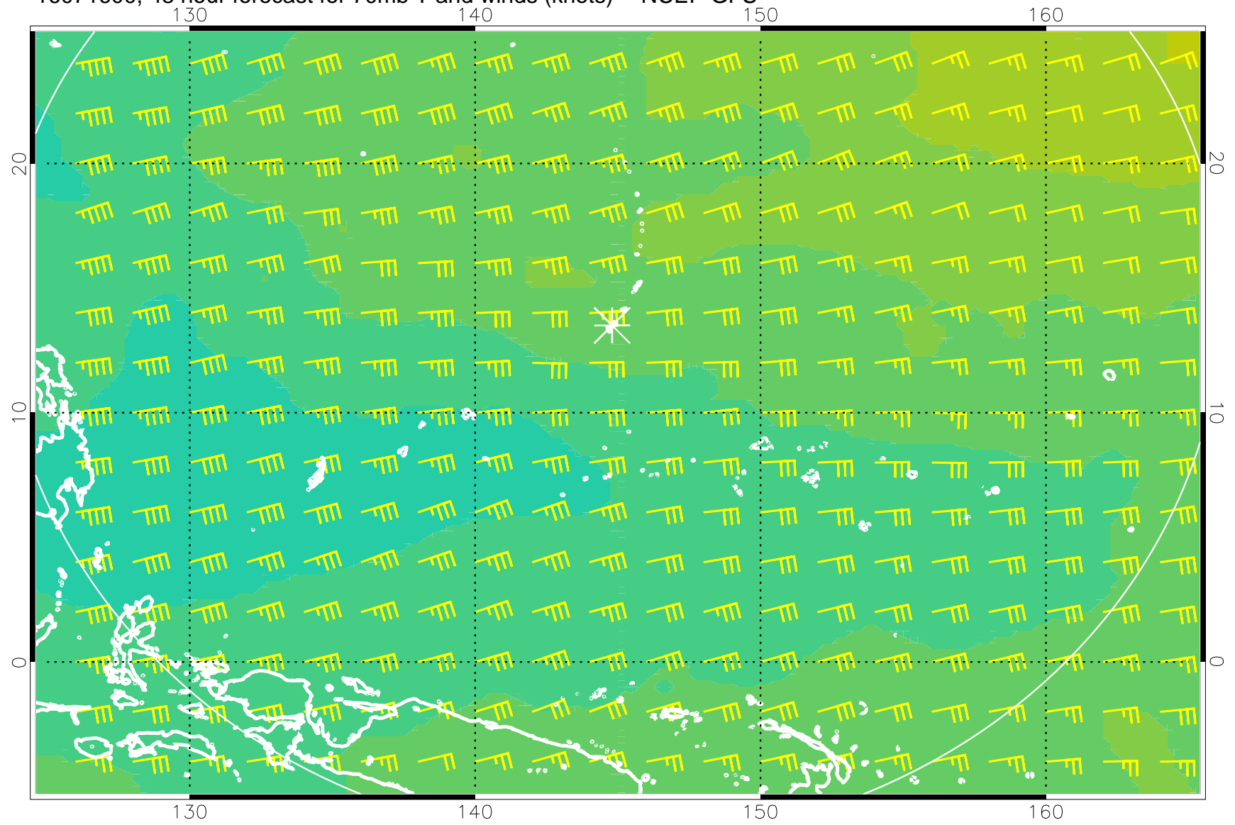
16071600, 48 hour forecast for 70mb T and winds (knots) -- NCEP GFS
