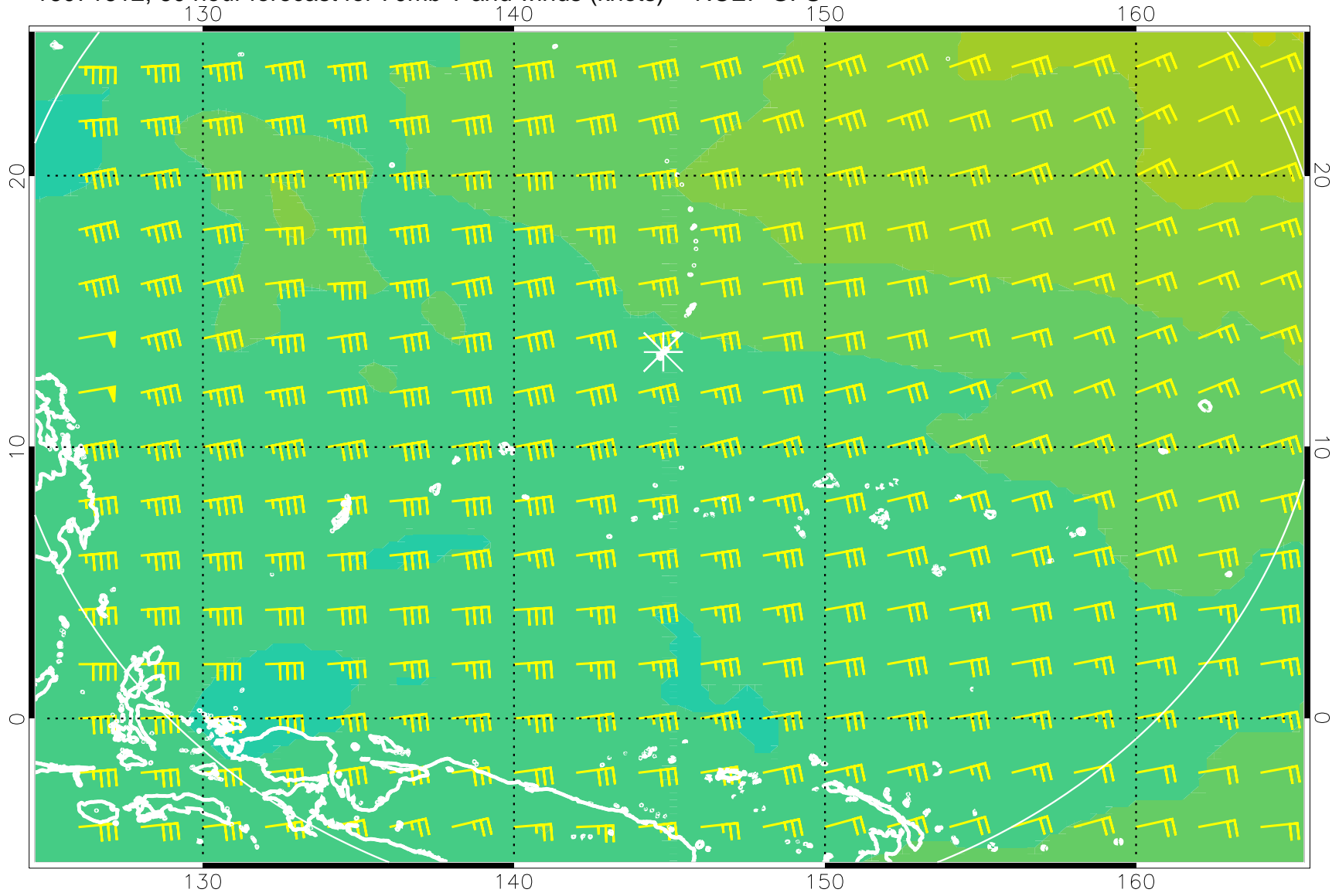
16071612, 60 hour forecast for 70mb T and winds (knots) -- NCEP GFS
