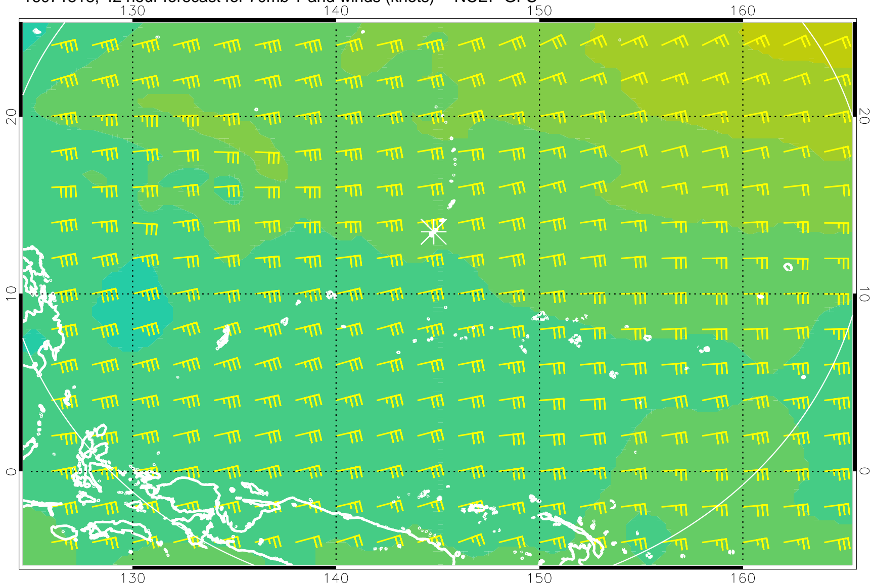
16071518, 42 hour forecast for 70mb T and winds (knots) -- NCEP GFS
