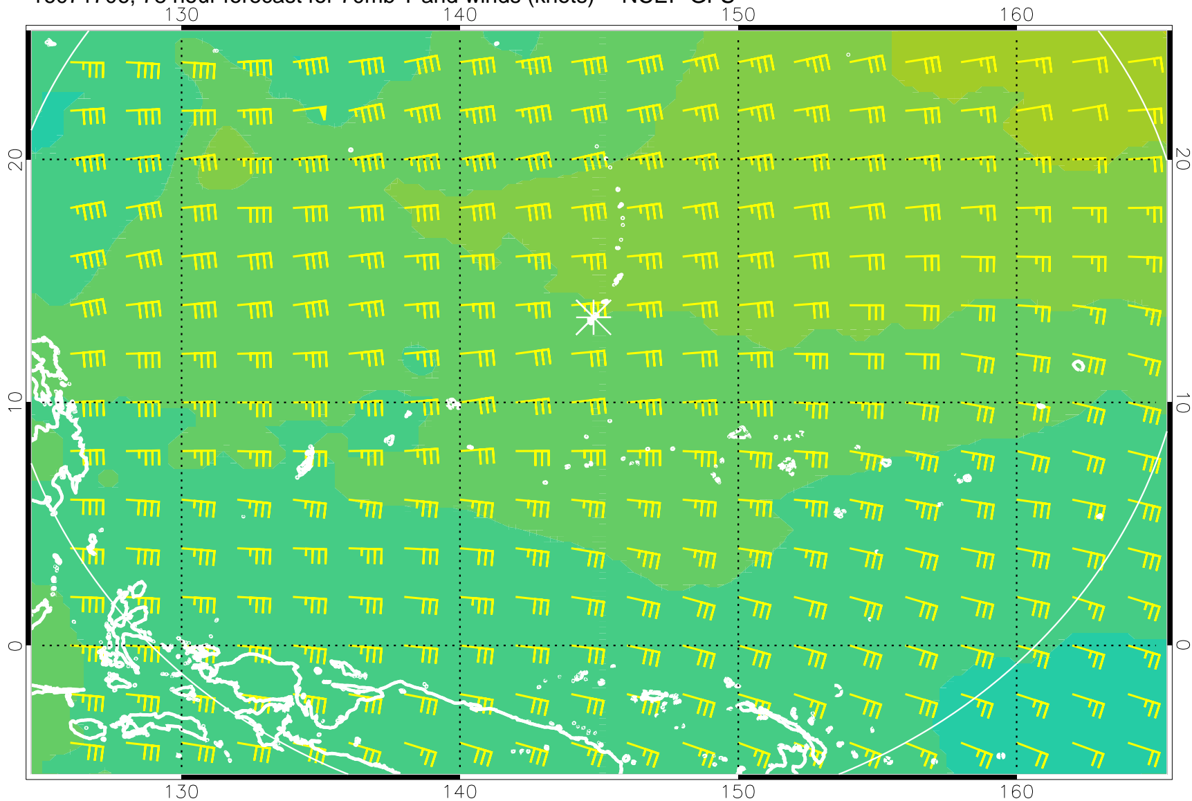
16071706, 78 hour forecast for 70mb T and winds (knots) -- NCEP GFS
