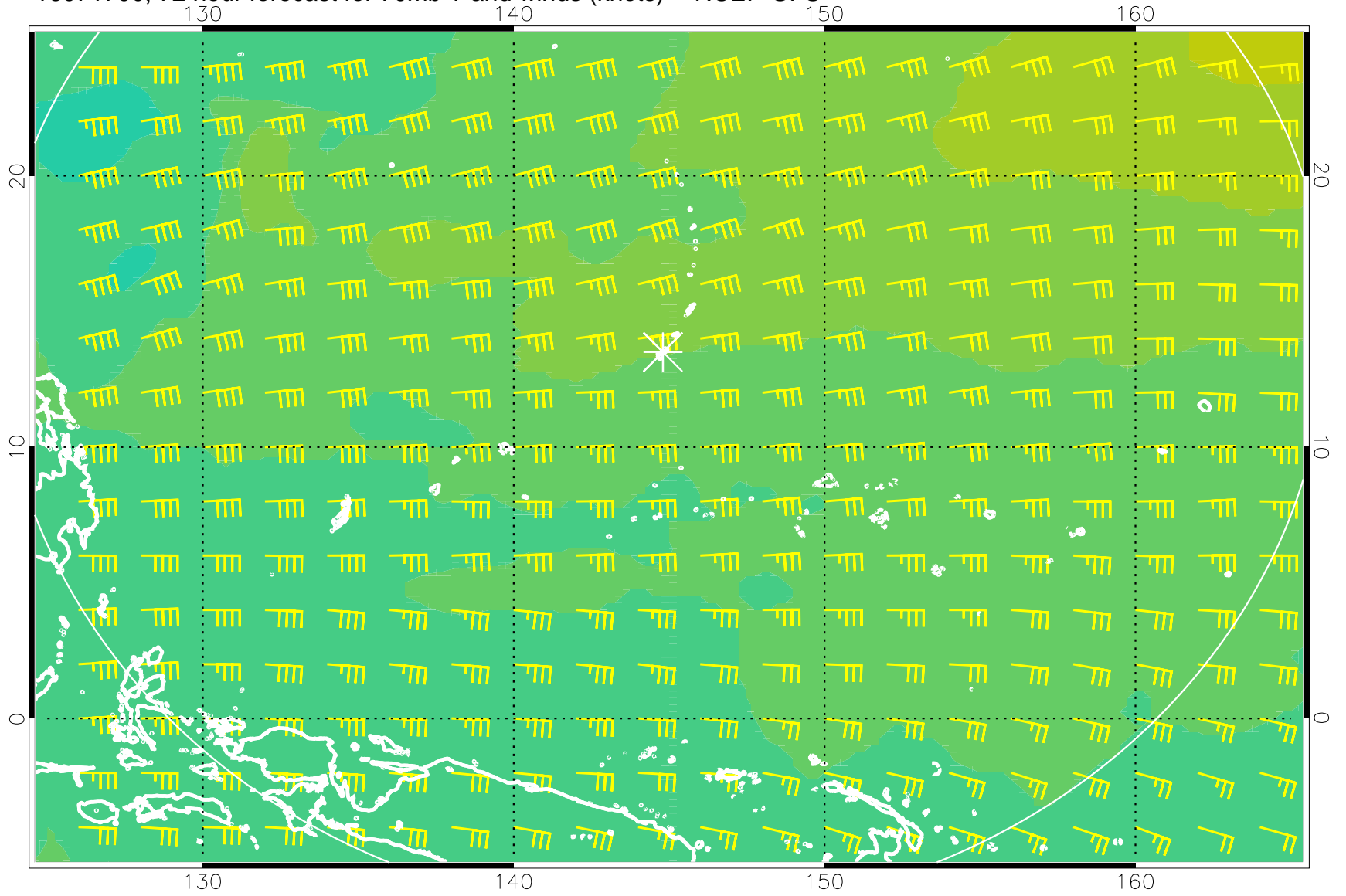
16071700, 72 hour forecast for 70mb T and winds (knots) -- NCEP GFS
