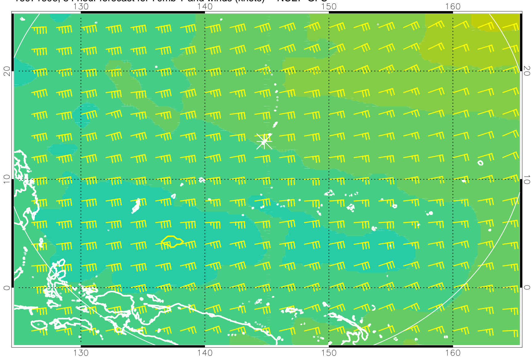
16071606, 54 hour forecast for 70mb T and winds (knots) -- NCEP GFS
