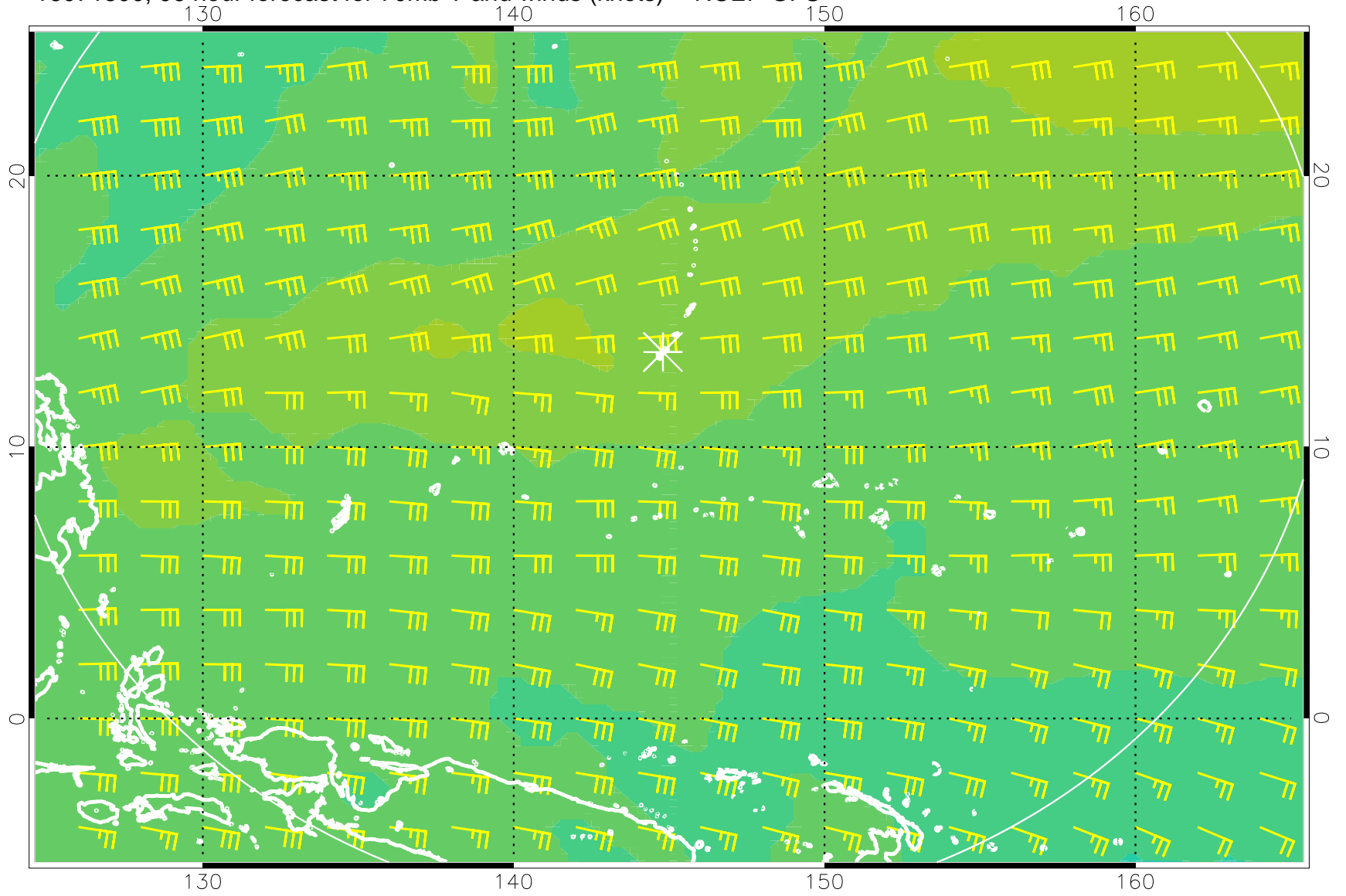
16071800, 96 hour forecast for 70mb T and winds (knots) -- NCEP GFS
