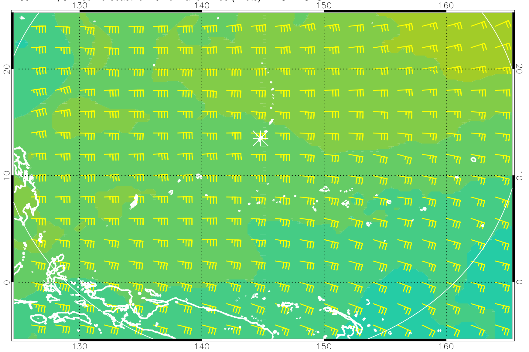
16071712, 84 hour forecast for 70mb T and winds (knots) -- NCEP GFS
