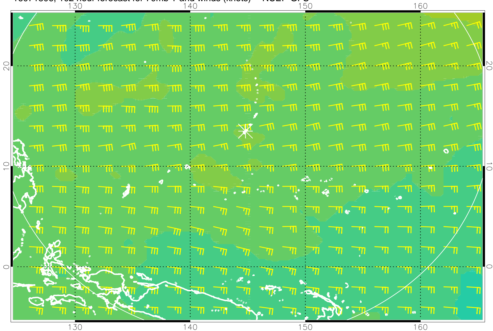
16071806, 102 hour forecast for 70mb T and winds (knots) -- NCEP GFS
