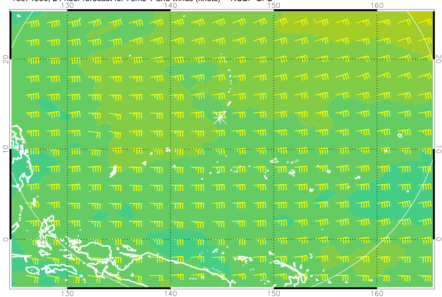
16071500, 24 hour forecast for 70mb T and winds (knots) -- NCEP GFS
