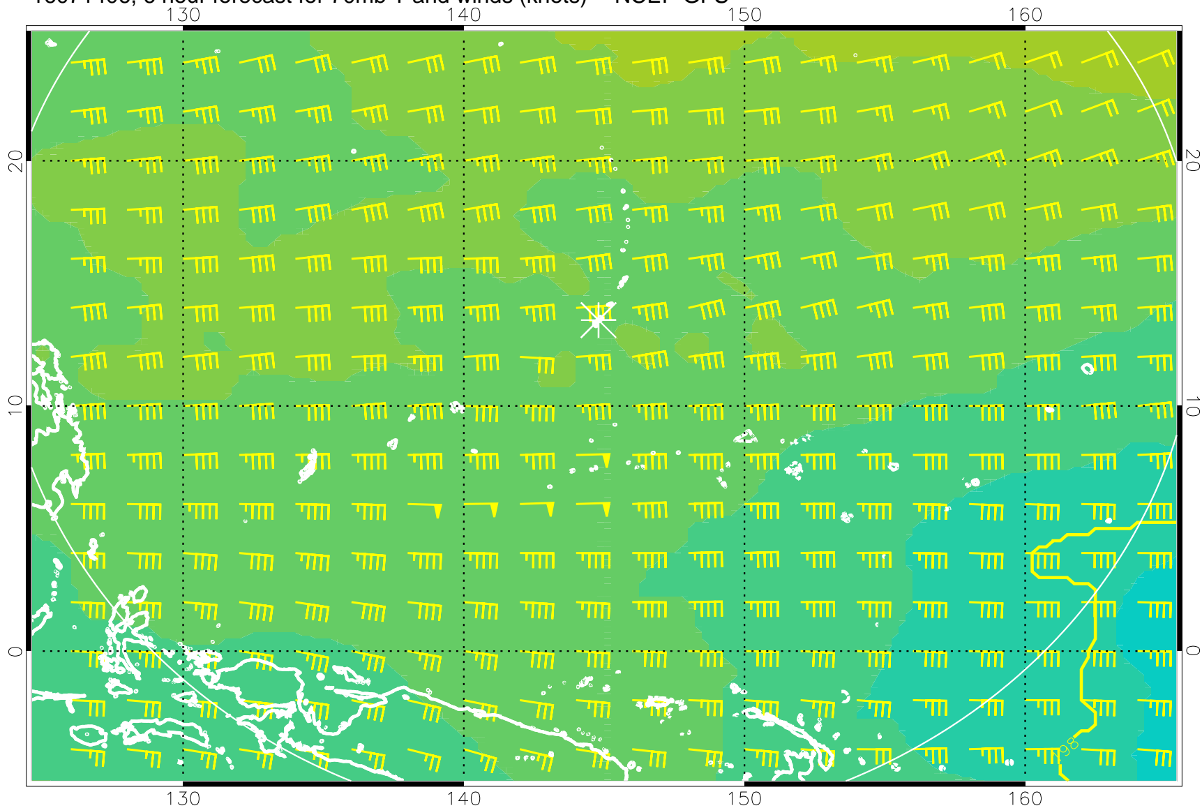
16071406, 6 hour forecast for 70mb T and winds (knots) -- NCEP GFS
