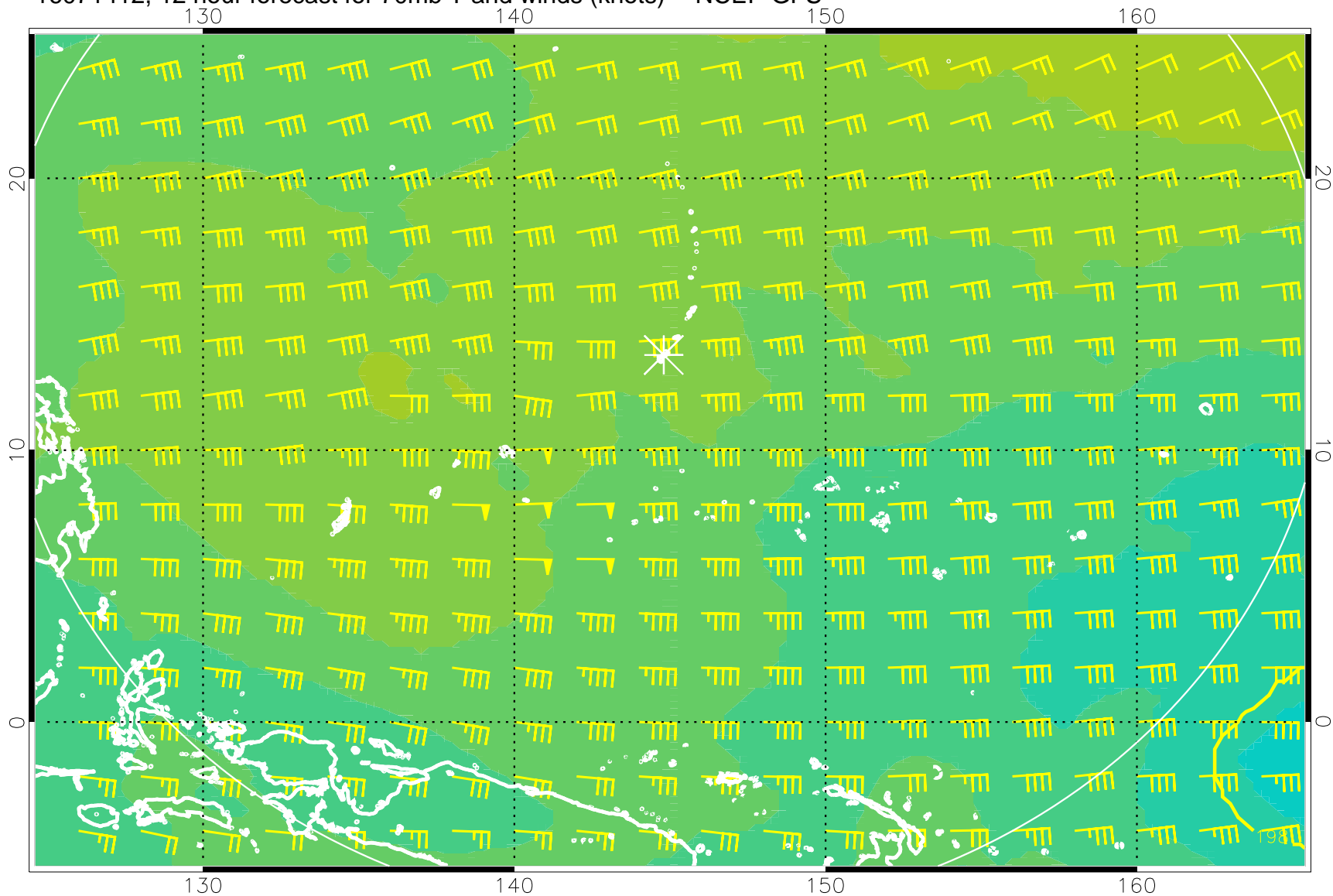
16071412, 12 hour forecast for 70mb T and winds (knots) -- NCEP GFS
