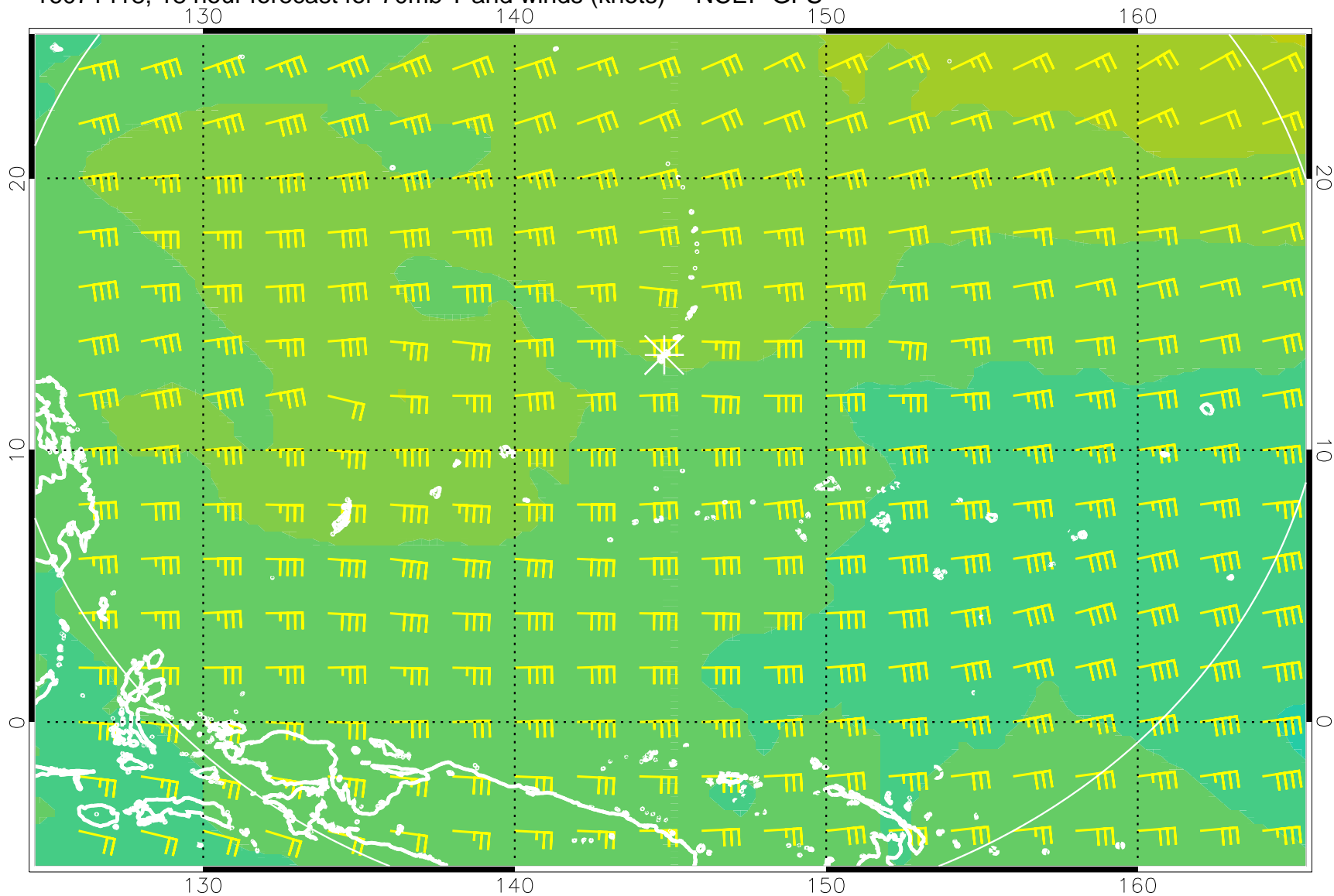
16071418, 18 hour forecast for 70mb T and winds (knots) -- NCEP GFS
