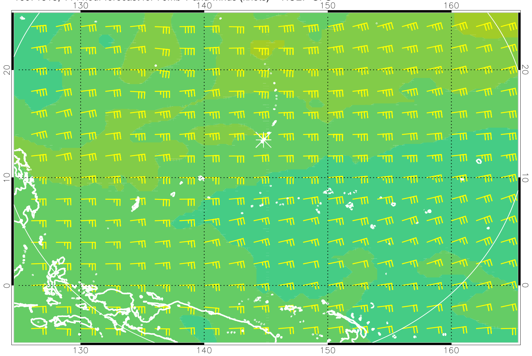
16071818, 114 hour forecast for 70mb T and winds (knots) -- NCEP GFS
