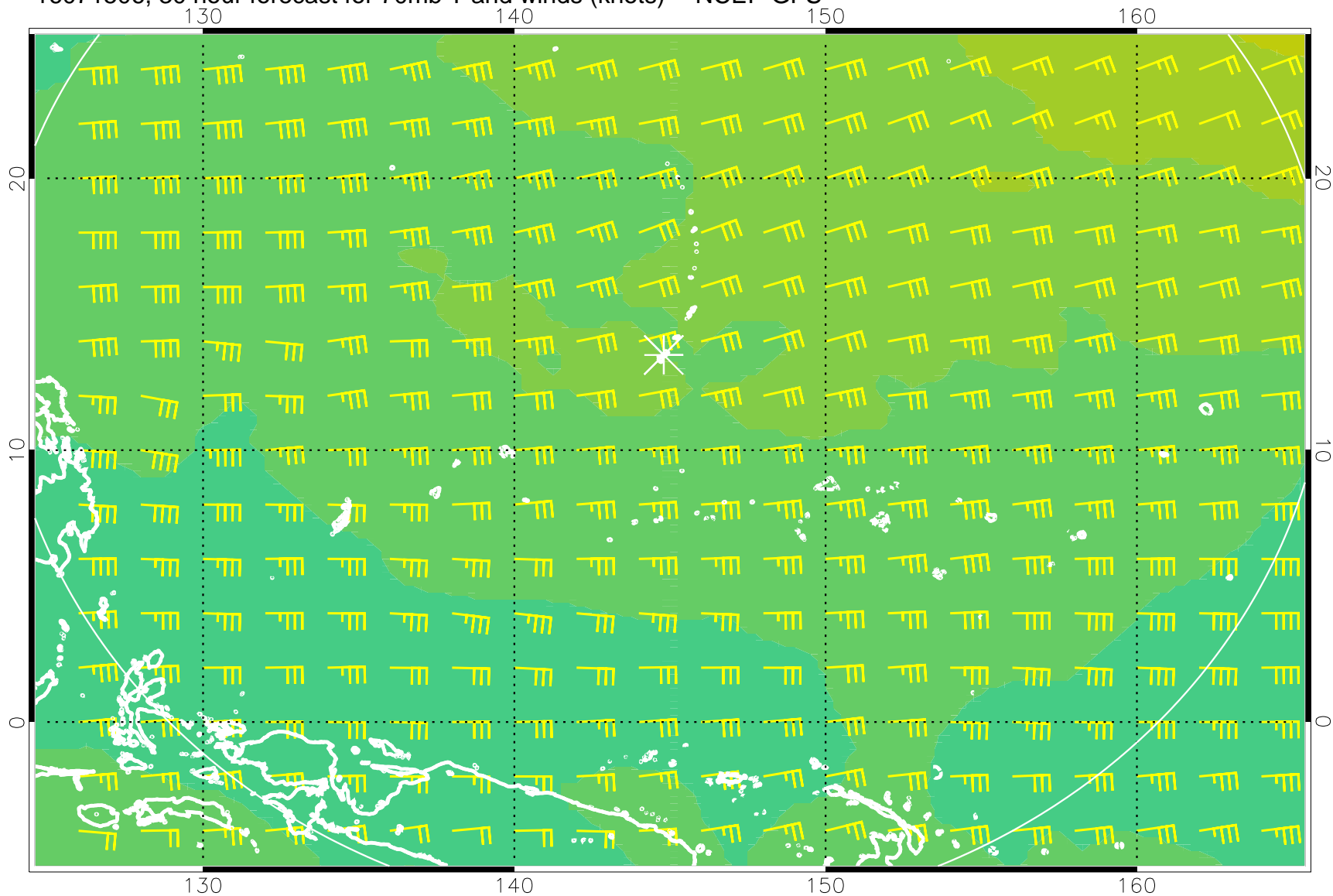
16071506, 30 hour forecast for 70mb T and winds (knots) -- NCEP GFS
