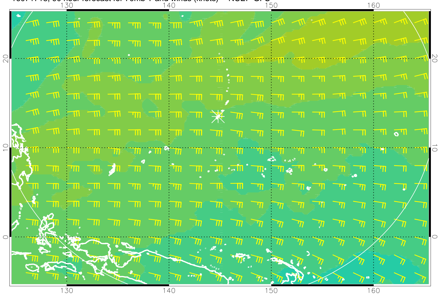
16071718, 90 hour forecast for 70mb T and winds (knots) -- NCEP GFS
