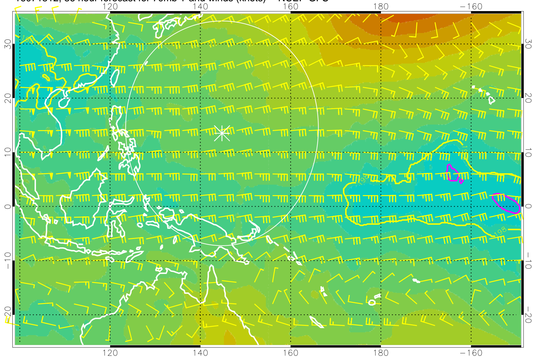
16071512, 36 hour forecast for 70mb T and winds (knots) -- NCEP GFS
