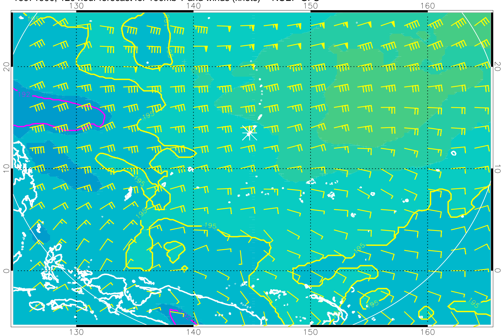
16071900, 120 hour forecast for 100mb T and winds (knots) -- NCEP GFS
