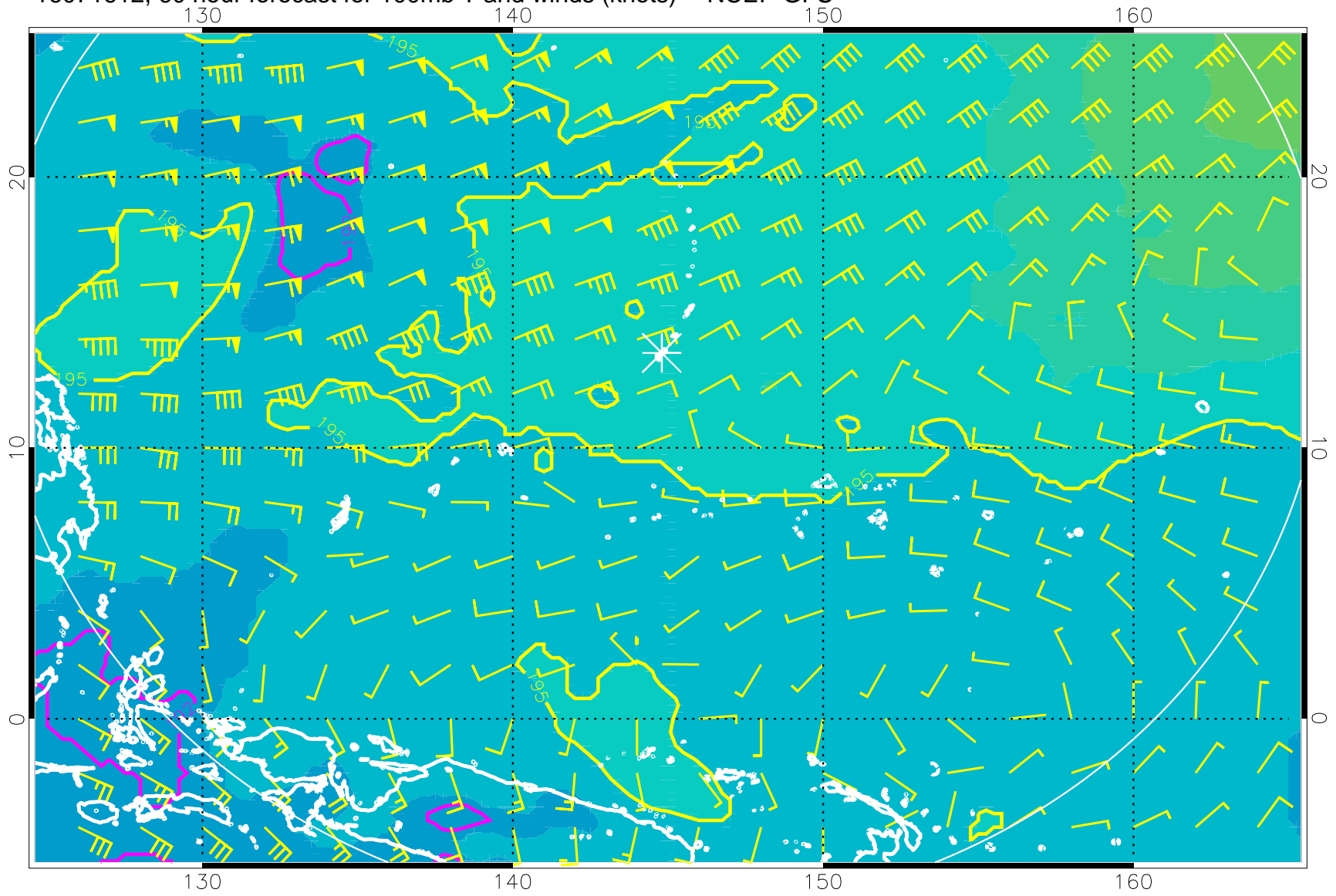
16071612, 60 hour forecast for 100mb T and winds (knots) -- NCEP GFS
