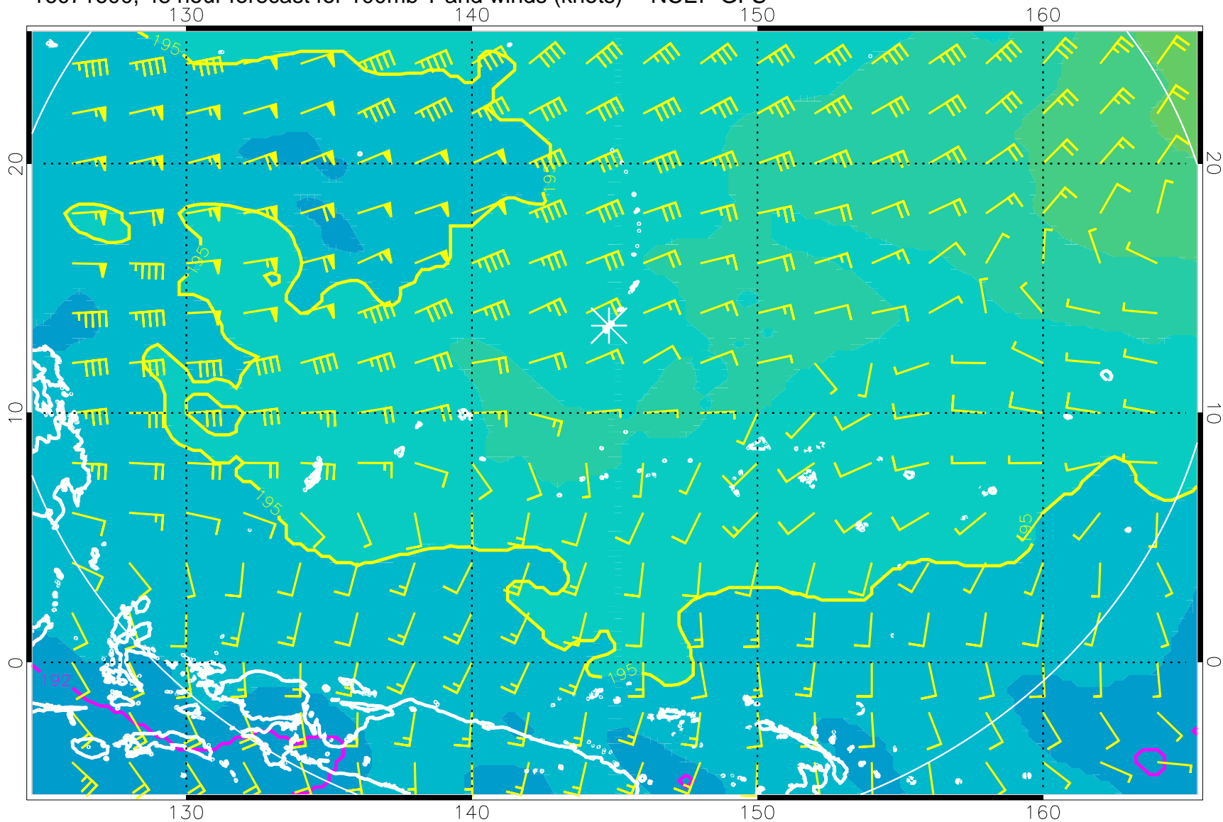
16071600, 48 hour forecast for 100mb T and winds (knots) -- NCEP GFS
