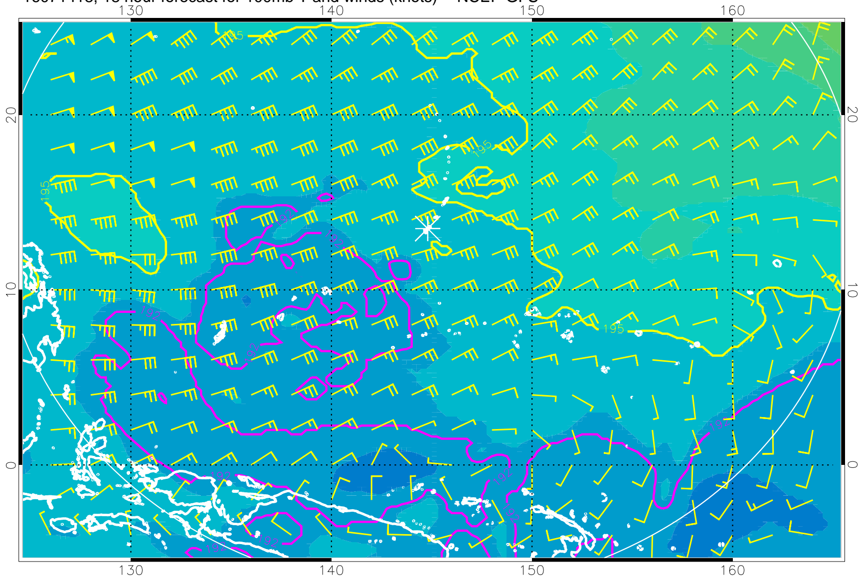
16071418, 18 hour forecast for 100mb T and winds (knots) -- NCEP GFS
