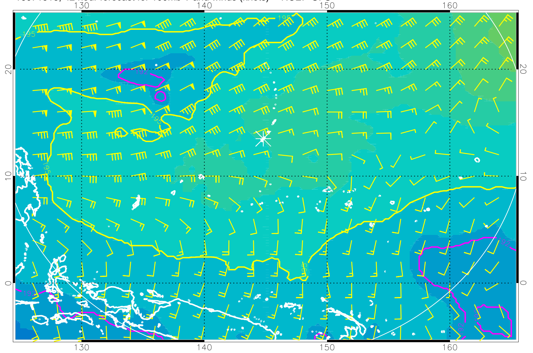
16071518, 42 hour forecast for 100mb T and winds (knots) -- NCEP GFS
