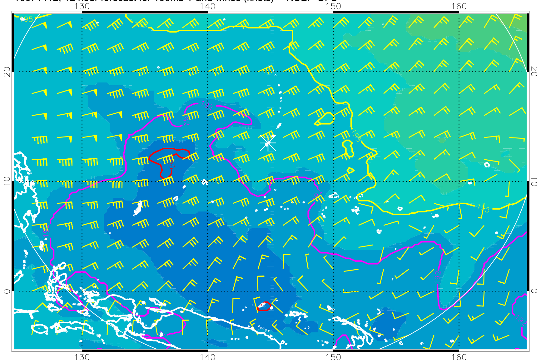
16071412, 12 hour forecast for 100mb T and winds (knots) -- NCEP GFS
