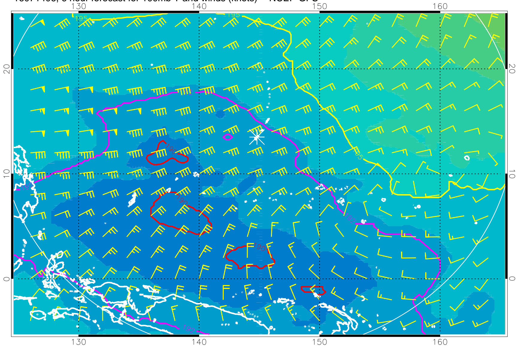
16071406, 6 hour forecast for 100mb T and winds (knots) -- NCEP GFS
