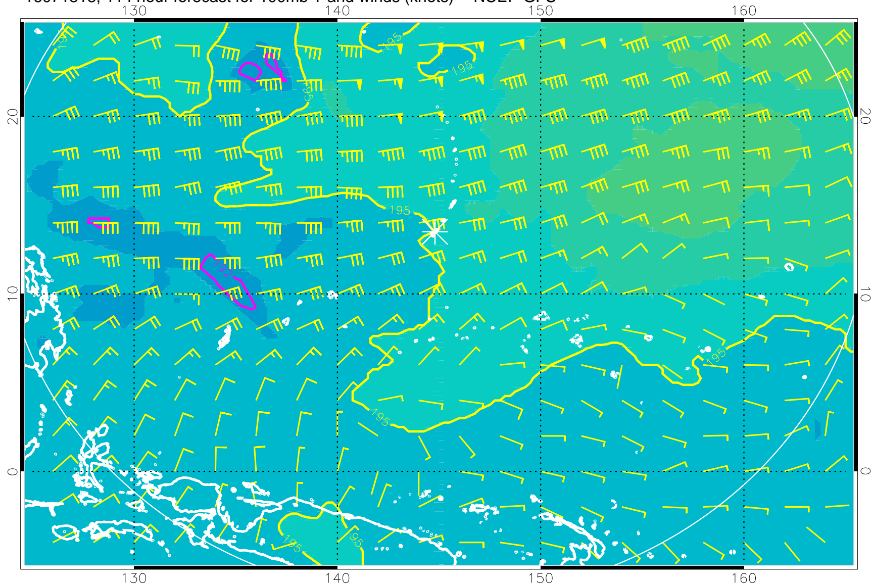
16071818, 114 hour forecast for 100mb T and winds (knots) -- NCEP GFS
