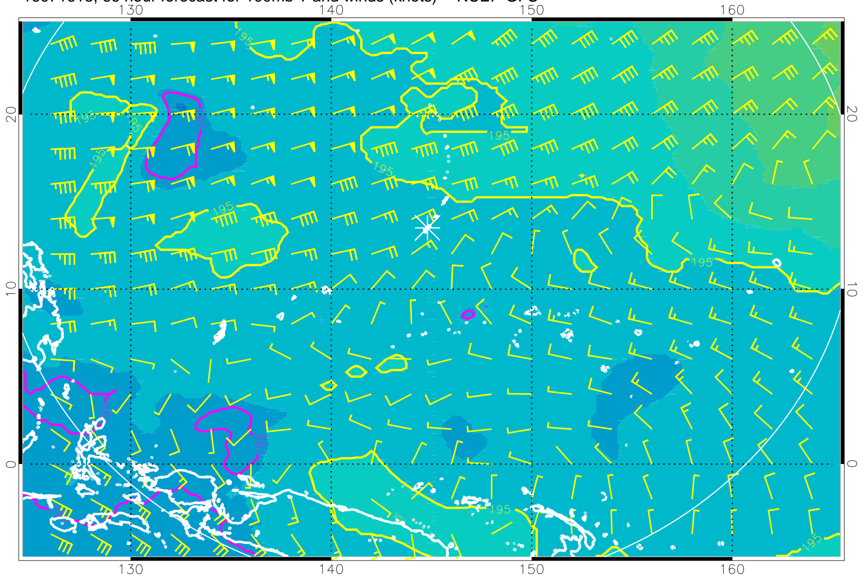
16071618, 66 hour forecast for 100mb T and winds (knots) -- NCEP GFS
