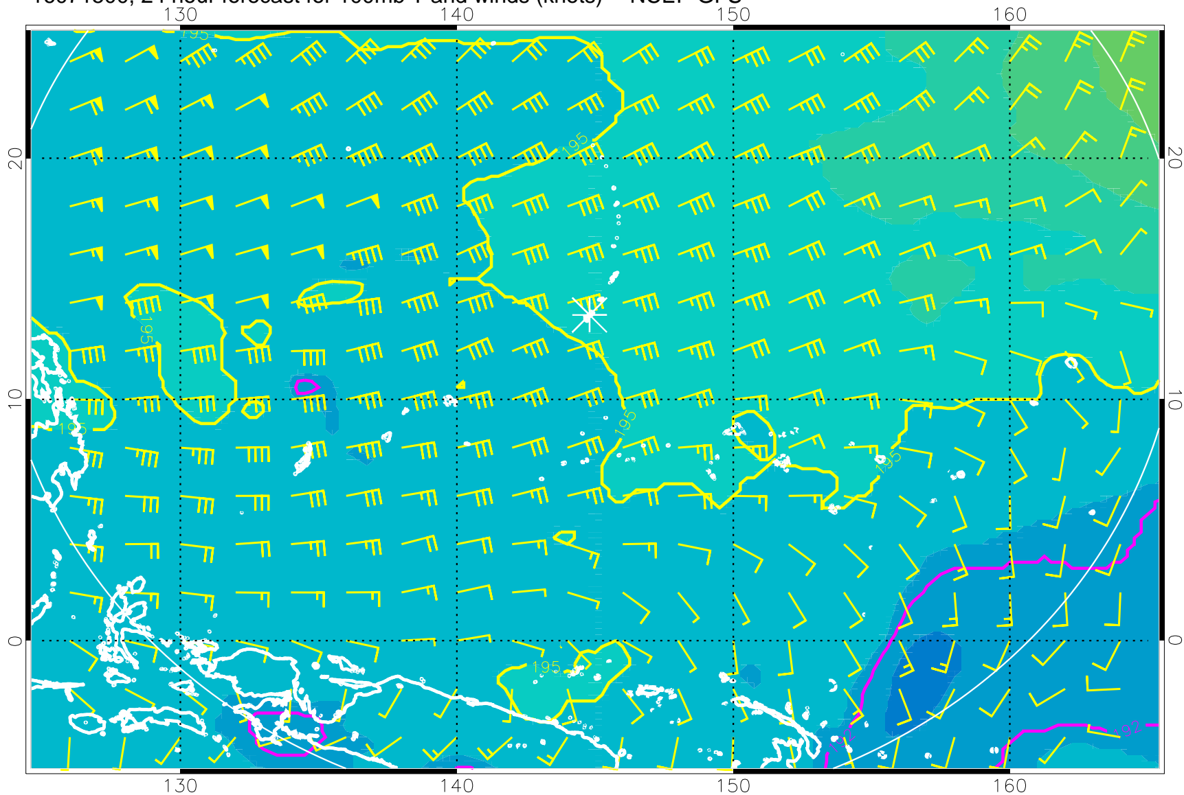
16071500, 24 hour forecast for 100mb T and winds (knots) -- NCEP GFS
