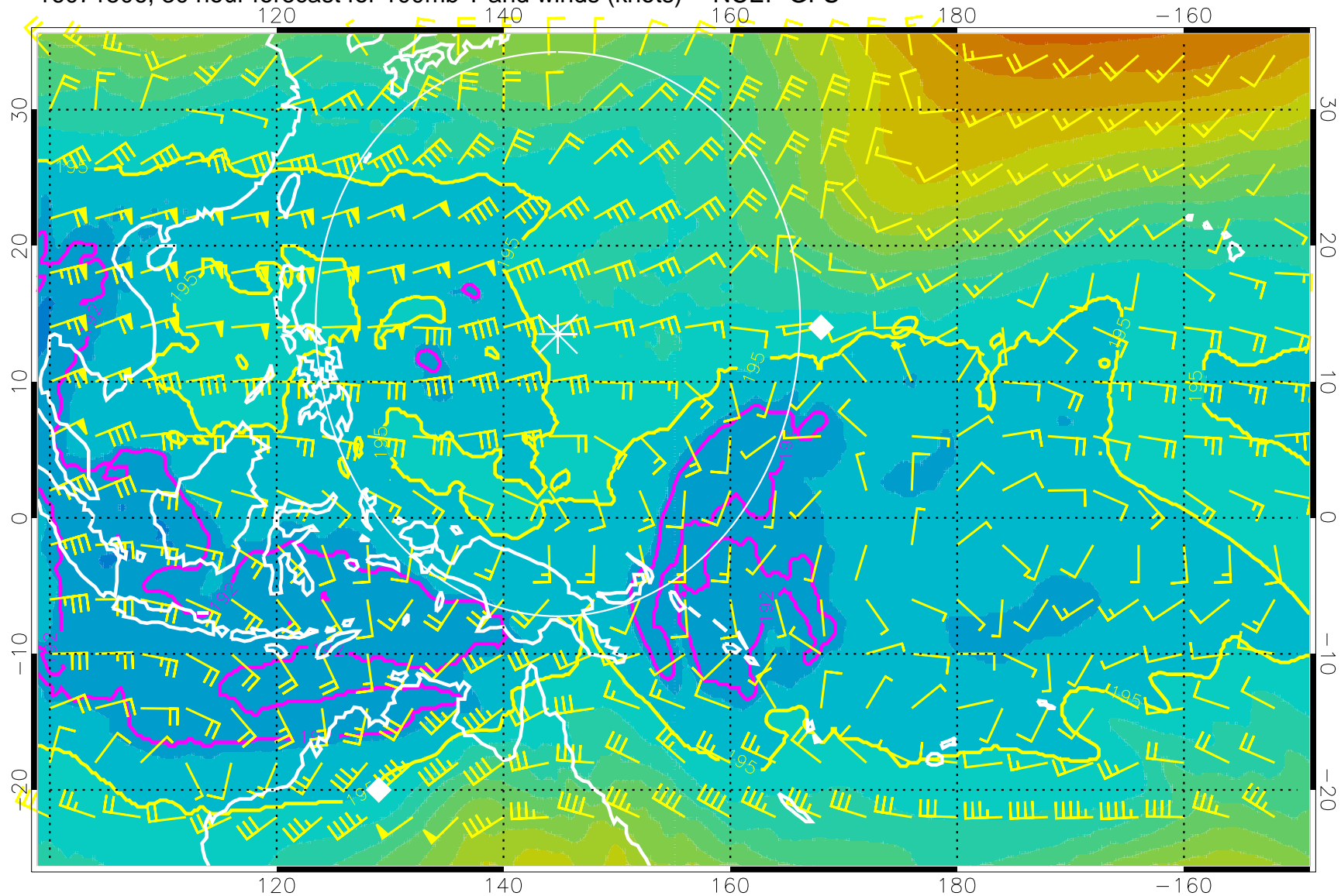
16071506, 30 hour forecast for 100mb T and winds (knots) -- NCEP GFS
