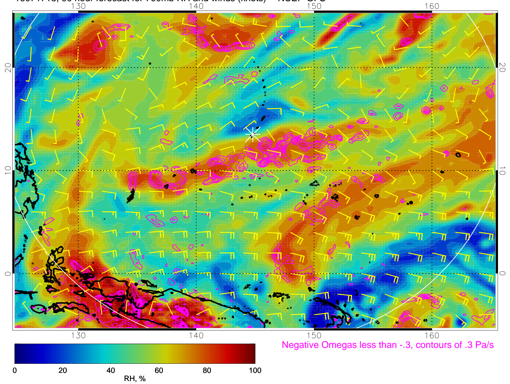
16071718, 90 hour forecast for 700mb RH and winds (knots) -- NCEP GFS
