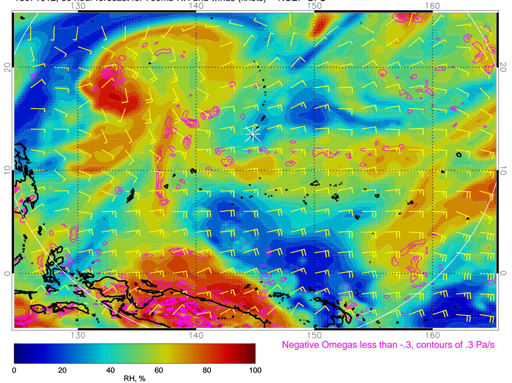
16071612, 60 hour forecast for 700mb RH and winds (knots) -- NCEP GFS
