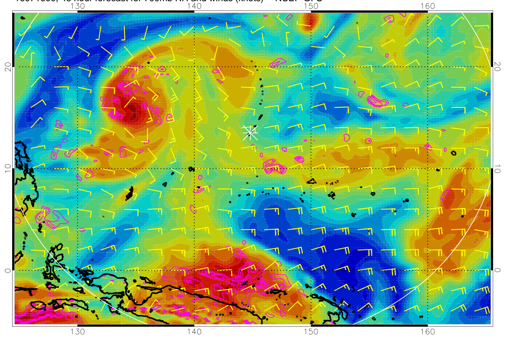
16071600, 48 hour forecast for 700mb RH and winds (knots) -- NCEP GFS
