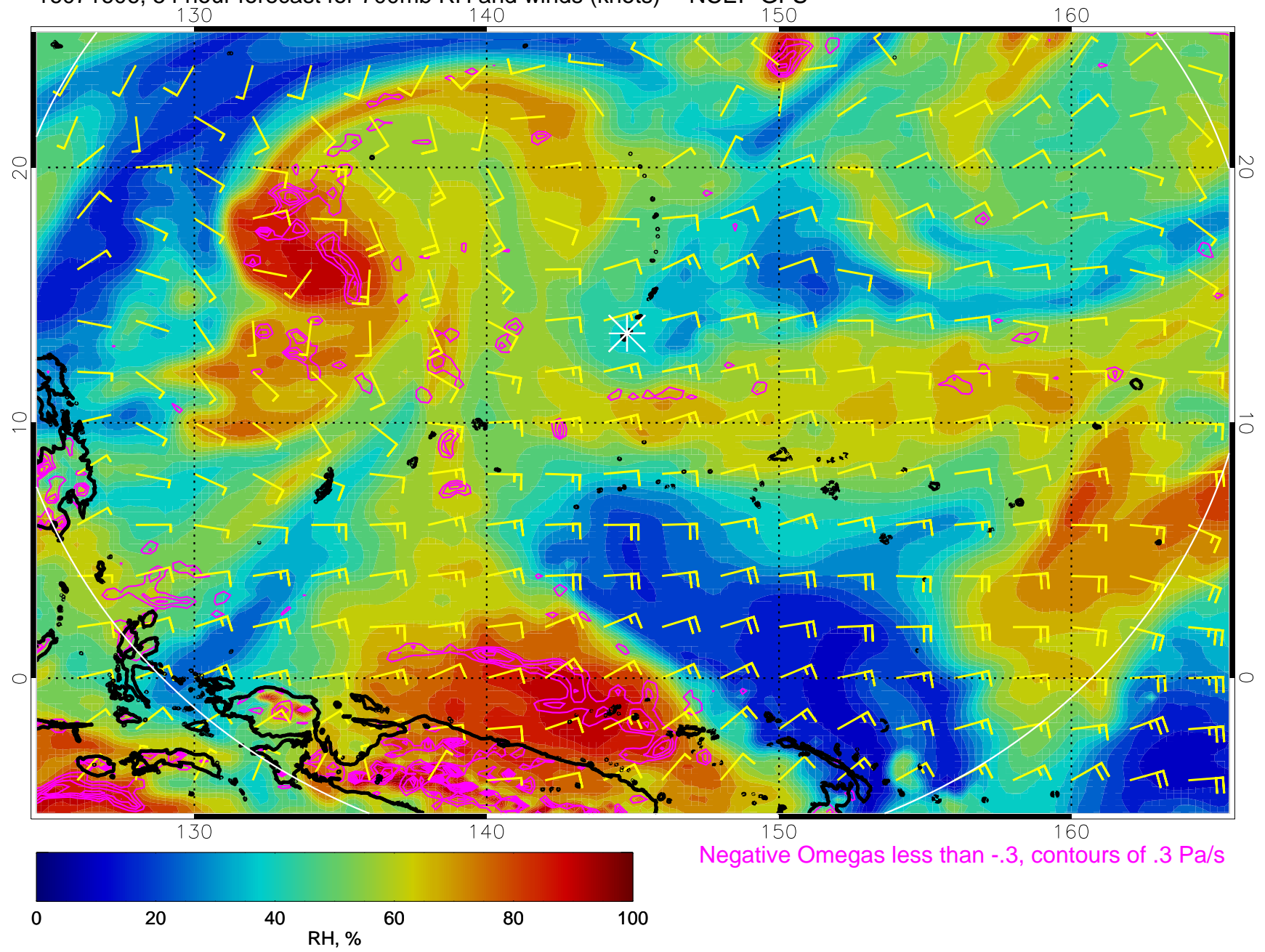
16071606, 54 hour forecast for 700mb RH and winds (knots) -- NCEP GFS
