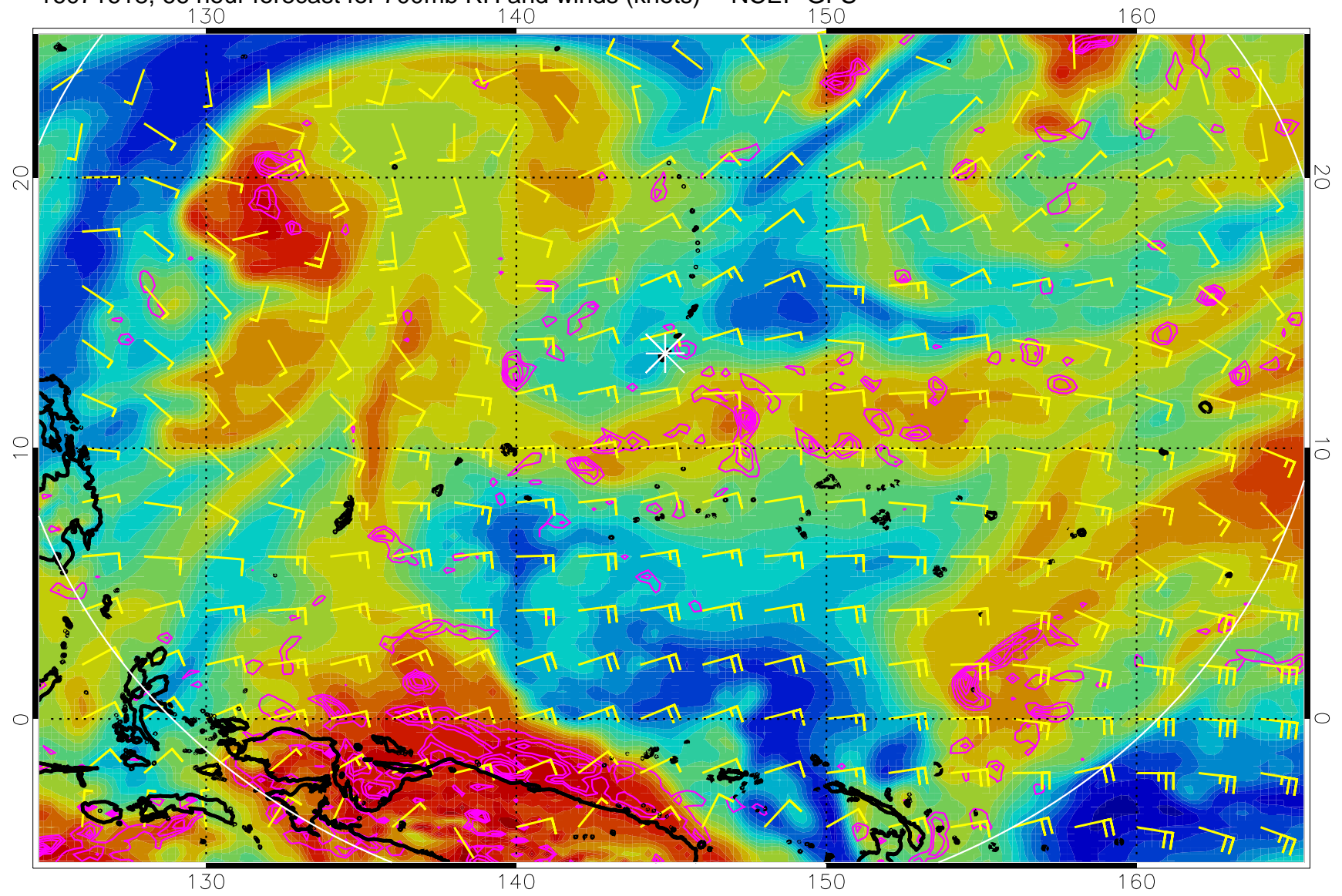
16071618, 66 hour forecast for 700mb RH and winds (knots) -- NCEP GFS
