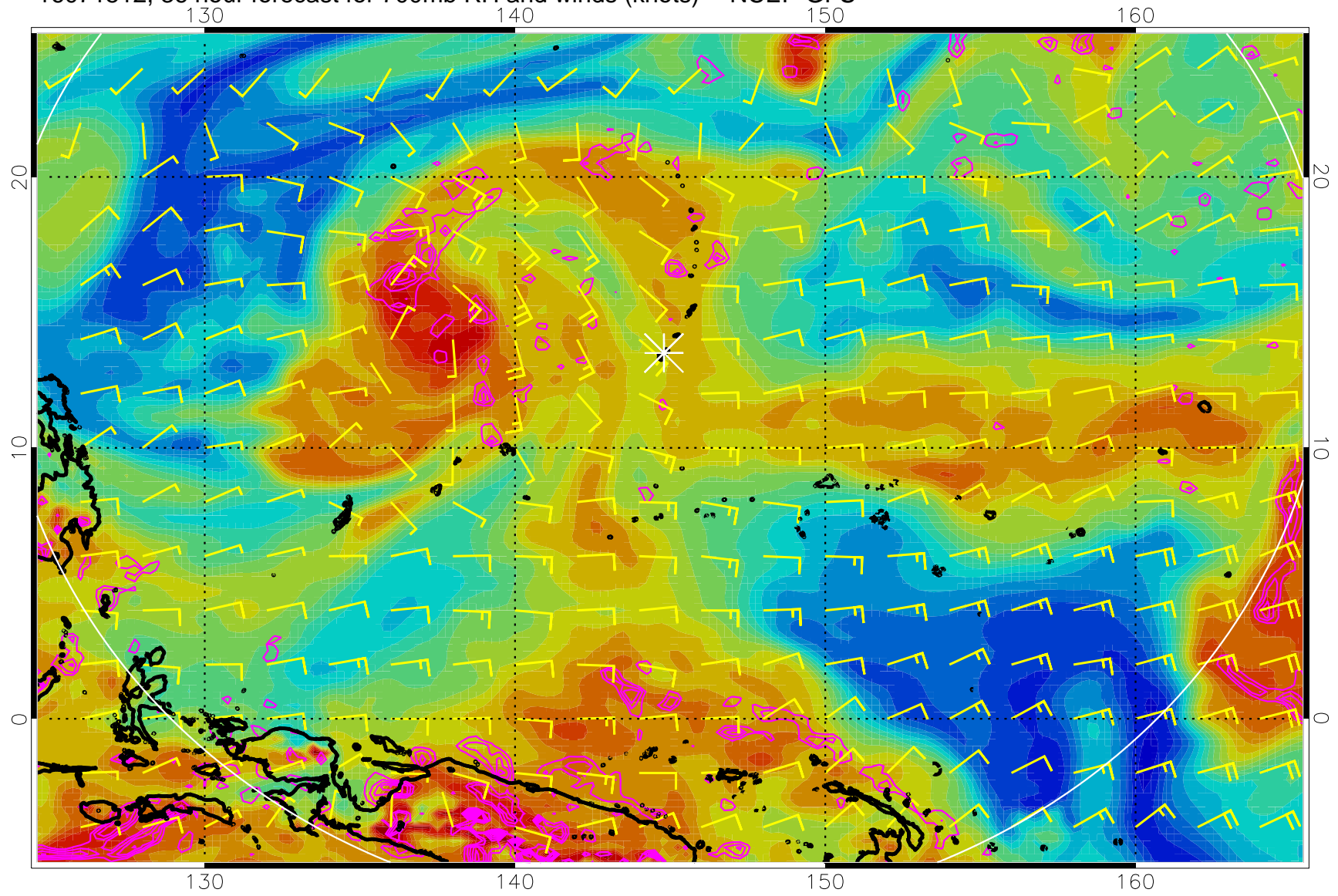
16071512, 36 hour forecast for 700mb RH and winds (knots) -- NCEP GFS
