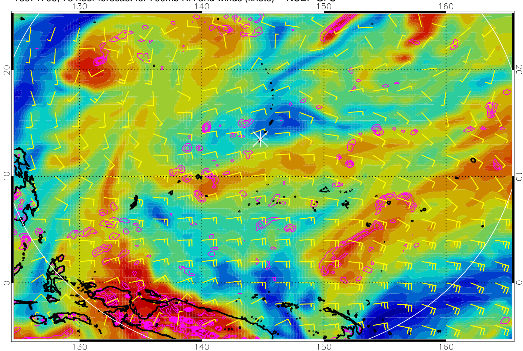
16071706, 78 hour forecast for 700mb RH and winds (knots) -- NCEP GFS
