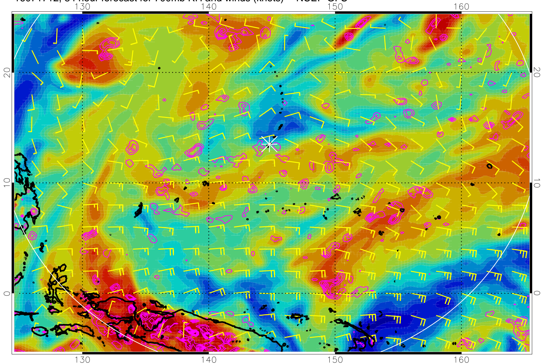
16071712, 84 hour forecast for 700mb RH and winds (knots) -- NCEP GFS
