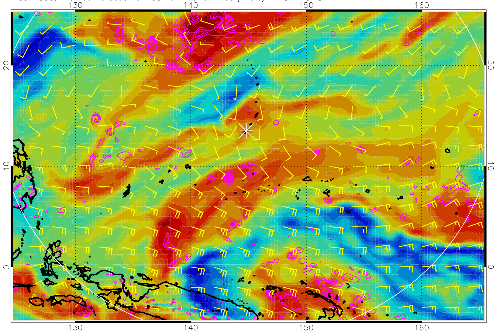
16071900, 120 hour forecast for 700mb RH and winds (knots) -- NCEP GFS
