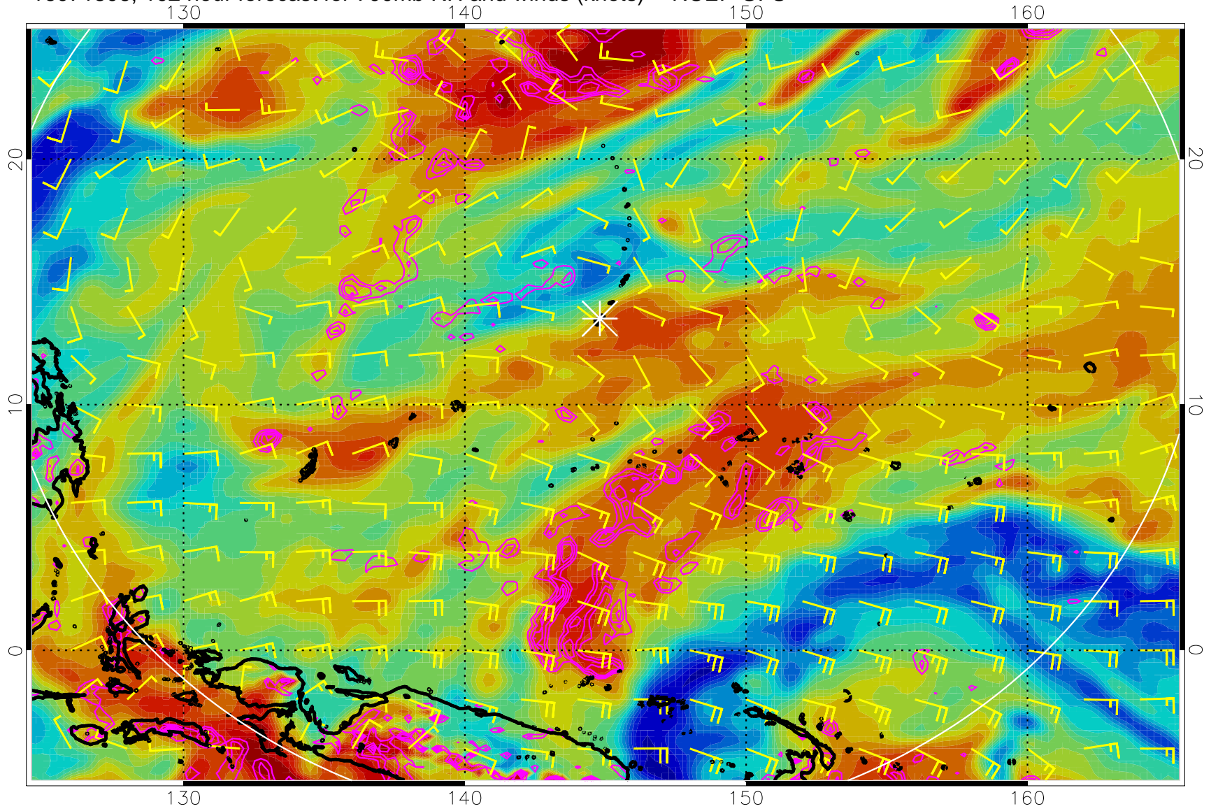
16071806, 102 hour forecast for 700mb RH and winds (knots) -- NCEP GFS
