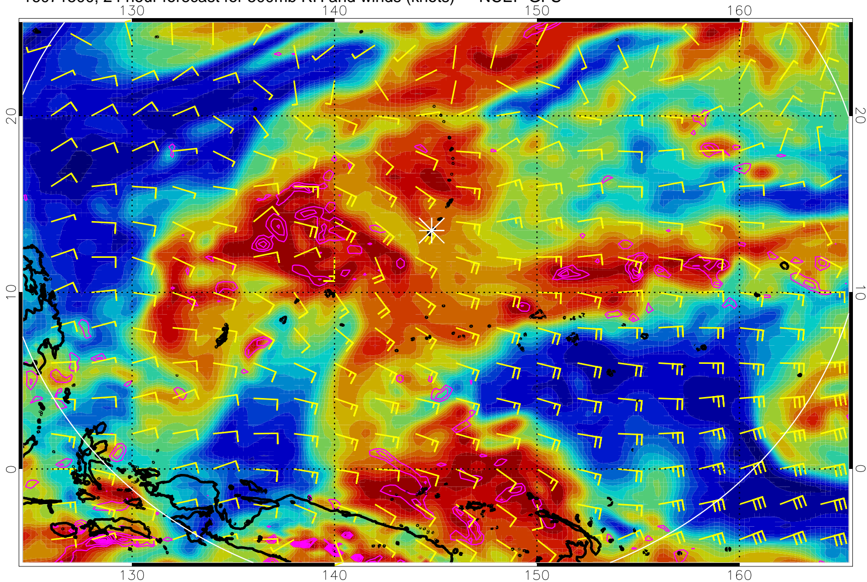
16071500, 24 hour forecast for 500mb RH and winds (knots) -- NCEP GFS
