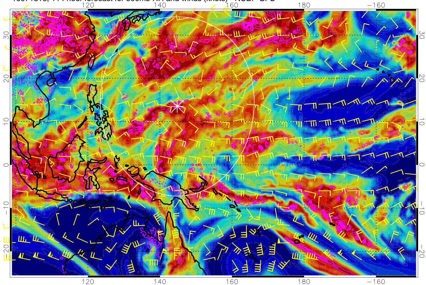
16071818, 114 hour forecast for 500mb RH and winds (knots) - NCEP GFS
