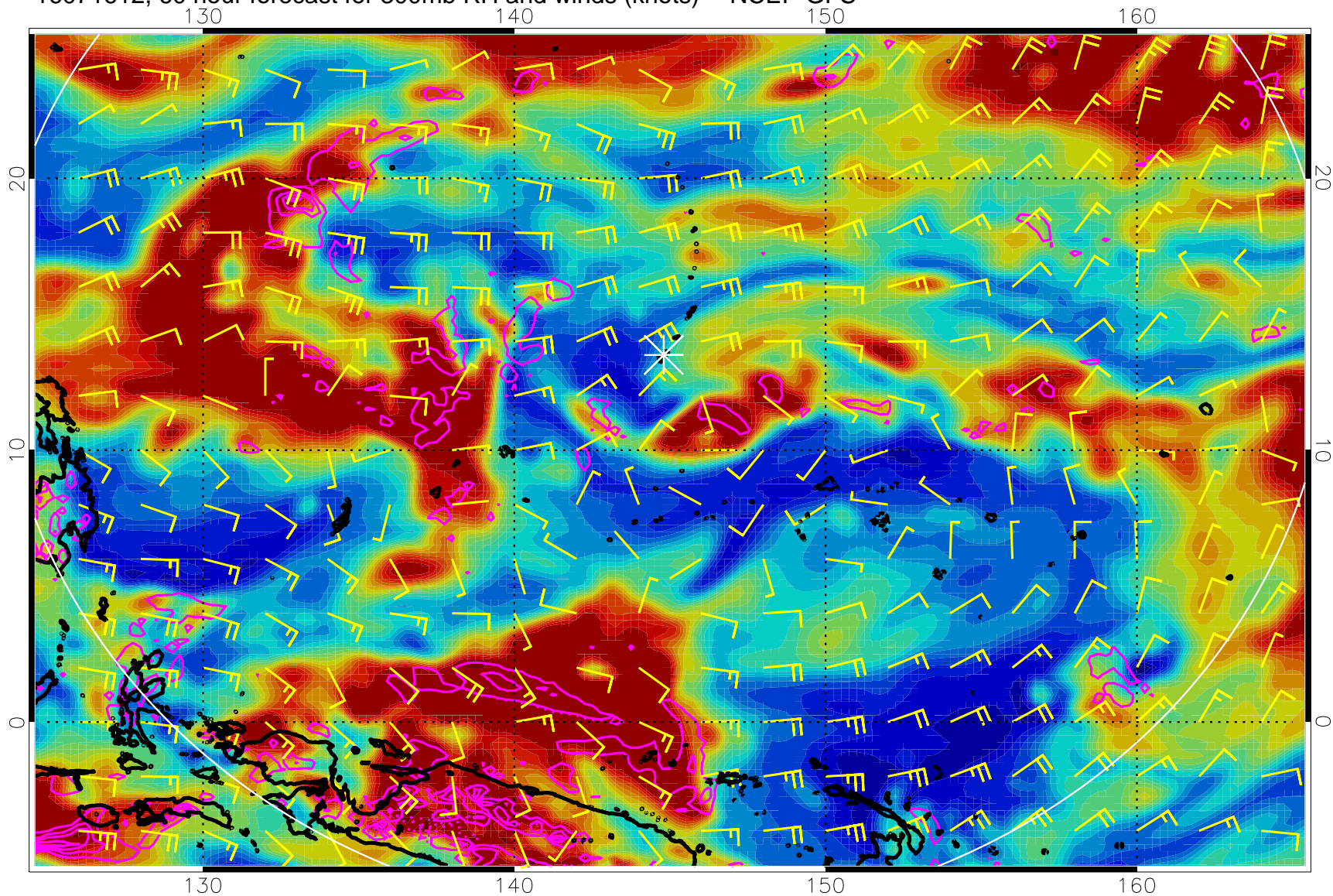
16071612, 60 hour forecast for 300mb RH and winds (knots) -- NCEP GFS
