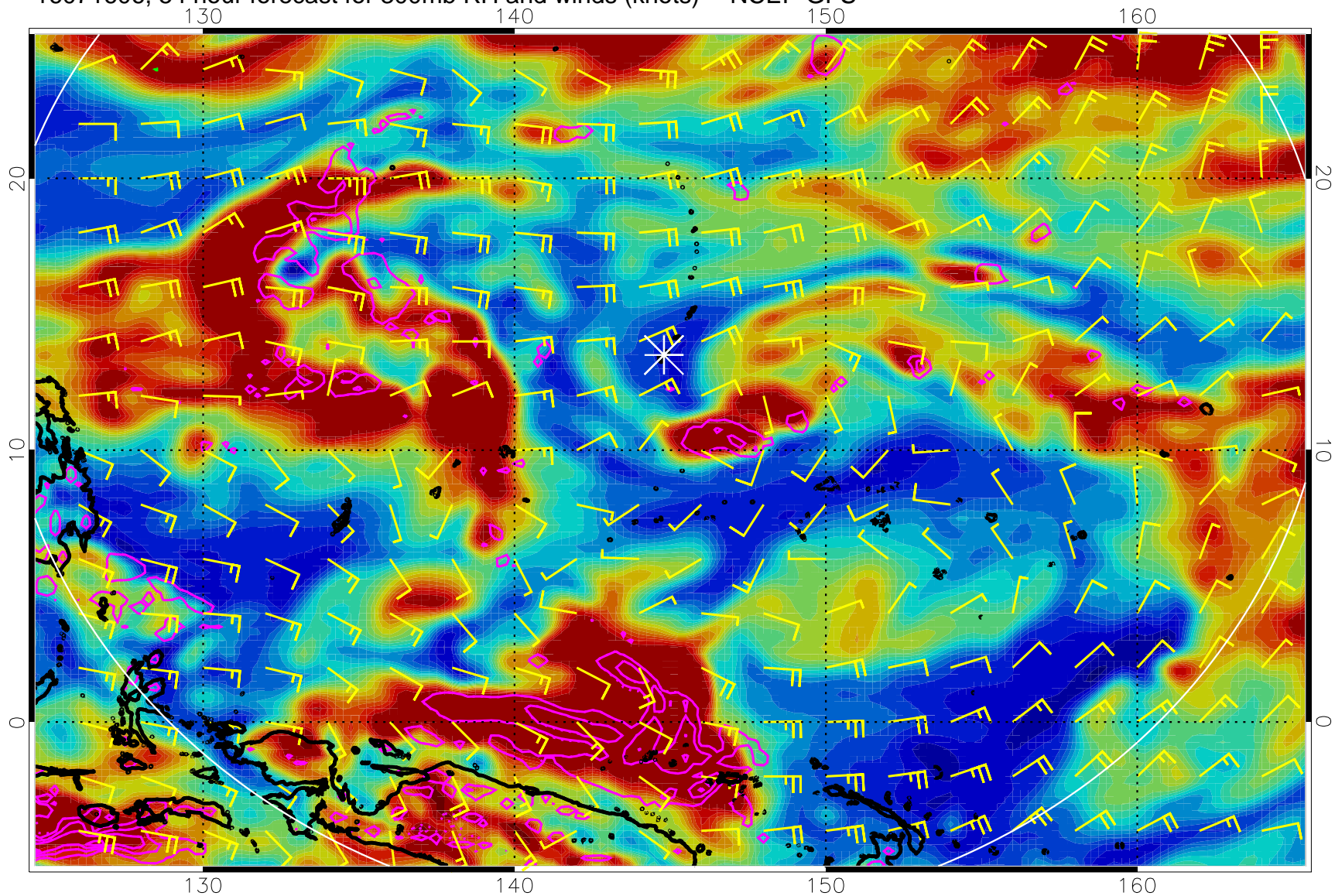
16071606, 54 hour forecast for 300mb RH and winds (knots) -- NCEP GFS
