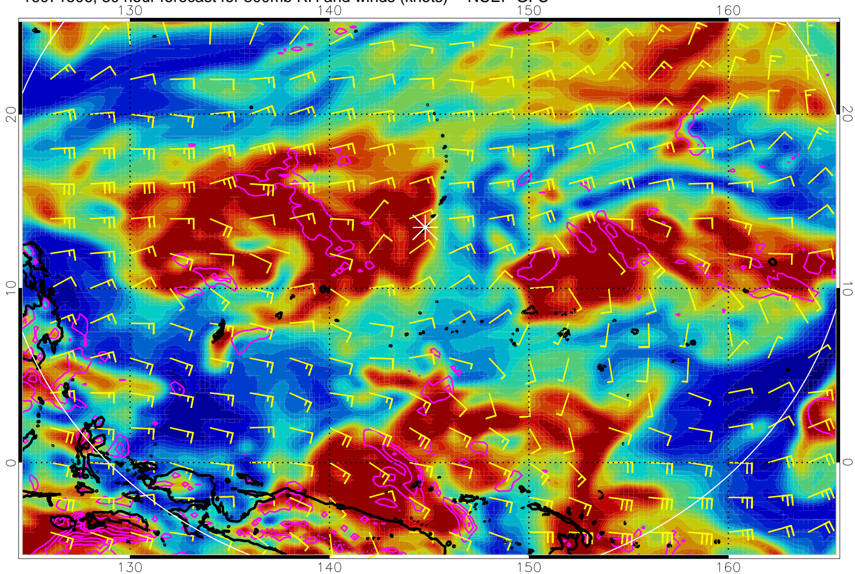
16071506, 30 hour forecast for 300mb RH and winds (knots) -- NCEP GFS
