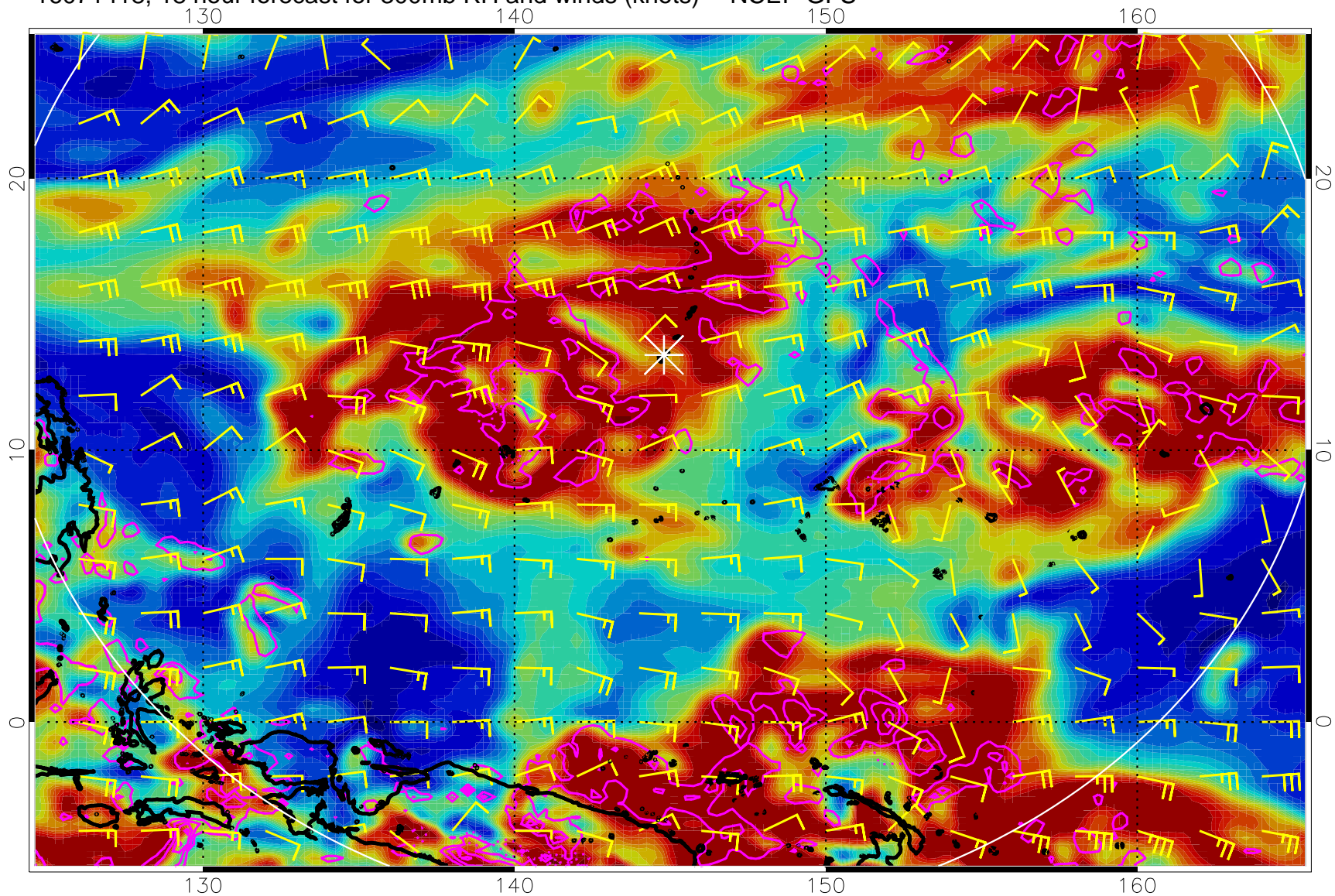
16071418, 18 hour forecast for 300mb RH and winds (knots) -- NCEP GFS
