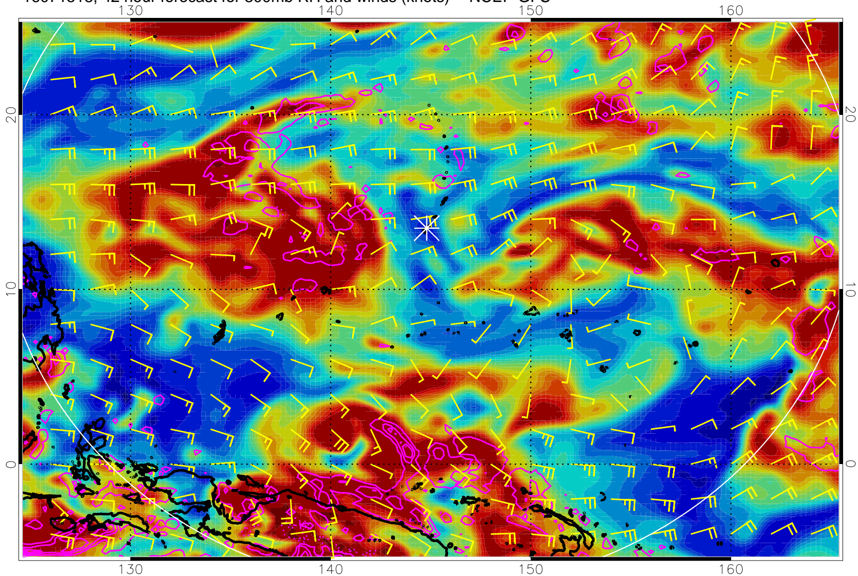
16071518, 42 hour forecast for 300mb RH and winds (knots) -- NCEP GFS
