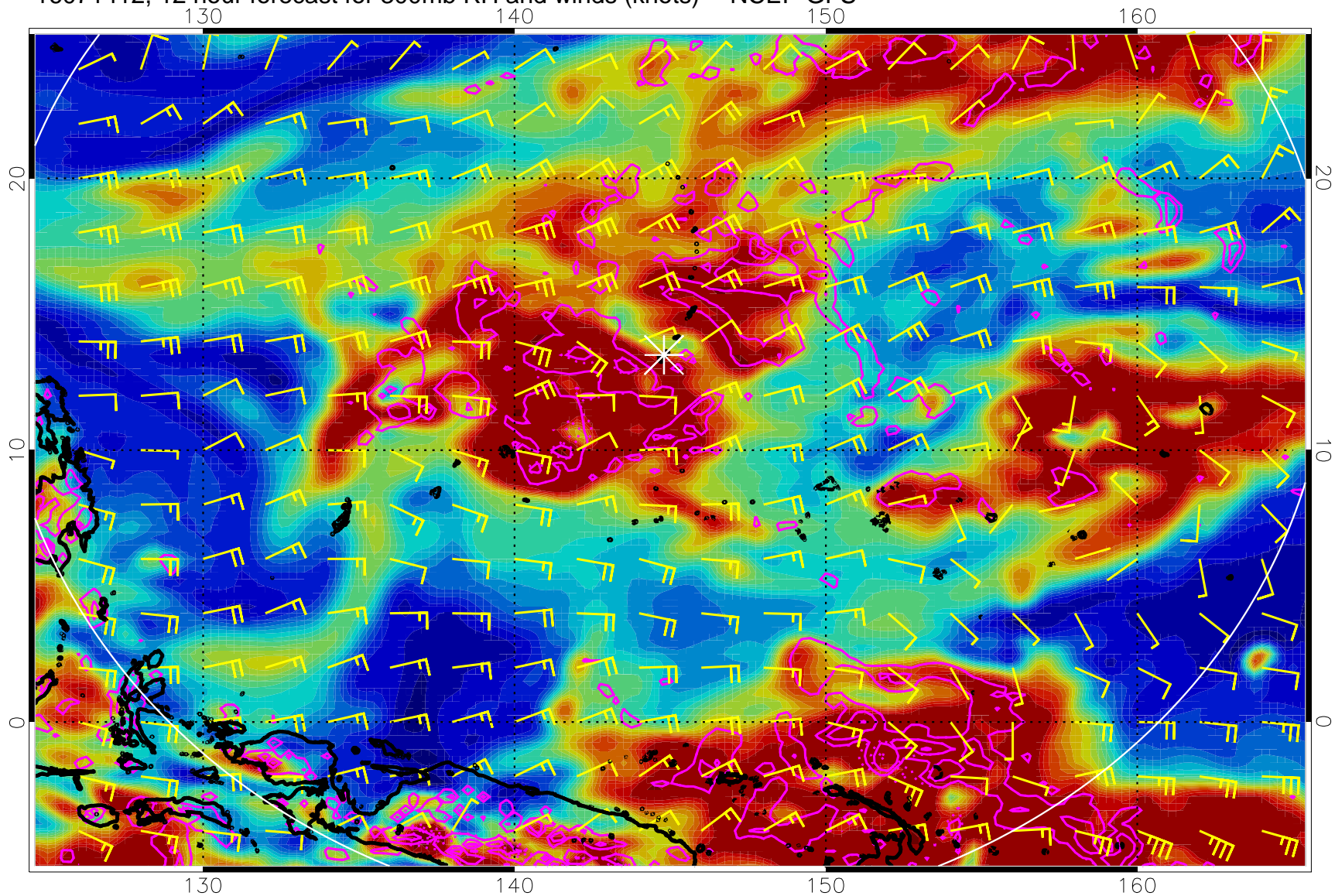
16071412, 12 hour forecast for 300mb RH and winds (knots) -- NCEP GFS
