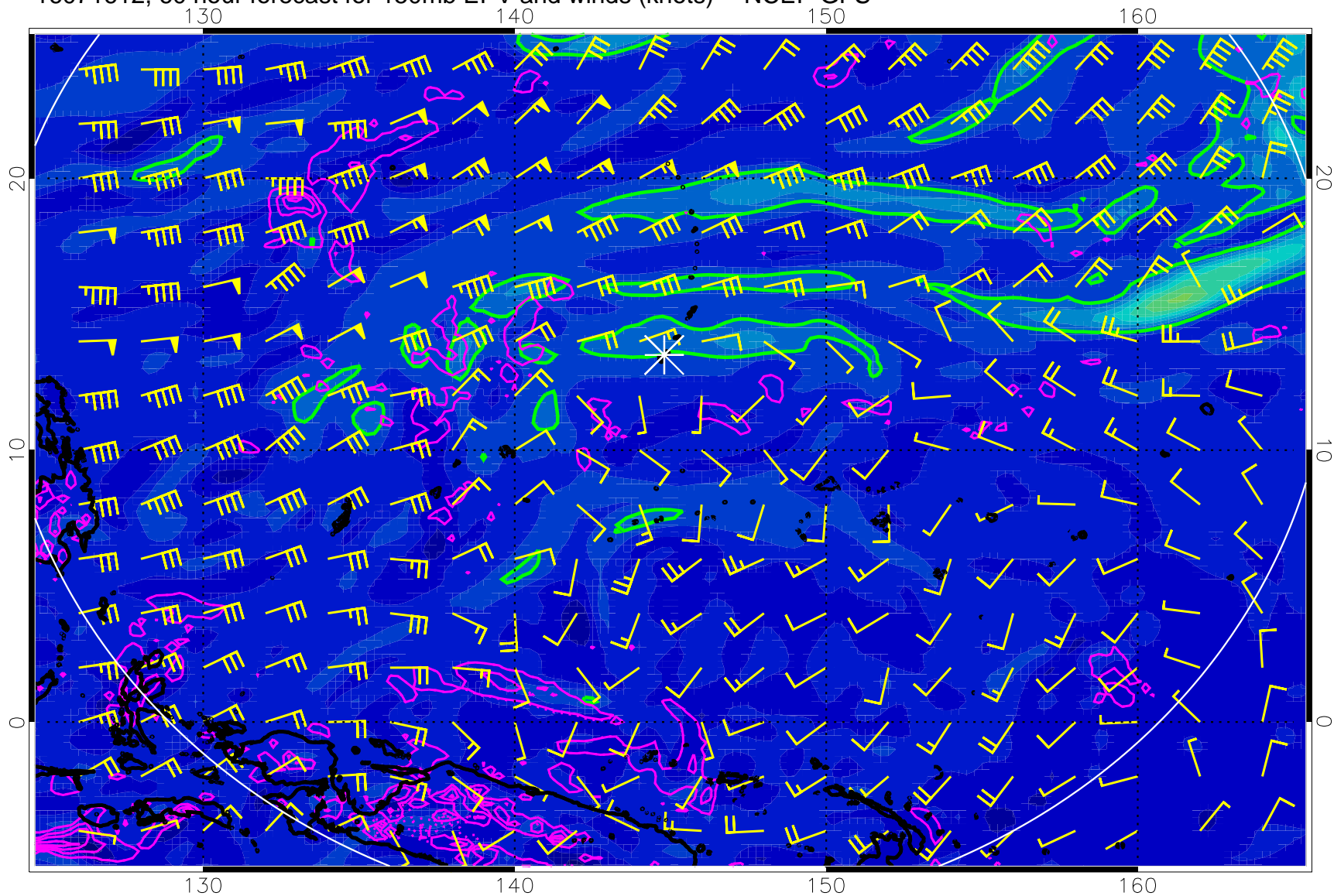
16071612, 60 hour forecast for 150mb EPV and winds (knots) -- NCEP GFS
