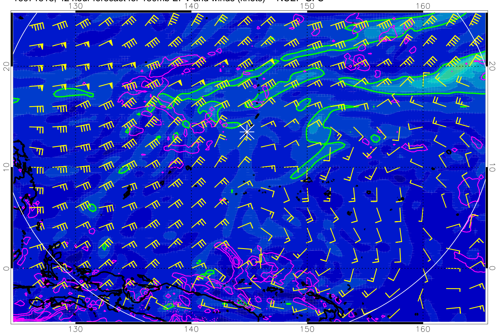
16071518, 42 hour forecast for 150mb EPV and winds (knots) -- NCEP GFS
