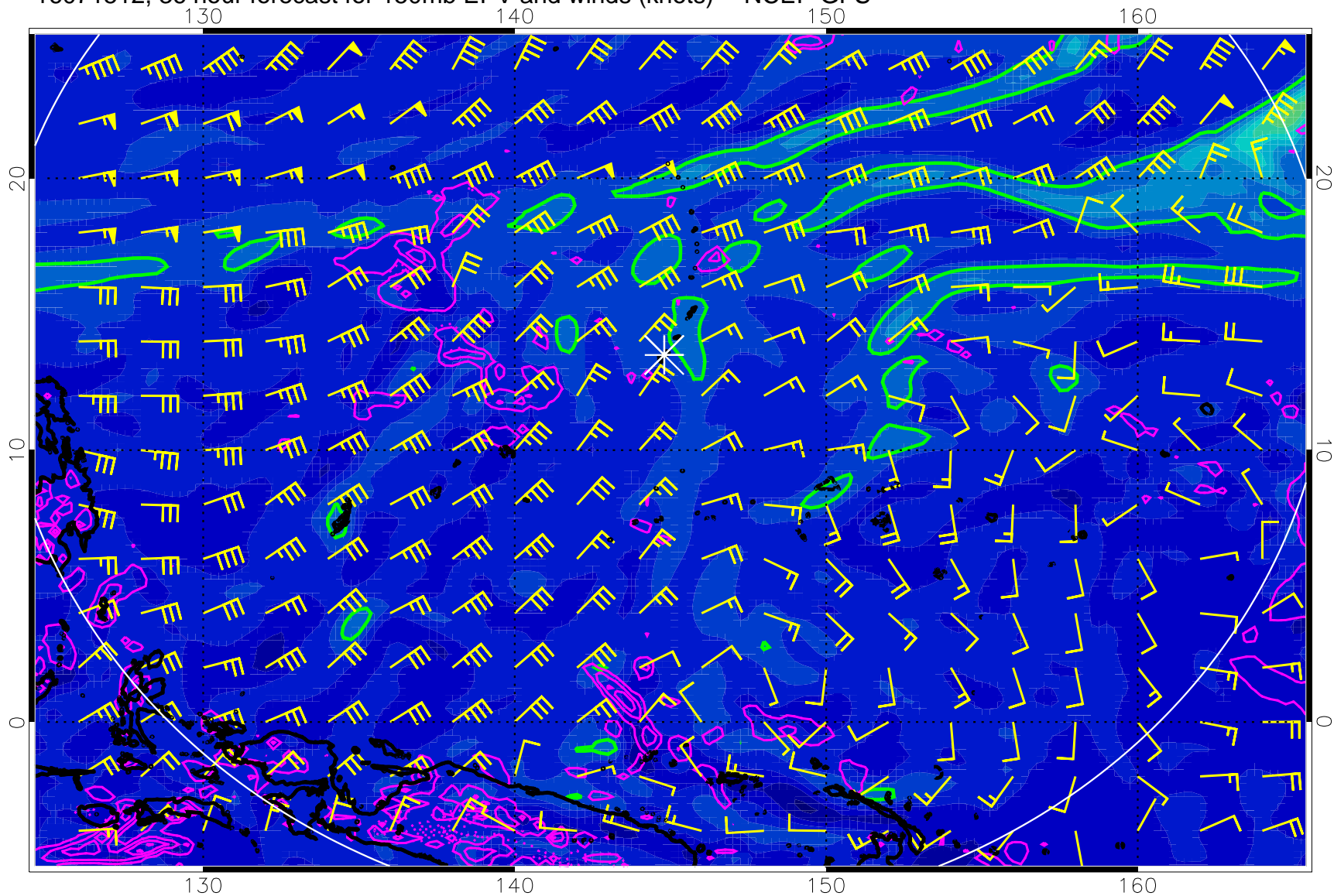
16071512, 36 hour forecast for 150mb EPV and winds (knots) -- NCEP GFS
