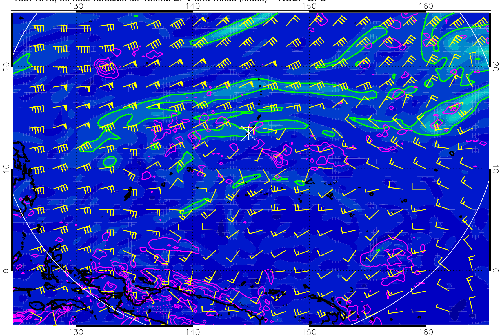
16071618, 66 hour forecast for 150mb EPV and winds (knots) -- NCEP GFS
