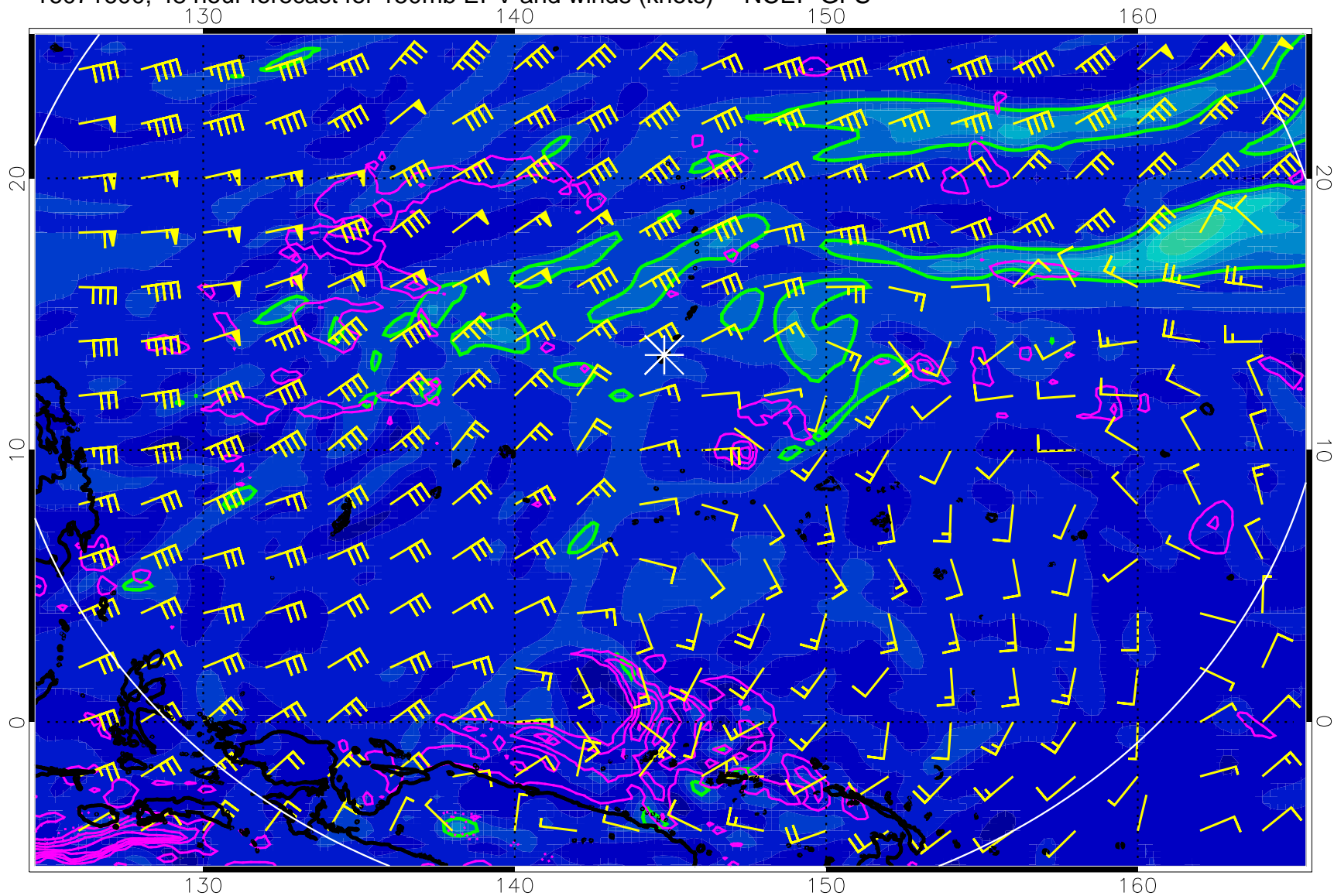
16071600, 48 hour forecast for 150mb EPV and winds (knots) -- NCEP GFS
