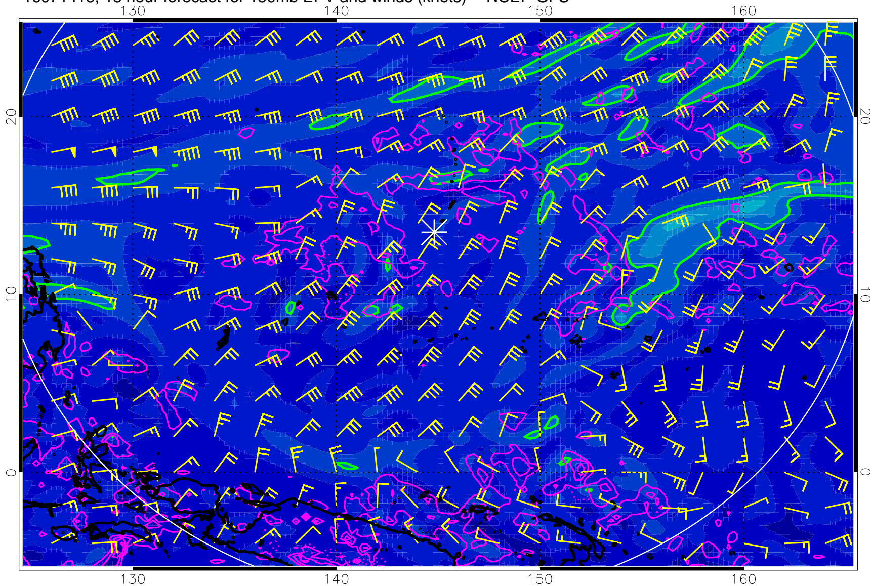
16071418, 18 hour forecast for 150mb EPV and winds (knots) -- NCEP GFS
