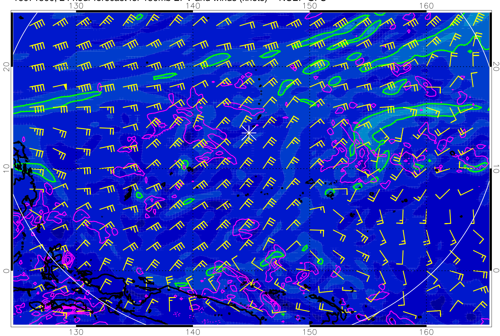
16071500, 24 hour forecast for 150mb EPV and winds (knots) -- NCEP GFS
