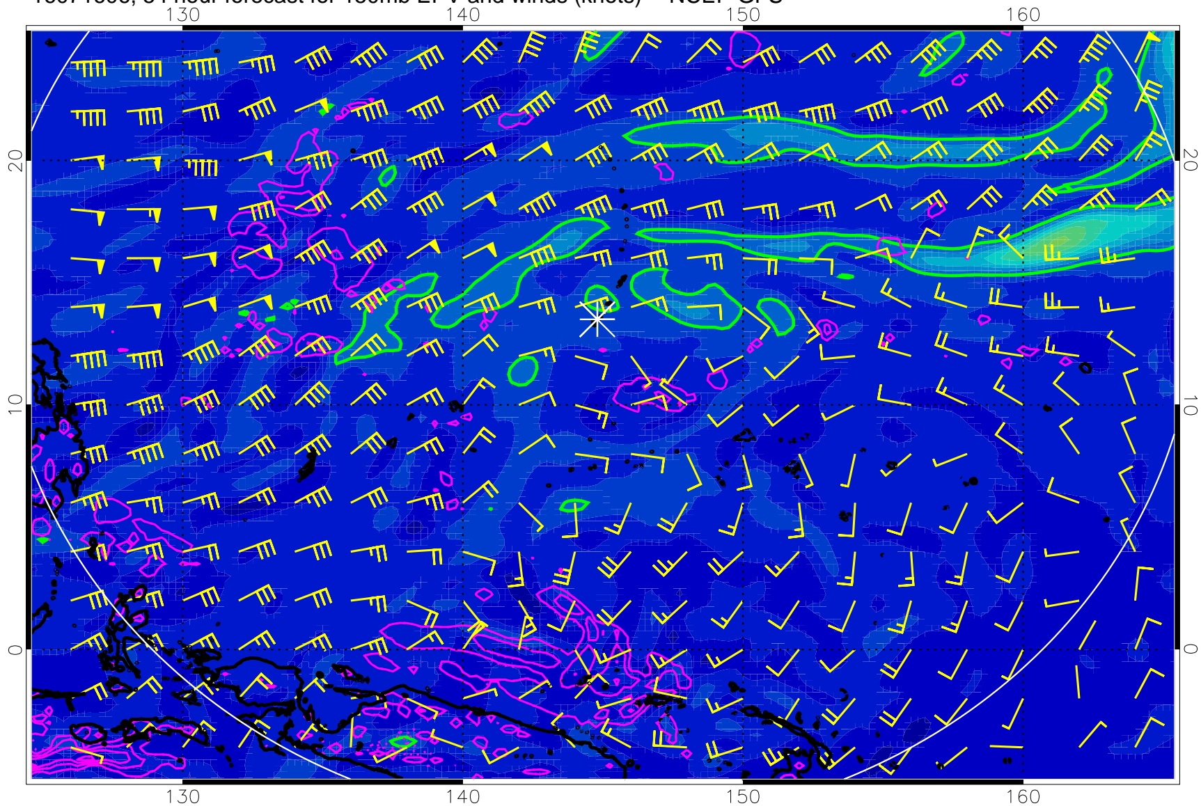
16071606, 54 hour forecast for 150mb EPV and winds (knots) -- NCEP GFS
