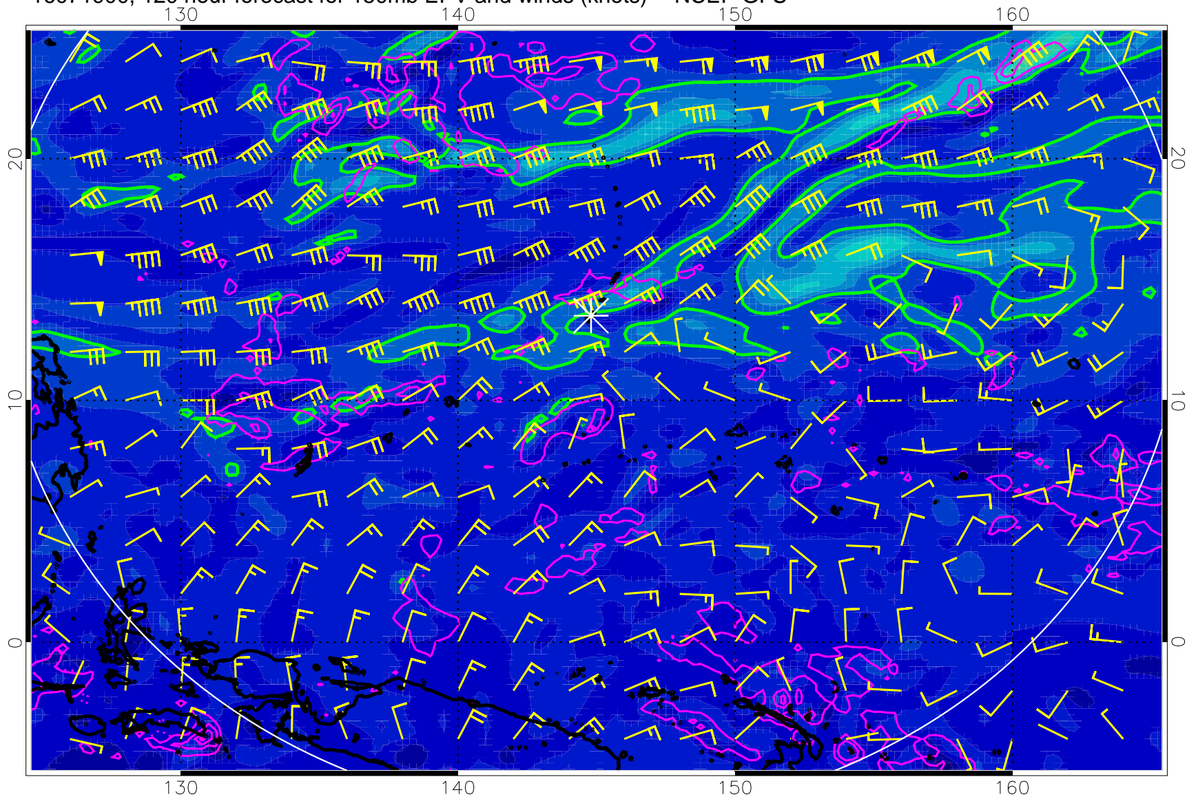
16071900, 120 hour forecast for 150mb EPV and winds (knots) -- NCEP GFS
