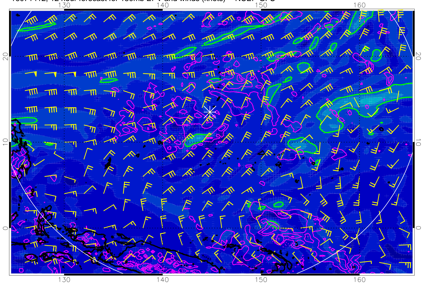
16071412, 12 hour forecast for 150mb EPV and winds (knots) -- NCEP GFS
