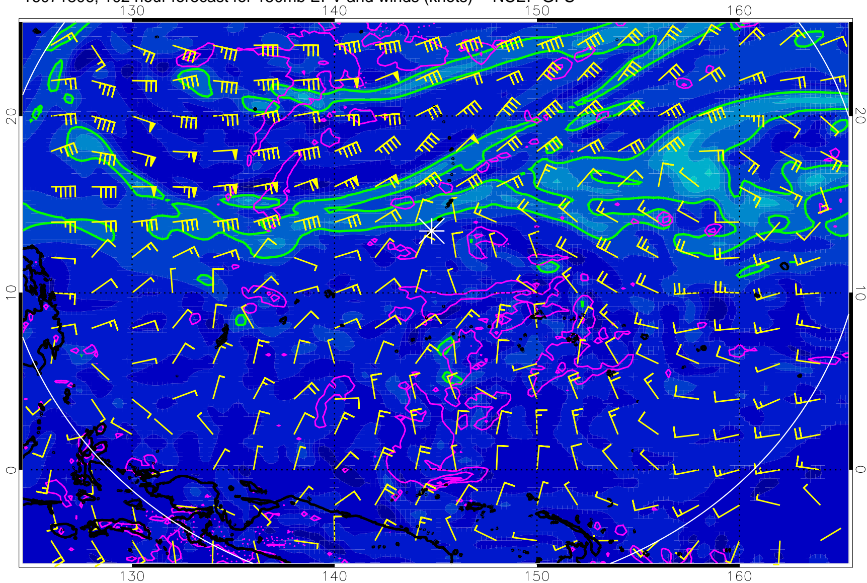
16071806, 102 hour forecast for 150mb EPV and winds (knots) -- NCEP GFS
