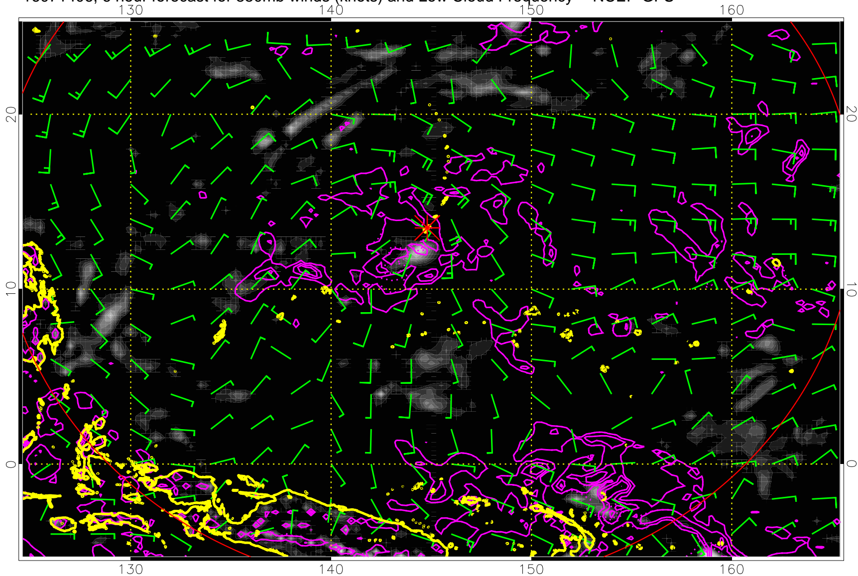
16071406, 6 hour forecast for 850mb winds (knots) and Low Cloud Frequency -- NCEP GFS
