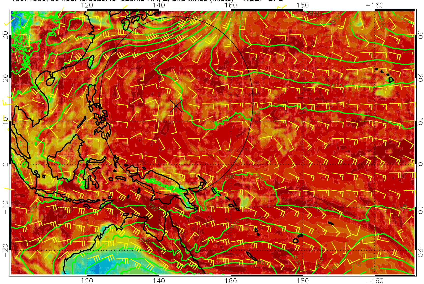
16071500, 36 hour forecast for 925mb RH, Z, and winds (knots) -- NCEP GFS
