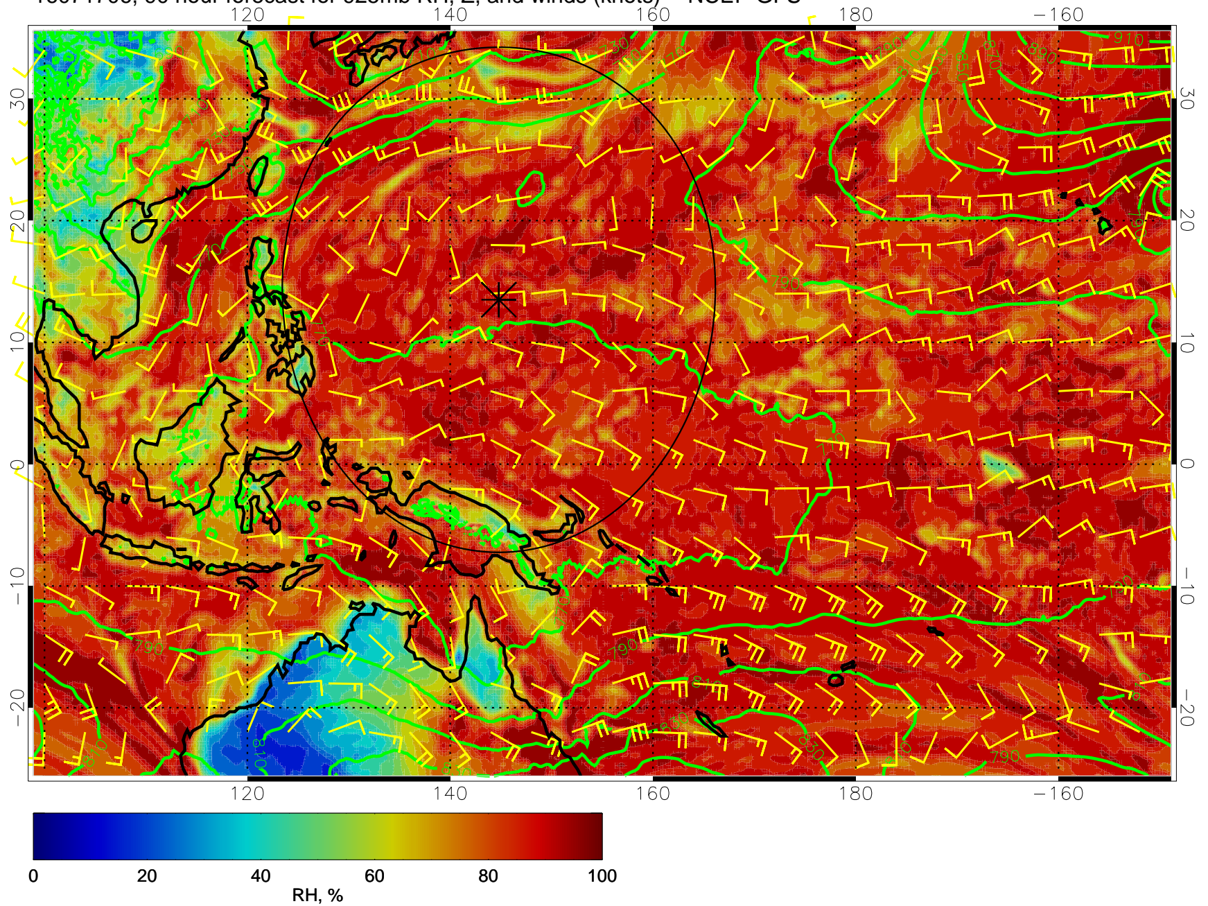
16071706, 90 hour forecast for 925mb RH, Z, and winds (knots) -- NCEP GFS
