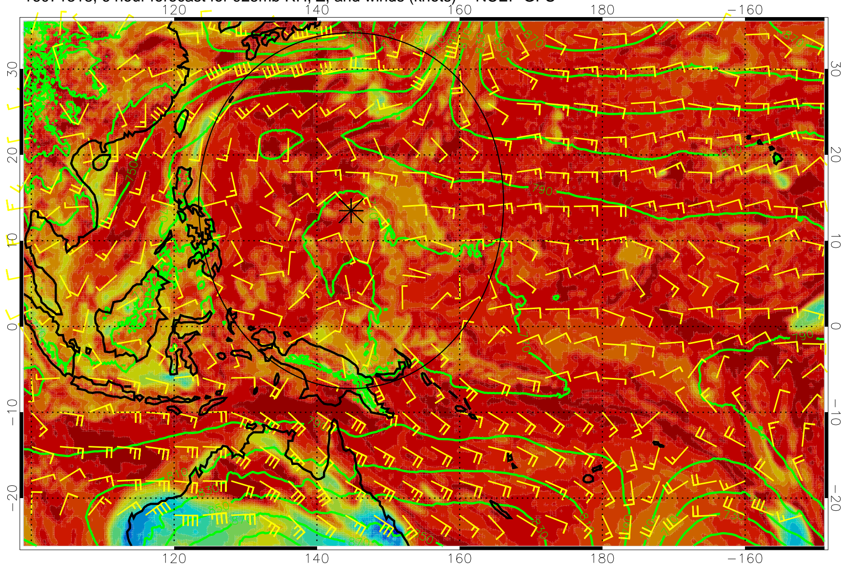
16071318, 6 hour forecast for 925mb RH, Z, and winds (knots) -- NCEP GFS
