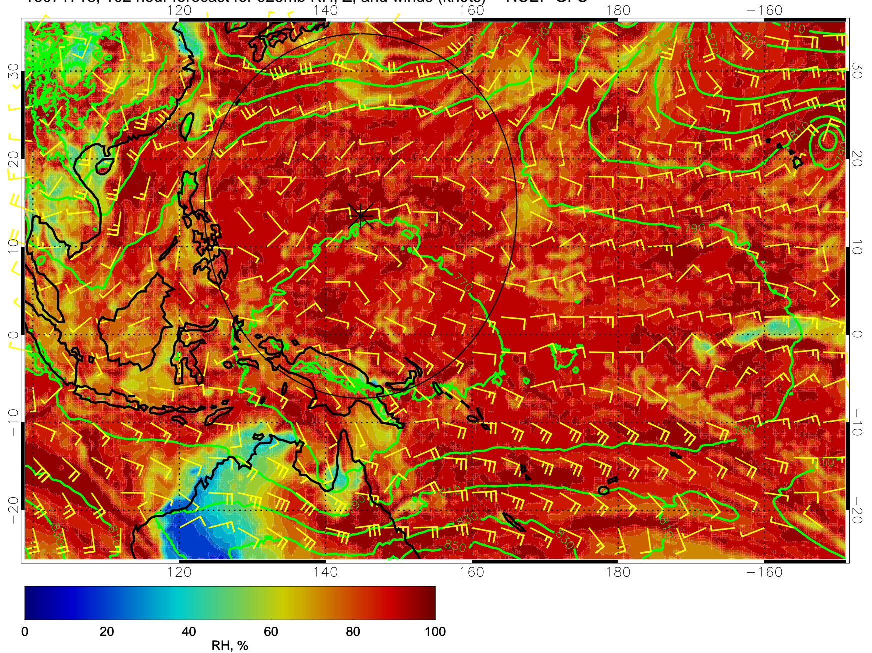
16071718, 102 hour forecast for 925mb RH, Z, and winds (knots) -- NCEP GFS
