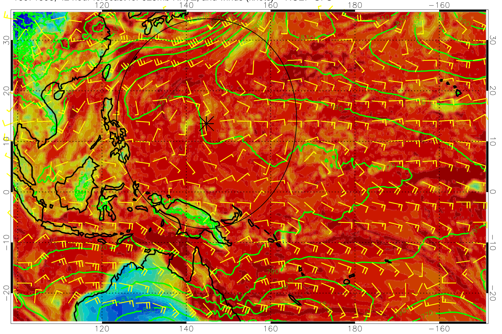
16071506, 42 hour forecast for 925mb RH, Z, and winds (knots) -- NCEP GFS
