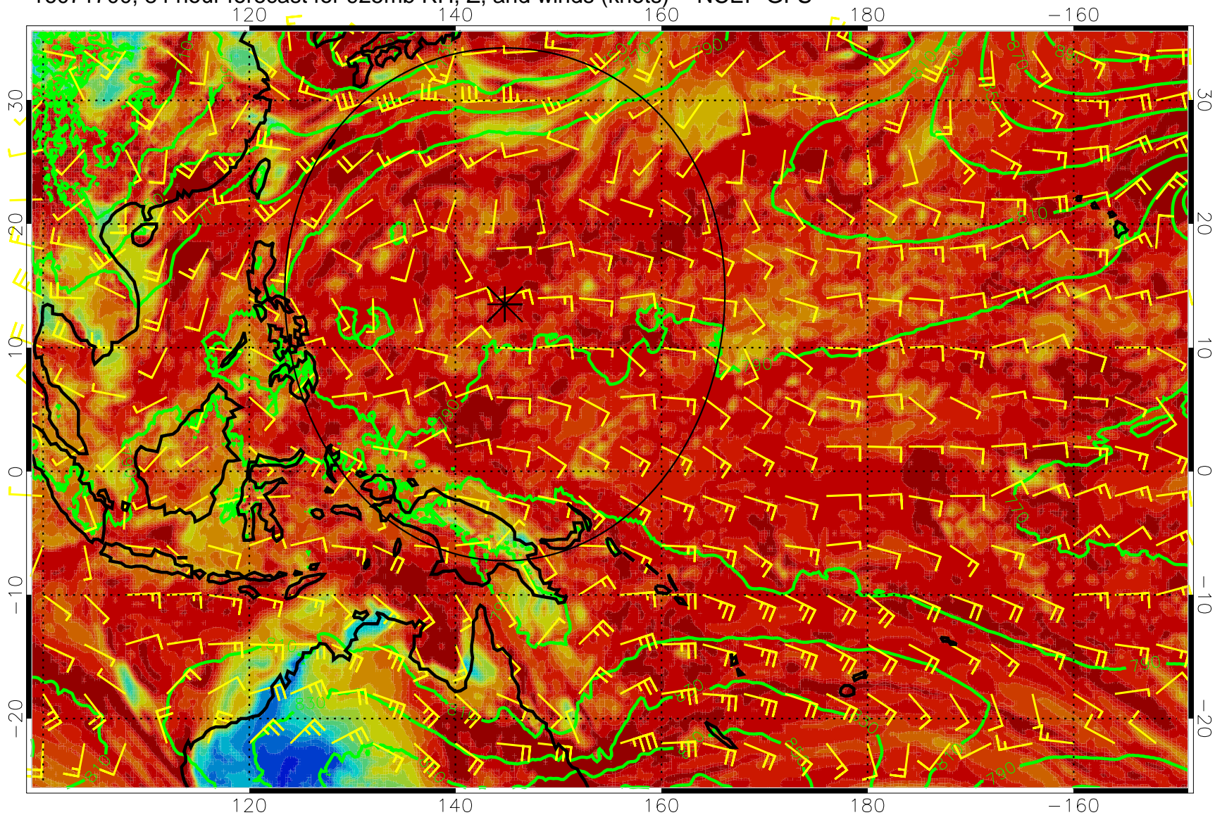
16071700, 84 hour forecast for 925mb RH, Z, and winds (knots) -- NCEP GFS
