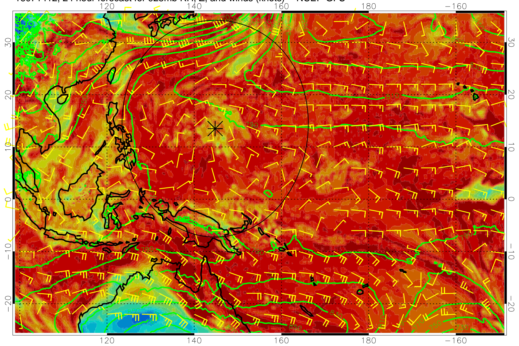
16071412, 24 hour forecast for 925mb RH, Z, and winds (knots) -- NCEP GFS
