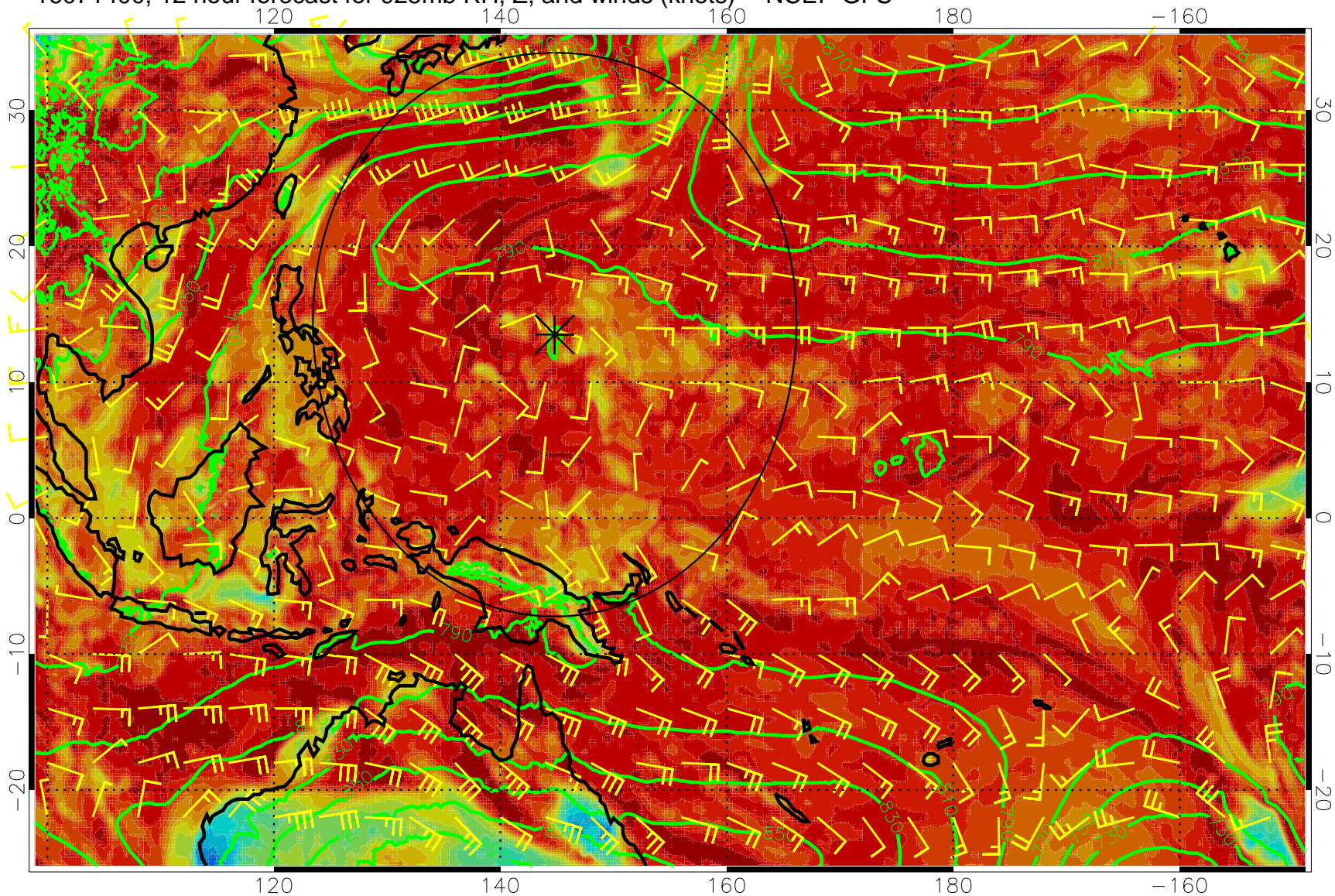
16071400, 12 hour forecast for 925mb RH, Z, and winds (knots) -- NCEP GFS
