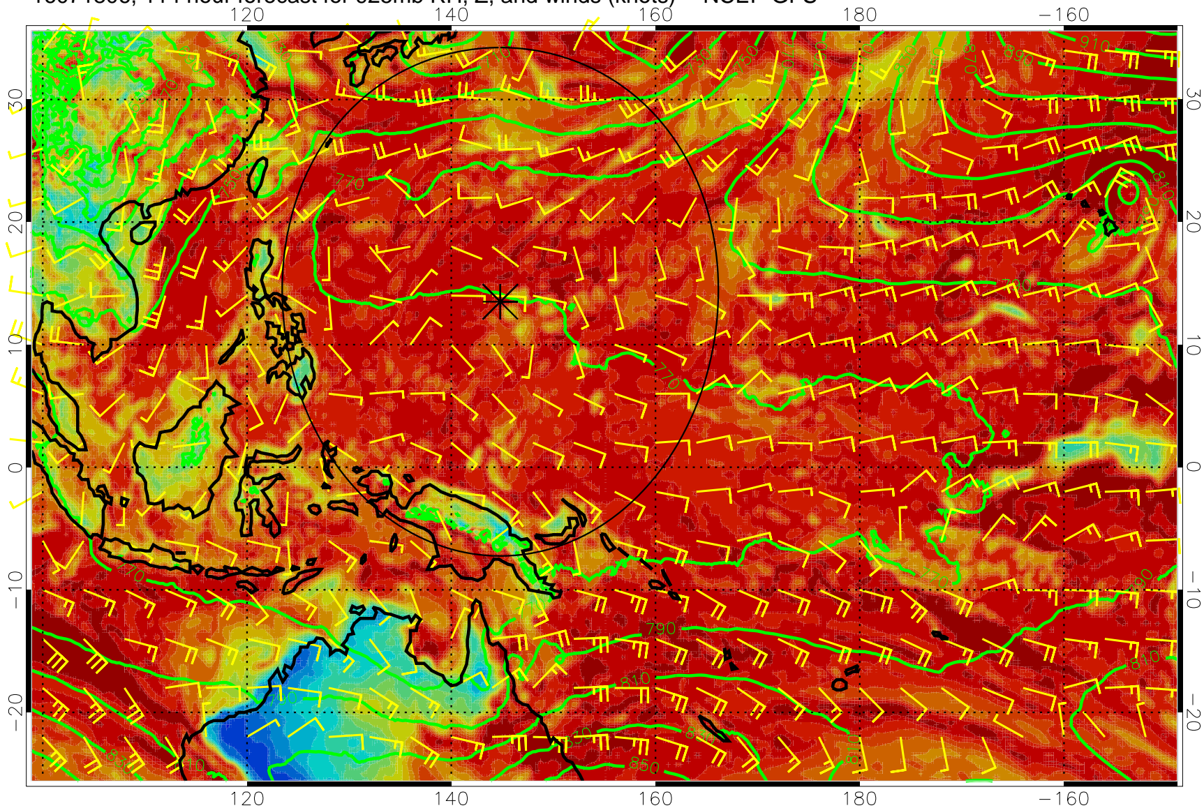
16071806, 114 hour forecast for 925mb RH, Z, and winds (knots) -- NCEP GFS
