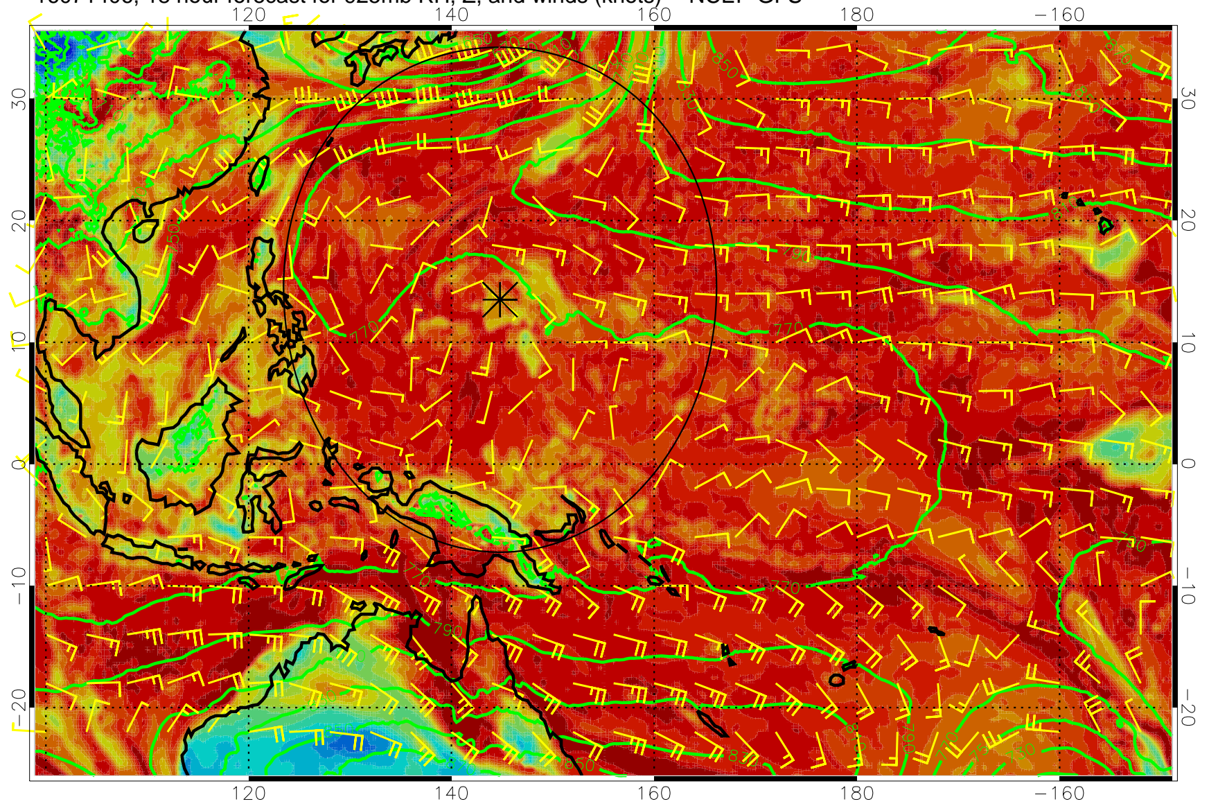
16071406, 18 hour forecast for 925mb RH, Z, and winds (knots) -- NCEP GFS
