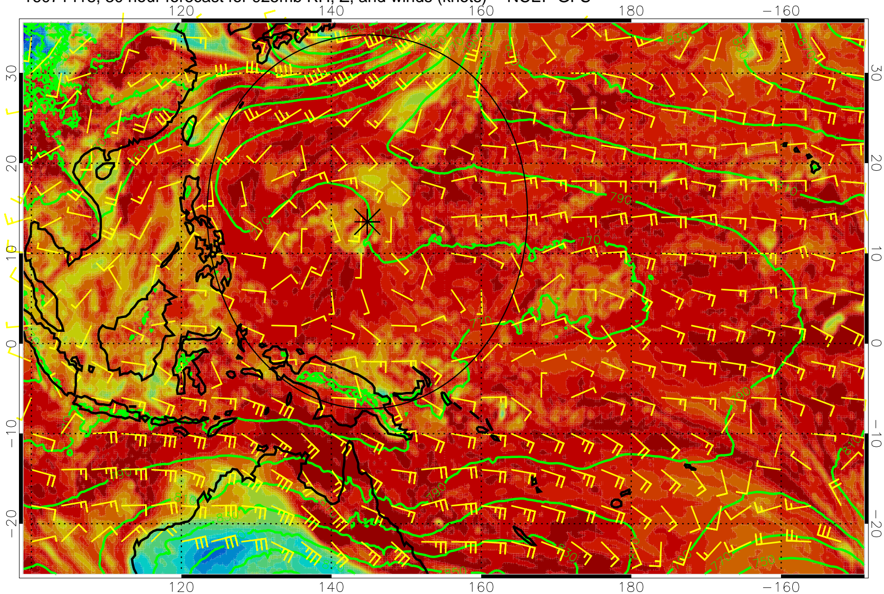
16071418, 30 hour forecast for 925mb RH, Z, and winds (knots) -- NCEP GFS
