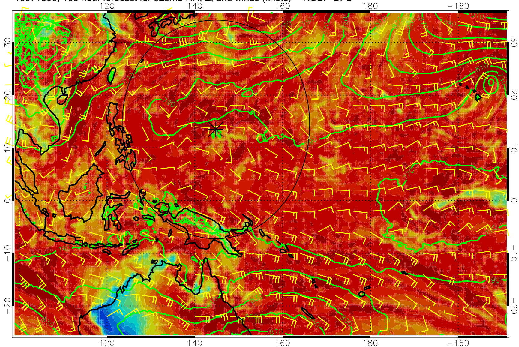
16071800, 108 hour forecast for 925mb RH, Z, and winds (knots) -- NCEP GFS
