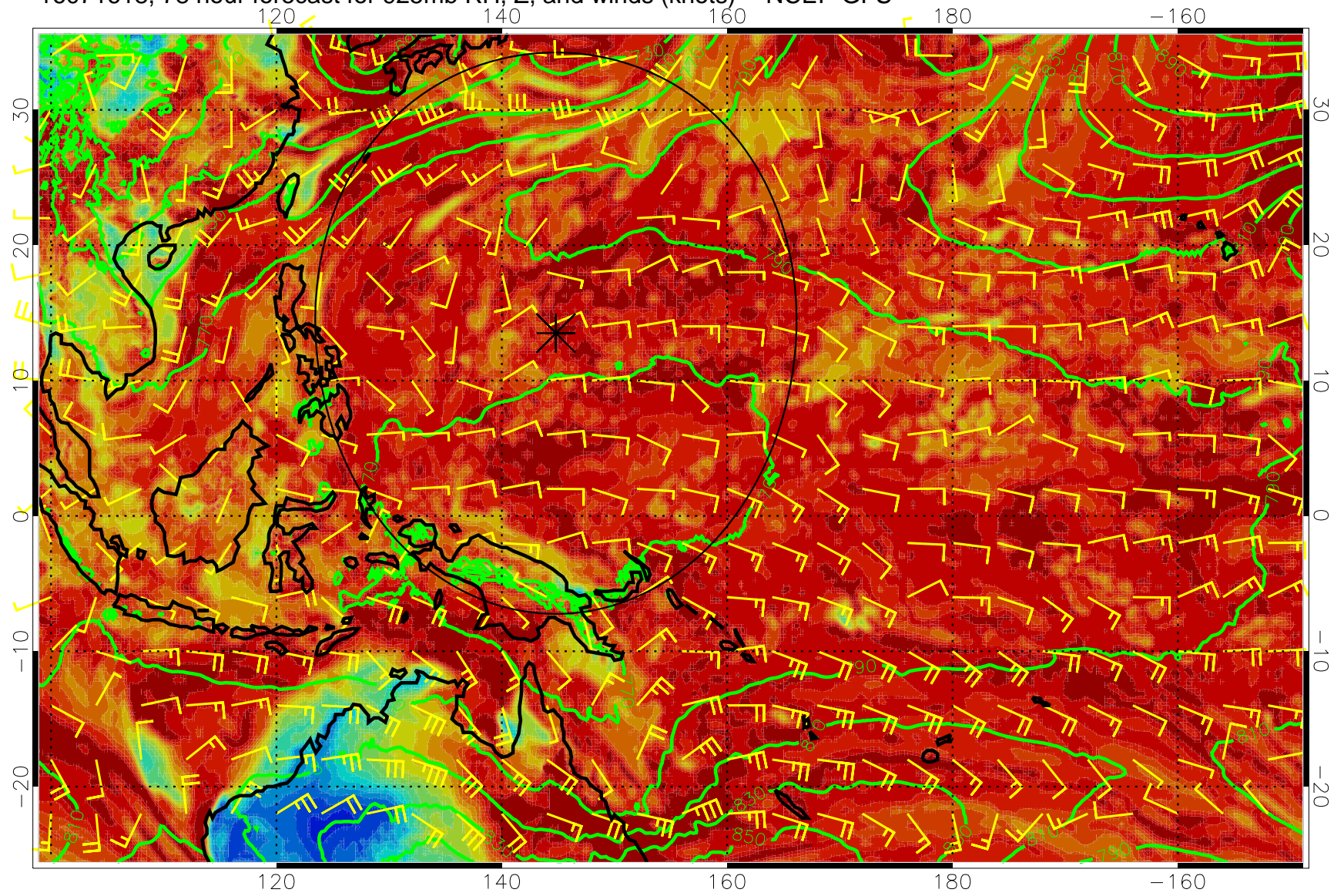
16071618, 78 hour forecast for 925mb RH, Z, and winds (knots) -- NCEP GFS
