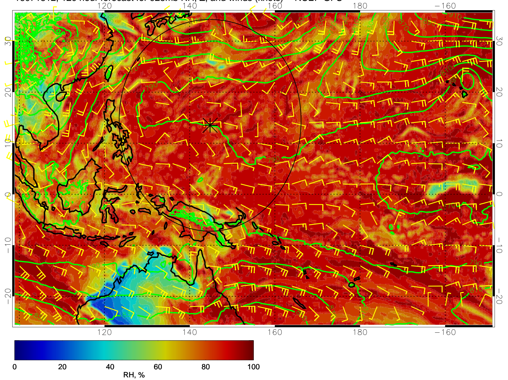
16071812, 120 hour forecast for 925mb RH, Z, and winds (knots) -- NCEP GFS
