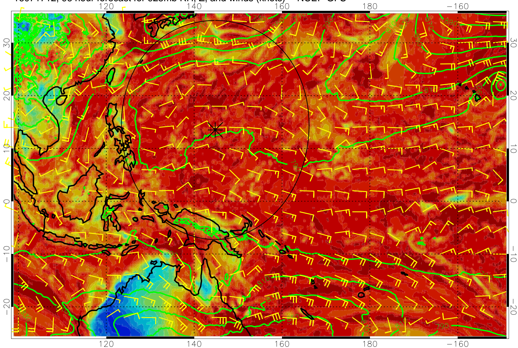
16071712, 96 hour forecast for 925mb RH, Z, and winds (knots) -- NCEP GFS
