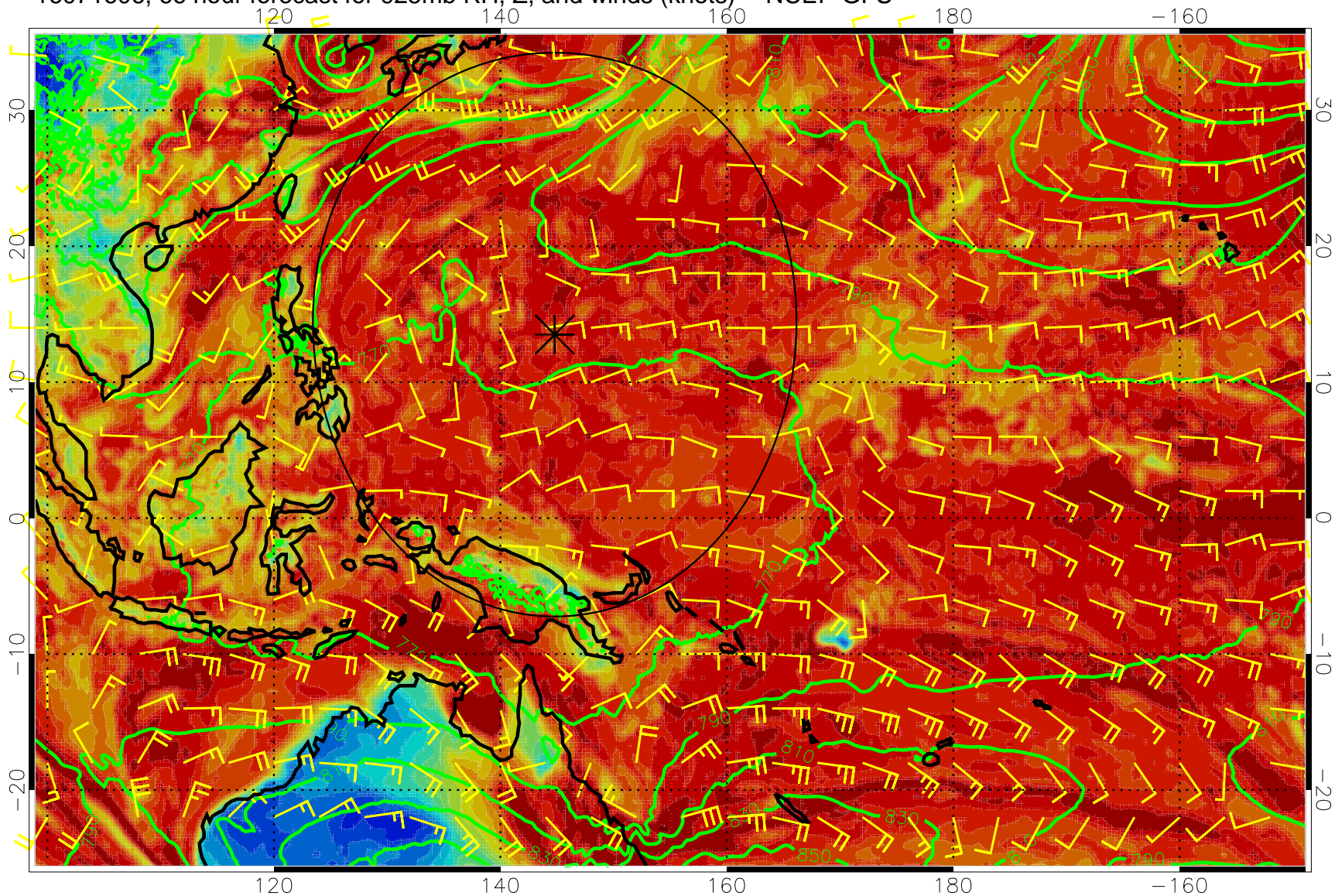
16071606, 66 hour forecast for 925mb RH, Z, and winds (knots) -- NCEP GFS
