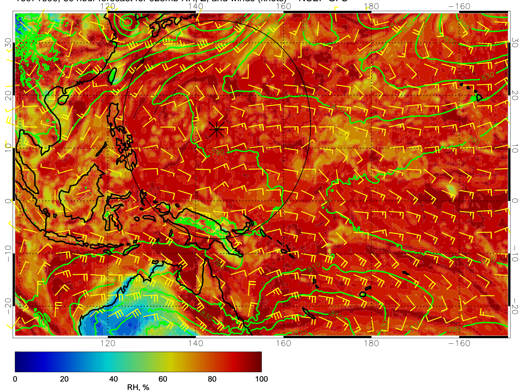
16071600, 60 hour forecast for 925mb RH, Z, and winds (knots) -- NCEP GFS
