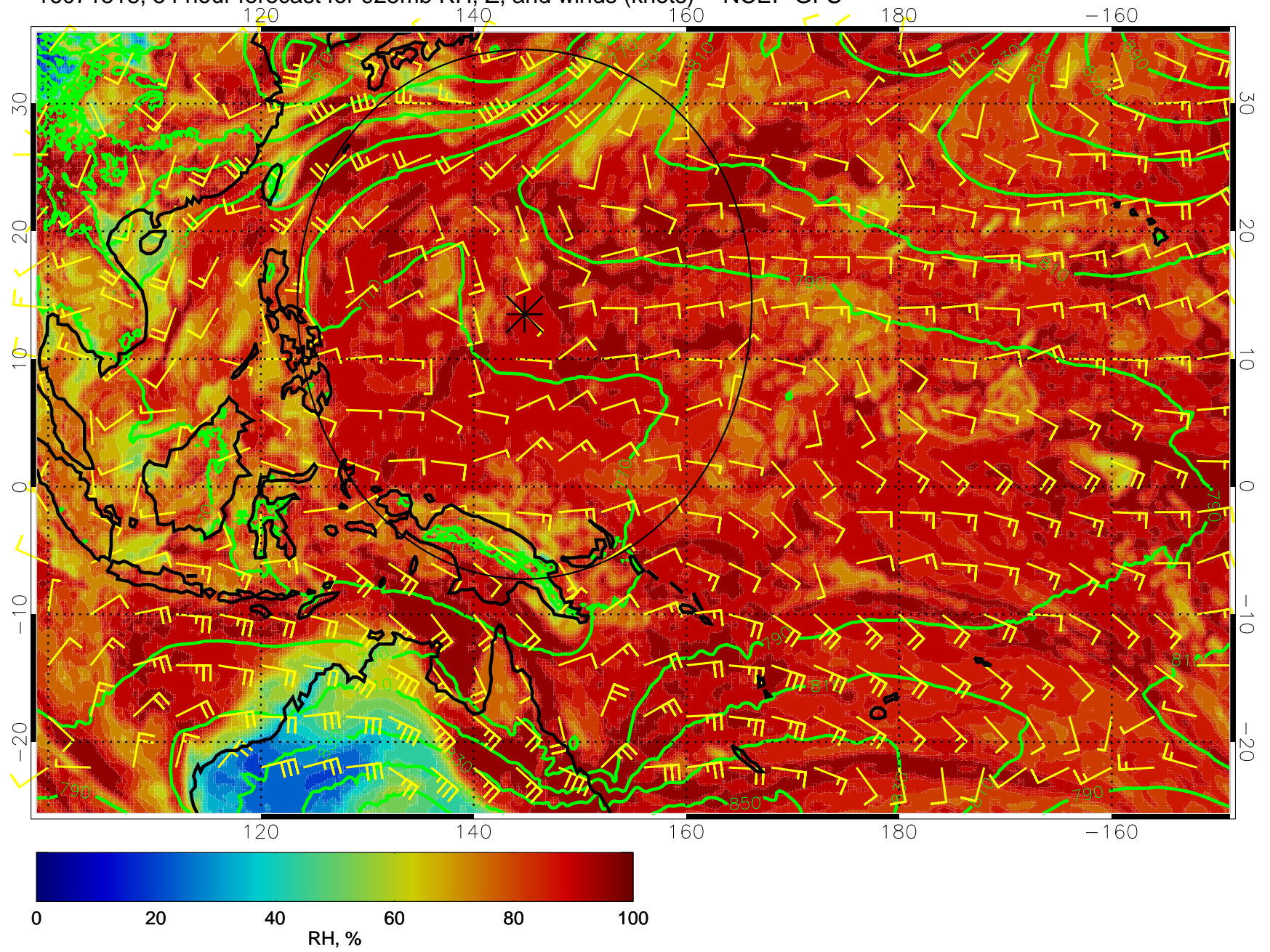
16071518, 54 hour forecast for 925mb RH, Z, and winds (knots) -- NCEP GFS
