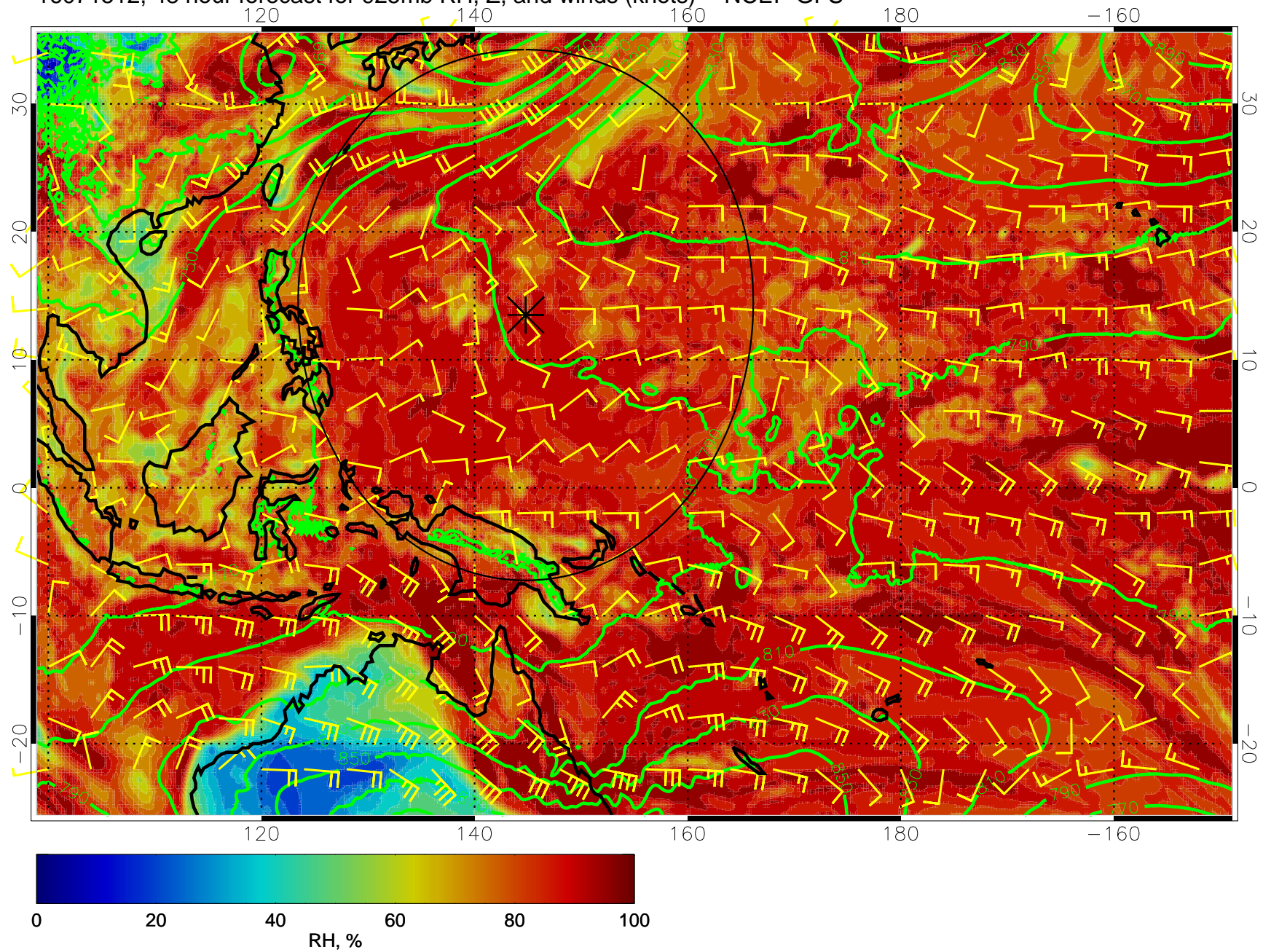
16071512, 48 hour forecast for 925mb RH, Z, and winds (knots) -- NCEP GFS
