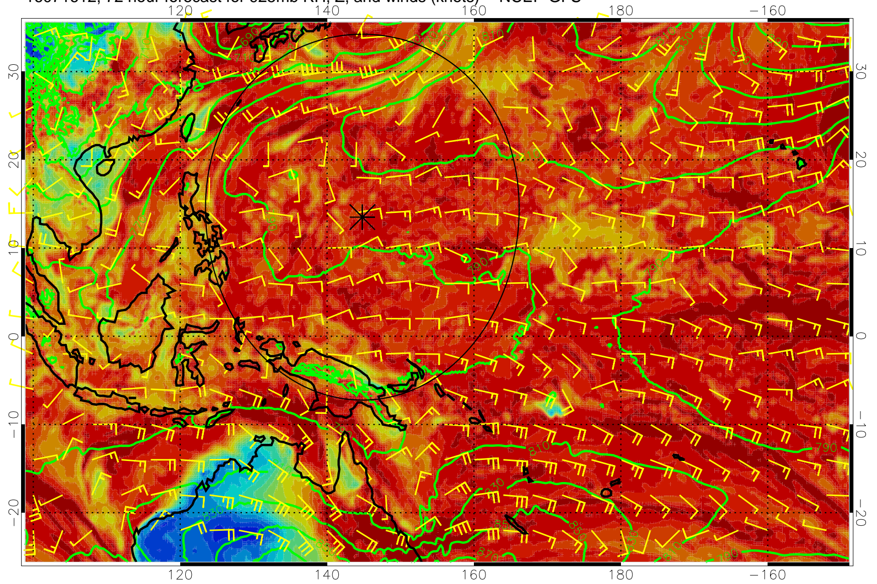
16071612, 72 hour forecast for 925mb RH, Z, and winds (knots) -- NCEP GFS
