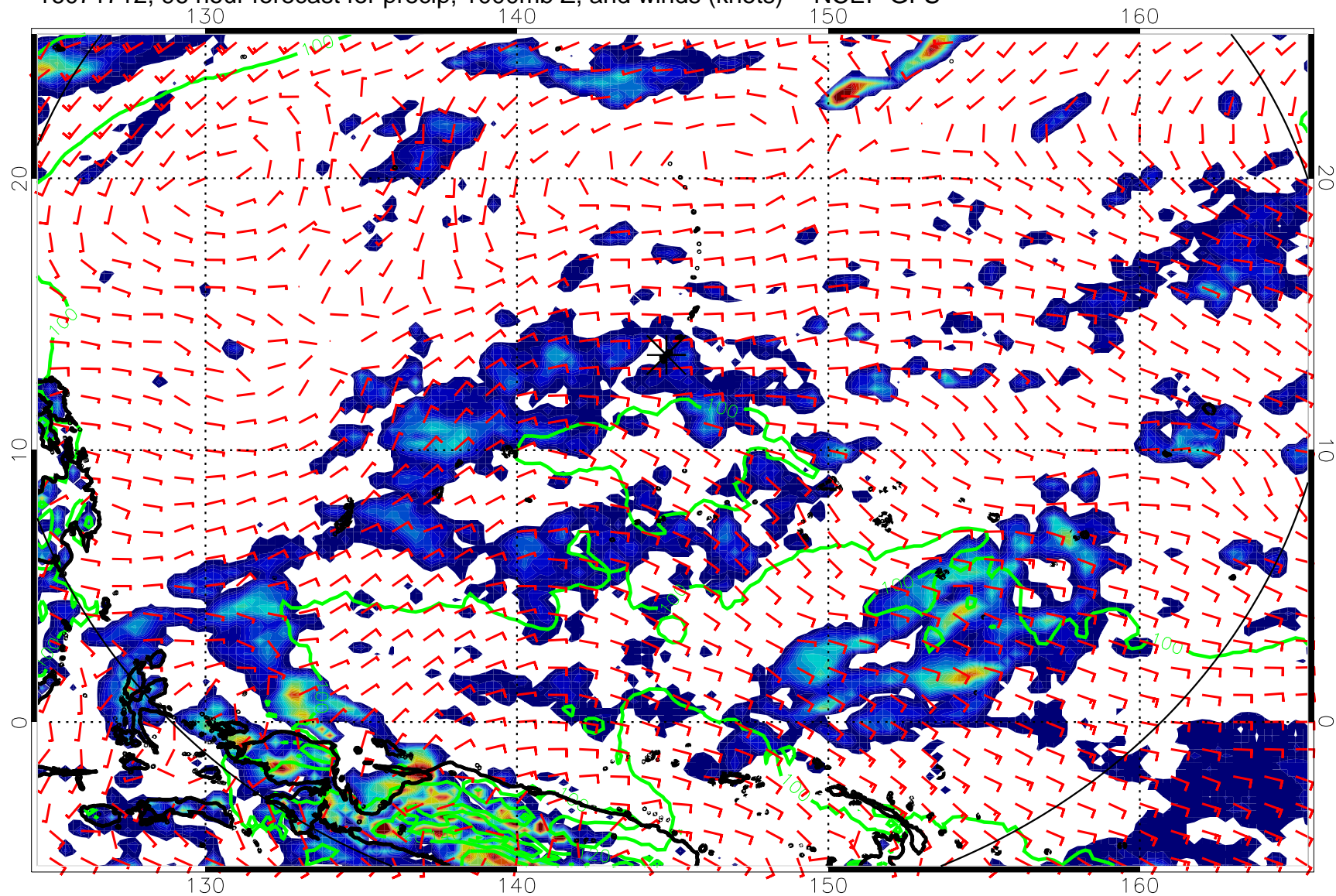
16071712, 96 hour forecast for precip, 1000mb Z, and winds (knots) -- NCEP GFS
