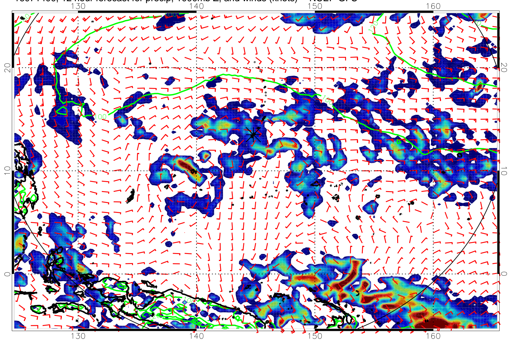
16071400, 12 hour forecast for precip, 1000mb Z, and winds (knots) -- NCEP GFS
