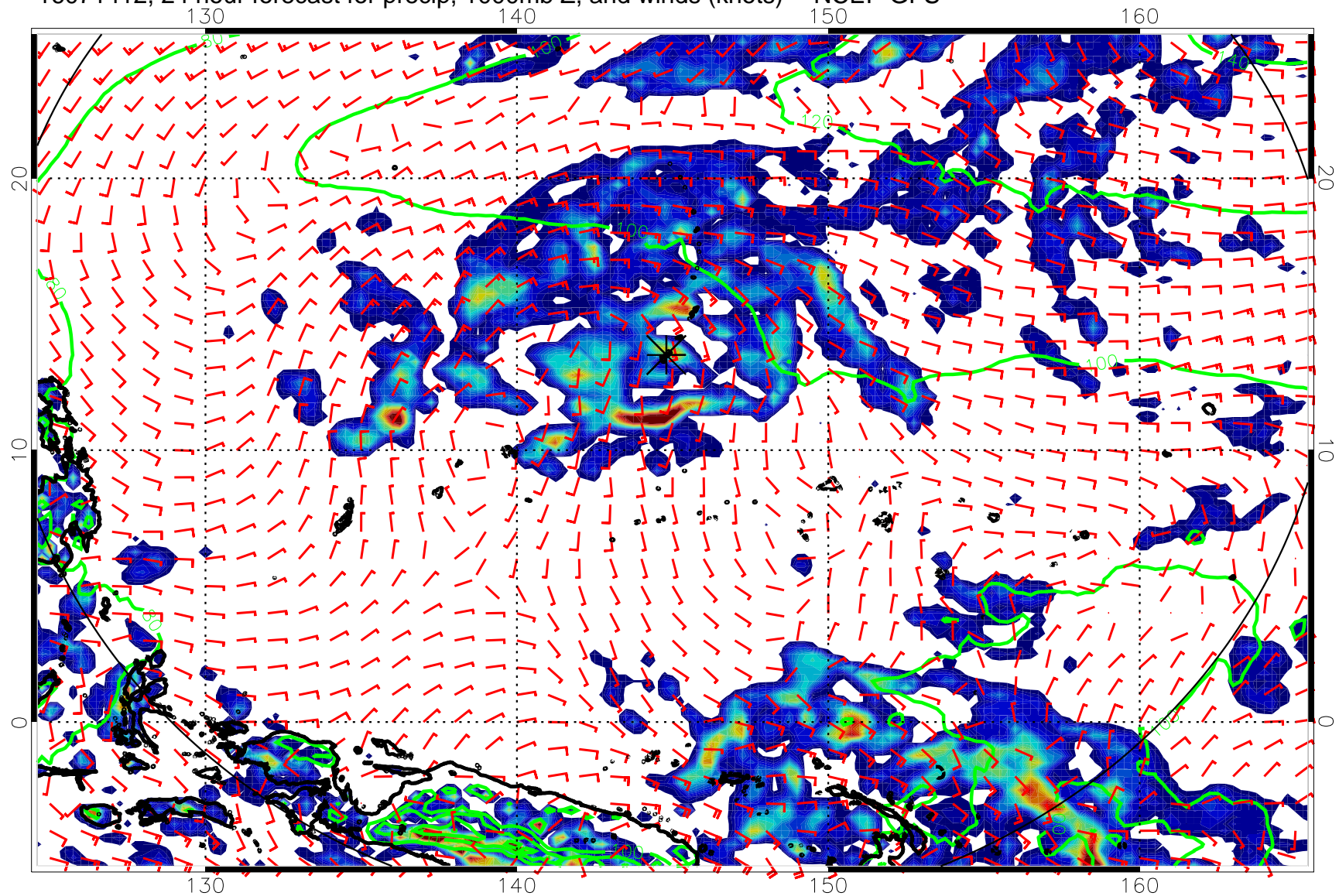
16071412, 24 hour forecast for precip, 1000mb Z, and winds (knots) -- NCEP GFS
