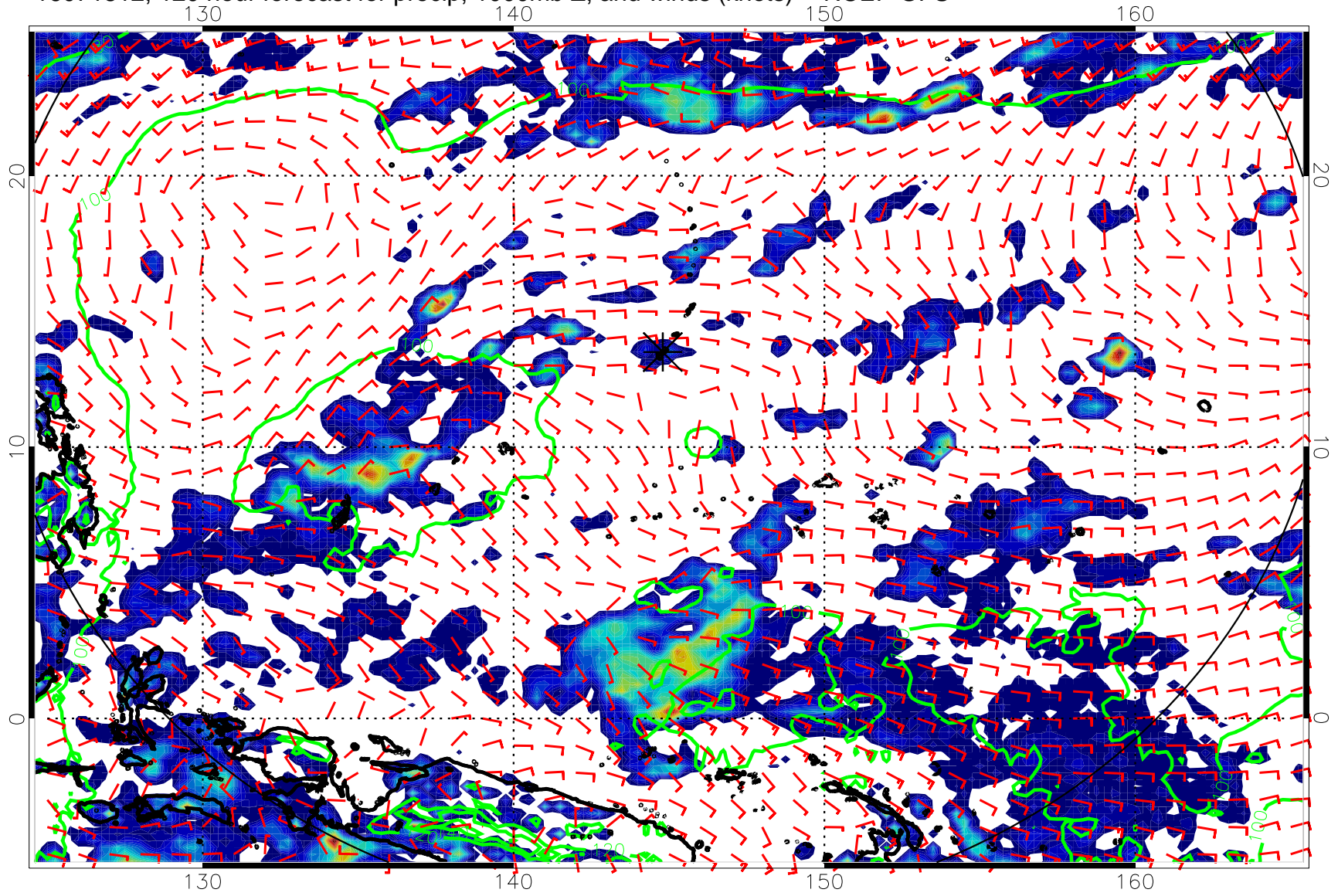
16071812, 120 hour forecast for precip, 1000mb Z, and winds (knots) -- NCEP GFS
