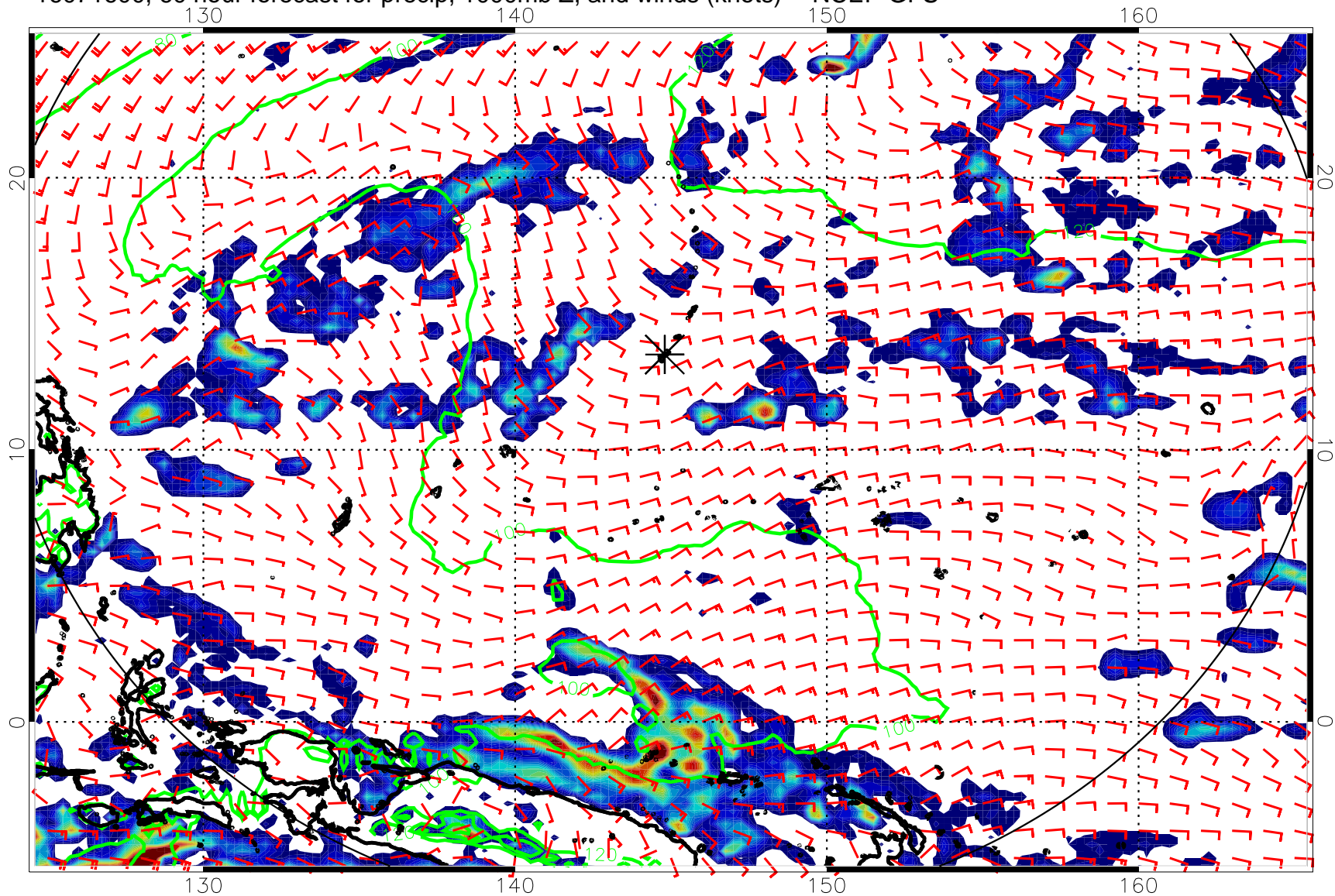
16071600, 60 hour forecast for precip, 1000mb Z, and winds (knots) -- NCEP GFS
