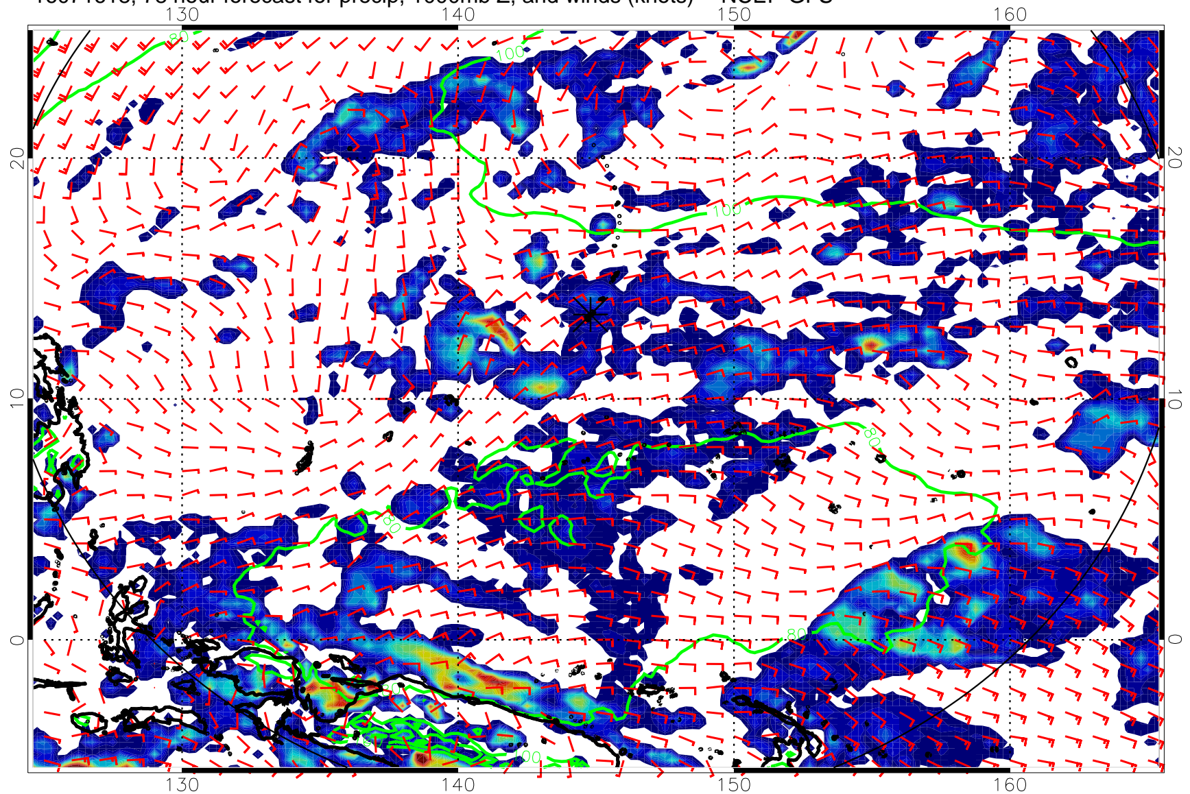
16071618, 78 hour forecast for precip, 1000mb Z, and winds (knots) -- NCEP GFS
