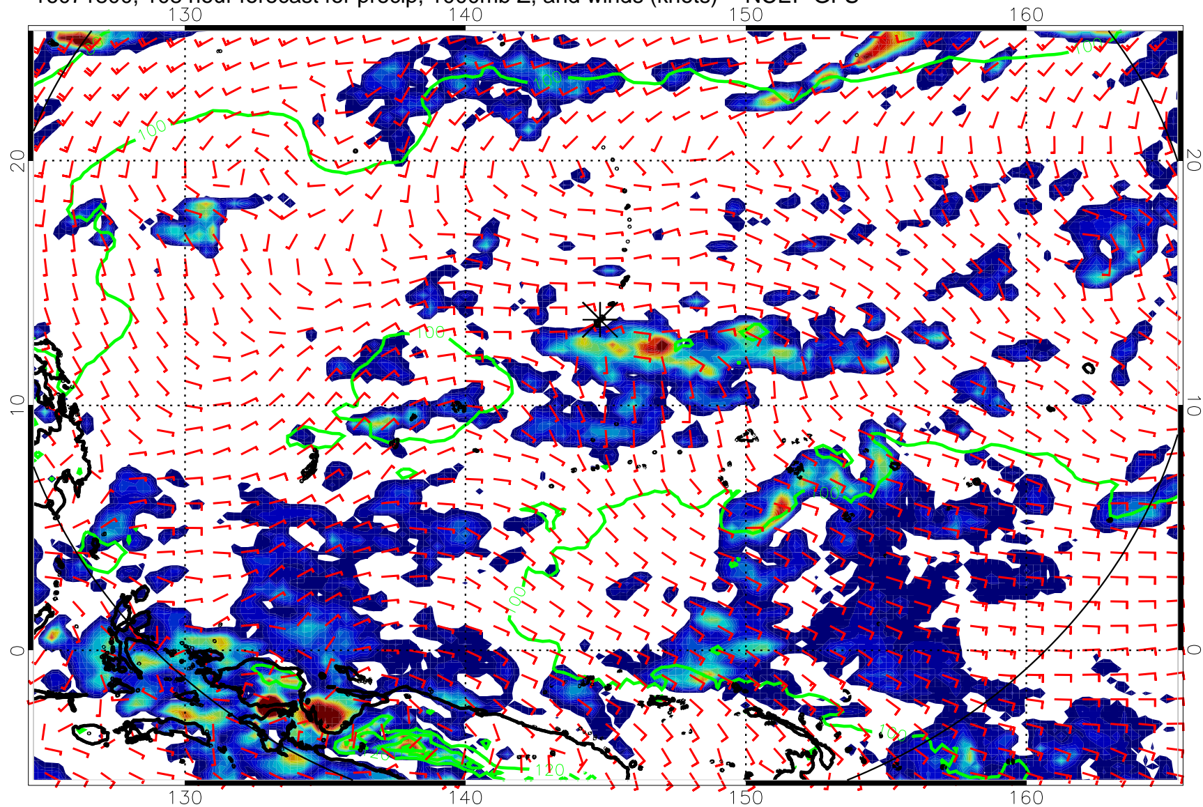
16071800, 108 hour forecast for precip, 1000mb Z, and winds (knots) -- NCEP GFS
