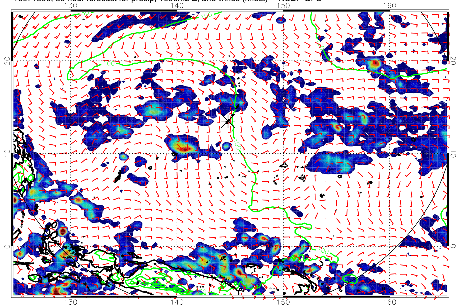
16071500, 36 hour forecast for precip, 1000mb Z, and winds (knots) -- NCEP GFS
