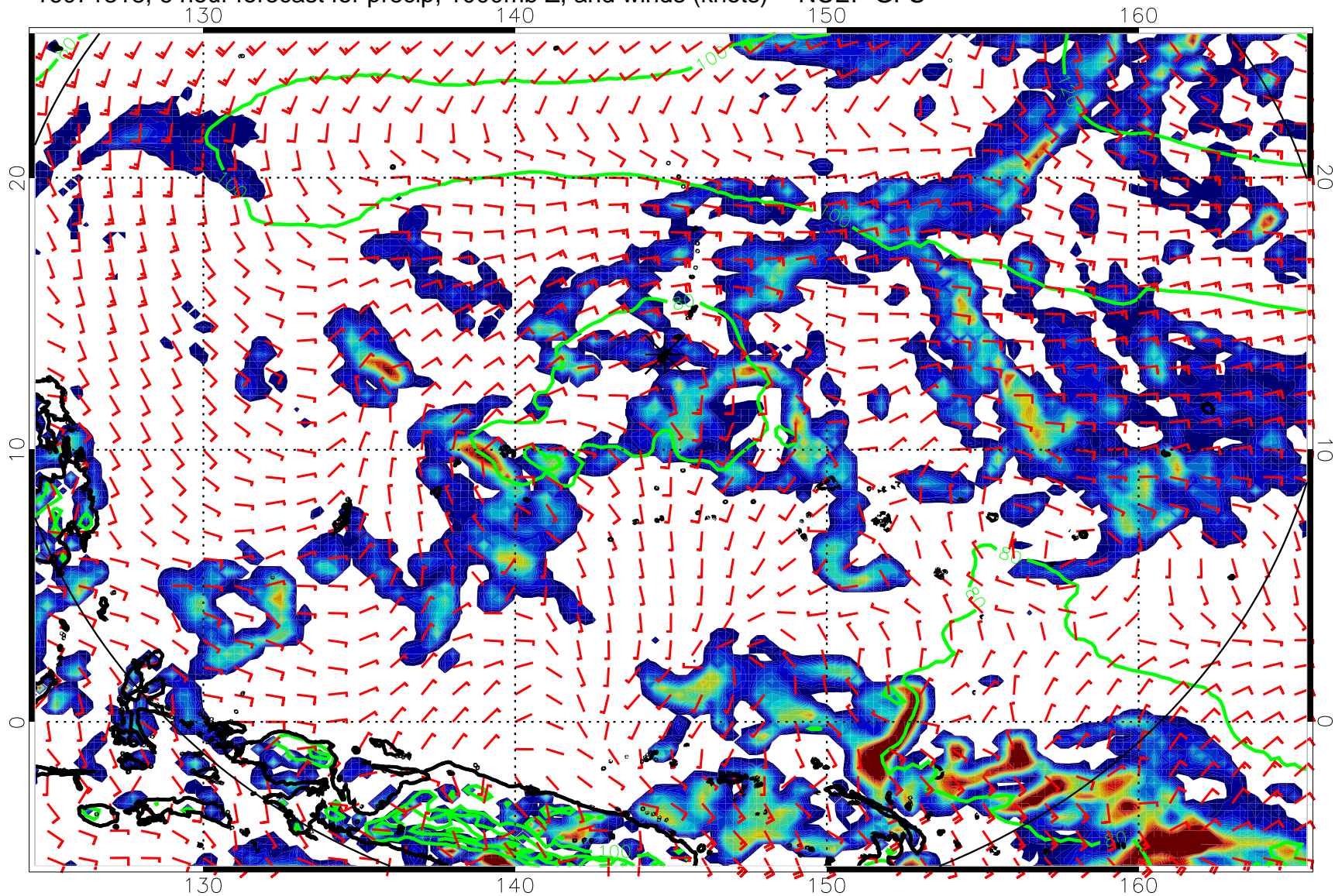
16071318, 6 hour forecast for precip, 1000mb Z, and winds (knots) -- NCEP GFS
