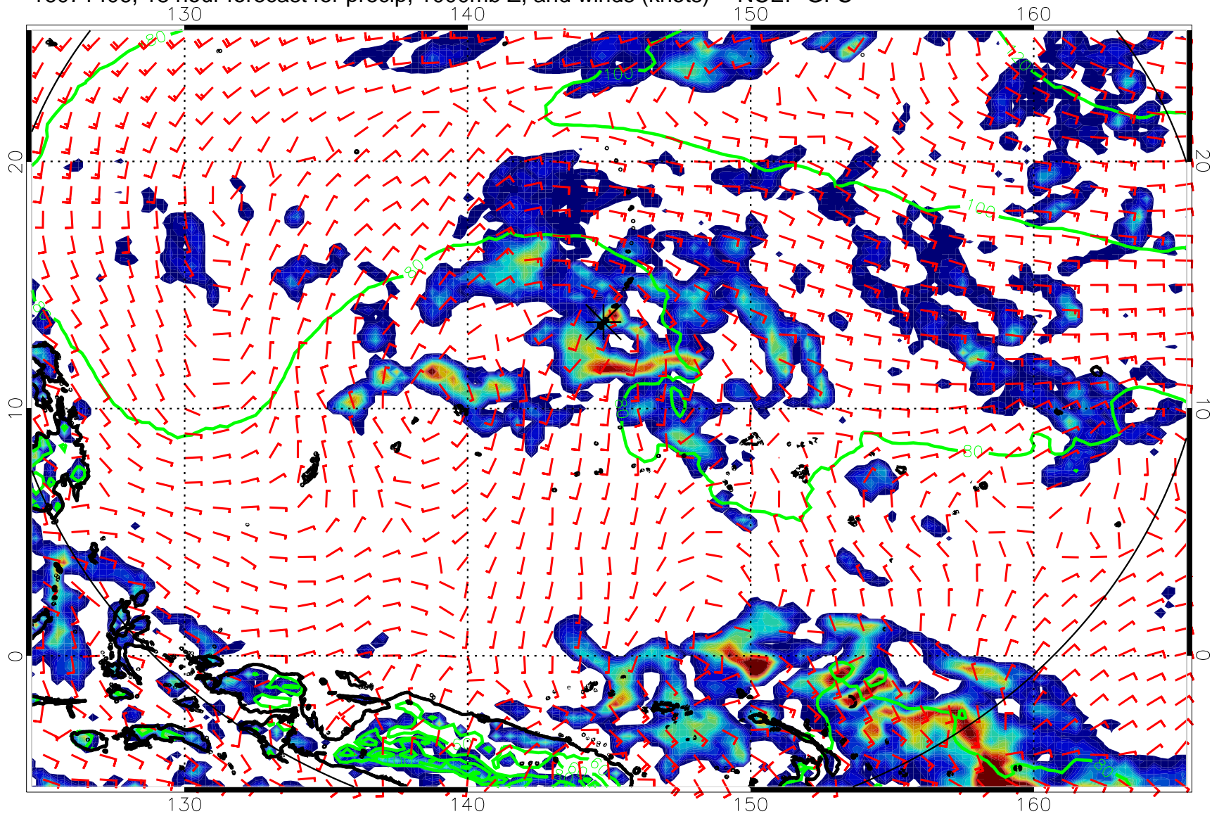
16071406, 18 hour forecast for precip, 1000mb Z, and winds (knots) -- NCEP GFS
