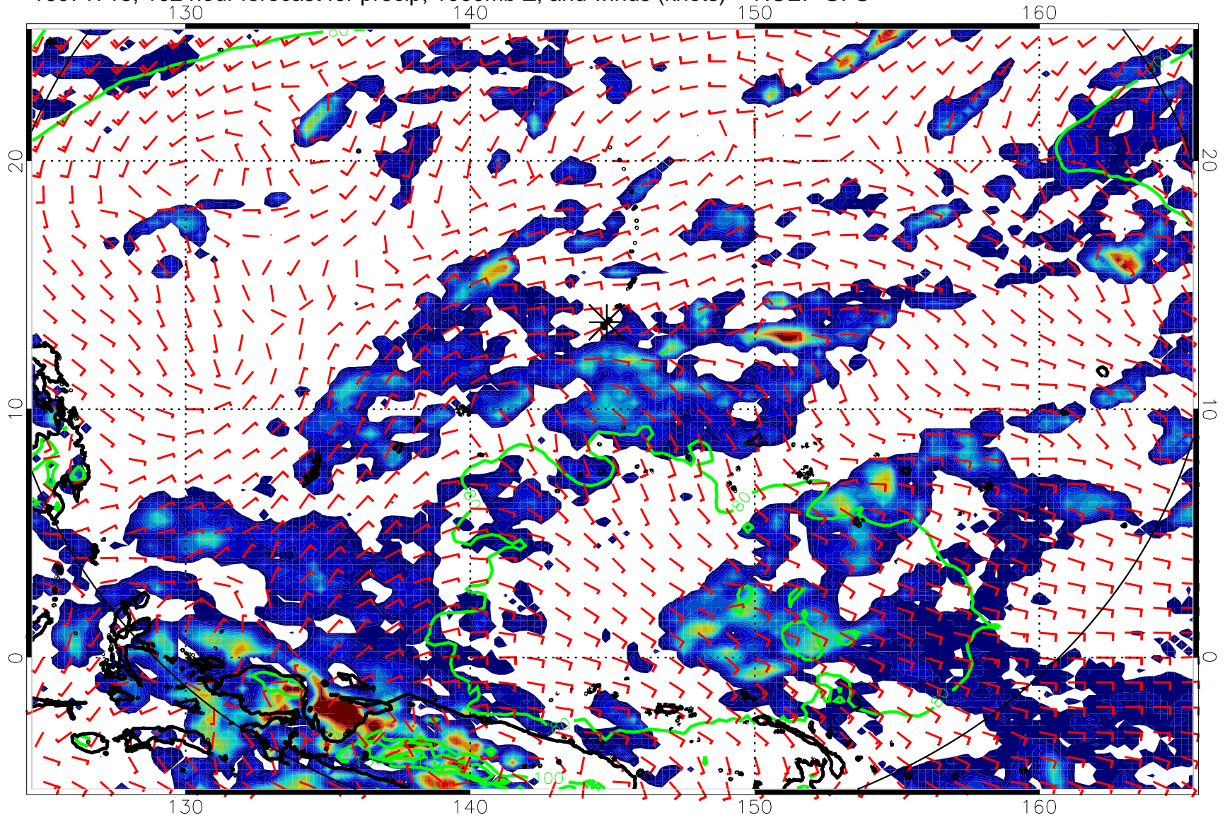
16071718, 102 hour forecast for precip, 1000mb Z, and winds (knots) -- NCEP GFS
