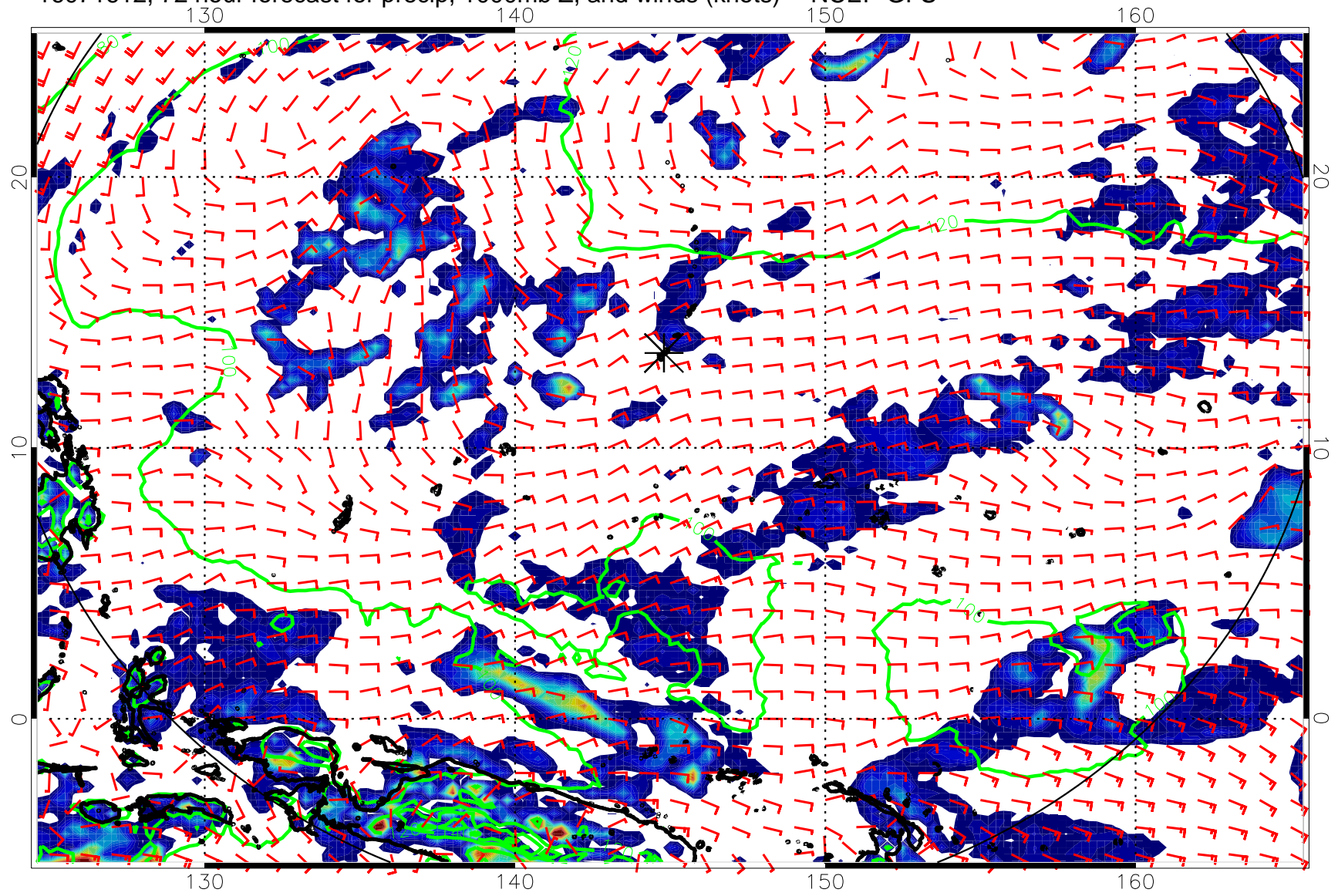
16071612, 72 hour forecast for precip, 1000mb Z, and winds (knots) -- NCEP GFS
