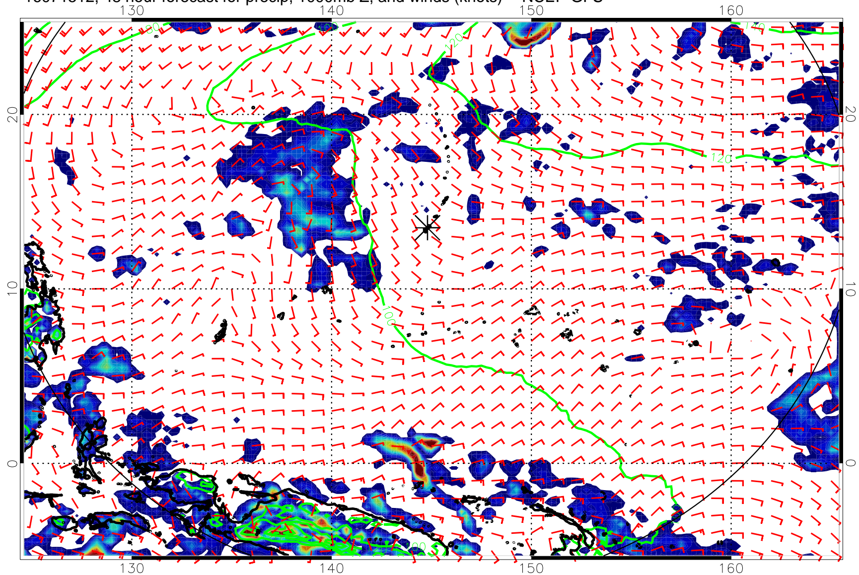
16071512, 48 hour forecast for precip, 1000mb Z, and winds (knots) -- NCEP GFS
