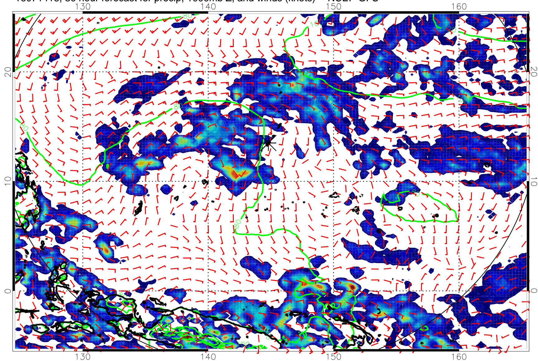
16071418, 30 hour forecast for precip, 1000mb Z, and winds (knots) -- NCEP GFS
