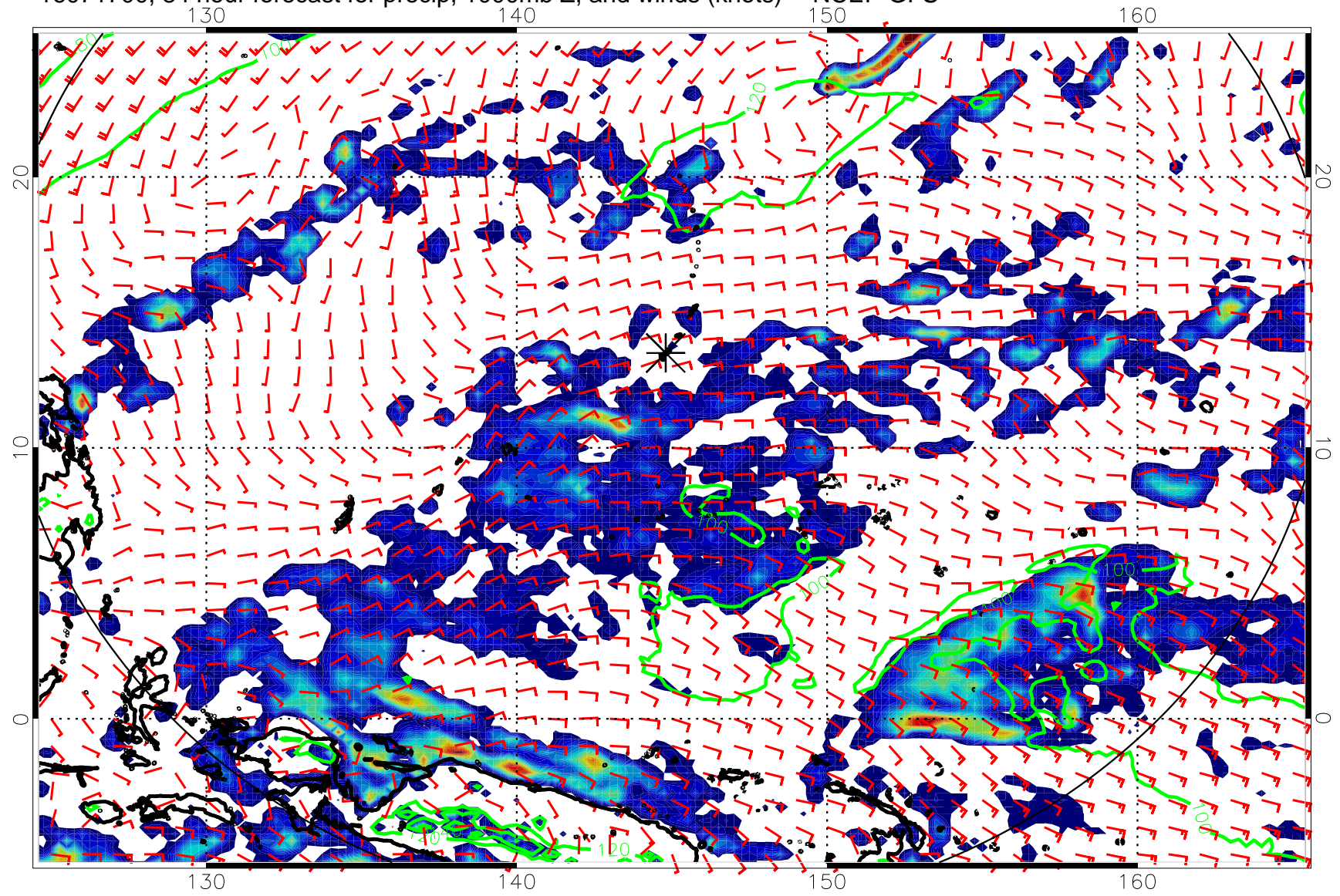
16071700, 84 hour forecast for precip, 1000mb Z, and winds (knots) -- NCEP GFS
