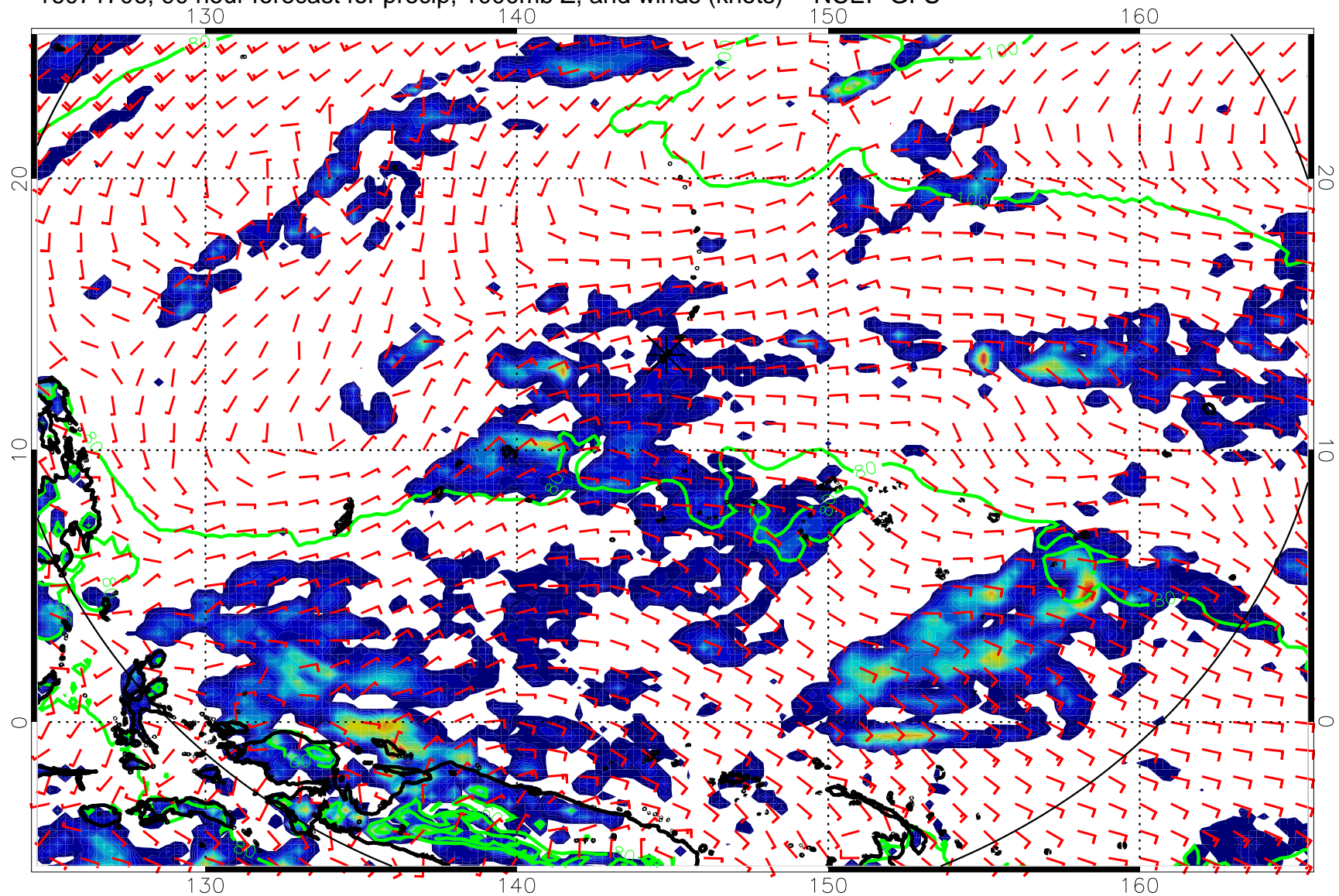
16071706, 90 hour forecast for precip, 1000mb Z, and winds (knots) -- NCEP GFS
