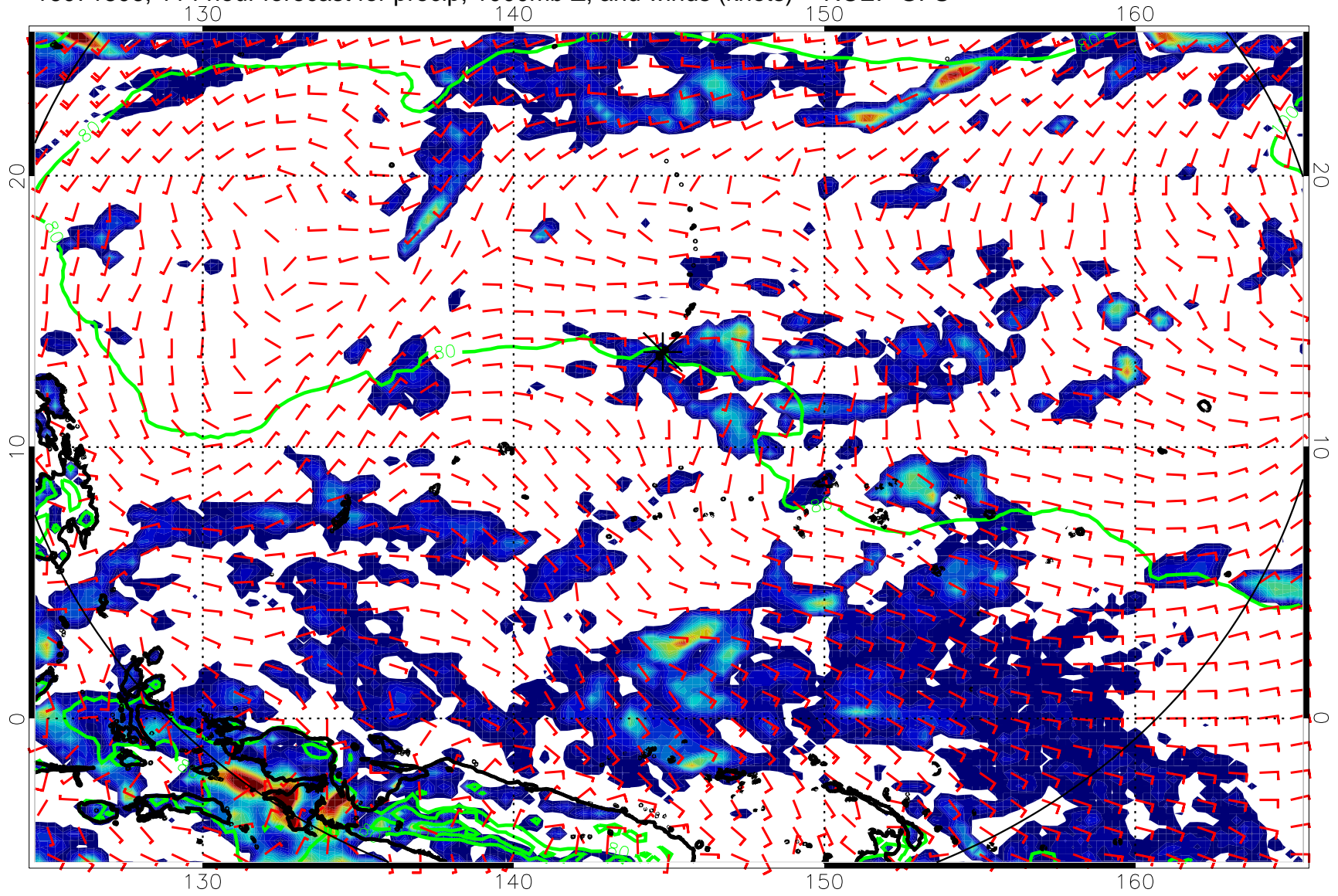
16071806, 114 hour forecast for precip, 1000mb Z, and winds (knots) -- NCEP GFS
