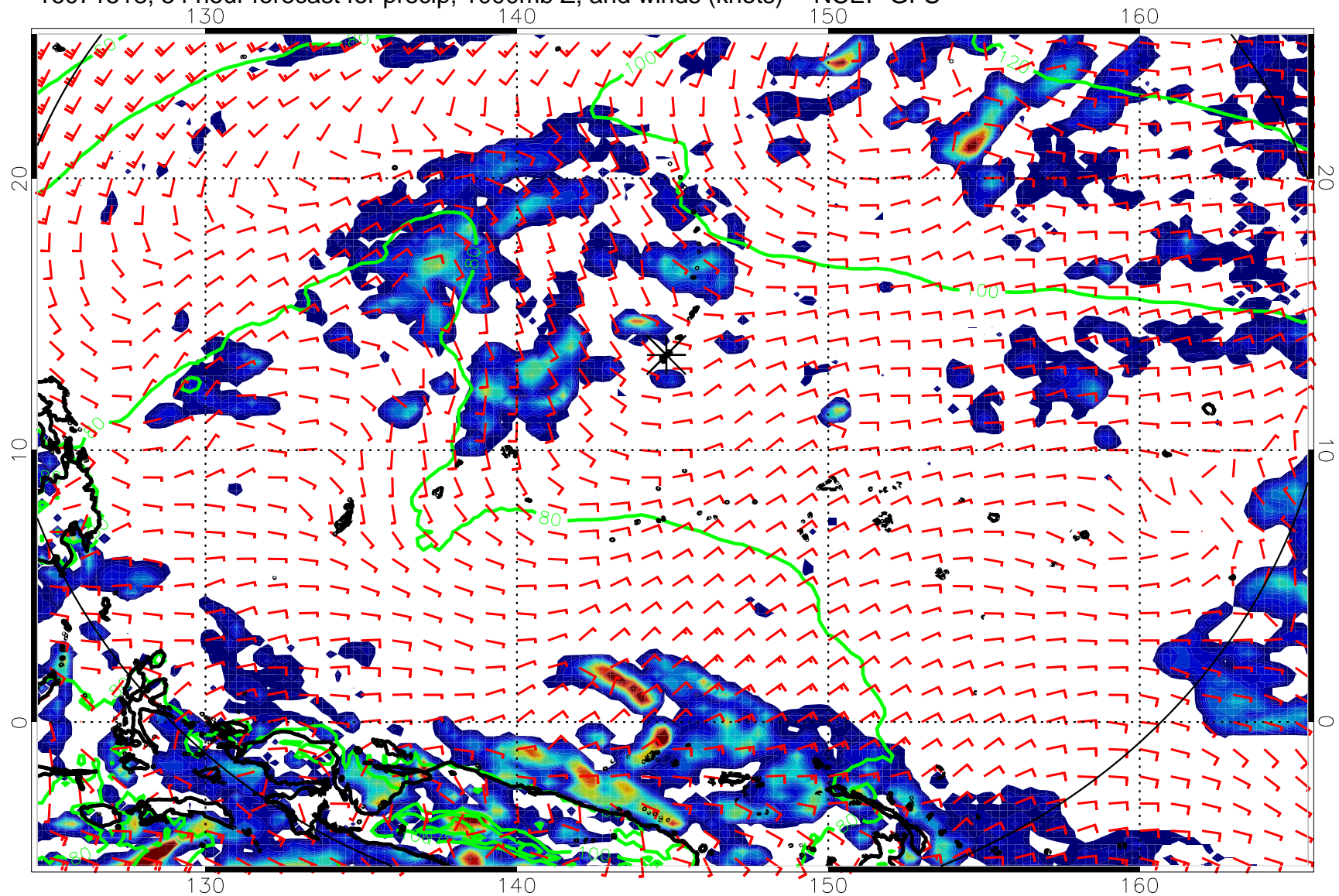
16071518, 54 hour forecast for precip, 1000mb Z, and winds (knots) -- NCEP GFS
