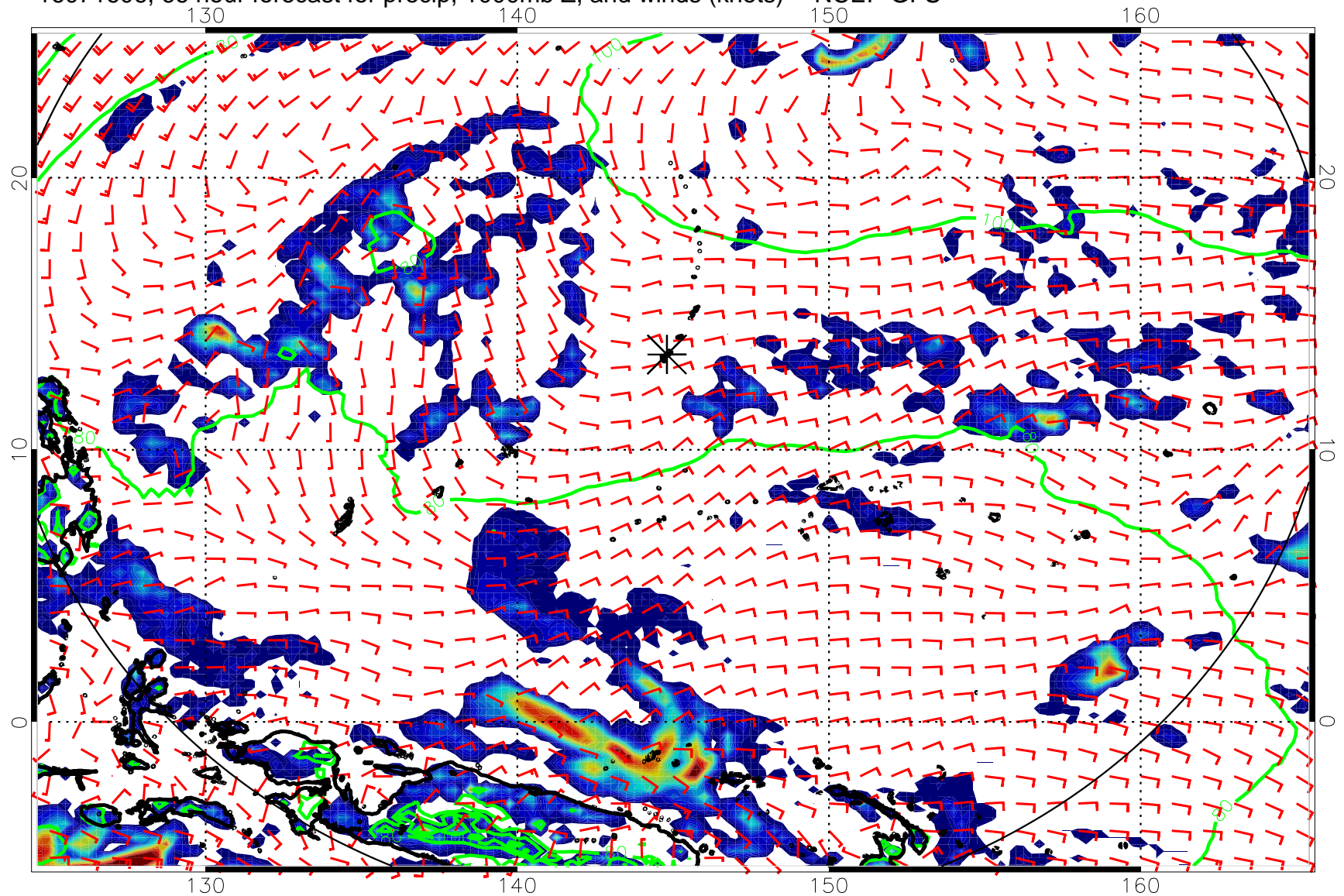
16071606, 66 hour forecast for precip, 1000mb Z, and winds (knots) -- NCEP GFS
