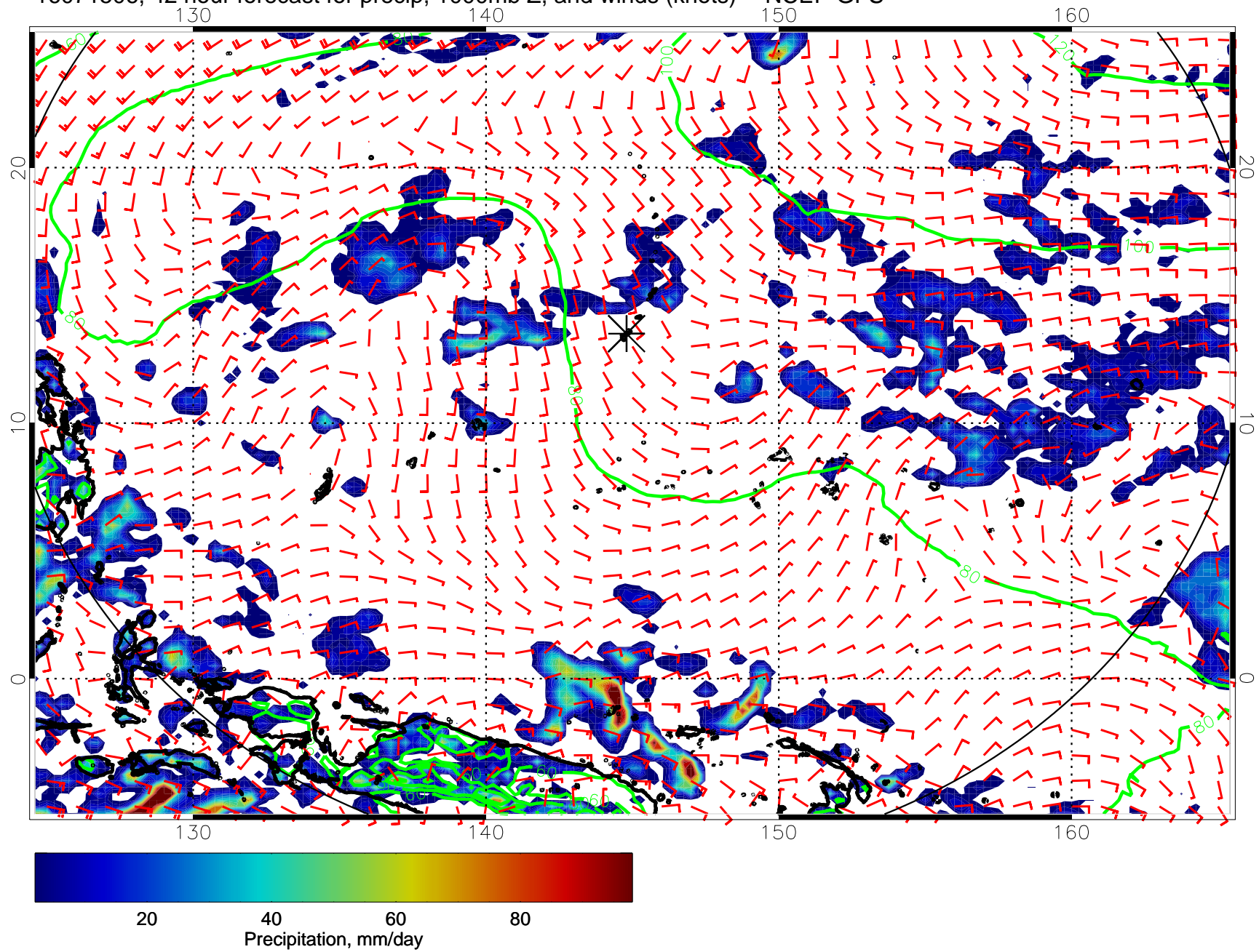
16071506, 42 hour forecast for precip, 1000mb Z, and winds (knots) -- NCEP GFS
