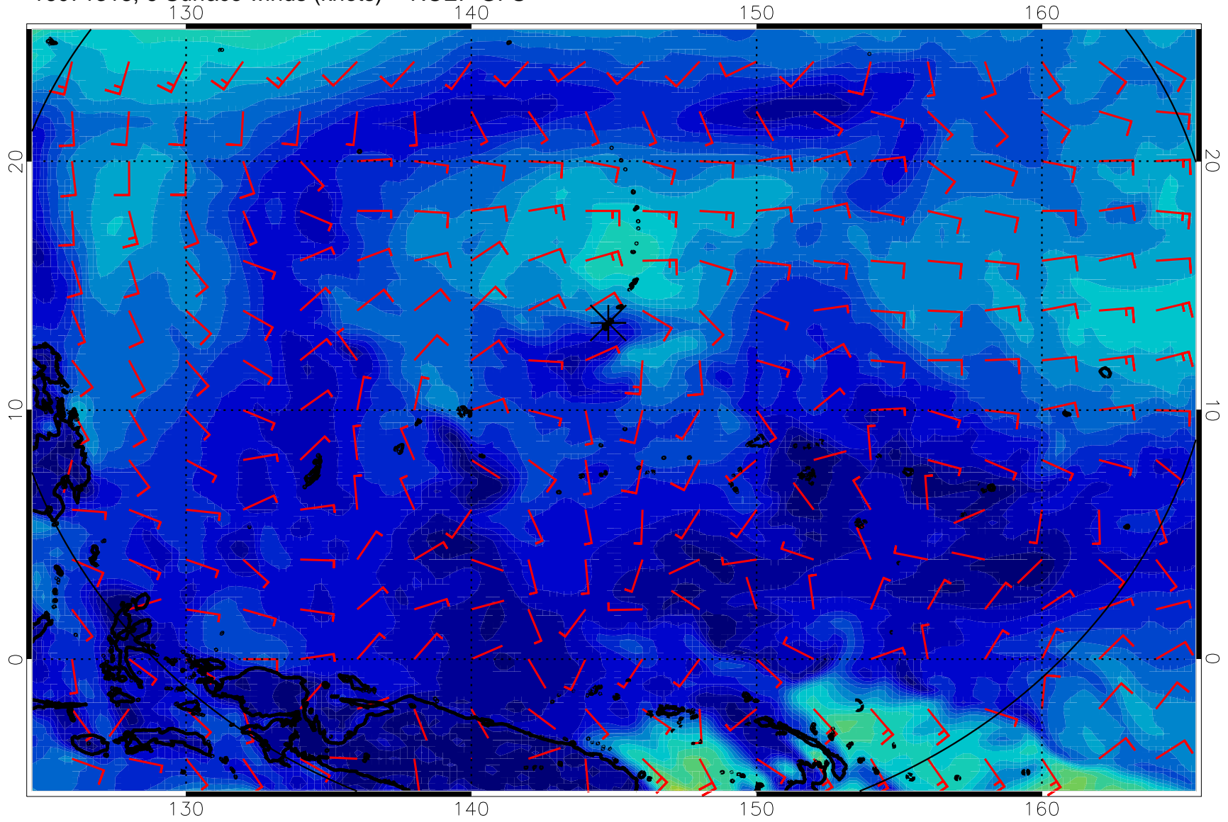
16071318, 6 Surface winds (knots) -- NCEP GFS
