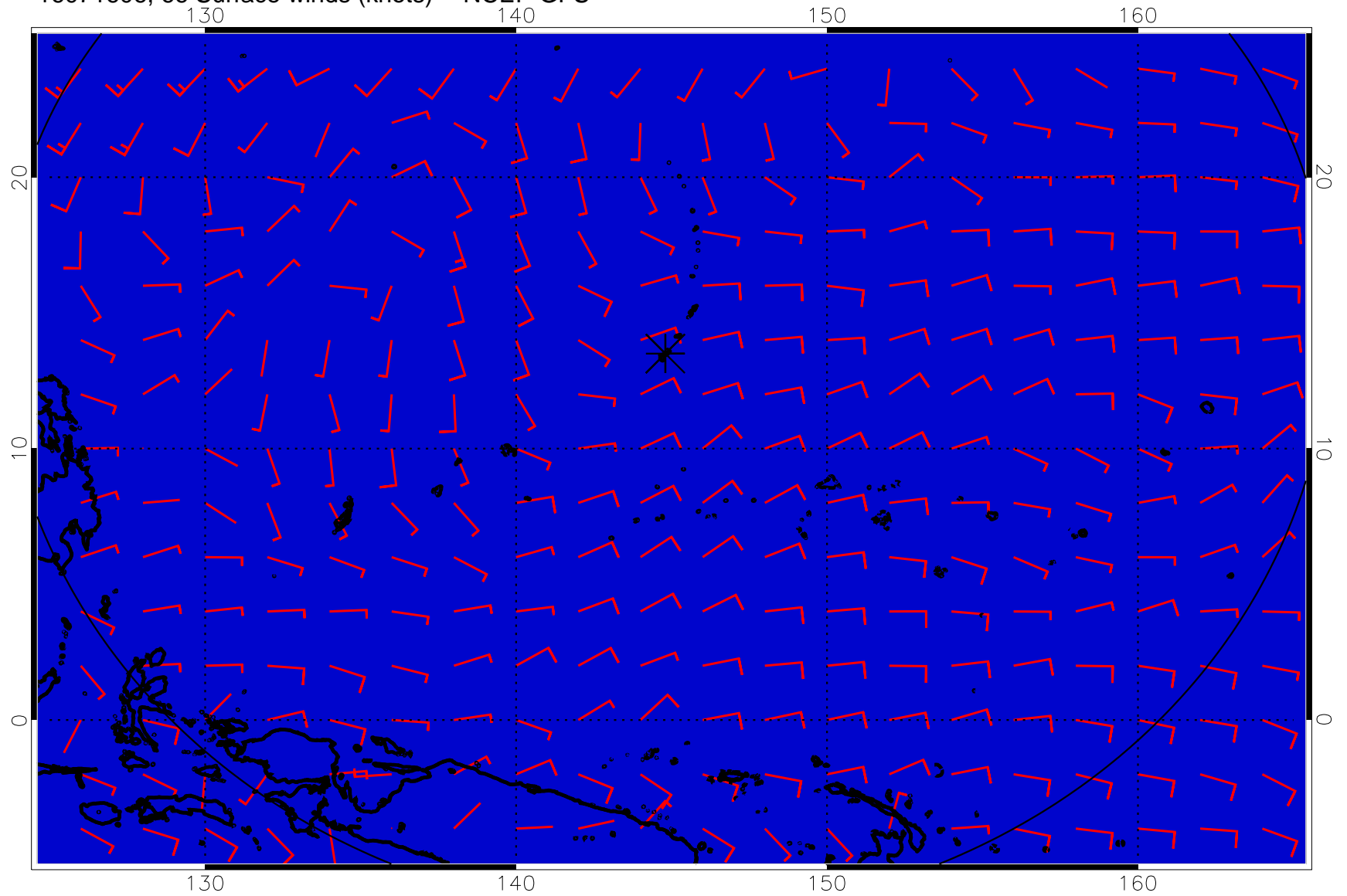
16071606, 66 Surface winds (knots) -- NCEP GFS
