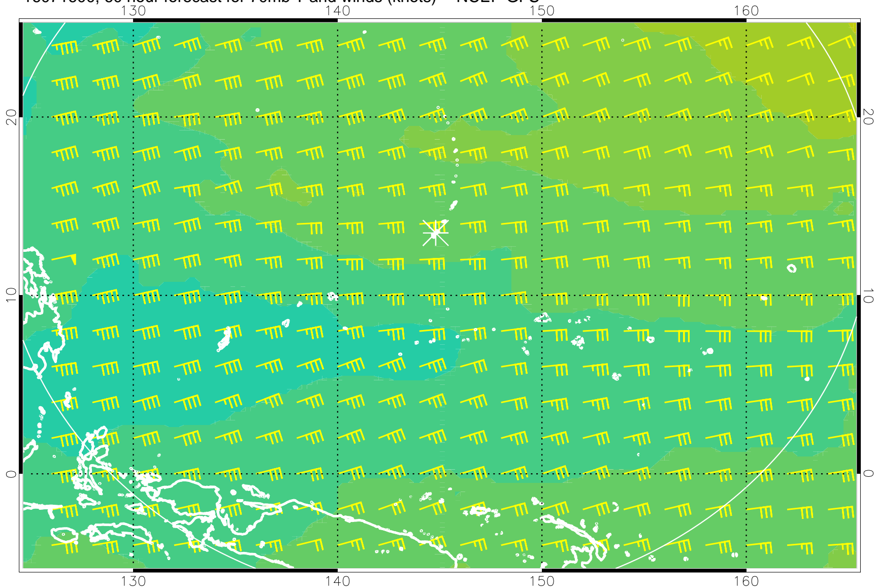
16071600, 60 hour forecast for 70mb T and winds (knots) -- NCEP GFS
