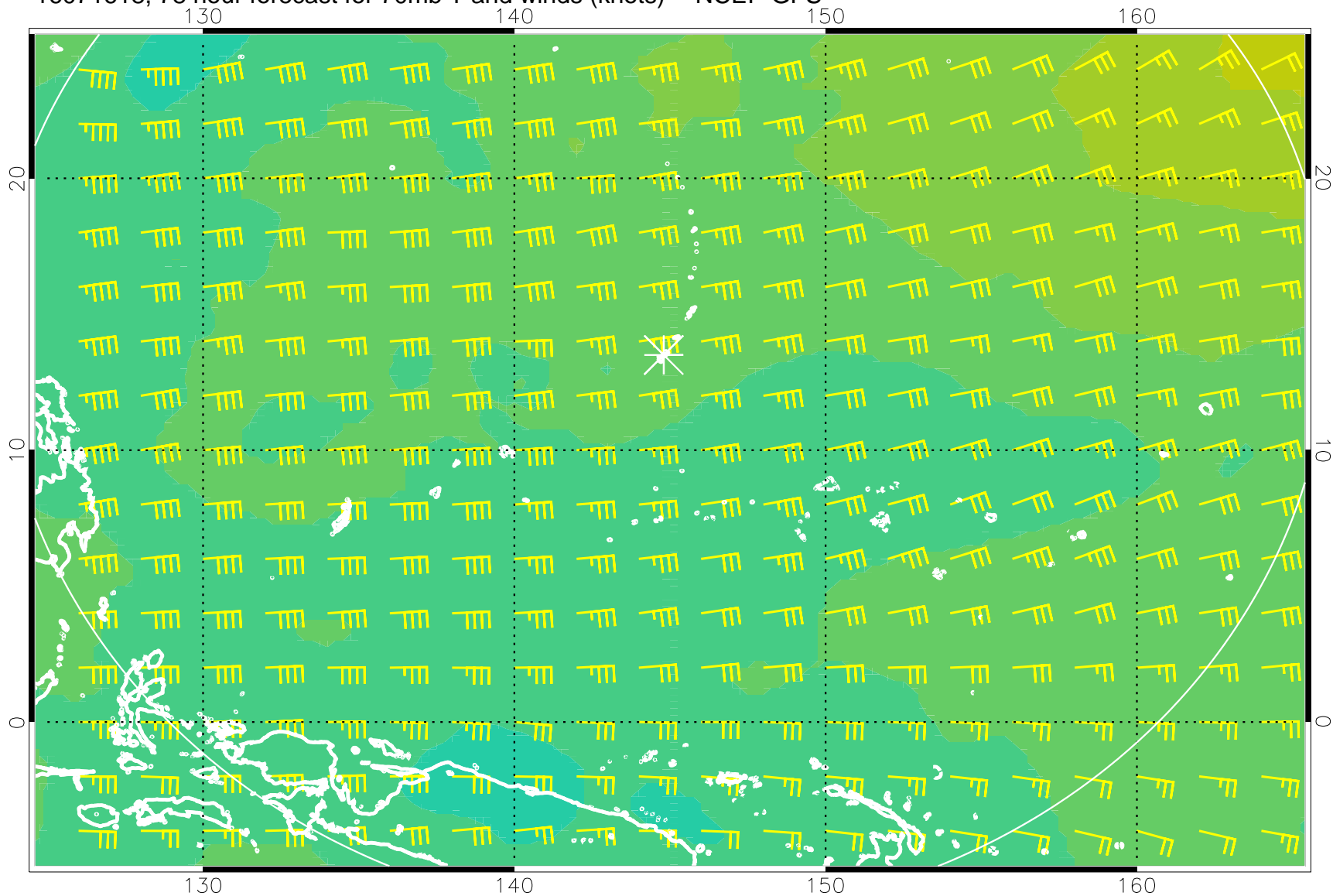
16071618, 78 hour forecast for 70mb T and winds (knots) -- NCEP GFS
