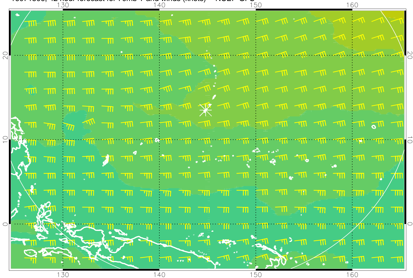
16071506, 42 hour forecast for 70mb T and winds (knots) -- NCEP GFS
