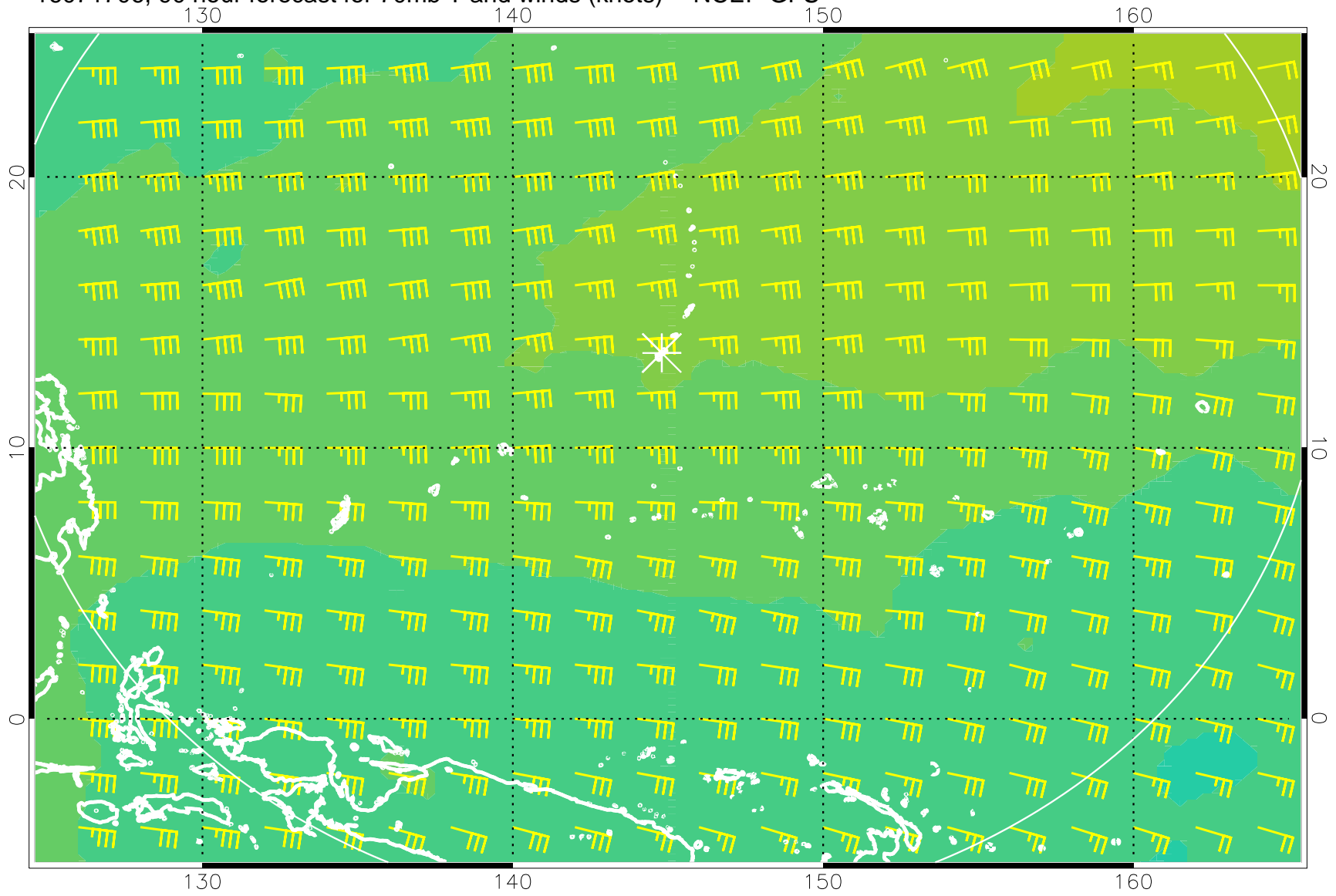
16071706, 90 hour forecast for 70mb T and winds (knots) -- NCEP GFS
