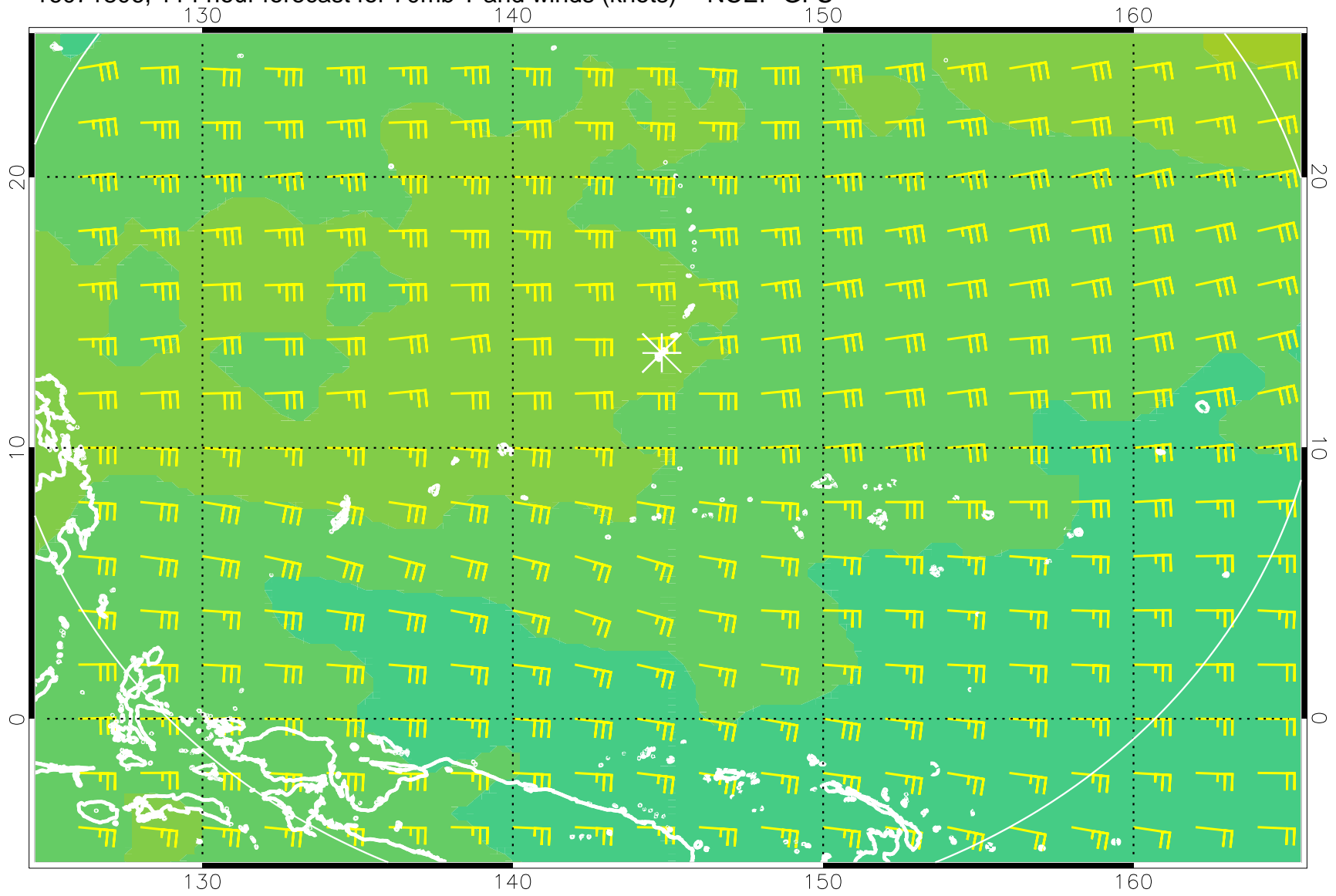
16071806, 114 hour forecast for 70mb T and winds (knots) -- NCEP GFS
