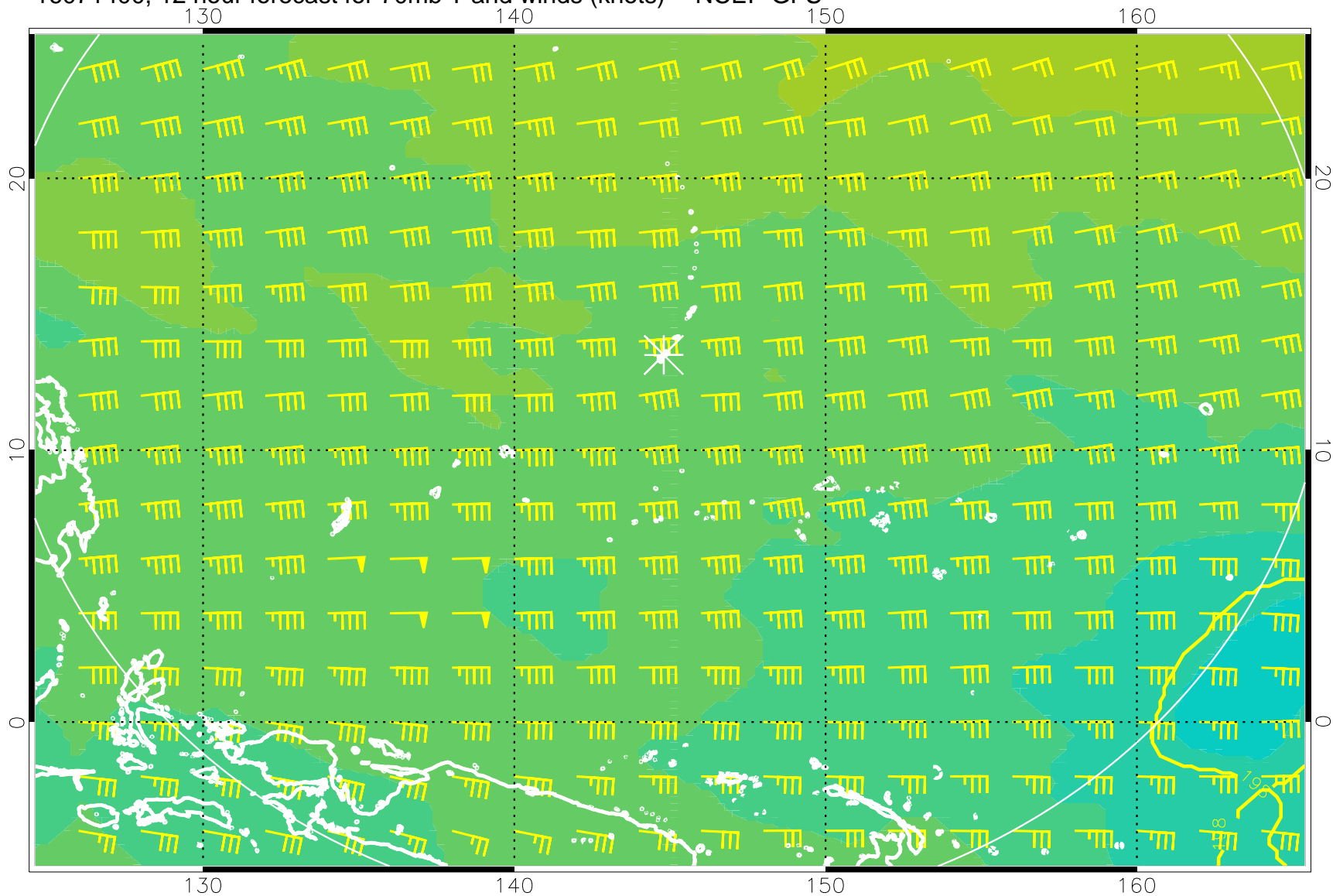
16071400, 12 hour forecast for 70mb T and winds (knots) -- NCEP GFS
