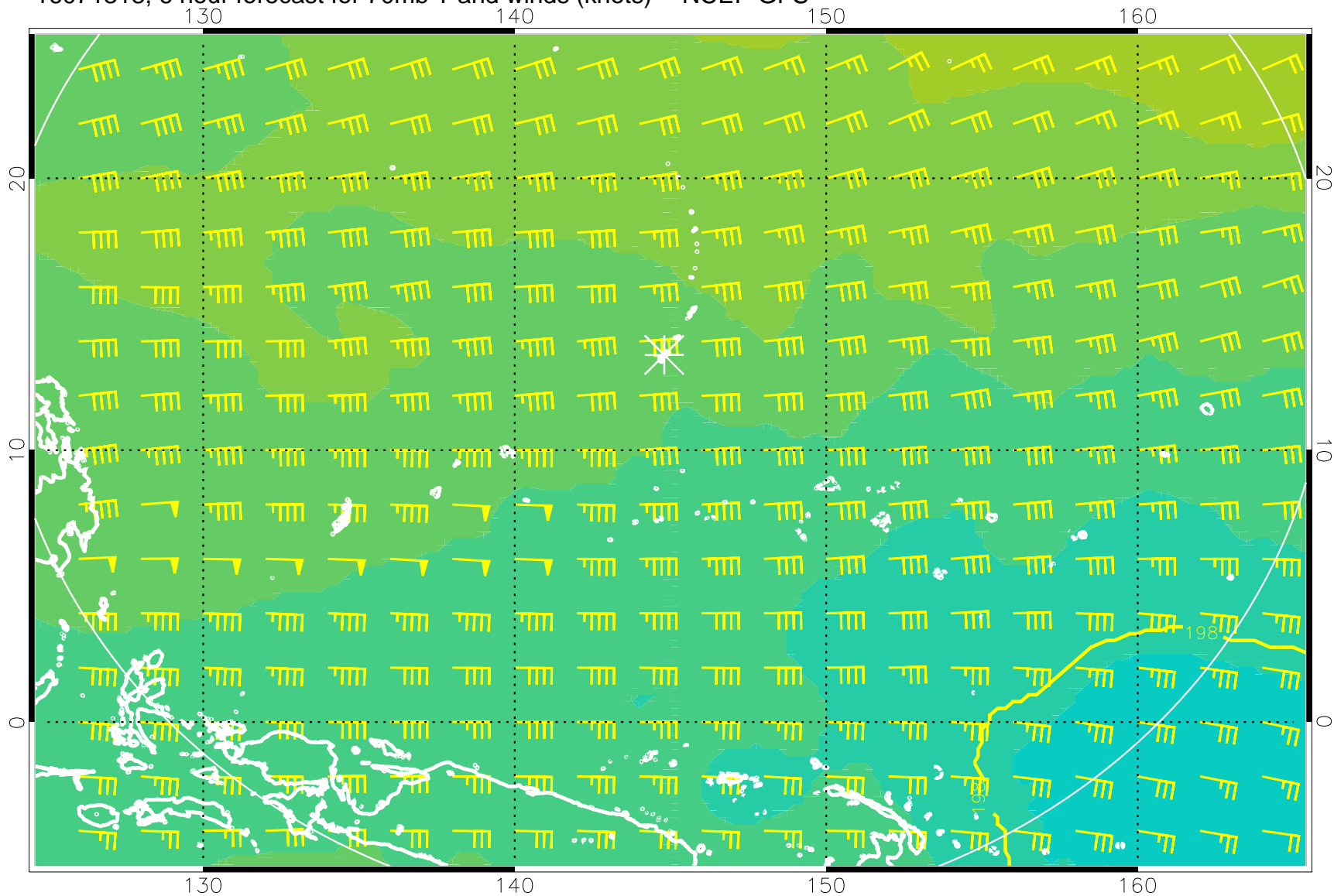
16071318, 6 hour forecast for 70mb T and winds (knots) -- NCEP GFS
