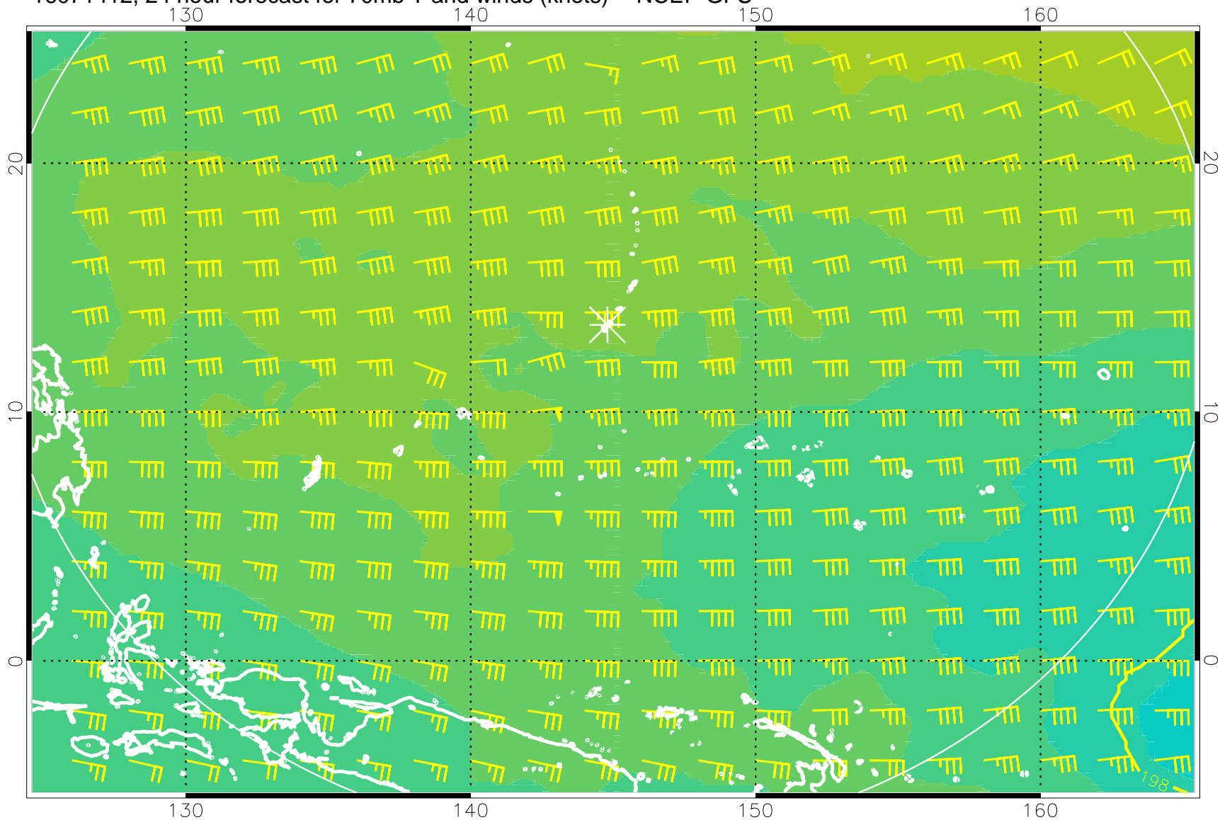
16071412, 24 hour forecast for 70mb T and winds (knots) -- NCEP GFS
