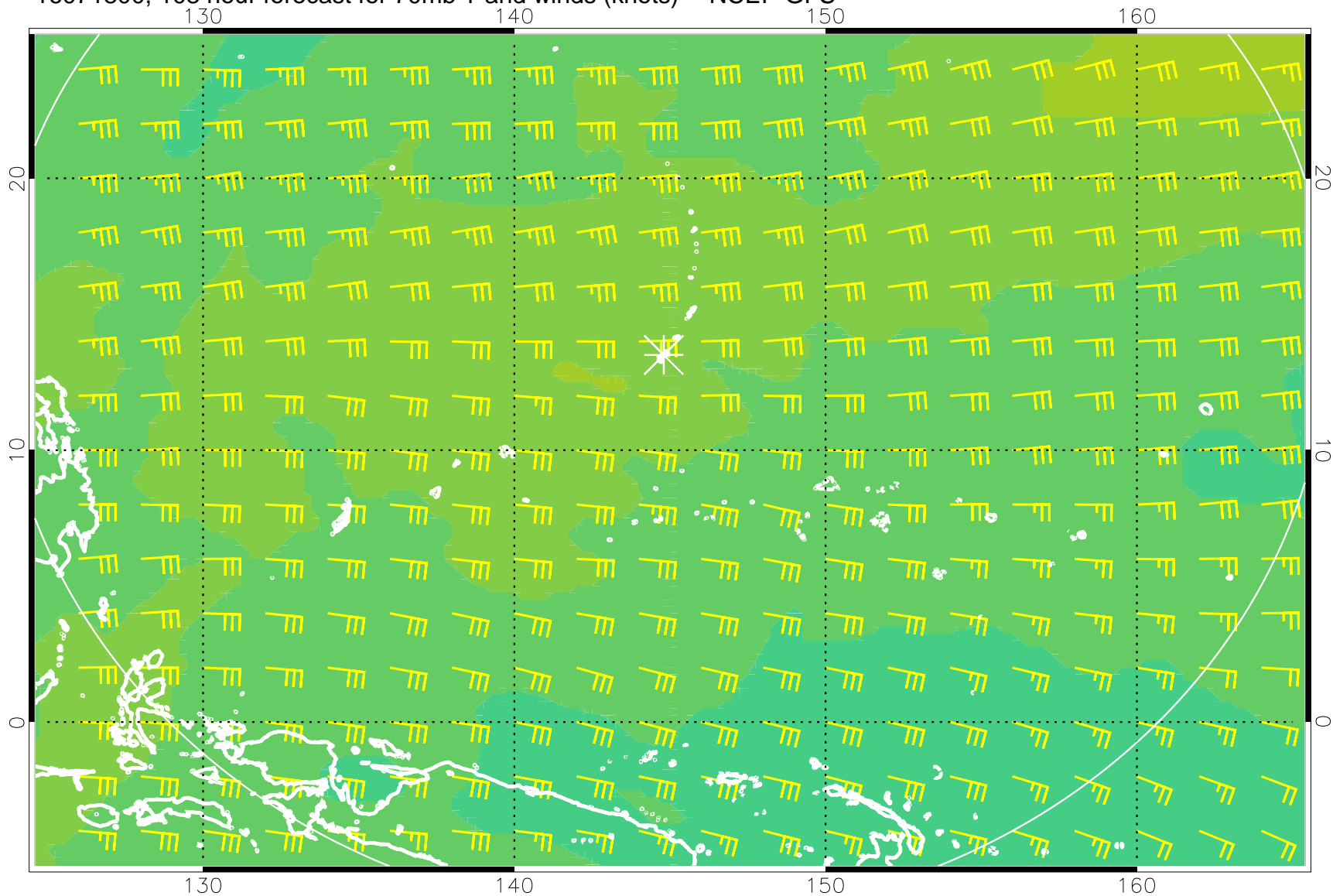
16071800, 108 hour forecast for 70mb T and winds (knots) -- NCEP GFS
