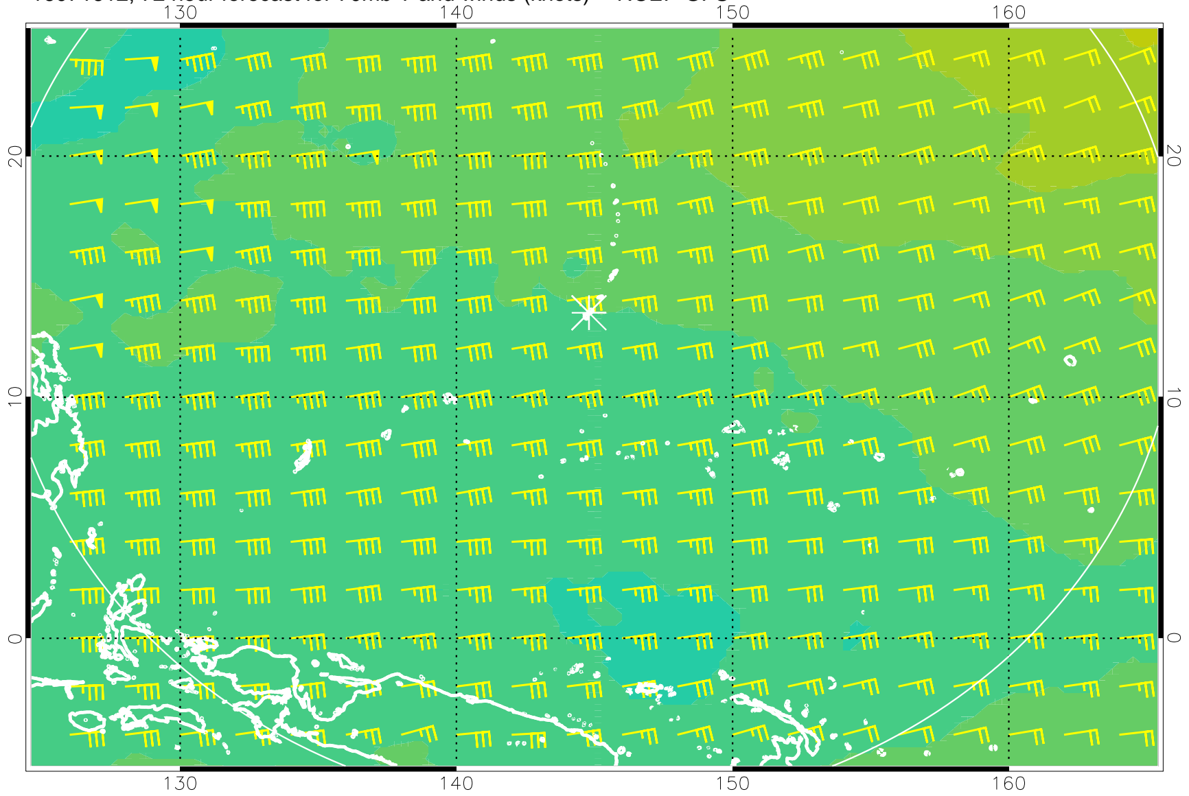
16071612, 72 hour forecast for 70mb T and winds (knots) -- NCEP GFS
