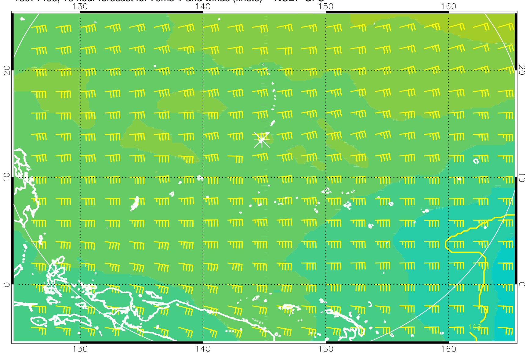
16071406, 18 hour forecast for 70mb T and winds (knots) -- NCEP GFS
