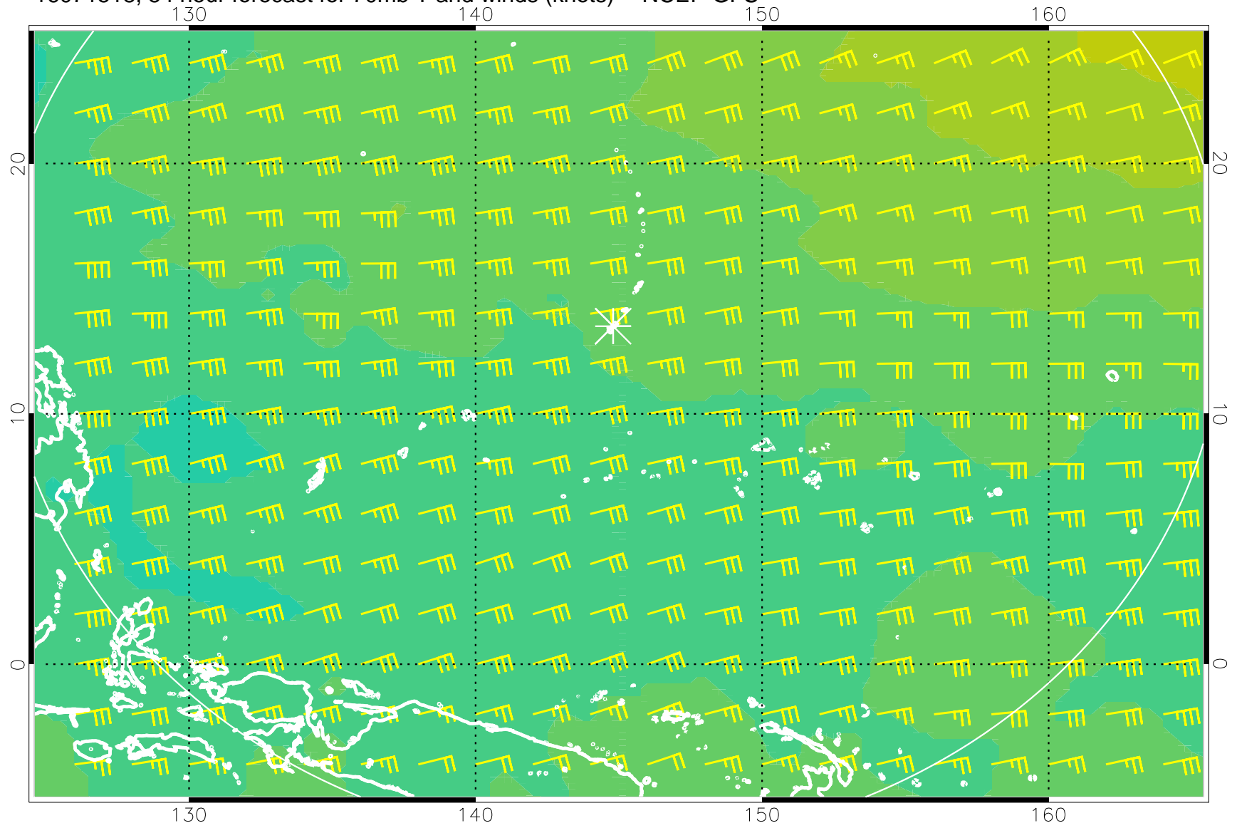
16071518, 54 hour forecast for 70mb T and winds (knots) -- NCEP GFS
