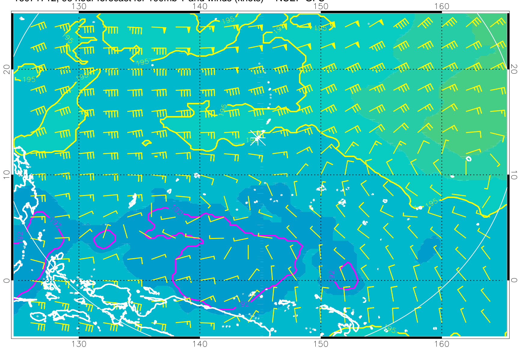
16071712, 96 hour forecast for 100mb T and winds (knots) -- NCEP GFS
