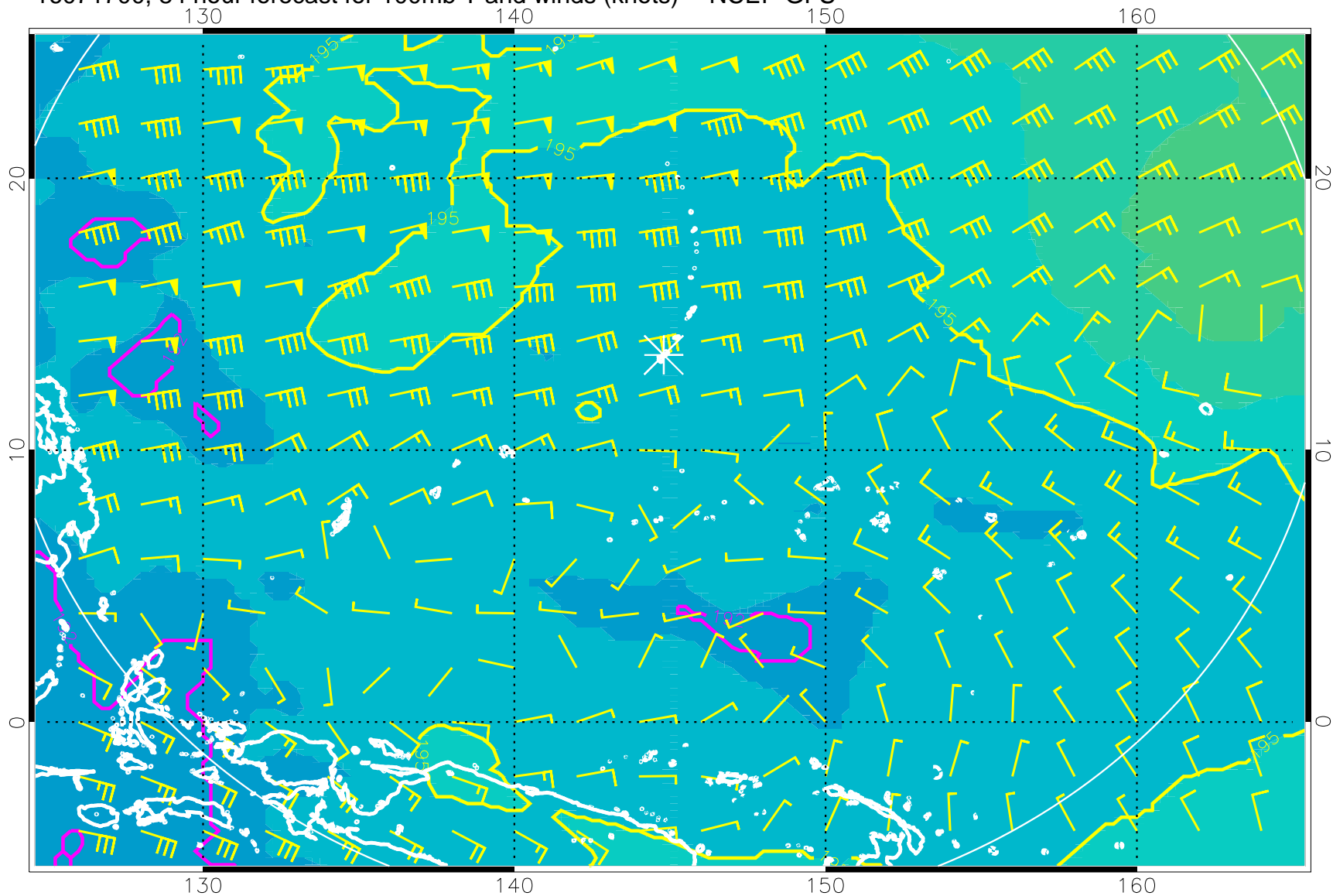
16071700, 84 hour forecast for 100mb T and winds (knots) -- NCEP GFS
