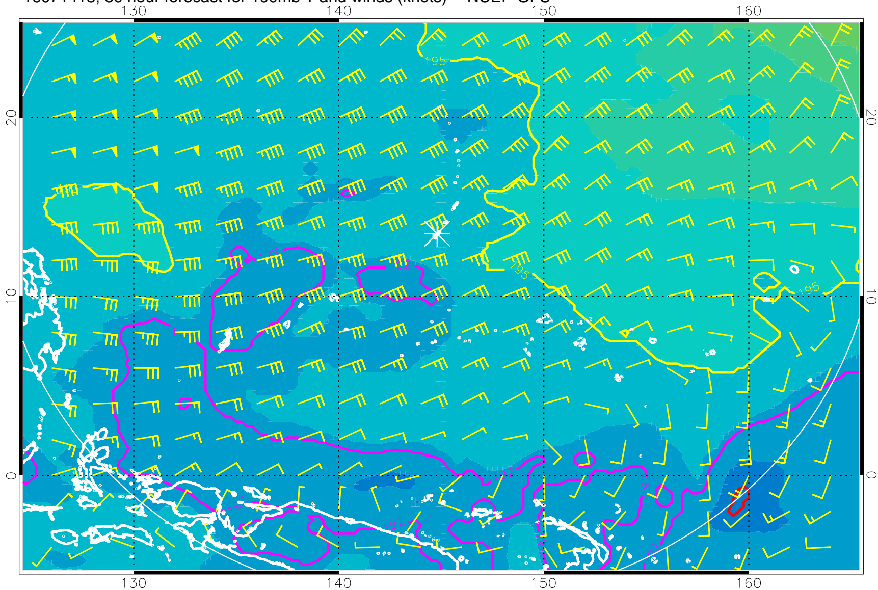
16071418, 30 hour forecast for 100mb T and winds (knots) -- NCEP GFS
