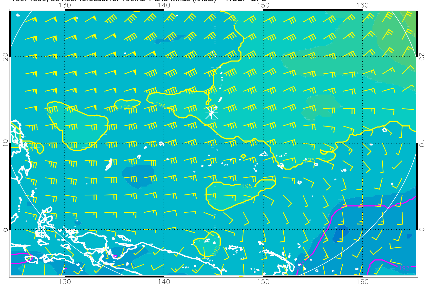
16071500, 36 hour forecast for 100mb T and winds (knots) -- NCEP GFS
