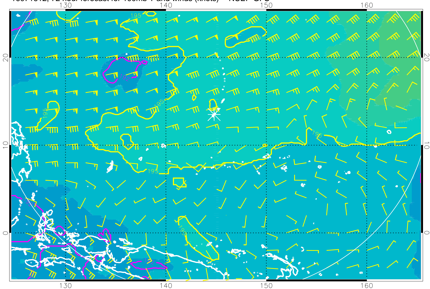
16071612, 72 hour forecast for 100mb T and winds (knots) -- NCEP GFS
