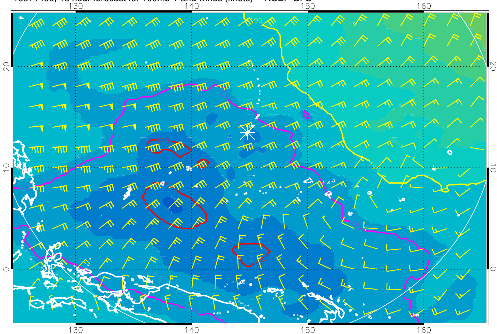
16071406, 18 hour forecast for 100mb T and winds (knots) -- NCEP GFS
