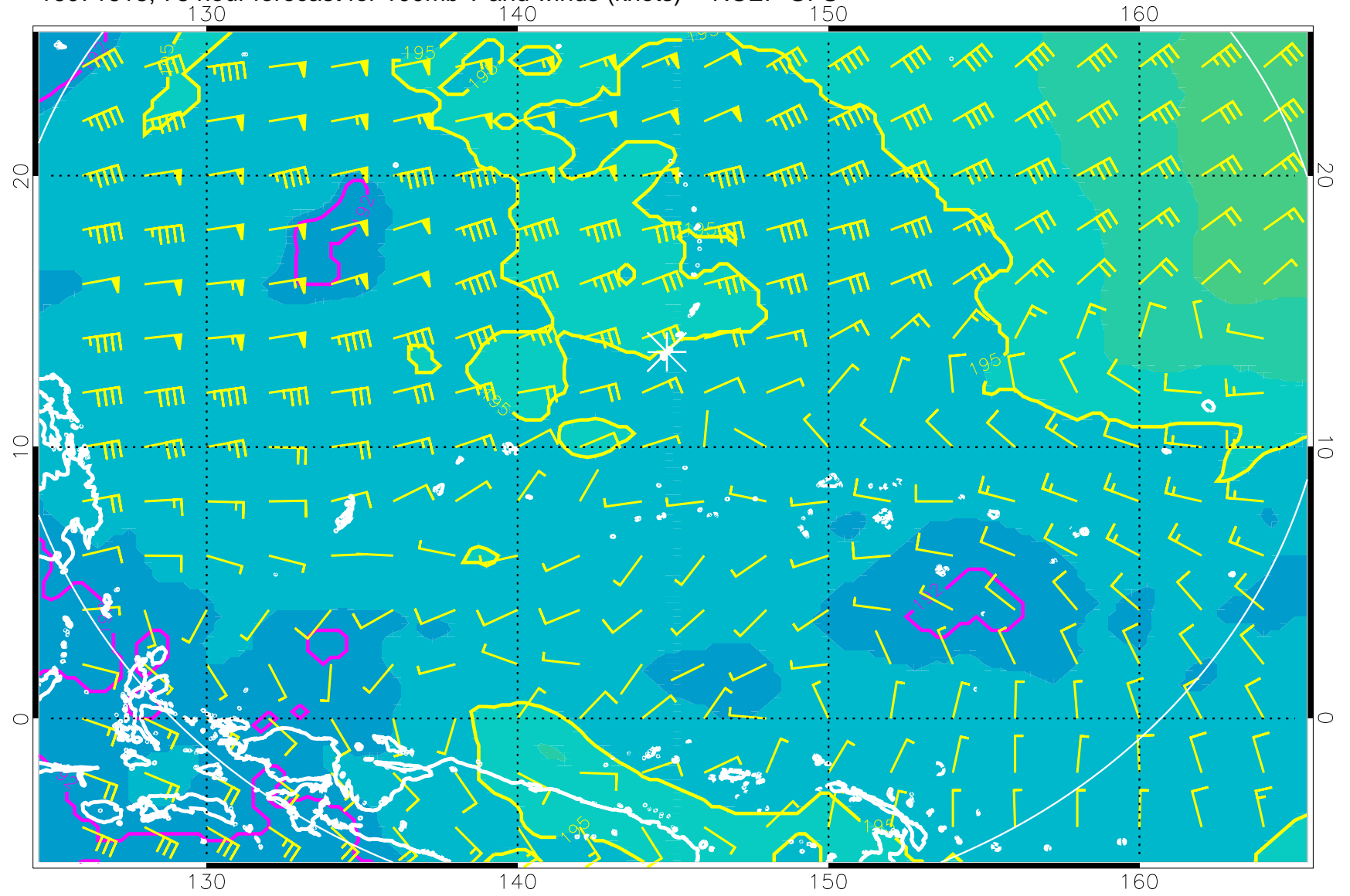
16071618, 78 hour forecast for 100mb T and winds (knots) -- NCEP GFS
