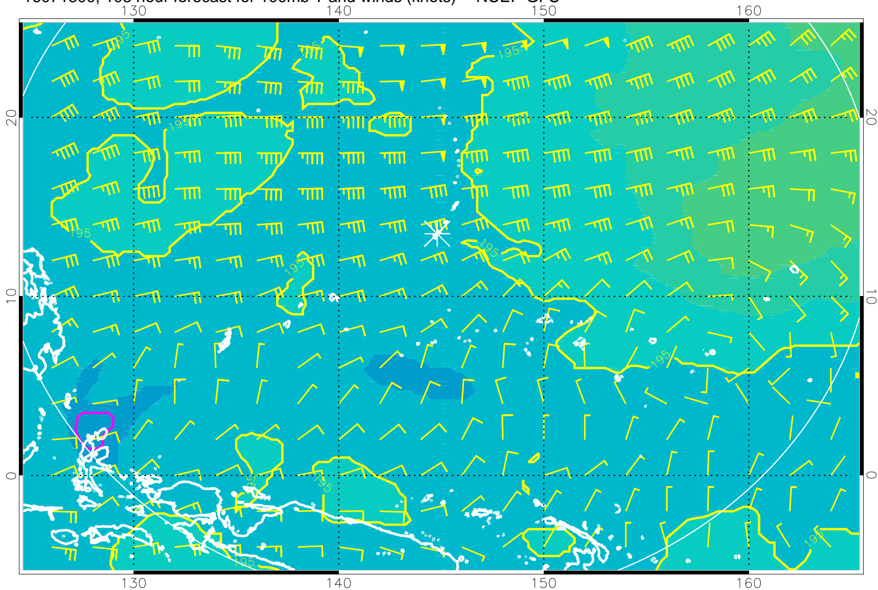
16071800, 108 hour forecast for 100mb T and winds (knots) -- NCEP GFS
