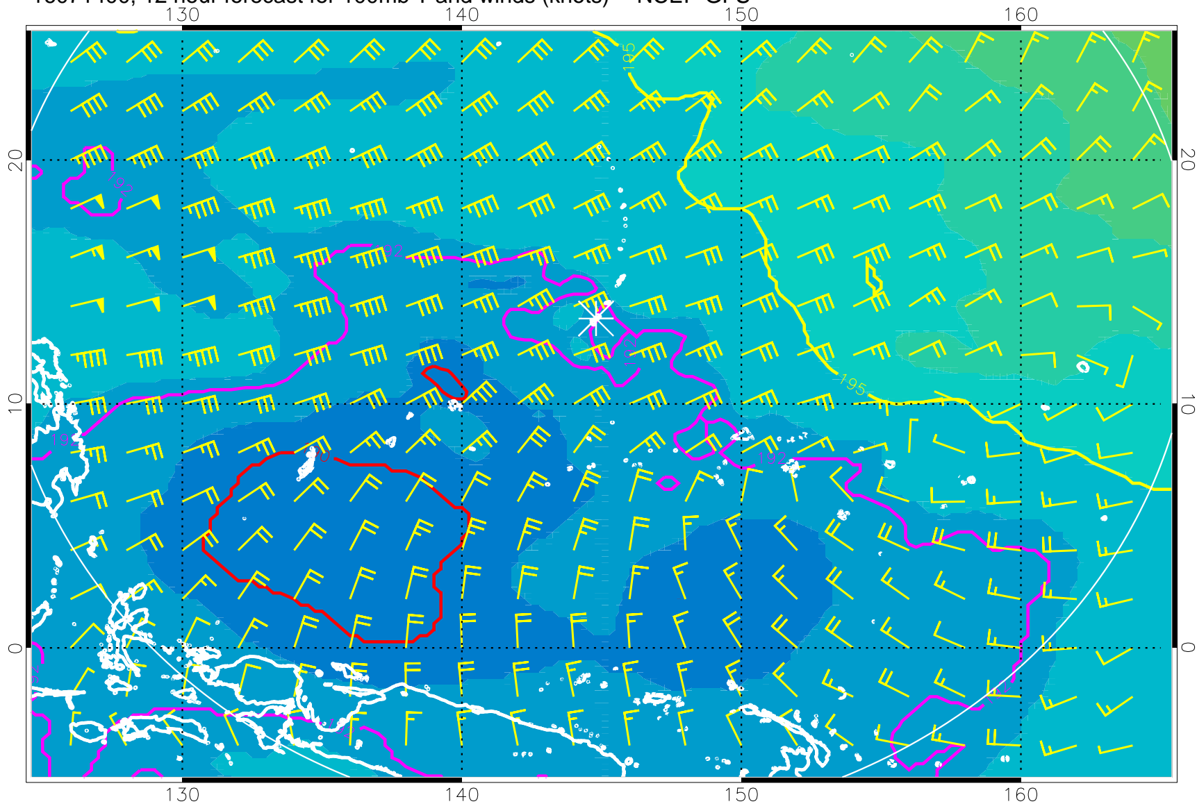
16071400, 12 hour forecast for 100mb T and winds (knots) -- NCEP GFS
