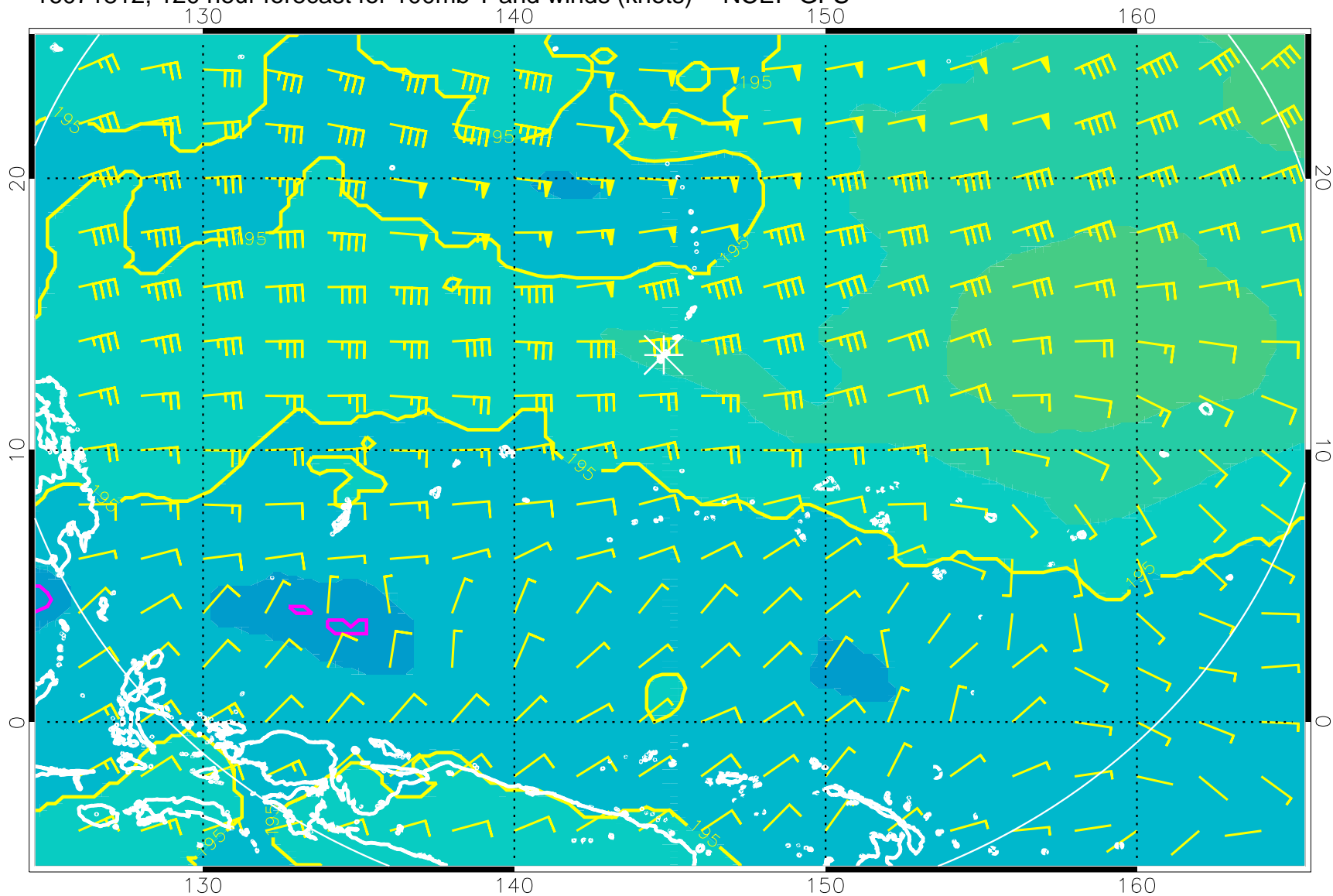
16071812, 120 hour forecast for 100mb T and winds (knots) -- NCEP GFS
