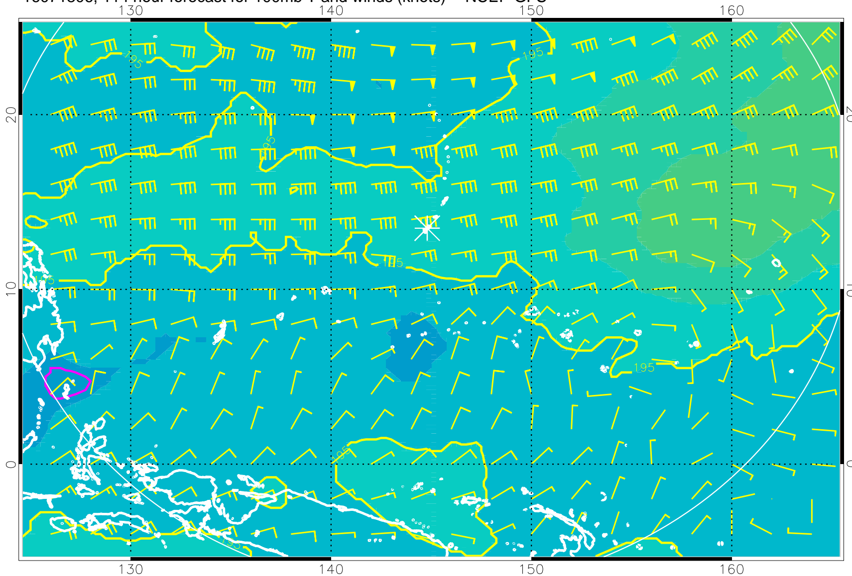
16071806, 114 hour forecast for 100mb T and winds (knots) -- NCEP GFS
