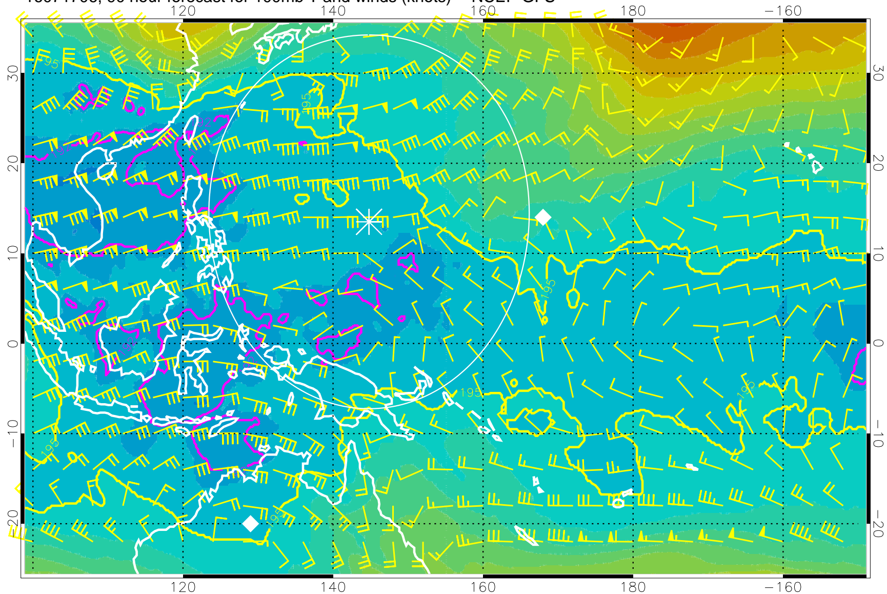
16071706, 90 hour forecast for 100mb T and winds (knots) -- NCEP GFS
