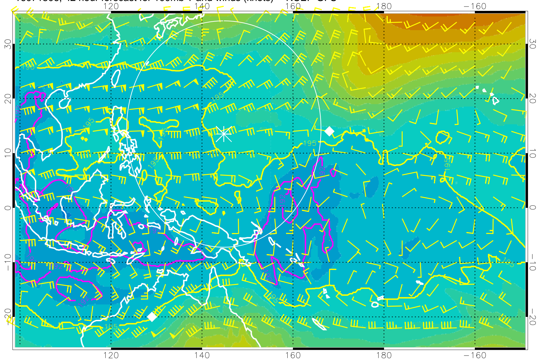
16071506, 42 hour forecast for 100mb T and winds (knots) -- NCEP GFS
