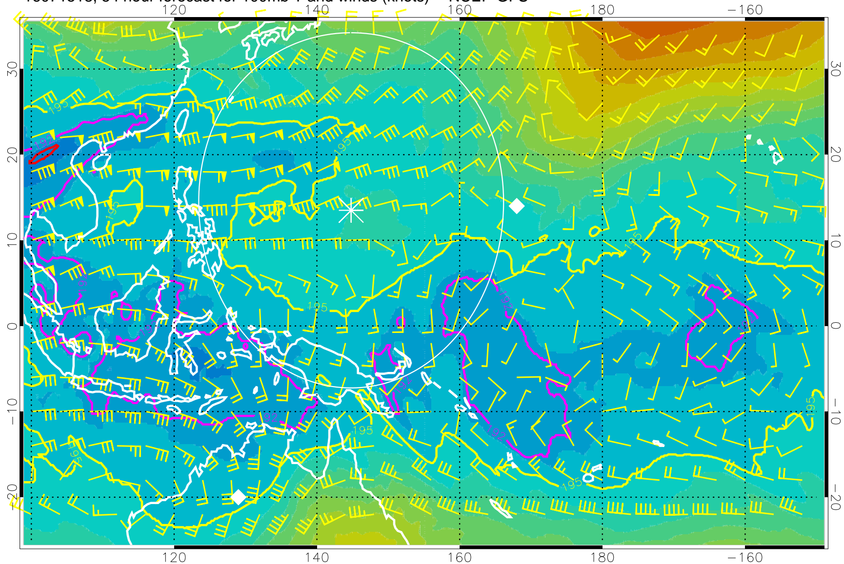
16071518, 54 hour forecast for 100mb T and winds (knots) -- NCEP GFS
