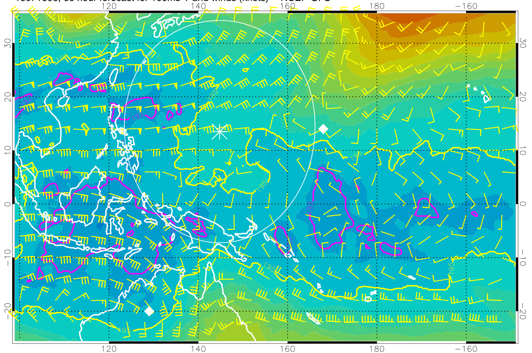
16071606, 66 hour forecast for 100mb T and winds (knots) -- NCEP GFS
