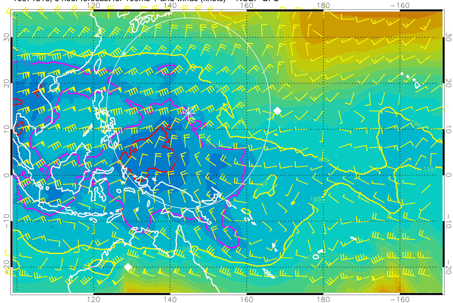
16071318, 6 hour forecast for 100mb T and winds (knots) -- NCEP GFS
