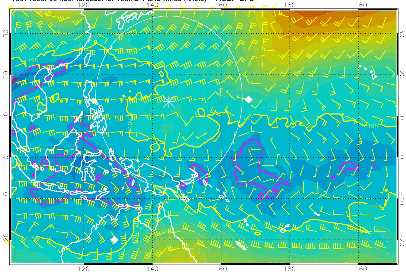
16071600, 60 hour forecast for 100mb T and winds (knots) -- NCEP GFS
