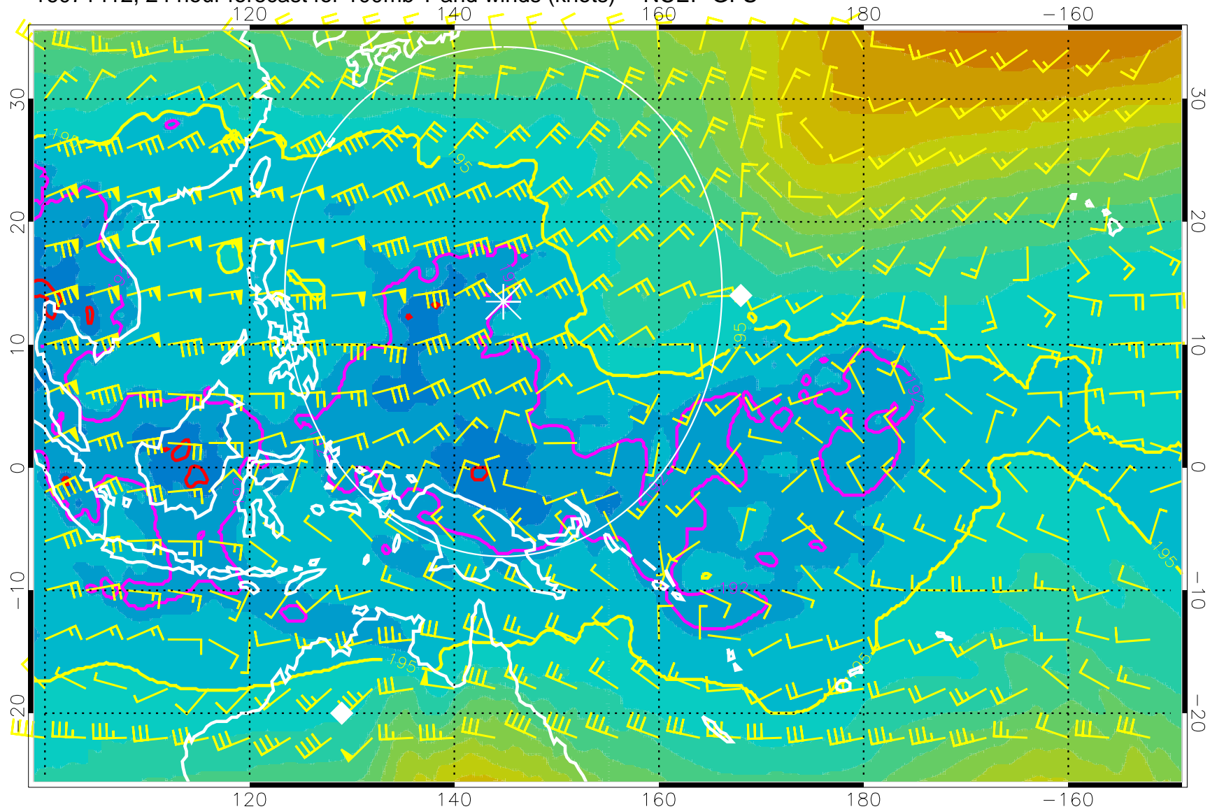
16071412, 24 hour forecast for 100mb T and winds (knots) -- NCEP GFS
