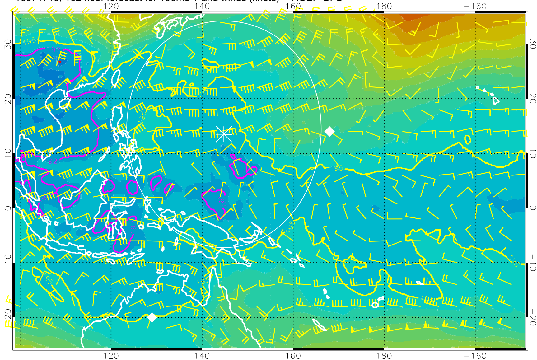
16071718, 102 hour forecast for 100mb T and winds (knots) -- NCEP GFS
