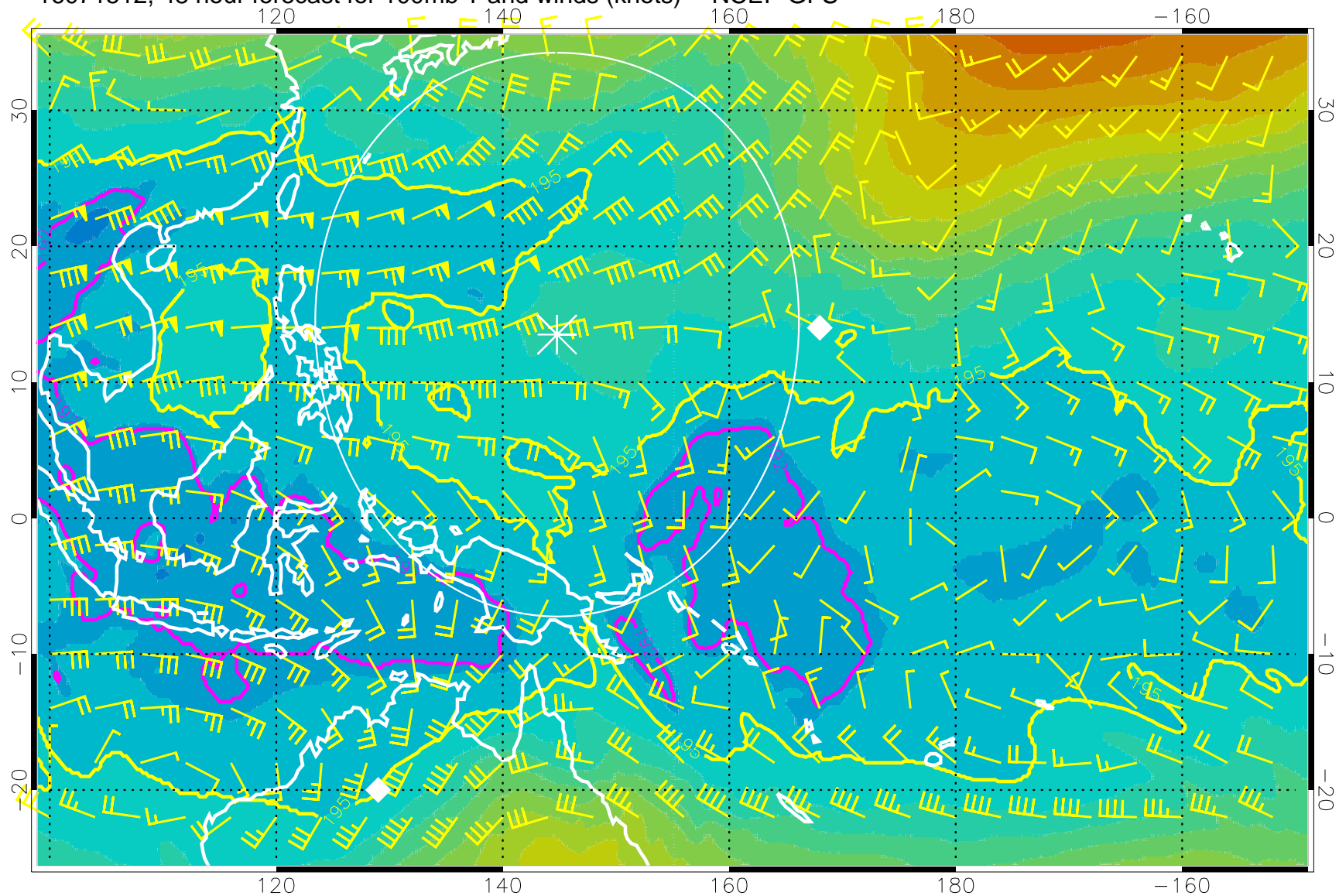
16071512, 48 hour forecast for 100mb T and winds (knots) -- NCEP GFS
