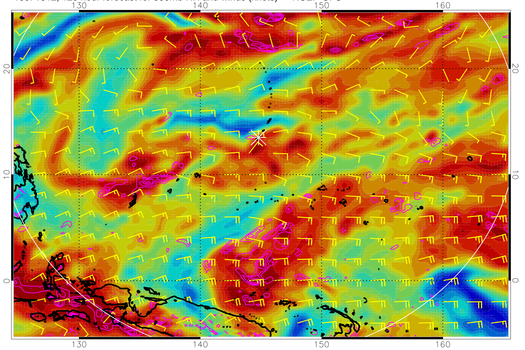
16071812, 120 hour forecast for 500mb RH and winds (knots) -- NCEP GFS
