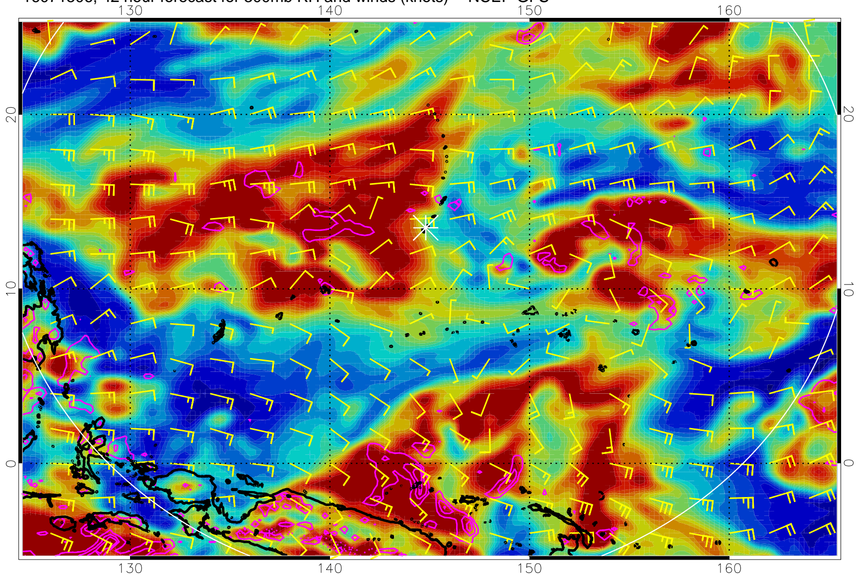
16071506, 42 hour forecast for 300mb RH and winds (knots) -- NCEP GFS
