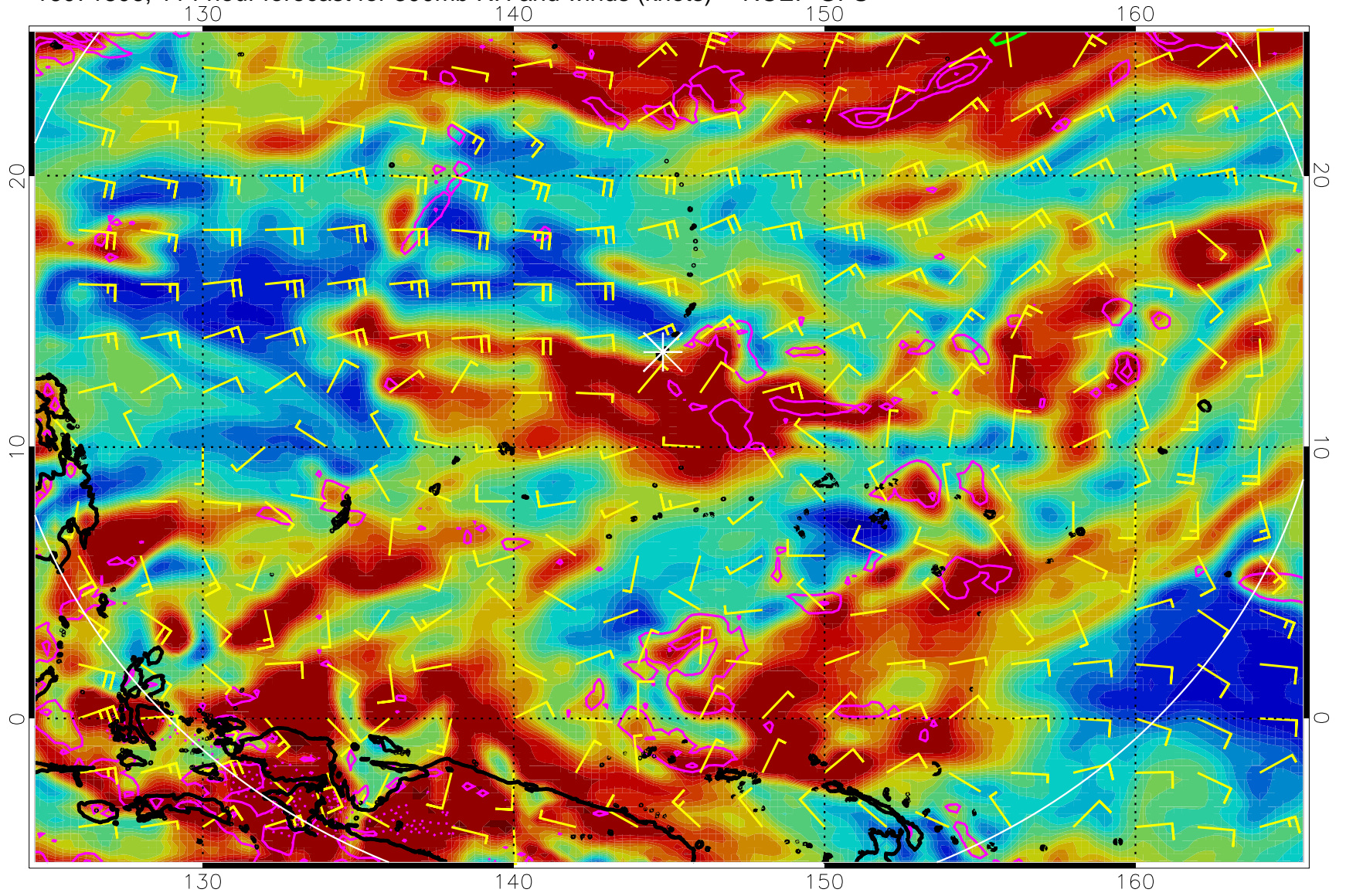
16071806, 114 hour forecast for 300mb RH and winds (knots) -- NCEP GFS
