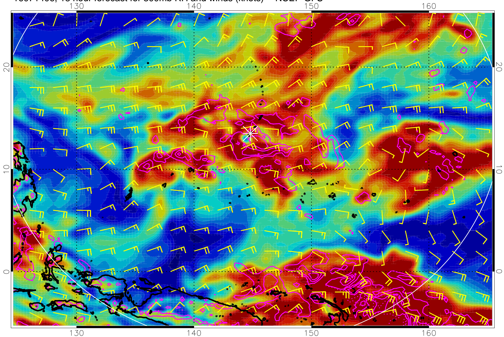
16071406, 18 hour forecast for 300mb RH and winds (knots) -- NCEP GFS
