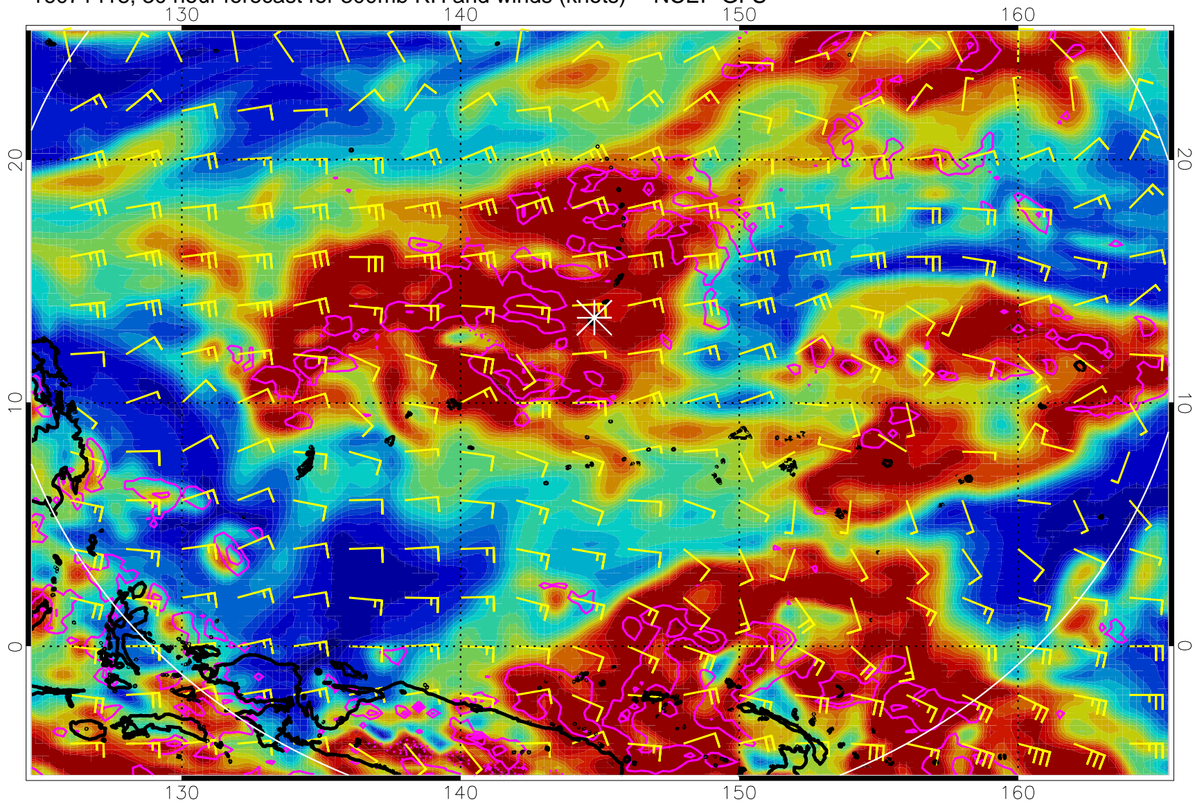
16071418, 30 hour forecast for 300mb RH and winds (knots) -- NCEP GFS
