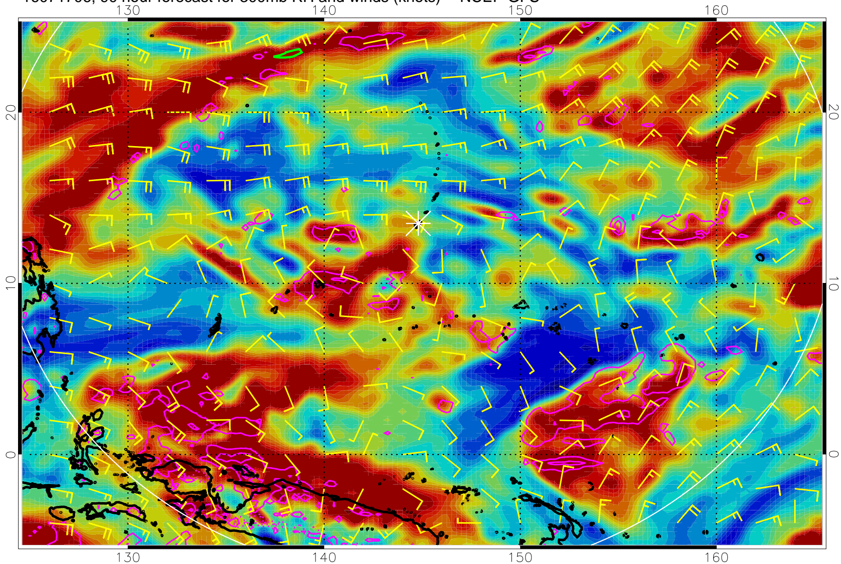
16071706, 90 hour forecast for 300mb RH and winds (knots) -- NCEP GFS
