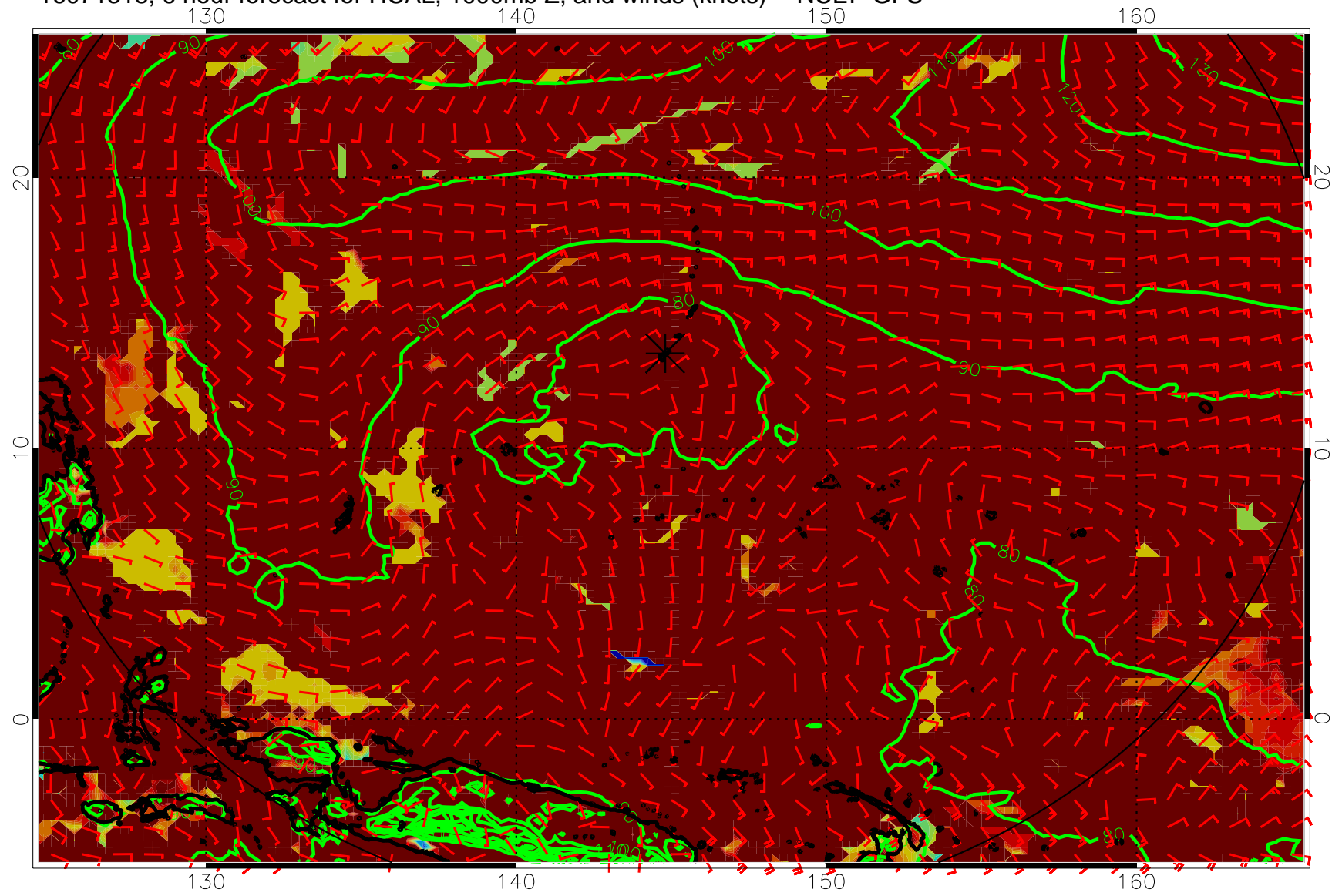
16071318, 6 hour forecast for HCAL, 1000mb Z, and winds (knots) -- NCEP GFS
