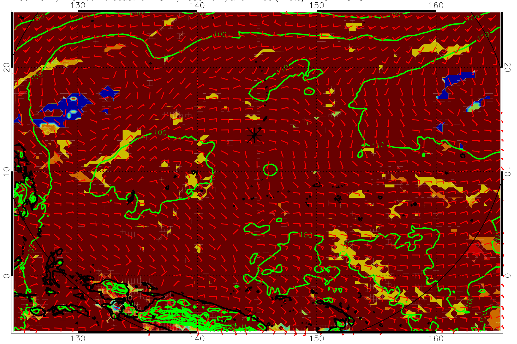
16071812, 120 hour forecast for HCAL, 1000mb Z, and winds (knots) -- NCEP GFS
