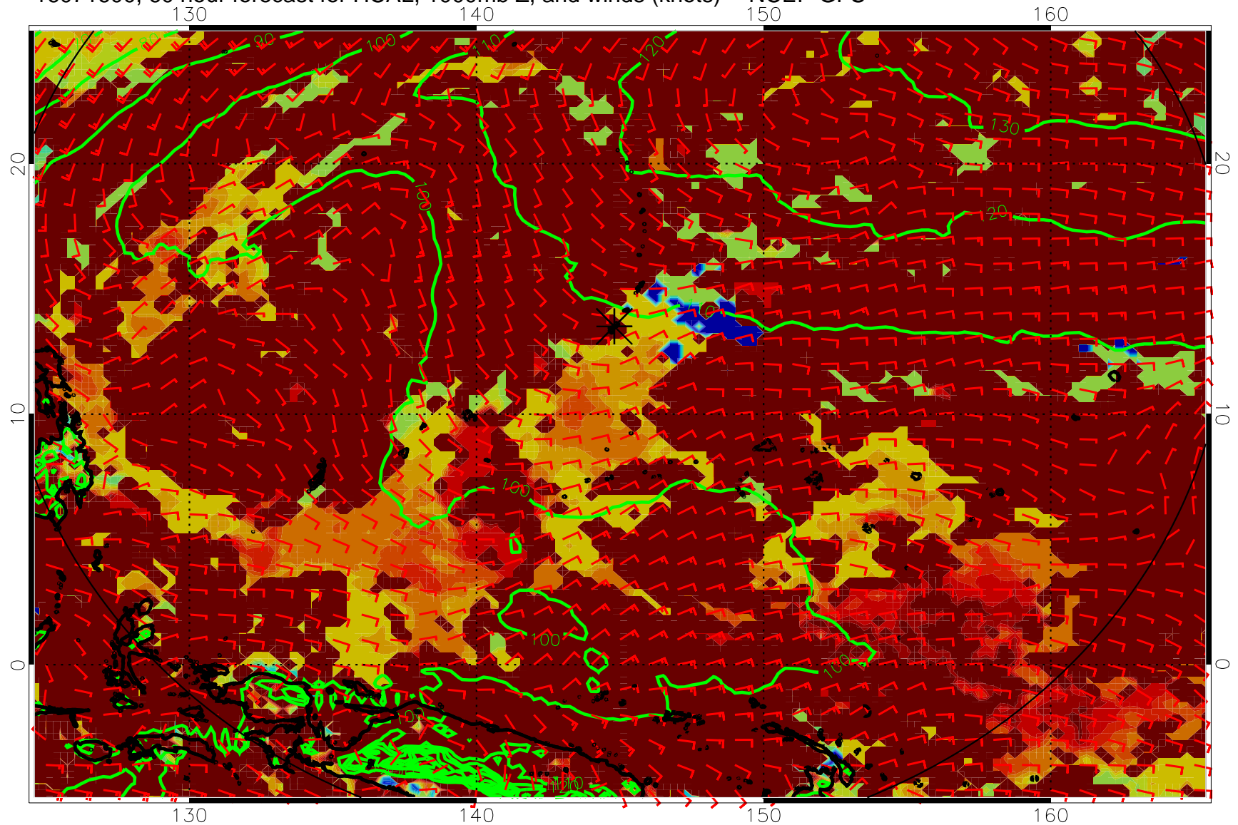
16071600, 60 hour forecast for HCAL, 1000mb Z, and winds (knots) -- NCEP GFS
