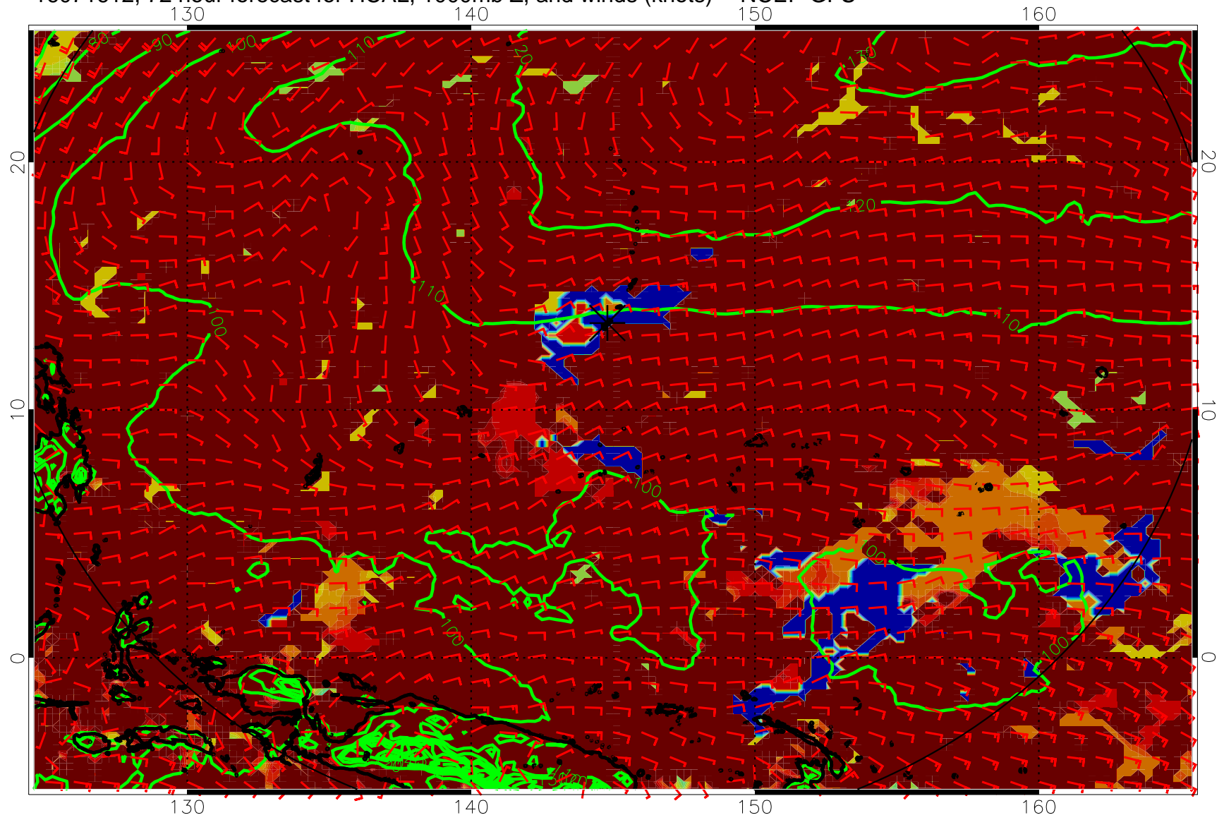
16071612, 72 hour forecast for HCAL, 1000mb Z, and winds (knots) -- NCEP GFS
