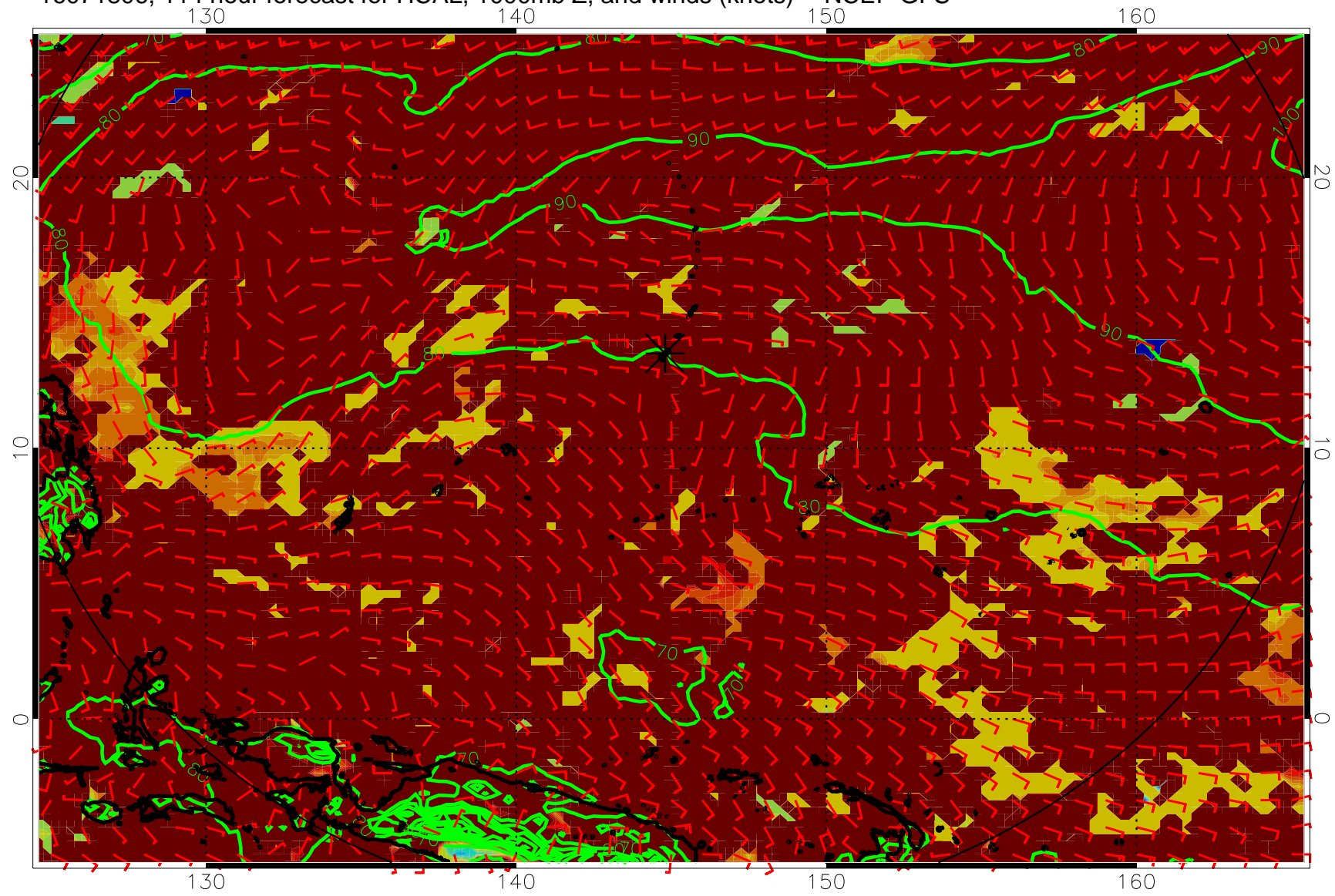
16071806, 114 hour forecast for HCAL, 1000mb Z, and winds (knots) -- NCEP GFS
