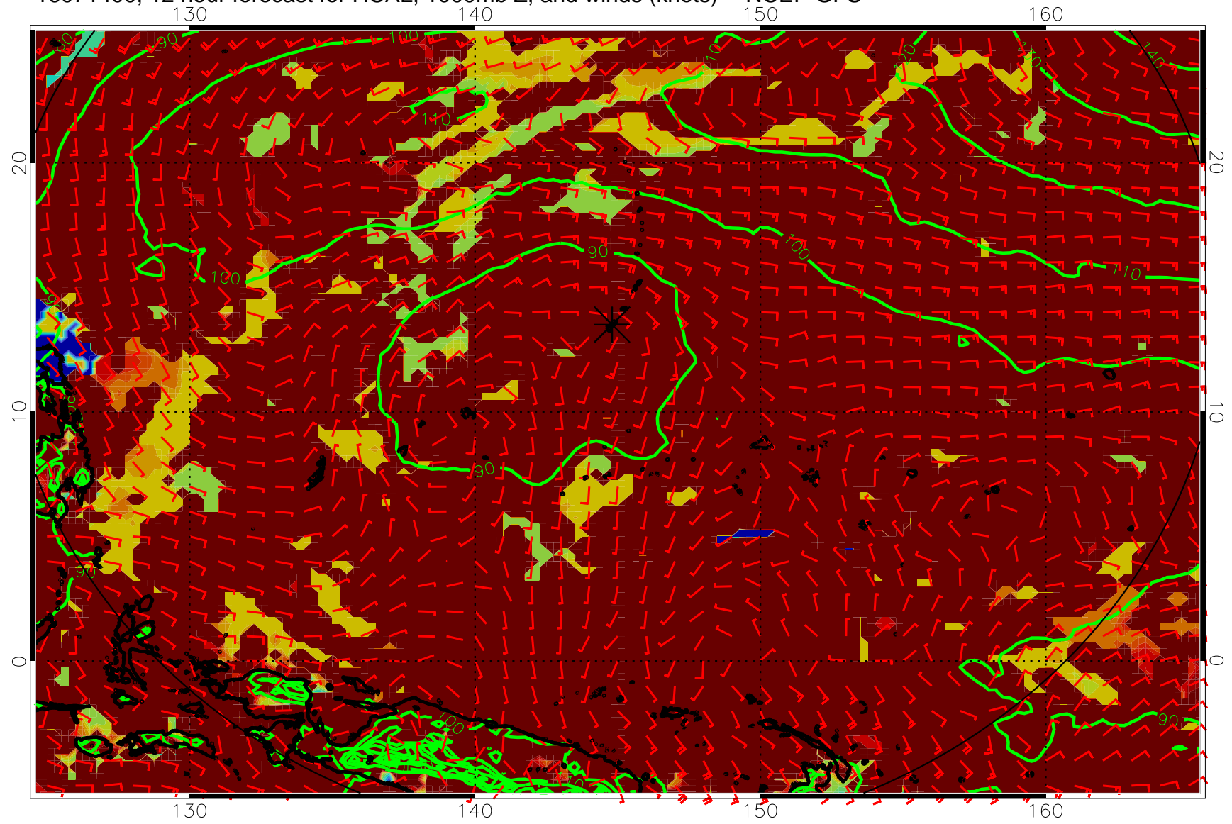
16071400, 12 hour forecast for HCAL, 1000mb Z, and winds (knots) -- NCEP GFS
