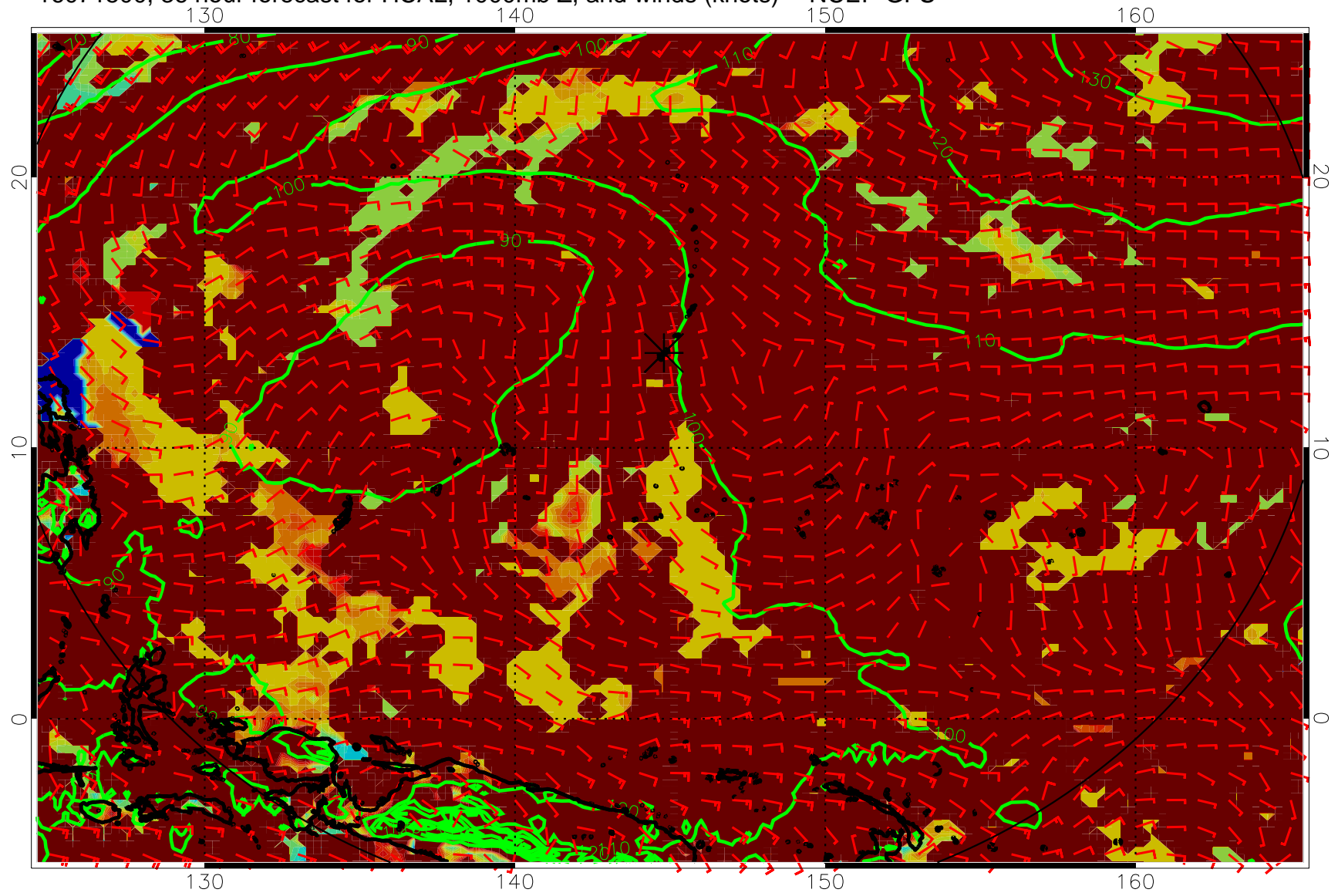
16071500, 36 hour forecast for HCAL, 1000mb Z, and winds (knots) -- NCEP GFS
