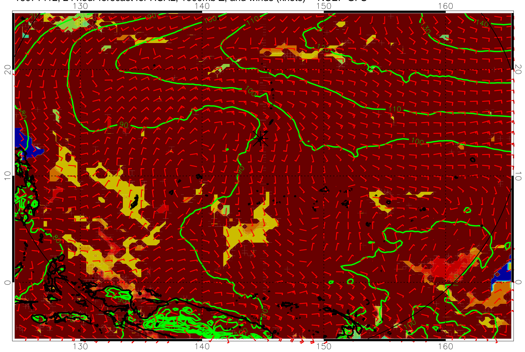
16071412, 24 hour forecast for HCAL, 1000mb Z, and winds (knots) -- NCEP GFS
