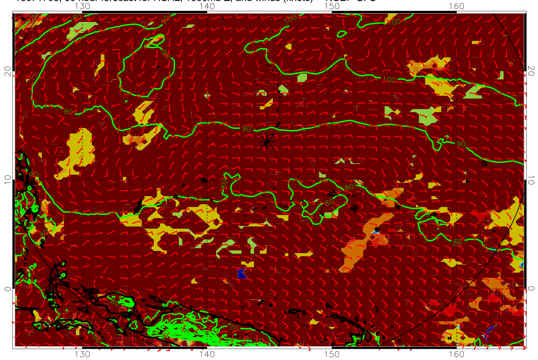
16071706, 90 hour forecast for HCAL, 1000mb Z, and winds (knots) -- NCEP GFS
