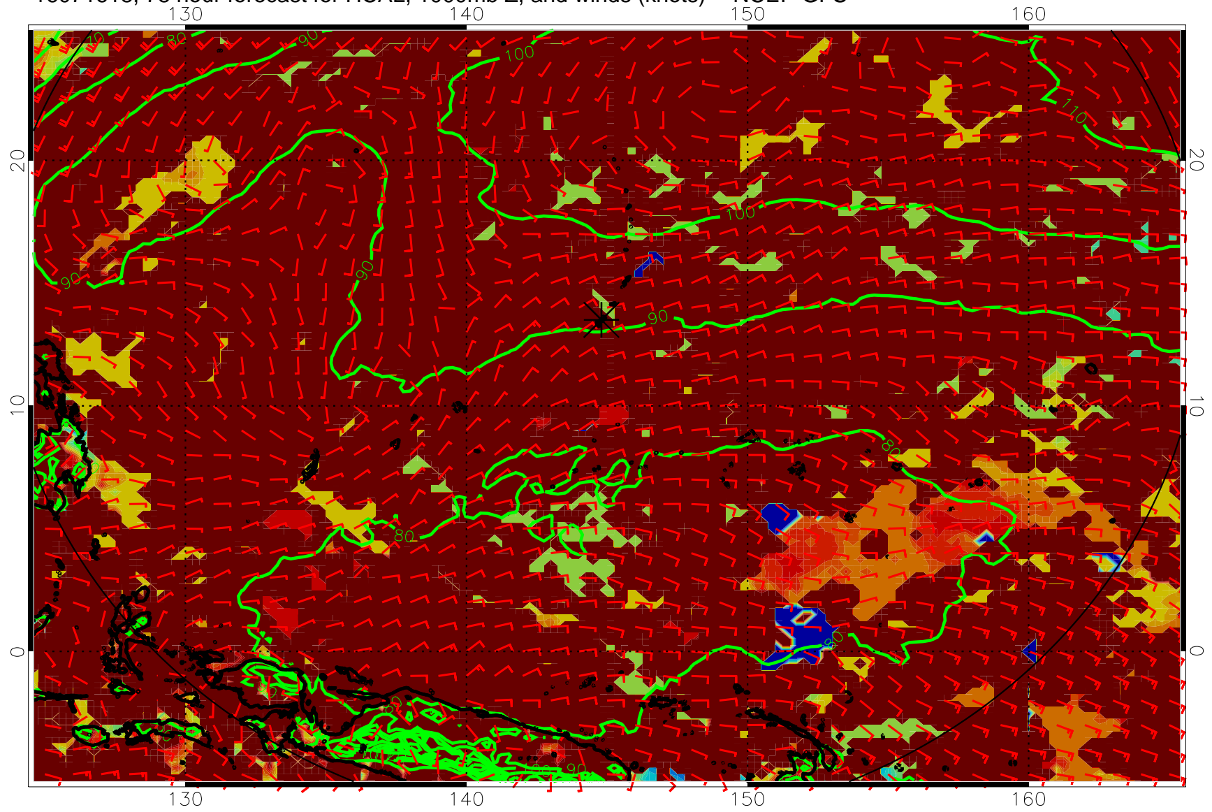
16071618, 78 hour forecast for HCAL, 1000mb Z, and winds (knots) -- NCEP GFS
