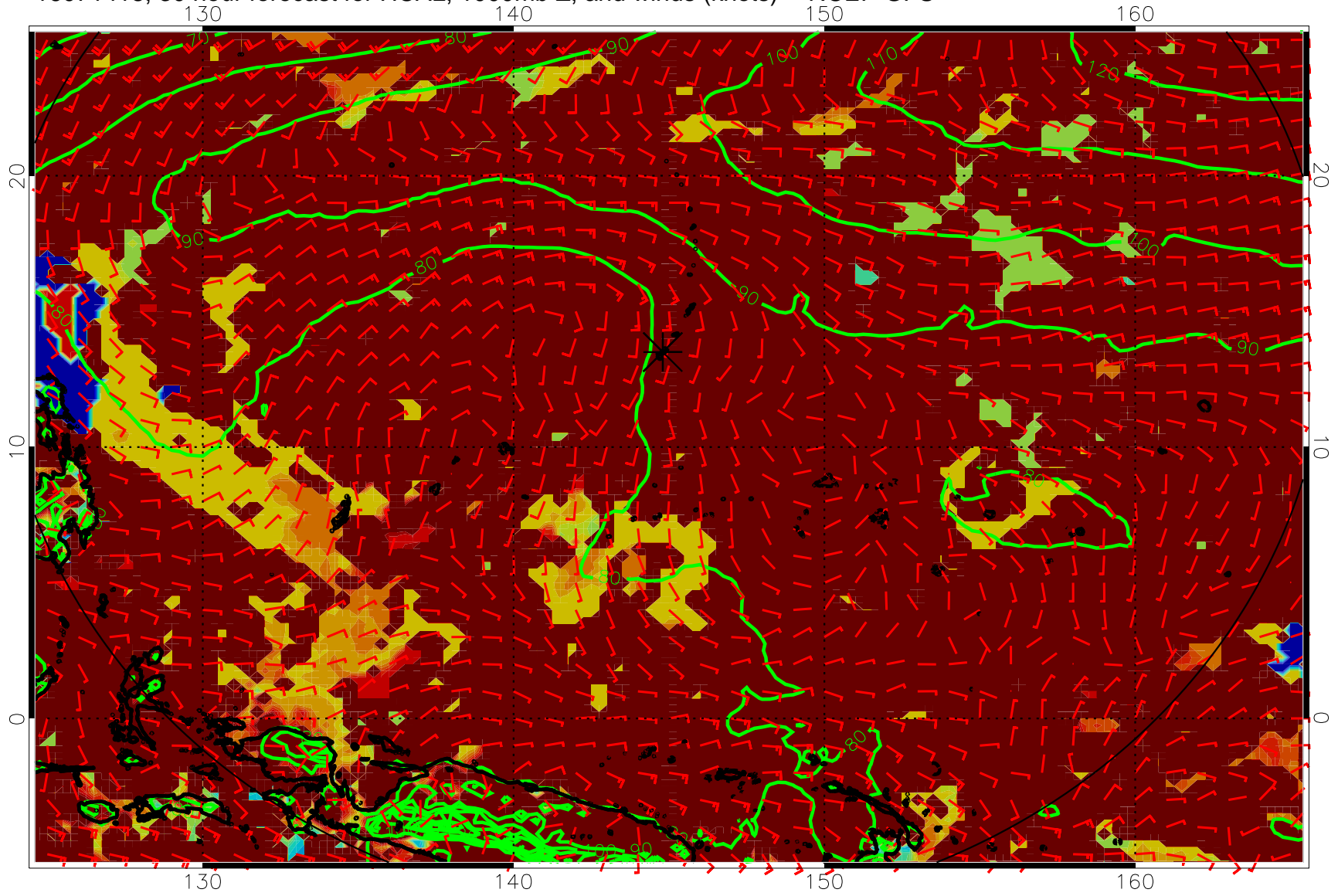
16071418, 30 hour forecast for HCAL, 1000mb Z, and winds (knots) -- NCEP GFS
