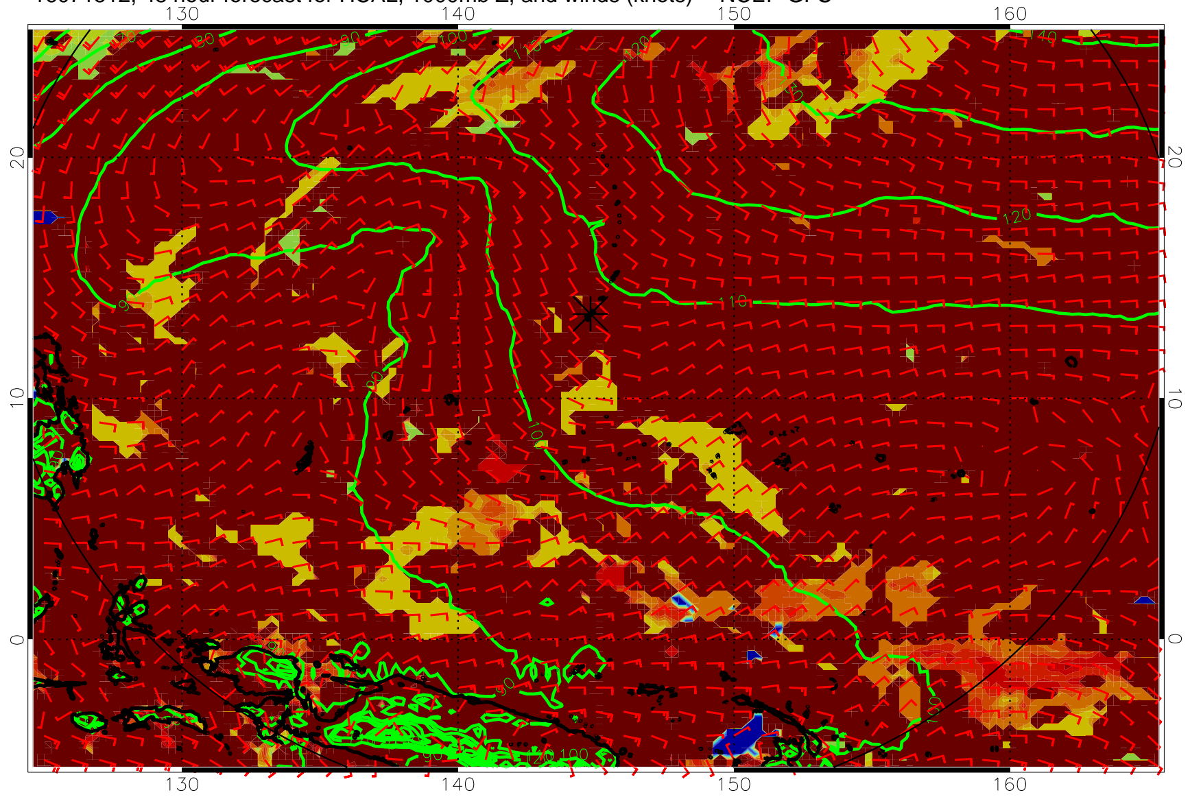
16071512, 48 hour forecast for HCAL, 1000mb Z, and winds (knots) -- NCEP GFS
