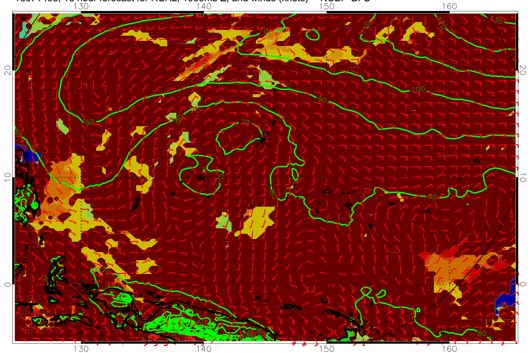
16071406, 18 hour forecast for HCAL, 1000mb Z, and winds (knots) -- NCEP GFS
