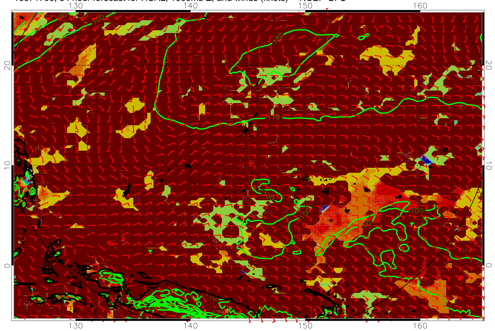
16071700, 84 hour forecast for HCAL, 1000mb Z, and winds (knots) -- NCEP GFS
