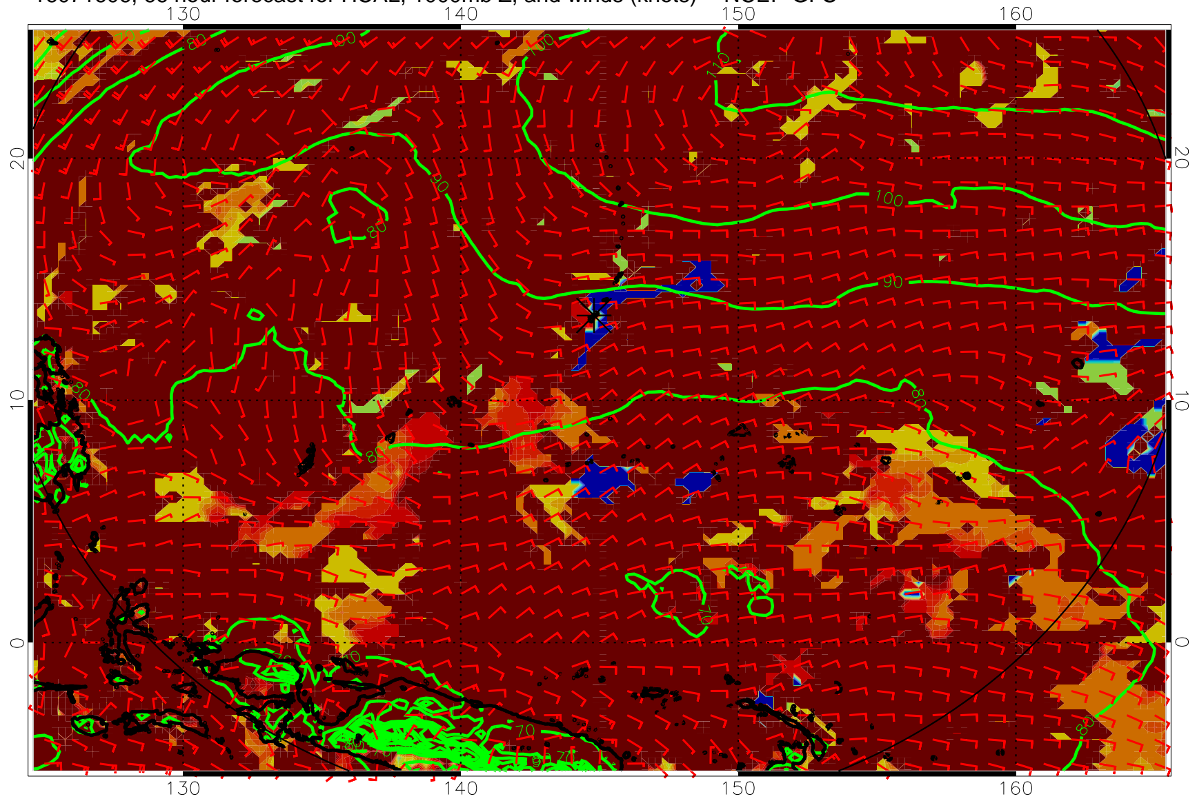
16071606, 66 hour forecast for HCAL, 1000mb Z, and winds (knots) -- NCEP GFS
