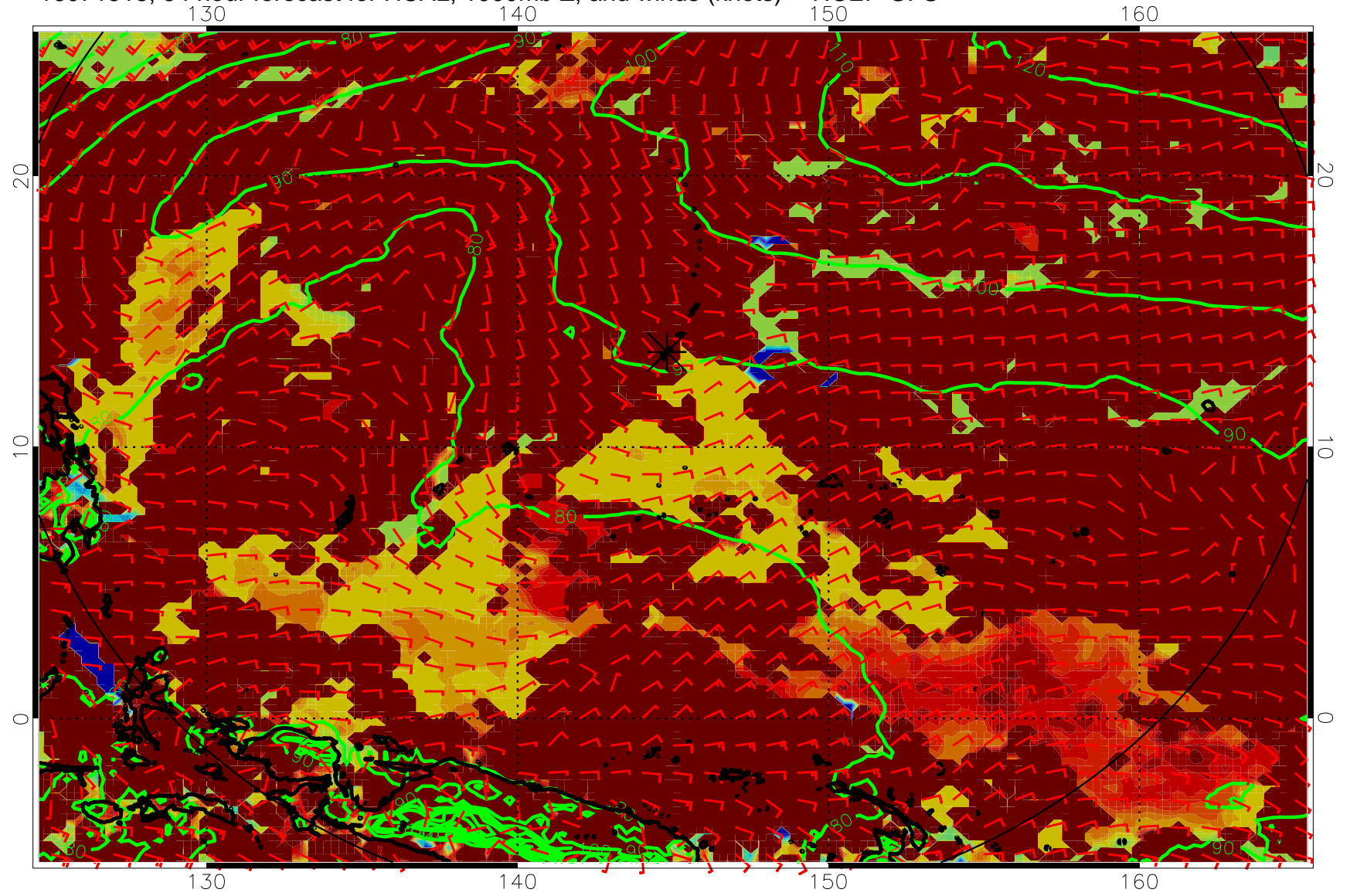
16071518, 54 hour forecast for HCAL, 1000mb Z, and winds (knots) -- NCEP GFS
