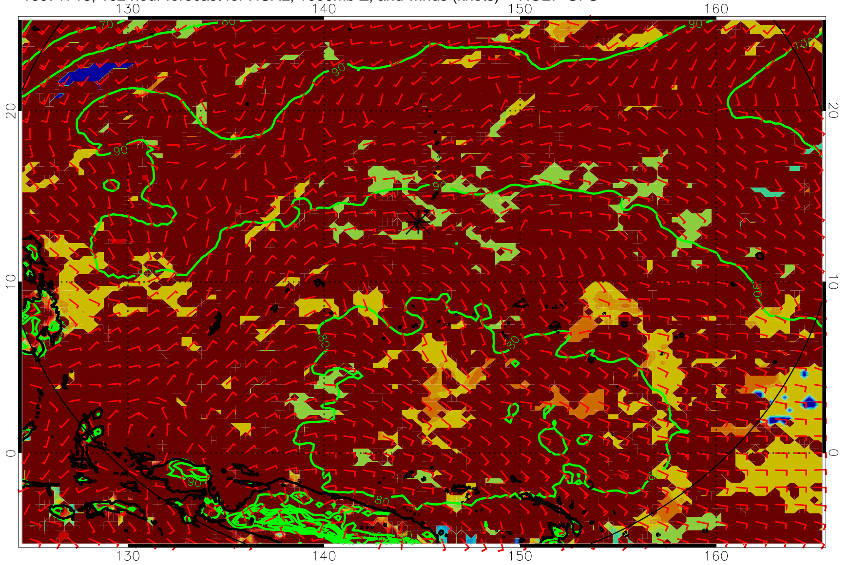
16071718, 102 hour forecast for HCAL, 1000mb Z, and winds (knots) -- NCEP GFS
