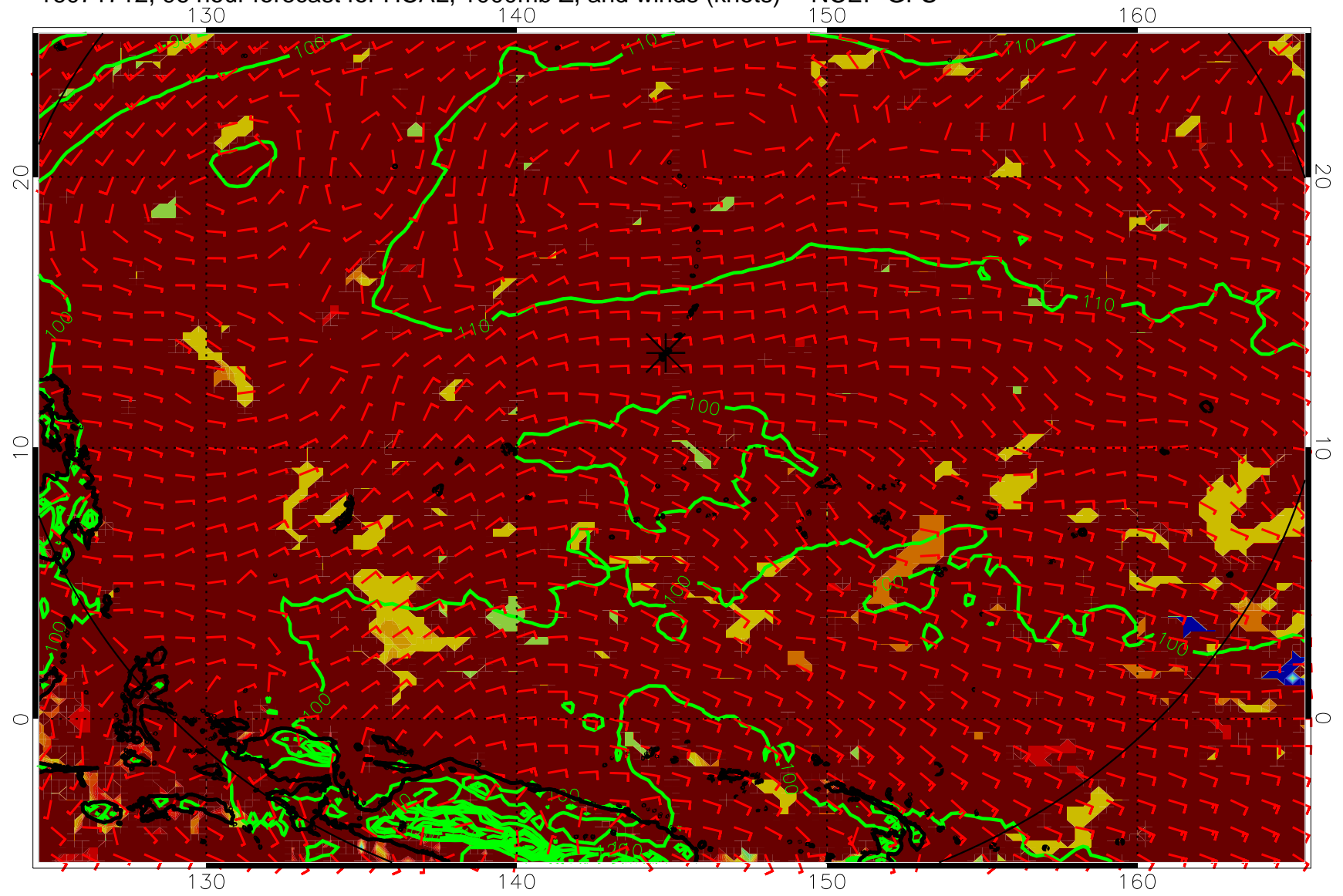
16071712, 96 hour forecast for HCAL, 1000mb Z, and winds (knots) -- NCEP GFS
