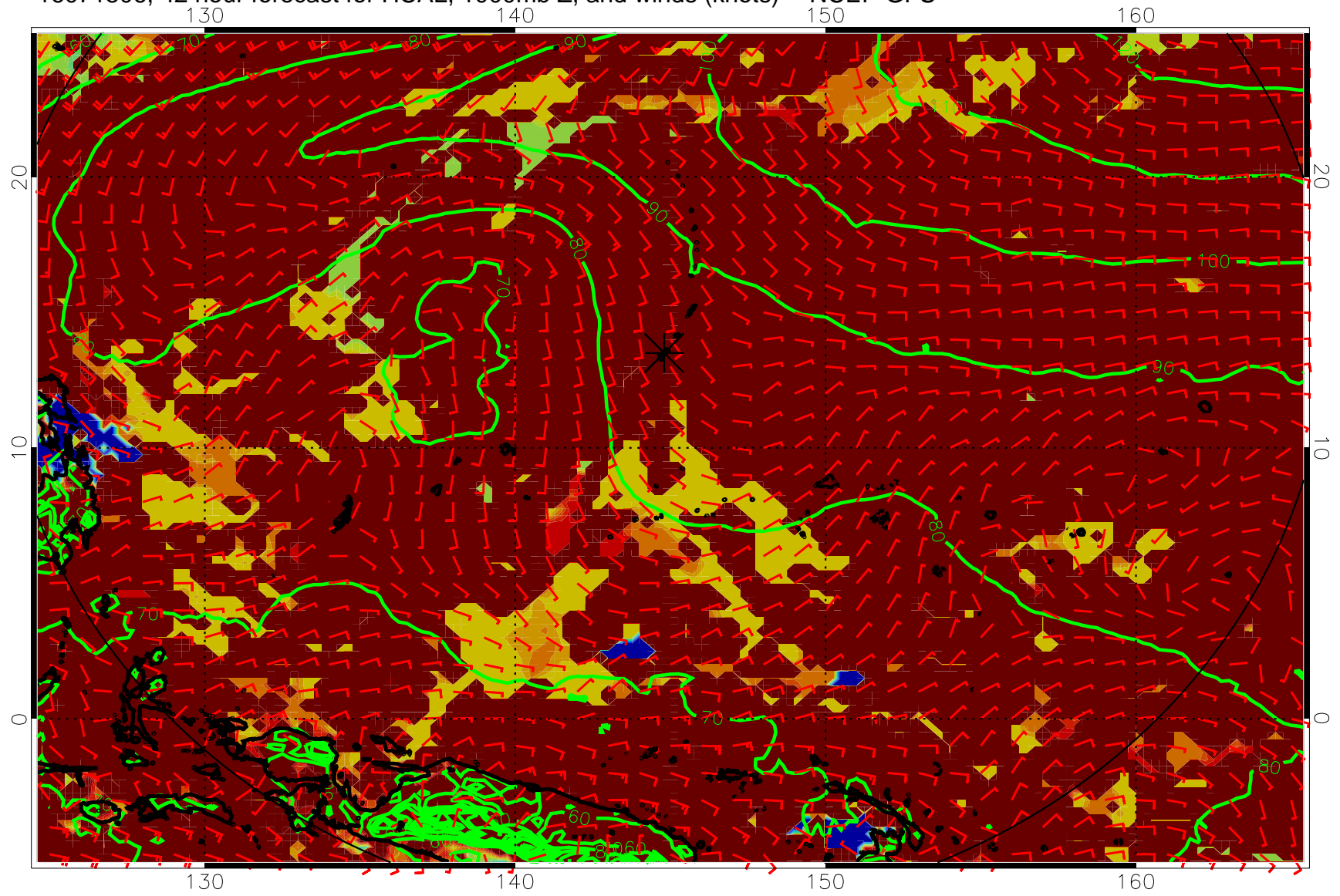
16071506, 42 hour forecast for HCAL, 1000mb Z, and winds (knots) -- NCEP GFS
