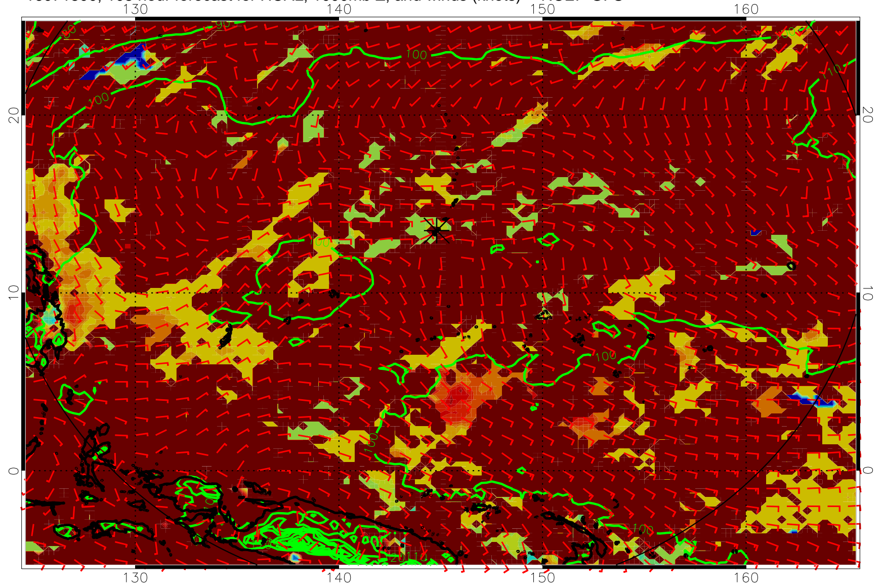
16071800, 108 hour forecast for HCAL, 1000mb Z, and winds (knots) -- NCEP GFS
