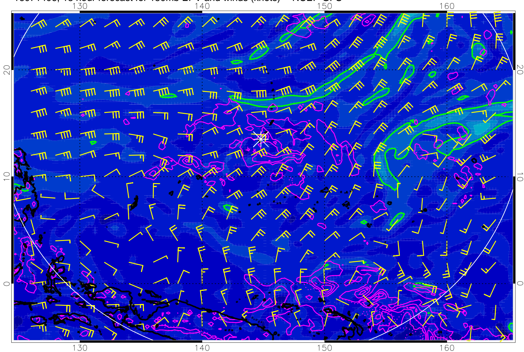
16071406, 18 hour forecast for 150mb EPV and winds (knots) -- NCEP GFS
