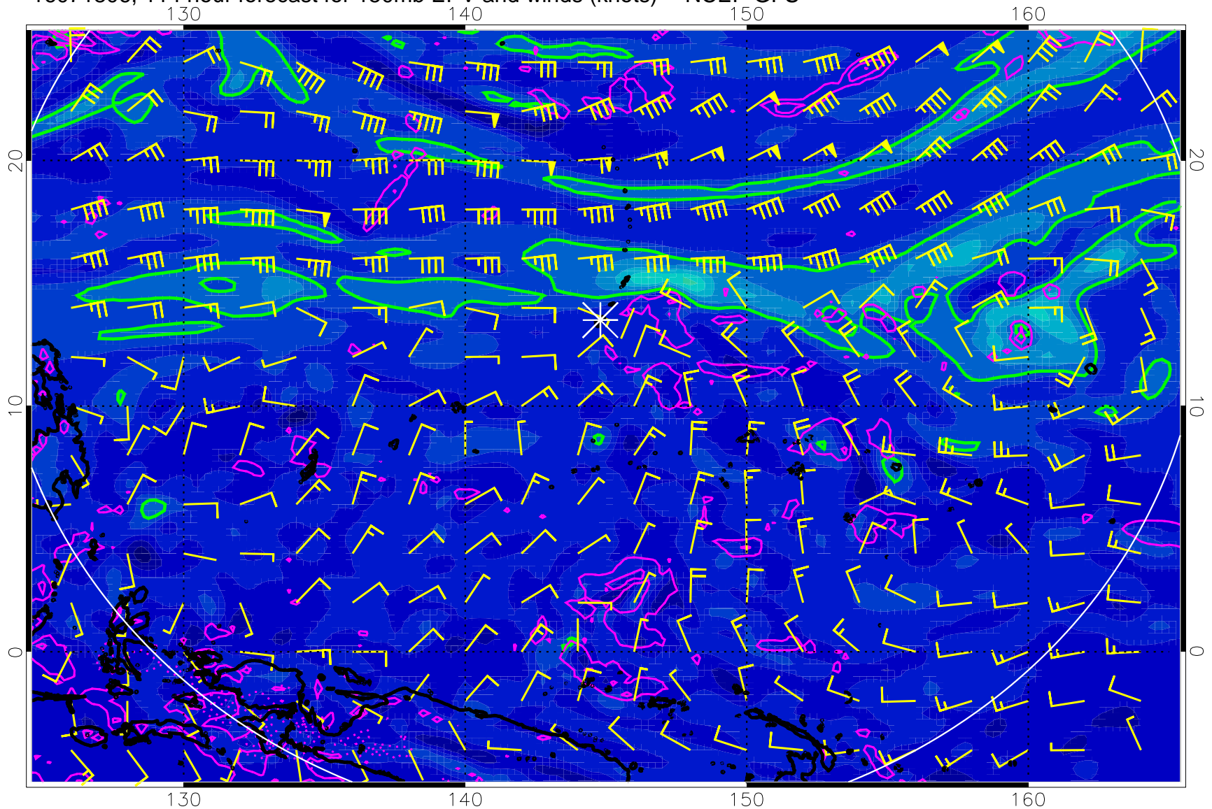
16071806, 114 hour forecast for 150mb EPV and winds (knots) -- NCEP GFS
