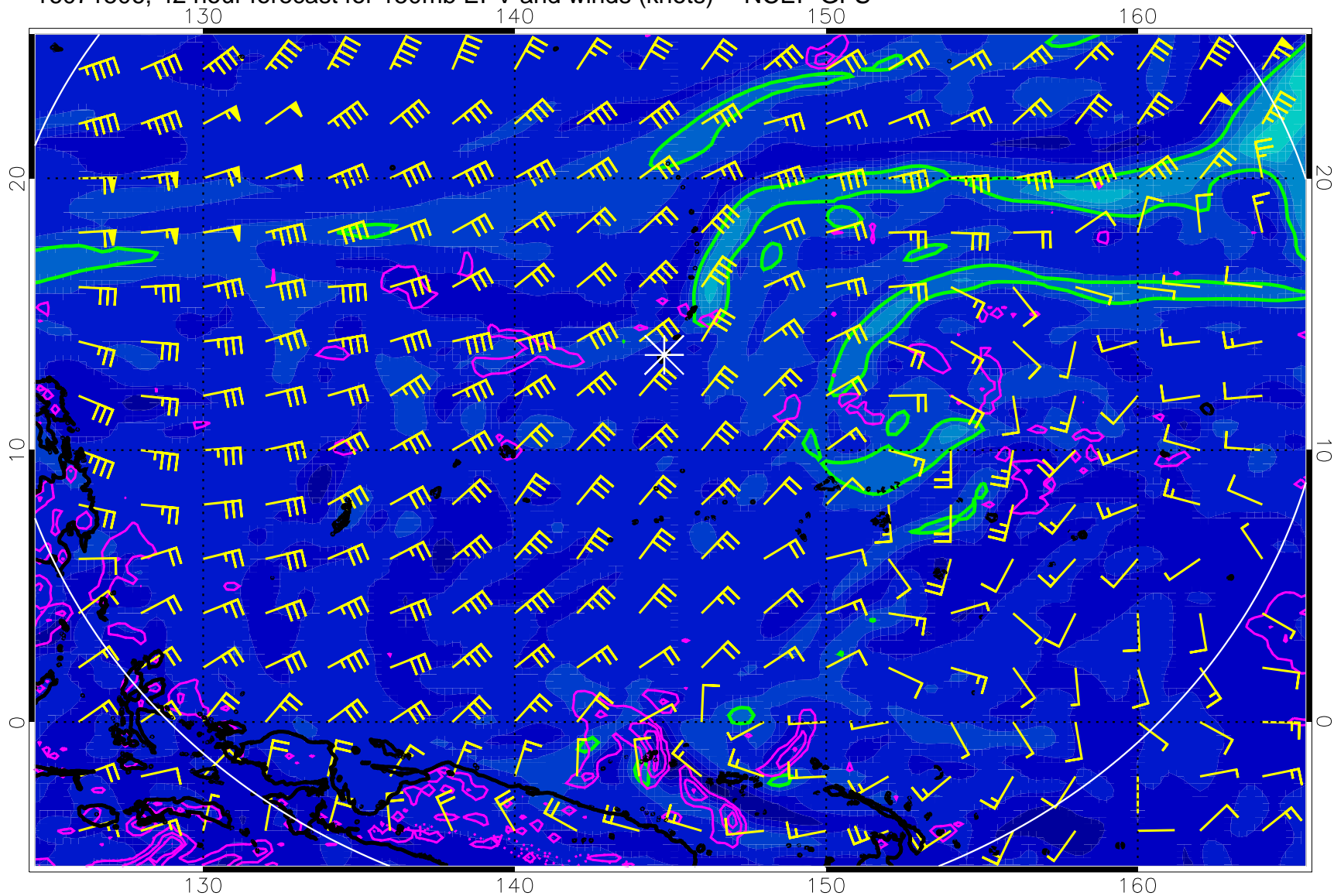
16071506, 42 hour forecast for 150mb EPV and winds (knots) -- NCEP GFS
