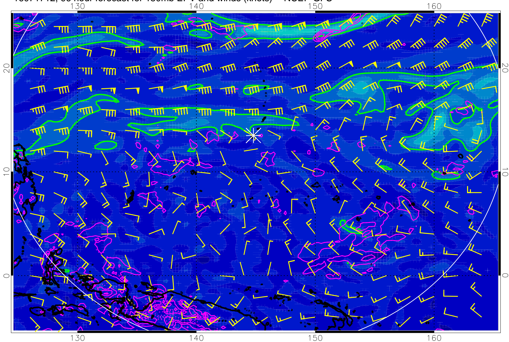
16071712, 96 hour forecast for 150mb EPV and winds (knots) -- NCEP GFS
