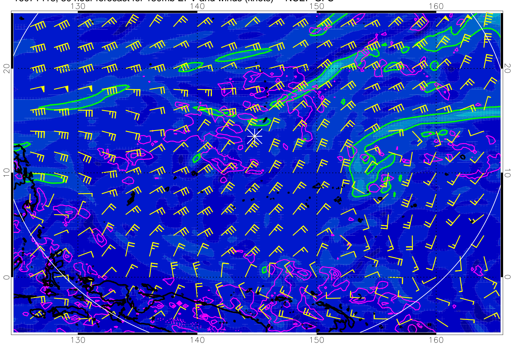
16071418, 30 hour forecast for 150mb EPV and winds (knots) -- NCEP GFS
