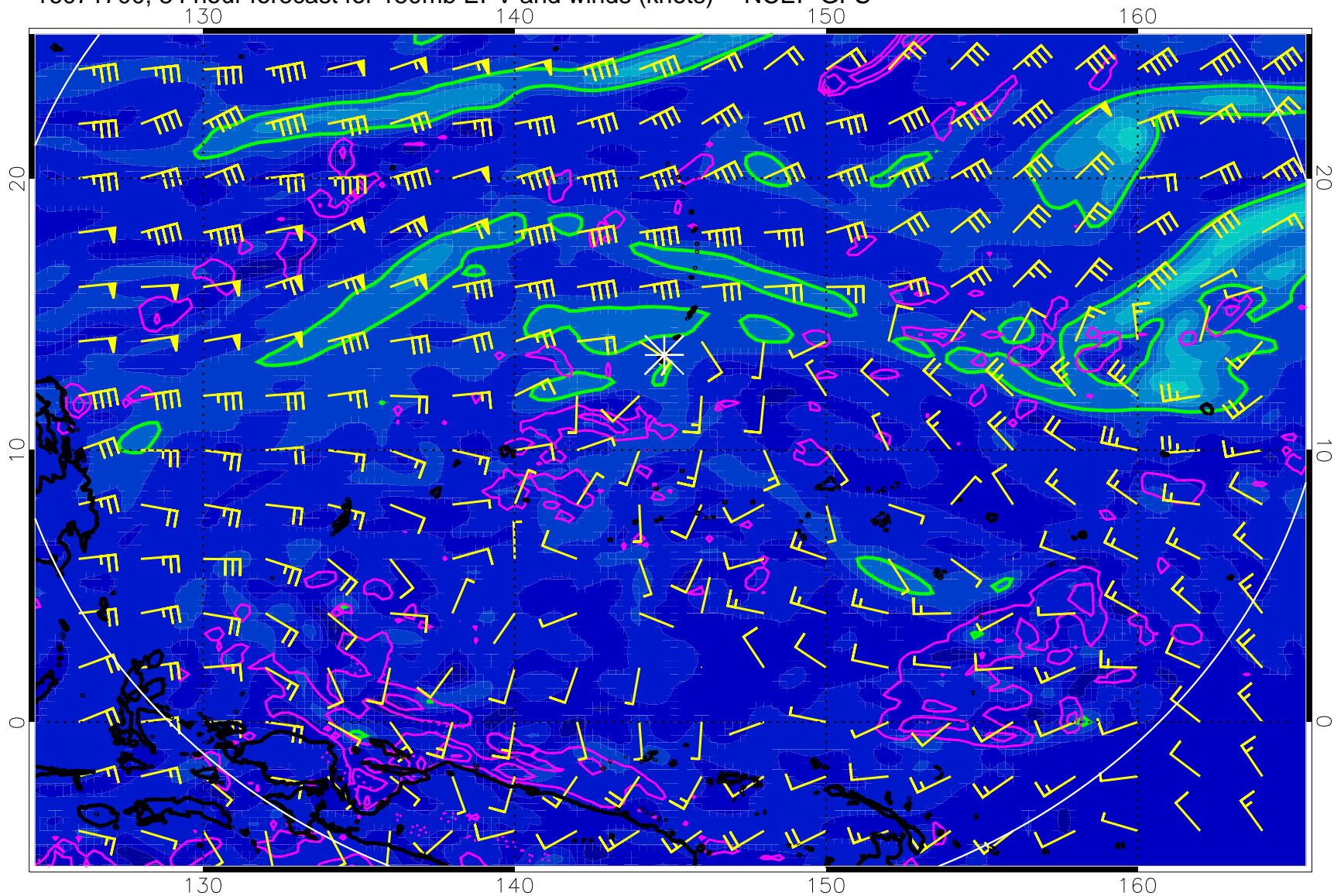
16071700, 84 hour forecast for 150mb EPV and winds (knots) -- NCEP GFS
