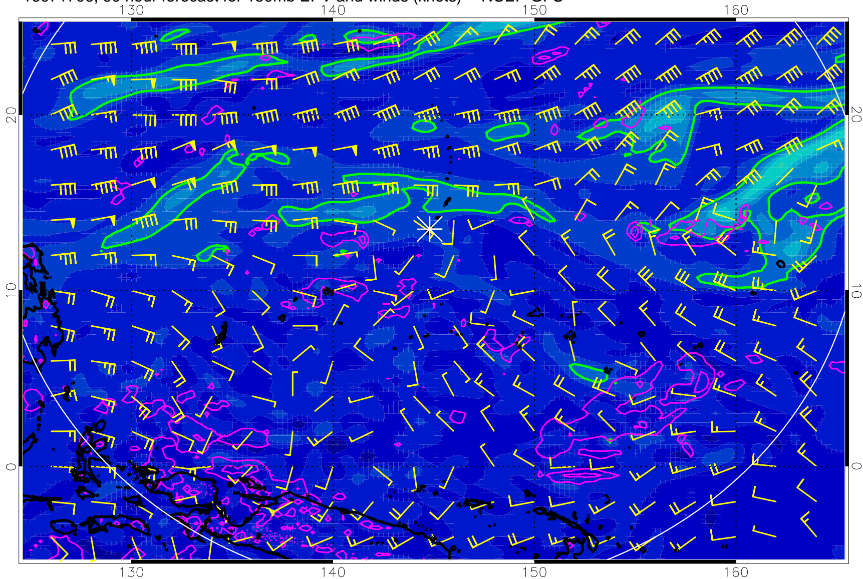
16071706, 90 hour forecast for 150mb EPV and winds (knots) -- NCEP GFS
