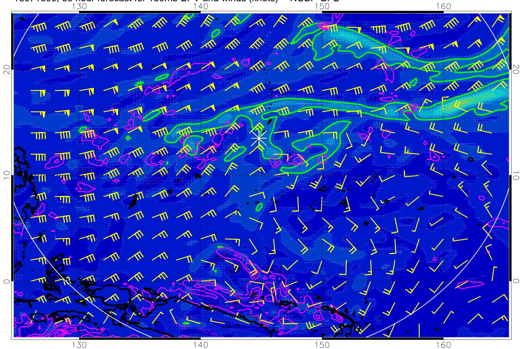
16071600, 60 hour forecast for 150mb EPV and winds (knots) -- NCEP GFS
