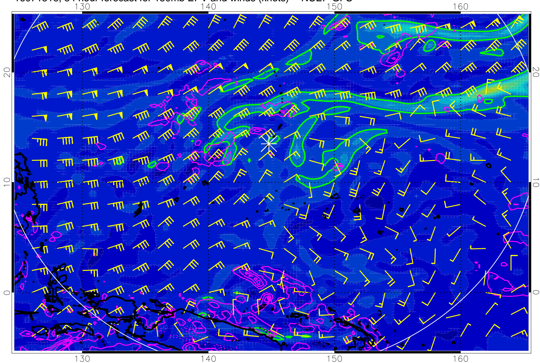
16071518, 54 hour forecast for 150mb EPV and winds (knots) -- NCEP GFS
