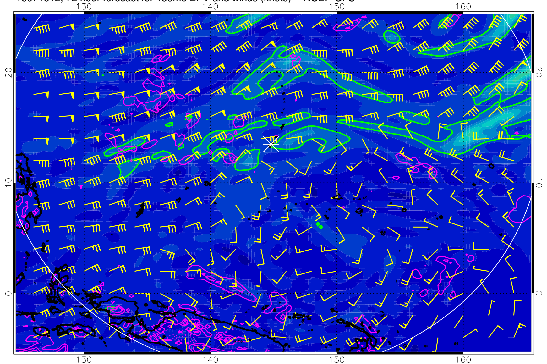
16071612, 72 hour forecast for 150mb EPV and winds (knots) -- NCEP GFS
