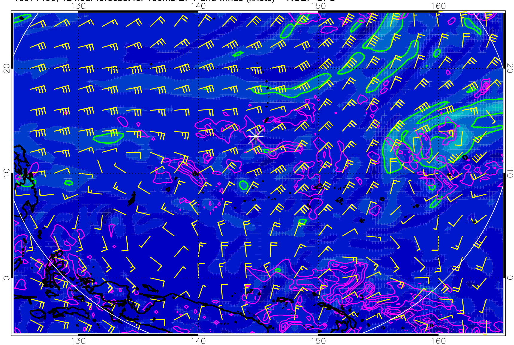
16071400, 12 hour forecast for 150mb EPV and winds (knots) -- NCEP GFS
