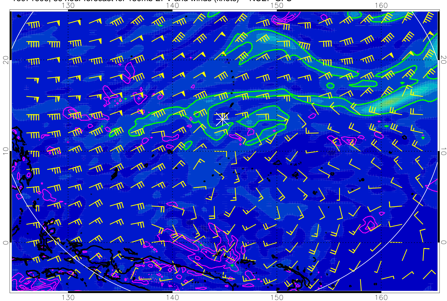
16071606, 66 hour forecast for 150mb EPV and winds (knots) -- NCEP GFS
