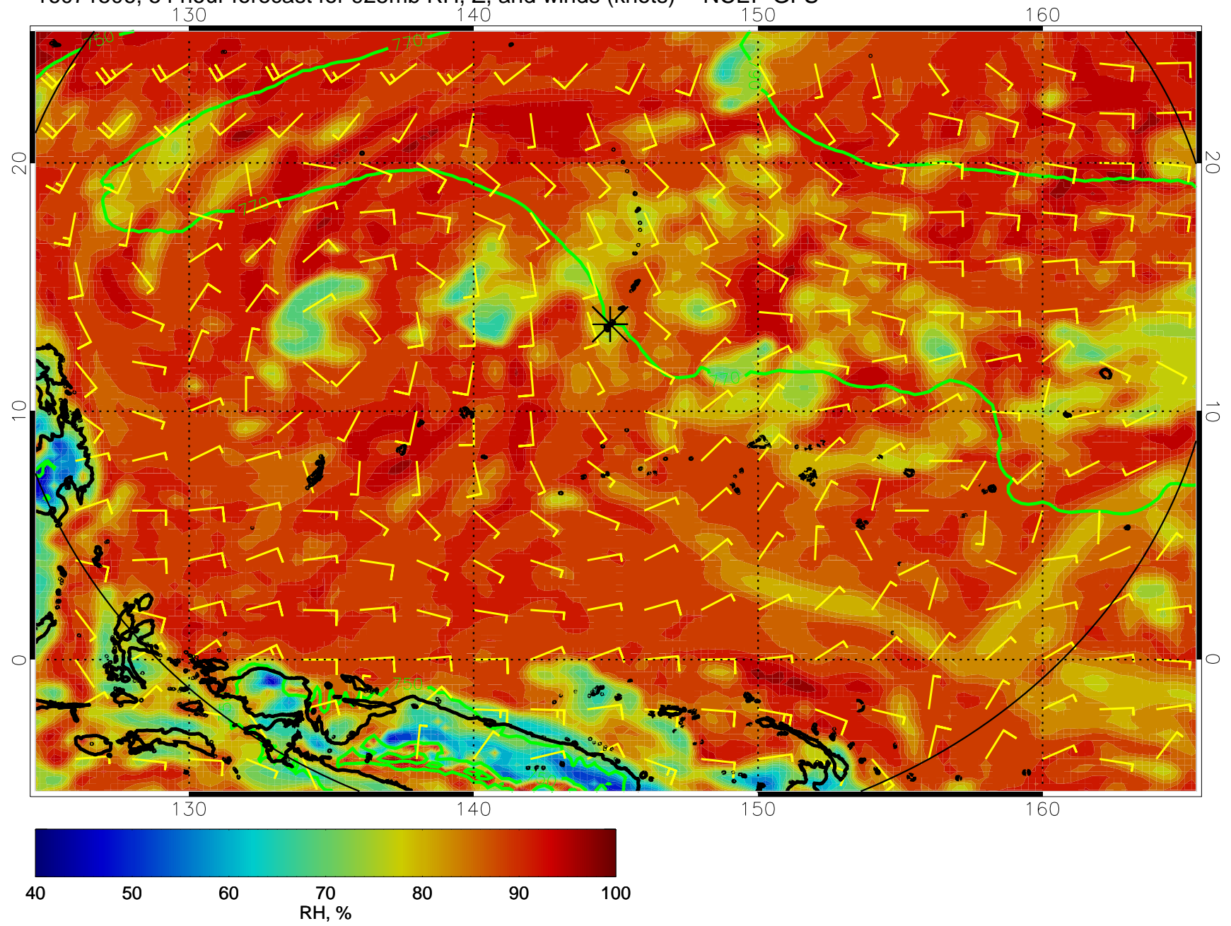
16071506, 54 hour forecast for 925mb RH, Z, and winds (knots) -- NCEP GFS
