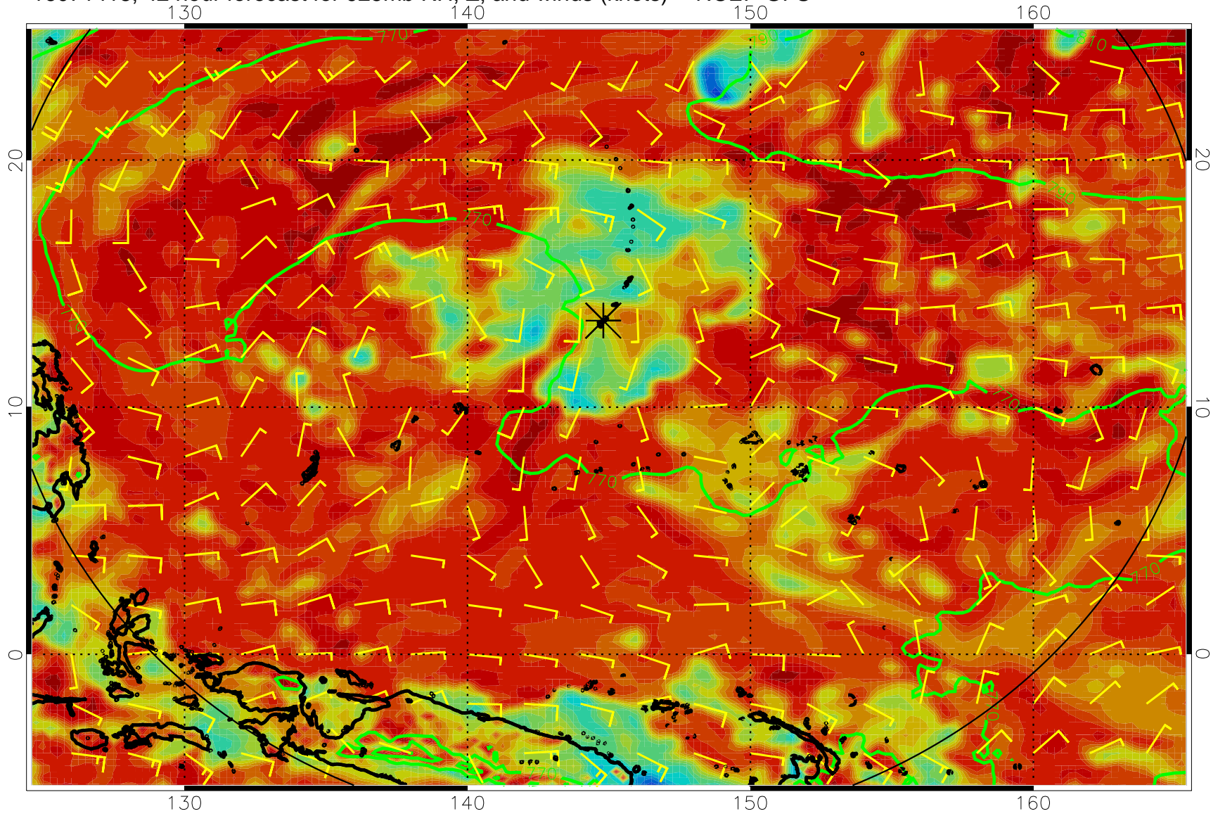
16071418, 42 hour forecast for 925mb RH, Z, and winds (knots) -- NCEP GFS
