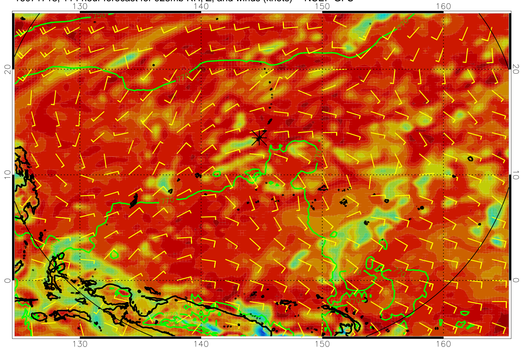
16071718, 114 hour forecast for 925mb RH, Z, and winds (knots) -- NCEP GFS
