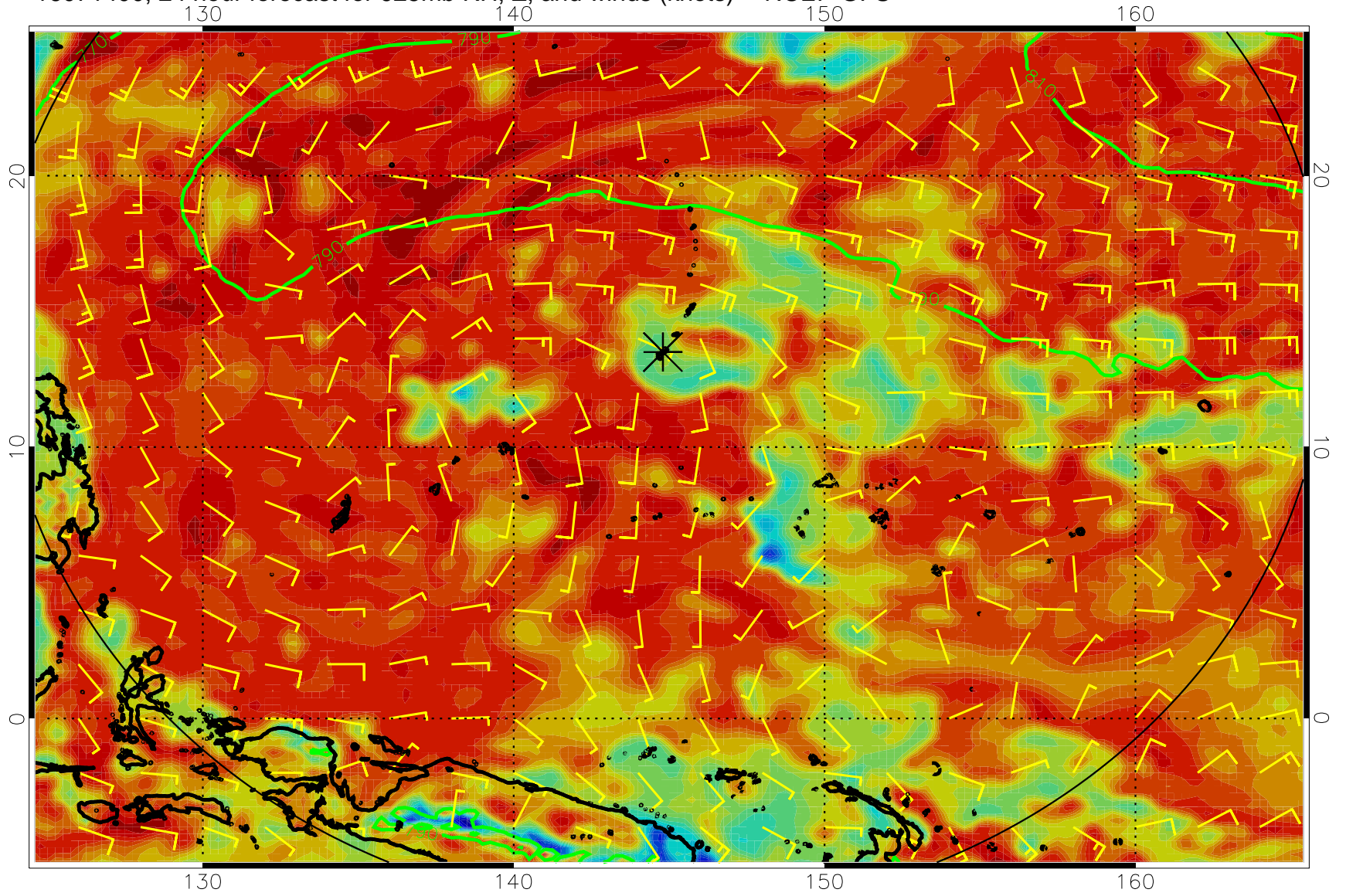
16071400, 24 hour forecast for 925mb RH, Z, and winds (knots) -- NCEP GFS
