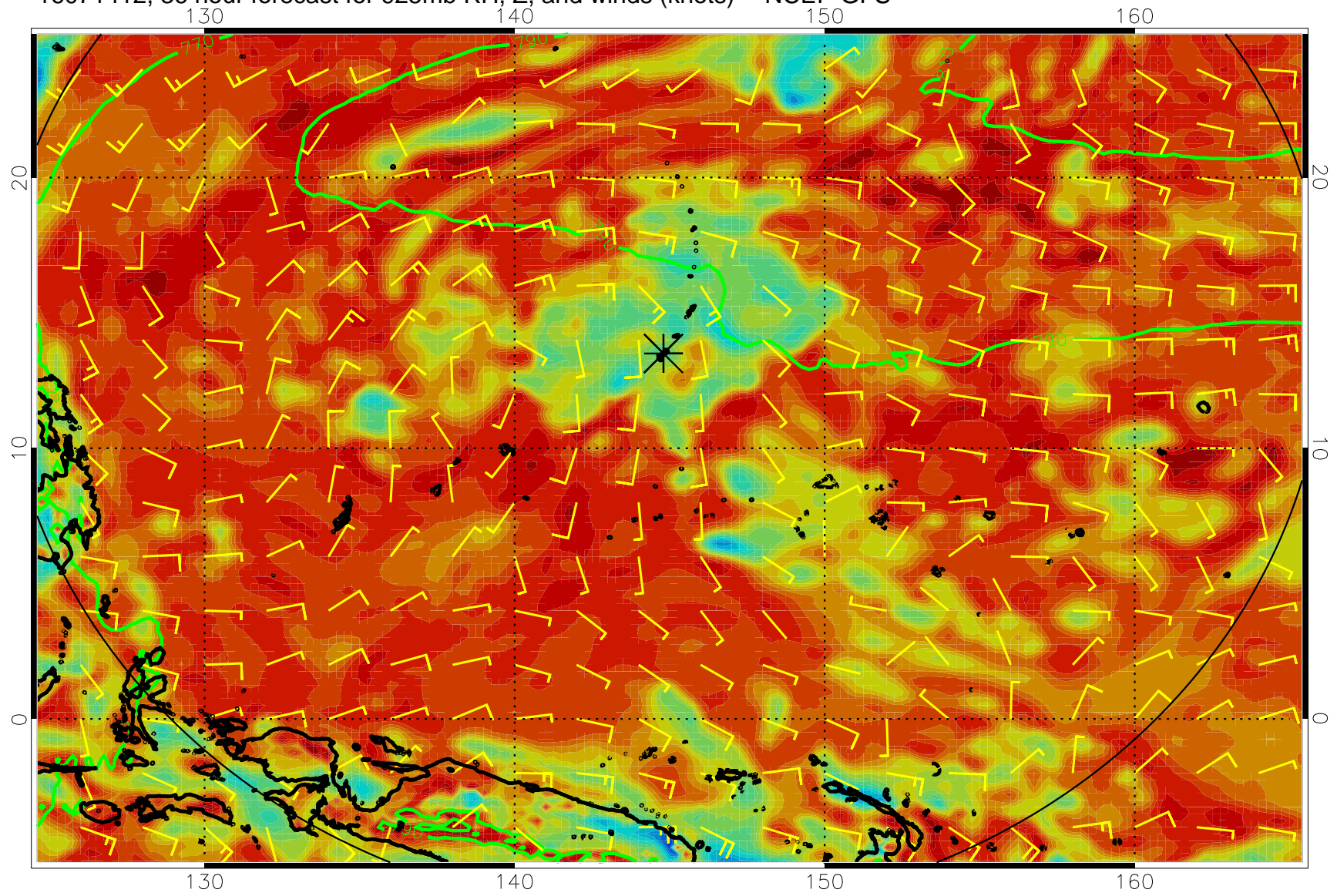
16071412, 36 hour forecast for 925mb RH, Z, and winds (knots) -- NCEP GFS
