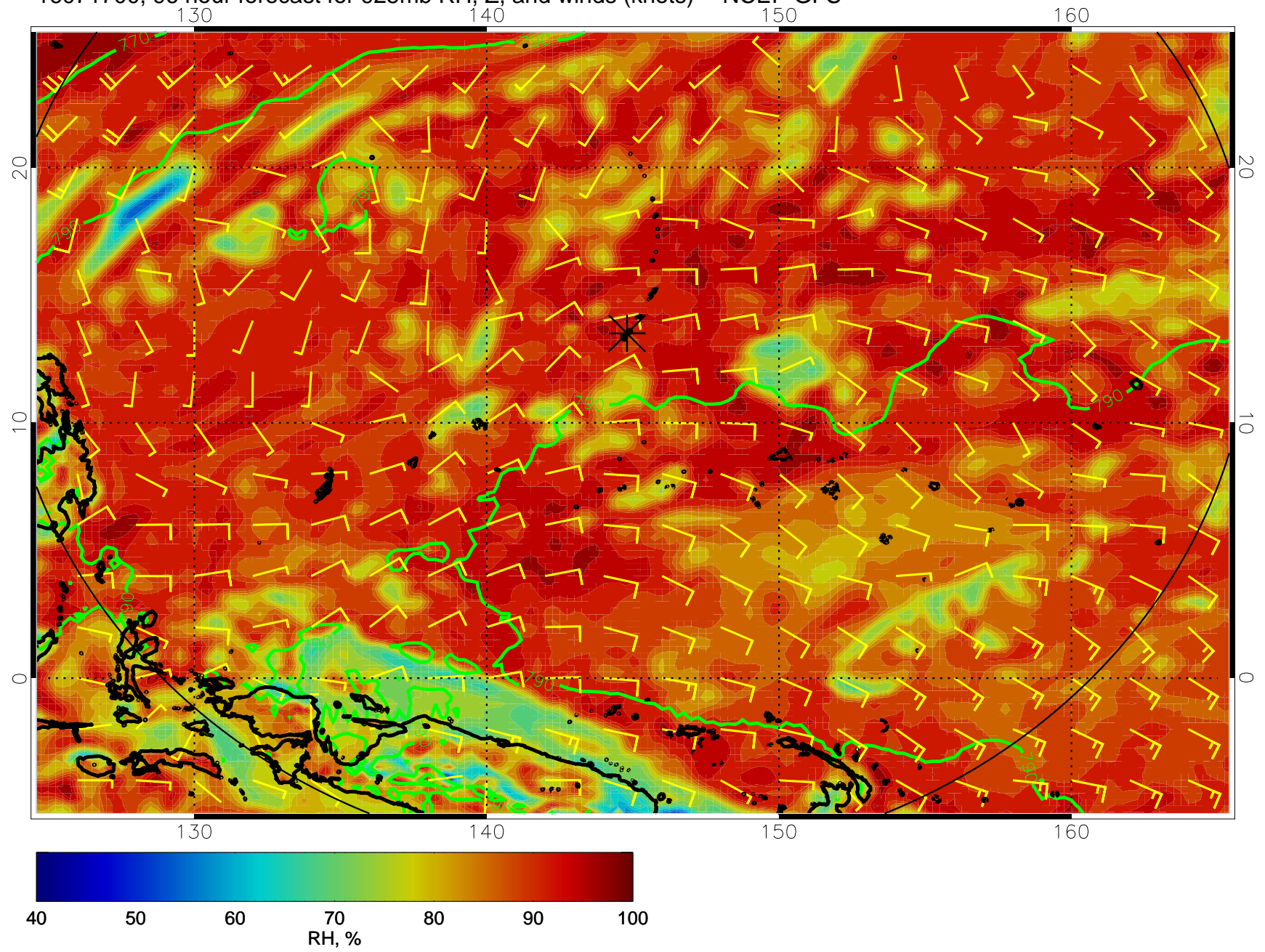
16071700, 96 hour forecast for 925mb RH, Z, and winds (knots) -- NCEP GFS
