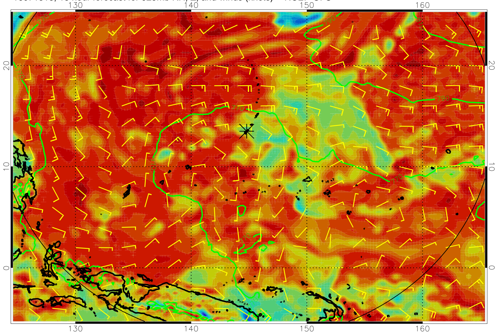
16071318, 18 hour forecast for 925mb RH, Z, and winds (knots) -- NCEP GFS
