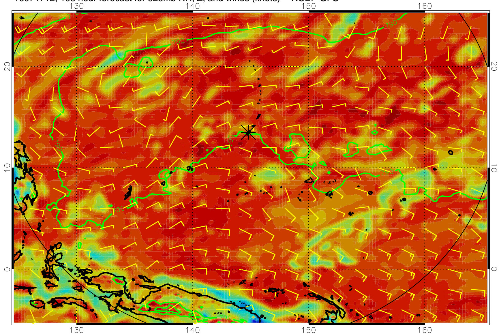
16071712, 108 hour forecast for 925mb RH, Z, and winds (knots) -- NCEP GFS
