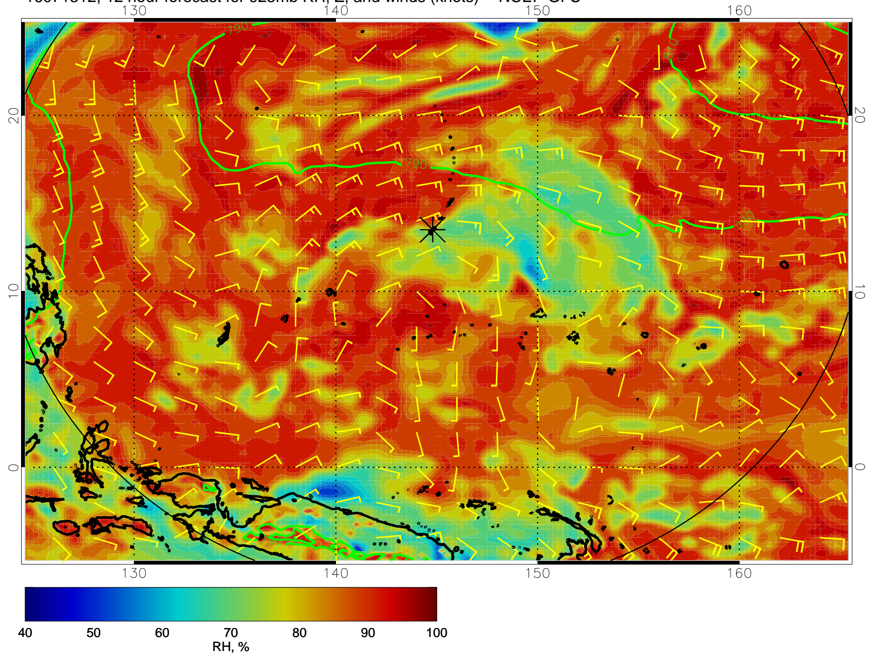
16071312, 12 hour forecast for 925mb RH, Z, and winds (knots) -- NCEP GFS
