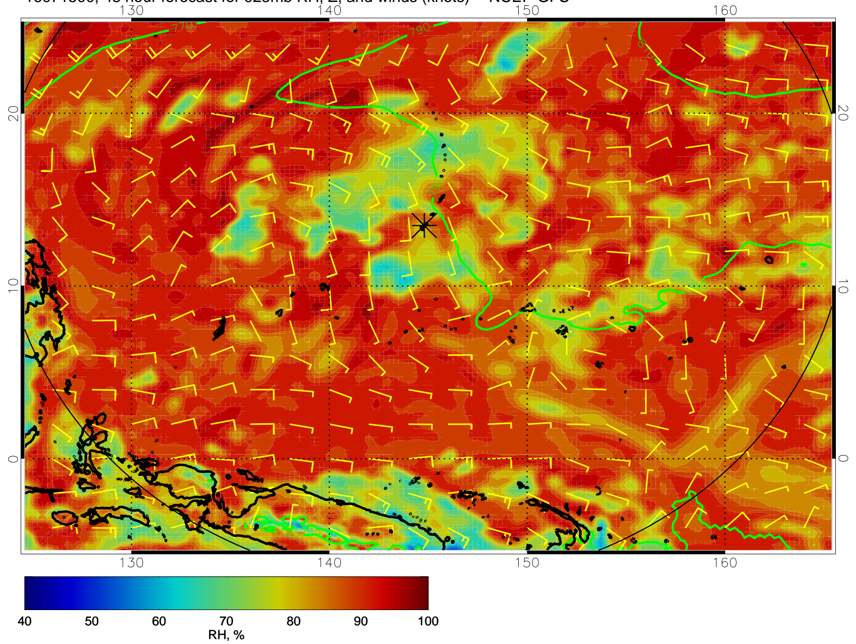
16071500, 48 hour forecast for 925mb RH, Z, and winds (knots) -- NCEP GFS
