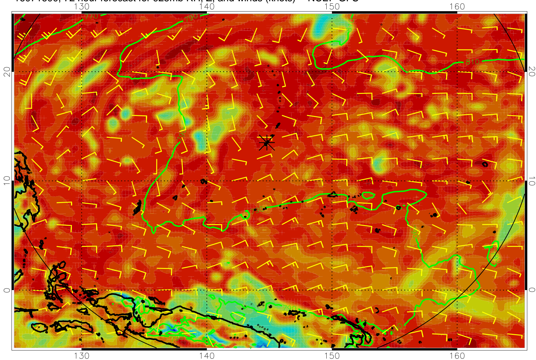
16071600, 72 hour forecast for 925mb RH, Z, and winds (knots) -- NCEP GFS
