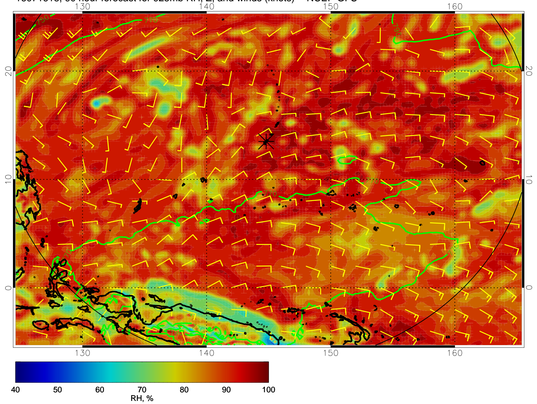
16071618, 90 hour forecast for 925mb RH, Z, and winds (knots) -- NCEP GFS
