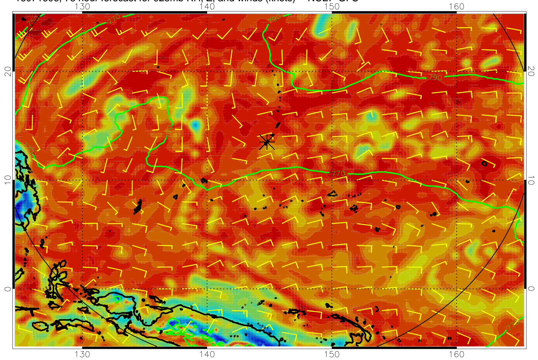
16071606, 78 hour forecast for 925mb RH, Z, and winds (knots) -- NCEP GFS
