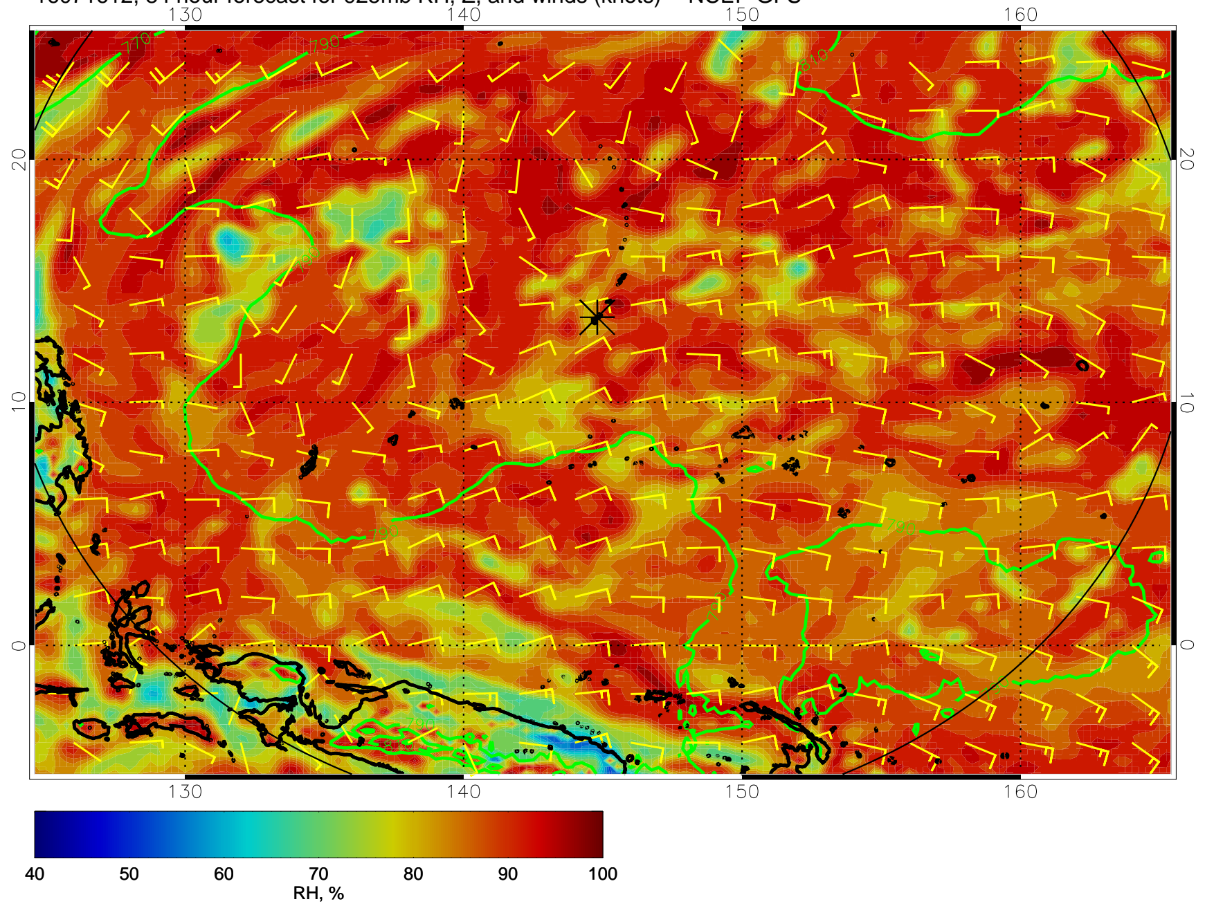
16071612, 84 hour forecast for 925mb RH, Z, and winds (knots) -- NCEP GFS
