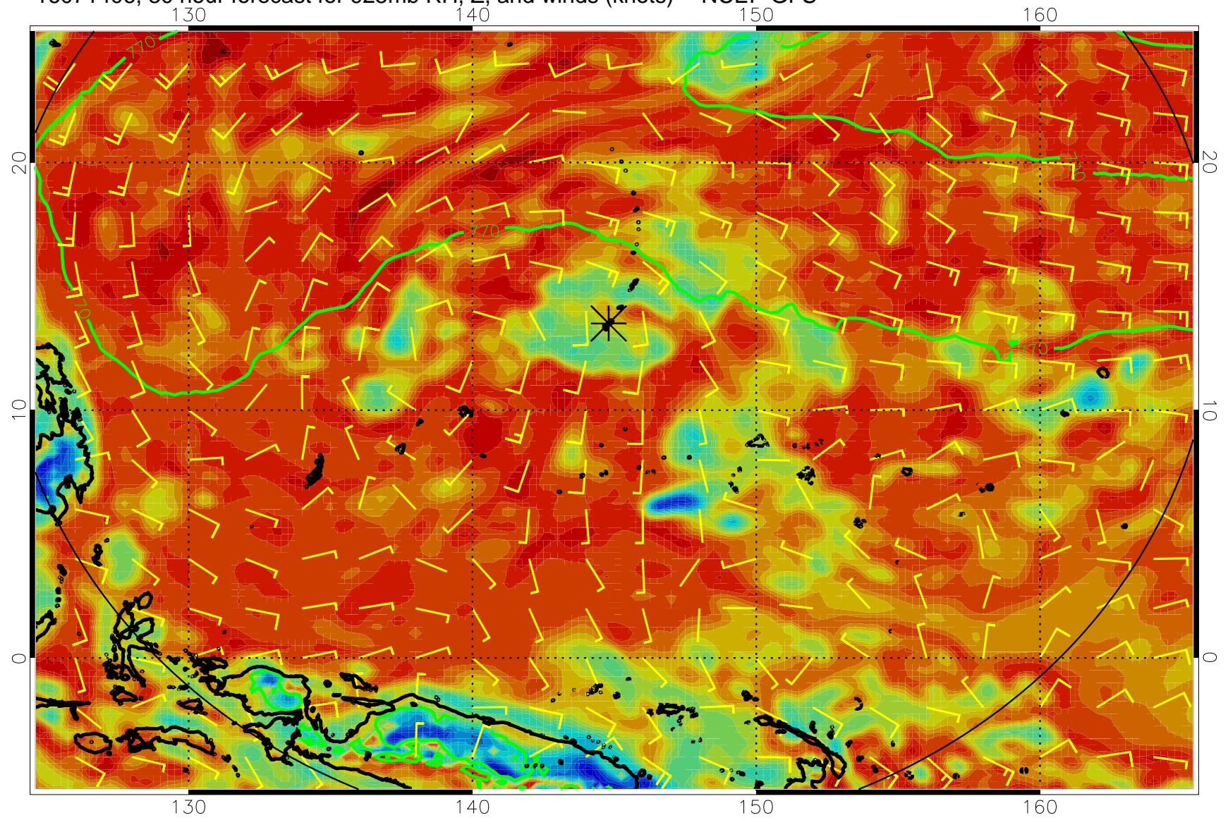
16071406, 30 hour forecast for 925mb RH, Z, and winds (knots) -- NCEP GFS
