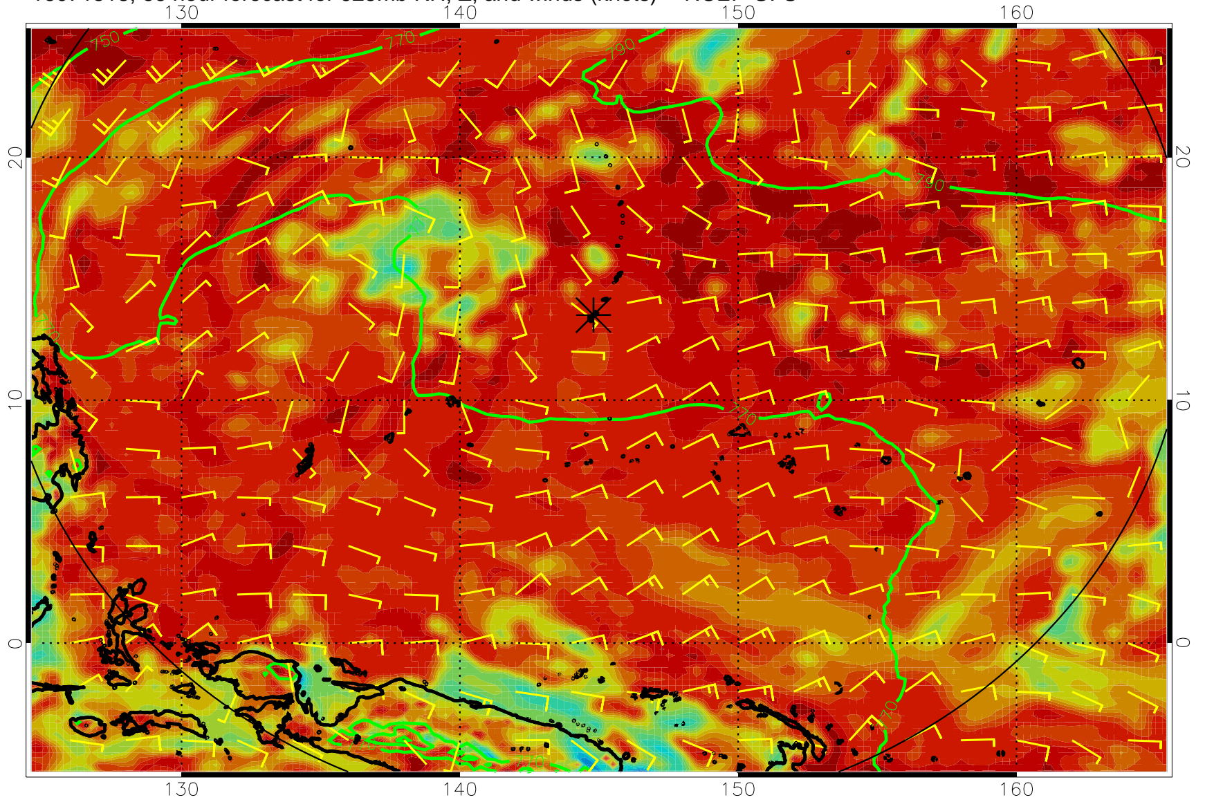
16071518, 66 hour forecast for 925mb RH, Z, and winds (knots) -- NCEP GFS
