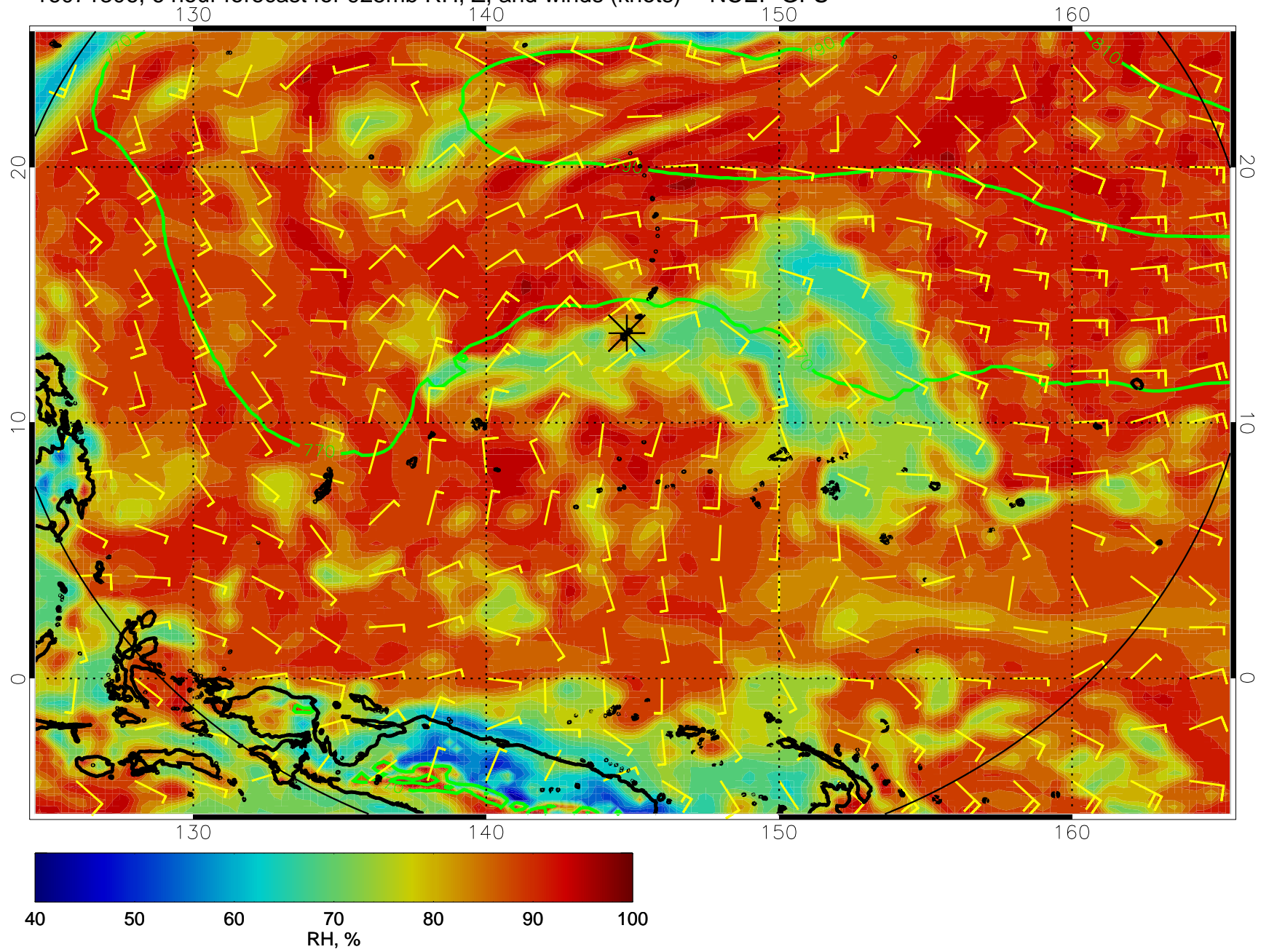
16071306, 6 hour forecast for 925mb RH, Z, and winds (knots) -- NCEP GFS
