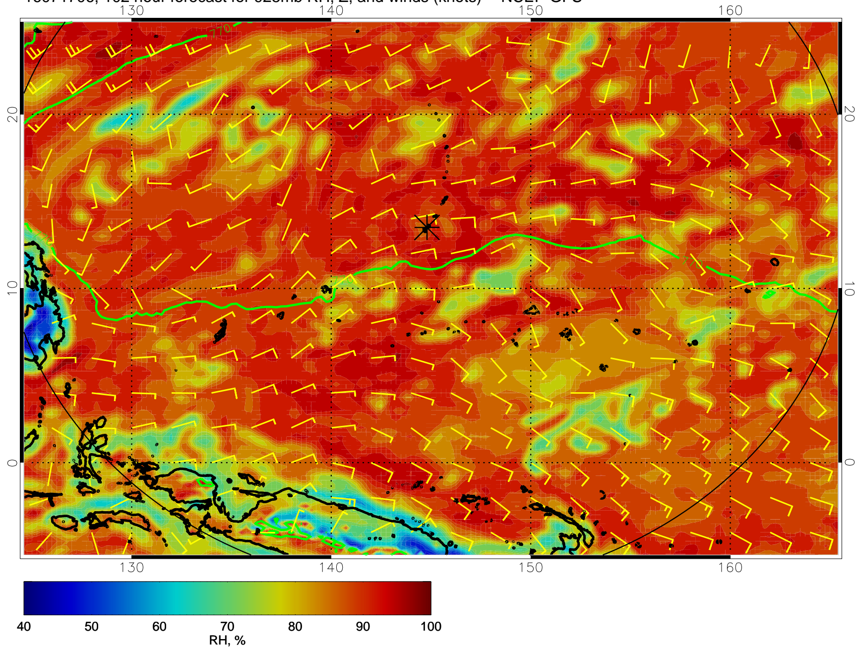
16071706, 102 hour forecast for 925mb RH, Z, and winds (knots) -- NCEP GFS
