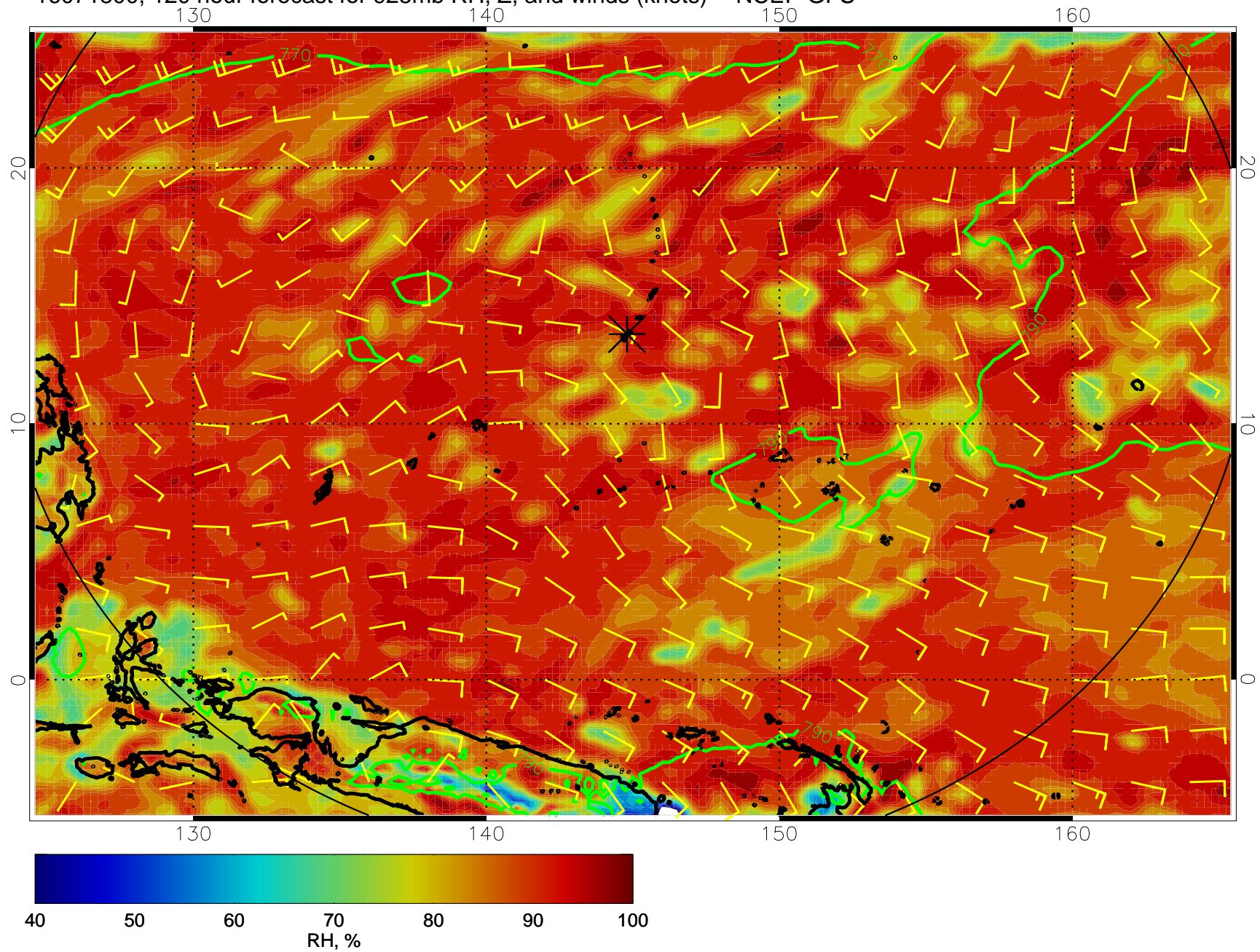
16071800, 120 hour forecast for 925mb RH, Z, and winds (knots) -- NCEP GFS
