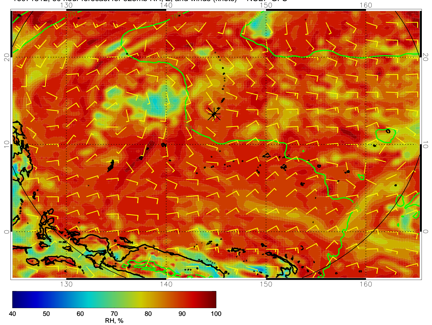
16071512, 60 hour forecast for 925mb RH, Z, and winds (knots) -- NCEP GFS
