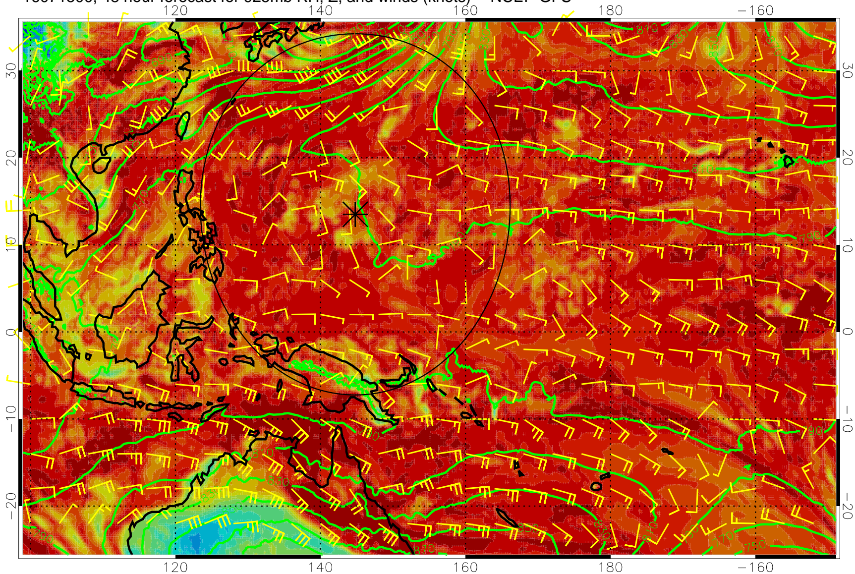
16071500, 48 hour forecast for 925mb RH, Z, and winds (knots) -- NCEP GFS
