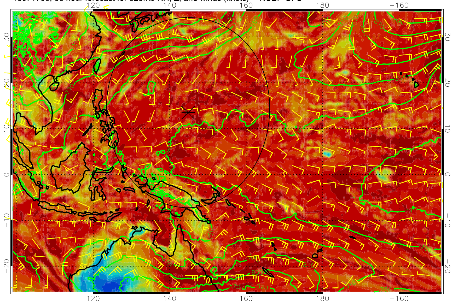
16071700, 96 hour forecast for 925mb RH, Z, and winds (knots) -- NCEP GFS
