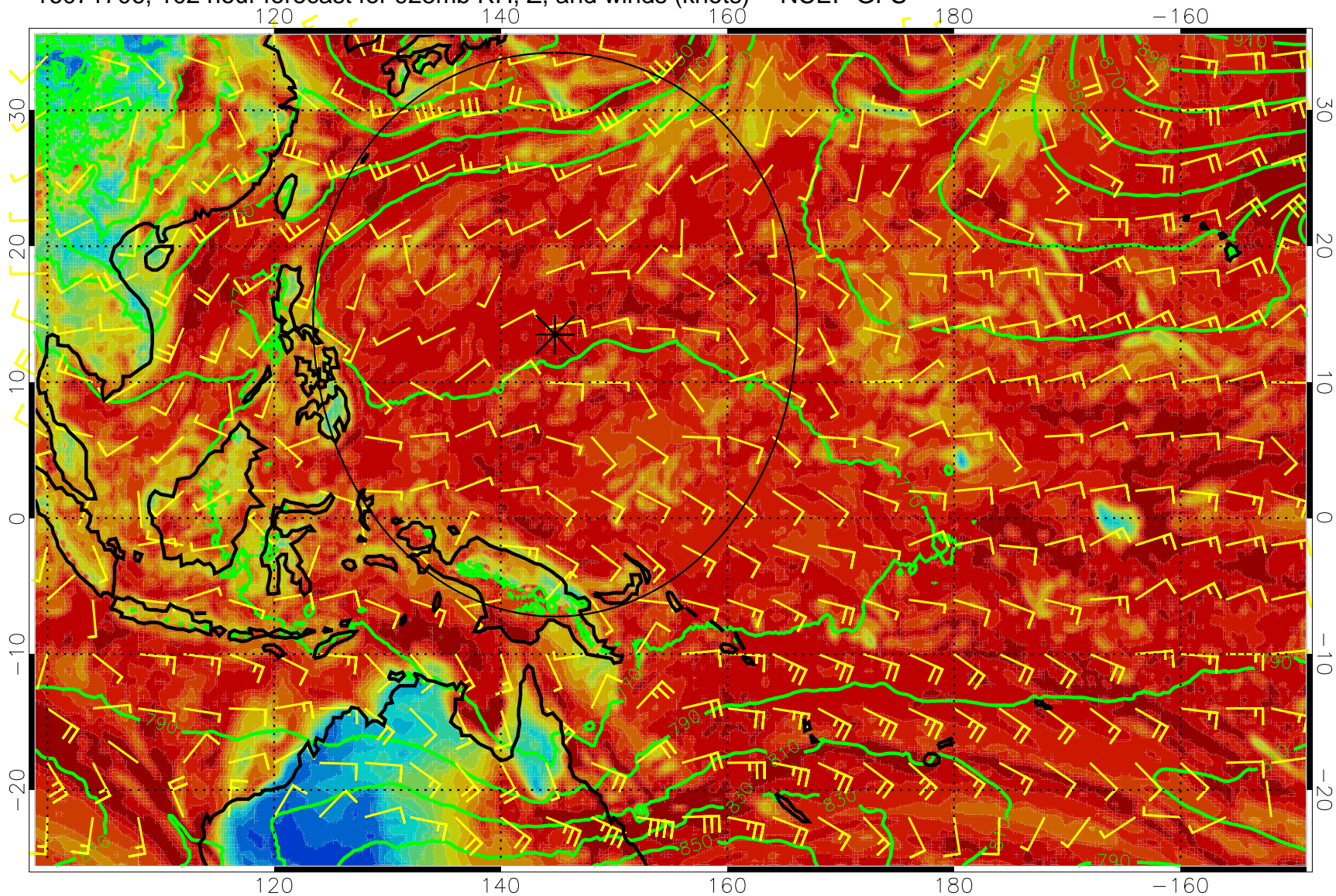
16071706, 102 hour forecast for 925mb RH, Z, and winds (knots) -- NCEP GFS
