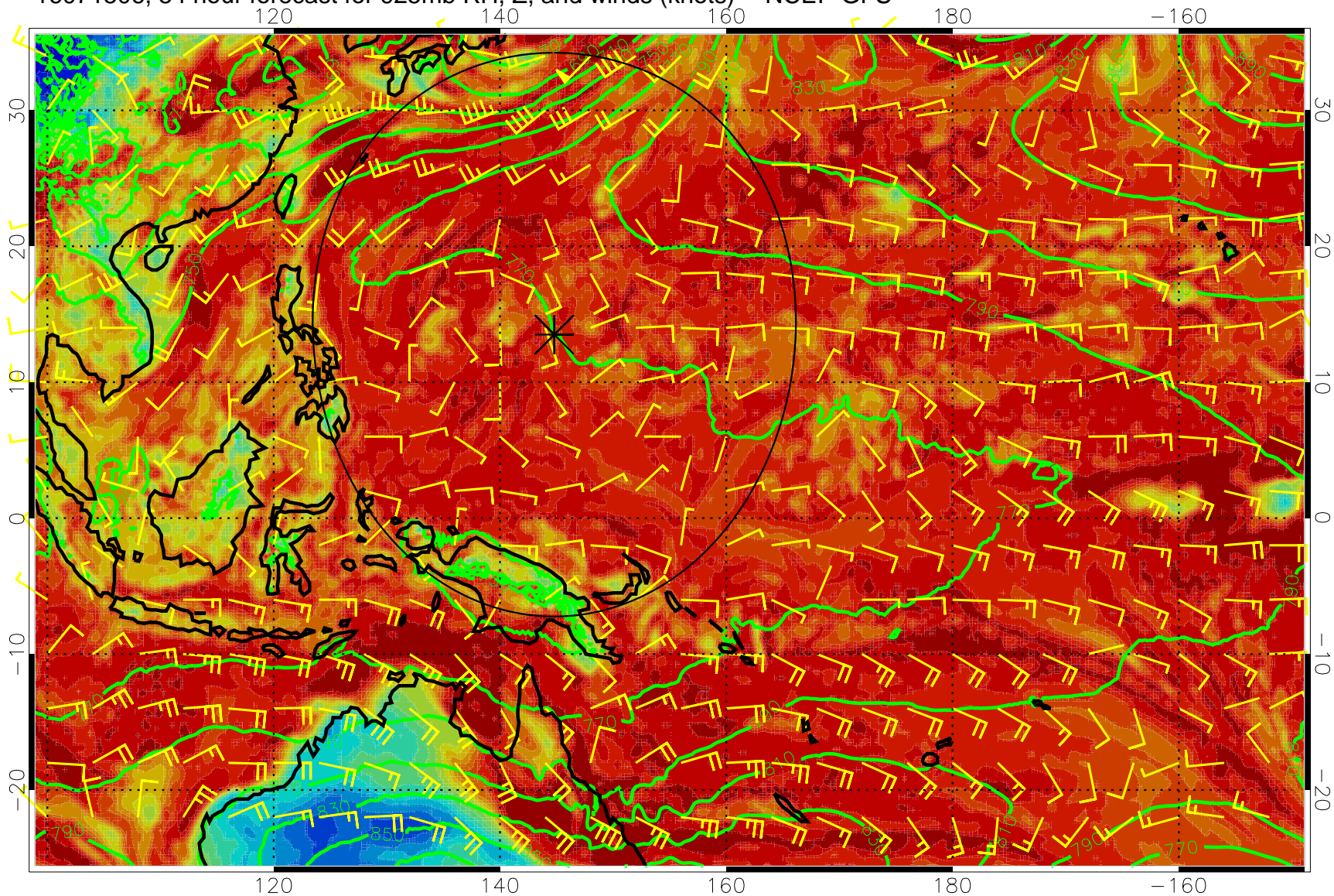
16071506, 54 hour forecast for 925mb RH, Z, and winds (knots) -- NCEP GFS
