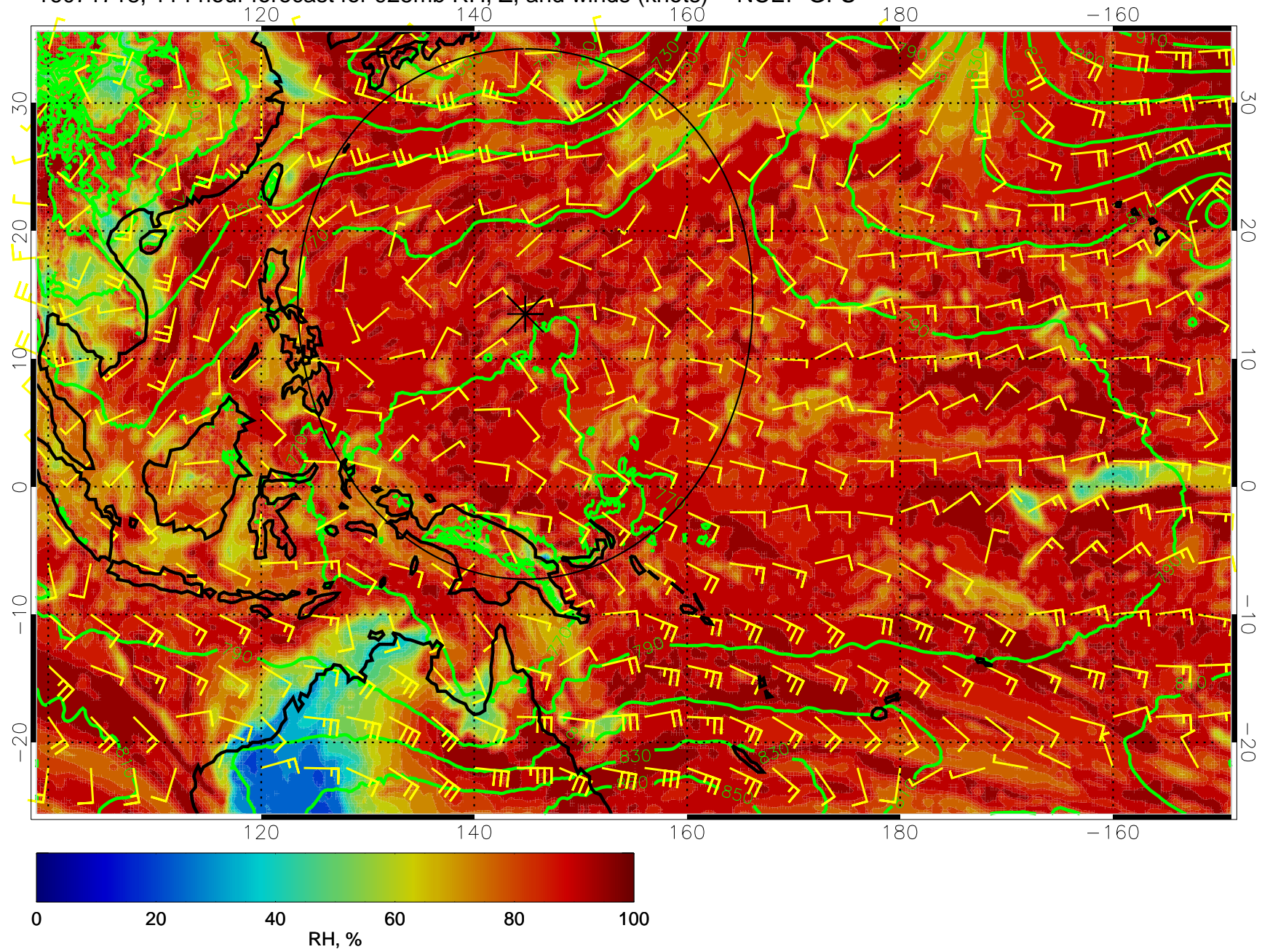
16071718, 114 hour forecast for 925mb RH, Z, and winds (knots) -- NCEP GFS
