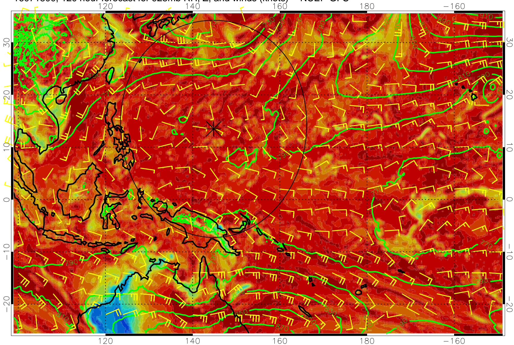
16071800, 120 hour forecast for 925mb RH, Z, and winds (knots) -- NCEP GFS
