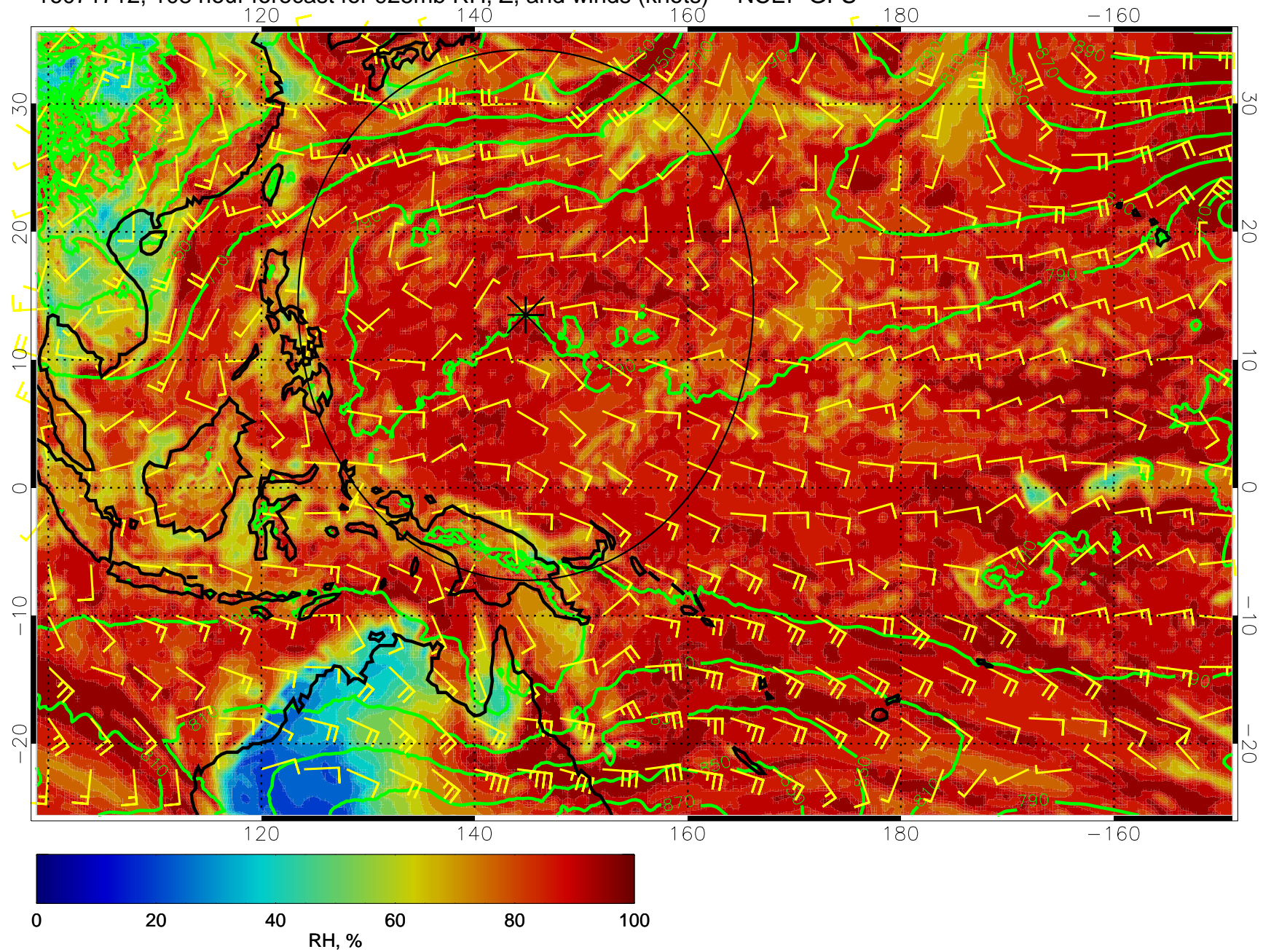
16071712, 108 hour forecast for 925mb RH, Z, and winds (knots) -- NCEP GFS
