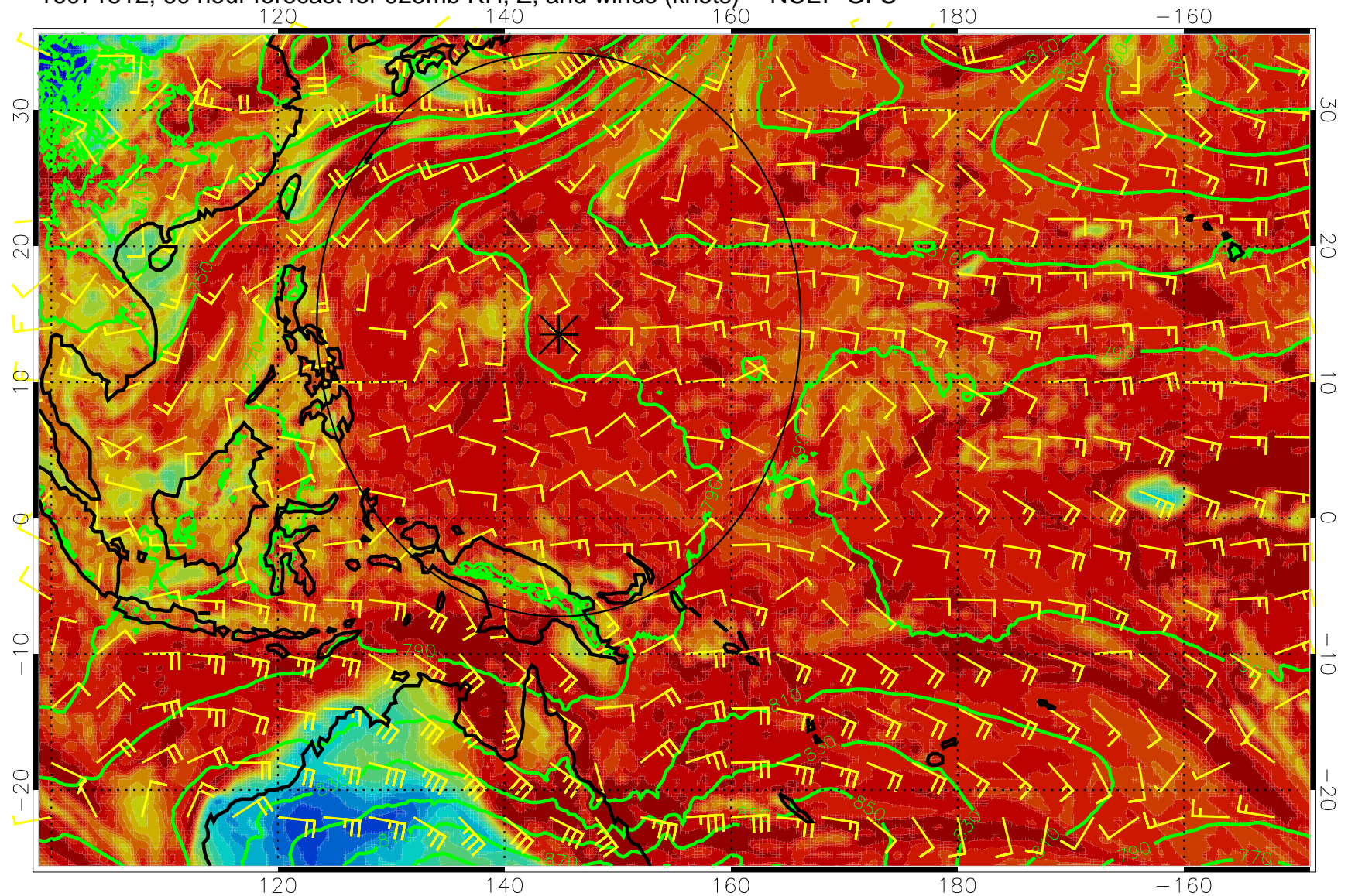
16071512, 60 hour forecast for 925mb RH, Z, and winds (knots) -- NCEP GFS
