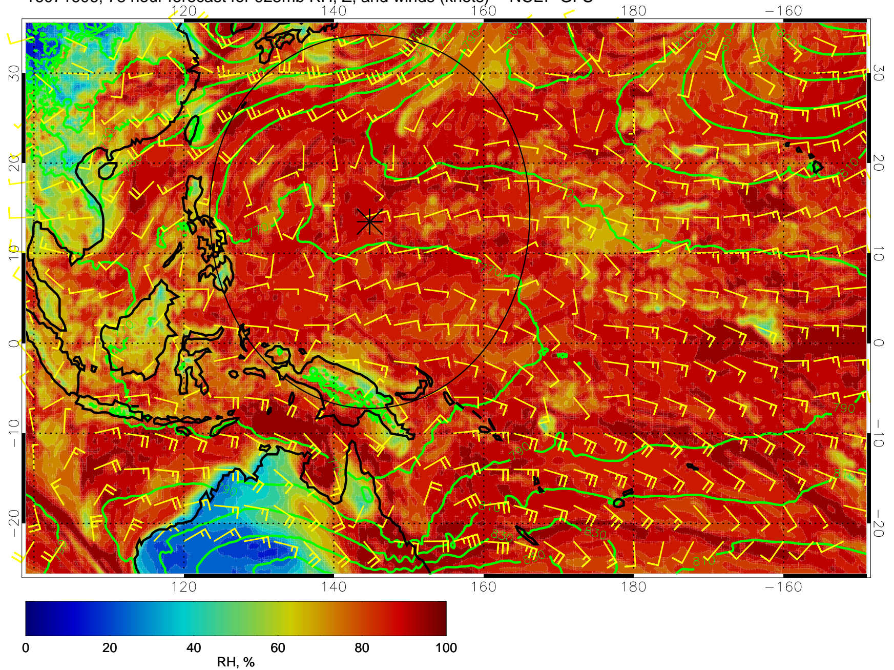
16071606, 78 hour forecast for 925mb RH, Z, and winds (knots) -- NCEP GFS
