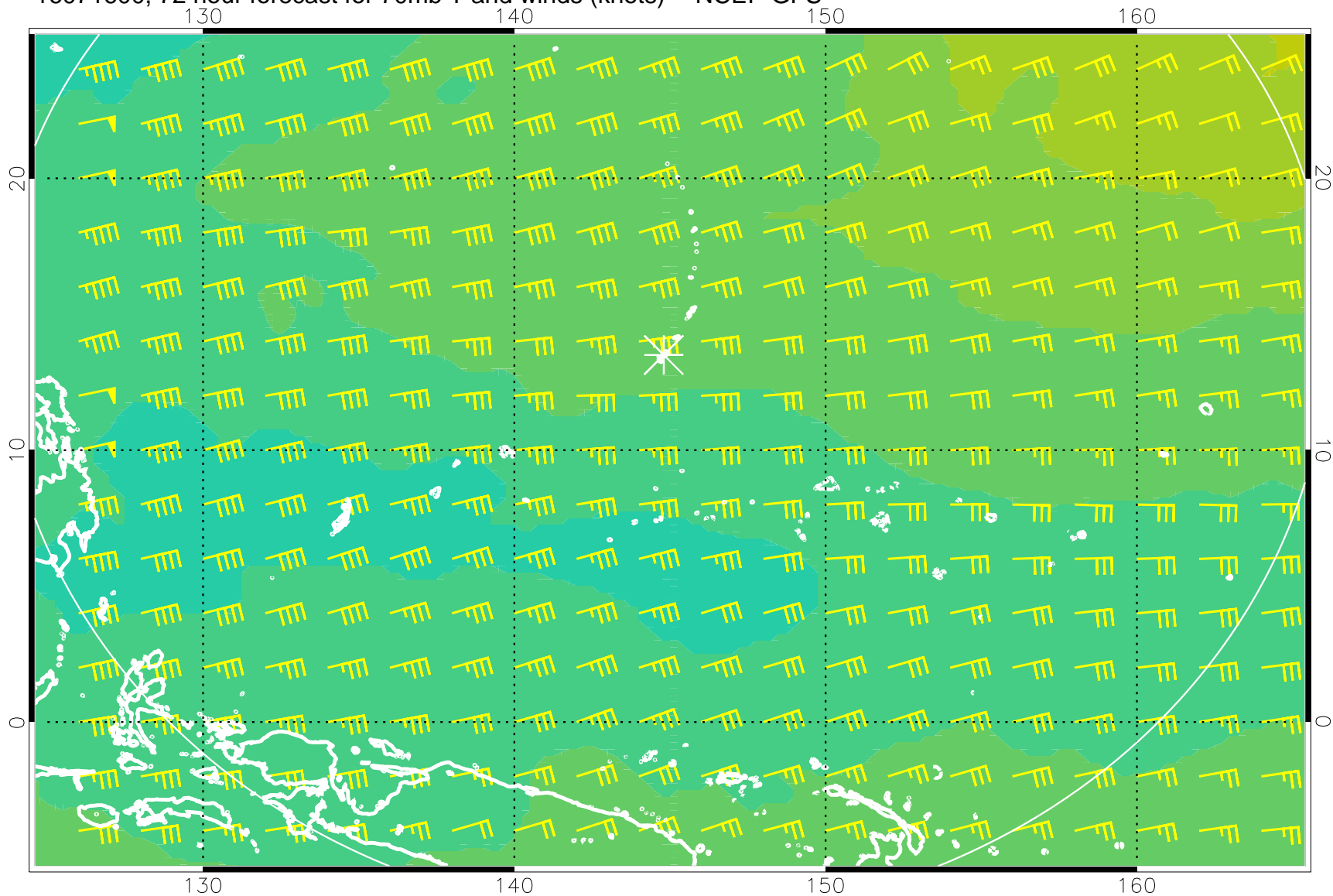
16071600, 72 hour forecast for 70mb T and winds (knots) -- NCEP GFS
