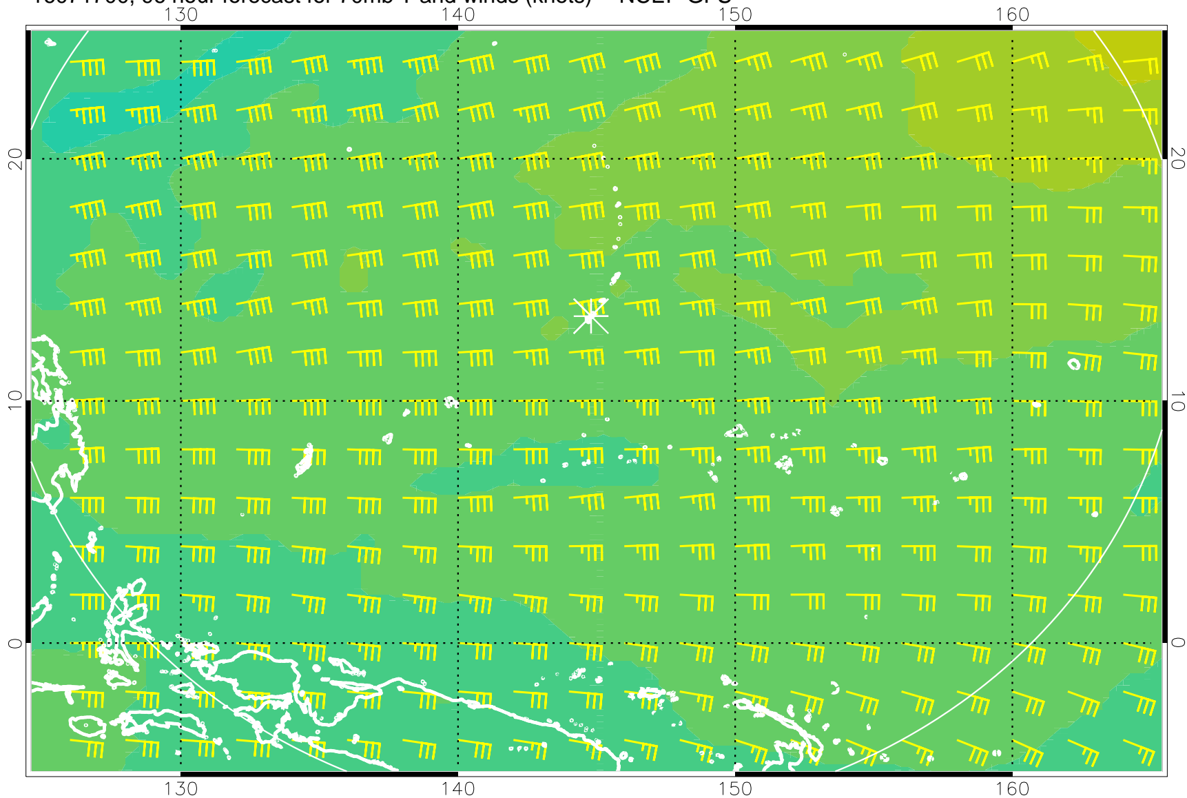
16071700, 96 hour forecast for 70mb T and winds (knots) -- NCEP GFS
