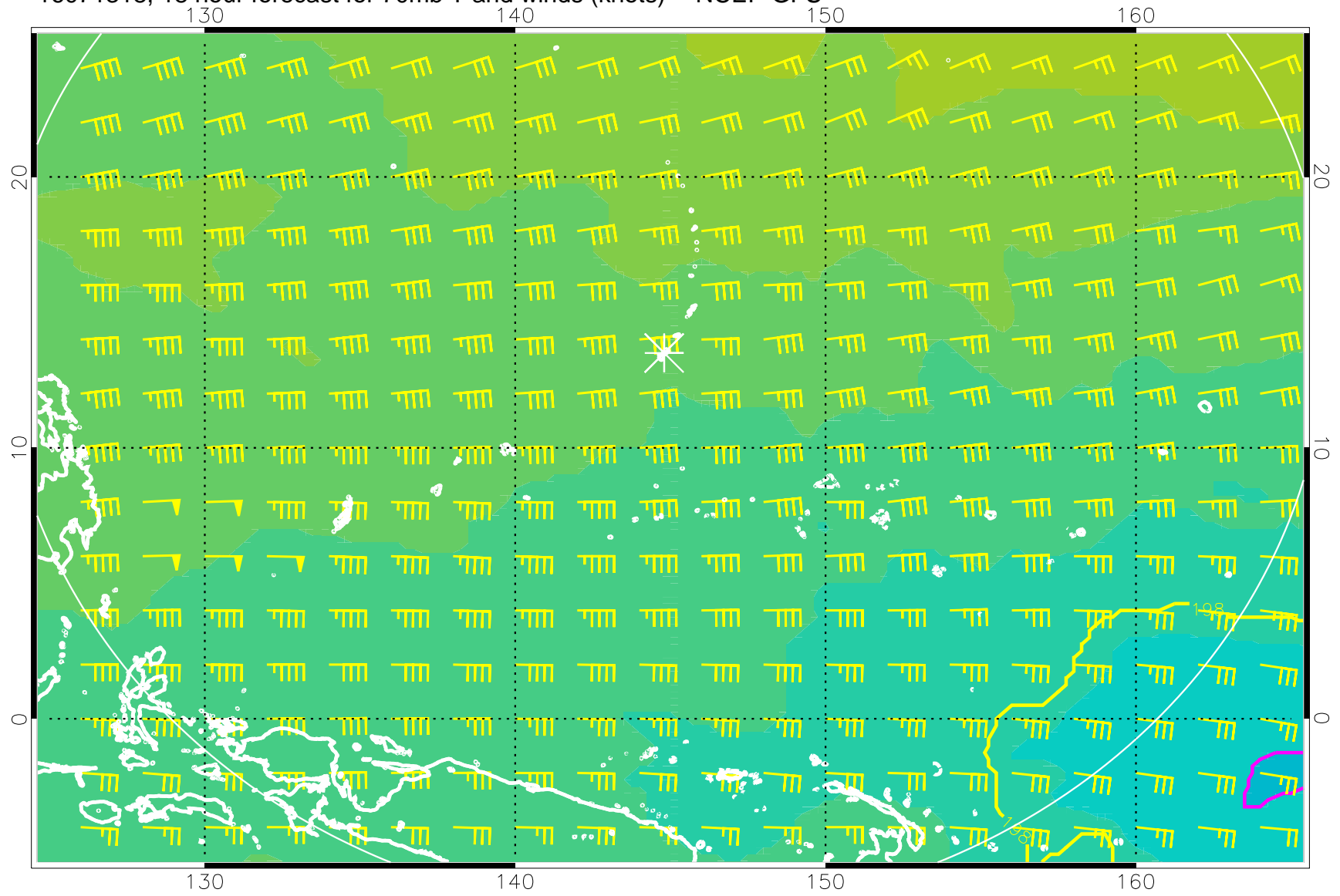
16071318, 18 hour forecast for 70mb T and winds (knots) -- NCEP GFS
