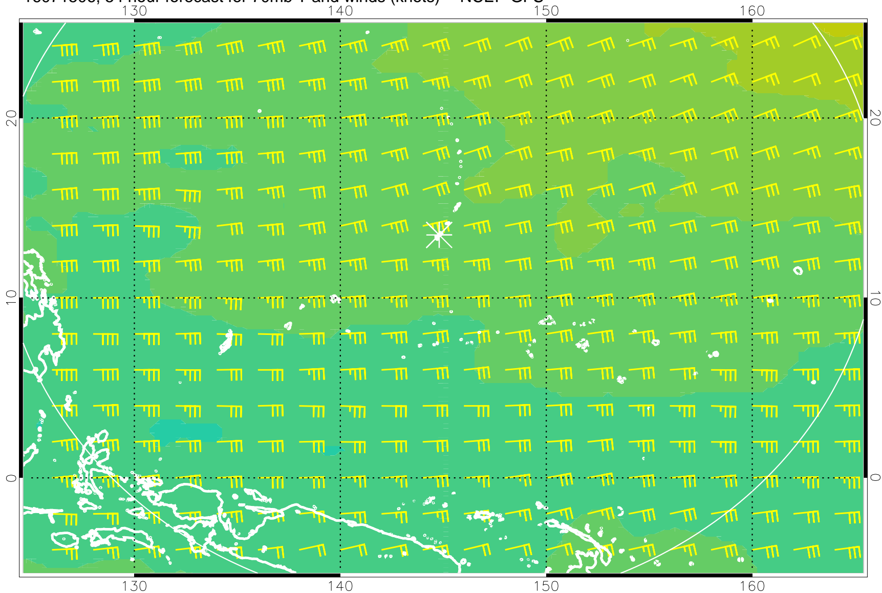
16071506, 54 hour forecast for 70mb T and winds (knots) -- NCEP GFS
