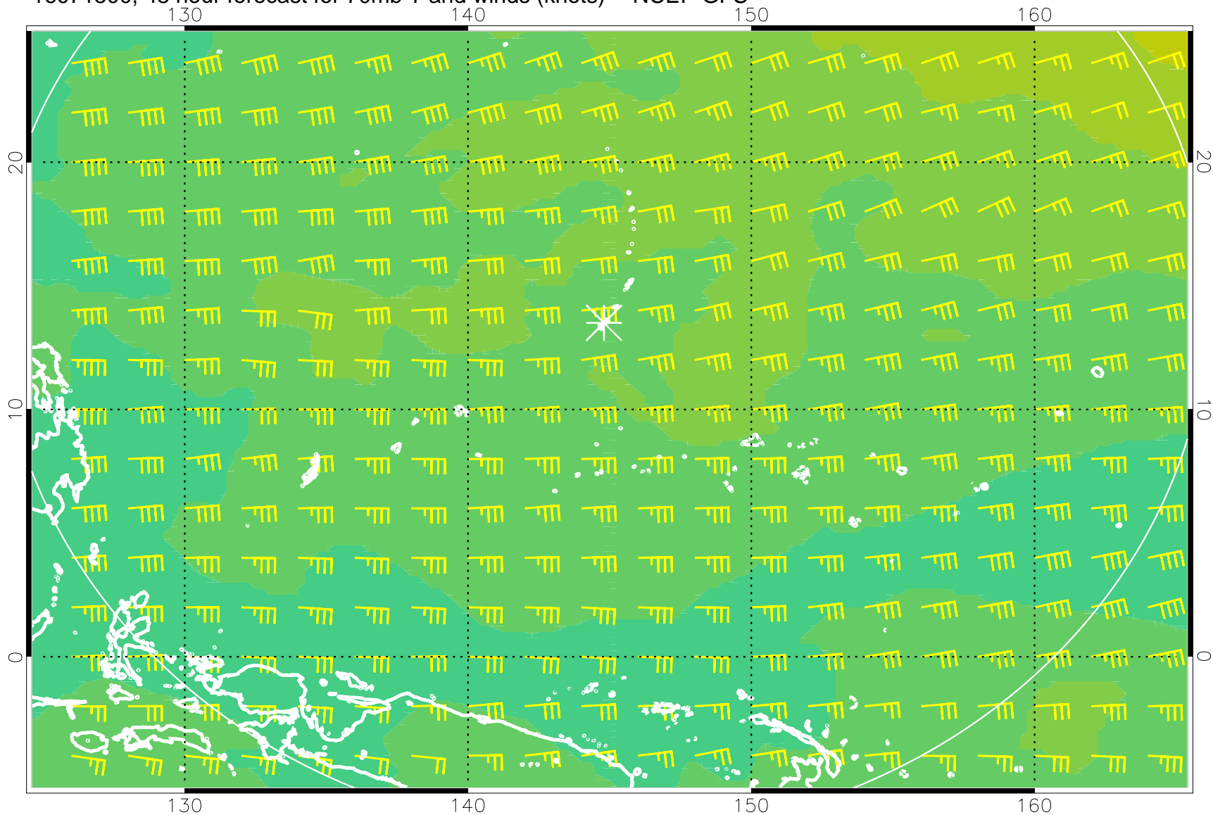
16071500, 48 hour forecast for 70mb T and winds (knots) -- NCEP GFS
