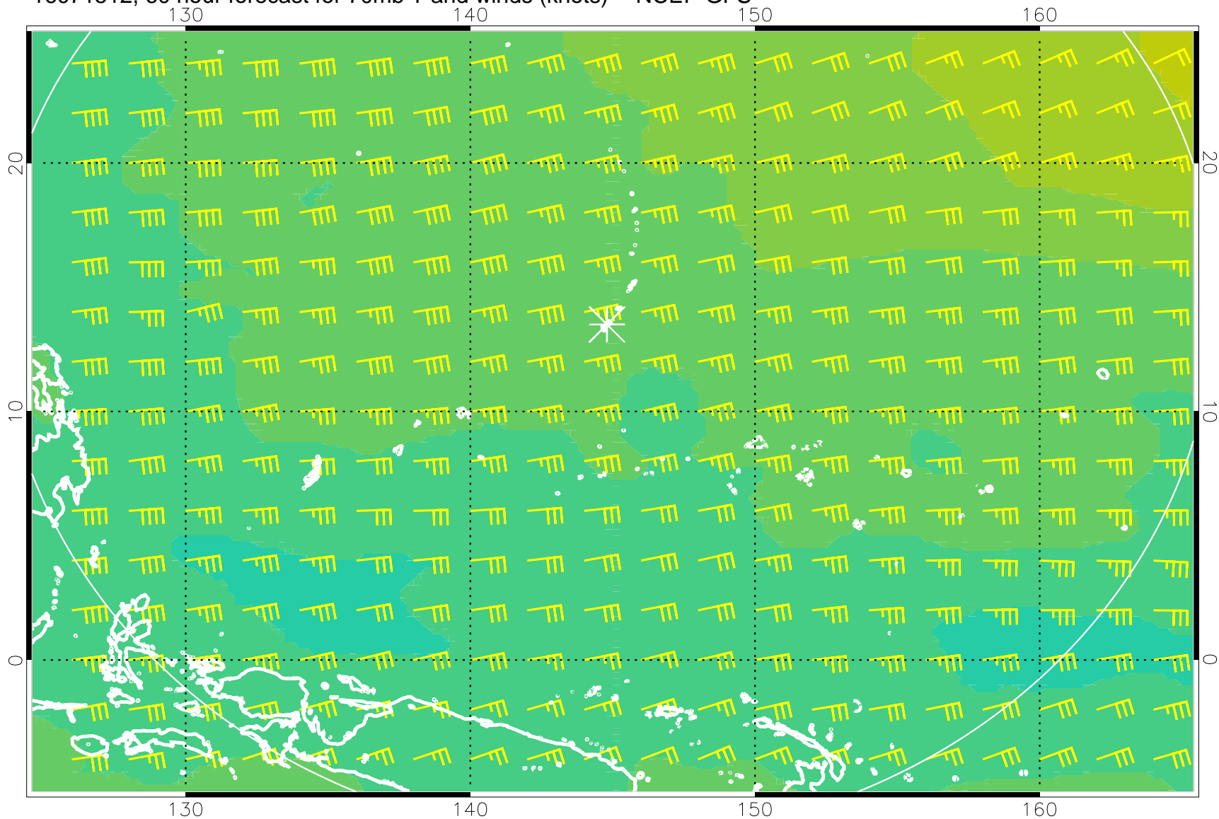
16071512, 60 hour forecast for 70mb T and winds (knots) -- NCEP GFS
