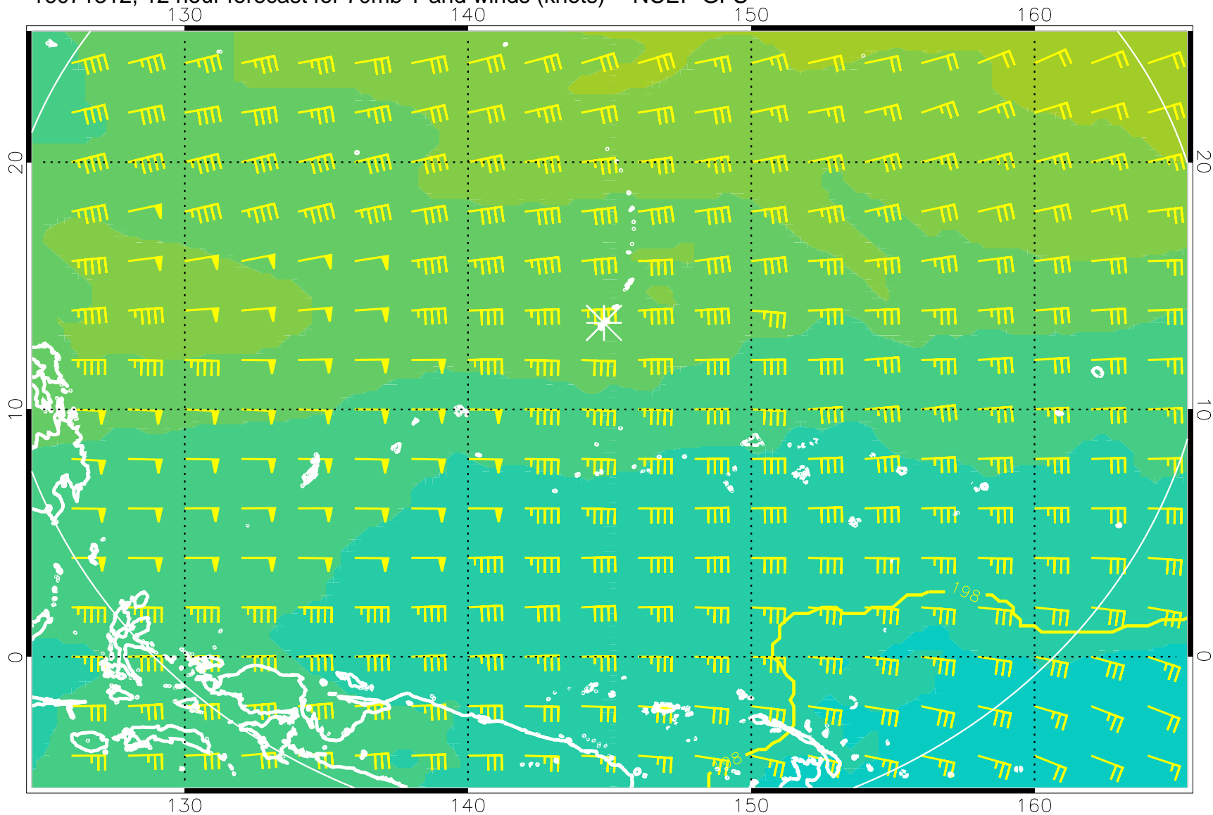
16071312, 12 hour forecast for 70mb T and winds (knots) -- NCEP GFS
