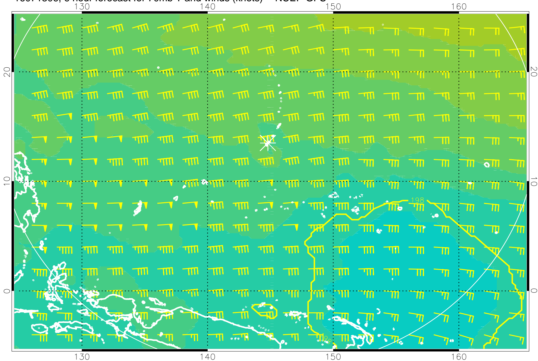
16071306, 6 hour forecast for 70mb T and winds (knots) -- NCEP GFS
