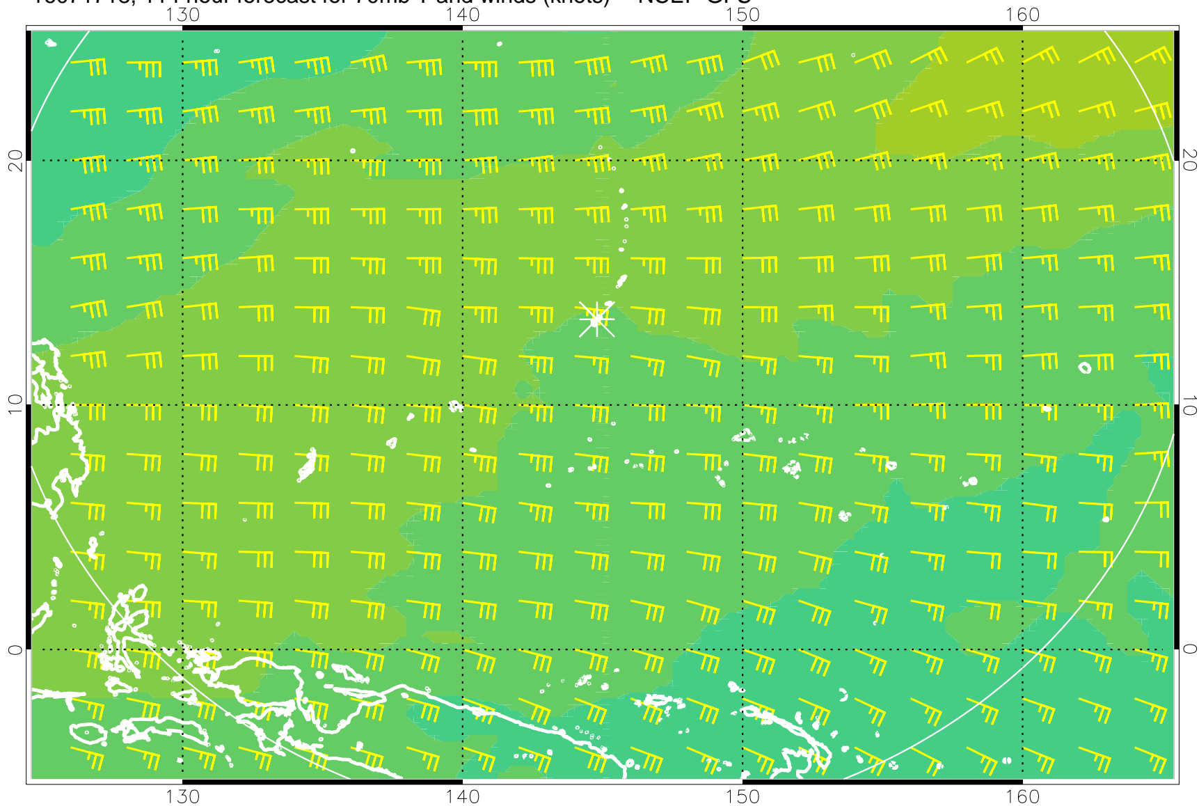
16071718, 114 hour forecast for 70mb T and winds (knots) -- NCEP GFS
