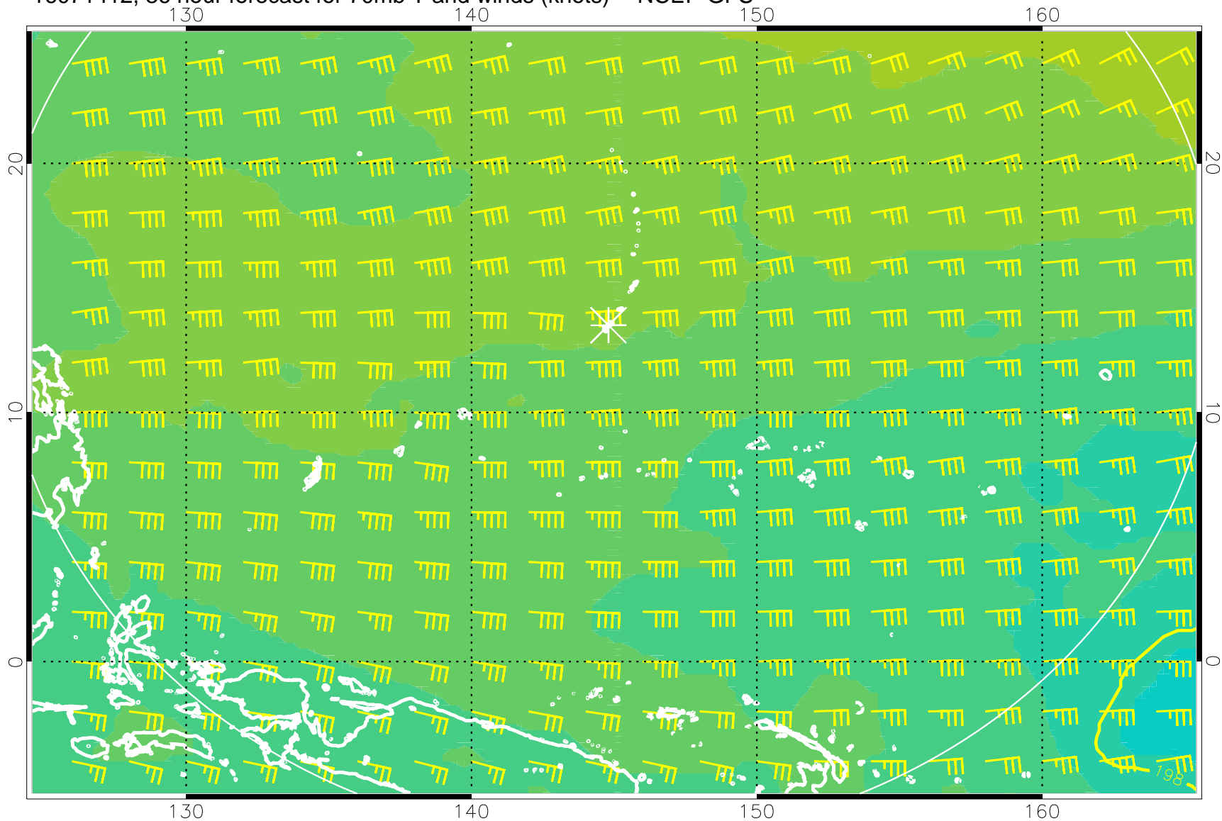
16071412, 36 hour forecast for 70mb T and winds (knots) -- NCEP GFS
