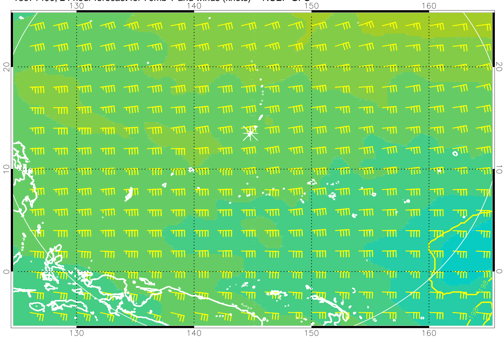
16071400, 24 hour forecast for 70mb T and winds (knots) -- NCEP GFS
