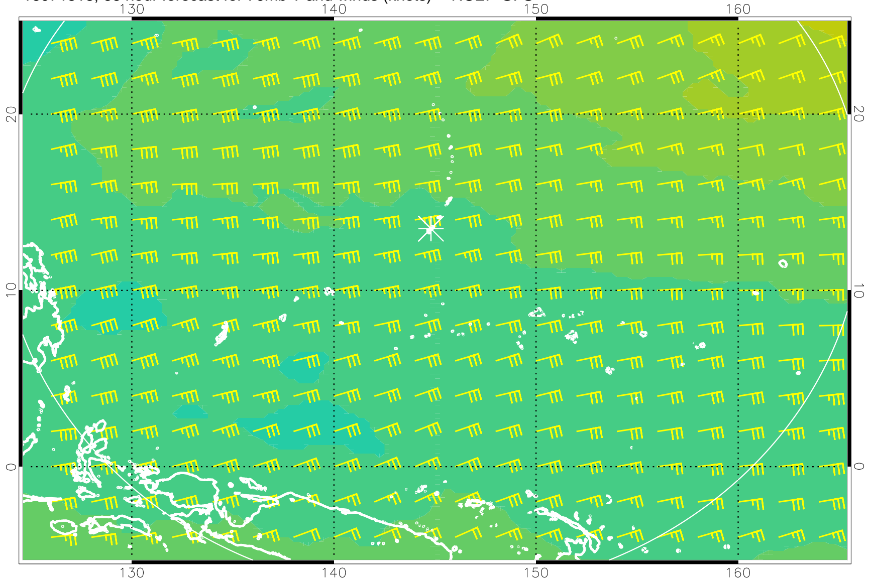
16071518, 66 hour forecast for 70mb T and winds (knots) -- NCEP GFS
