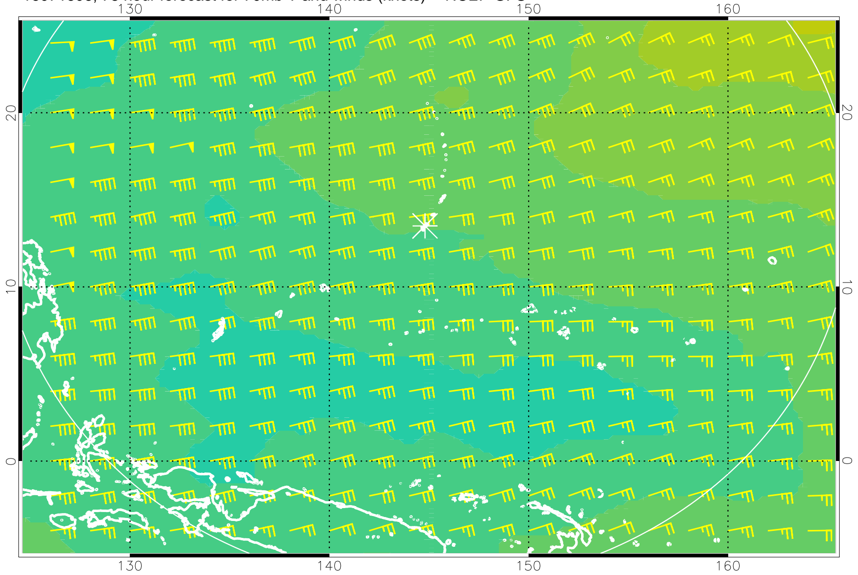
16071606, 78 hour forecast for 70mb T and winds (knots) -- NCEP GFS
