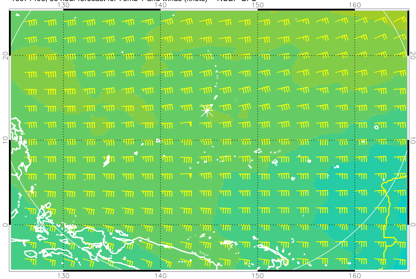
16071406, 30 hour forecast for 70mb T and winds (knots) -- NCEP GFS
