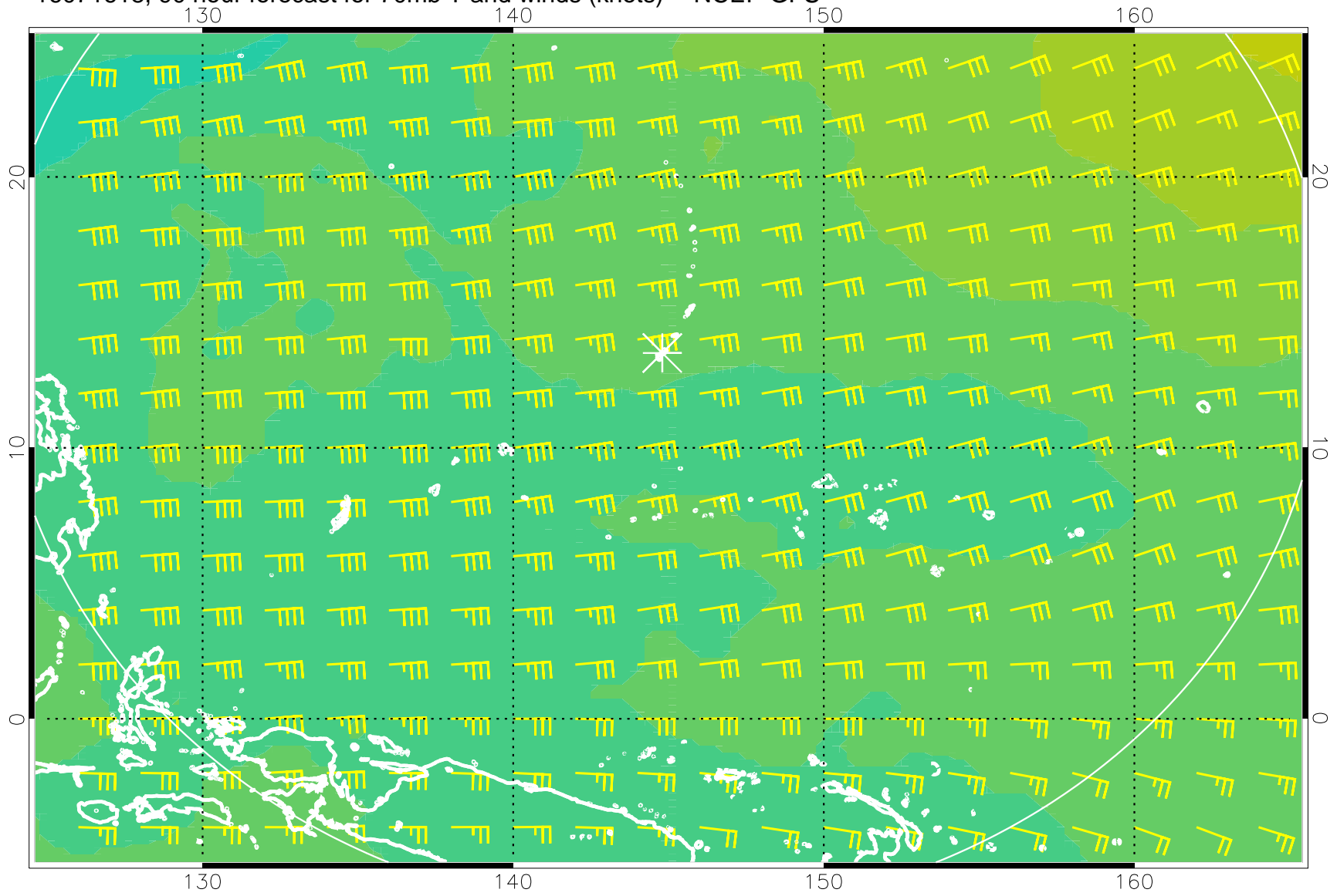
16071618, 90 hour forecast for 70mb T and winds (knots) -- NCEP GFS
