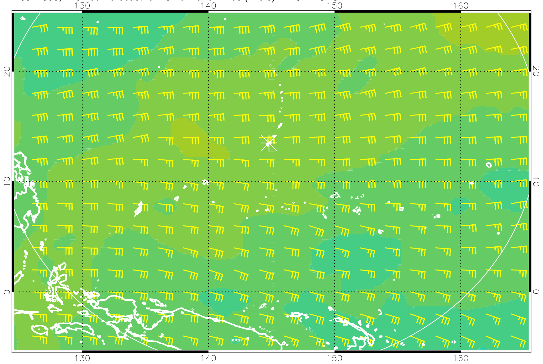
16071800, 120 hour forecast for 70mb T and winds (knots) -- NCEP GFS
