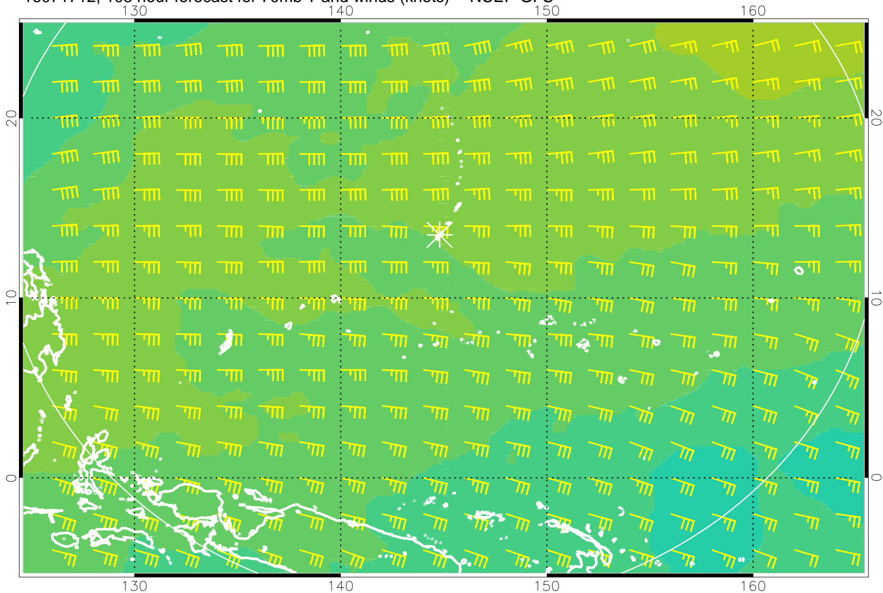
16071712, 108 hour forecast for 70mb T and winds (knots) -- NCEP GFS
