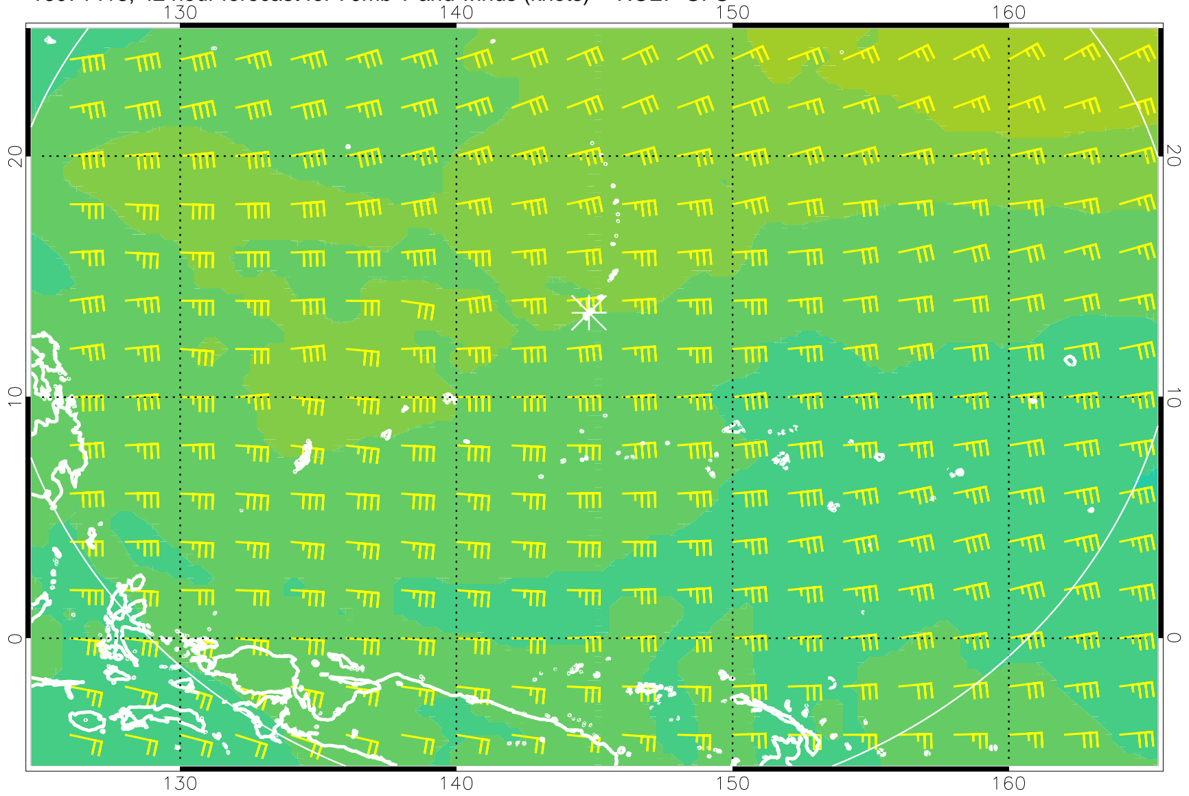
16071418, 42 hour forecast for 70mb T and winds (knots) -- NCEP GFS
