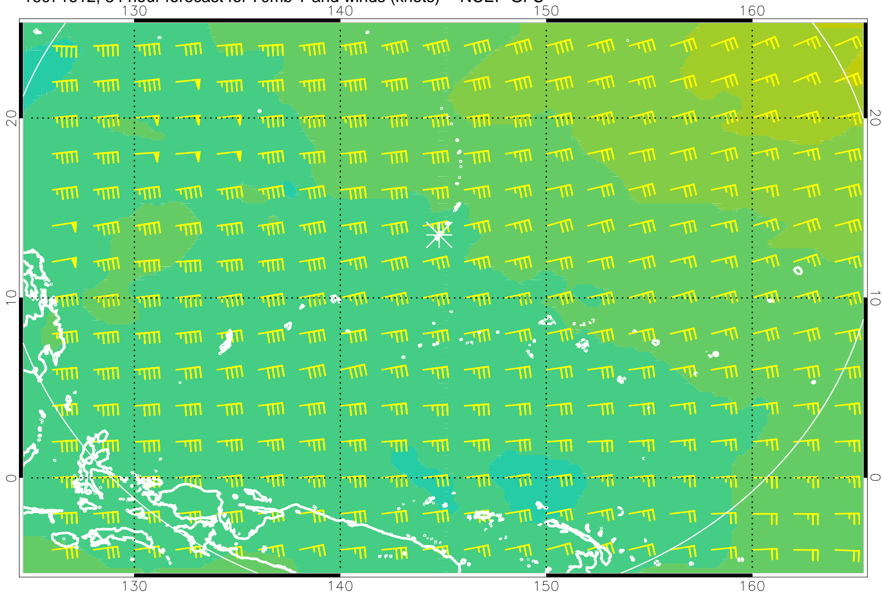
16071612, 84 hour forecast for 70mb T and winds (knots) -- NCEP GFS
