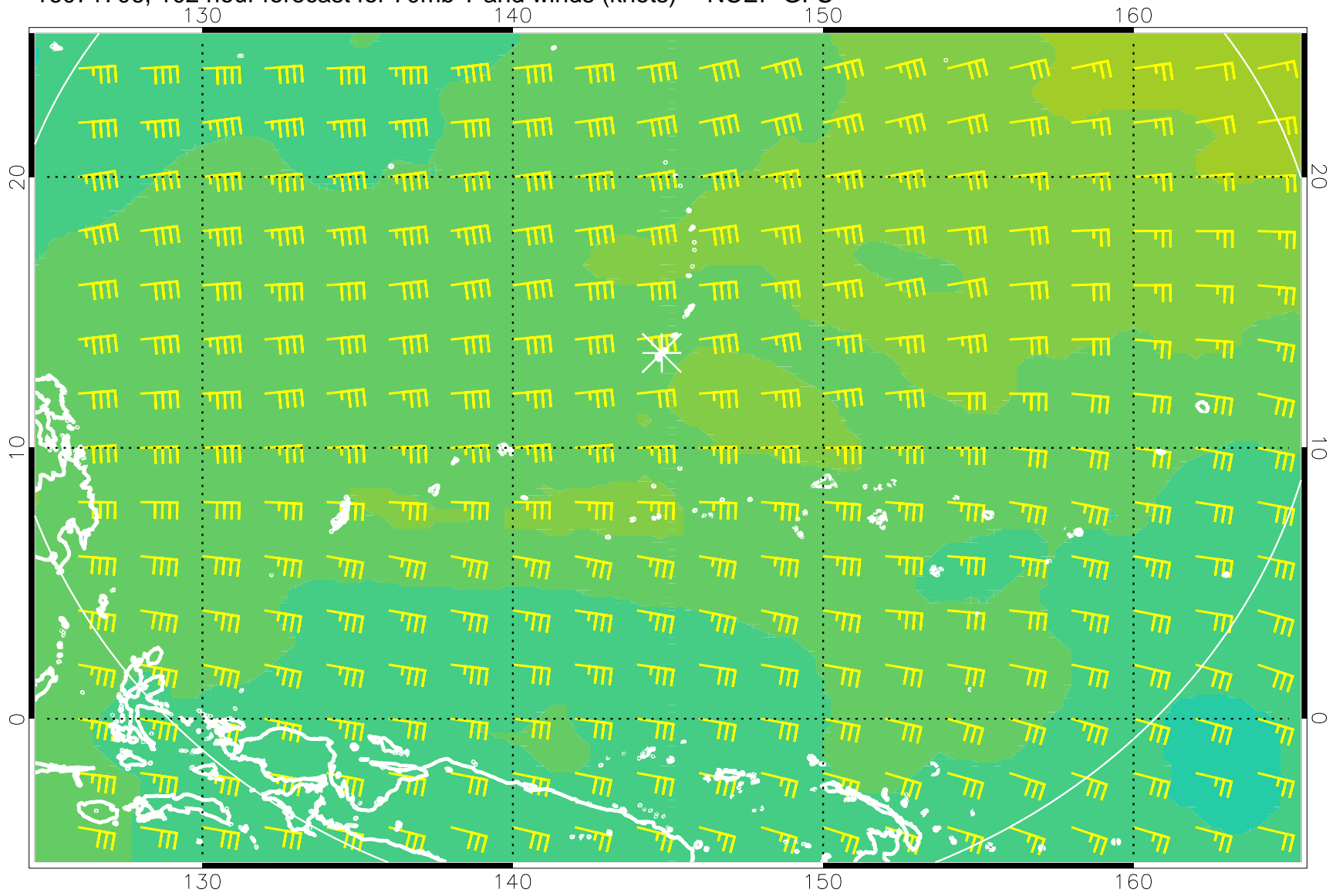
16071706, 102 hour forecast for 70mb T and winds (knots) -- NCEP GFS
