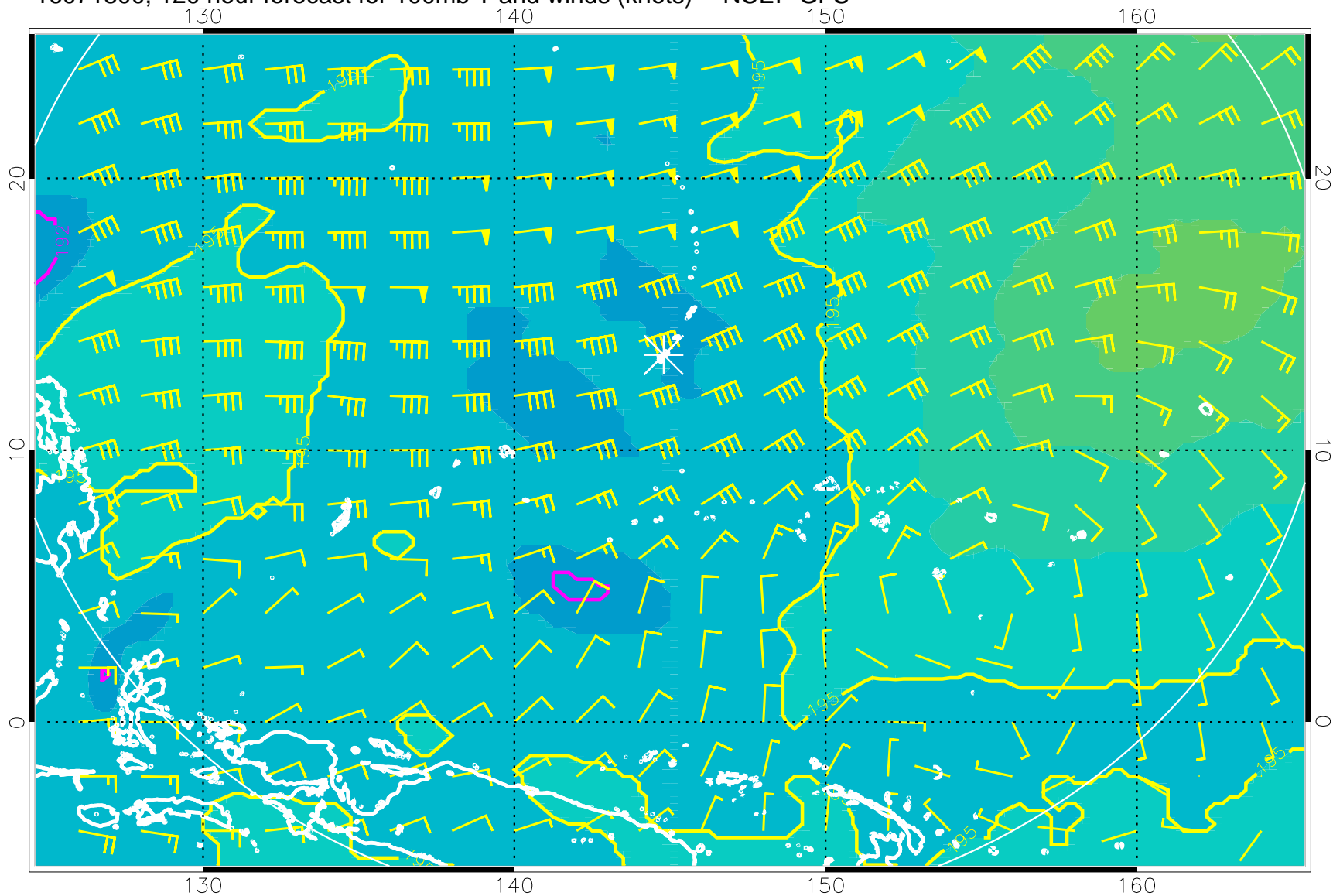
16071800, 120 hour forecast for 100mb T and winds (knots) -- NCEP GFS
