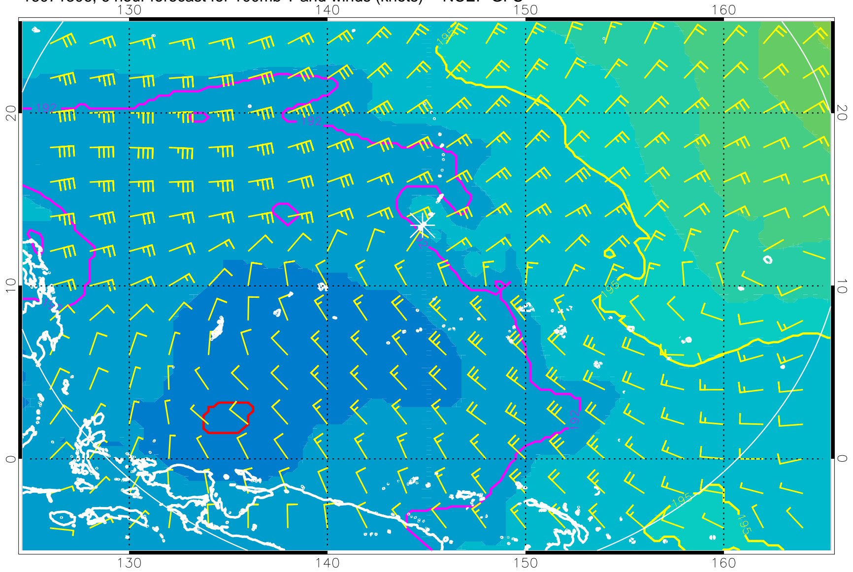
16071306, 6 hour forecast for 100mb T and winds (knots) -- NCEP GFS
