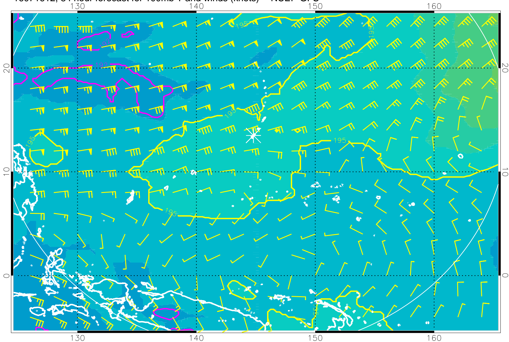
16071612, 84 hour forecast for 100mb T and winds (knots) -- NCEP GFS
