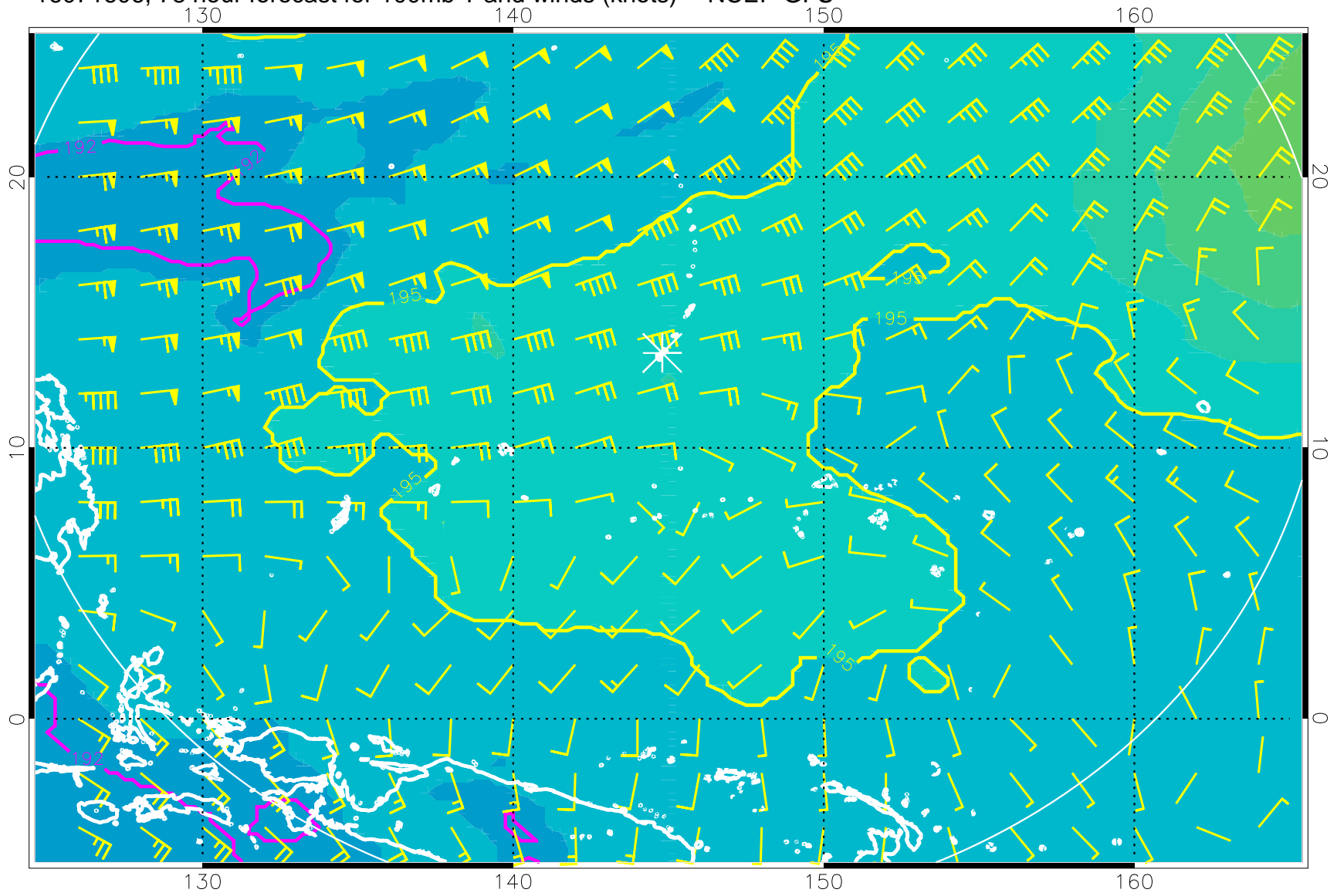
16071606, 78 hour forecast for 100mb T and winds (knots) -- NCEP GFS
