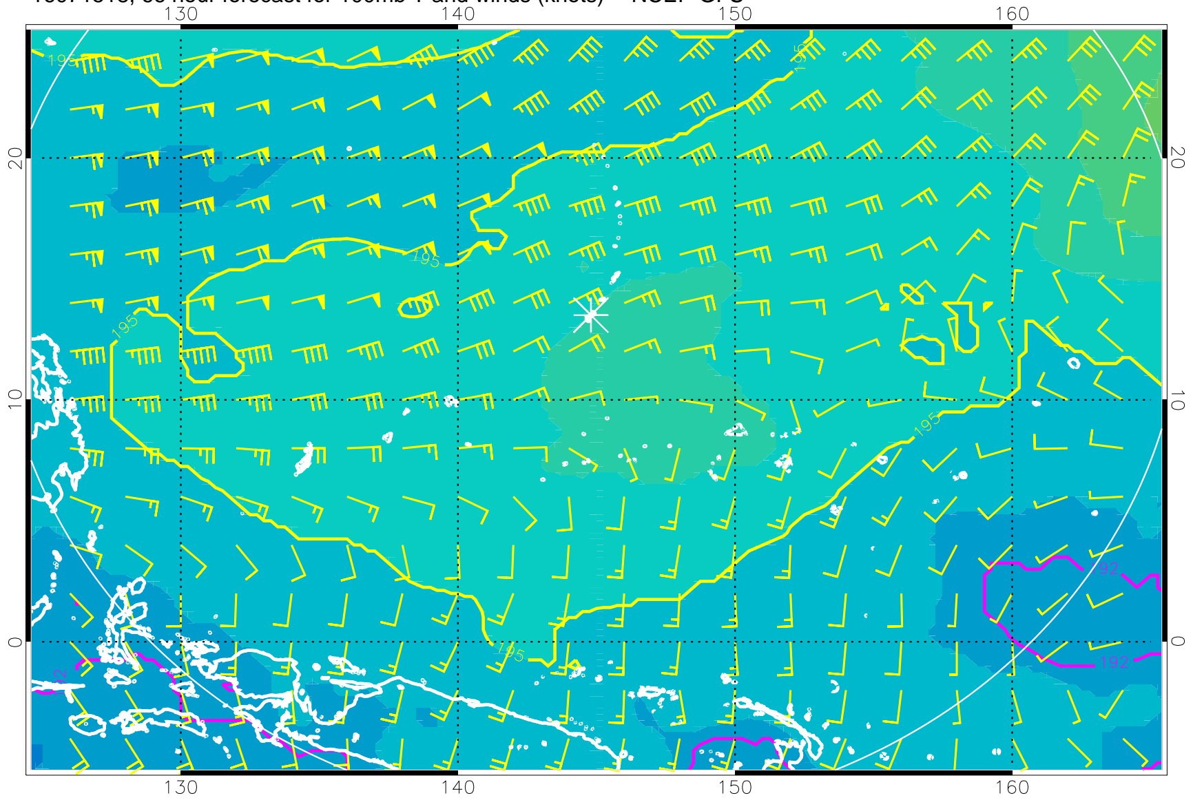
16071518, 66 hour forecast for 100mb T and winds (knots) -- NCEP GFS
