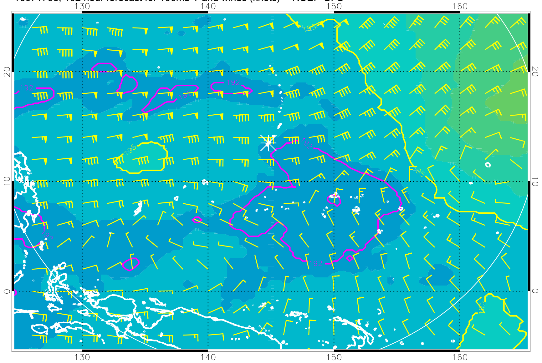
16071706, 102 hour forecast for 100mb T and winds (knots) -- NCEP GFS
