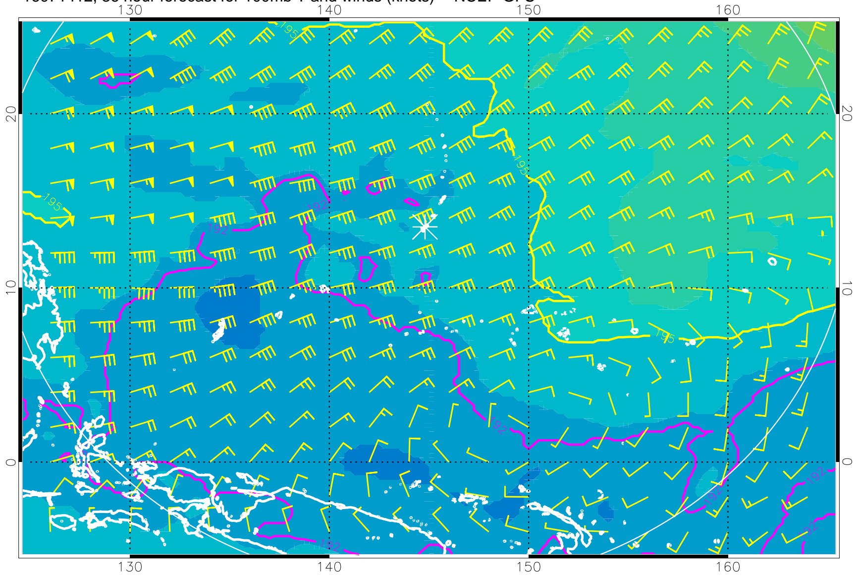
16071412, 36 hour forecast for 100mb T and winds (knots) -- NCEP GFS
