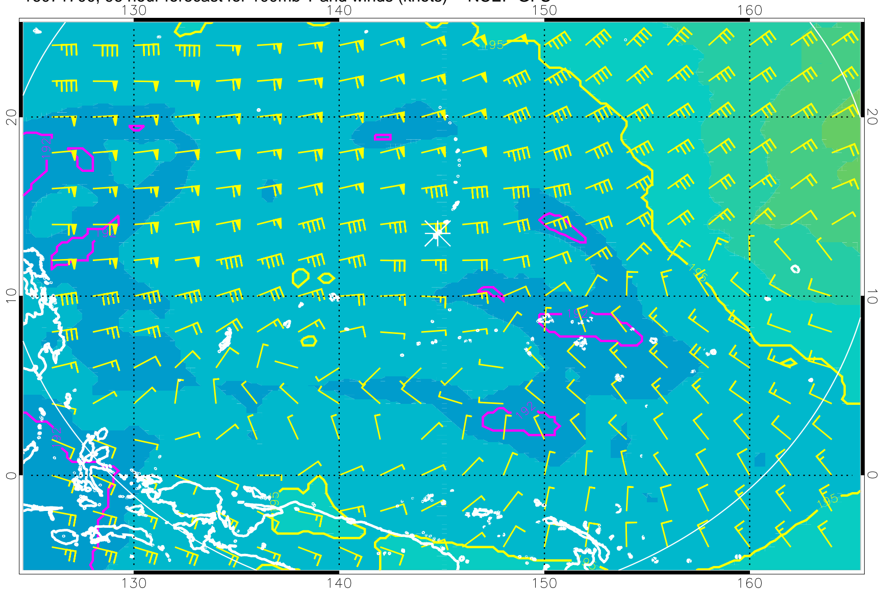
16071700, 96 hour forecast for 100mb T and winds (knots) -- NCEP GFS
