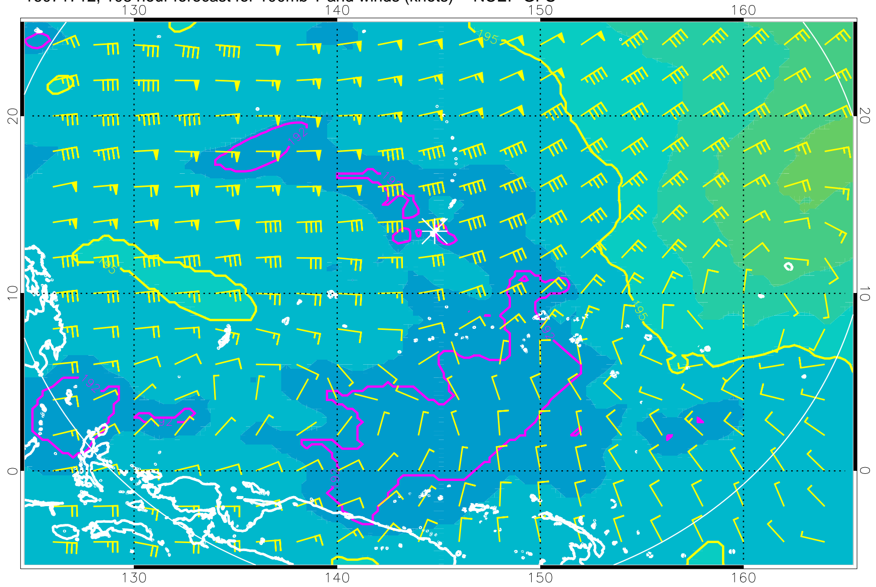
16071712, 108 hour forecast for 100mb T and winds (knots) -- NCEP GFS
