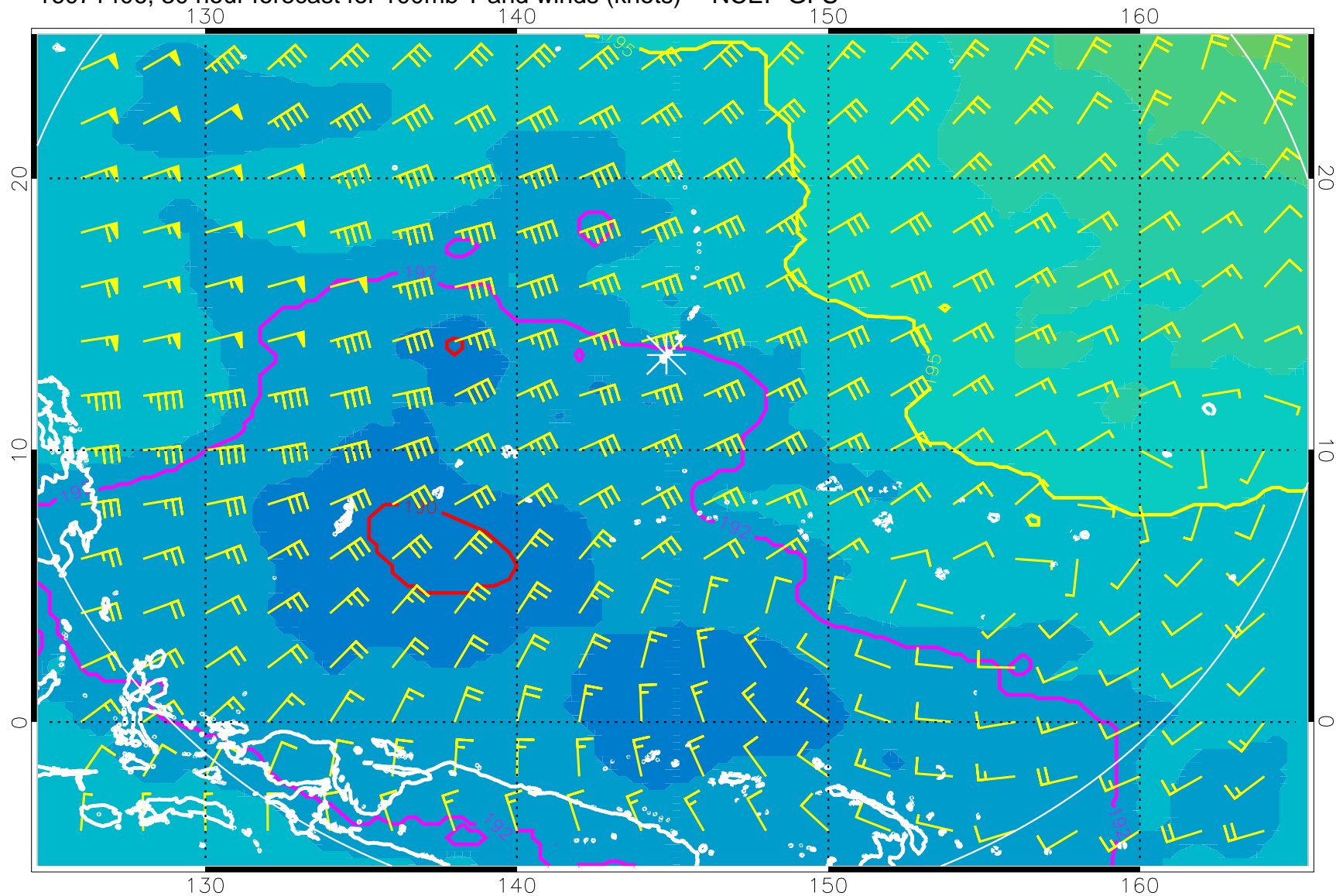
16071406, 30 hour forecast for 100mb T and winds (knots) -- NCEP GFS
