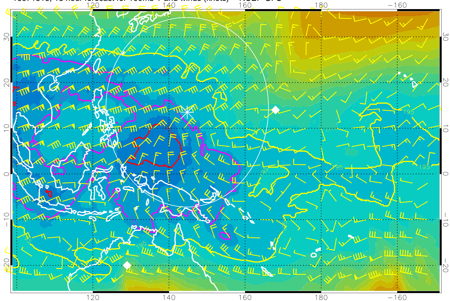
16071318, 18 hour forecast for 100mb T and winds (knots) -- NCEP GFS
