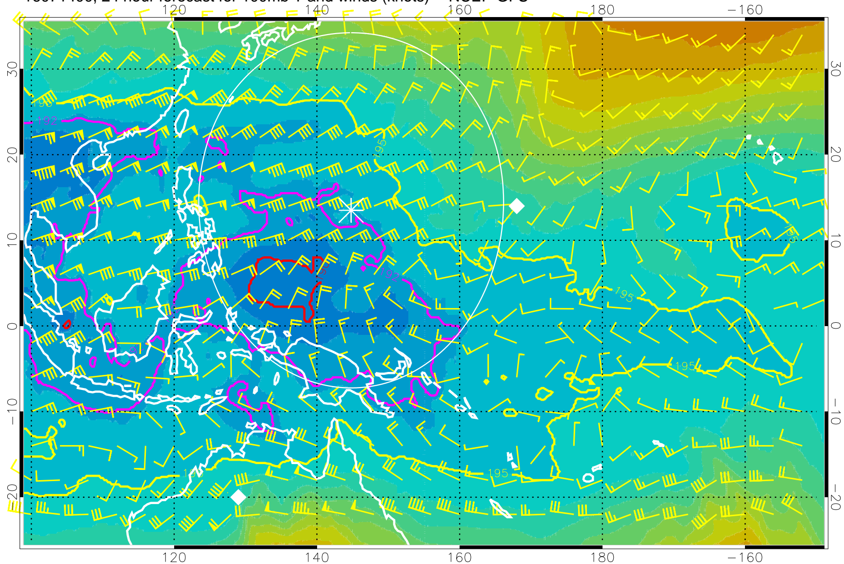
16071400, 24 hour forecast for 100mb T and winds (knots) -- NCEP GFS
