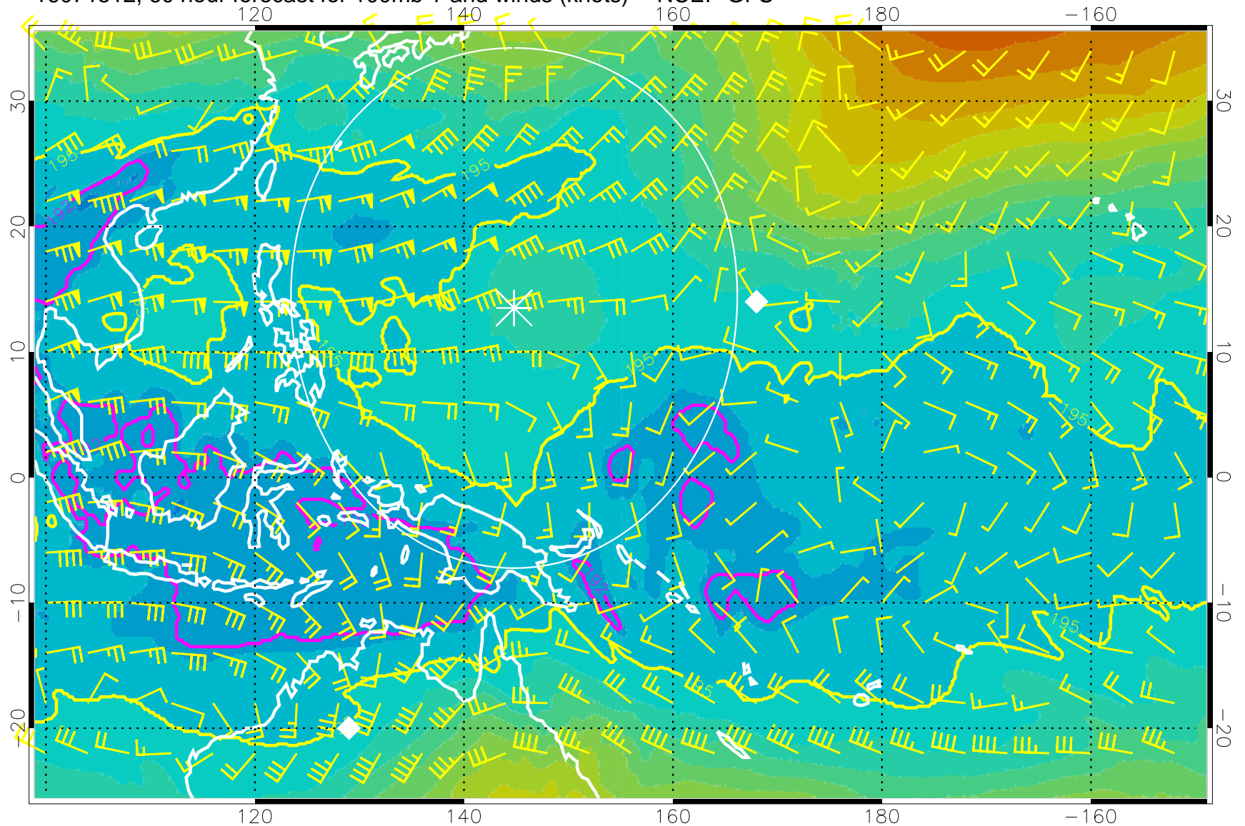
16071512, 60 hour forecast for 100mb T and winds (knots) -- NCEP GFS
