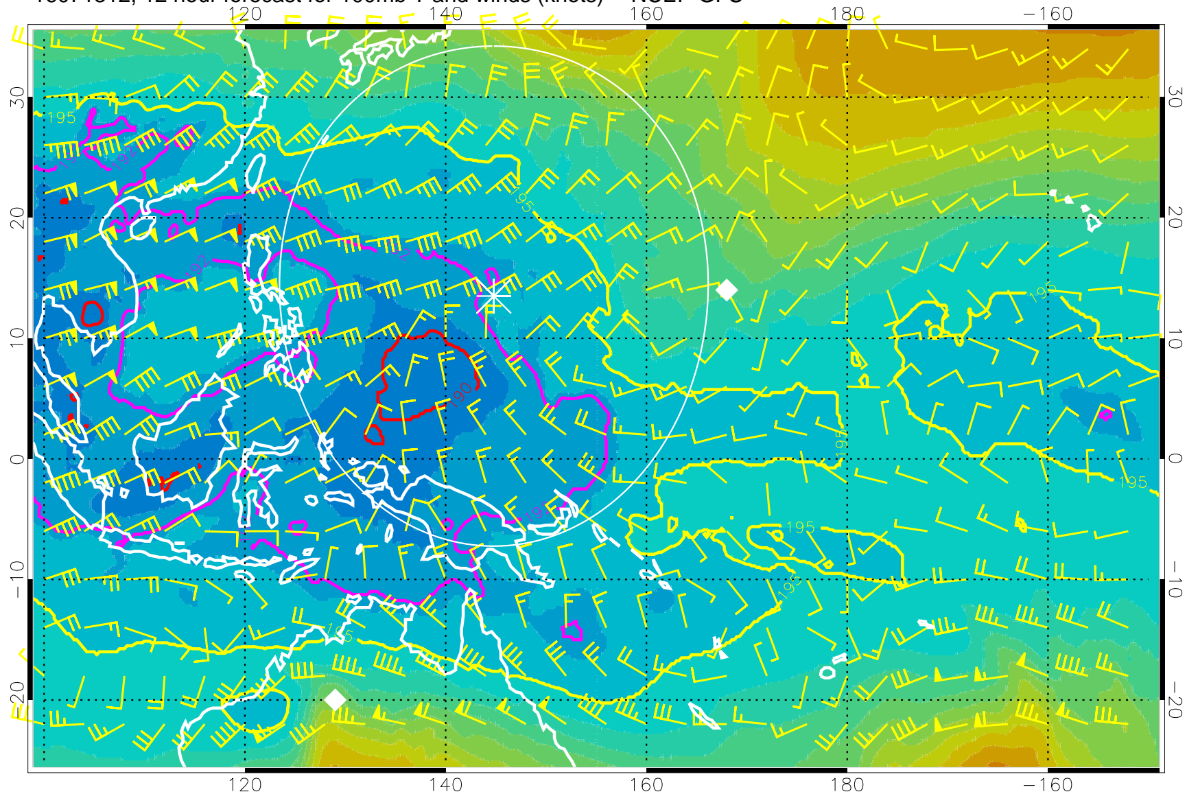
16071312, 12 hour forecast for 100mb T and winds (knots) -- NCEP GFS
