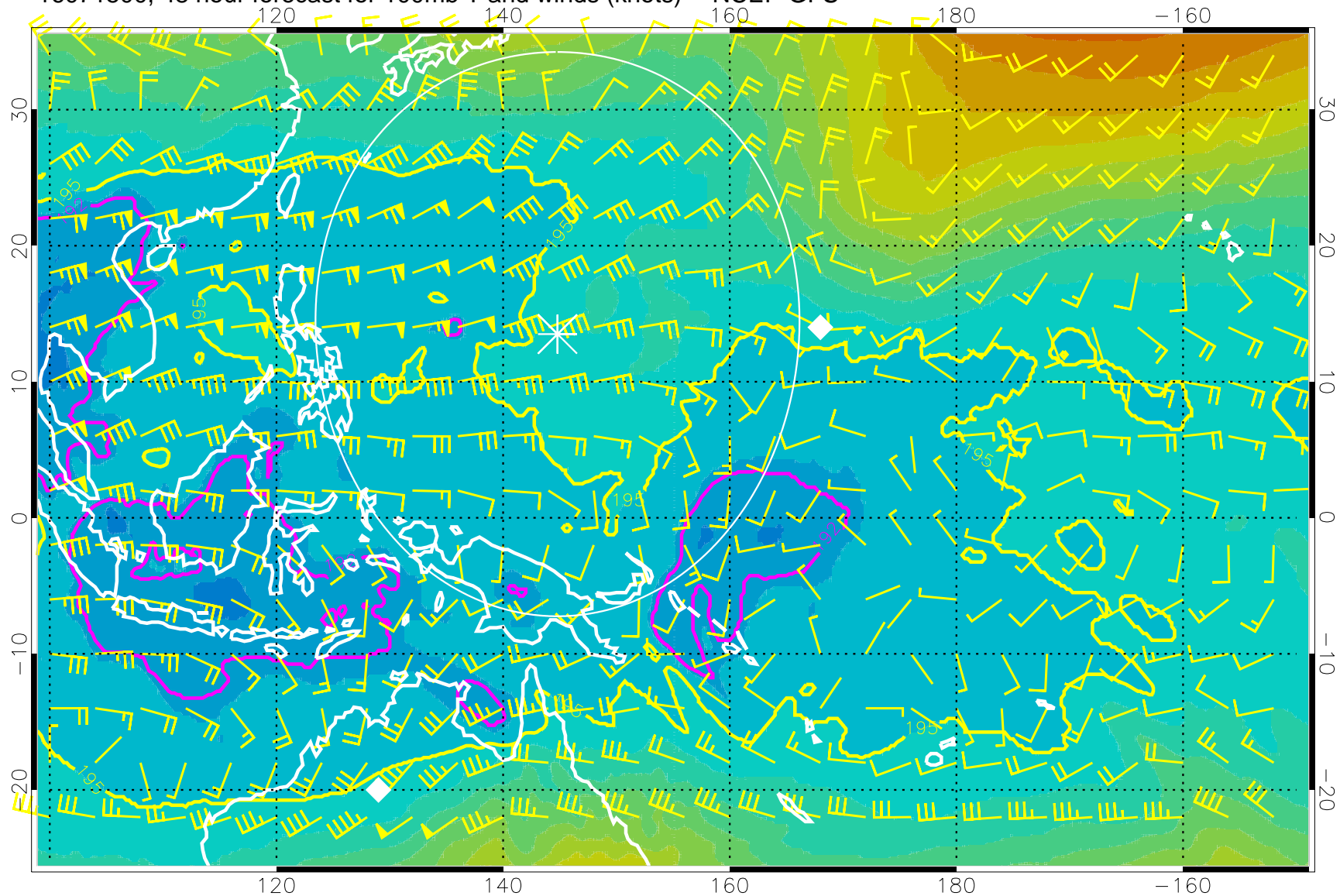
16071500, 48 hour forecast for 100mb T and winds (knots) -- NCEP GFS
