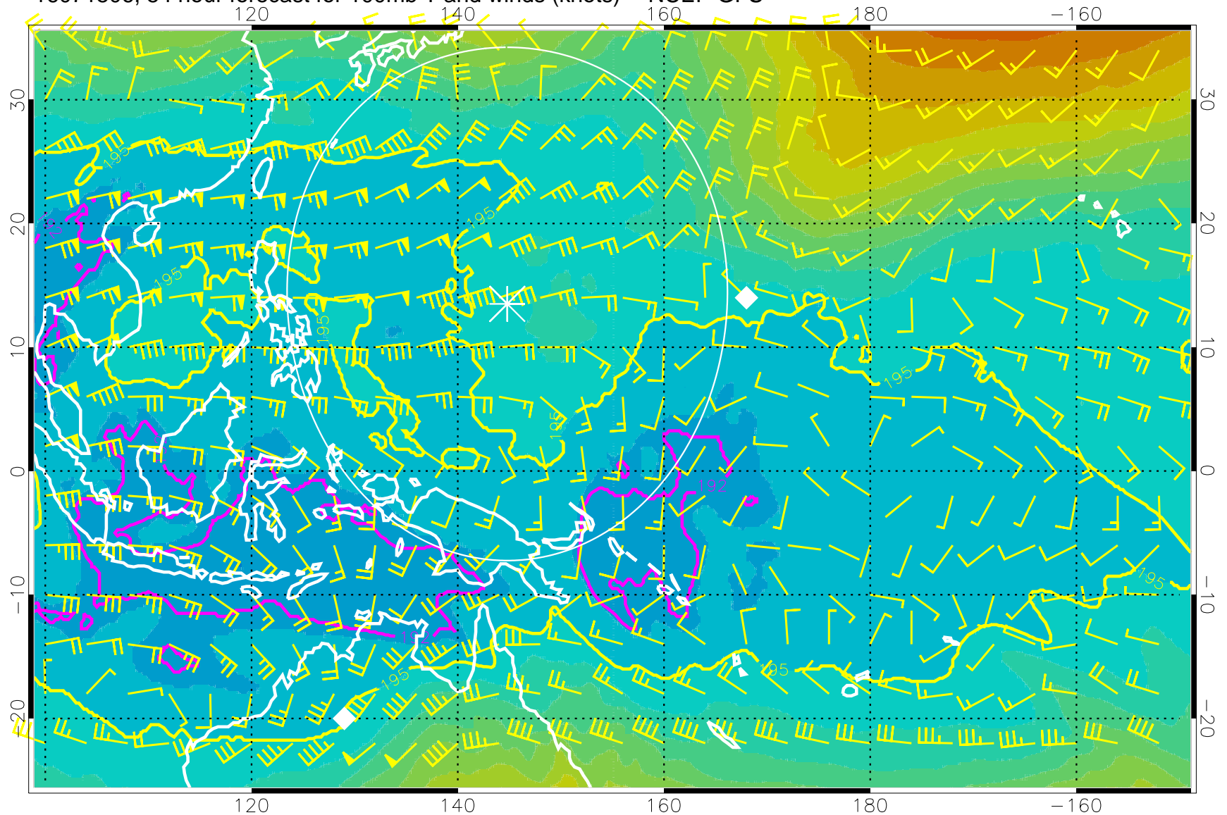
16071506, 54 hour forecast for 100mb T and winds (knots) -- NCEP GFS
