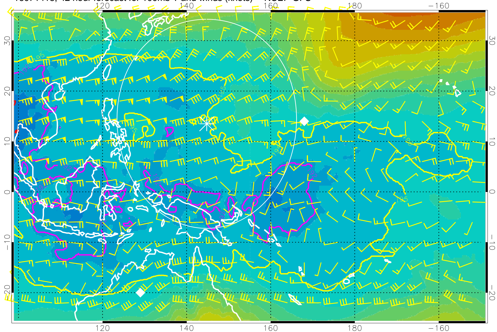
16071418, 42 hour forecast for 100mb T and winds (knots) -- NCEP GFS
