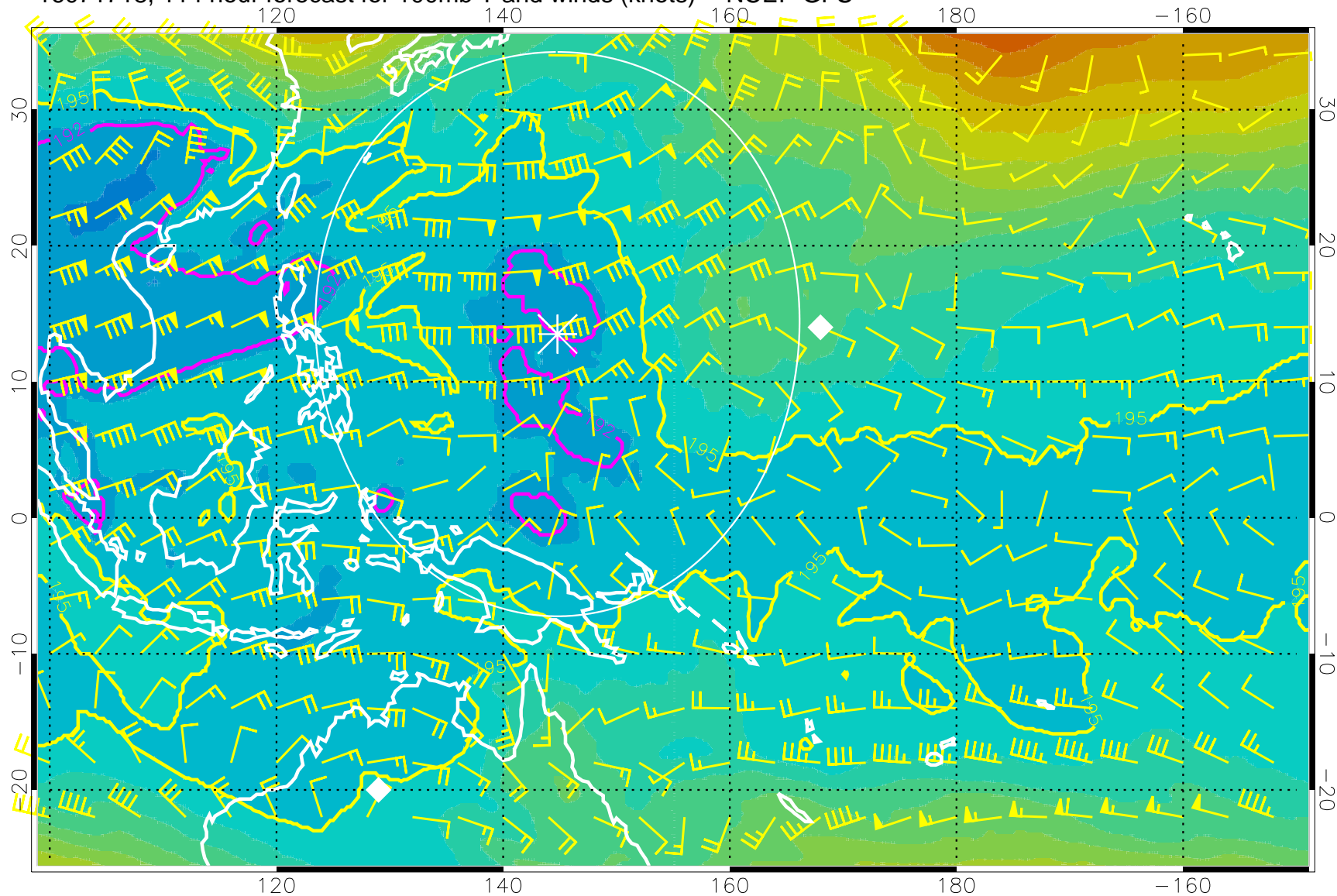
16071718, 114 hour forecast for 100mb T and winds (knots) -- NCEP GFS
