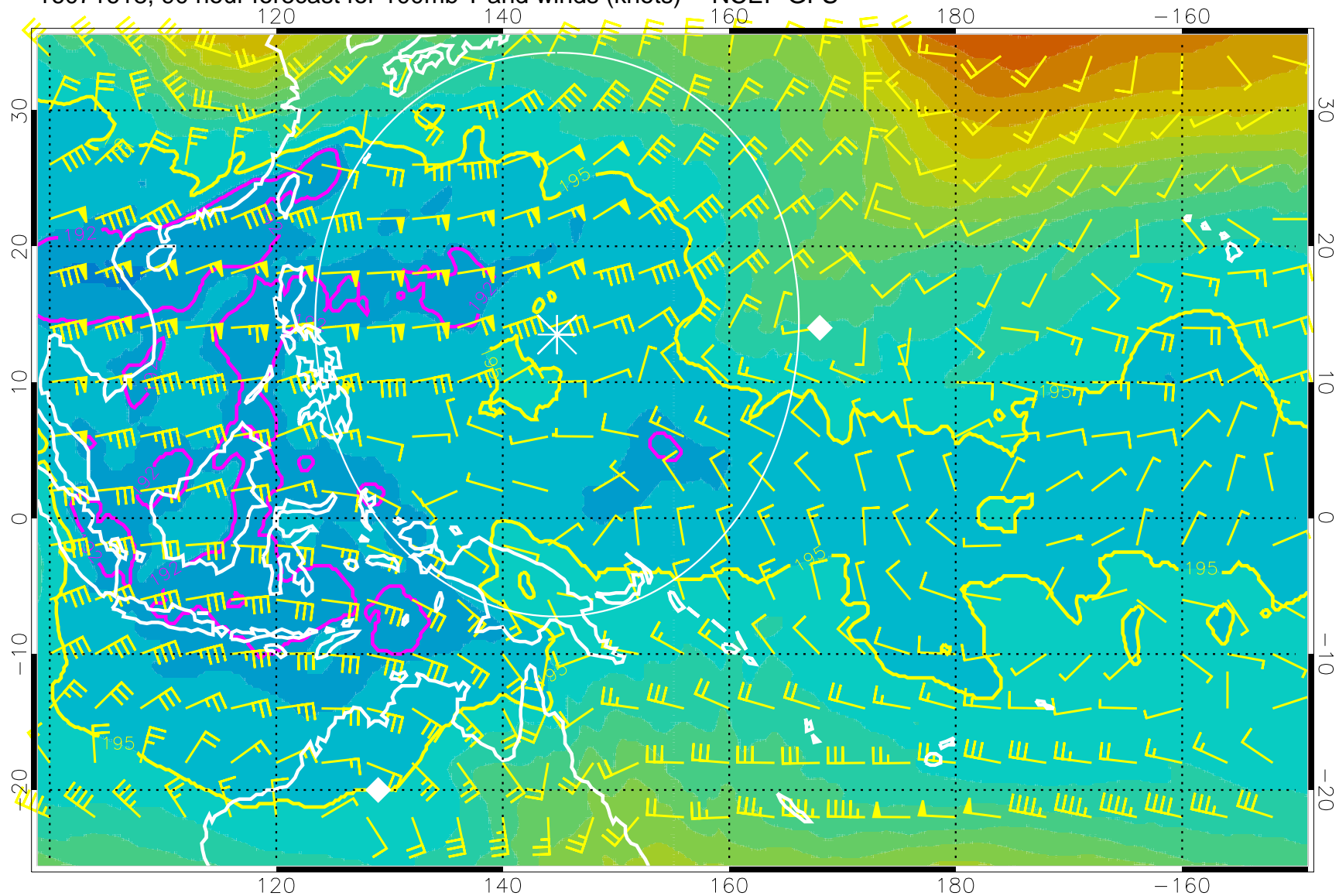
16071618, 90 hour forecast for 100mb T and winds (knots) -- NCEP GFS
