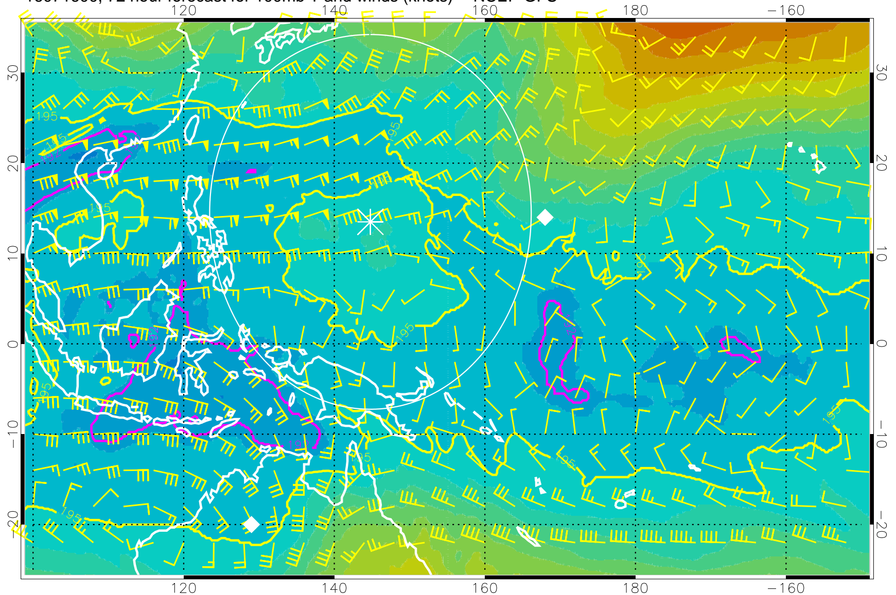
16071600, 72 hour forecast for 100mb T and winds (knots) -- NCEP GFS
