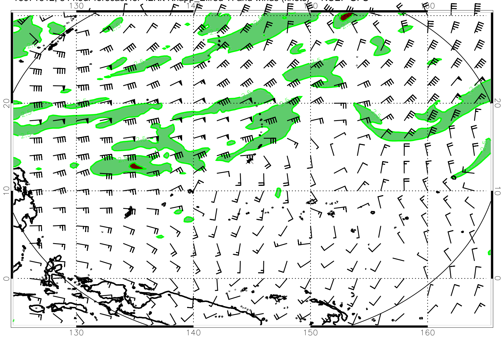
16071612, 84 hour forecast for 42Kft Knapp_Ellrod TI and winds (knots) -- NCEP GFS
