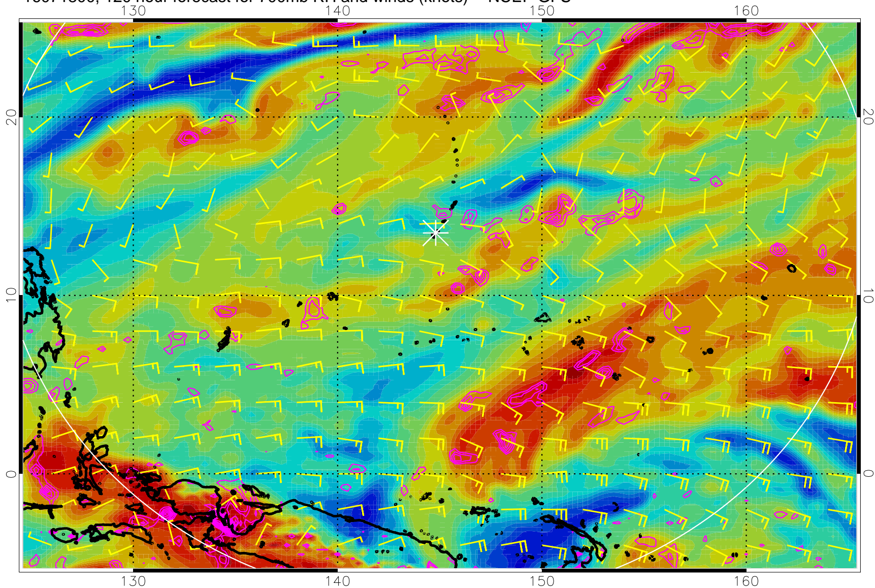
16071800, 120 hour forecast for 700mb RH and winds (knots) -- NCEP GFS
