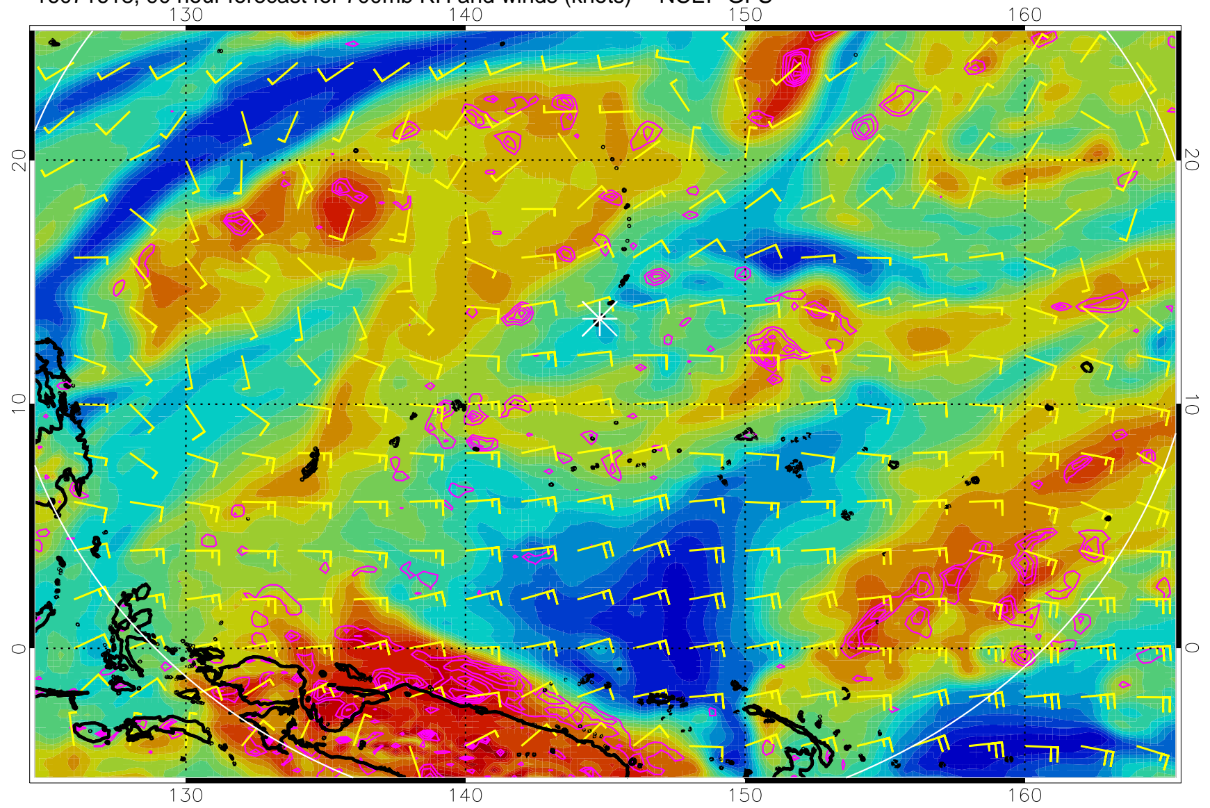
16071618, 90 hour forecast for 700mb RH and winds (knots) -- NCEP GFS
