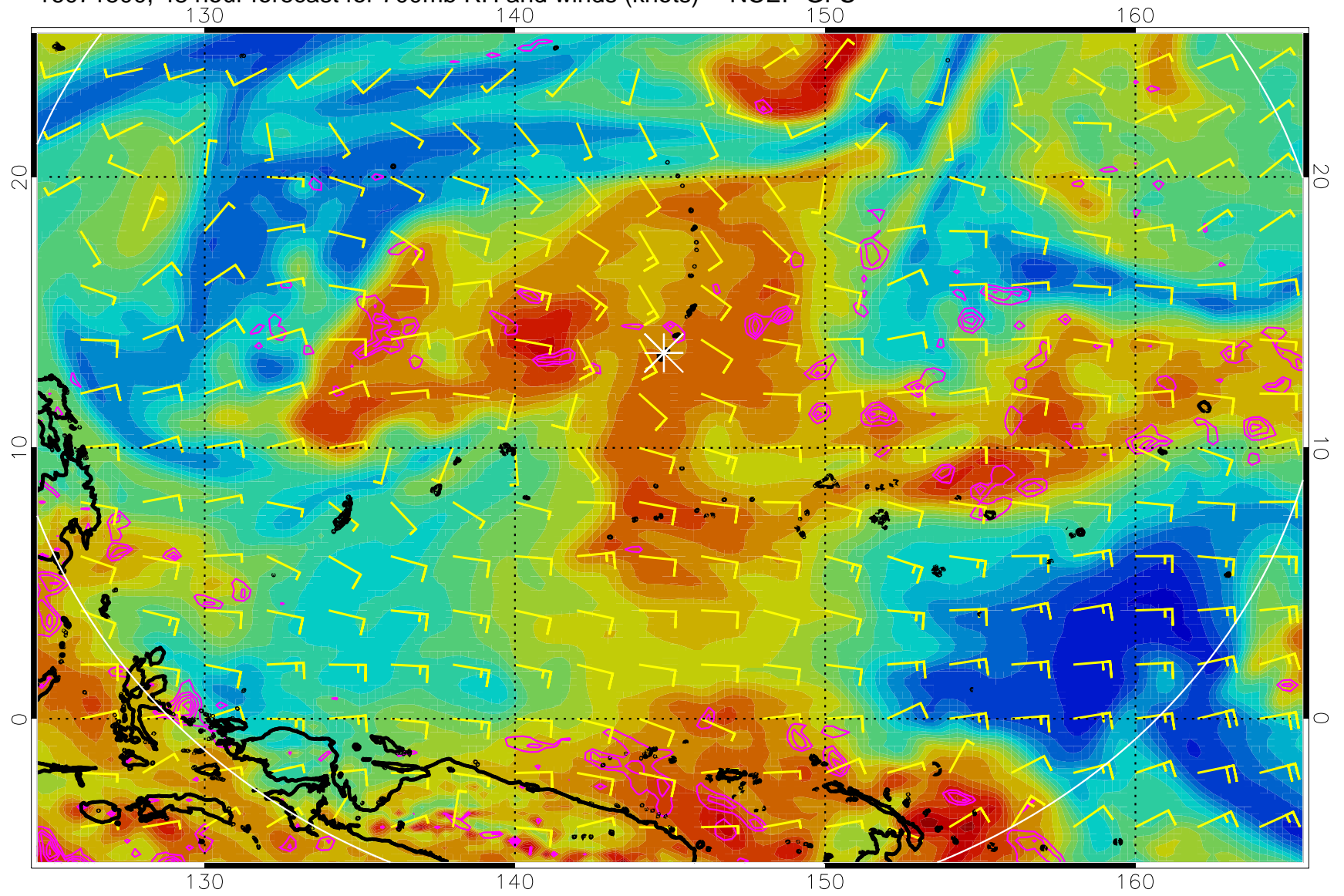
16071500, 48 hour forecast for 700mb RH and winds (knots) -- NCEP GFS
