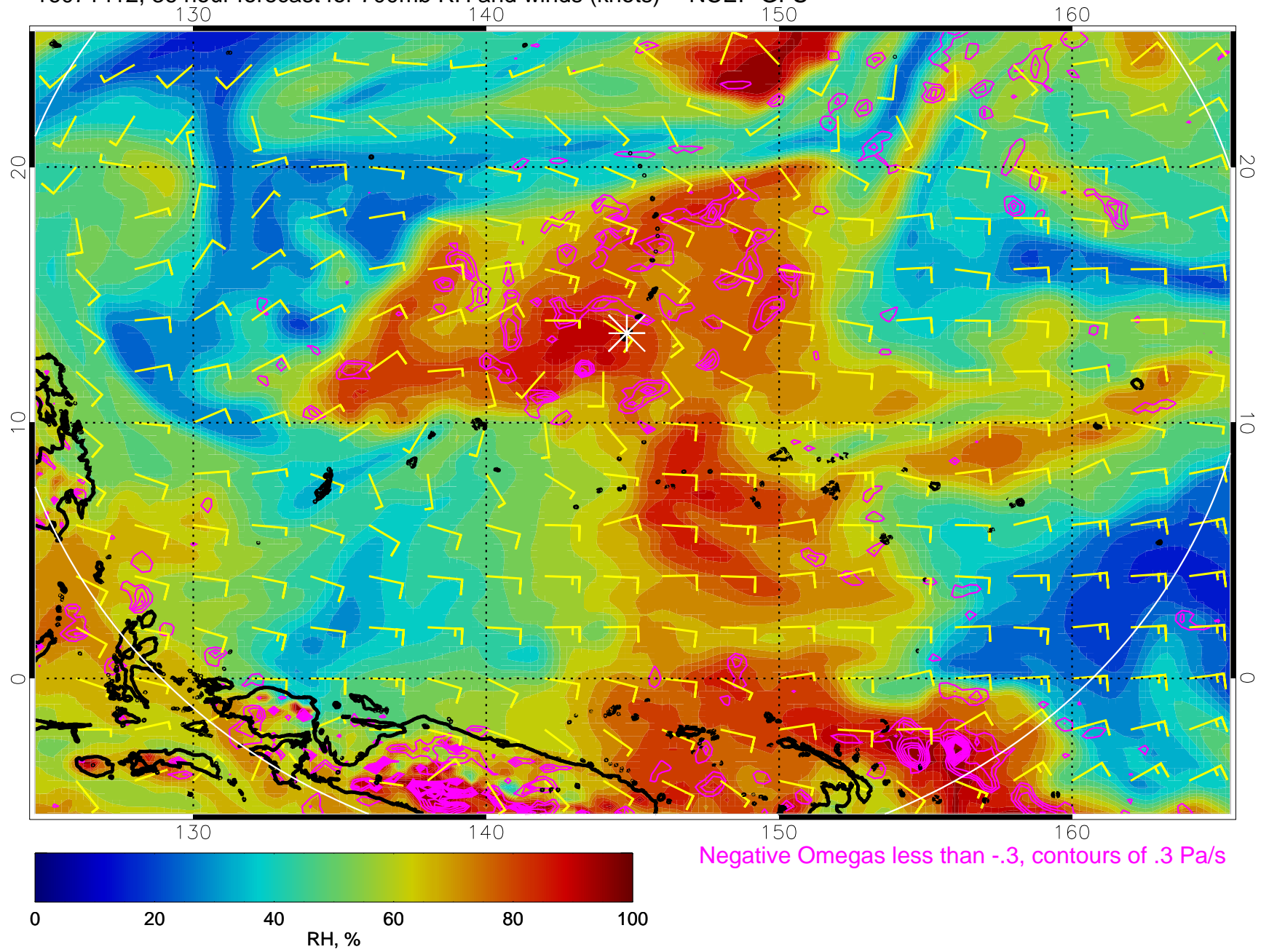
16071412, 36 hour forecast for 700mb RH and winds (knots) -- NCEP GFS
