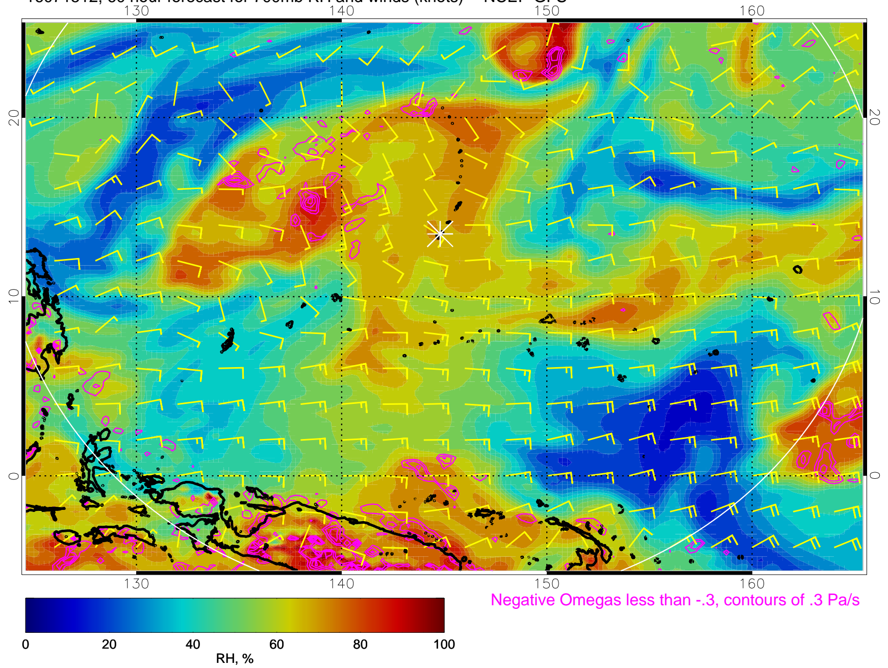
16071512, 60 hour forecast for 700mb RH and winds (knots) -- NCEP GFS
