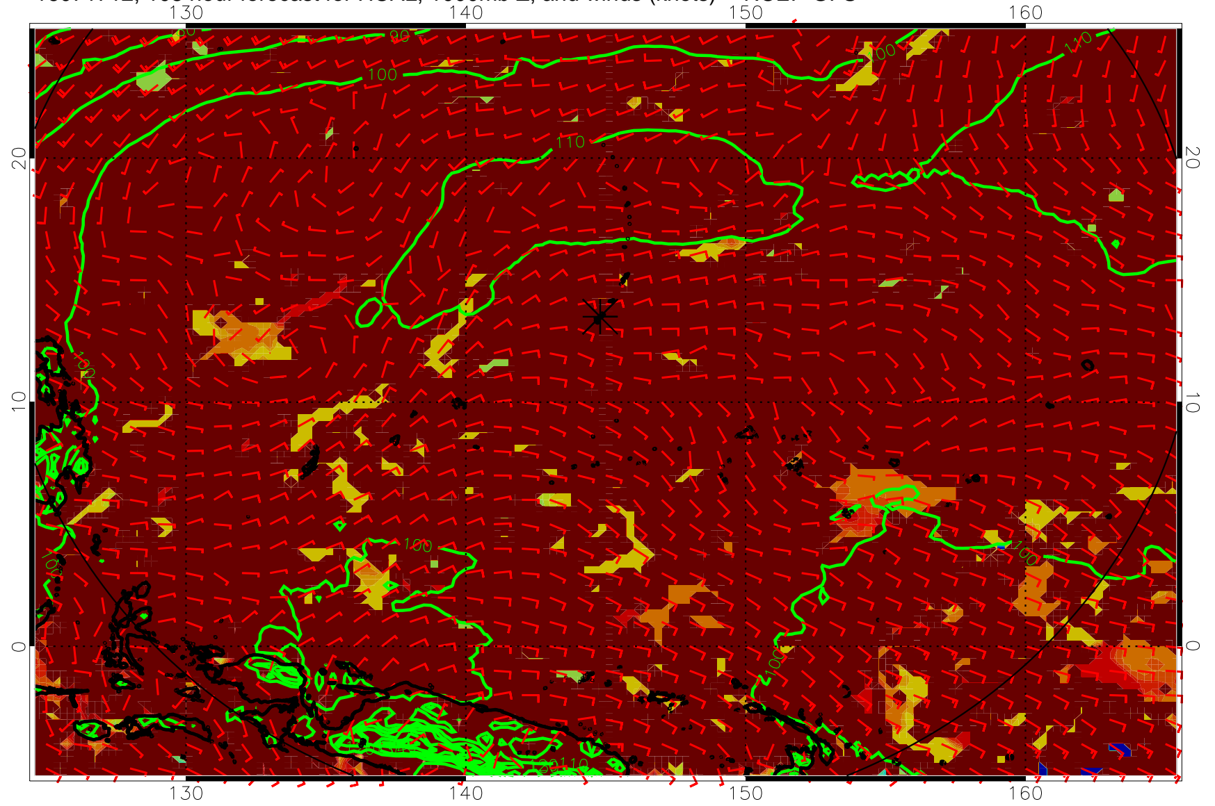
16071712, 108 hour forecast for HCAL, 1000mb Z, and winds (knots) -- NCEP GFS
