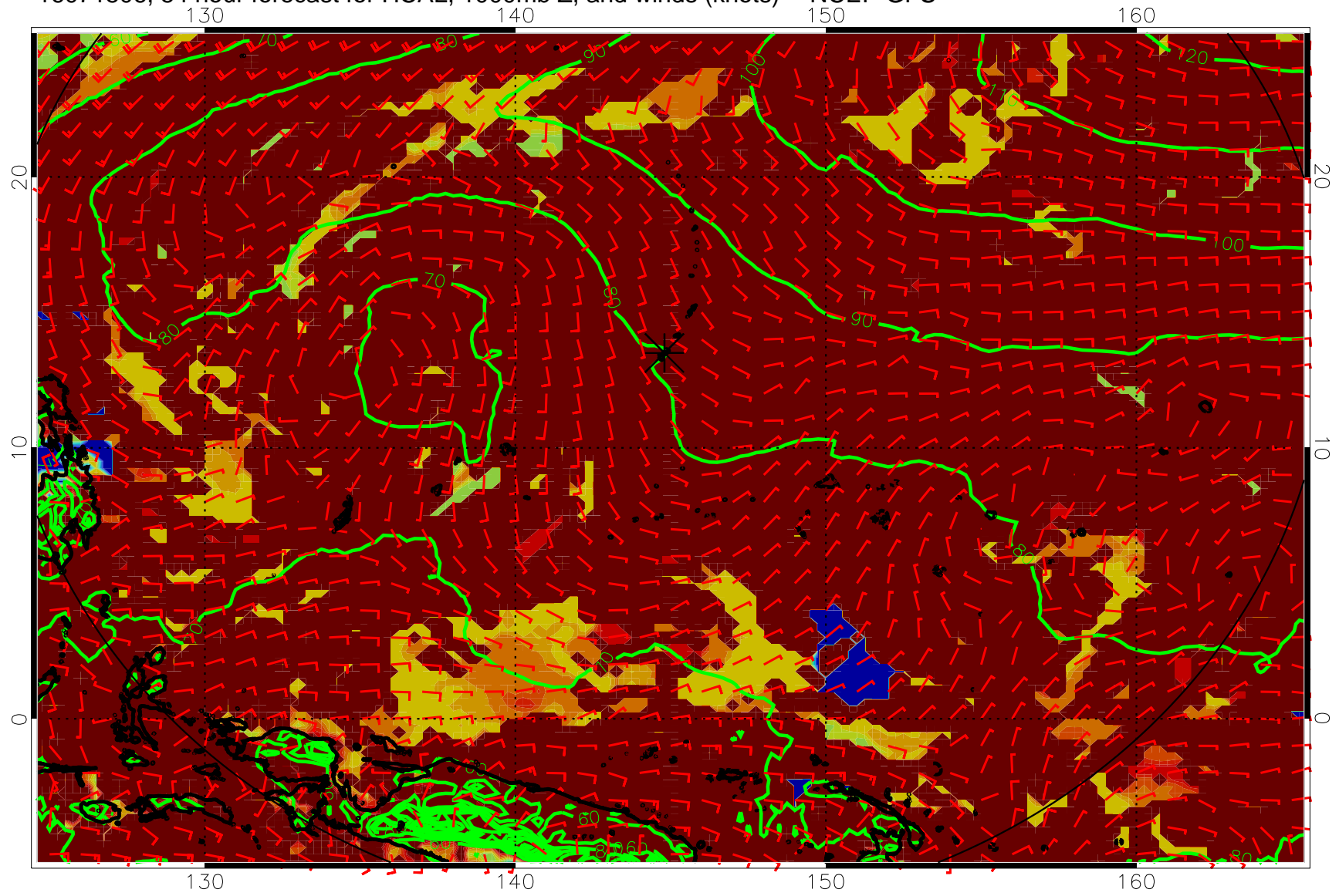
16071506, 54 hour forecast for HCAL, 1000mb Z, and winds (knots) -- NCEP GFS
