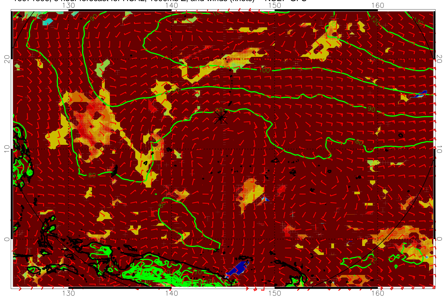
16071306, 6 hour forecast for HCAL, 1000mb Z, and winds (knots) -- NCEP GFS
