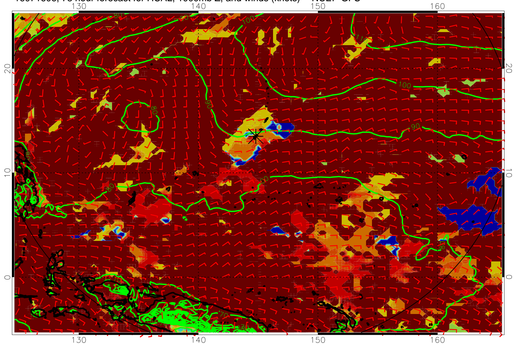
16071606, 78 hour forecast for HCAL, 1000mb Z, and winds (knots) -- NCEP GFS
