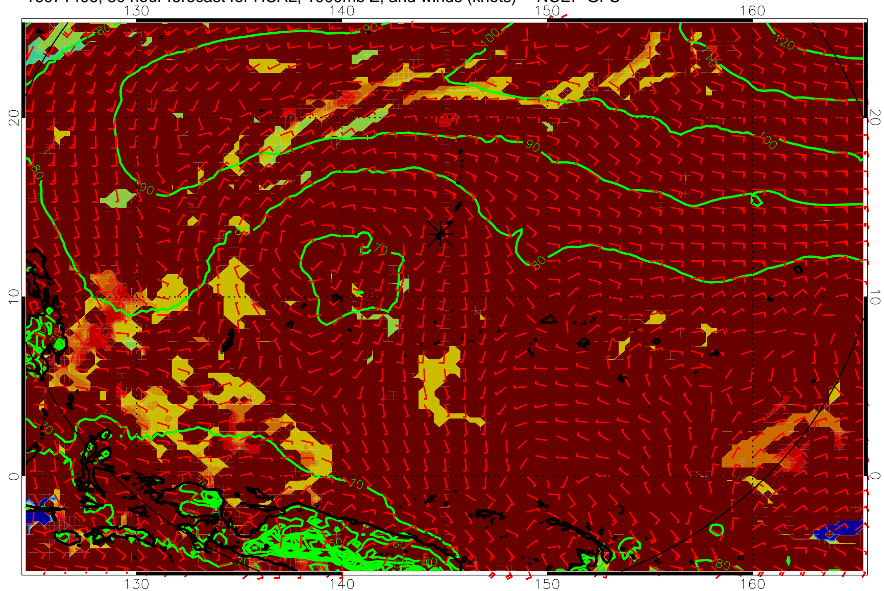
16071406, 30 hour forecast for HCAL, 1000mb Z, and winds (knots) -- NCEP GFS
