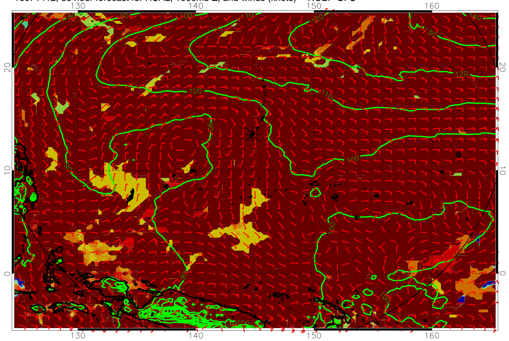
16071412, 36 hour forecast for HCAL, 1000mb Z, and winds (knots) -- NCEP GFS
