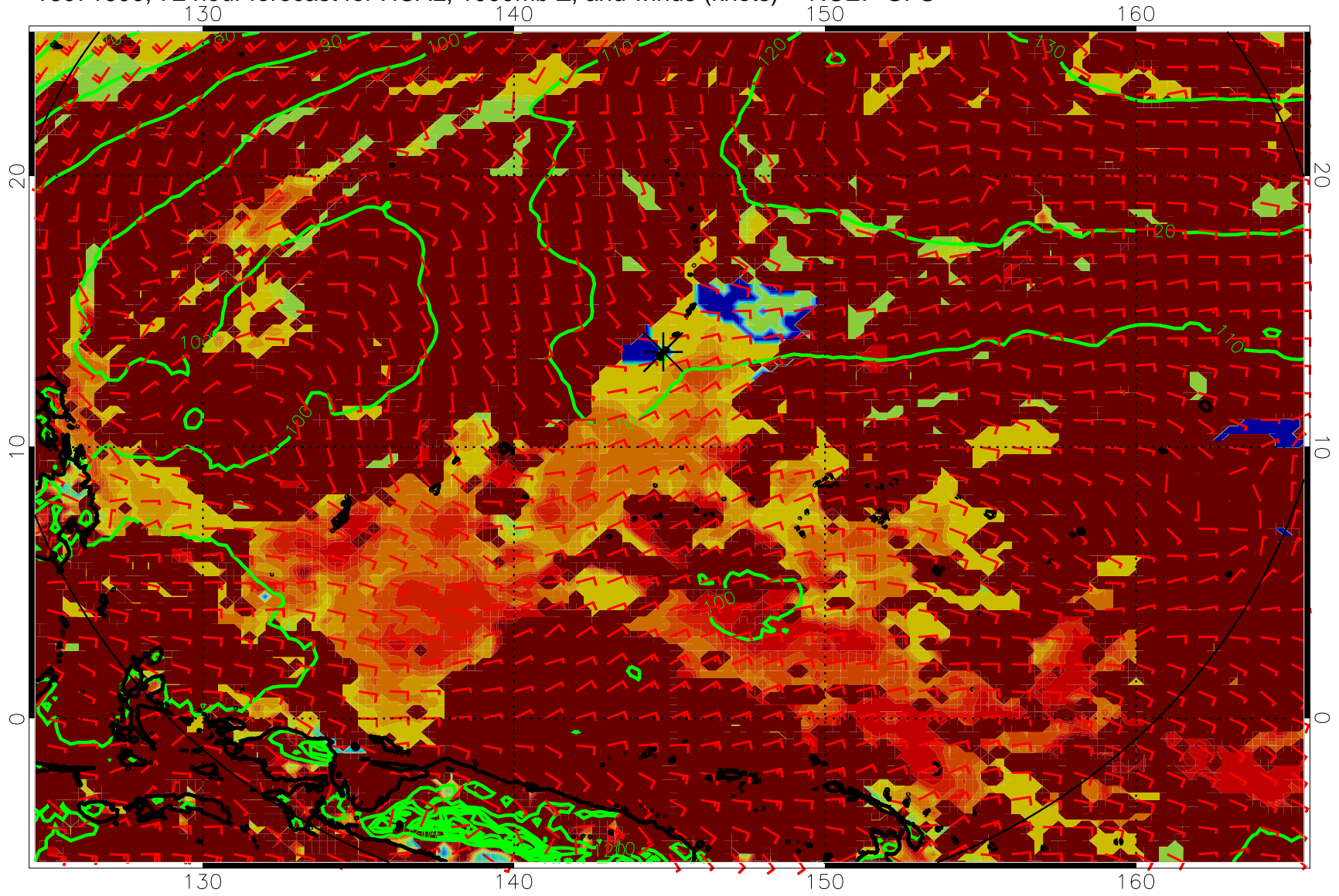
16071600, 72 hour forecast for HCAL, 1000mb Z, and winds (knots) -- NCEP GFS
