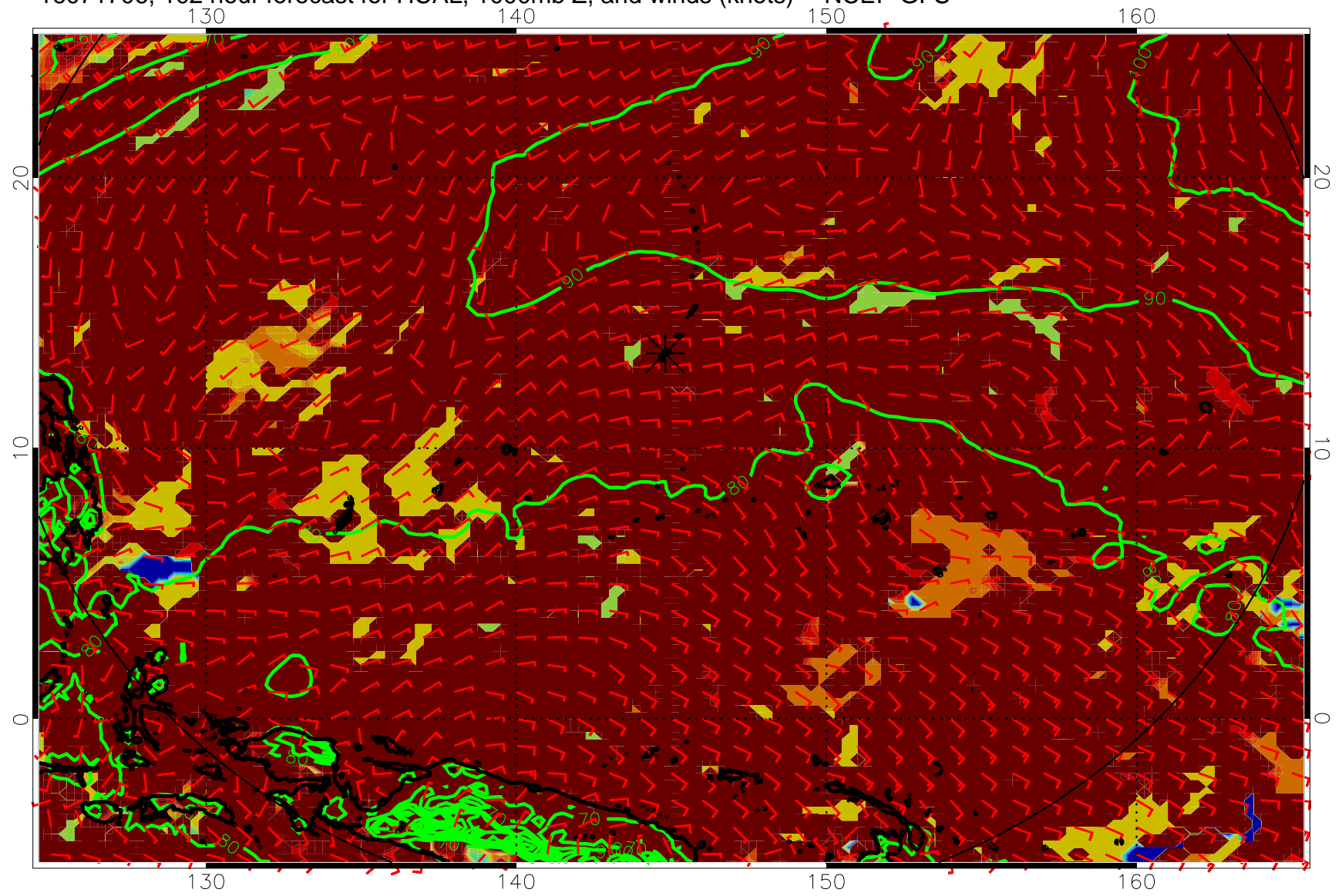
16071706, 102 hour forecast for HCAL, 1000mb Z, and winds (knots) -- NCEP GFS
