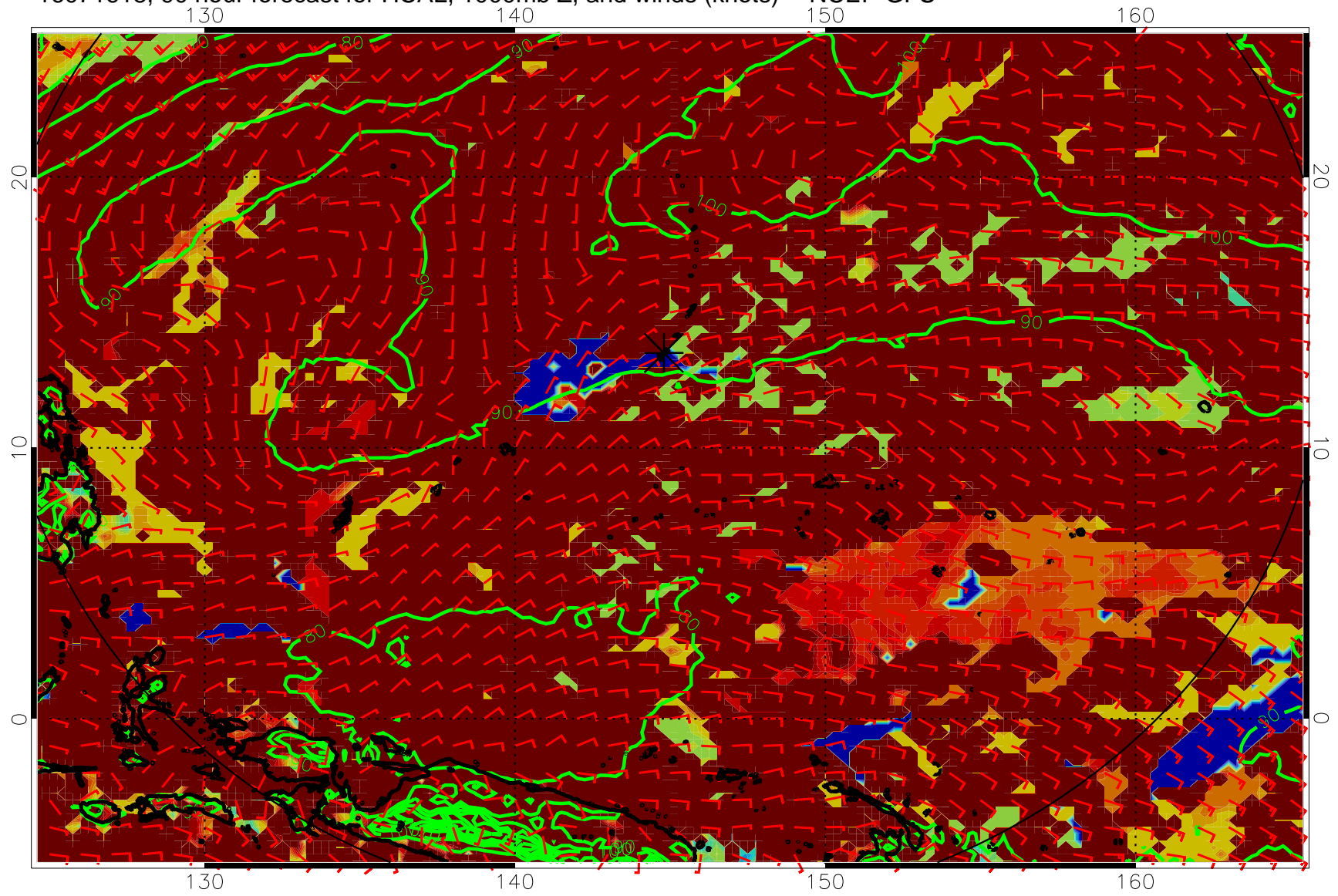
16071618, 90 hour forecast for HCAL, 1000mb Z, and winds (knots) -- NCEP GFS
