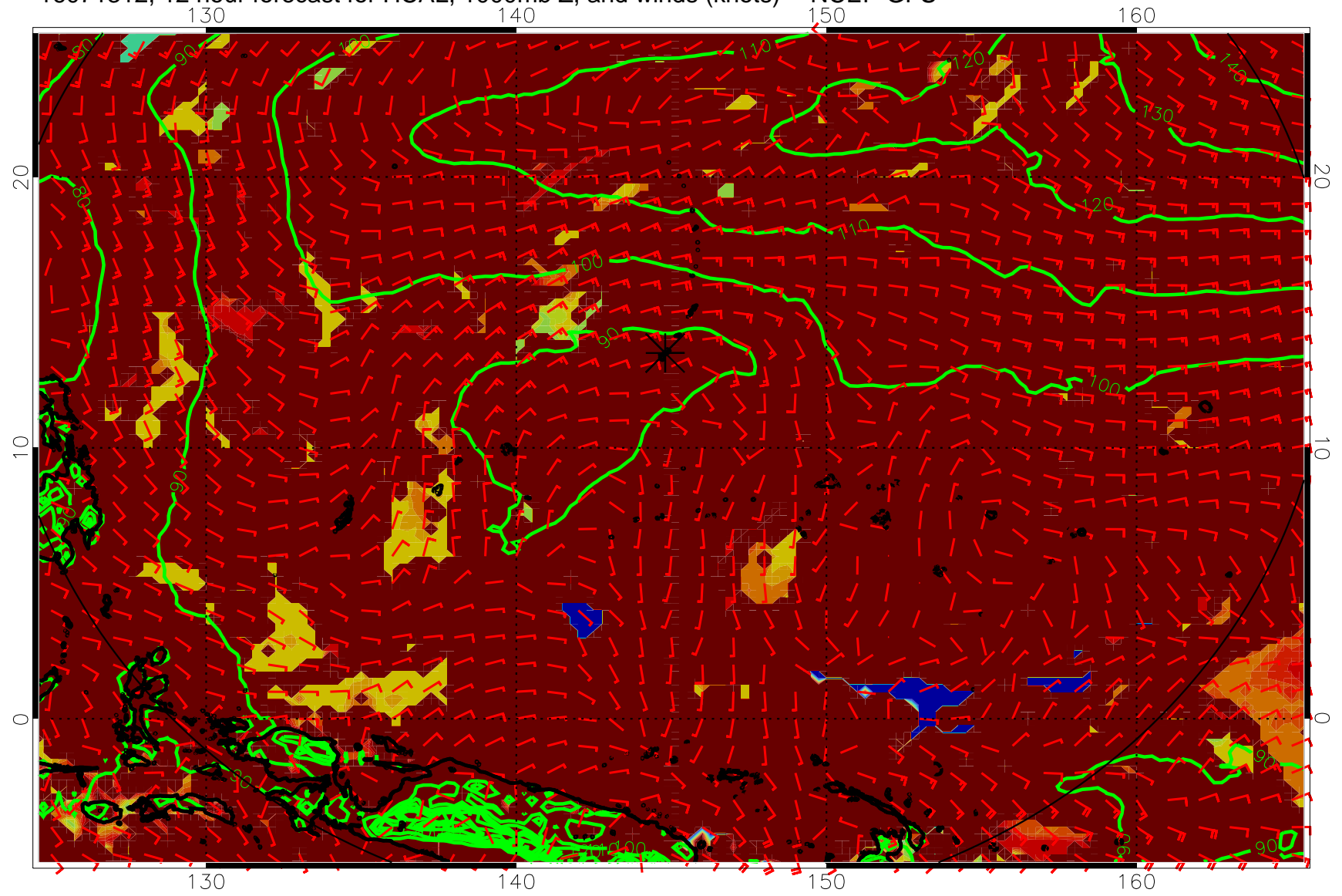
16071312, 12 hour forecast for HCAL, 1000mb Z, and winds (knots) -- NCEP GFS
