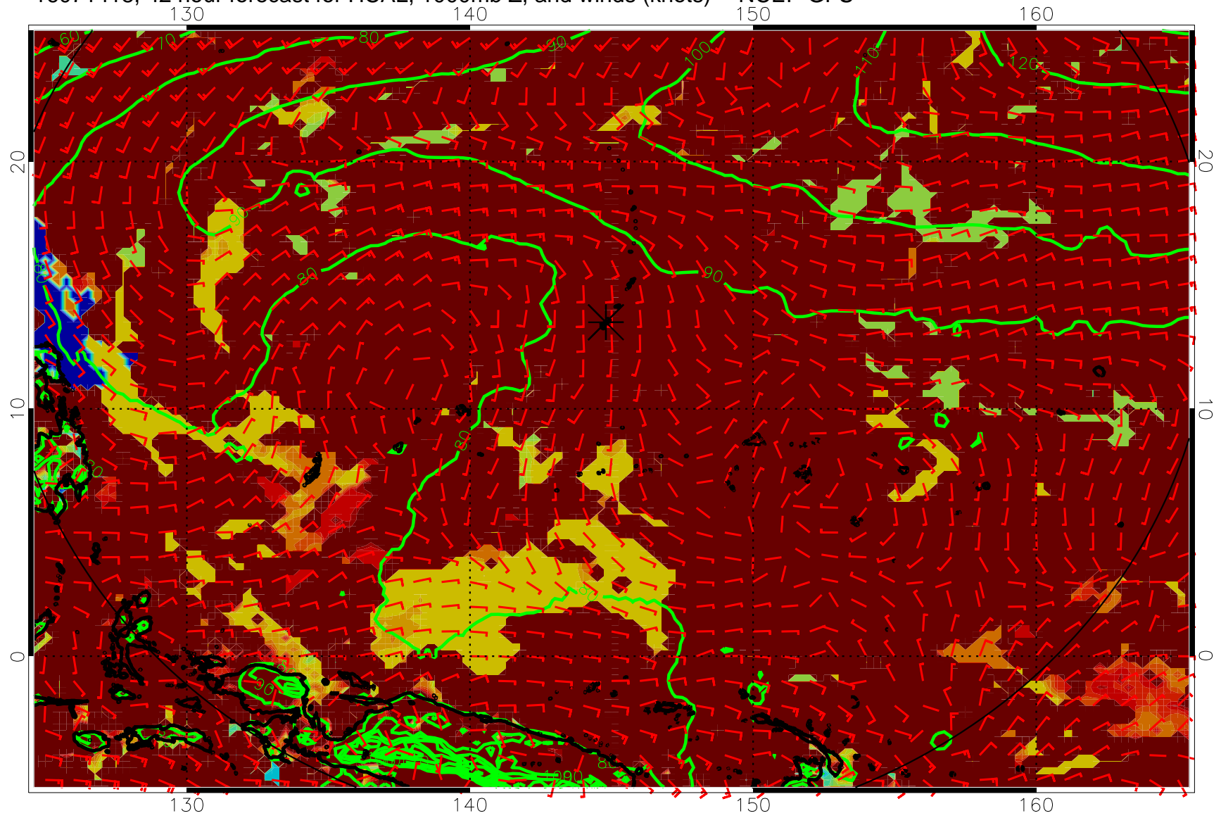
16071418, 42 hour forecast for HCAL, 1000mb Z, and winds (knots) -- NCEP GFS
