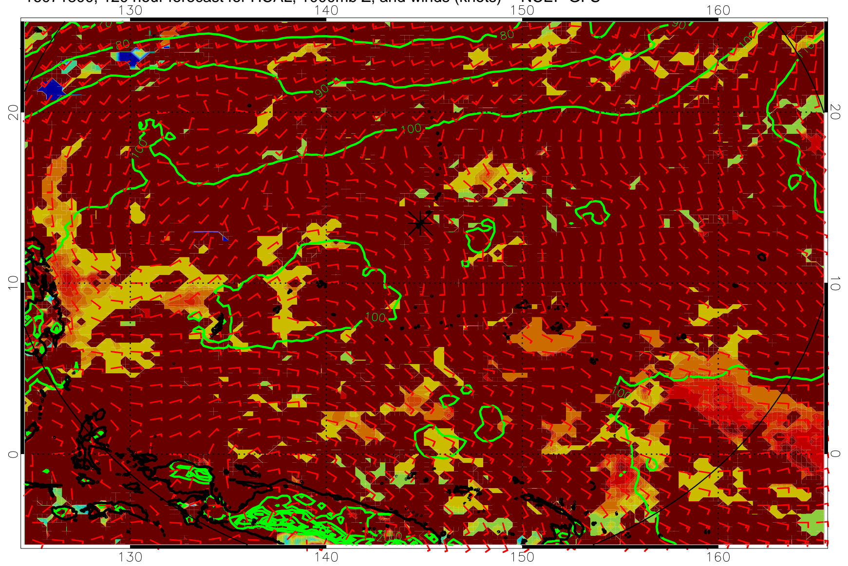
16071800, 120 hour forecast for HCAL, 1000mb Z, and winds (knots) -- NCEP GFS
