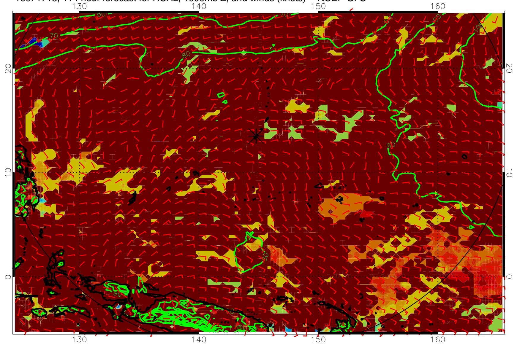
16071718, 114 hour forecast for HCAL, 1000mb Z, and winds (knots) -- NCEP GFS
