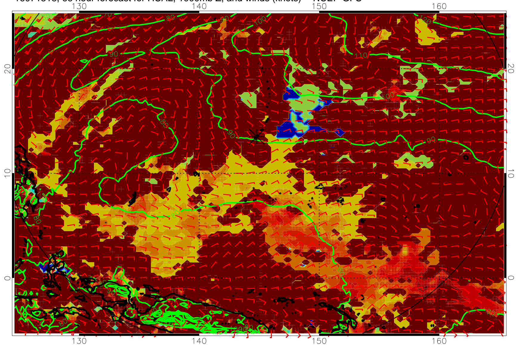
16071518, 66 hour forecast for HCAL, 1000mb Z, and winds (knots) -- NCEP GFS
