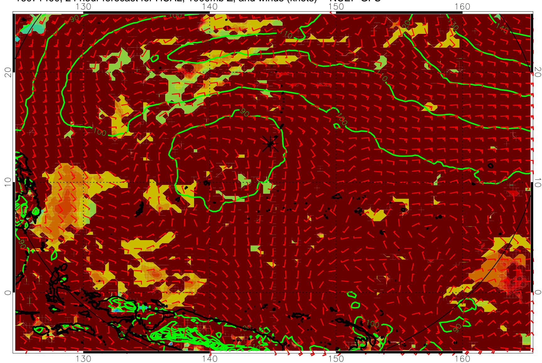
16071400, 24 hour forecast for HCAL, 1000mb Z, and winds (knots) -- NCEP GFS
