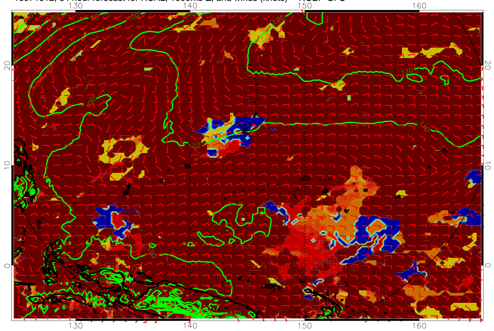
16071612, 84 hour forecast for HCAL, 1000mb Z, and winds (knots) -- NCEP GFS
