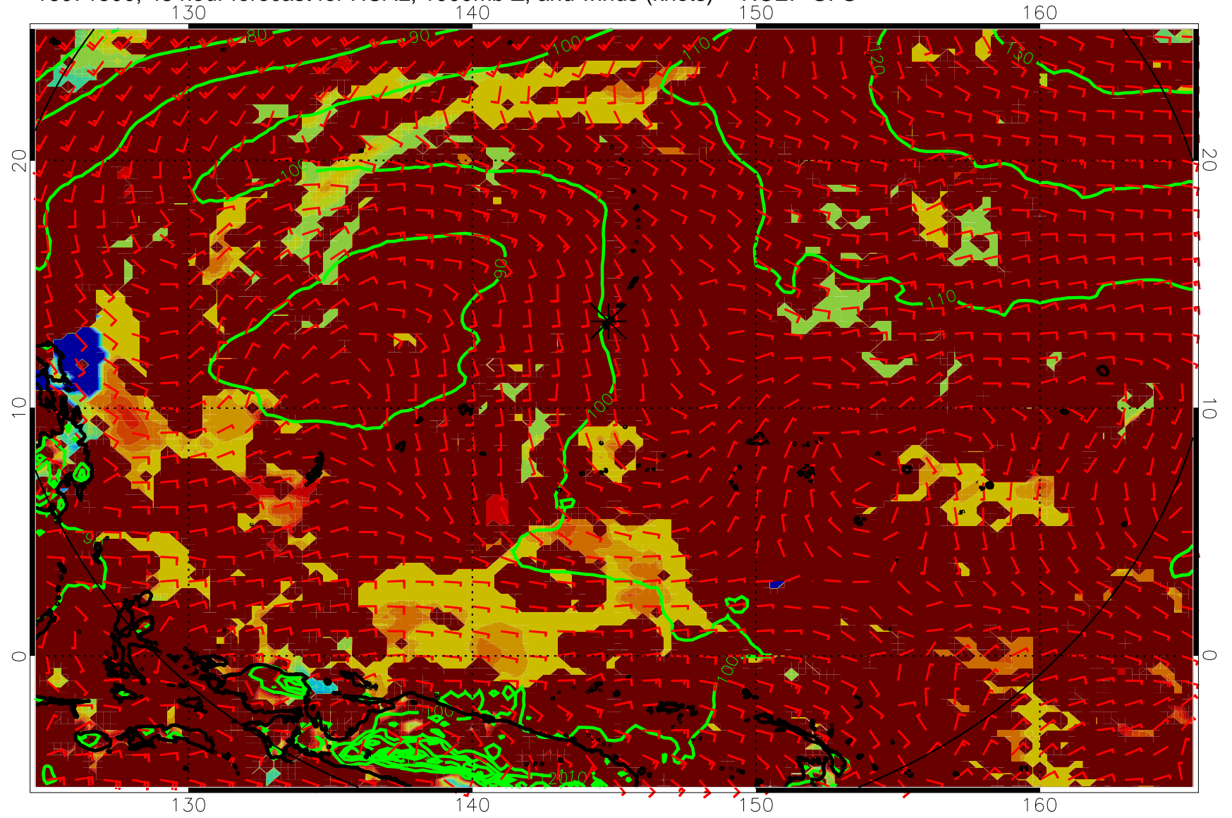
16071500, 48 hour forecast for HCAL, 1000mb Z, and winds (knots) -- NCEP GFS
