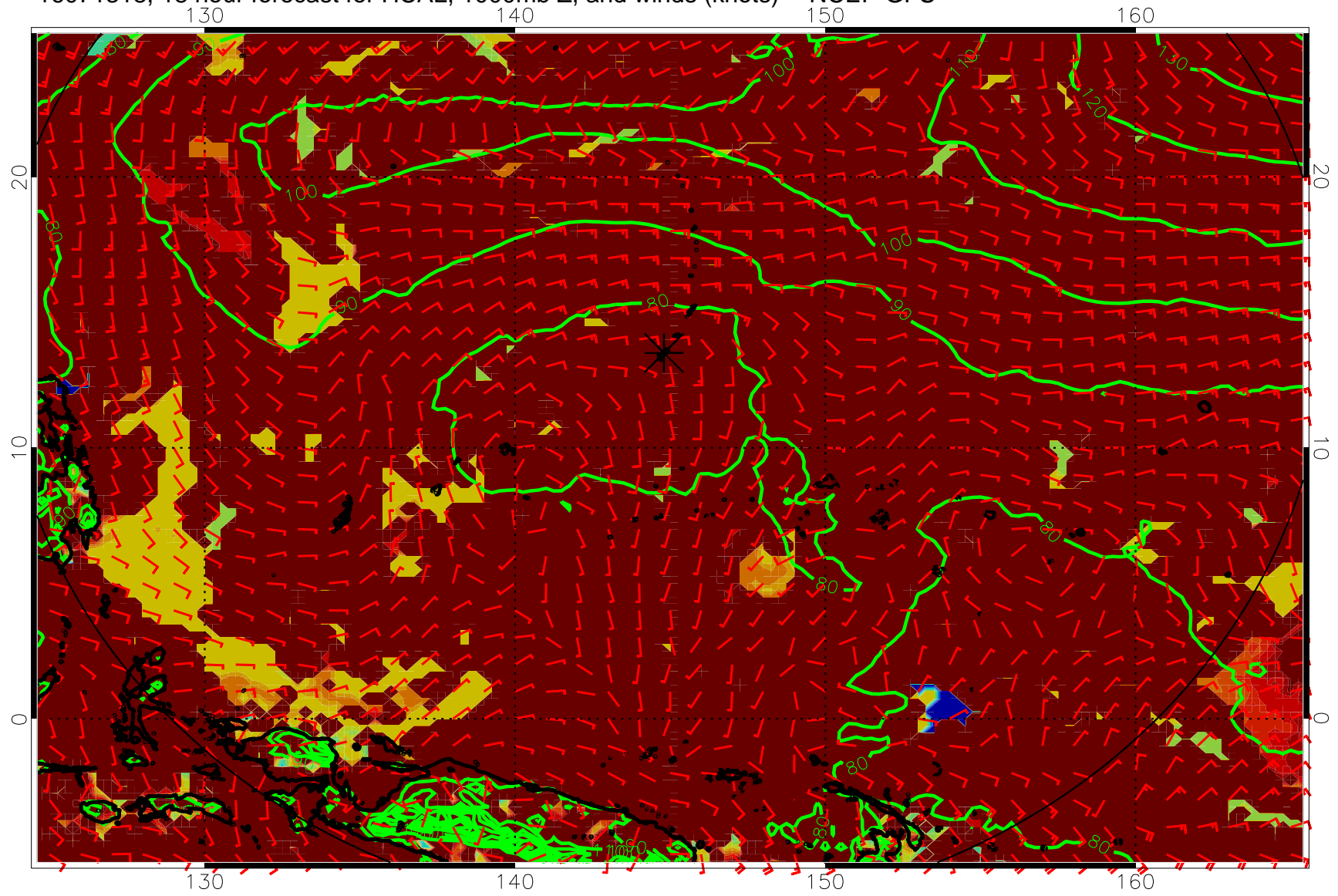
16071318, 18 hour forecast for HCAL, 1000mb Z, and winds (knots) -- NCEP GFS
