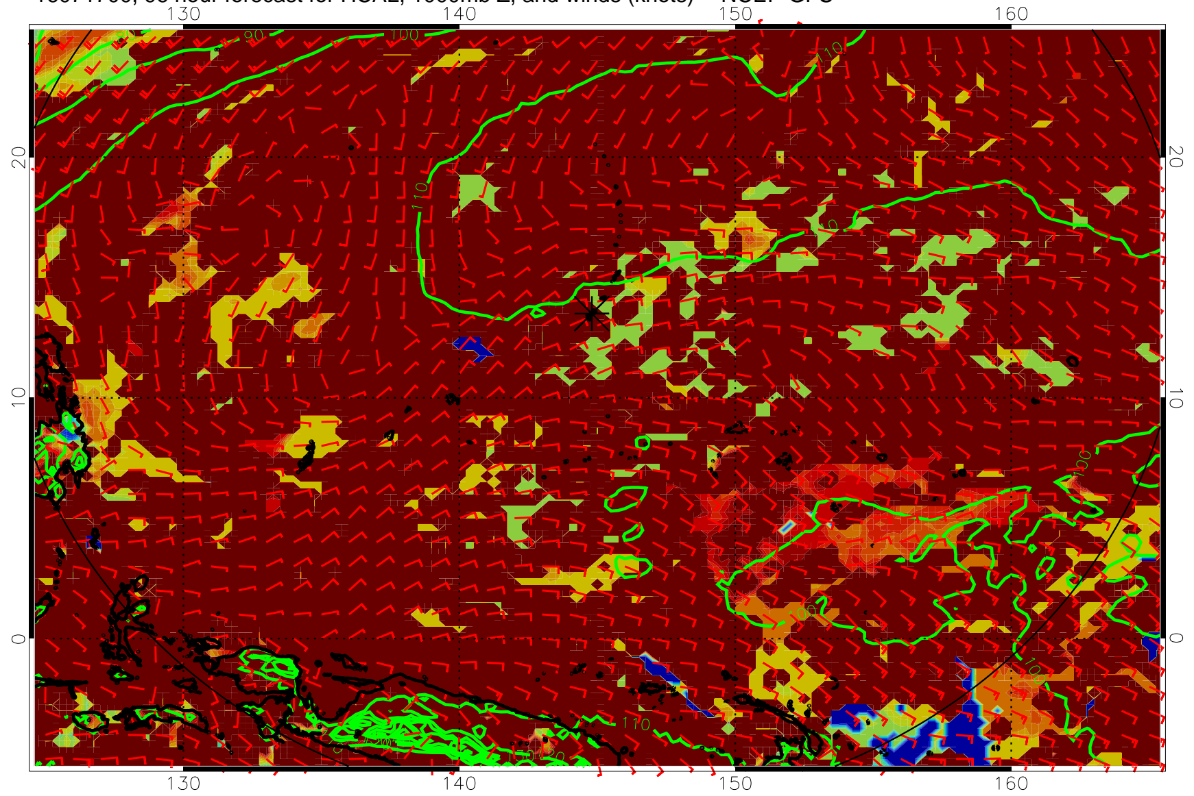
16071700, 96 hour forecast for HCAL, 1000mb Z, and winds (knots) -- NCEP GFS
