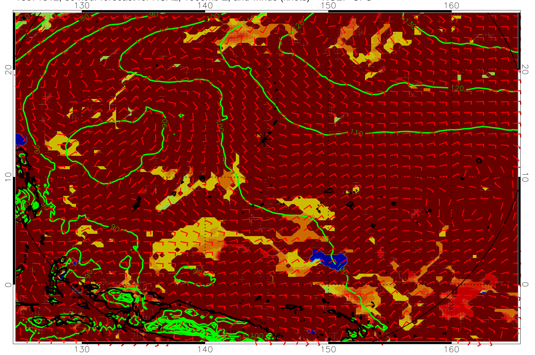
16071512, 60 hour forecast for HCAL, 1000mb Z, and winds (knots) -- NCEP GFS
