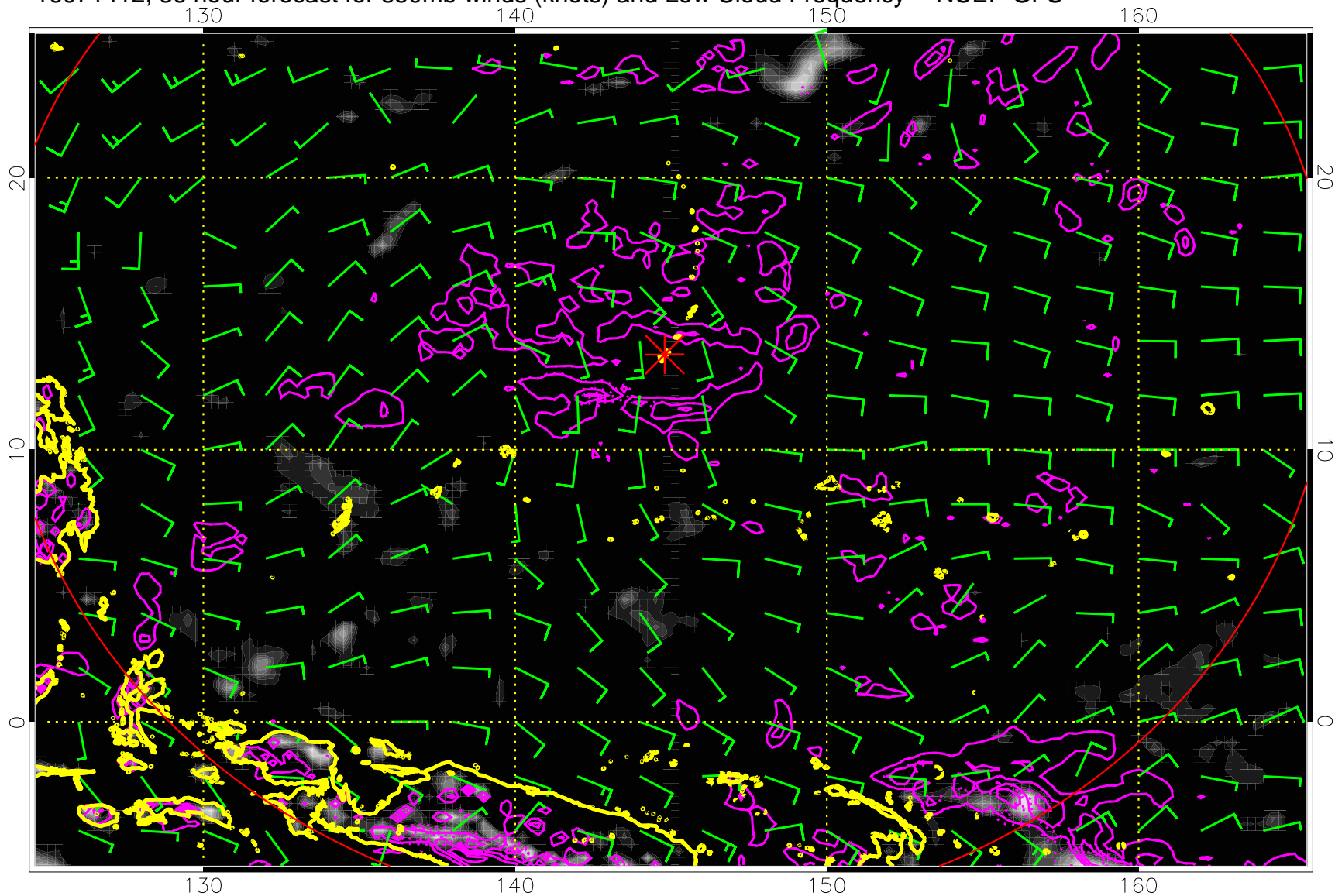
16071412, 36 hour forecast for 850mb winds (knots) and Low Cloud Frequency -- NCEP GFS
