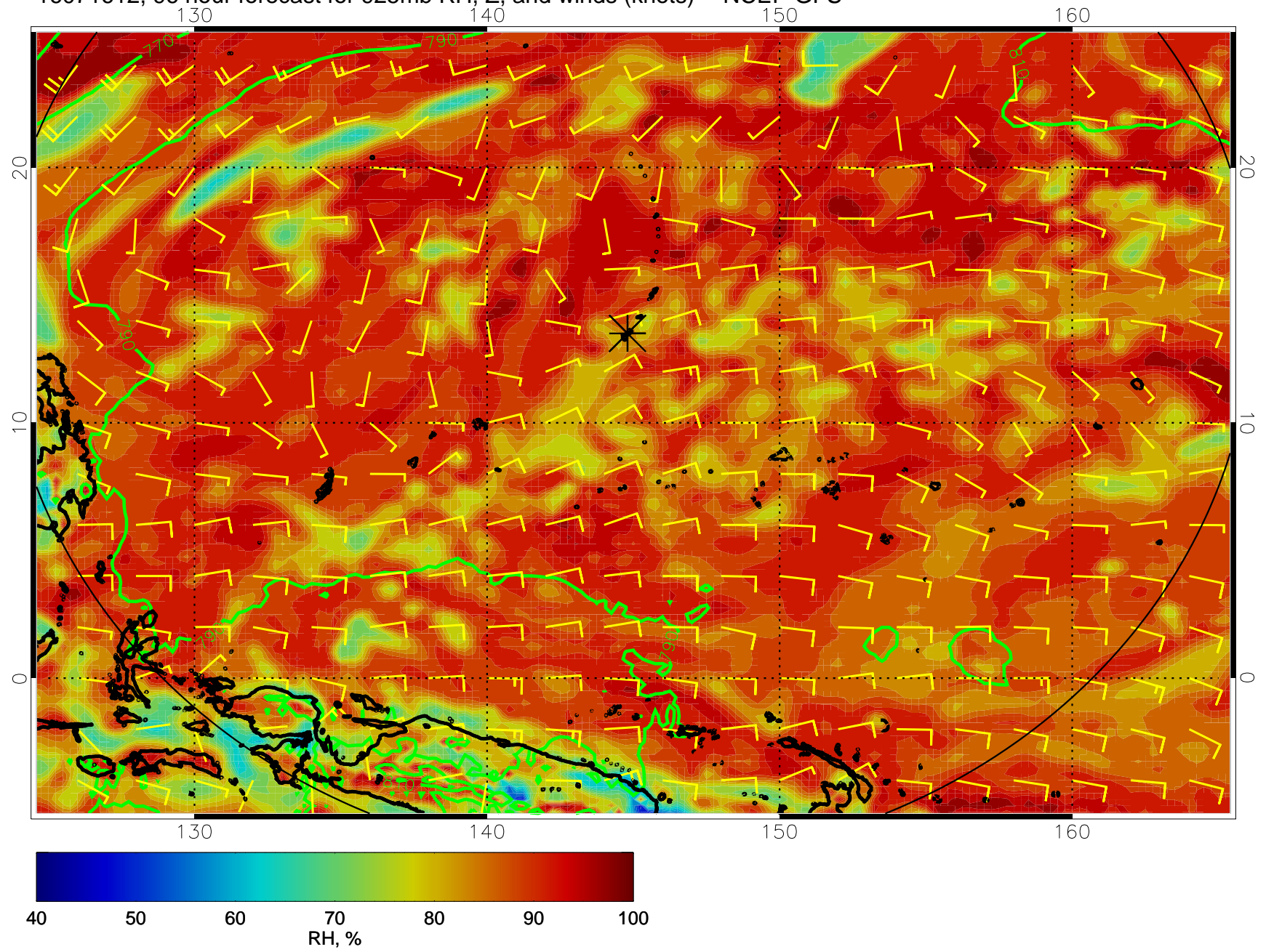
16071612, 96 hour forecast for 925mb RH, Z, and winds (knots) -- NCEP GFS
