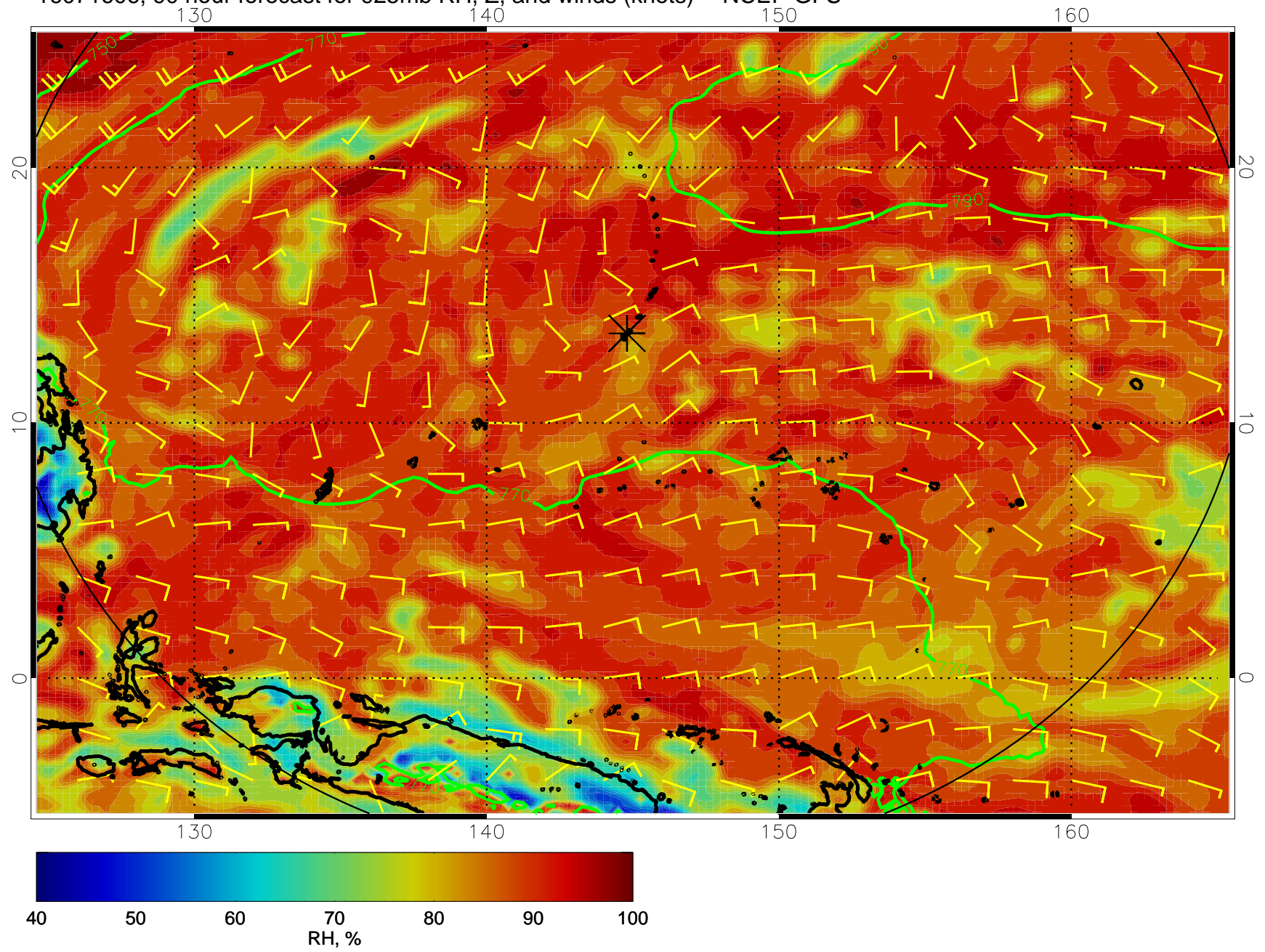
16071606, 90 hour forecast for 925mb RH, Z, and winds (knots) -- NCEP GFS
