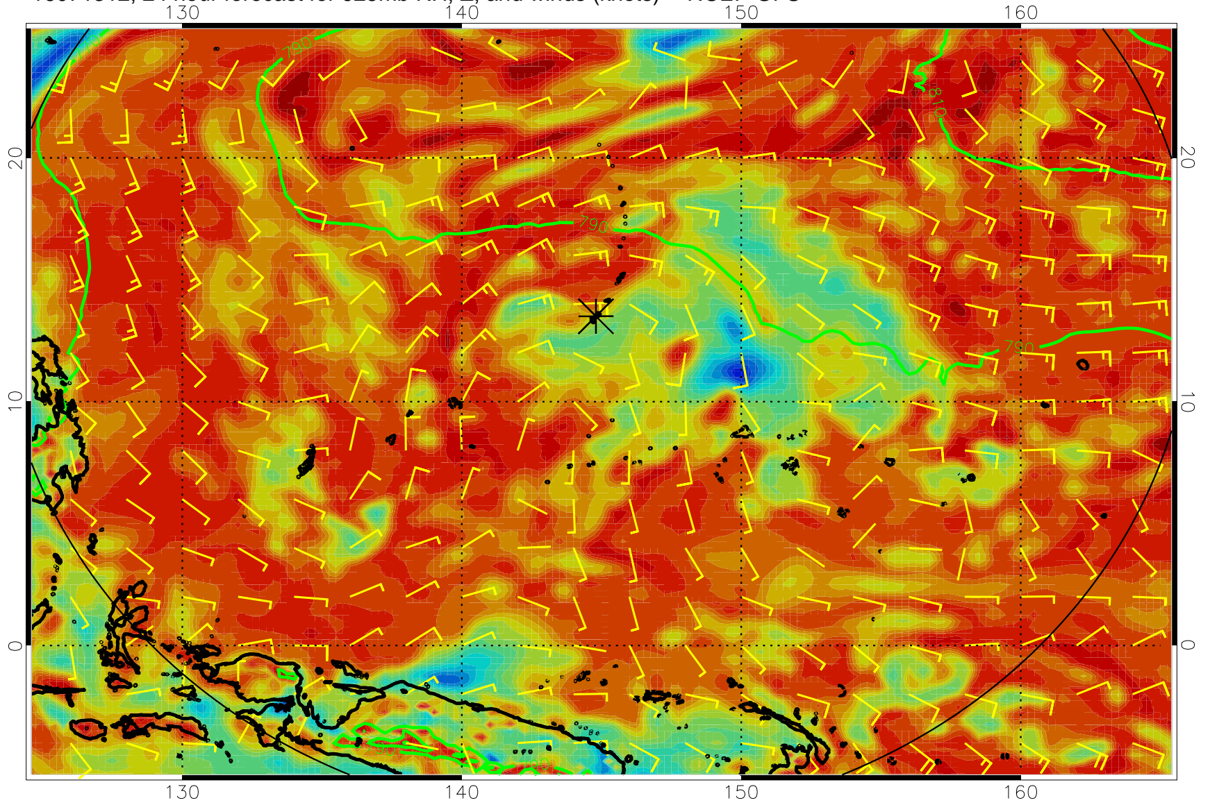
16071312, 24 hour forecast for 925mb RH, Z, and winds (knots) -- NCEP GFS
