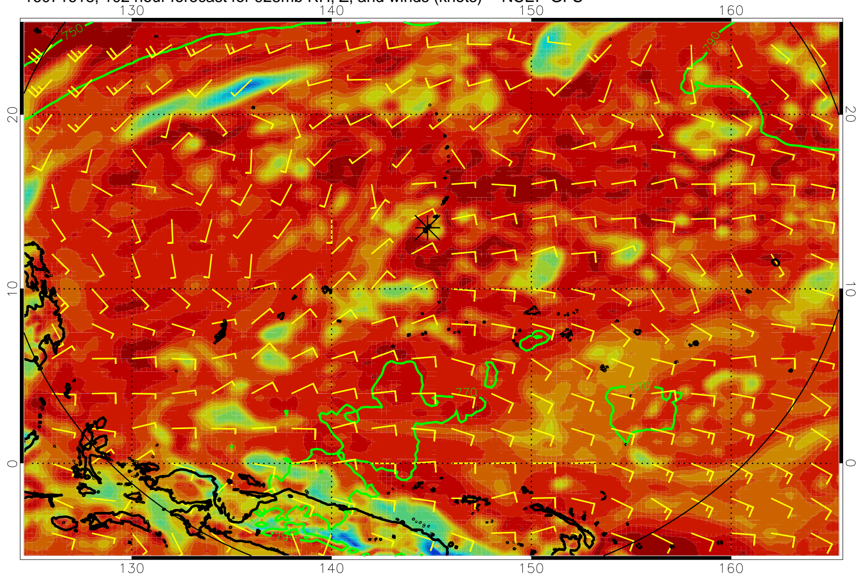
16071618, 102 hour forecast for 925mb RH, Z, and winds (knots) -- NCEP GFS
