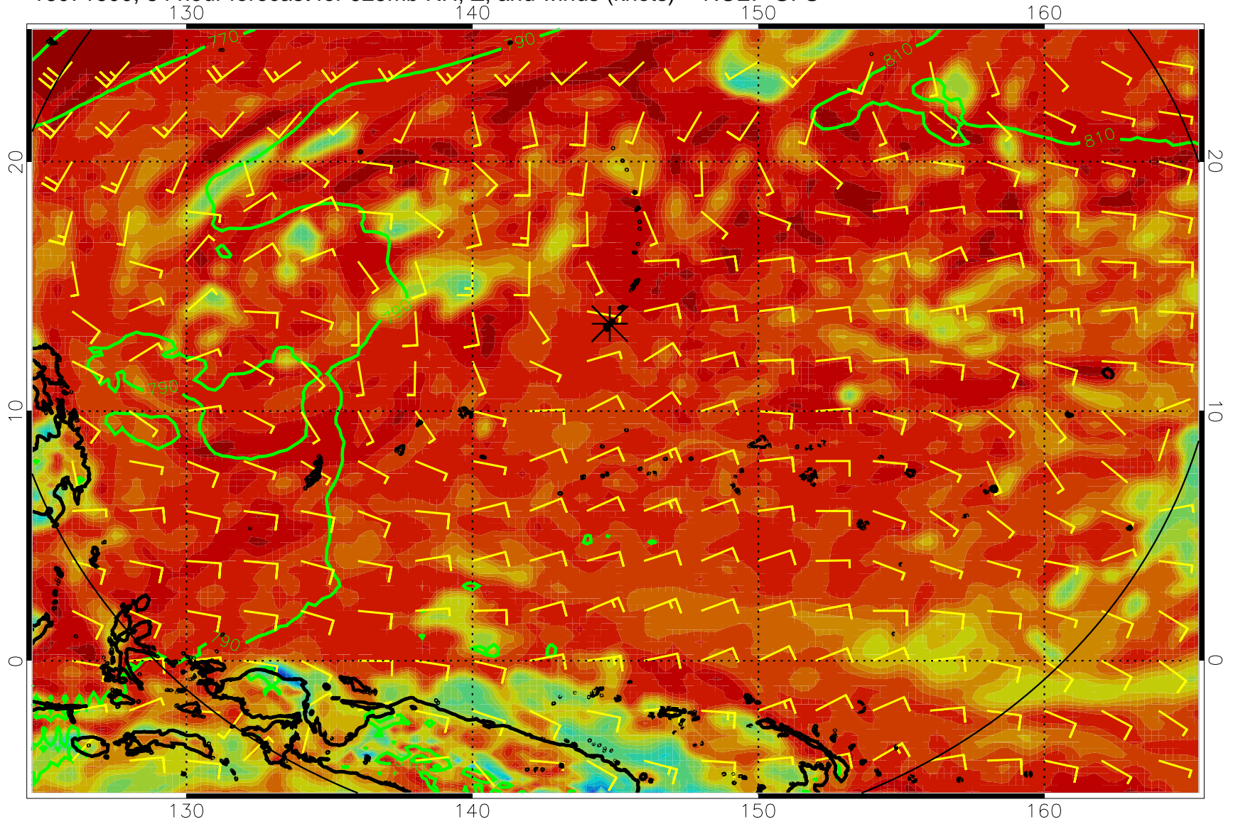
16071600, 84 hour forecast for 925mb RH, Z, and winds (knots) -- NCEP GFS
