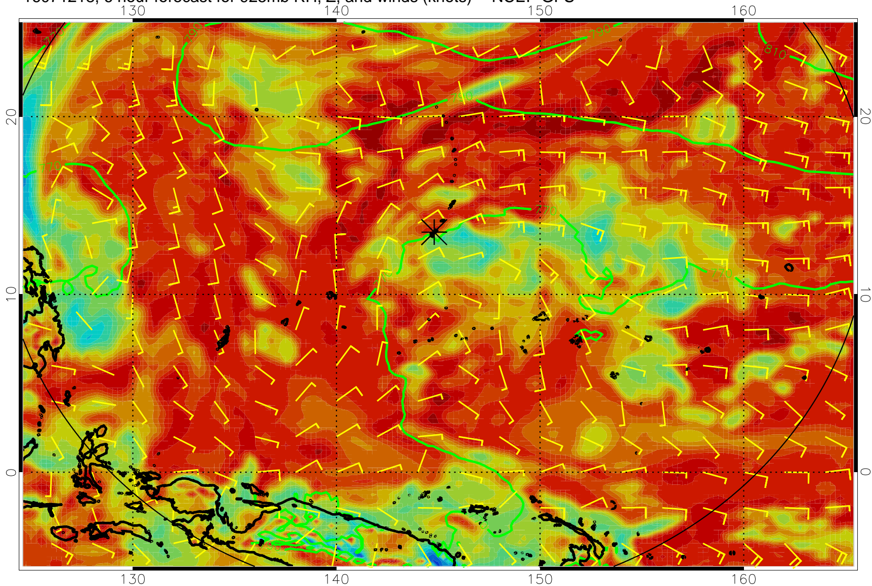
16071218, 6 hour forecast for 925mb RH, Z, and winds (knots) -- NCEP GFS
