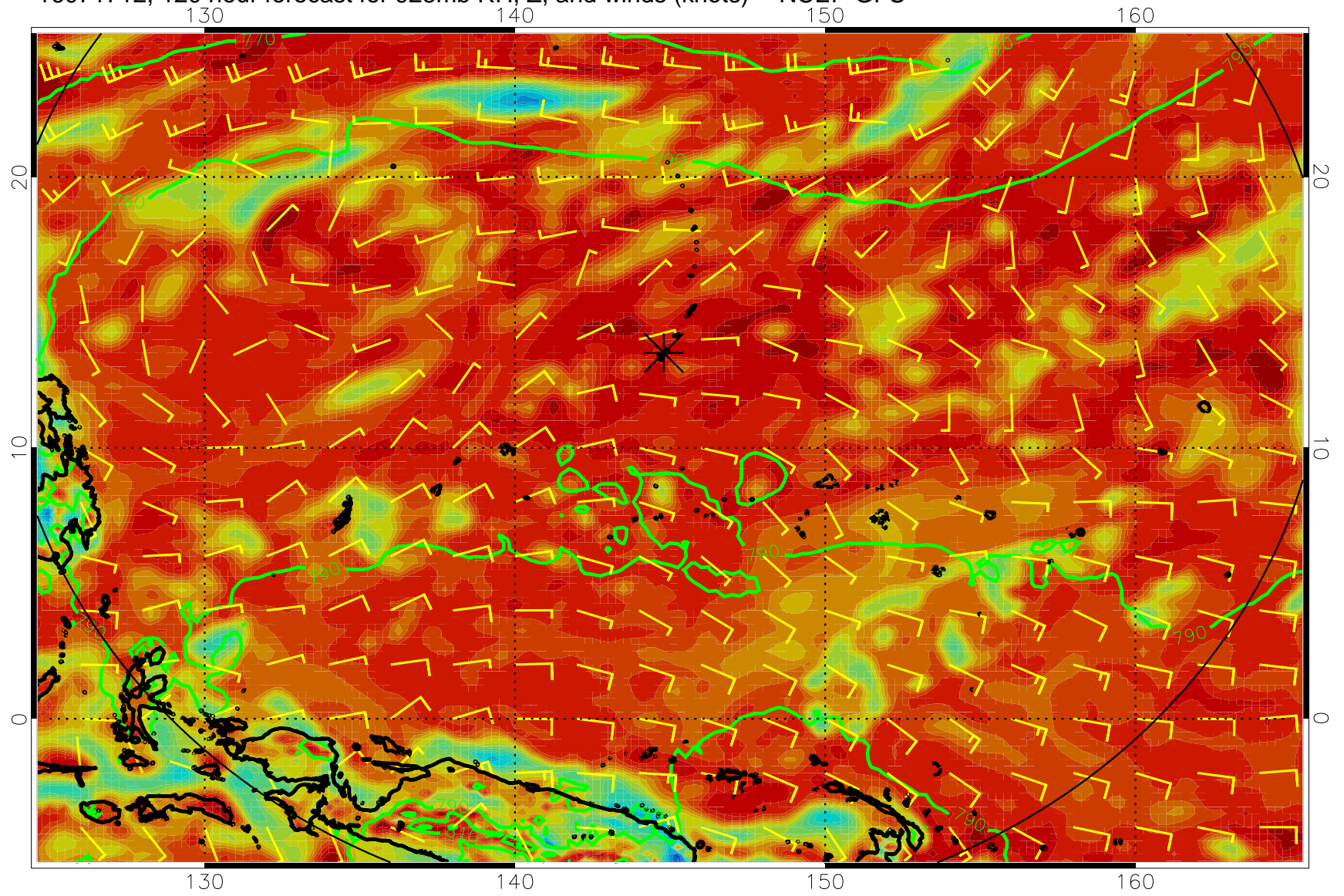
16071712, 120 hour forecast for 925mb RH, Z, and winds (knots) -- NCEP GFS
