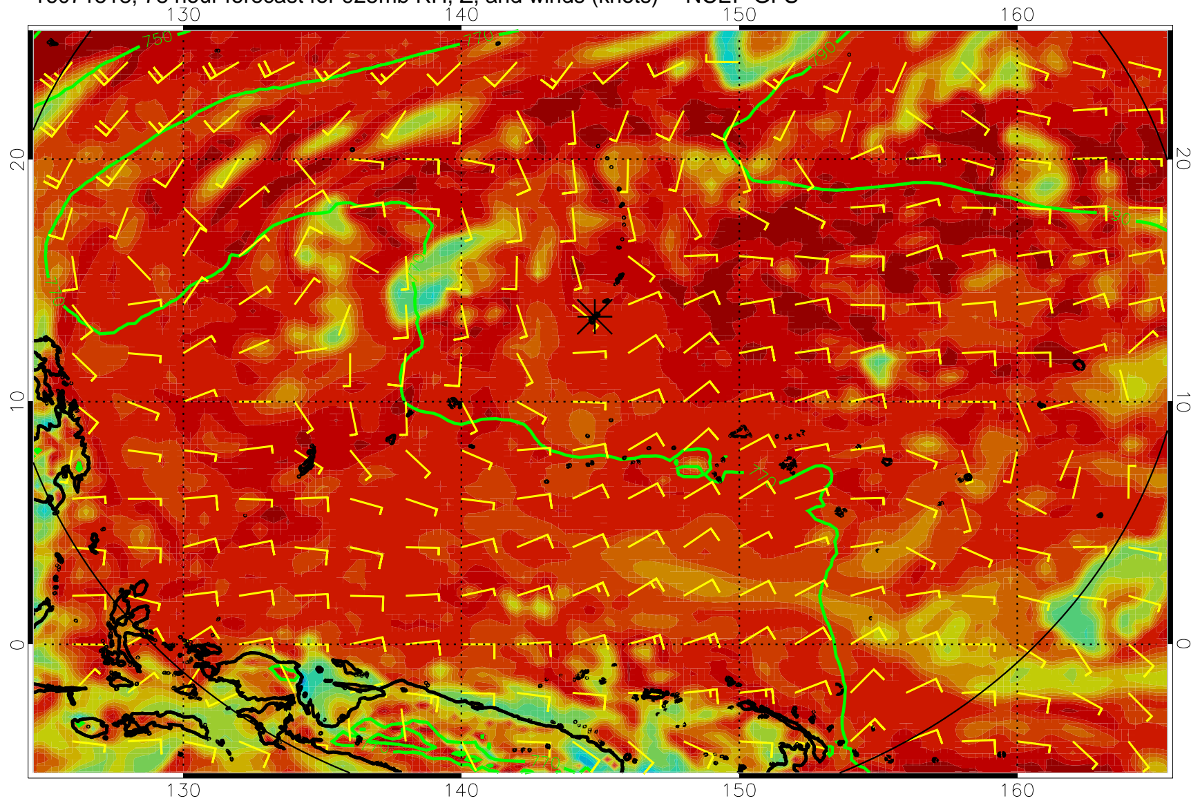
16071518, 78 hour forecast for 925mb RH, Z, and winds (knots) -- NCEP GFS
