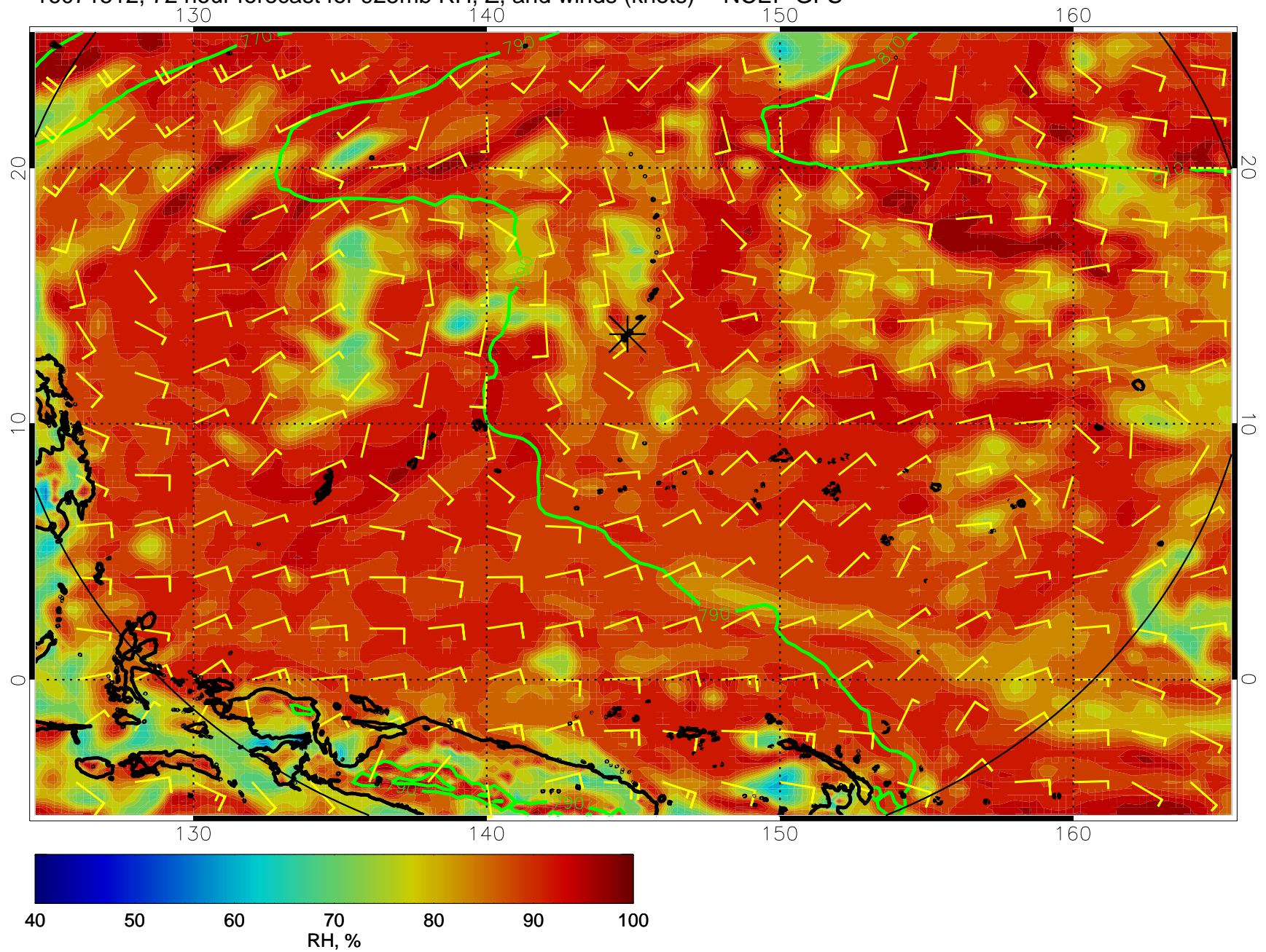
16071512, 72 hour forecast for 925mb RH, Z, and winds (knots) -- NCEP GFS
