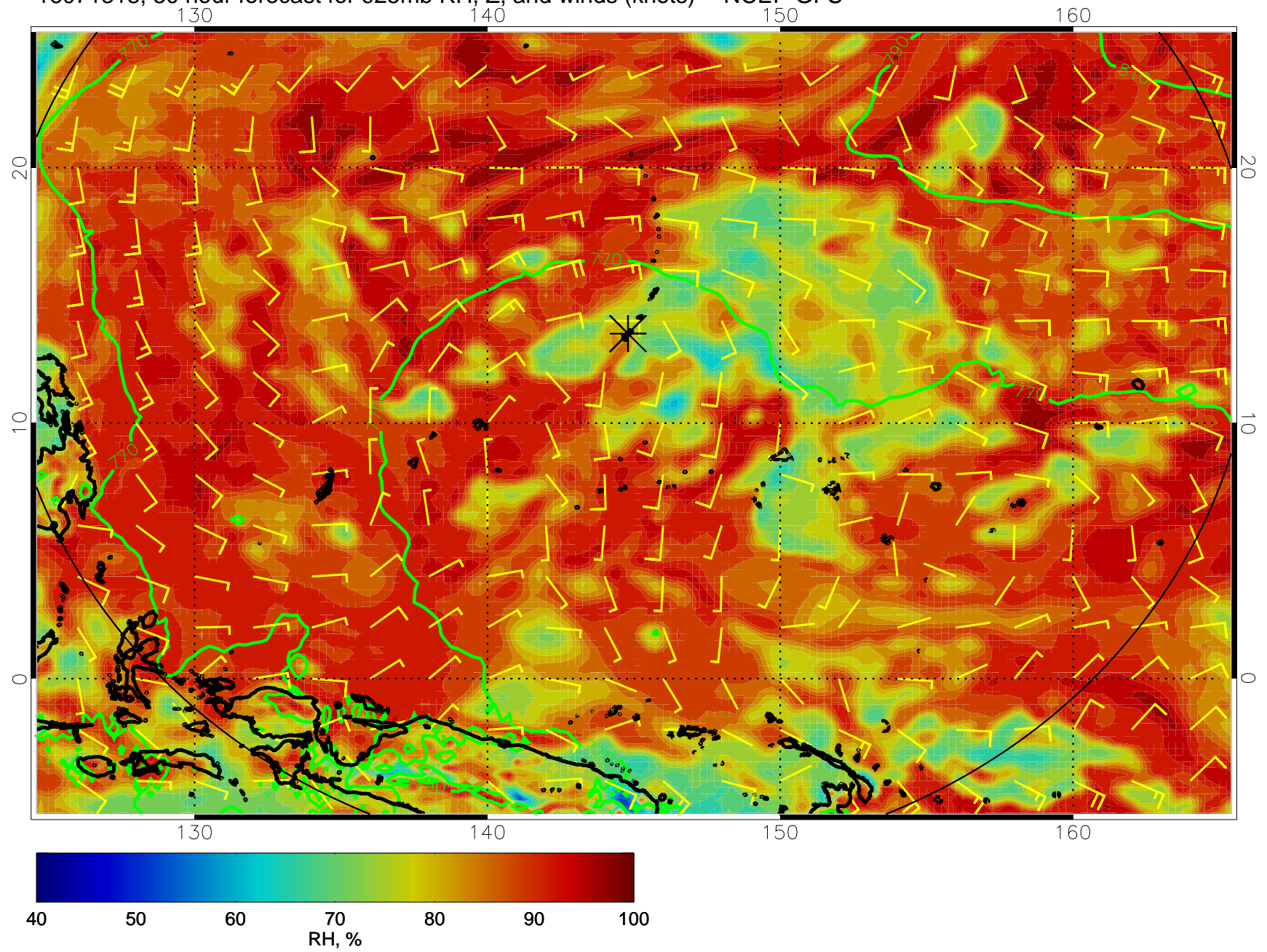
16071318, 30 hour forecast for 925mb RH, Z, and winds (knots) -- NCEP GFS
