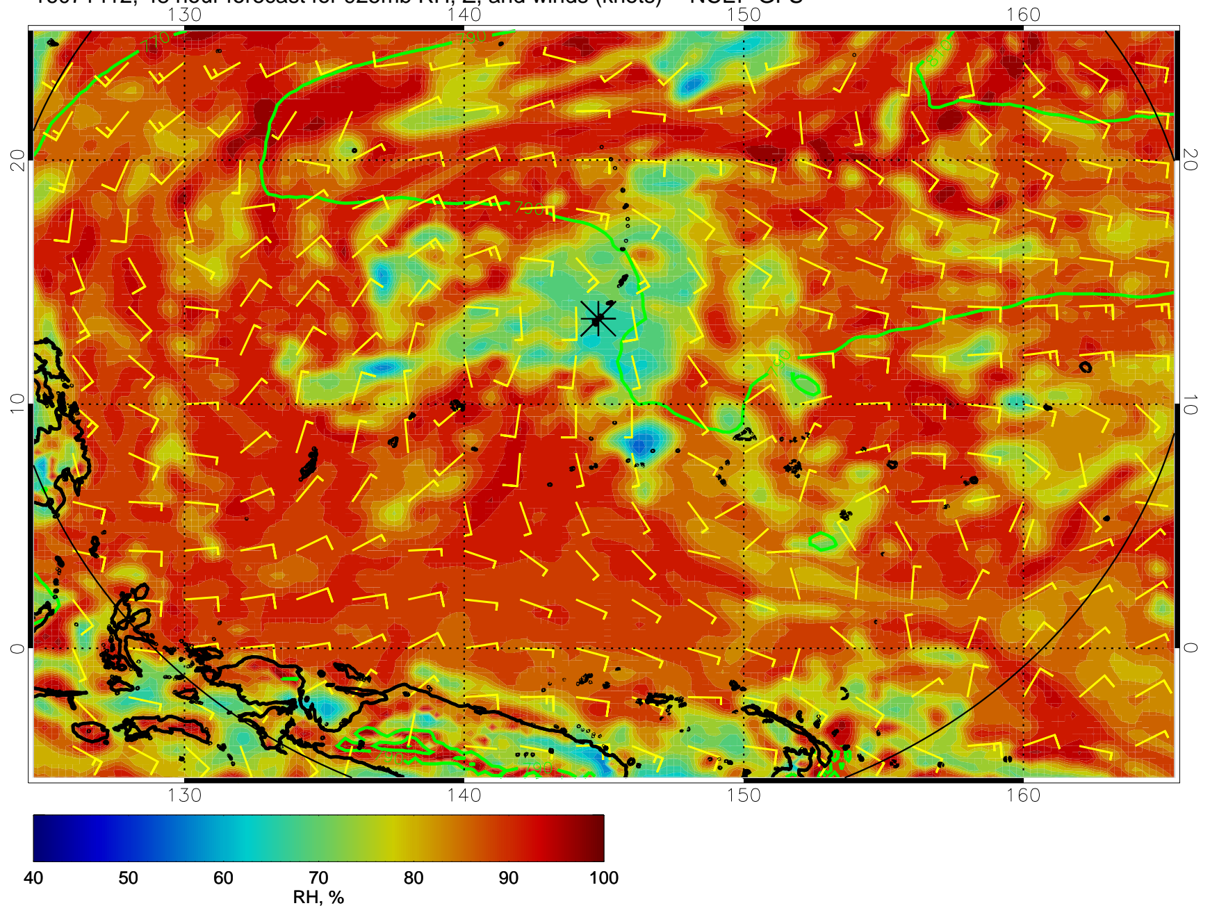
16071412, 48 hour forecast for 925mb RH, Z, and winds (knots) -- NCEP GFS
