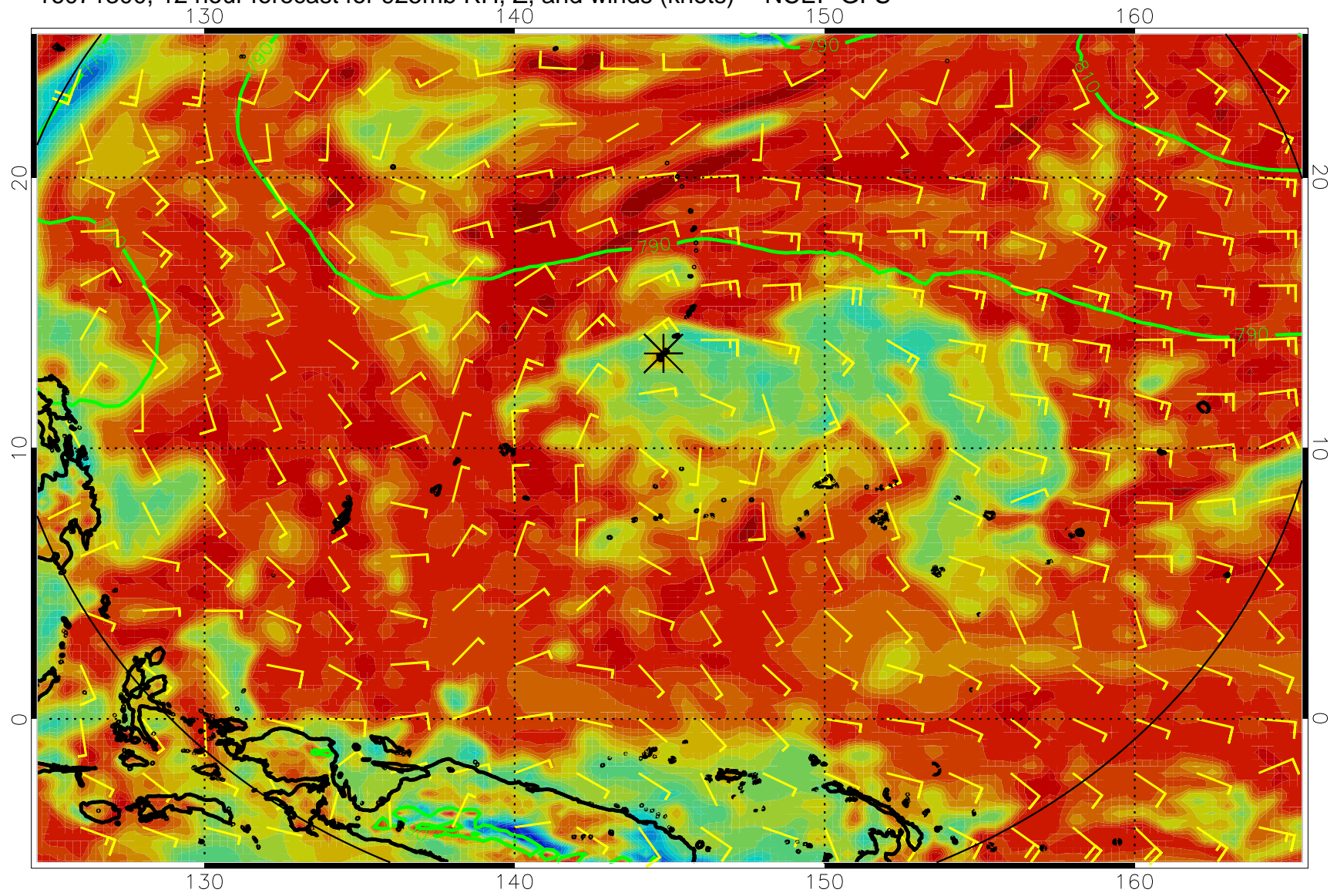
16071300, 12 hour forecast for 925mb RH, Z, and winds (knots) -- NCEP GFS
