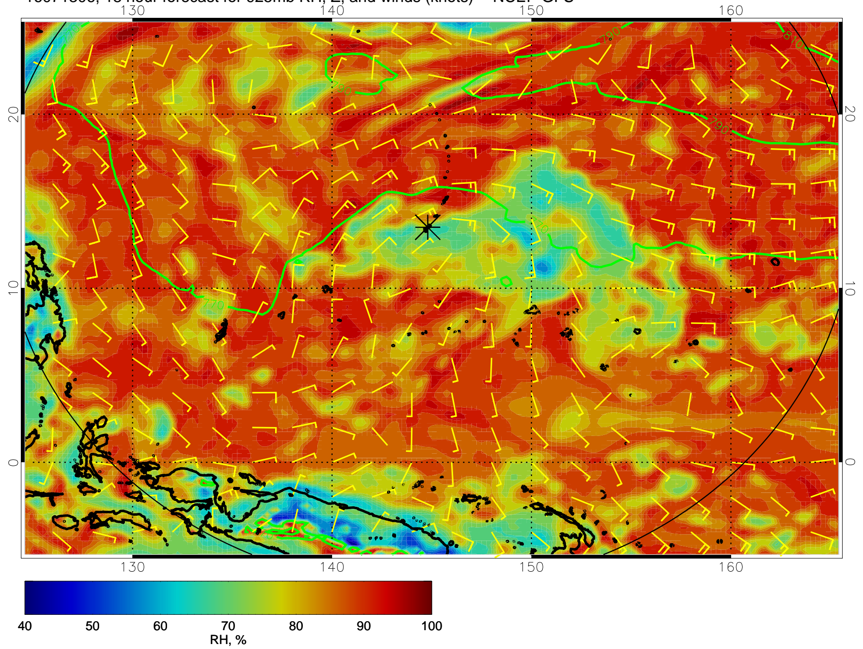
16071306, 18 hour forecast for 925mb RH, Z, and winds (knots) -- NCEP GFS
