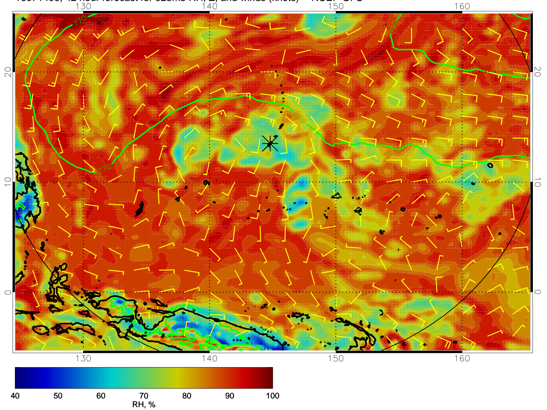
16071406, 42 hour forecast for 925mb RH, Z, and winds (knots) -- NCEP GFS
