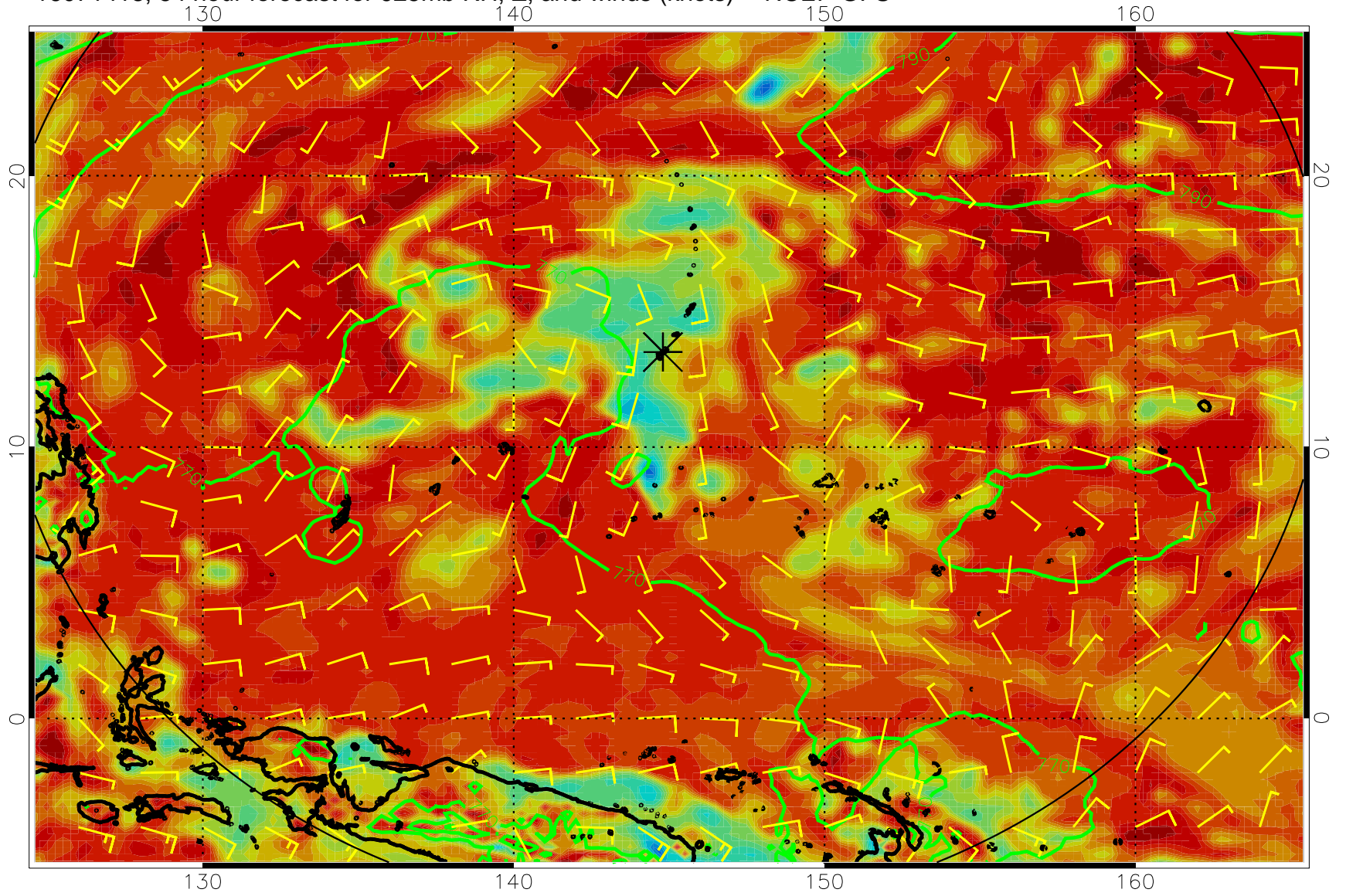
16071418, 54 hour forecast for 925mb RH, Z, and winds (knots) -- NCEP GFS
