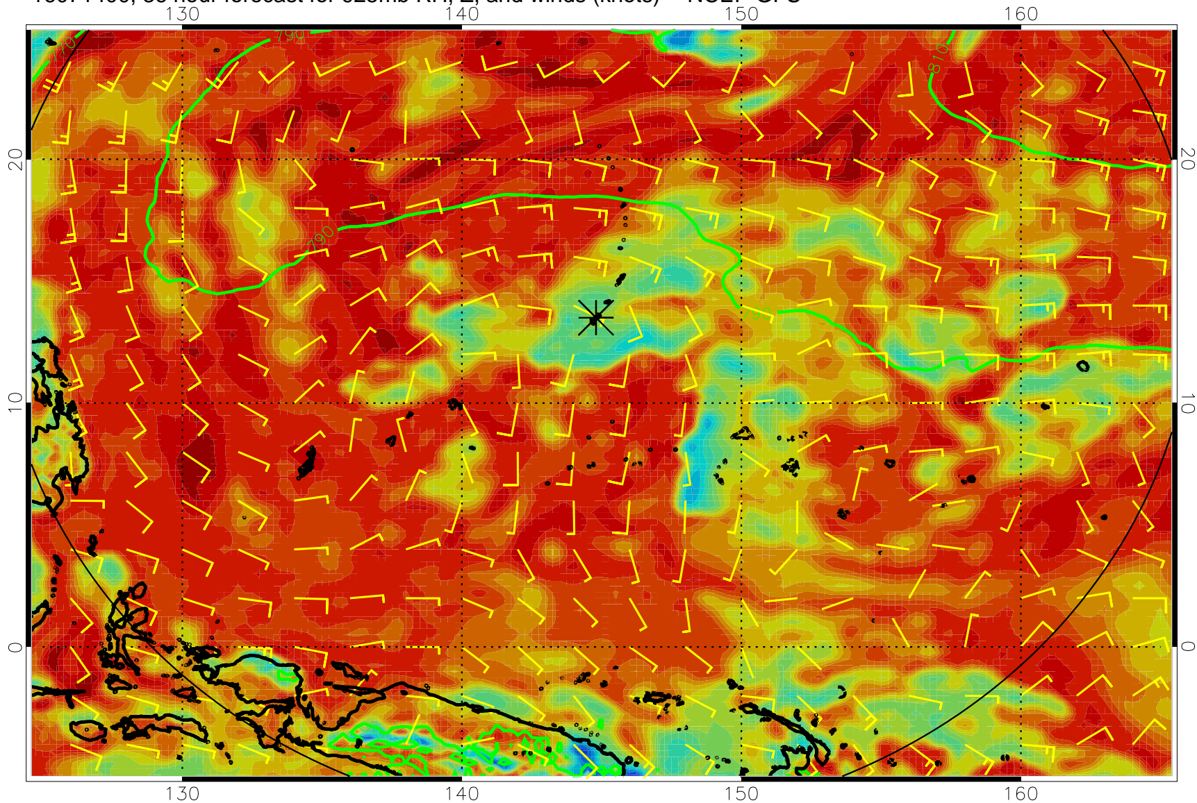
16071400, 36 hour forecast for 925mb RH, Z, and winds (knots) -- NCEP GFS
