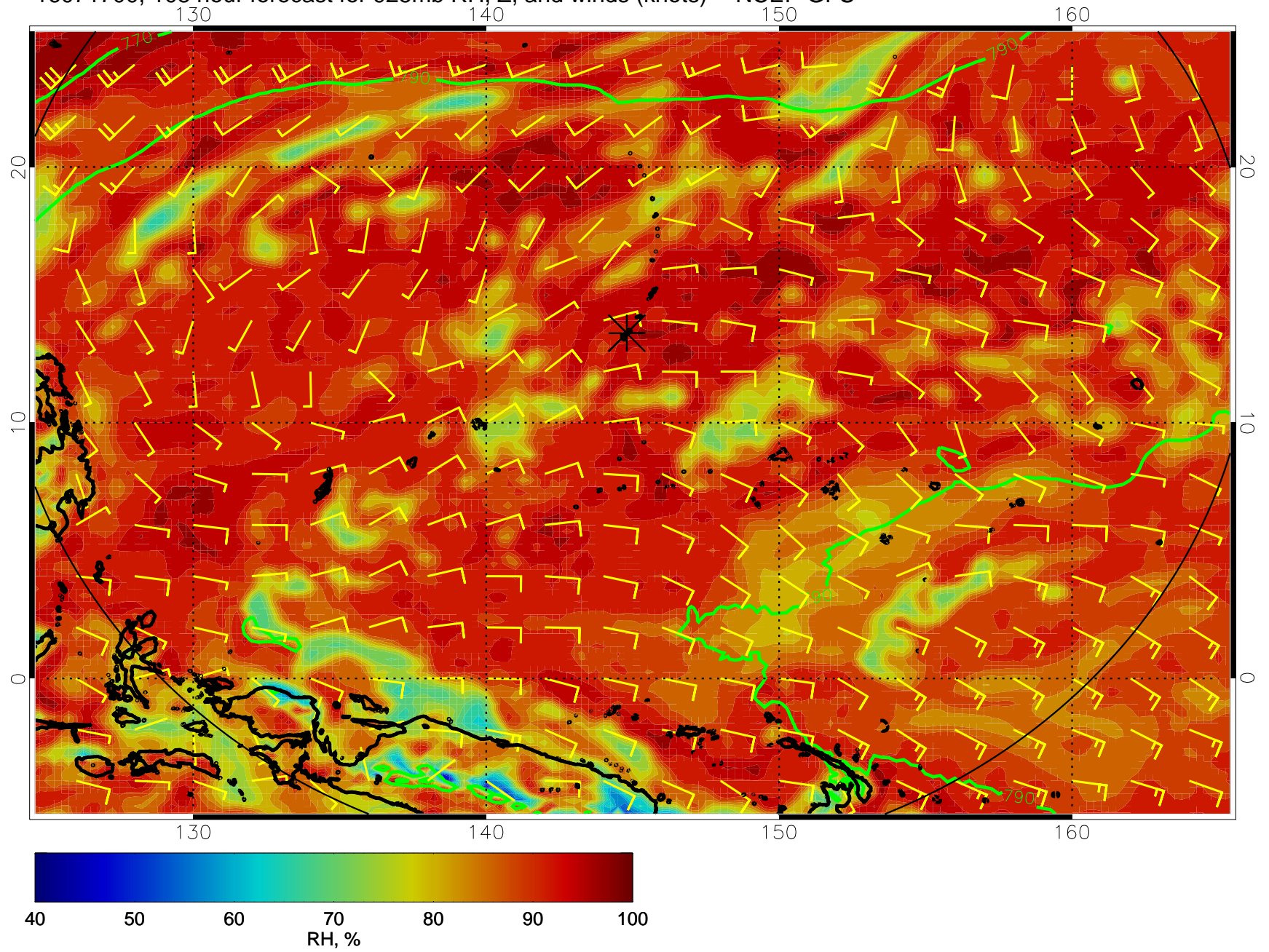
16071700, 108 hour forecast for 925mb RH, Z, and winds (knots) -- NCEP GFS
