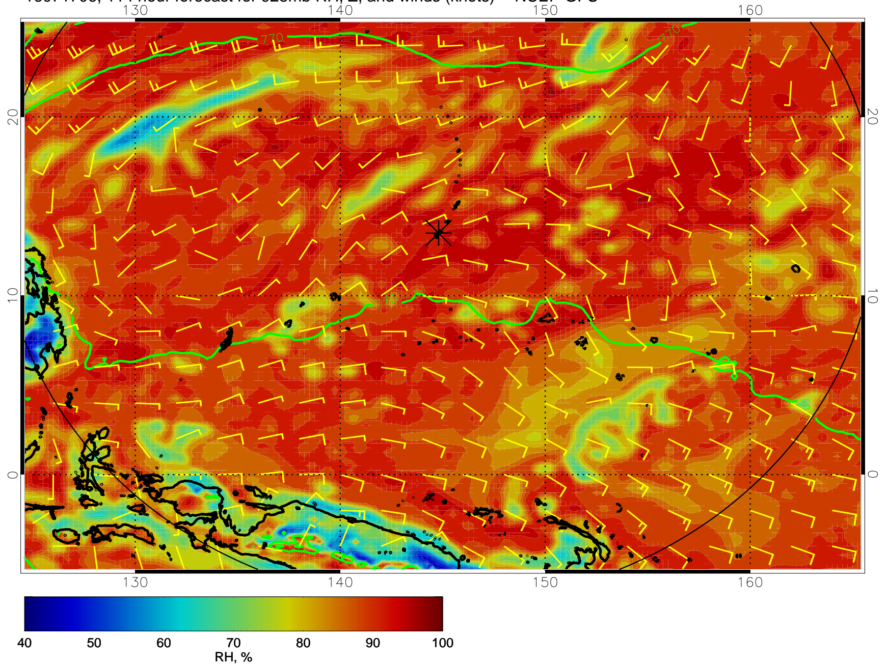
16071706, 114 hour forecast for 925mb RH, Z, and winds (knots) -- NCEP GFS
