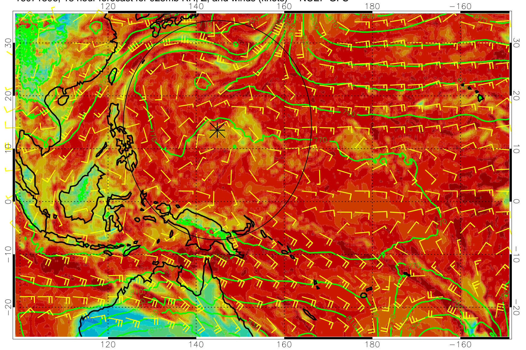
16071306, 18 hour forecast for 925mb RH, Z, and winds (knots) -- NCEP GFS
