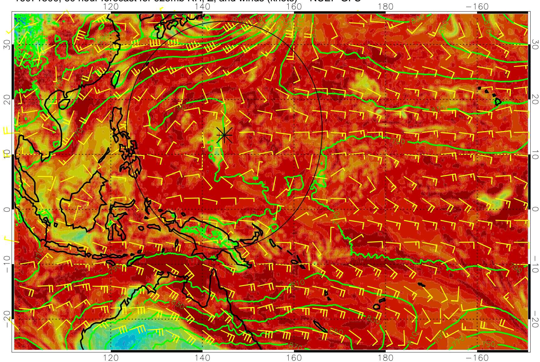
16071500, 60 hour forecast for 925mb RH, Z, and winds (knots) -- NCEP GFS
