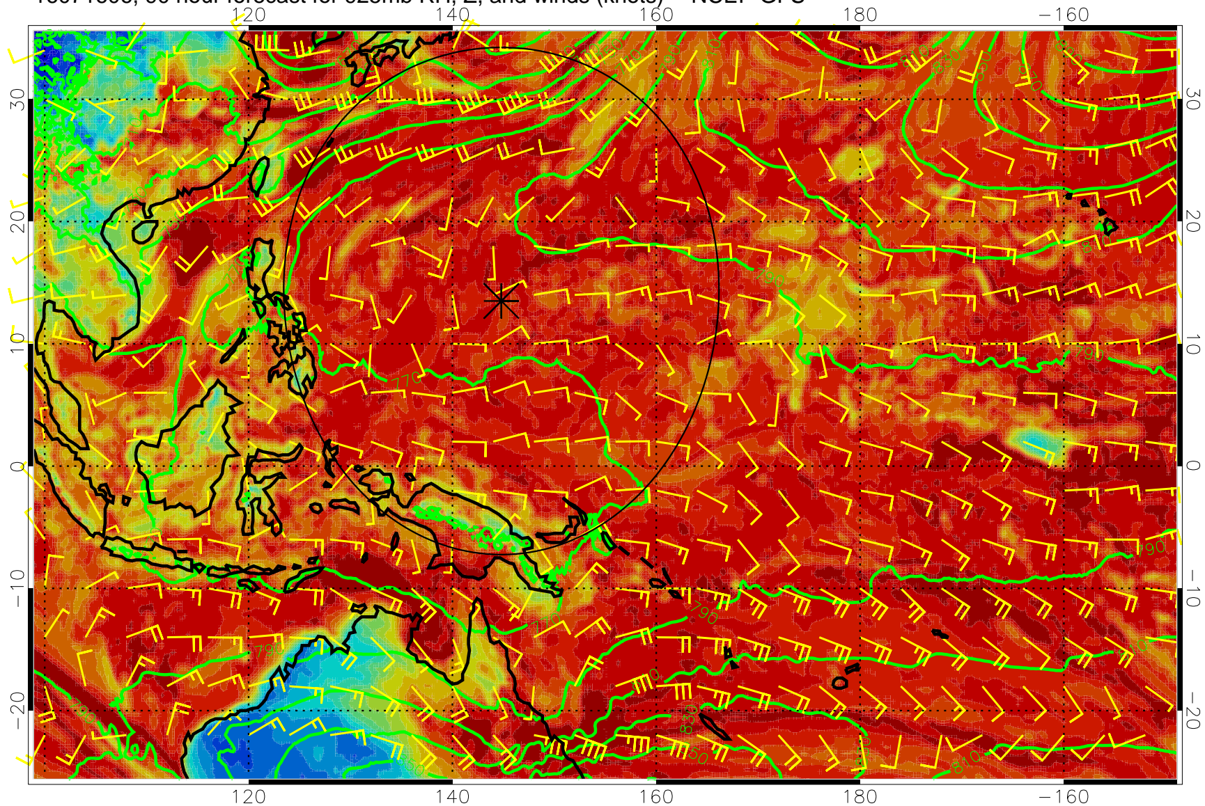
16071606, 90 hour forecast for 925mb RH, Z, and winds (knots) -- NCEP GFS
