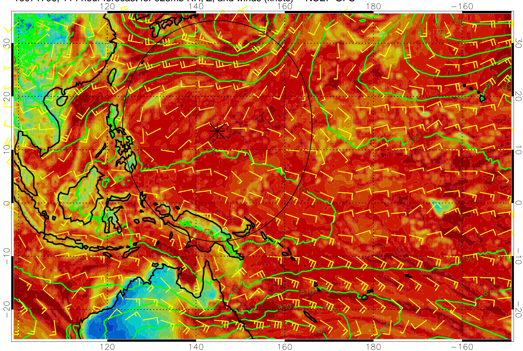
16071706, 114 hour forecast for 925mb RH, Z, and winds (knots) -- NCEP GFS
