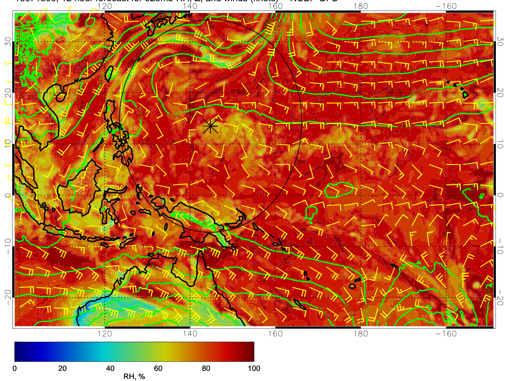
16071300, 12 hour forecast for 925mb RH, Z, and winds (knots) -- NCEP GFS
