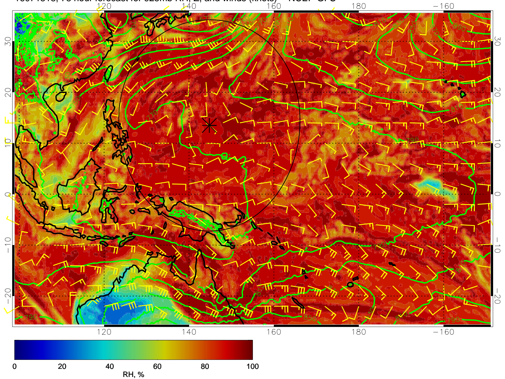
16071518, 78 hour forecast for 925mb RH, Z, and winds (knots) -- NCEP GFS
