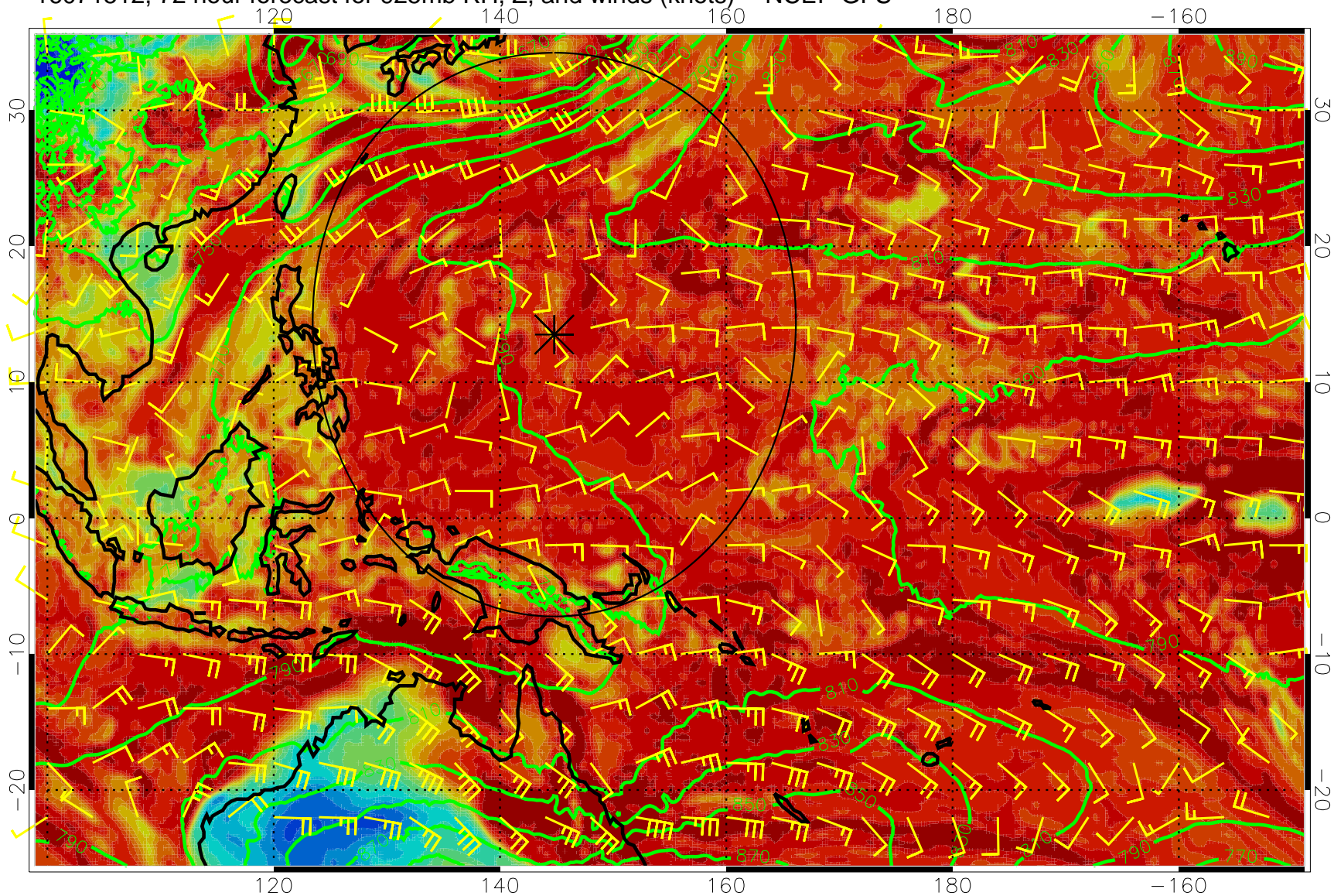
16071512, 72 hour forecast for 925mb RH, Z, and winds (knots) -- NCEP GFS
