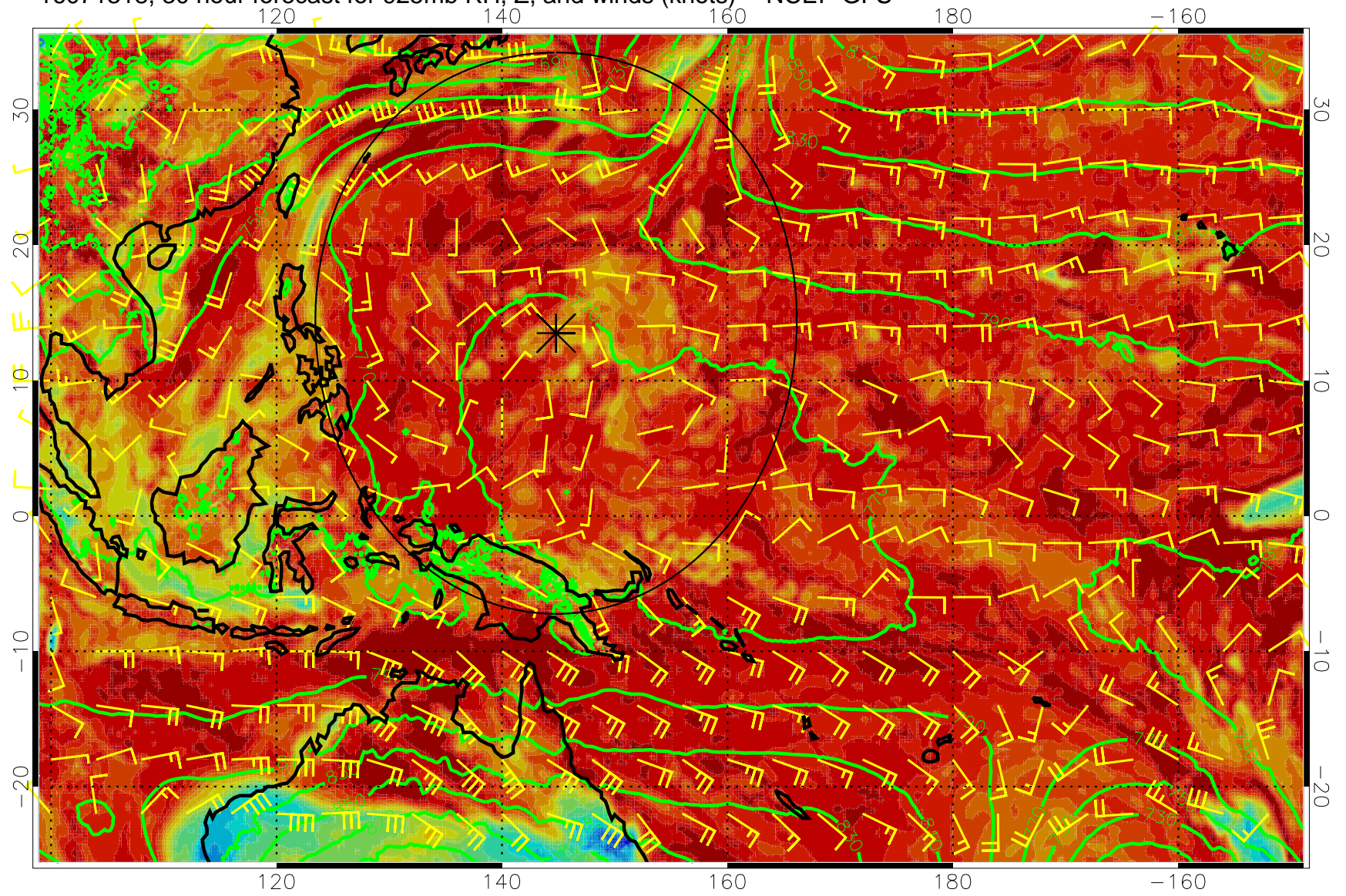
16071318, 30 hour forecast for 925mb RH, Z, and winds (knots) -- NCEP GFS
