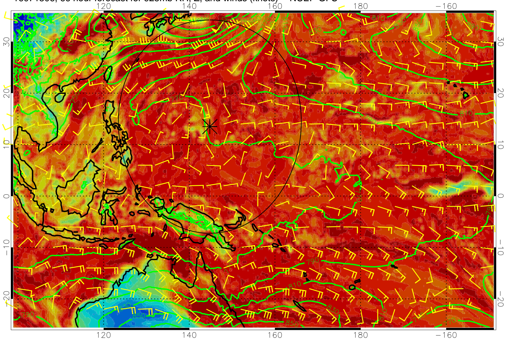
16071506, 66 hour forecast for 925mb RH, Z, and winds (knots) -- NCEP GFS
