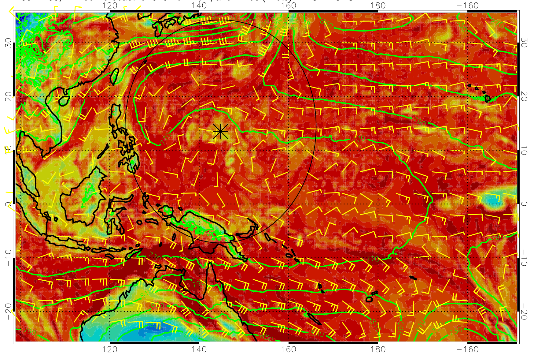
16071406, 42 hour forecast for 925mb RH, Z, and winds (knots) -- NCEP GFS
