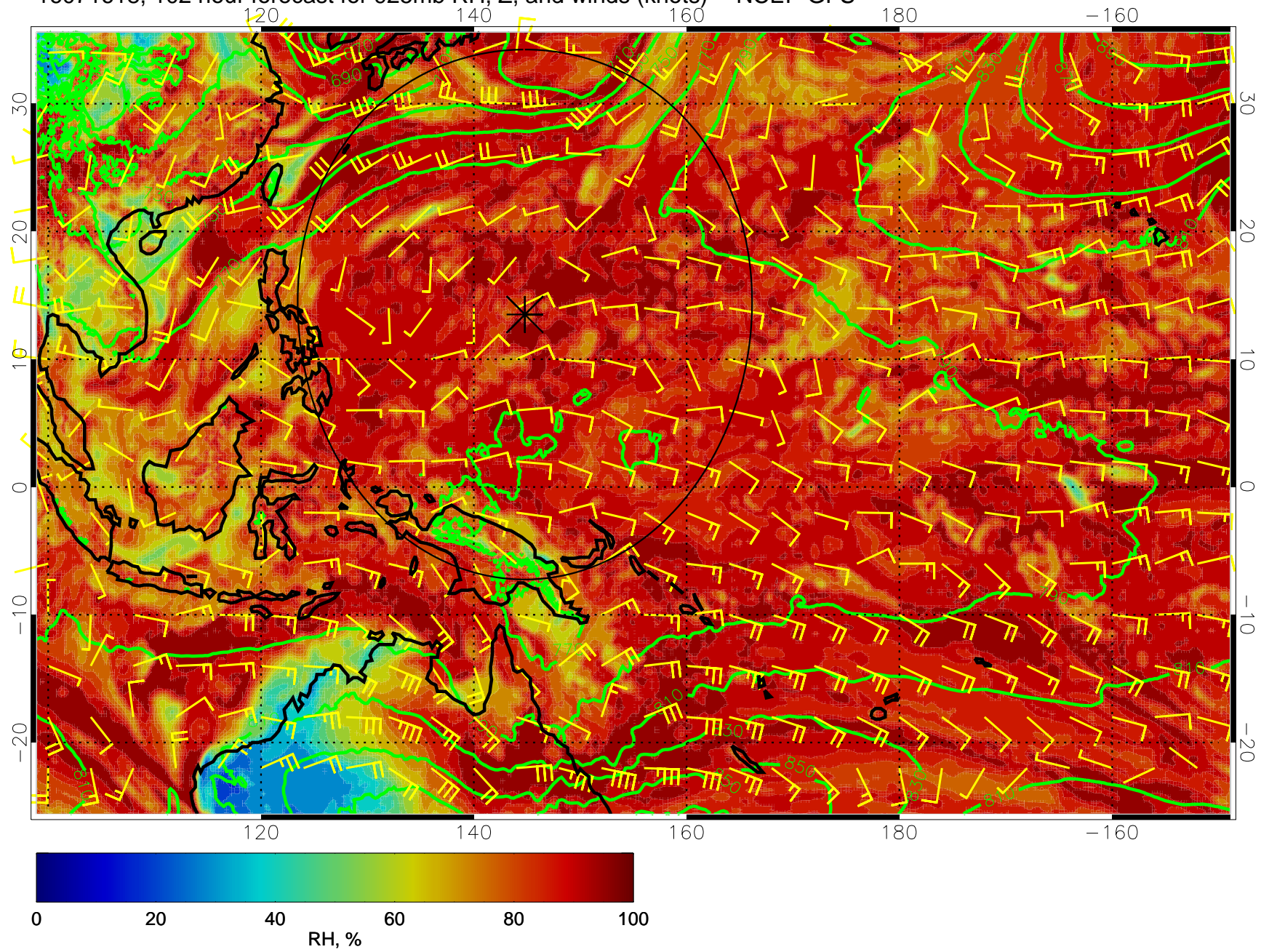
16071618, 102 hour forecast for 925mb RH, Z, and winds (knots) -- NCEP GFS
