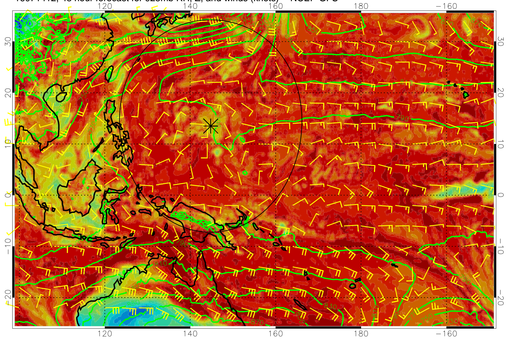
16071412, 48 hour forecast for 925mb RH, Z, and winds (knots) -- NCEP GFS
