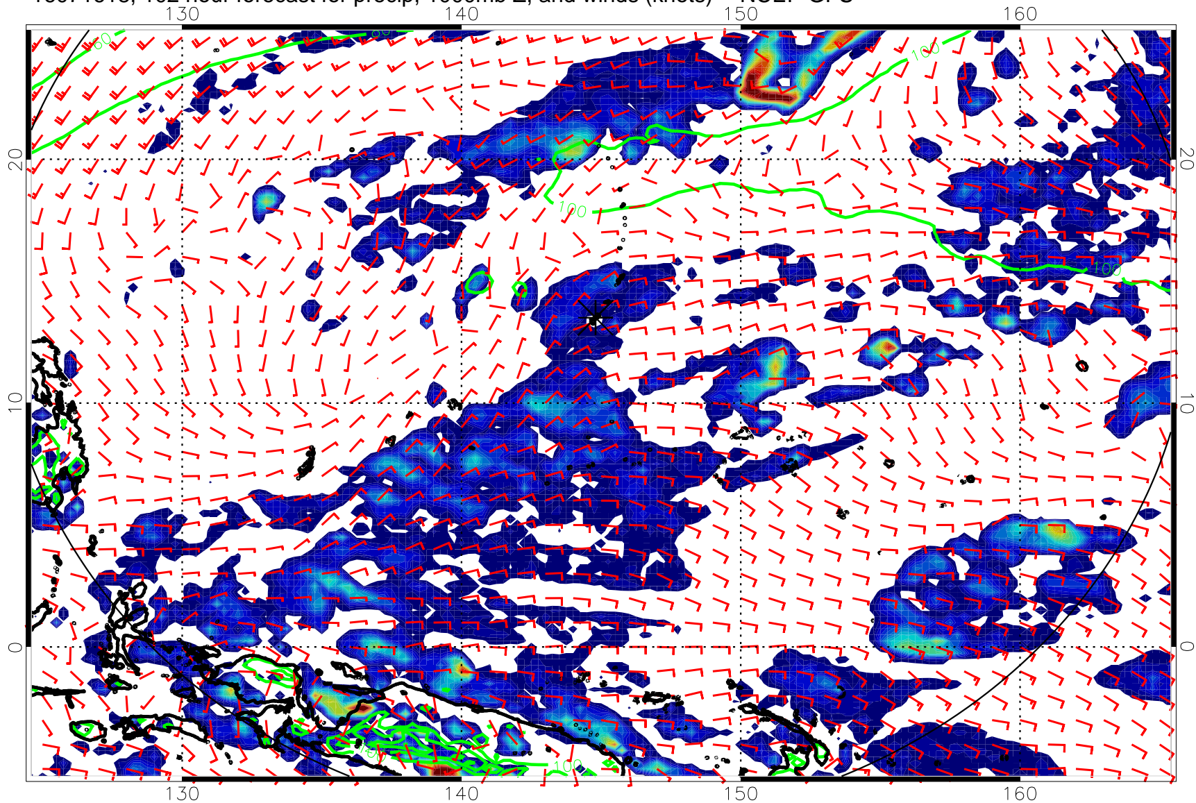
16071618, 102 hour forecast for precip, 1000mb Z, and winds (knots) -- NCEP GFS
