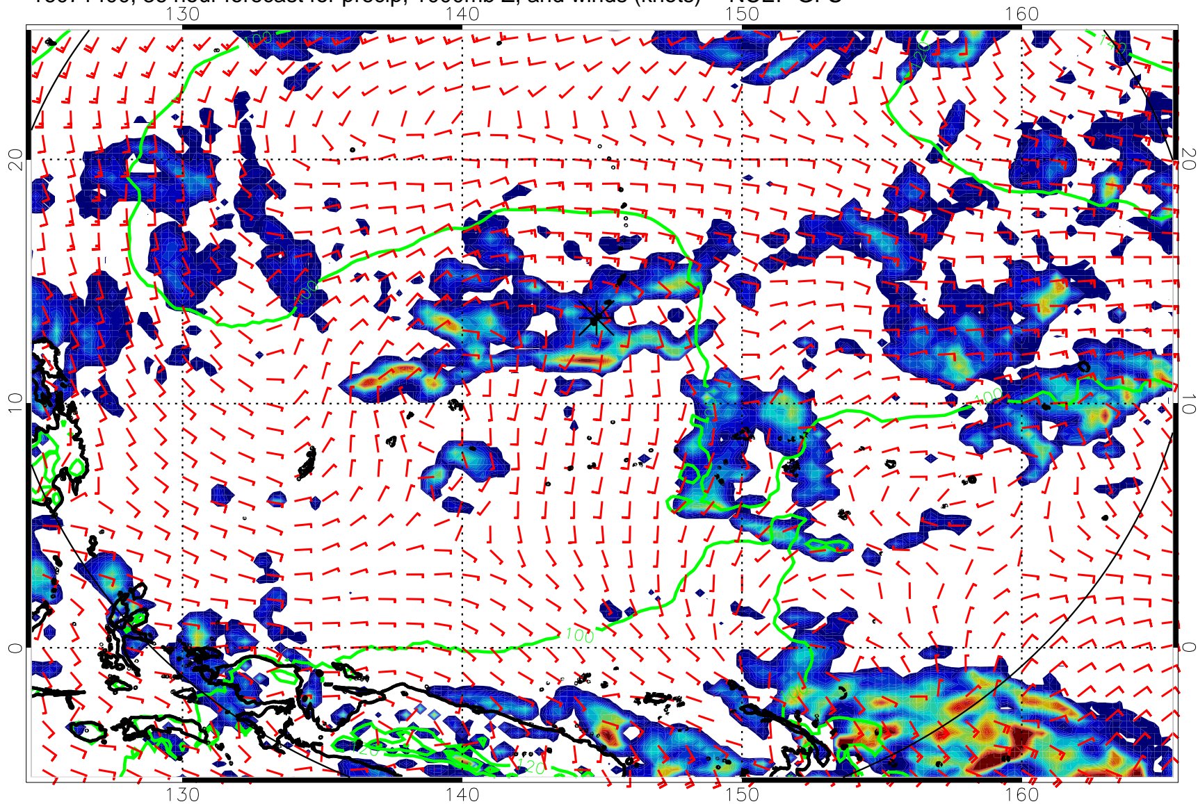
16071400, 36 hour forecast for precip, 1000mb Z, and winds (knots) -- NCEP GFS
