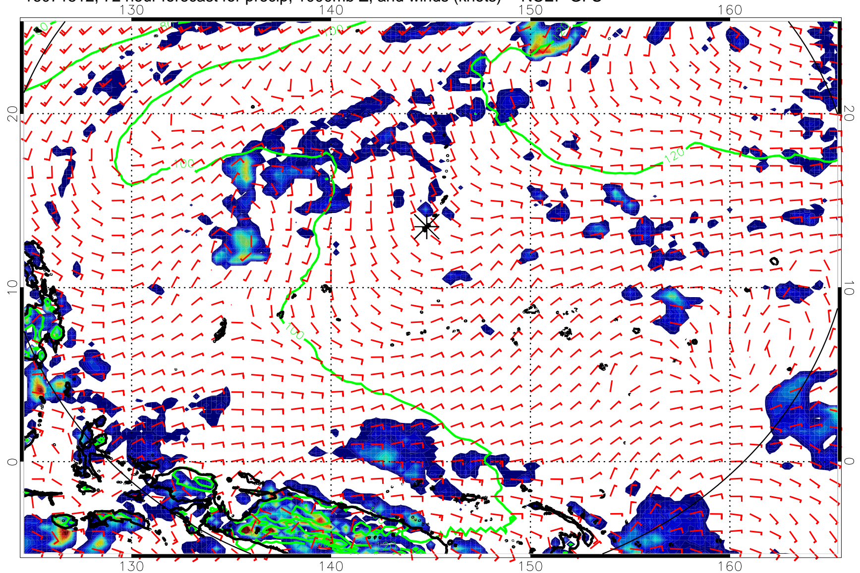
16071512, 72 hour forecast for precip, 1000mb Z, and winds (knots) -- NCEP GFS
