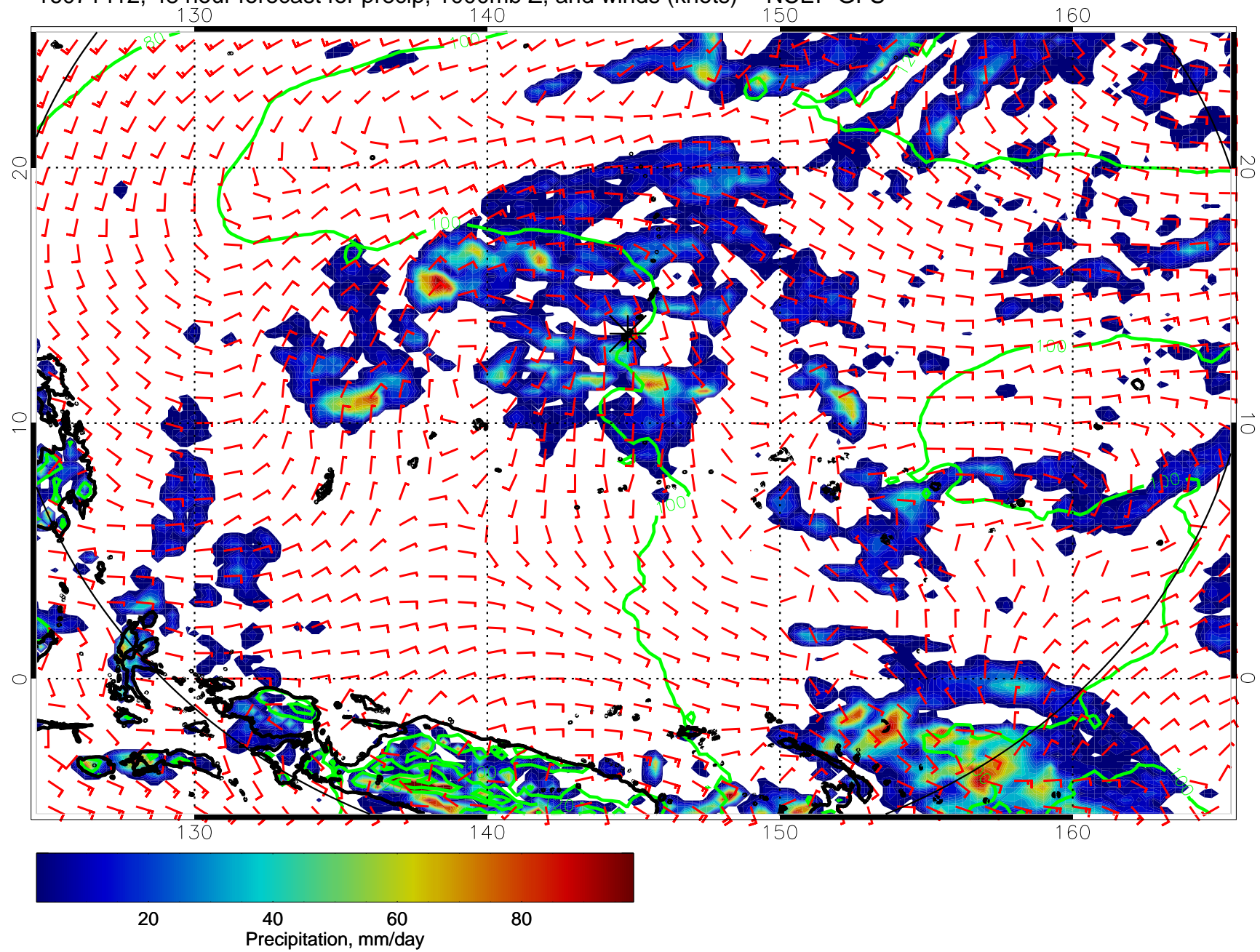
16071412, 48 hour forecast for precip, 1000mb Z, and winds (knots) -- NCEP GFS
