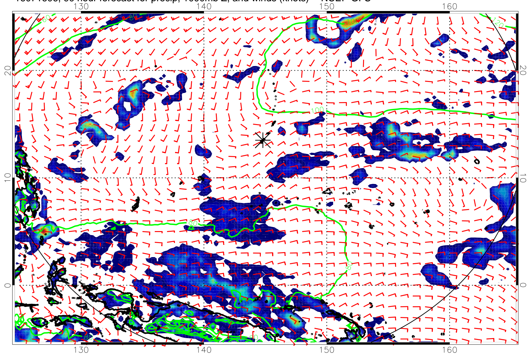
16071606, 90 hour forecast for precip, 1000mb Z, and winds (knots) -- NCEP GFS
