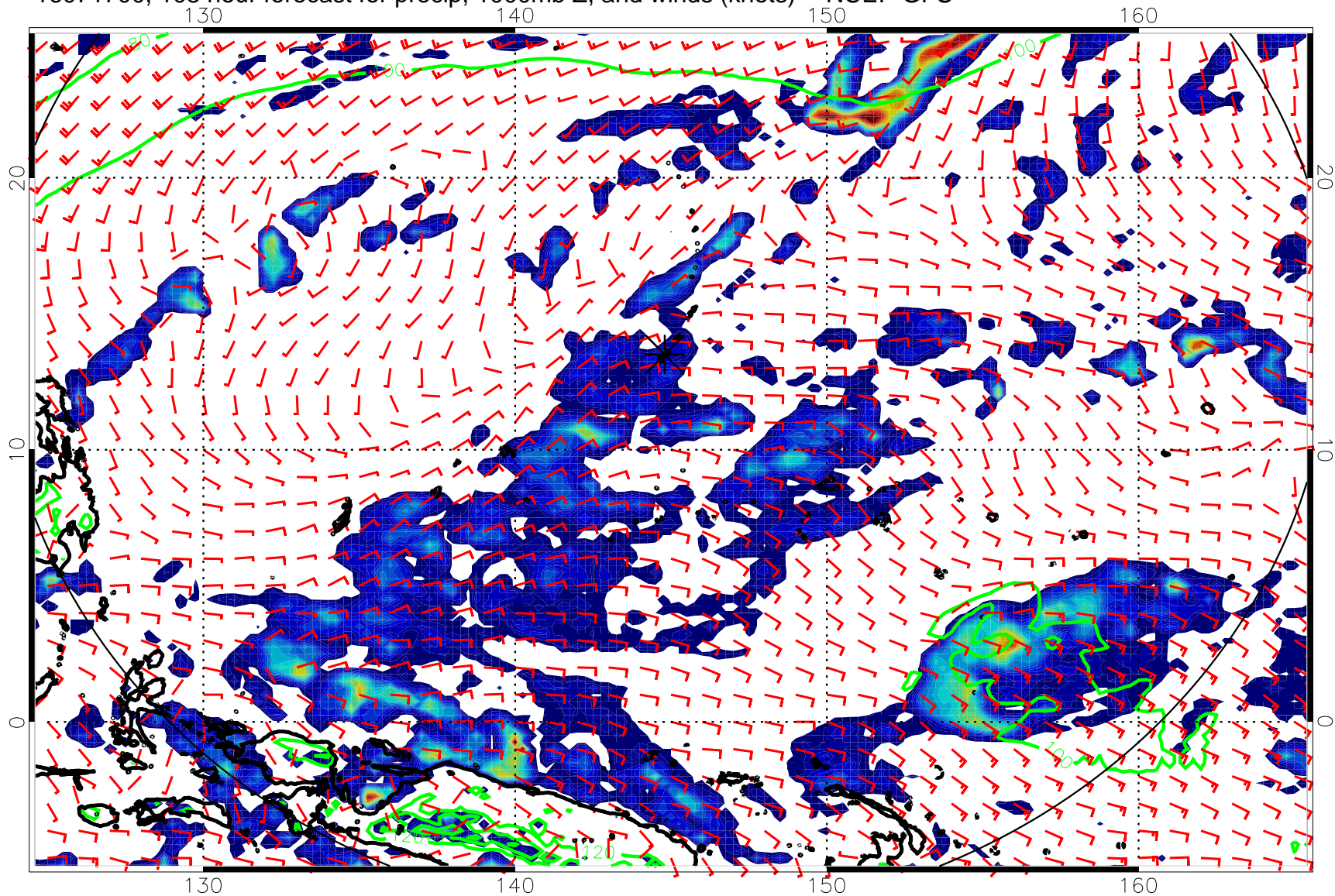
16071700, 108 hour forecast for precip, 1000mb Z, and winds (knots) -- NCEP GFS
