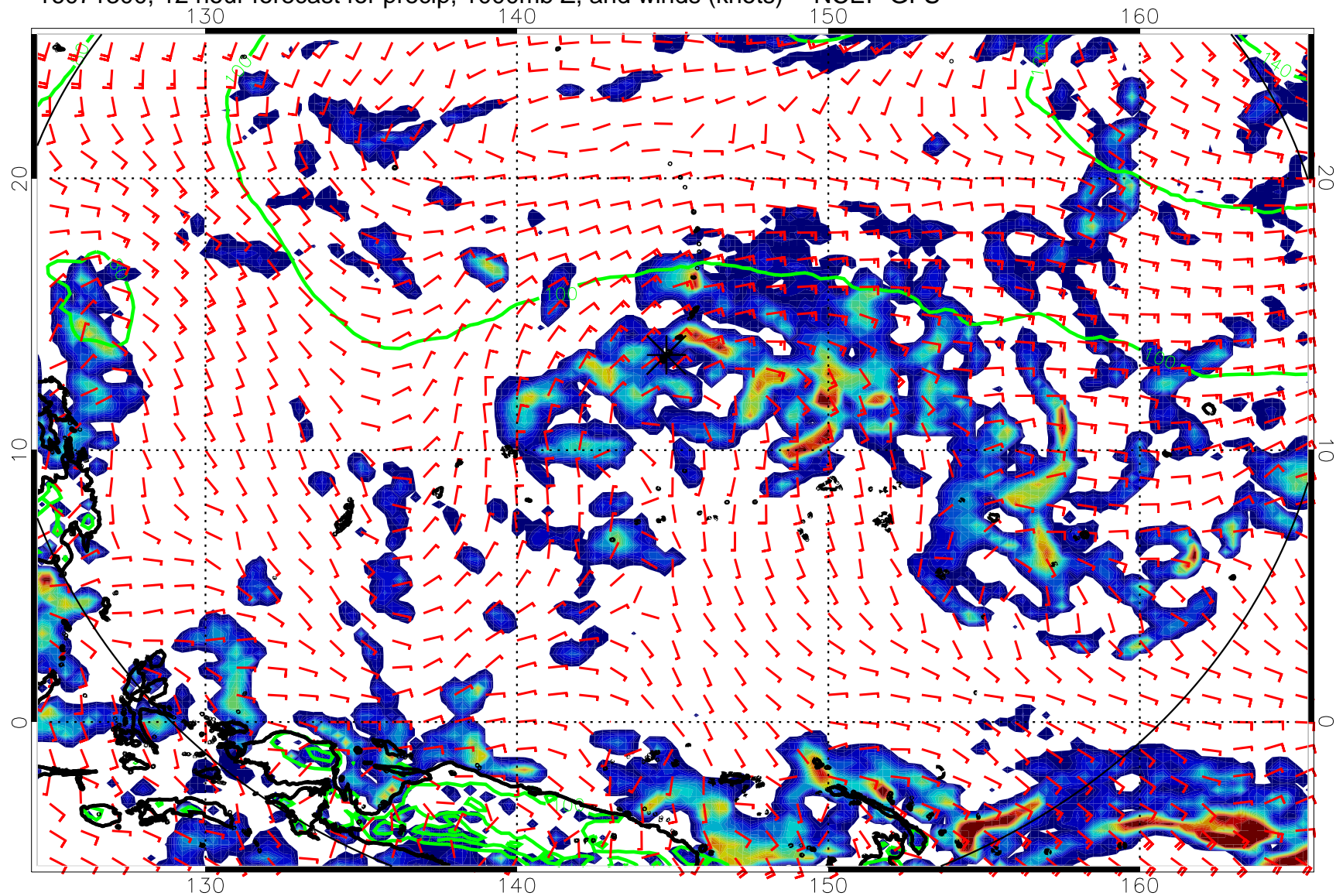
16071300, 12 hour forecast for precip, 1000mb Z, and winds (knots) -- NCEP GFS
