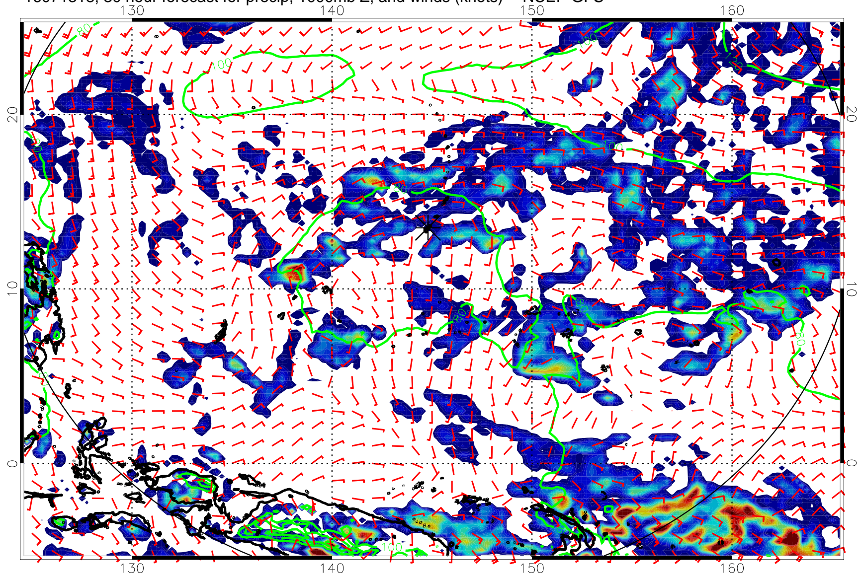
16071318, 30 hour forecast for precip, 1000mb Z, and winds (knots) -- NCEP GFS
