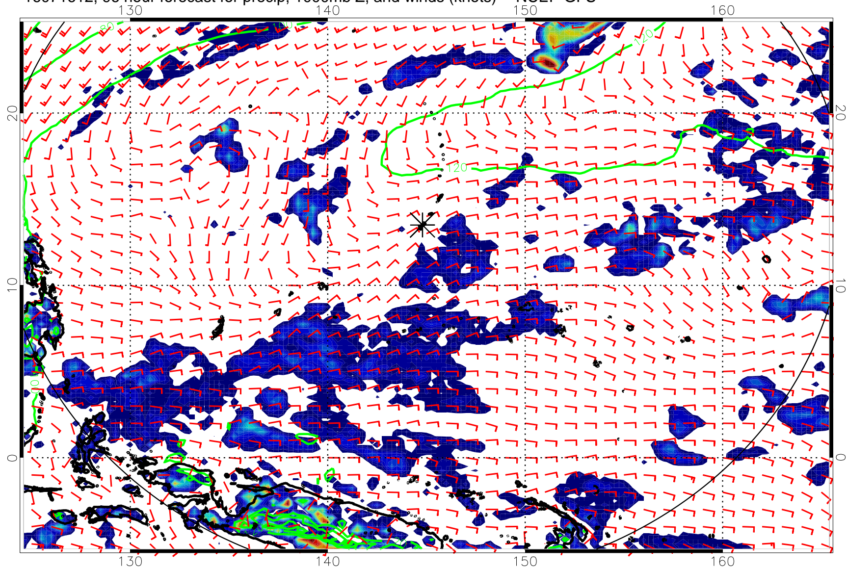
16071612, 96 hour forecast for precip, 1000mb Z, and winds (knots) -- NCEP GFS
