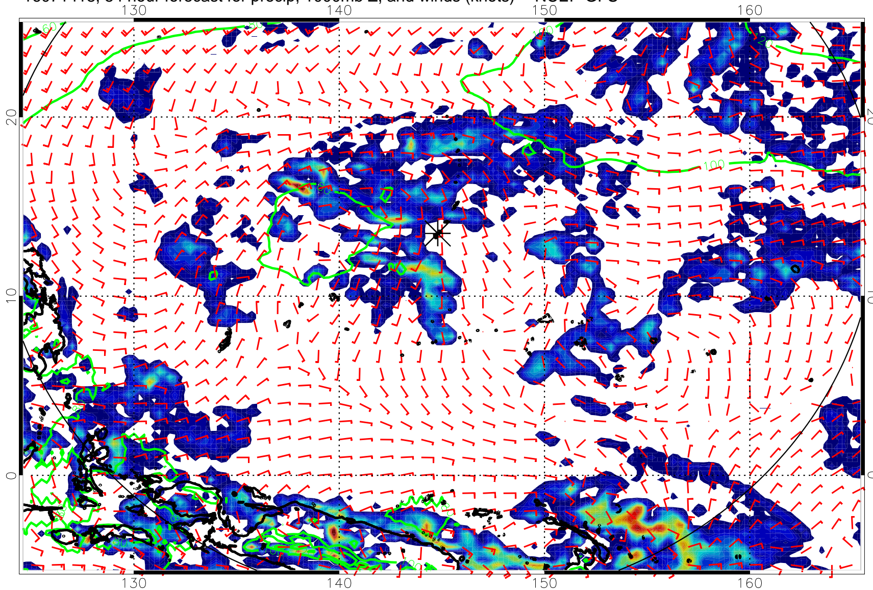
16071418, 54 hour forecast for precip, 1000mb Z, and winds (knots) -- NCEP GFS
