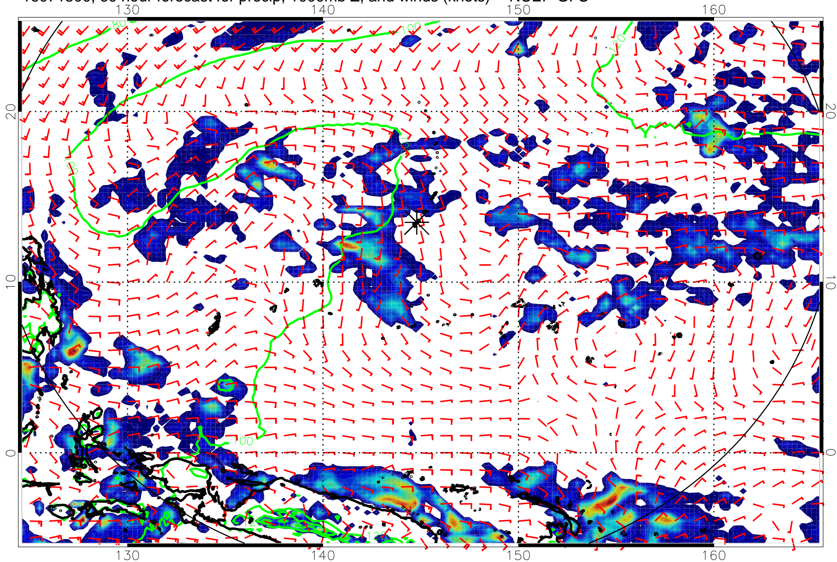
16071500, 60 hour forecast for precip, 1000mb Z, and winds (knots) -- NCEP GFS
