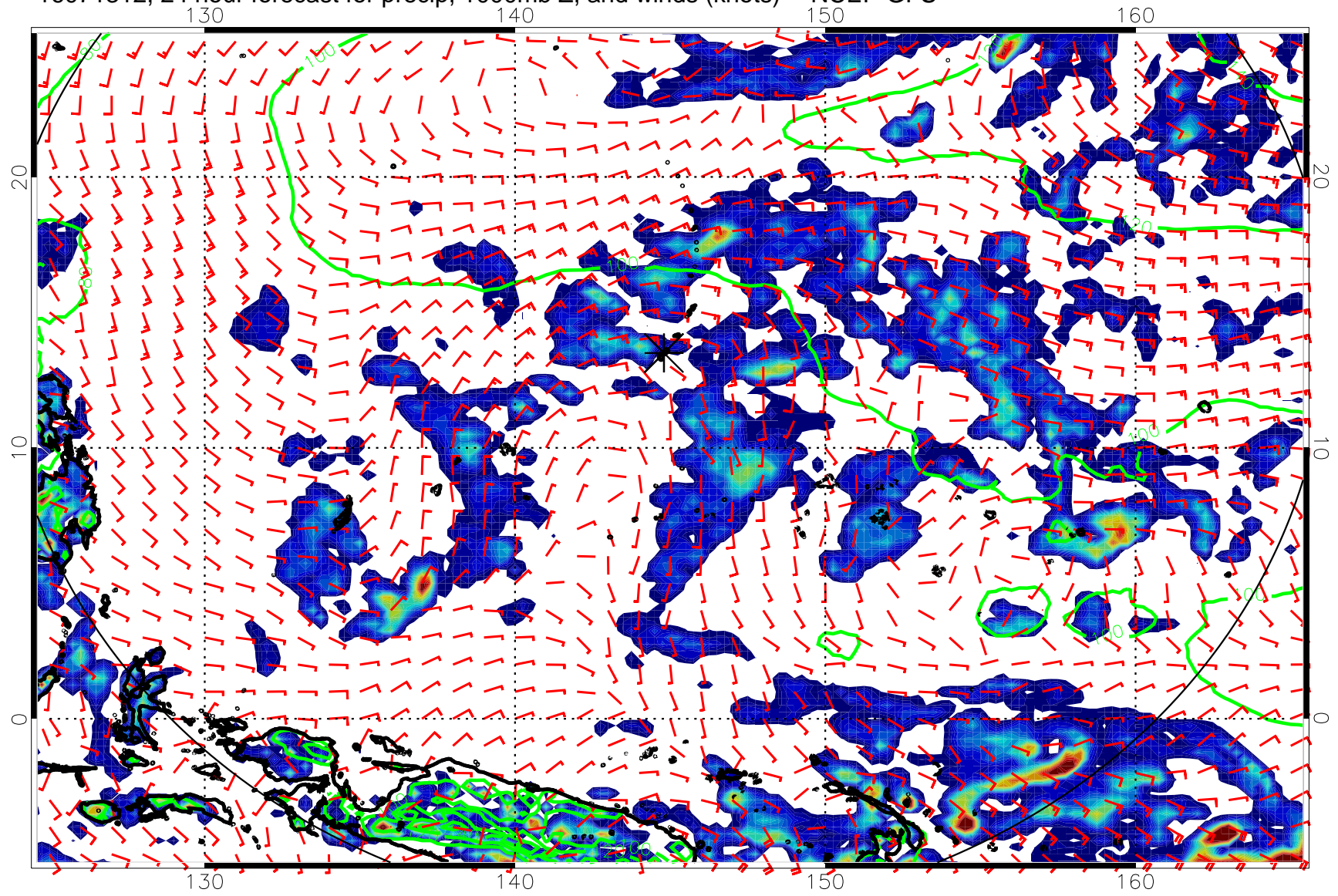
16071312, 24 hour forecast for precip, 1000mb Z, and winds (knots) -- NCEP GFS
