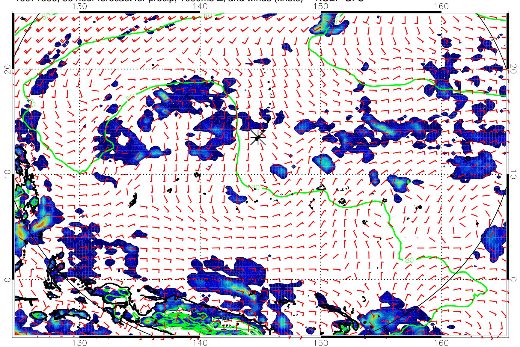
16071506, 66 hour forecast for precip, 1000mb Z, and winds (knots) -- NCEP GFS
