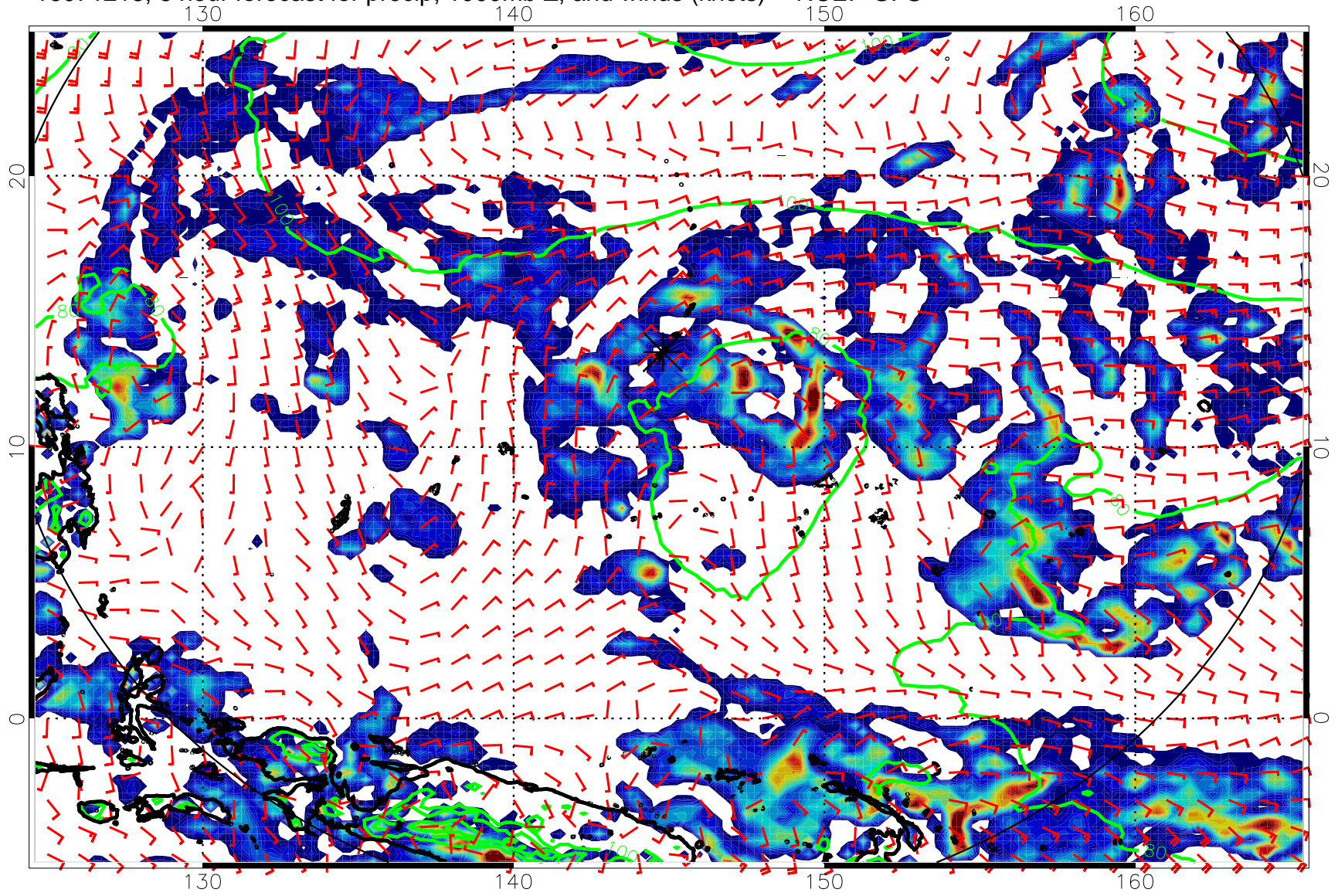
16071218, 6 hour forecast for precip, 1000mb Z, and winds (knots) -- NCEP GFS
