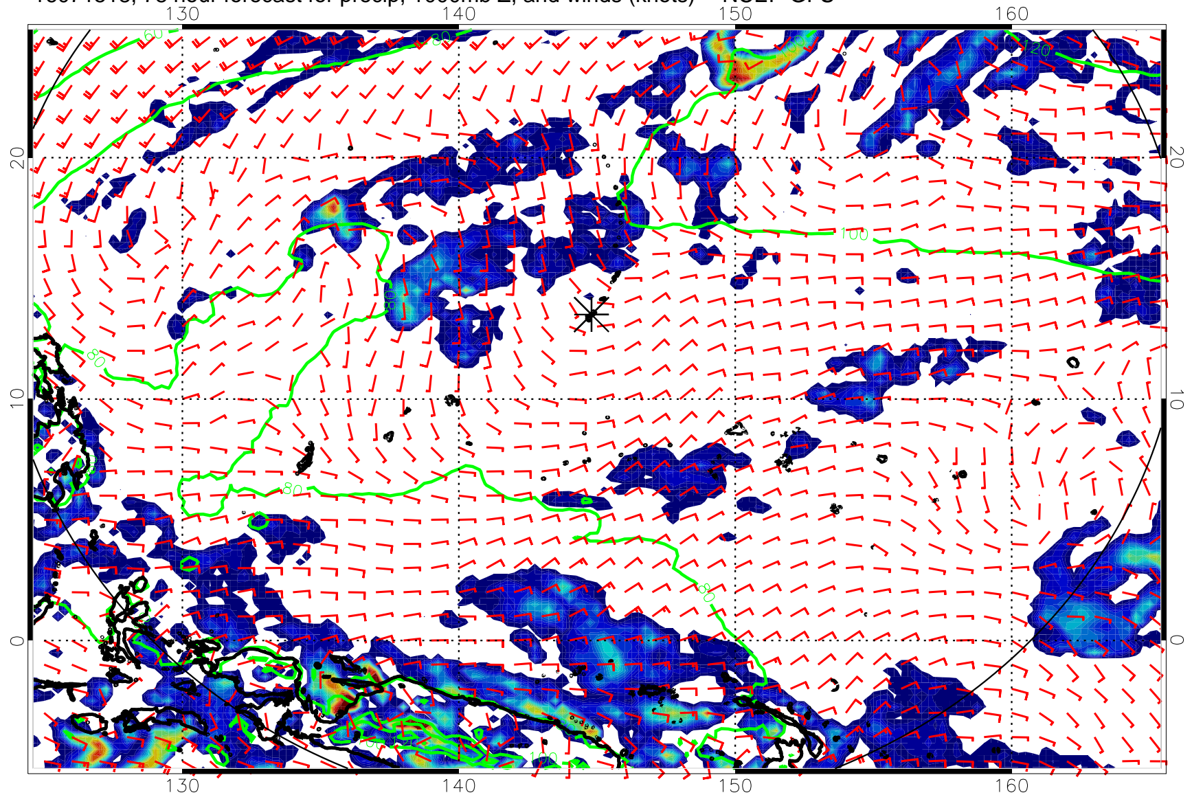
16071518, 78 hour forecast for precip, 1000mb Z, and winds (knots) -- NCEP GFS
