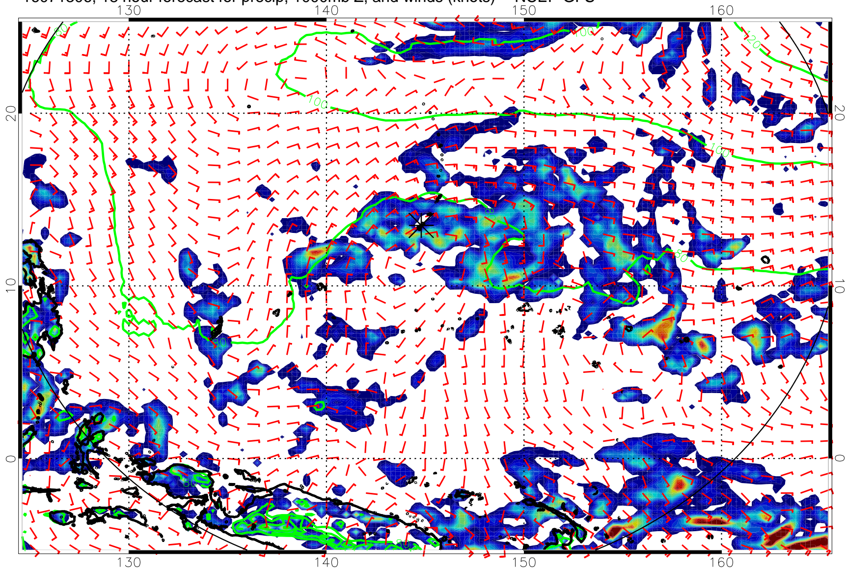
16071306, 18 hour forecast for precip, 1000mb Z, and winds (knots) -- NCEP GFS
