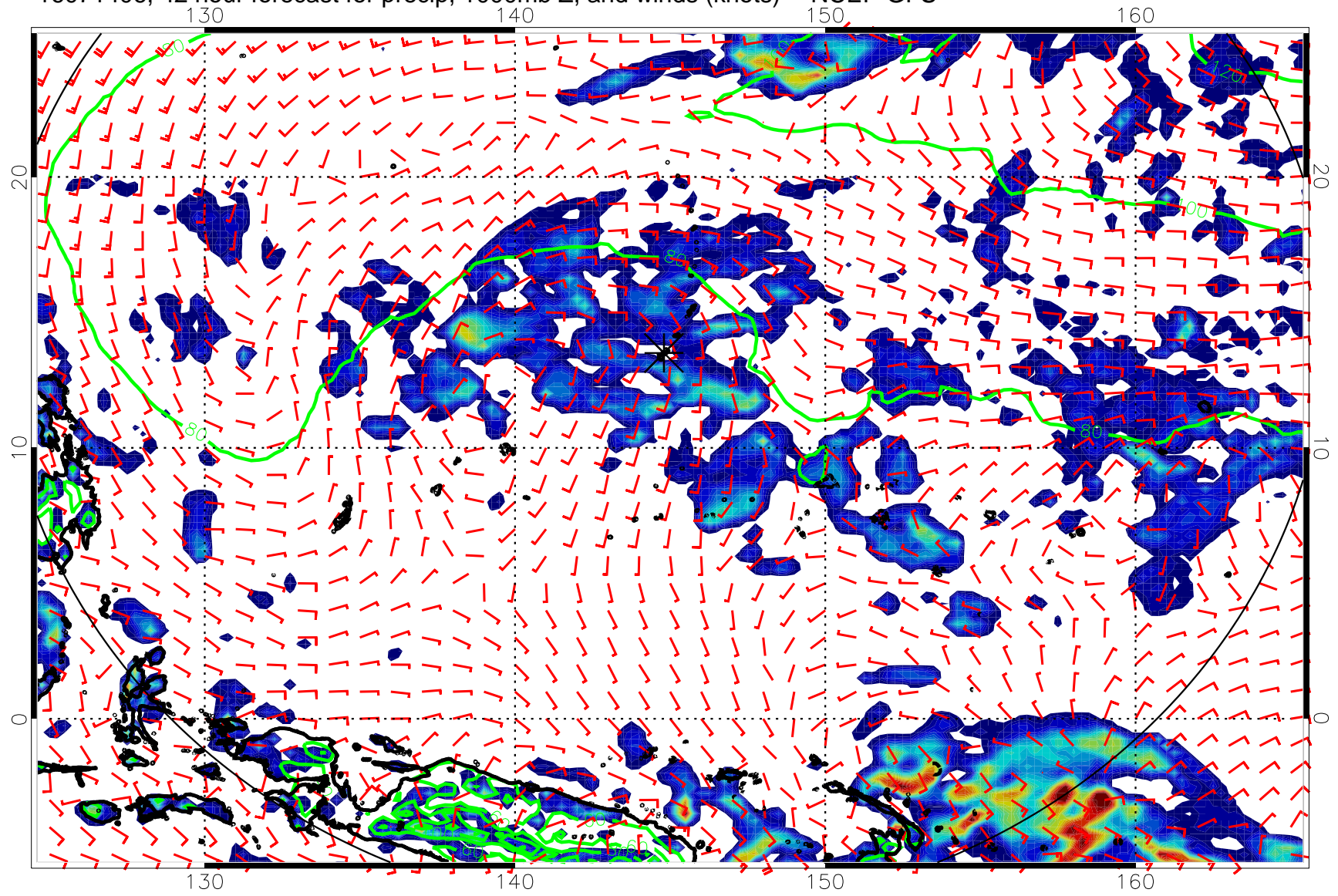
16071406, 42 hour forecast for precip, 1000mb Z, and winds (knots) -- NCEP GFS
