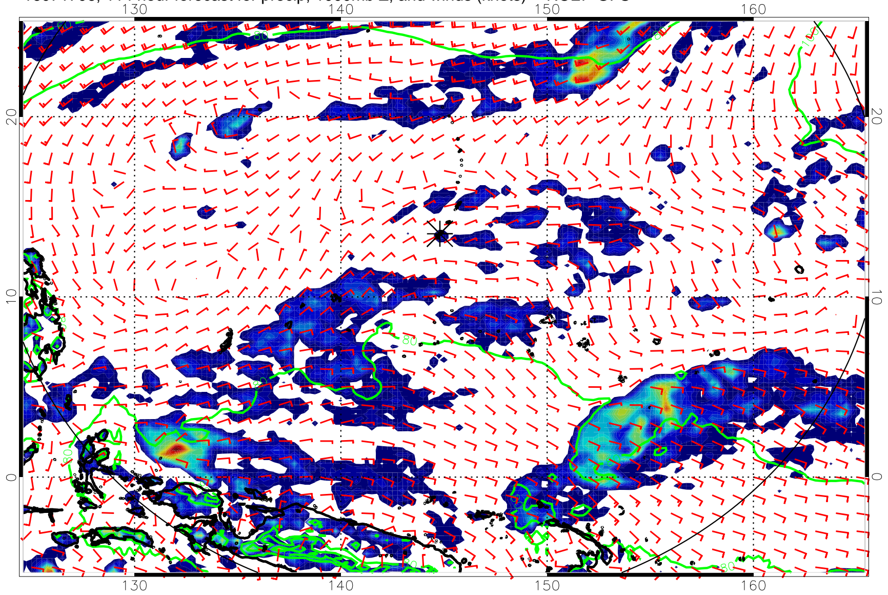
16071706, 114 hour forecast for precip, 1000mb Z, and winds (knots) -- NCEP GFS
