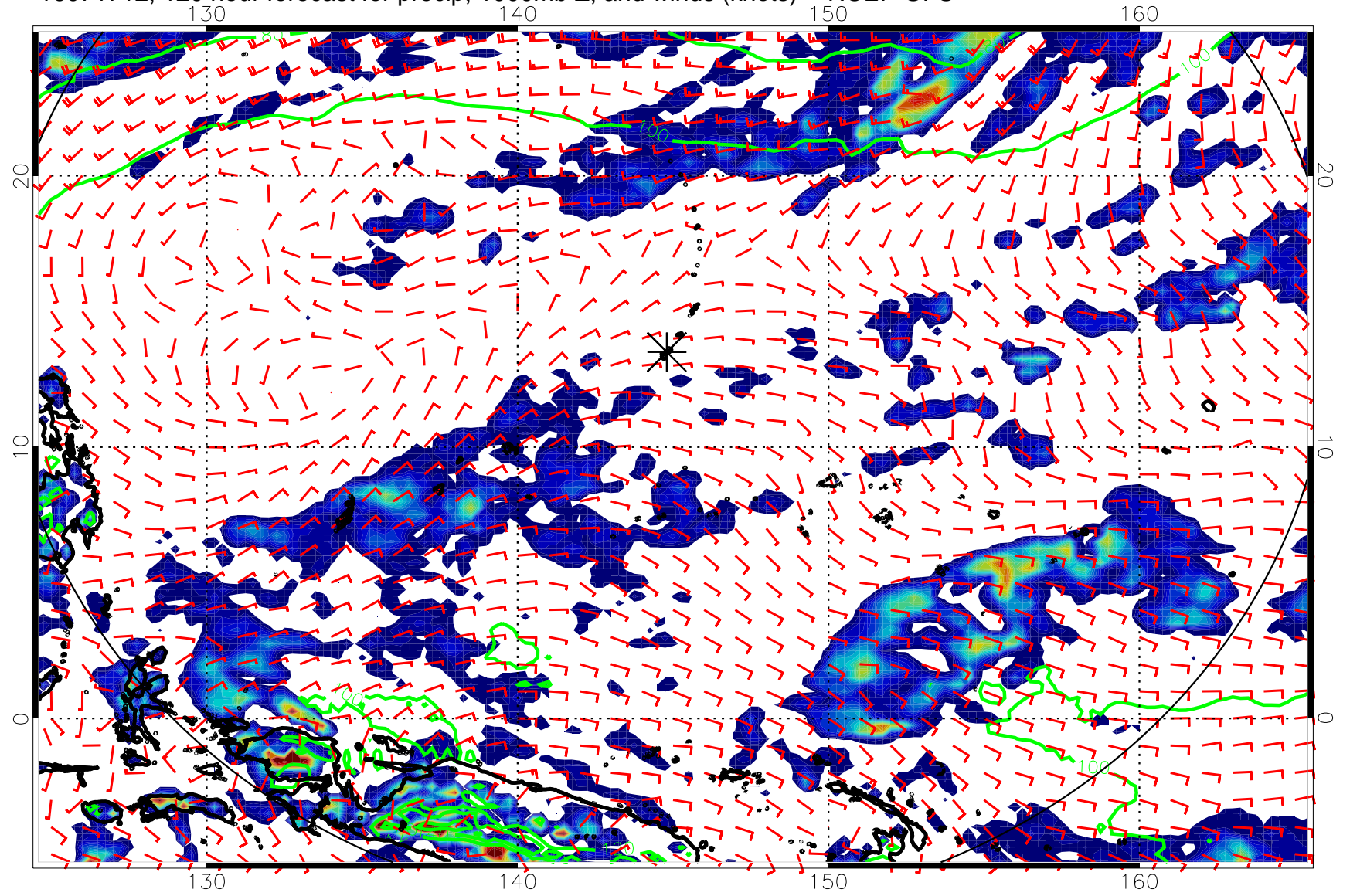
16071712, 120 hour forecast for precip, 1000mb Z, and winds (knots) -- NCEP GFS
