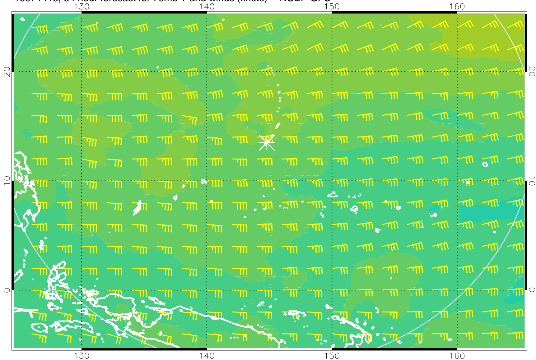
16071418, 54 hour forecast for 70mb T and winds (knots) -- NCEP GFS
