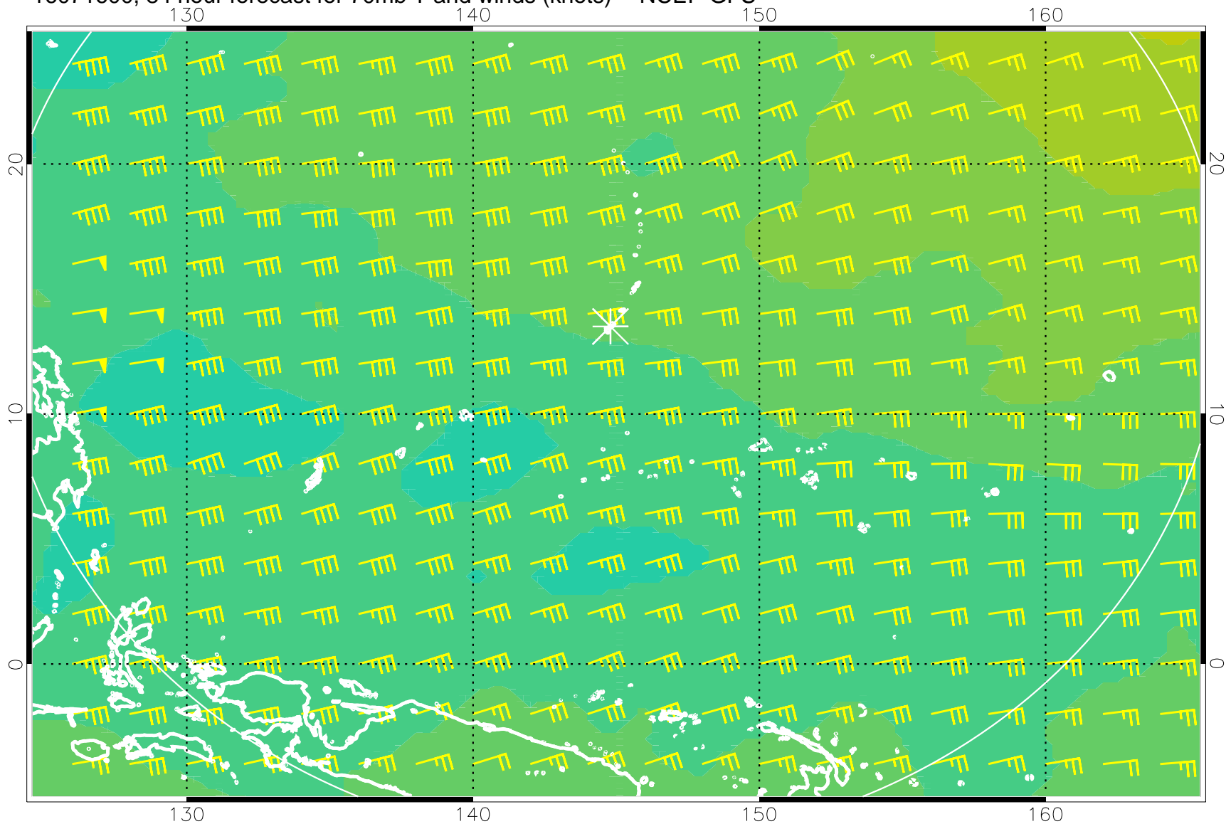
16071600, 84 hour forecast for 70mb T and winds (knots) -- NCEP GFS
