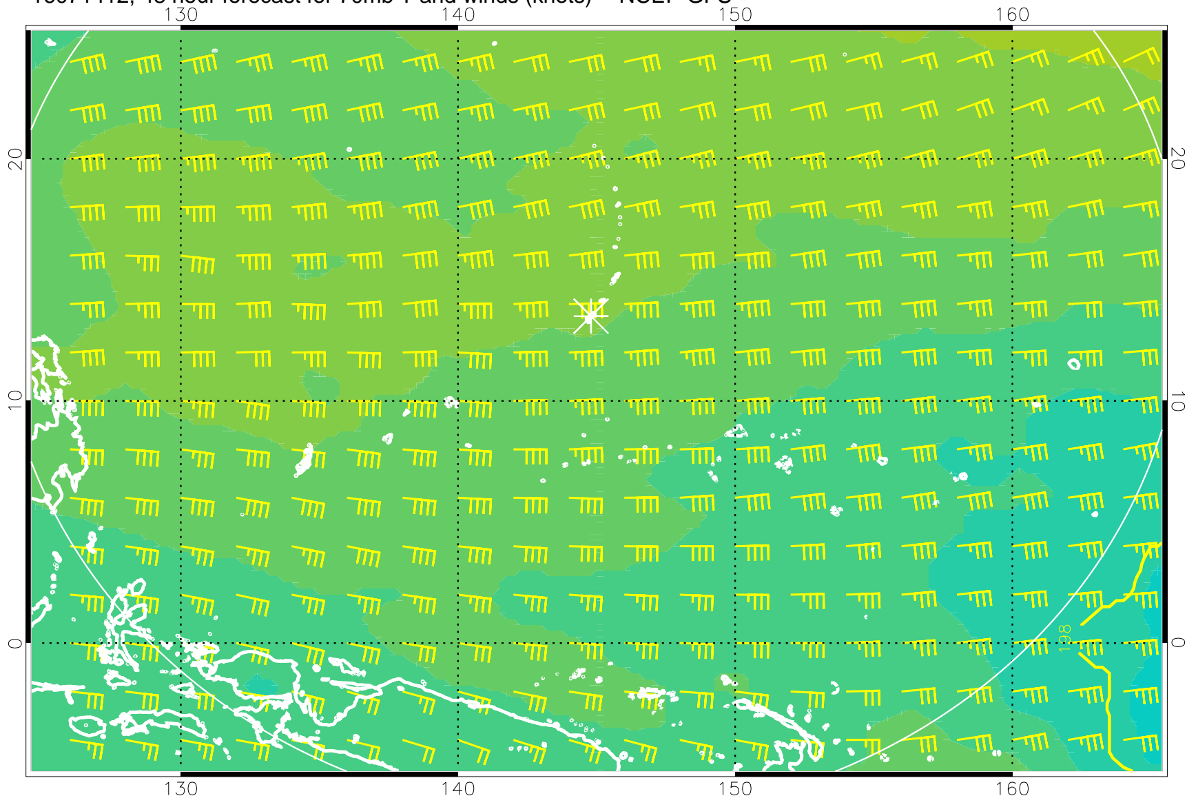
16071412, 48 hour forecast for 70mb T and winds (knots) -- NCEP GFS
