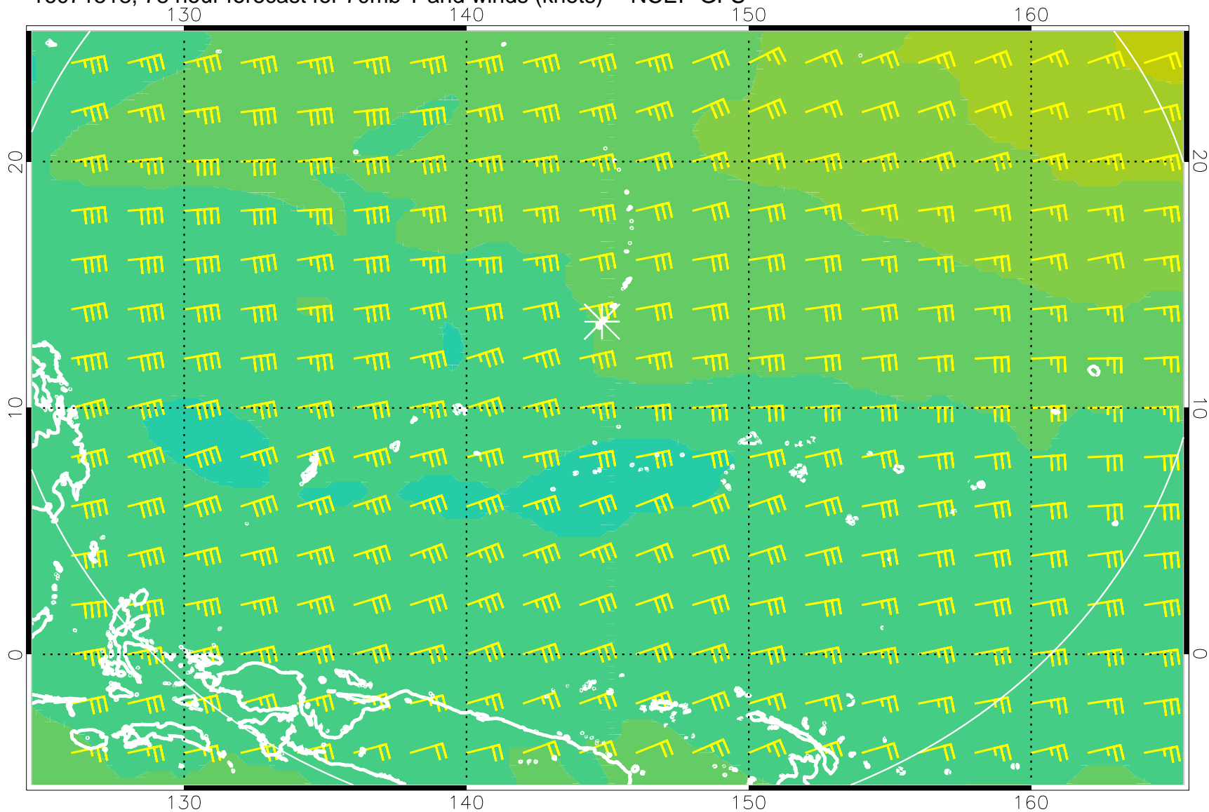
16071518, 78 hour forecast for 70mb T and winds (knots) -- NCEP GFS
