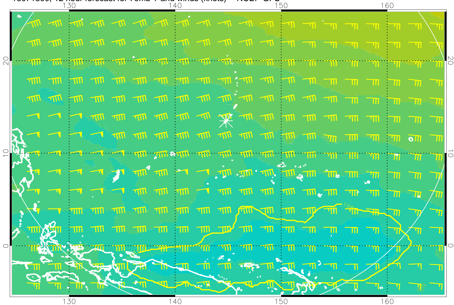
16071300, 12 hour forecast for 70mb T and winds (knots) -- NCEP GFS
