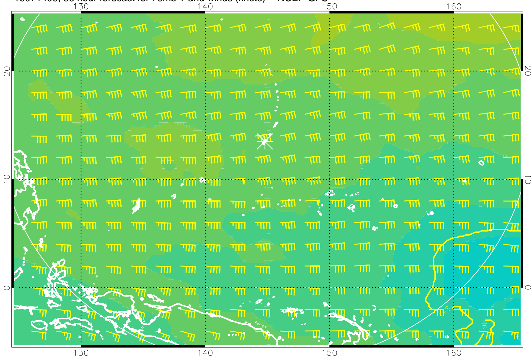
16071400, 36 hour forecast for 70mb T and winds (knots) -- NCEP GFS
