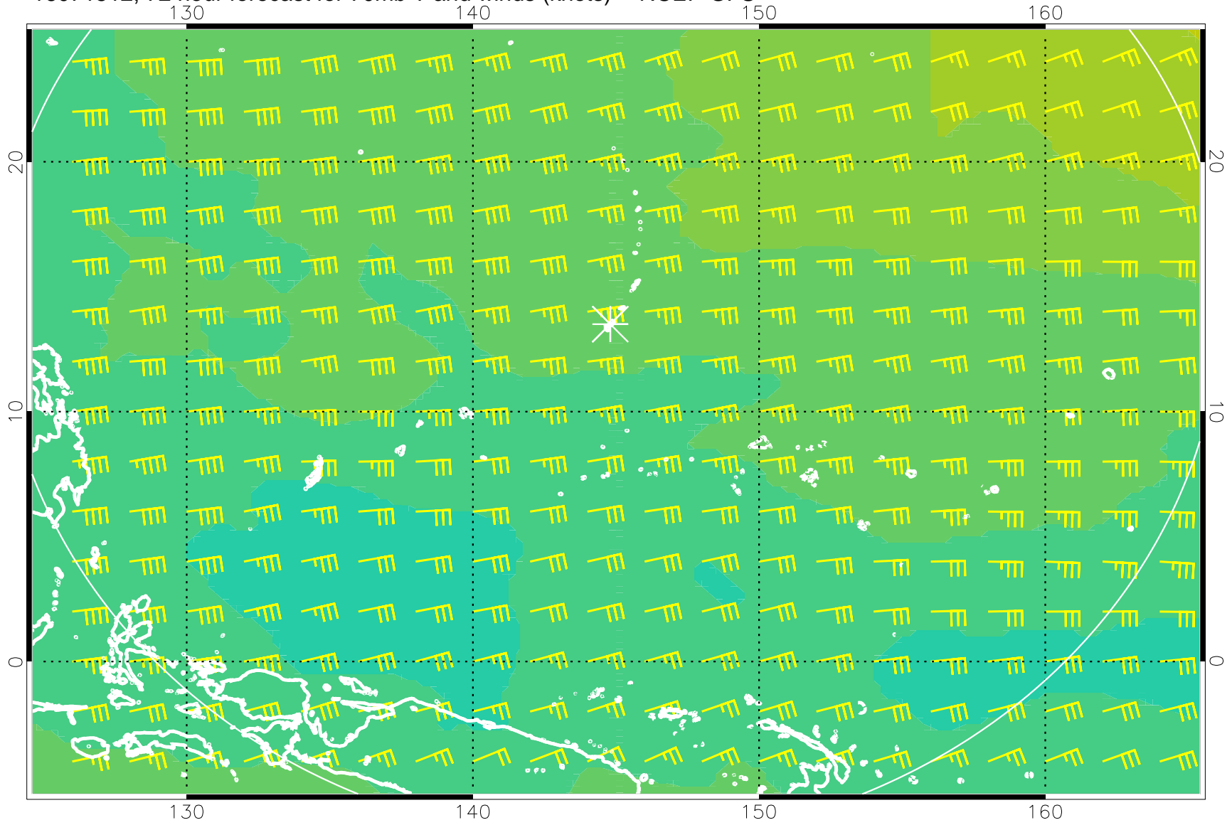
16071512, 72 hour forecast for 70mb T and winds (knots) -- NCEP GFS
