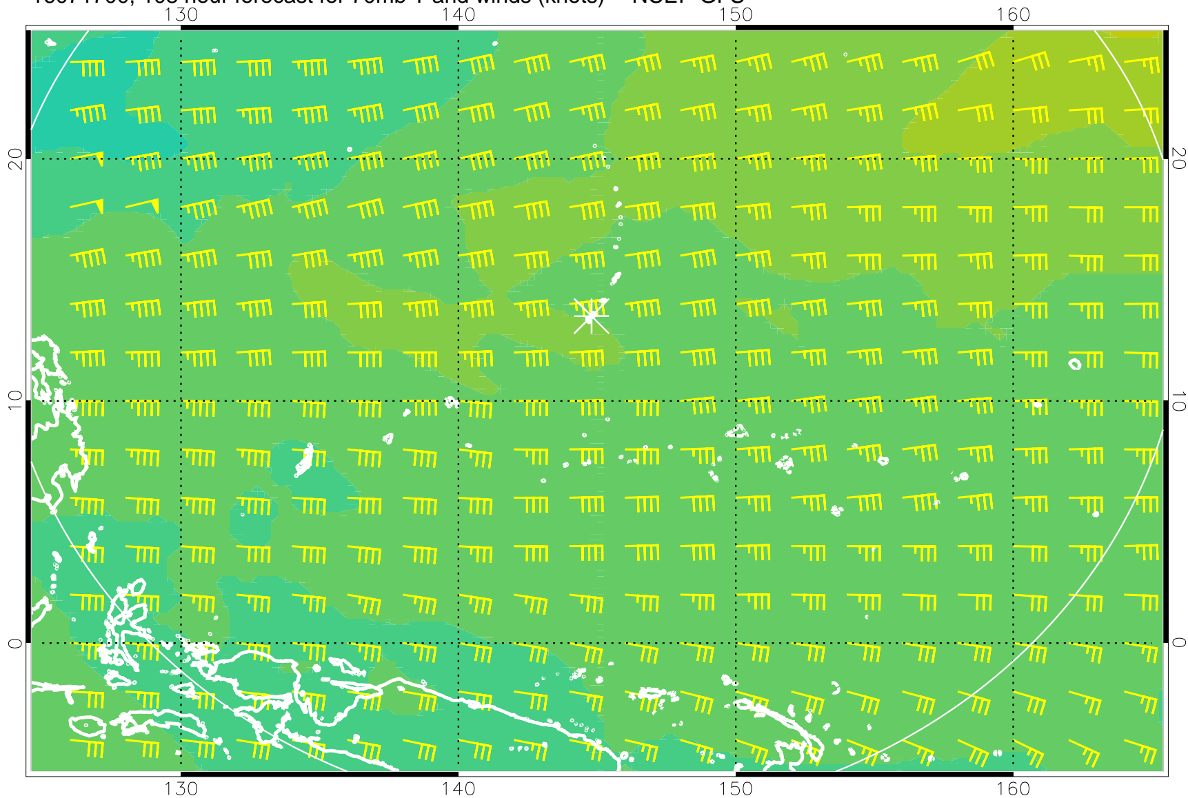
16071700, 108 hour forecast for 70mb T and winds (knots) -- NCEP GFS
