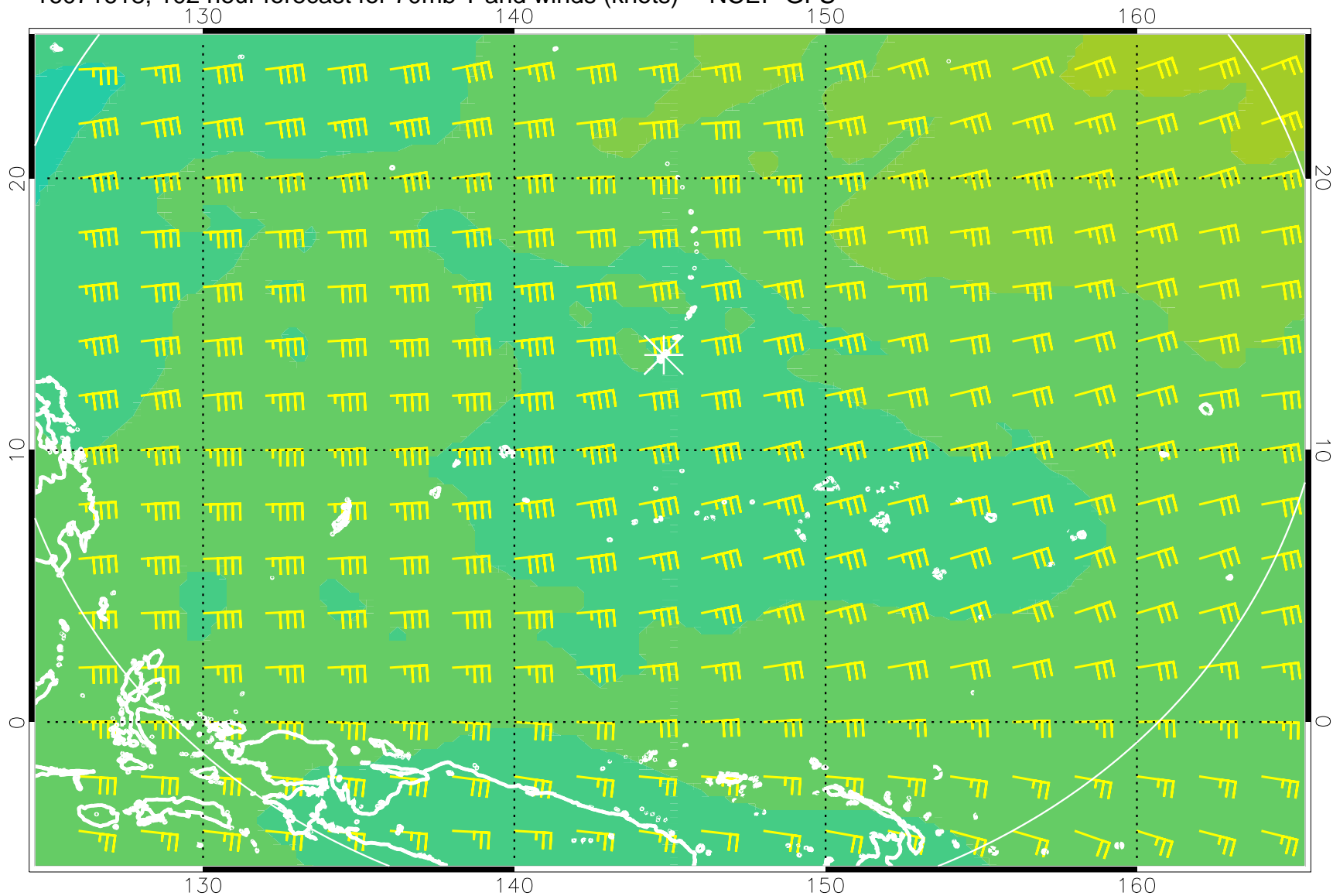
16071618, 102 hour forecast for 70mb T and winds (knots) -- NCEP GFS
