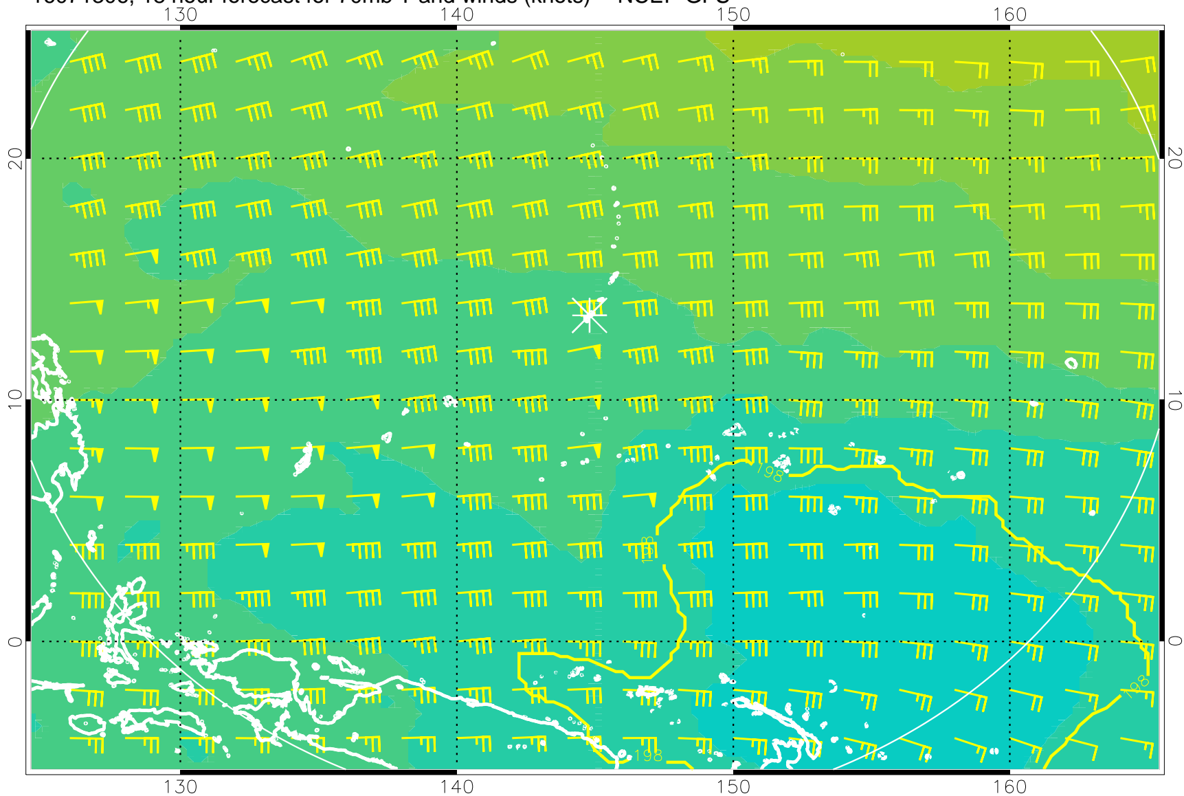
16071306, 18 hour forecast for 70mb T and winds (knots) -- NCEP GFS
