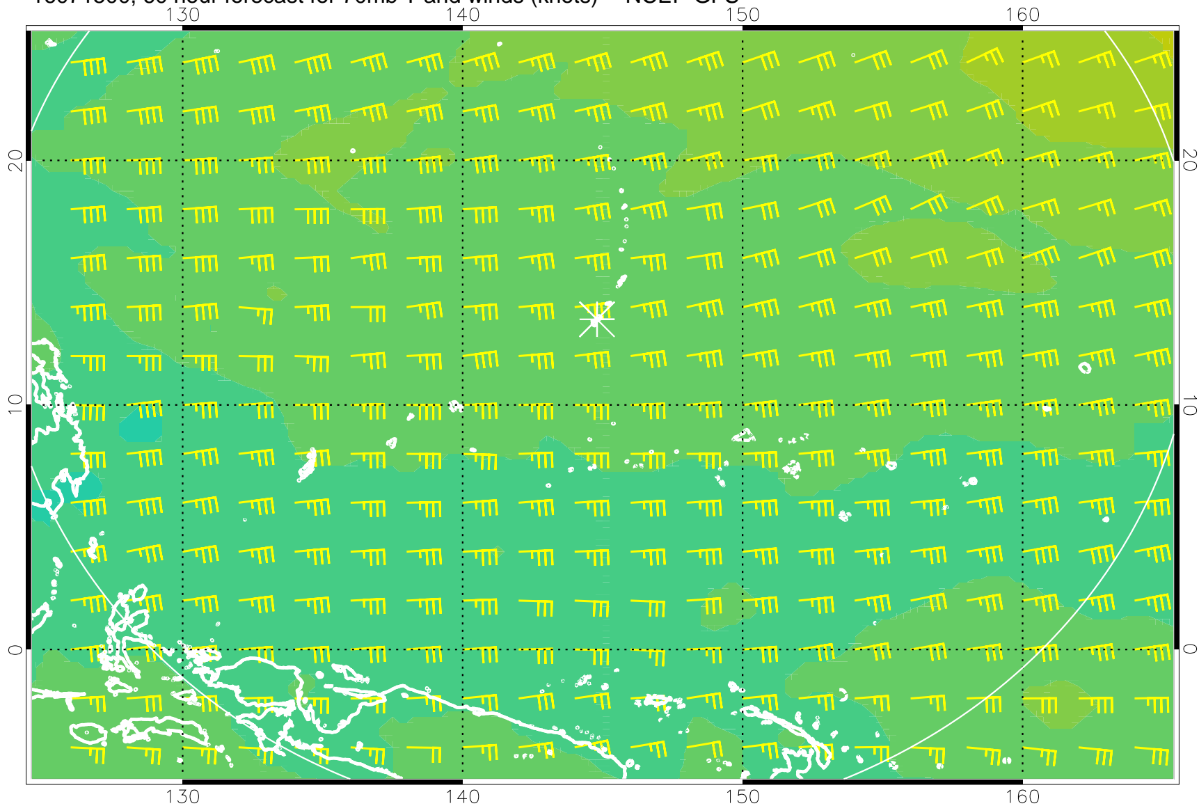
16071500, 60 hour forecast for 70mb T and winds (knots) -- NCEP GFS
