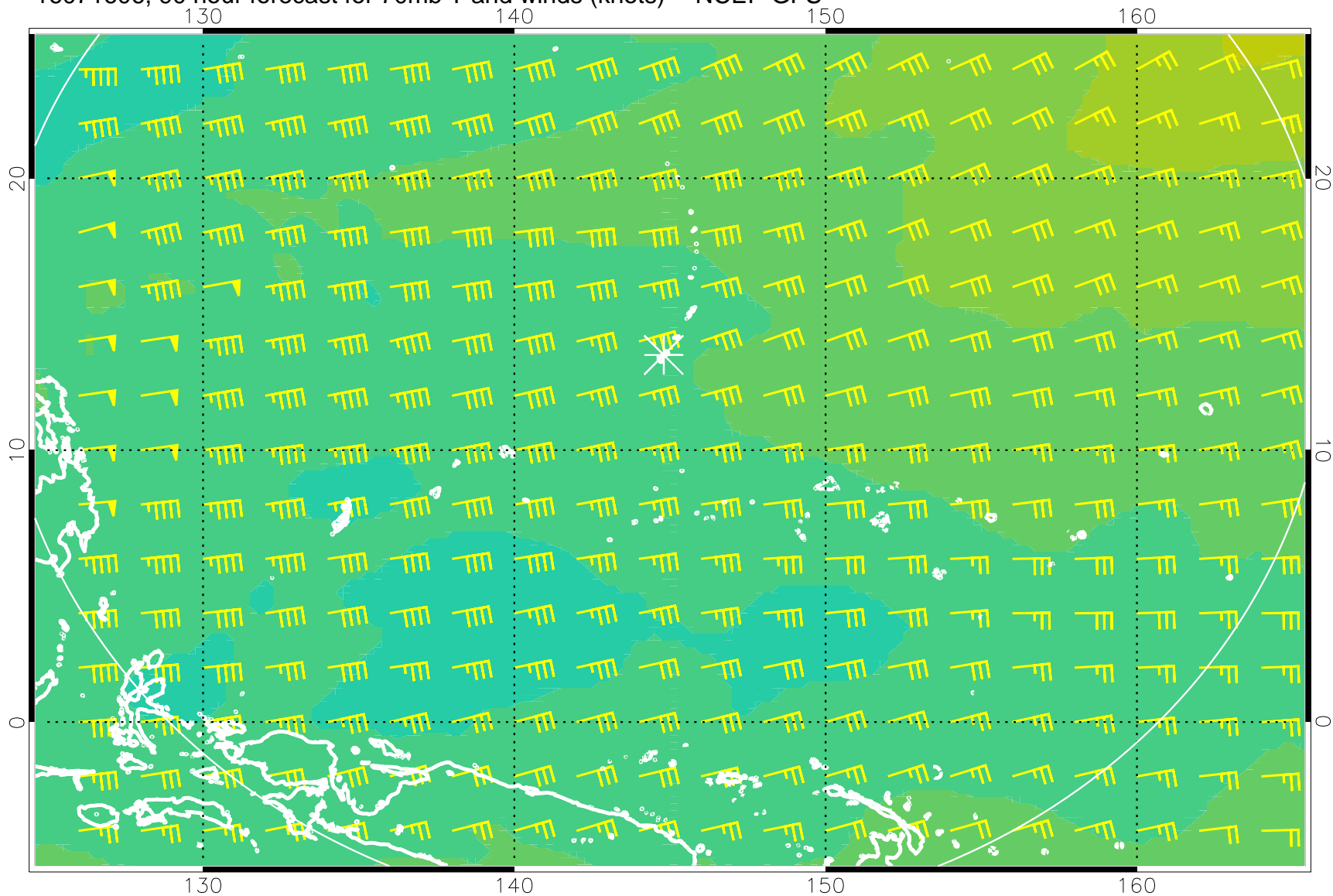
16071606, 90 hour forecast for 70mb T and winds (knots) -- NCEP GFS
