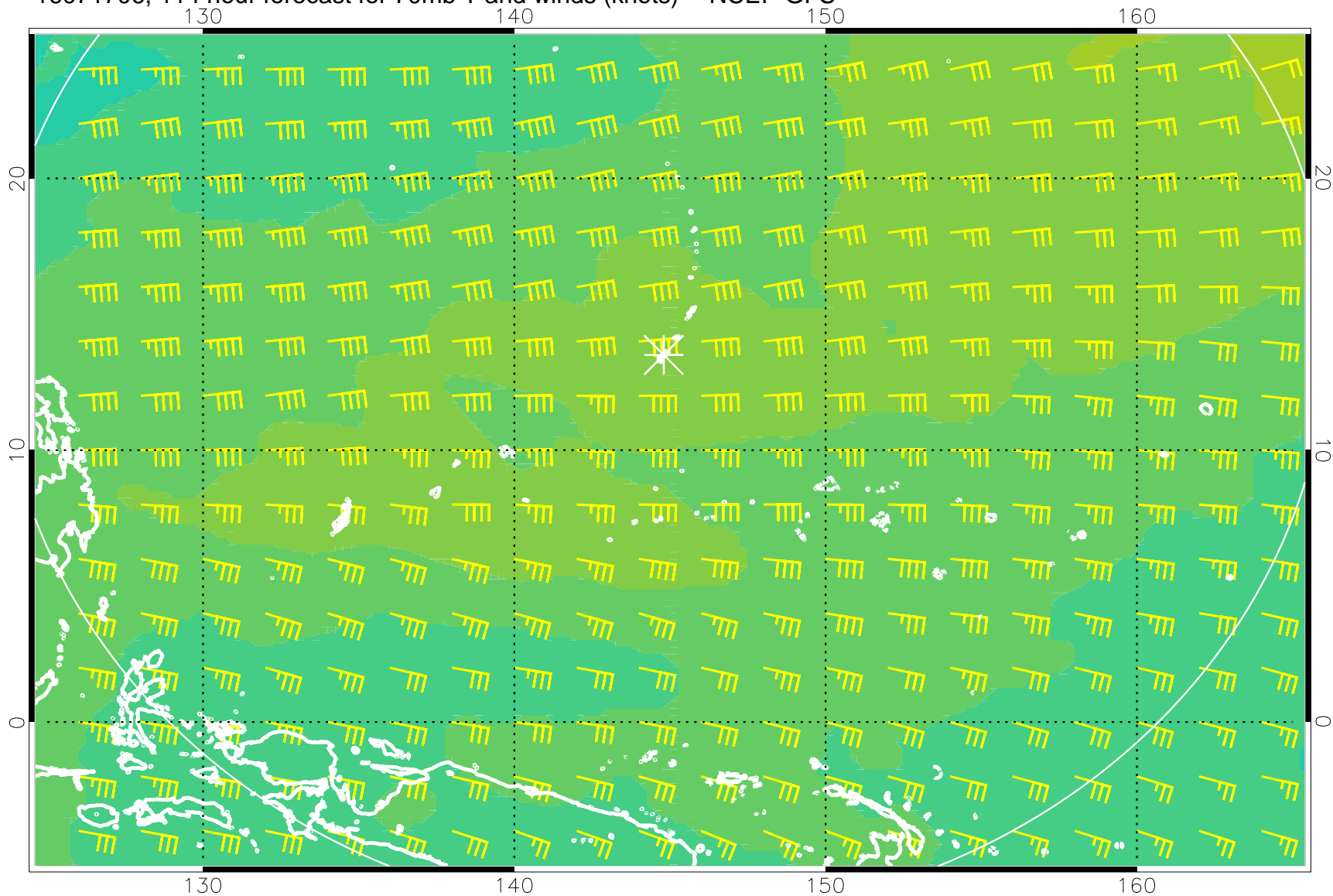
16071706, 114 hour forecast for 70mb T and winds (knots) -- NCEP GFS
