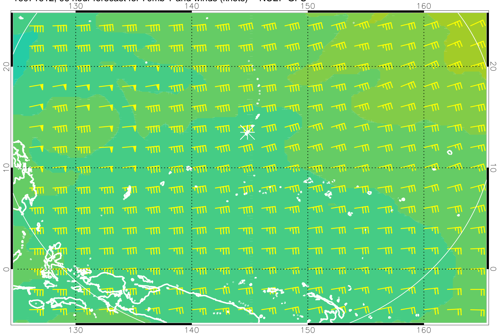
16071612, 96 hour forecast for 70mb T and winds (knots) -- NCEP GFS
