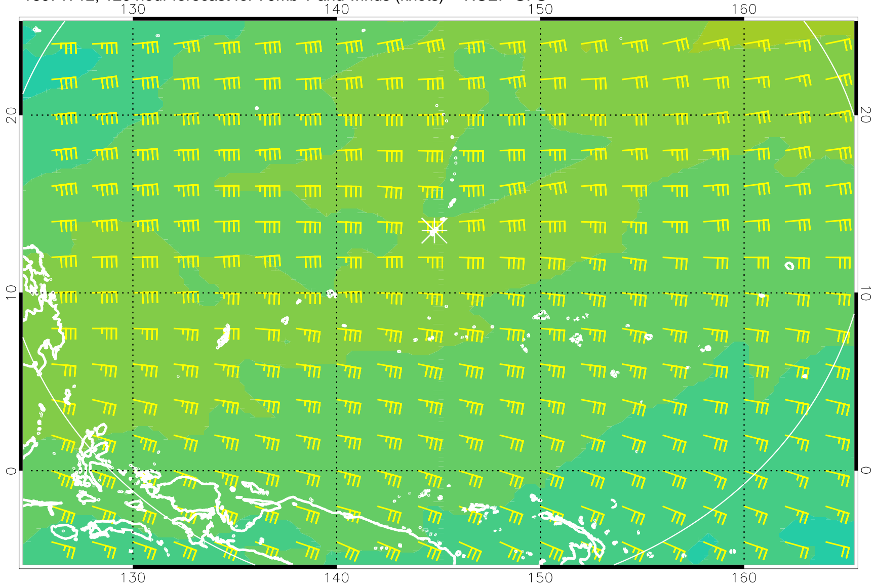
16071712, 120 hour forecast for 70mb T and winds (knots) -- NCEP GFS
