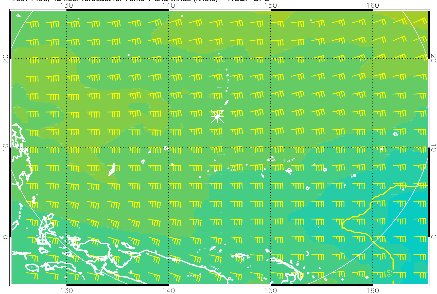
16071406, 42 hour forecast for 70mb T and winds (knots) -- NCEP GFS
