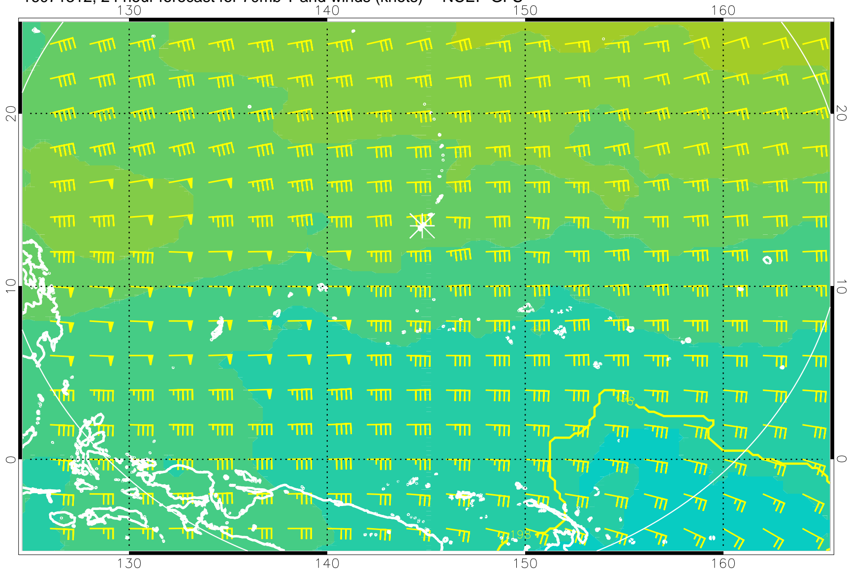
16071312, 24 hour forecast for 70mb T and winds (knots) -- NCEP GFS
