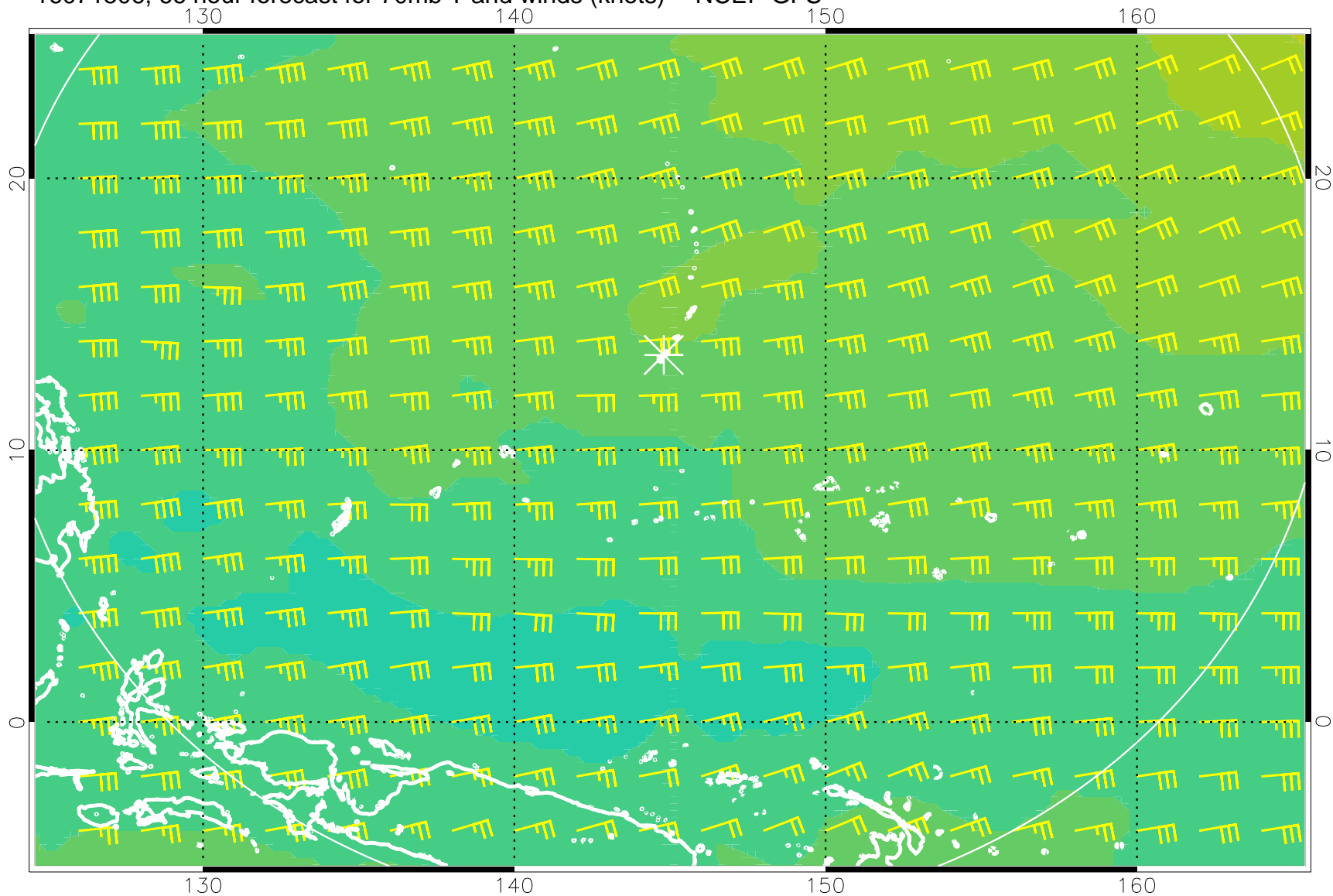
16071506, 66 hour forecast for 70mb T and winds (knots) -- NCEP GFS
