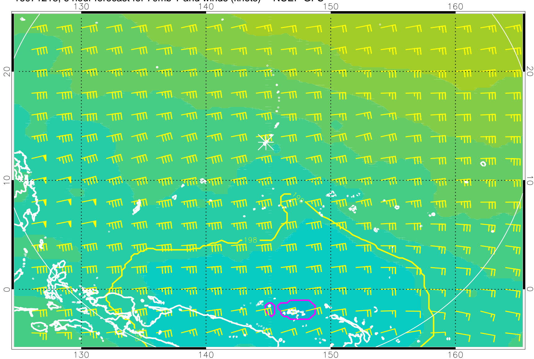
16071218, 6 hour forecast for 70mb T and winds (knots) -- NCEP GFS
