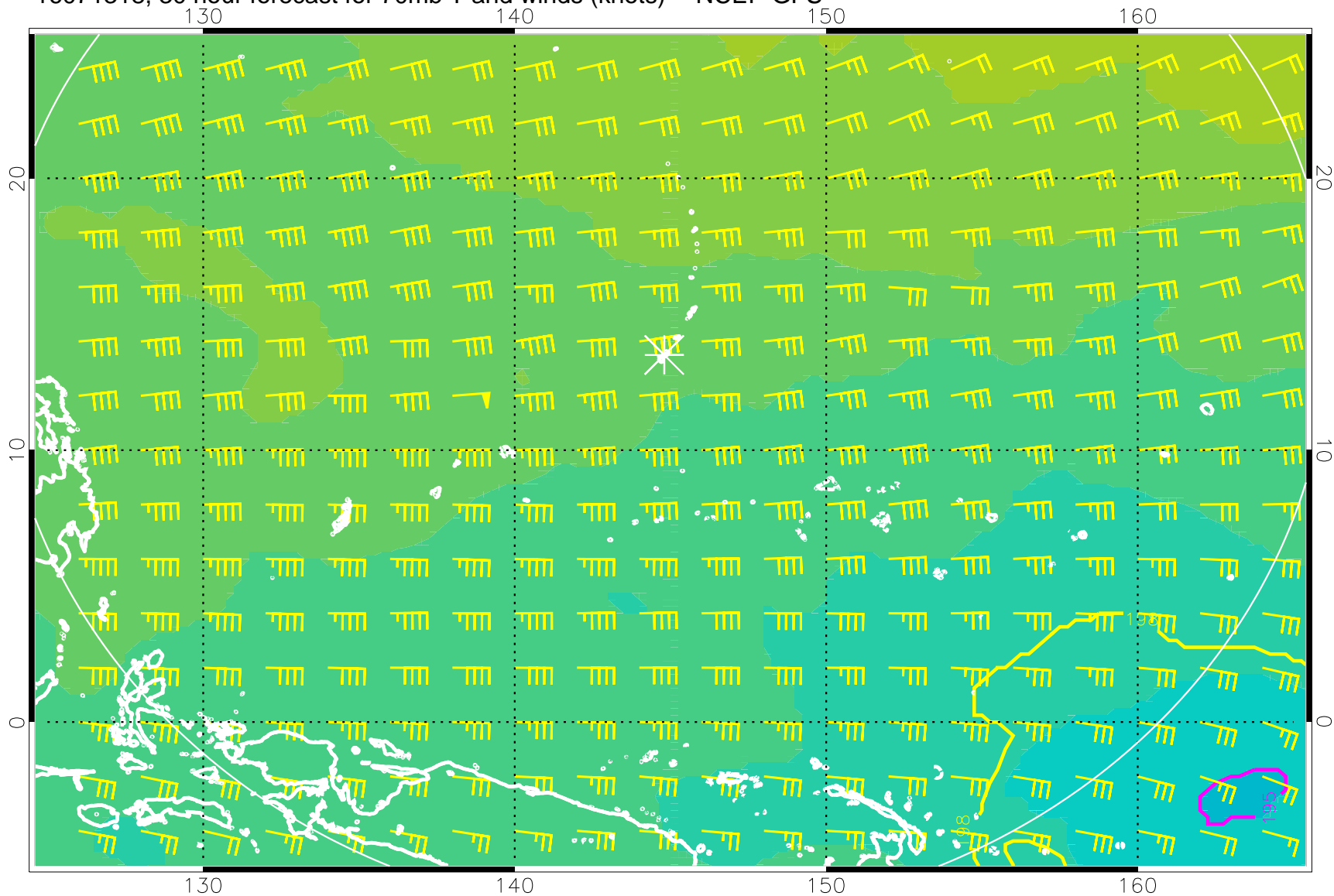
16071318, 30 hour forecast for 70mb T and winds (knots) -- NCEP GFS
