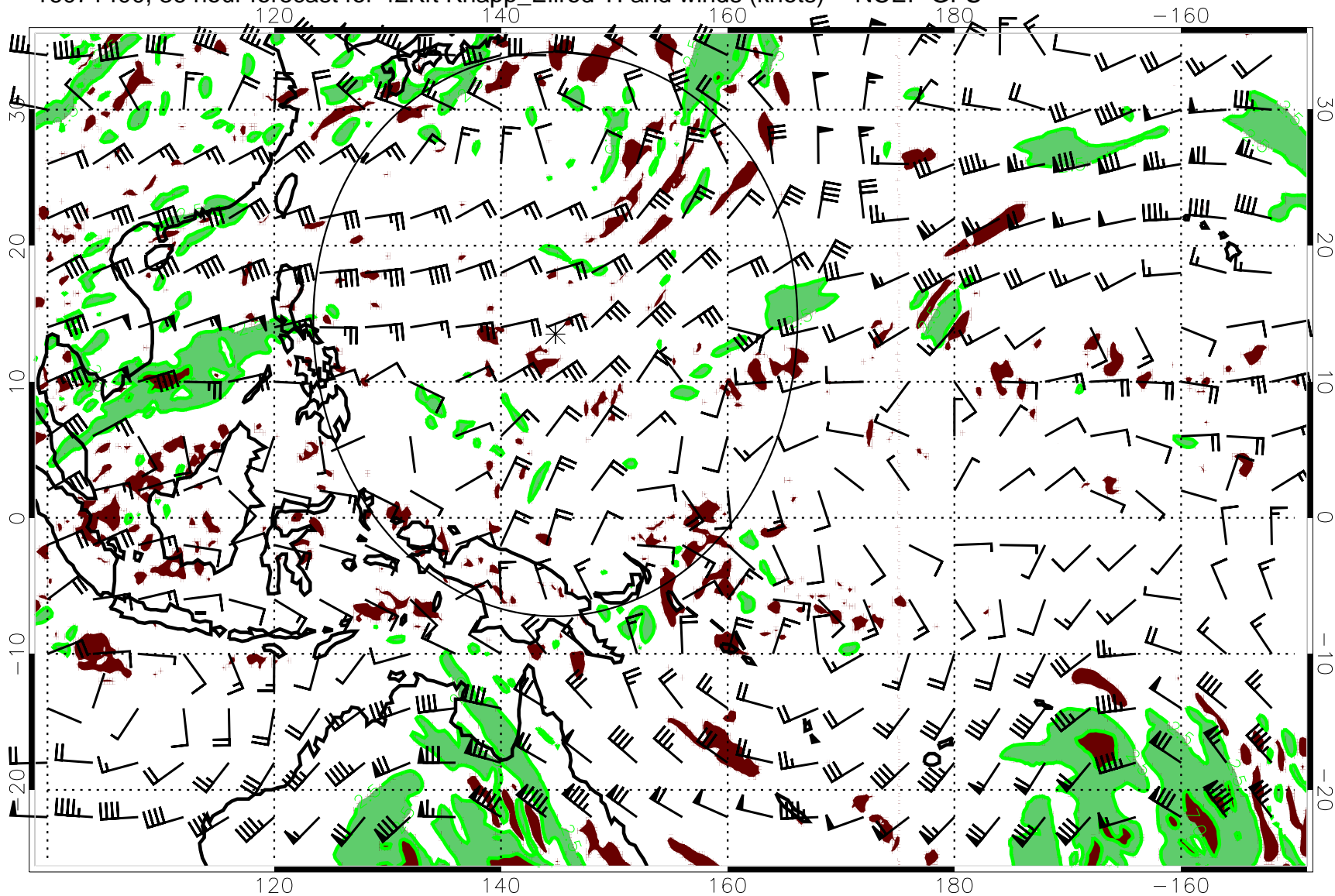
16071400, 36 hour forecast for 42Kft Knapp_Ellrod TI and winds (knots) -- NCEP GFS
