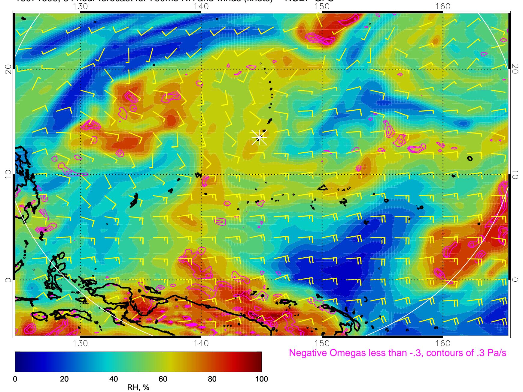
16071600, 84 hour forecast for 700mb RH and winds (knots) -- NCEP GFS
