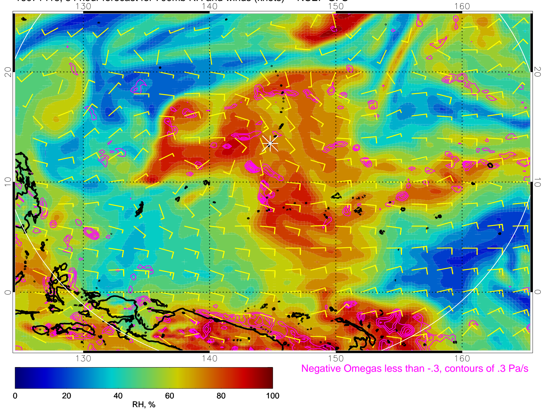
16071418, 54 hour forecast for 700mb RH and winds (knots) -- NCEP GFS
