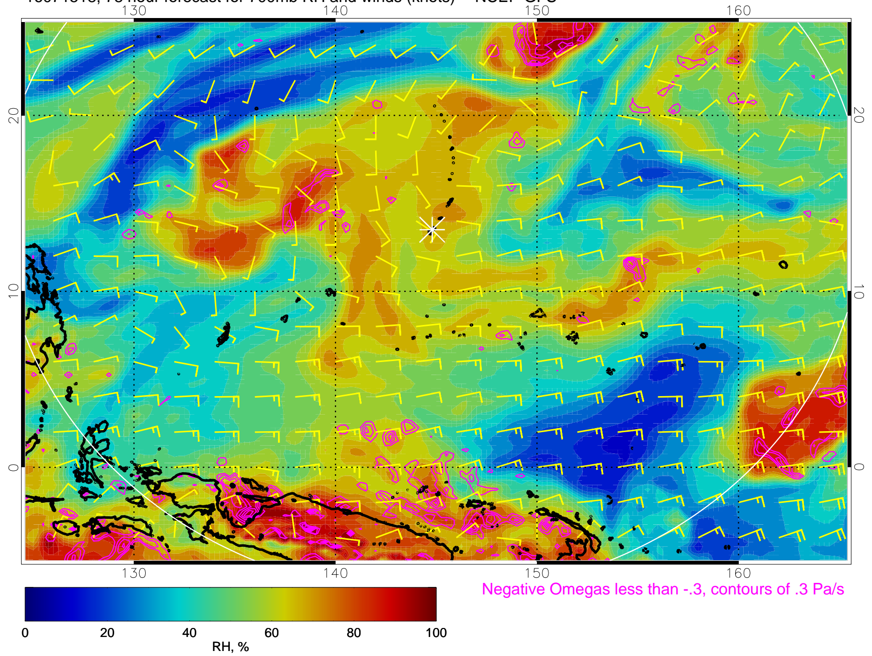
16071518, 78 hour forecast for 700mb RH and winds (knots) -- NCEP GFS
