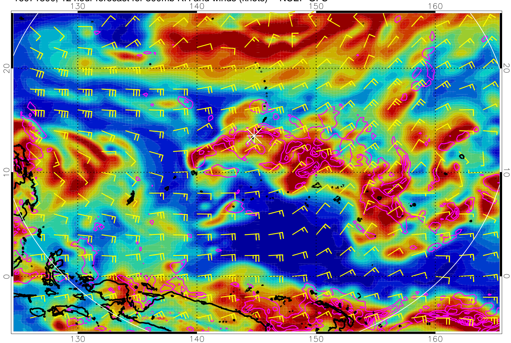
16071300, 12 hour forecast for 300mb RH and winds (knots) -- NCEP GFS
