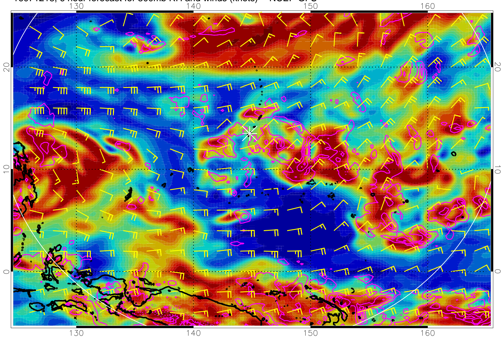
16071218, 6 hour forecast for 300mb RH and winds (knots) -- NCEP GFS
