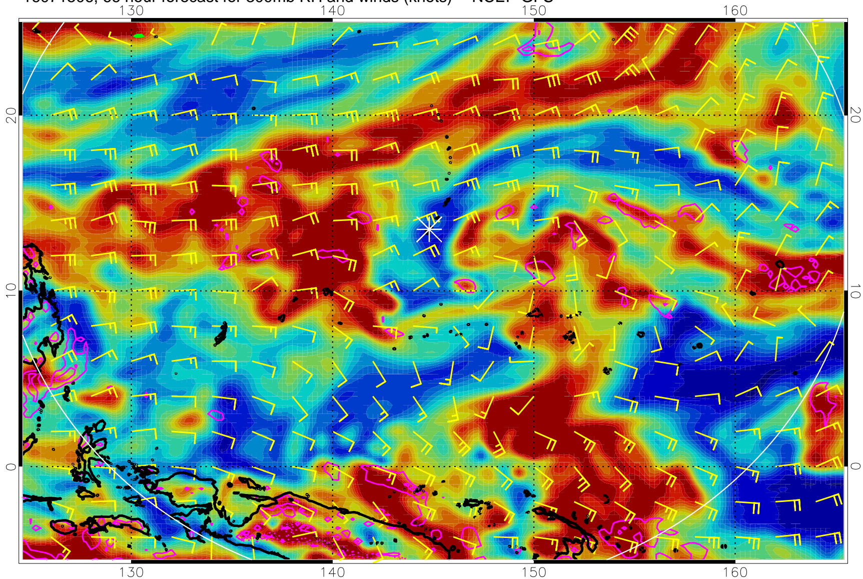
16071506, 66 hour forecast for 300mb RH and winds (knots) -- NCEP GFS
