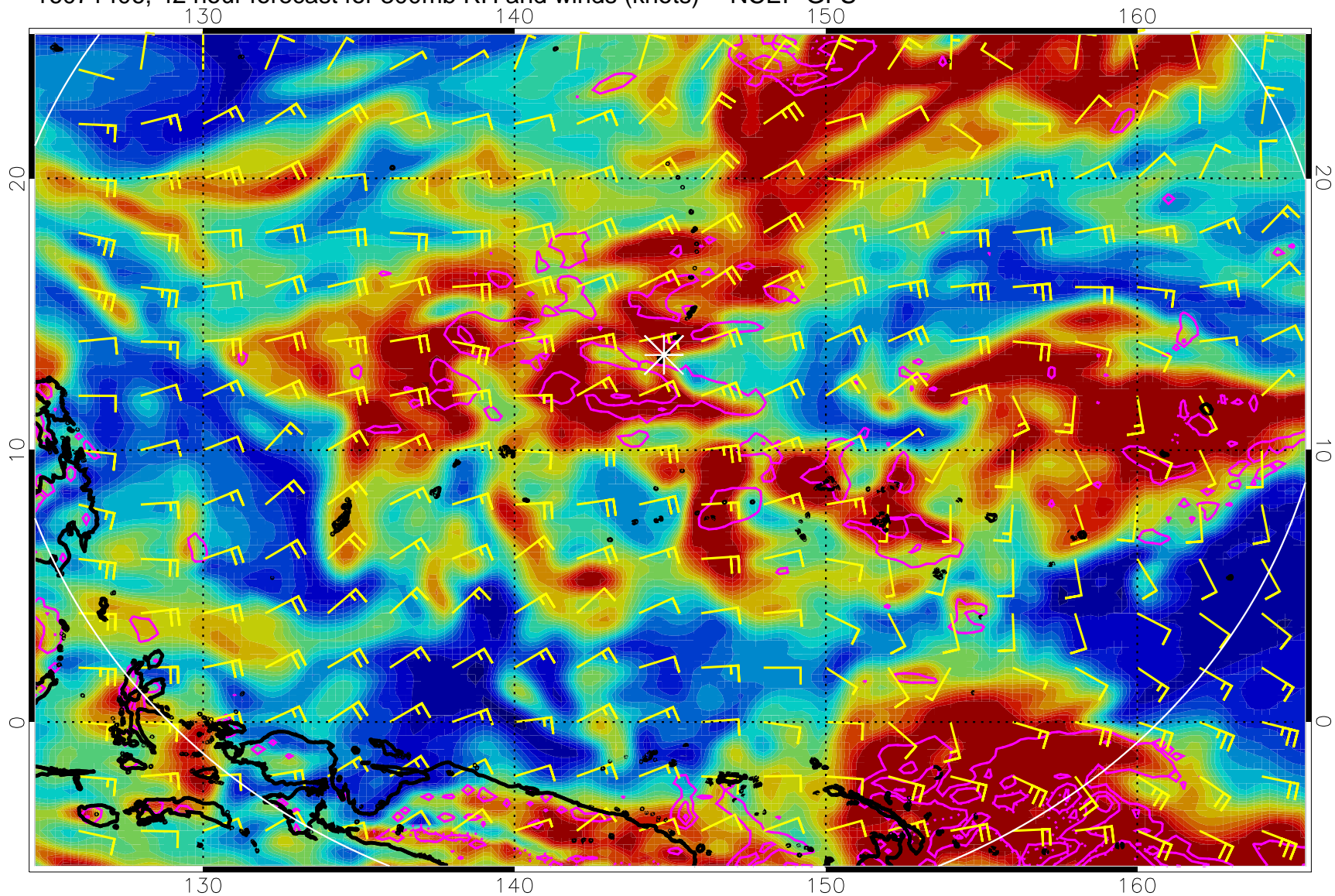
16071406, 42 hour forecast for 300mb RH and winds (knots) -- NCEP GFS
