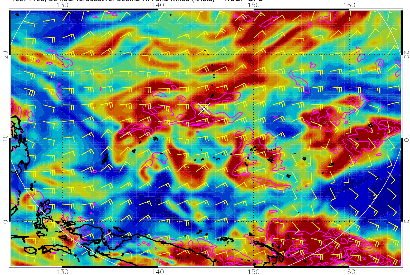
16071400, 36 hour forecast for 300mb RH and winds (knots) -- NCEP GFS
