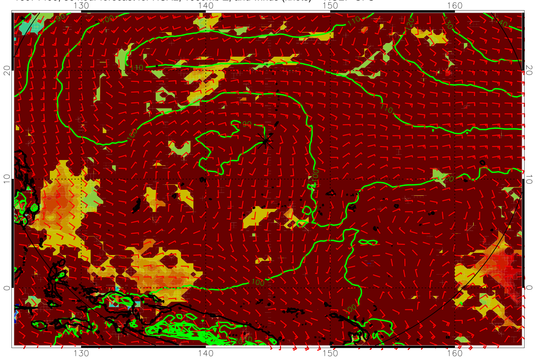
16071400, 36 hour forecast for HCAL, 1000mb Z, and winds (knots) -- NCEP GFS
