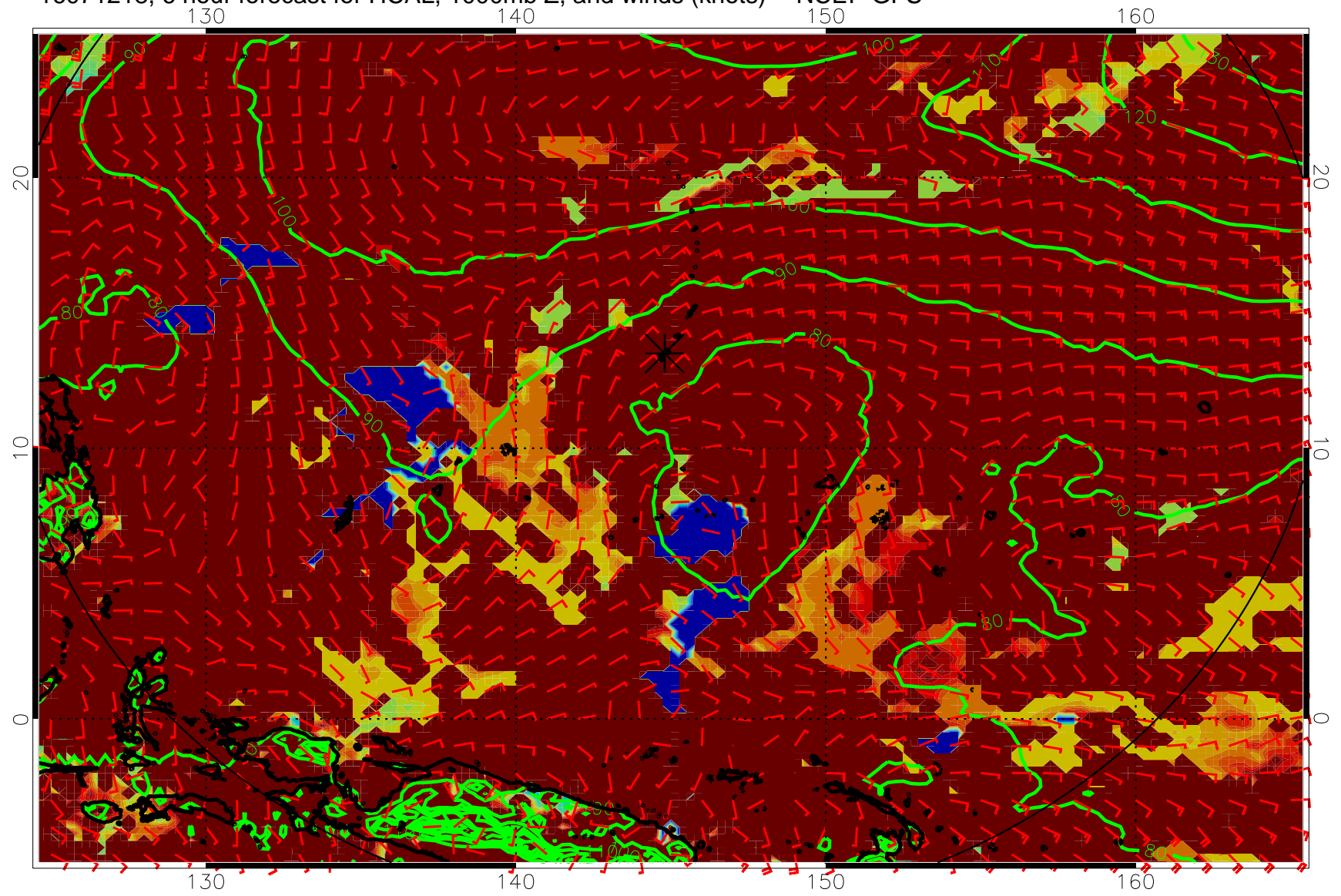
16071218, 6 hour forecast for HCAL, 1000mb Z, and winds (knots) -- NCEP GFS
