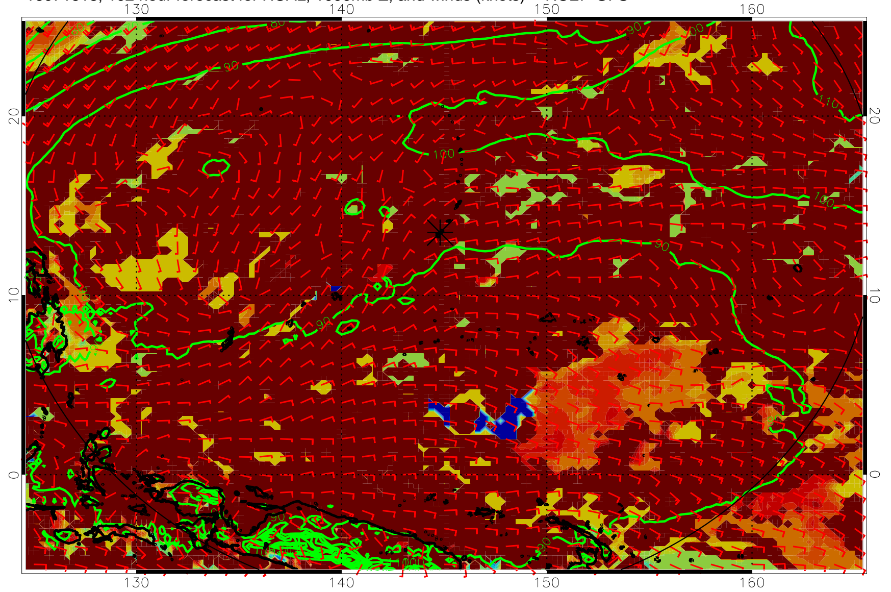
16071618, 102 hour forecast for HCAL, 1000mb Z, and winds (knots) -- NCEP GFS
