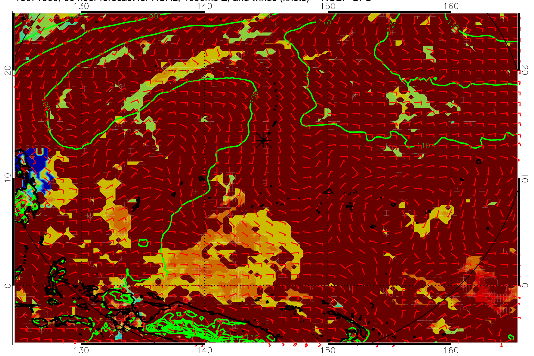
16071500, 60 hour forecast for HCAL, 1000mb Z, and winds (knots) -- NCEP GFS
