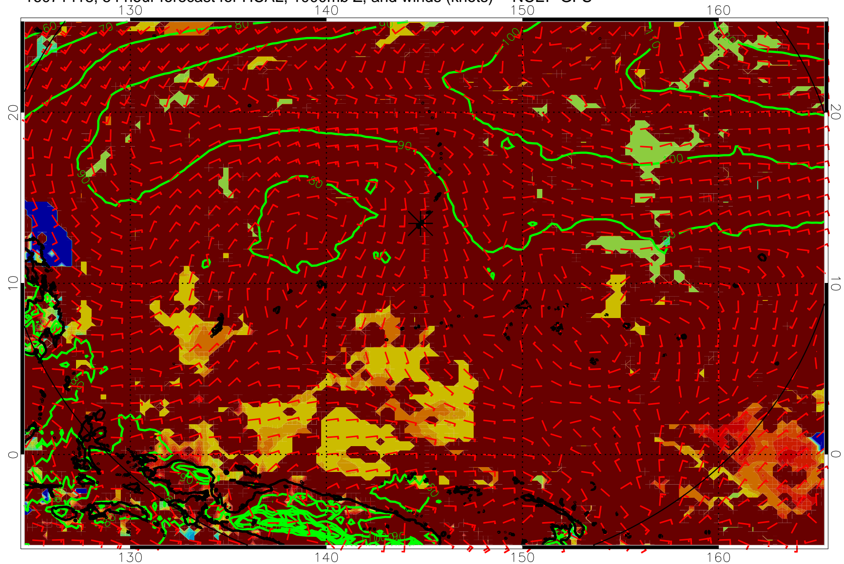
16071418, 54 hour forecast for HCAL, 1000mb Z, and winds (knots) -- NCEP GFS
