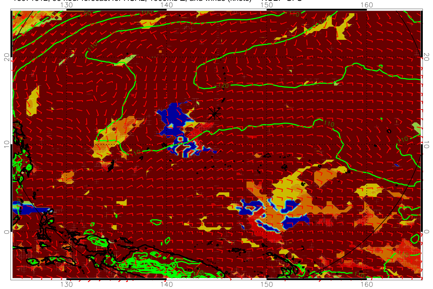
16071612, 96 hour forecast for HCAL, 1000mb Z, and winds (knots) -- NCEP GFS
