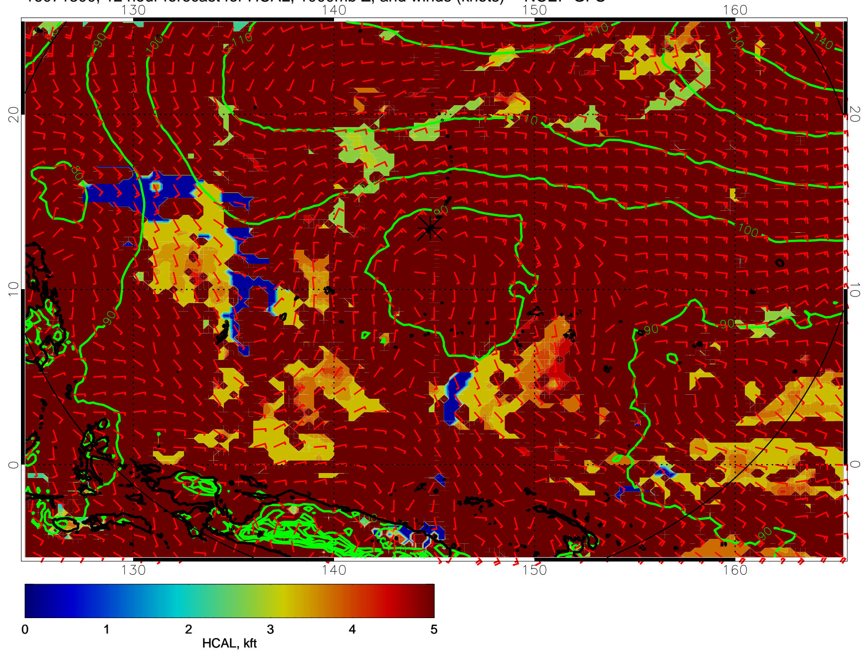
16071300, 12 hour forecast for HCAL, 1000mb Z, and winds (knots) -- NCEP GFS
