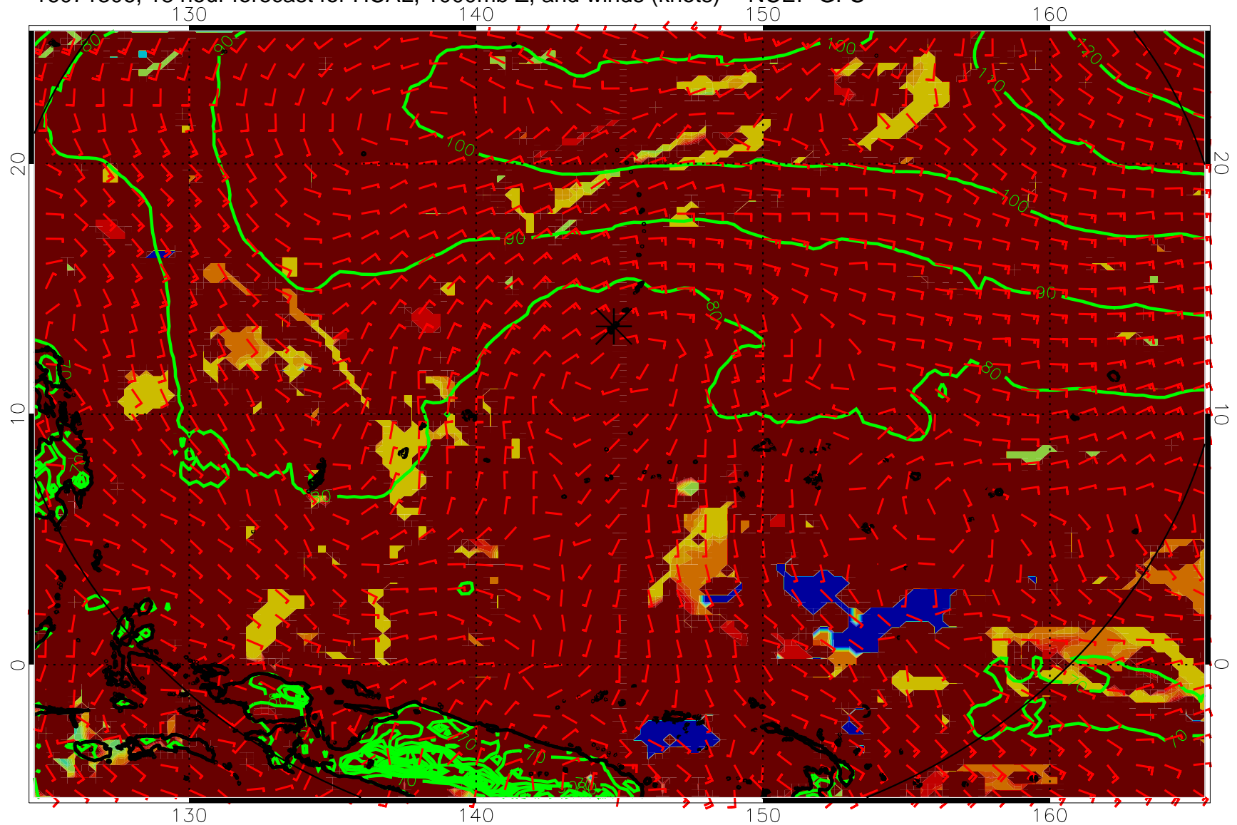
16071306, 18 hour forecast for HCAL, 1000mb Z, and winds (knots) -- NCEP GFS
