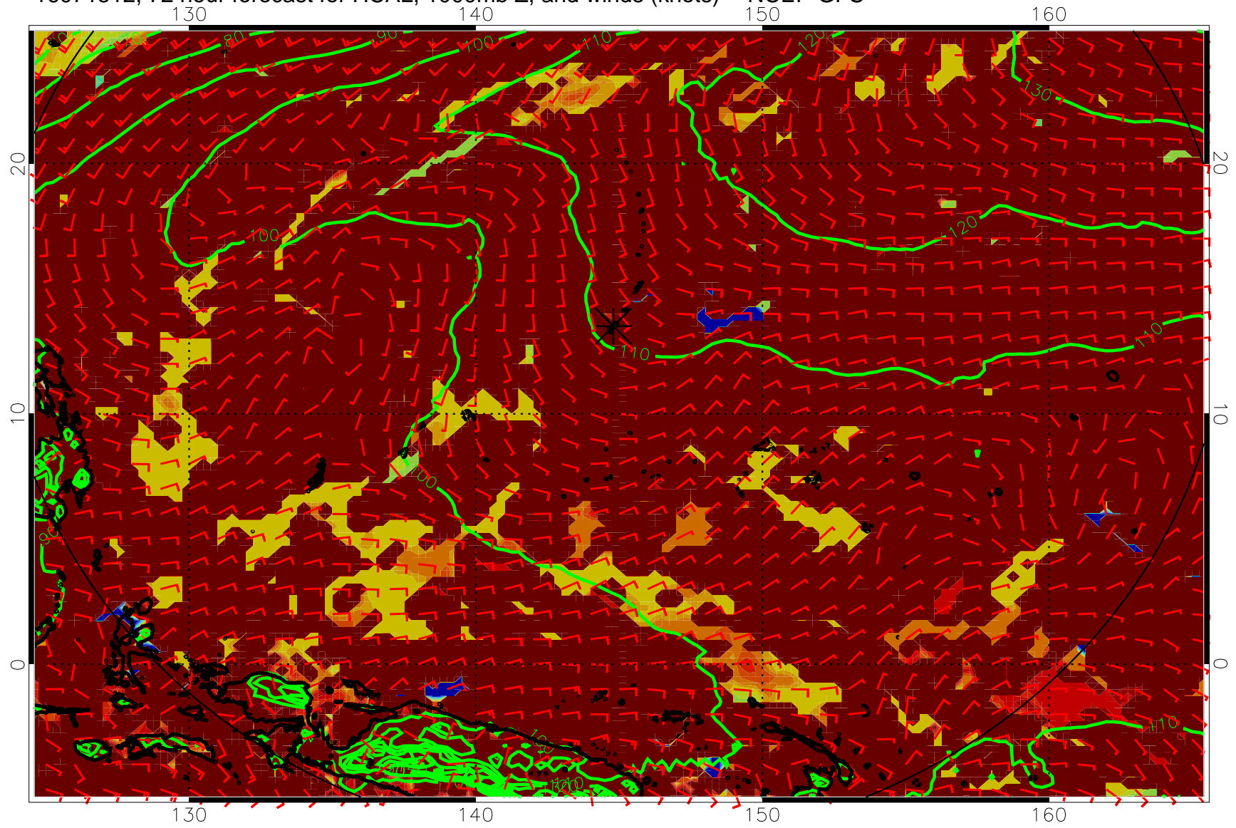
16071512, 72 hour forecast for HCAL, 1000mb Z, and winds (knots) -- NCEP GFS
