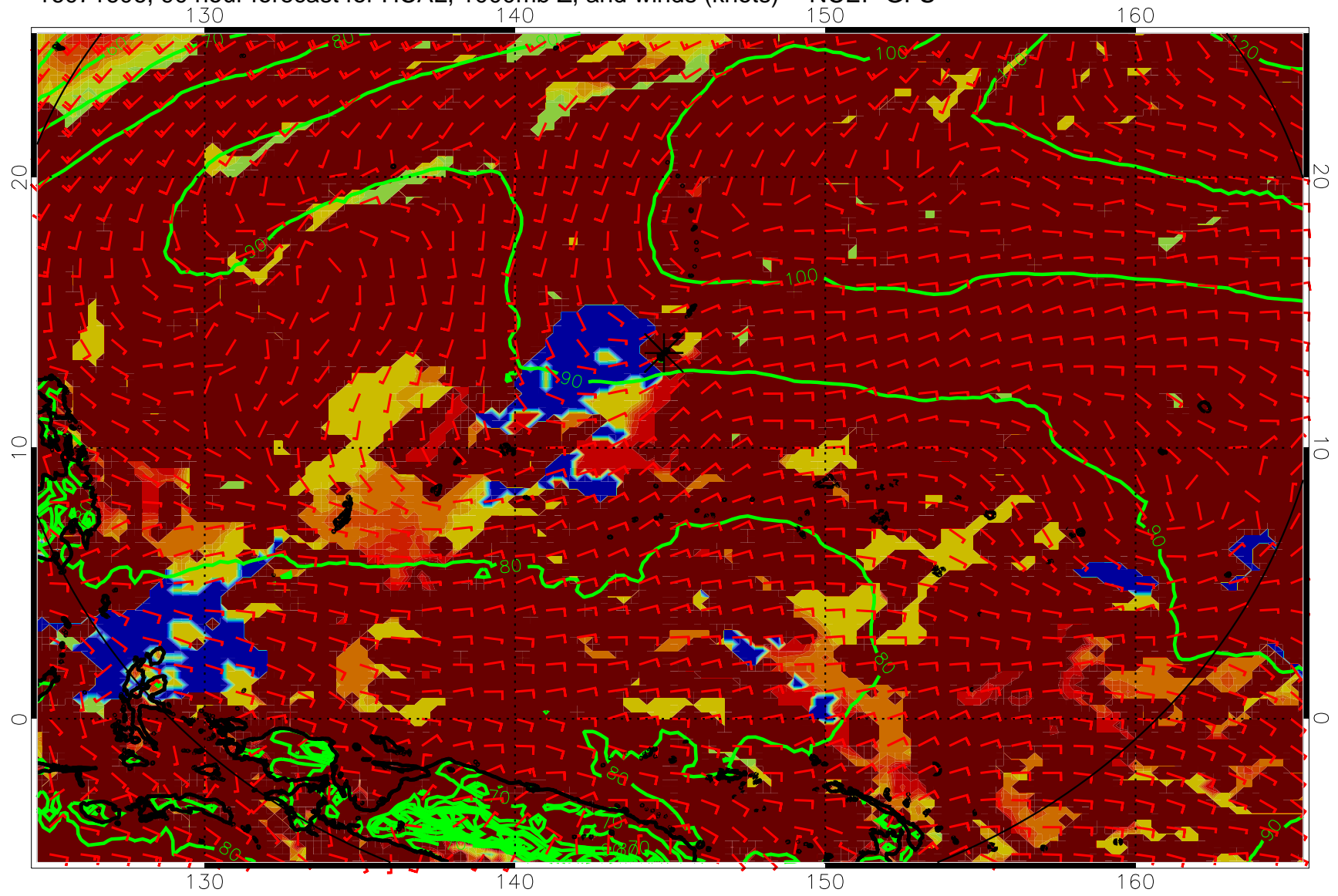
16071606, 90 hour forecast for HCAL, 1000mb Z, and winds (knots) -- NCEP GFS
