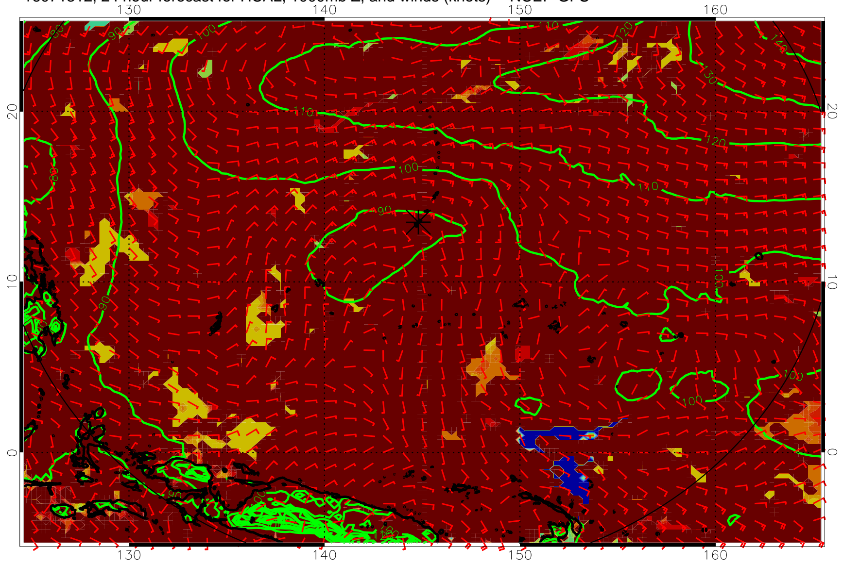
16071312, 24 hour forecast for HCAL, 1000mb Z, and winds (knots) -- NCEP GFS
