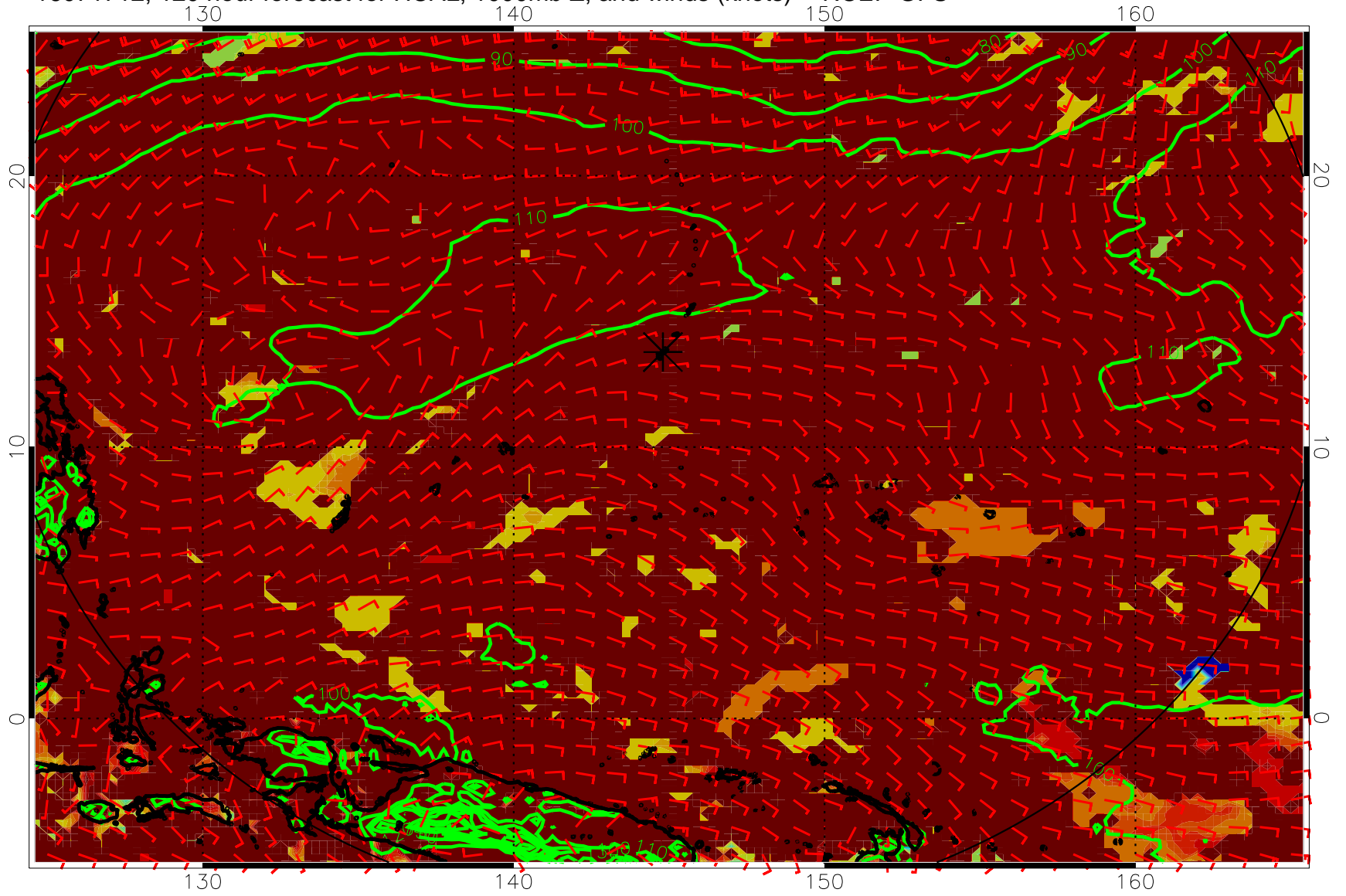
16071712, 120 hour forecast for HCAL, 1000mb Z, and winds (knots) -- NCEP GFS
