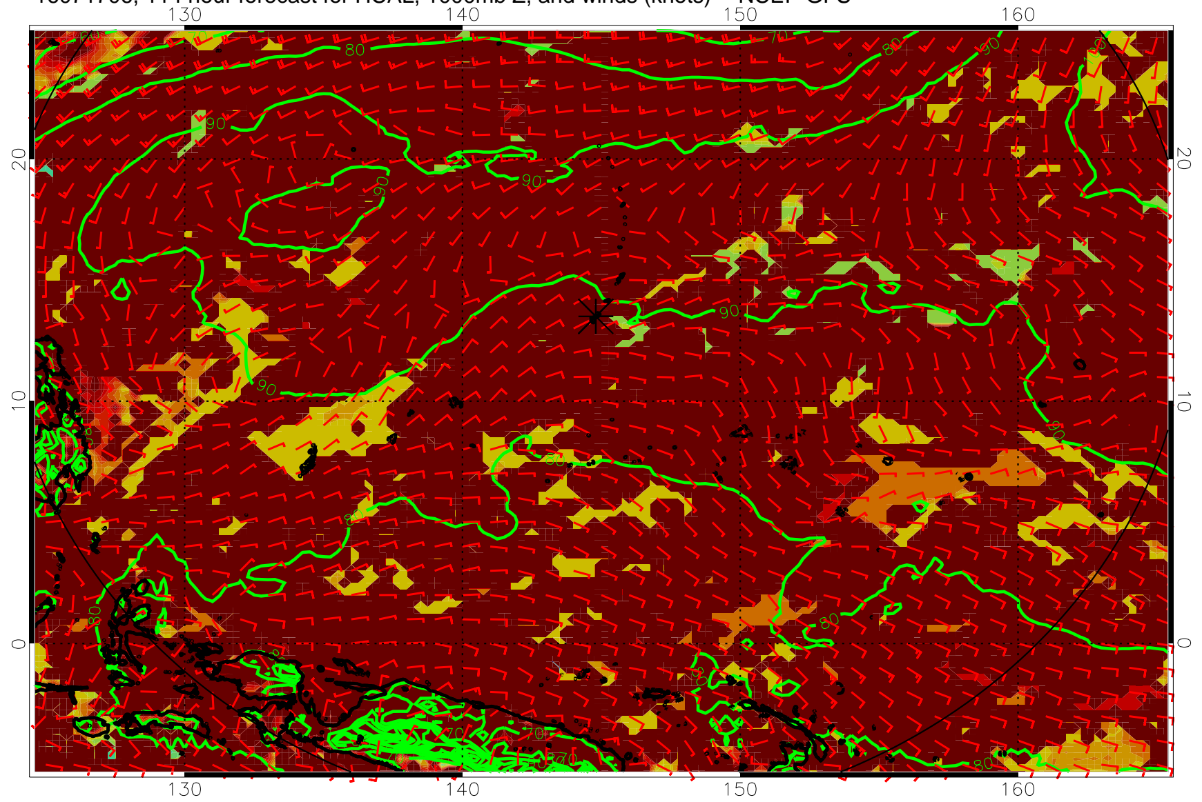
16071706, 114 hour forecast for HCAL, 1000mb Z, and winds (knots) -- NCEP GFS
