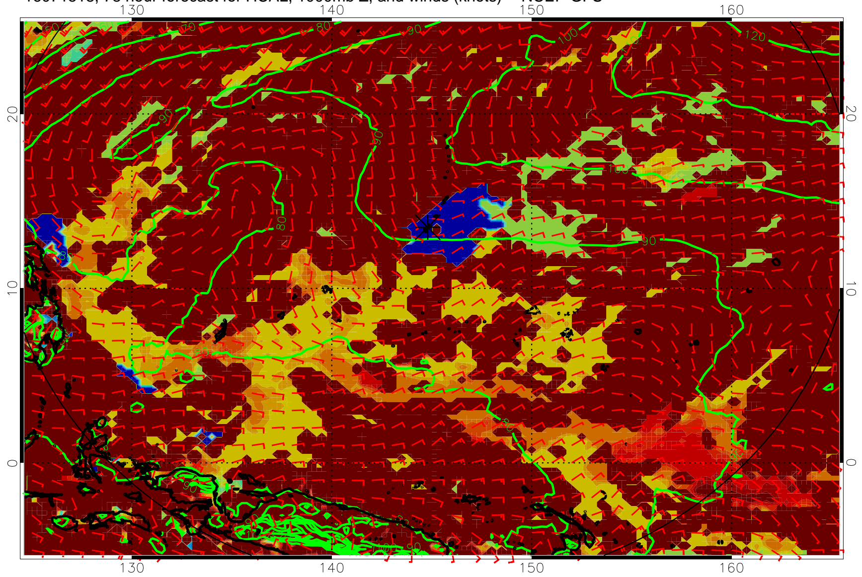
16071518, 78 hour forecast for HCAL, 1000mb Z, and winds (knots) -- NCEP GFS
