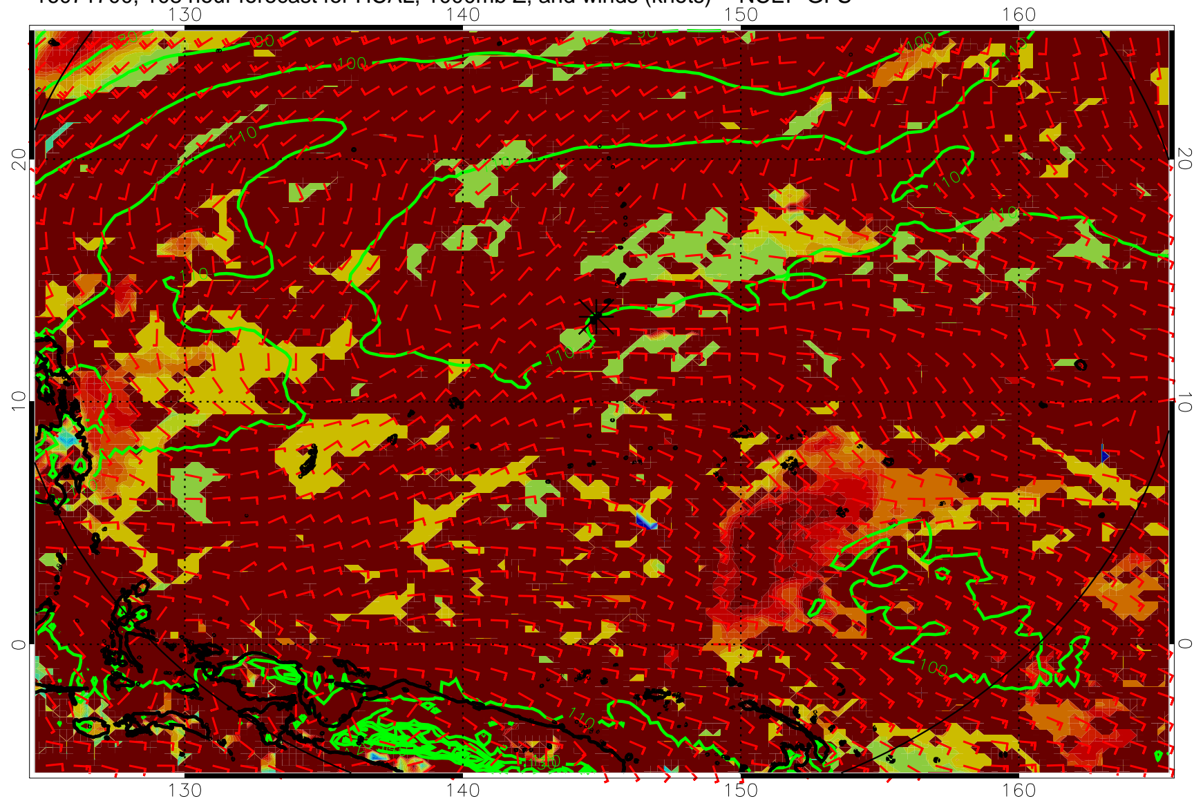
16071700, 108 hour forecast for HCAL, 1000mb Z, and winds (knots) -- NCEP GFS
