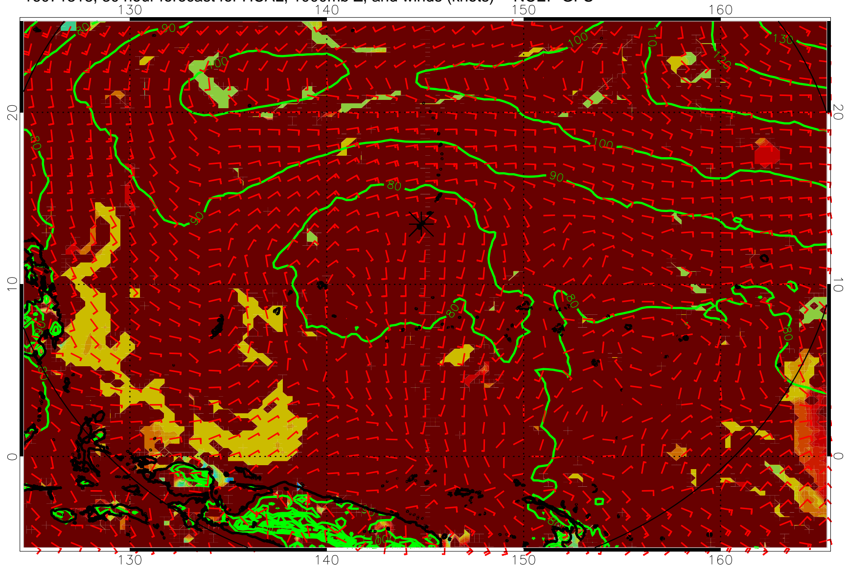
16071318, 30 hour forecast for HCAL, 1000mb Z, and winds (knots) -- NCEP GFS
