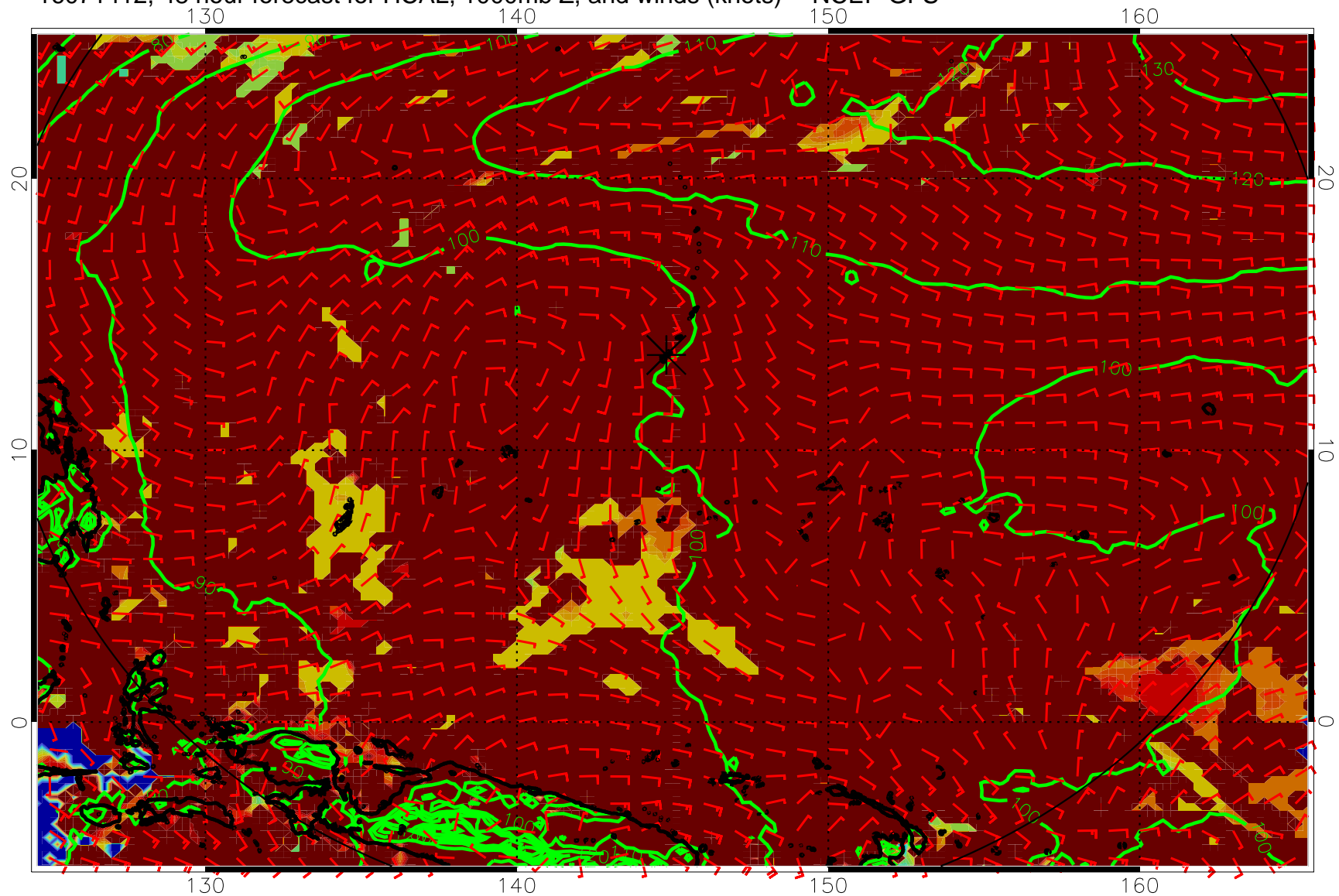
16071412, 48 hour forecast for HCAL, 1000mb Z, and winds (knots) -- NCEP GFS
