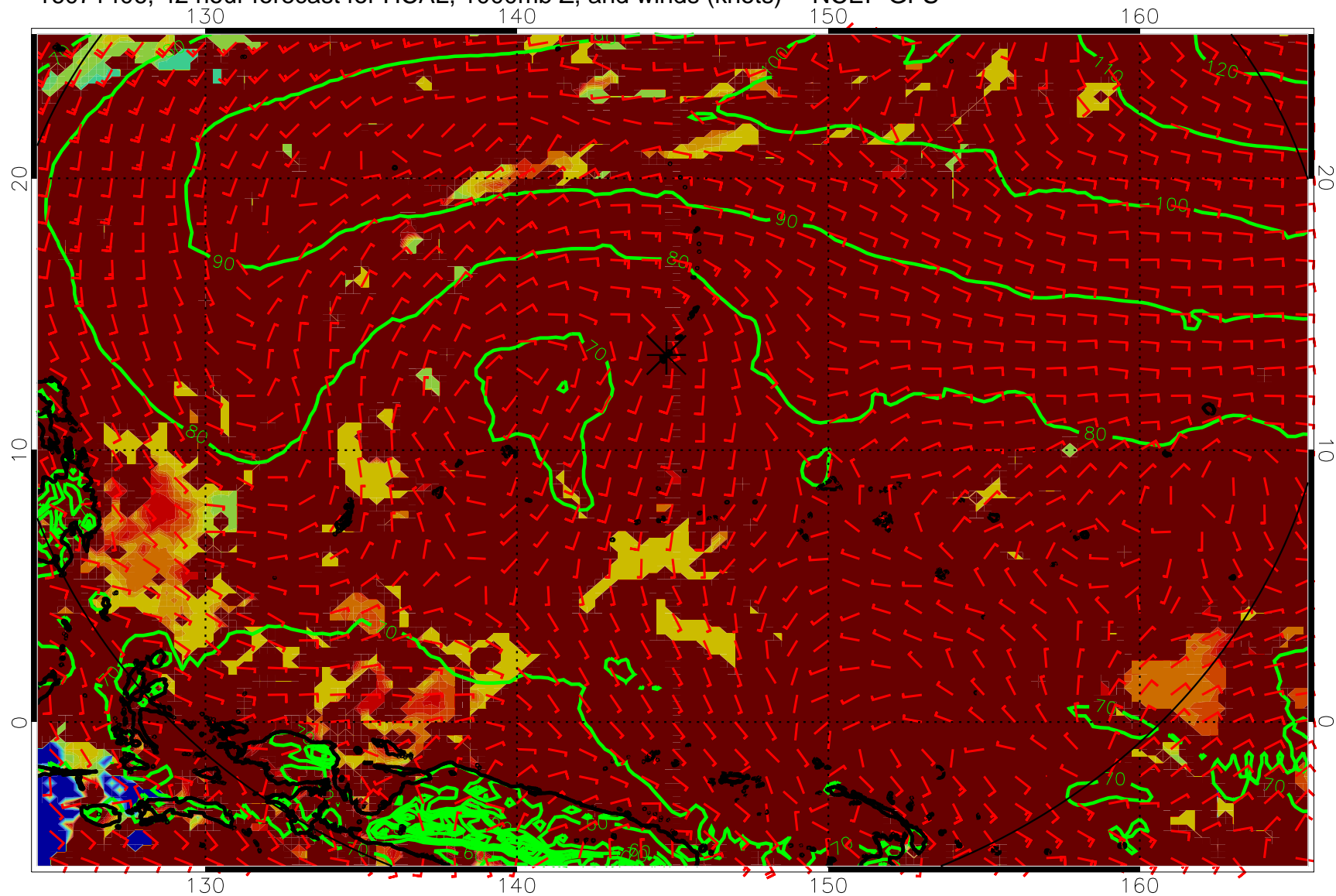
16071406, 42 hour forecast for HCAL, 1000mb Z, and winds (knots) -- NCEP GFS
