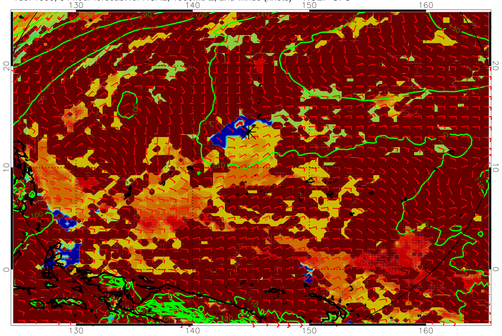
16071600, 84 hour forecast for HCAL, 1000mb Z, and winds (knots) -- NCEP GFS
