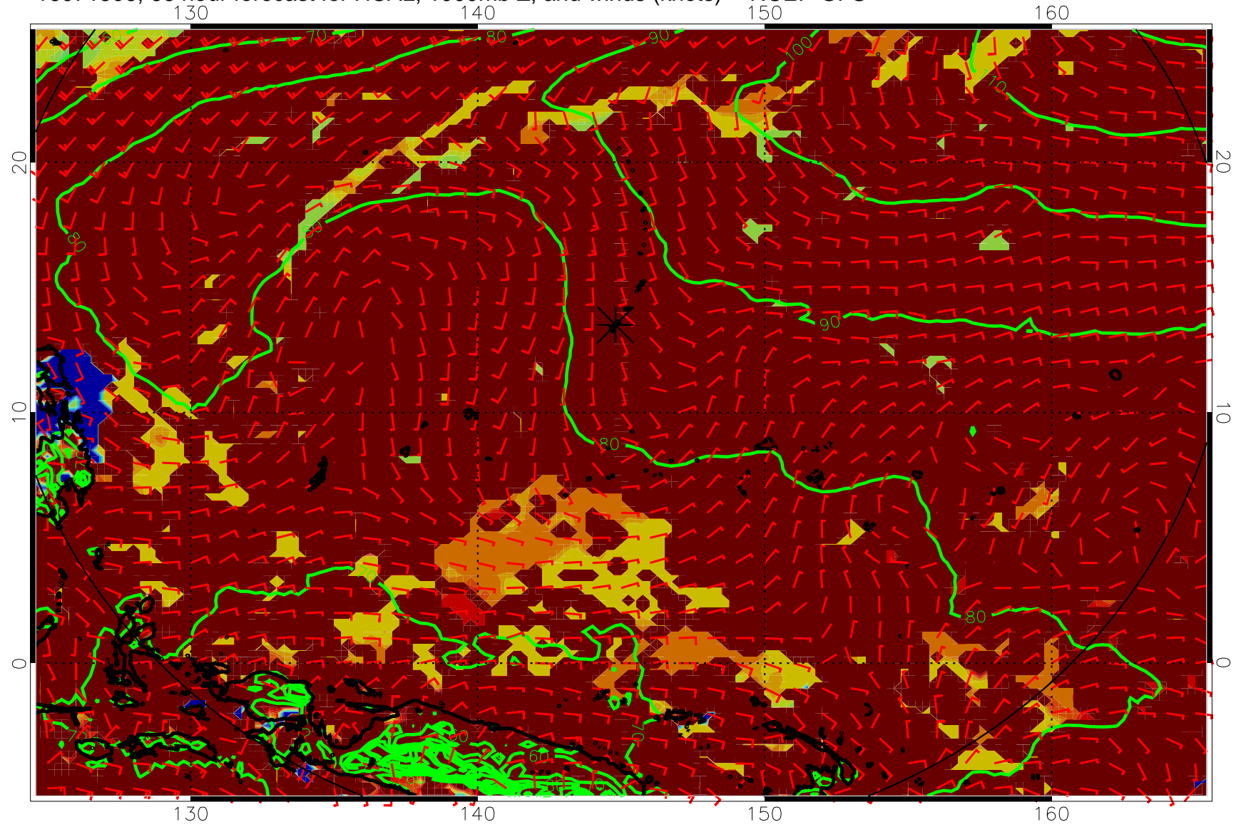
16071506, 66 hour forecast for HCAL, 1000mb Z, and winds (knots) -- NCEP GFS
