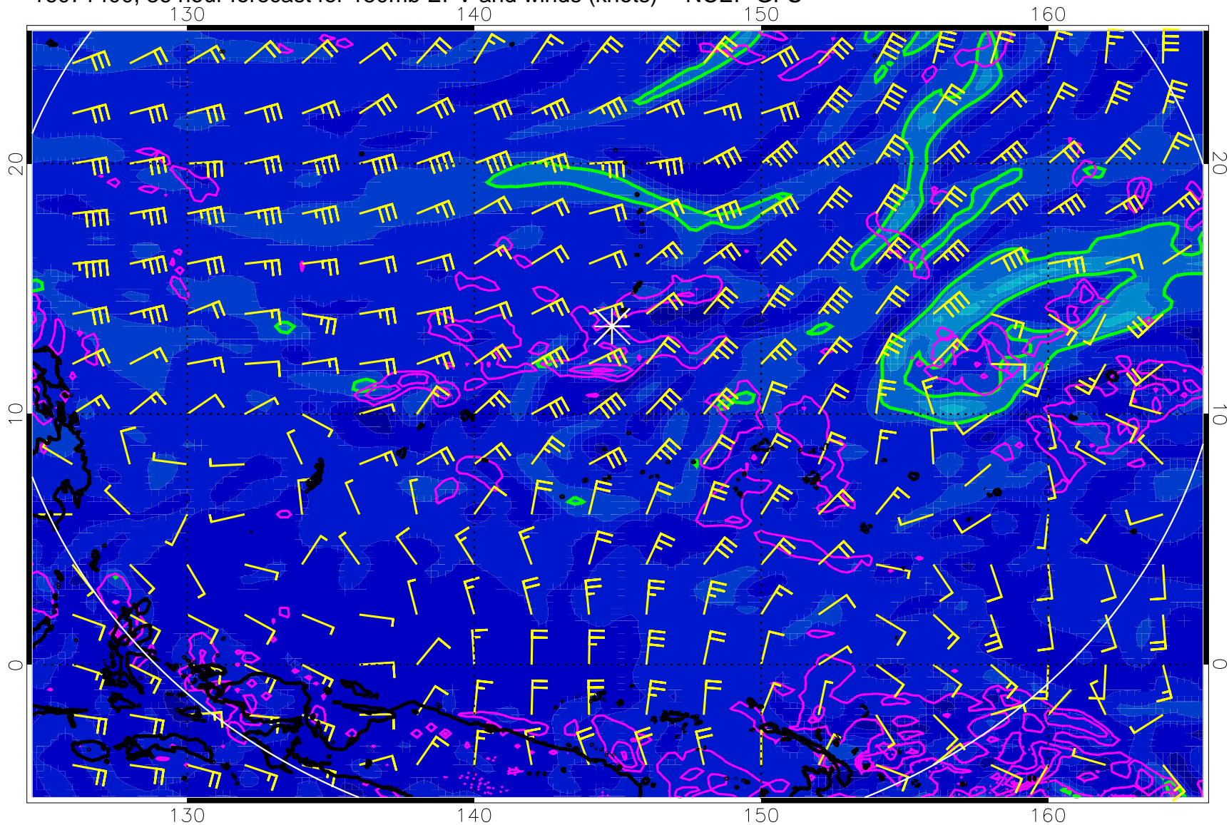
16071400, 36 hour forecast for 150mb EPV and winds (knots) -- NCEP GFS
