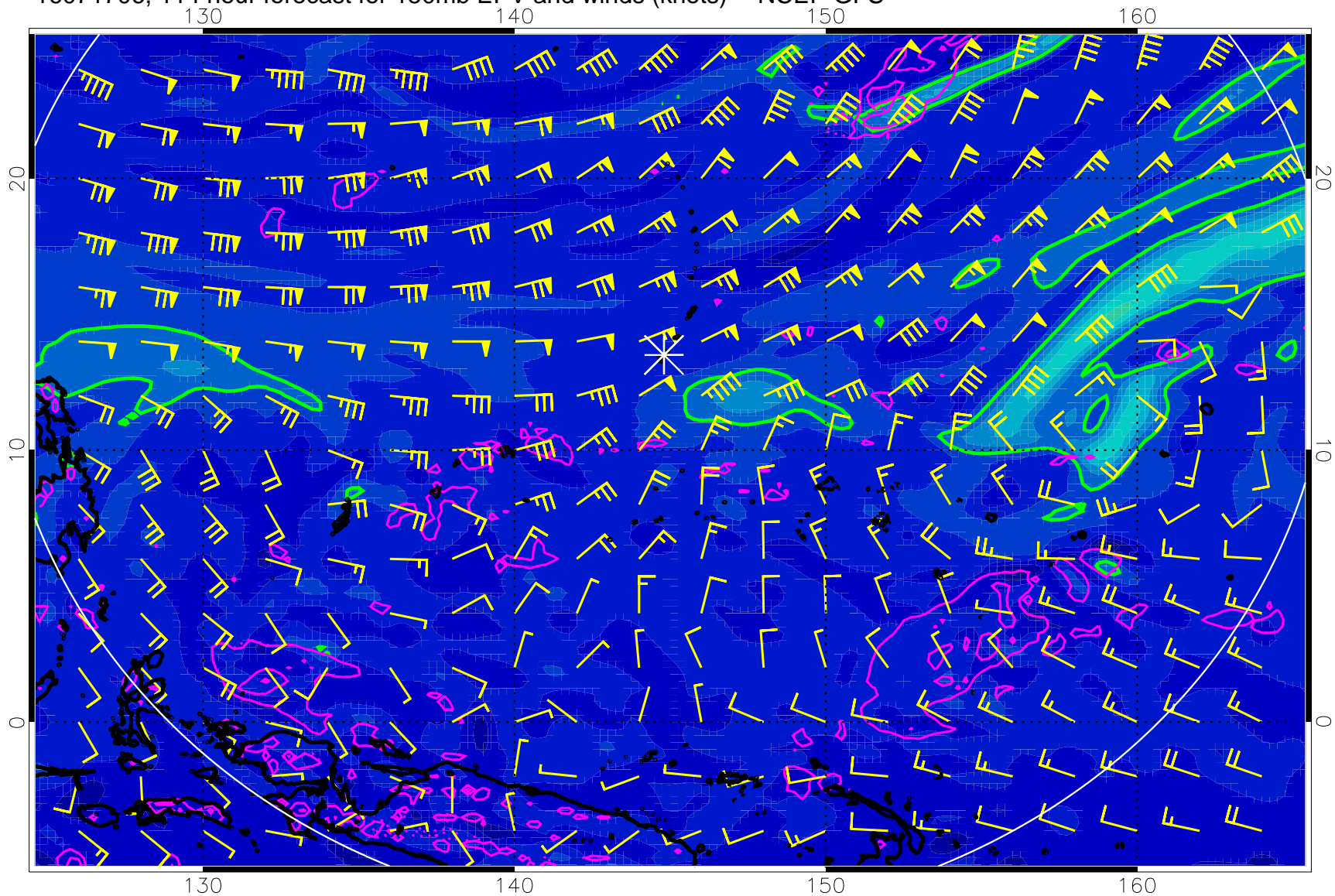
16071706, 114 hour forecast for 150mb EPV and winds (knots) -- NCEP GFS
