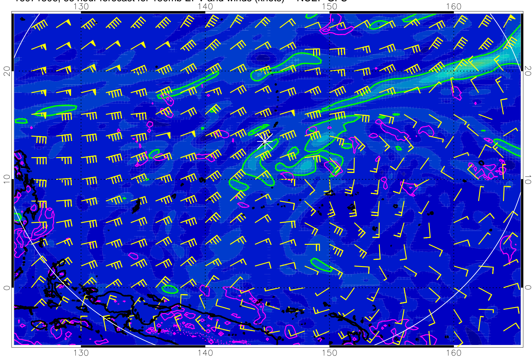
16071506, 66 hour forecast for 150mb EPV and winds (knots) -- NCEP GFS
