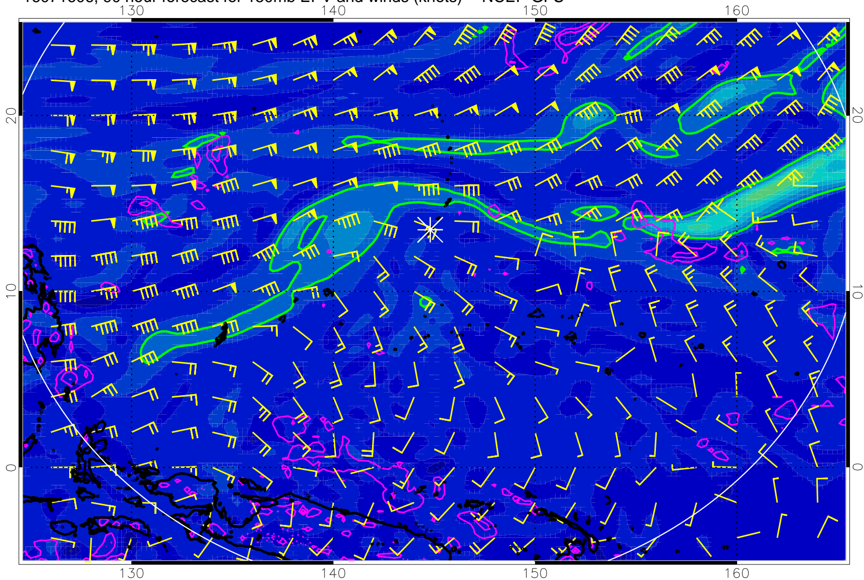
16071606, 90 hour forecast for 150mb EPV and winds (knots) -- NCEP GFS
