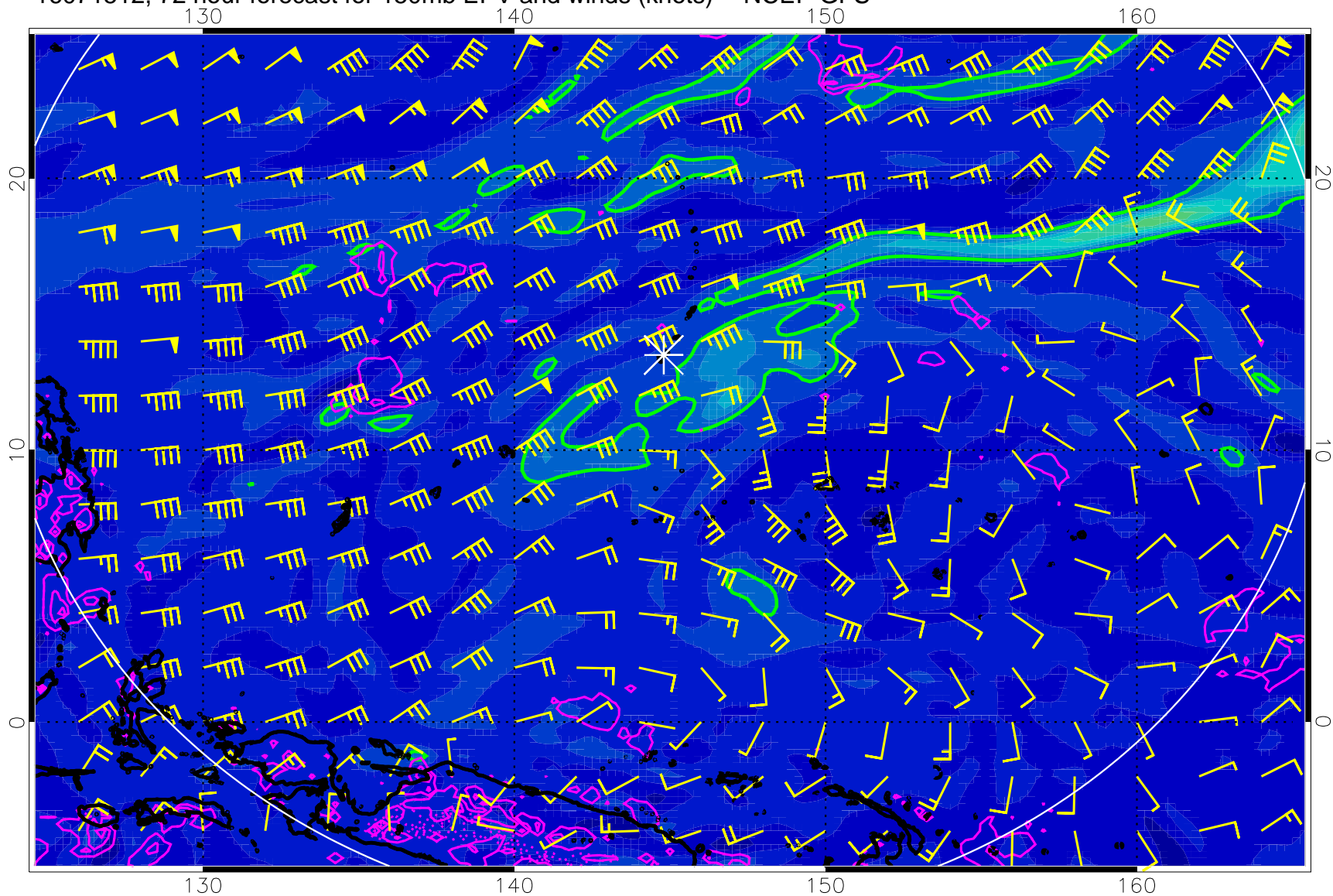
16071512, 72 hour forecast for 150mb EPV and winds (knots) -- NCEP GFS
