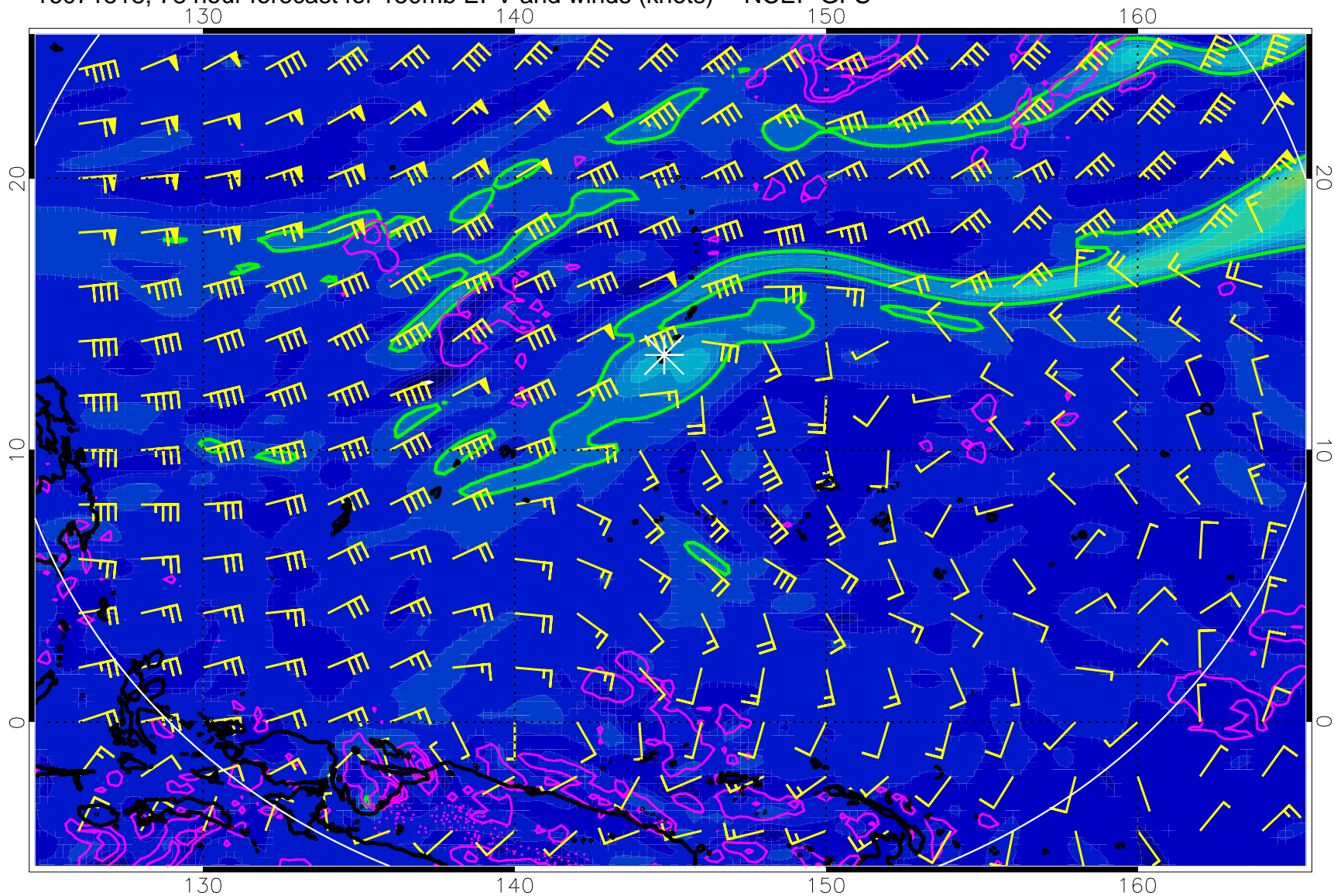
16071518, 78 hour forecast for 150mb EPV and winds (knots) -- NCEP GFS
