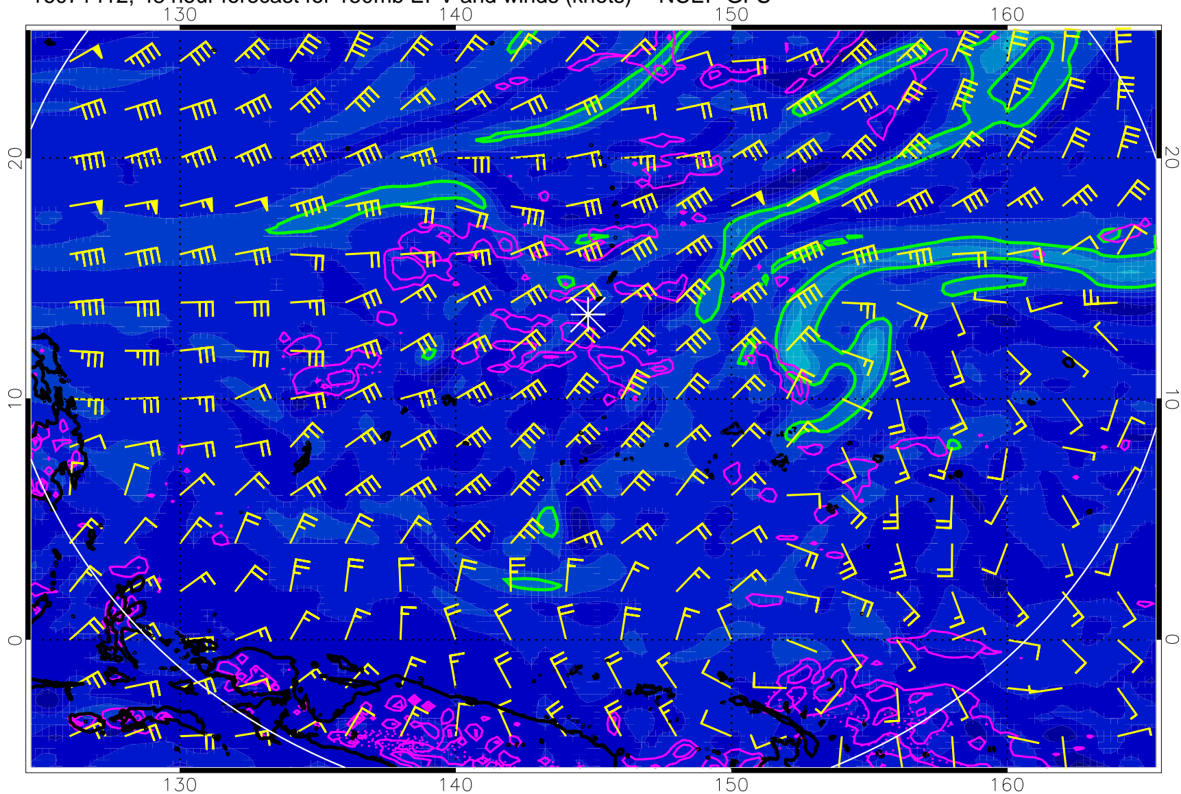
16071412, 48 hour forecast for 150mb EPV and winds (knots) -- NCEP GFS
