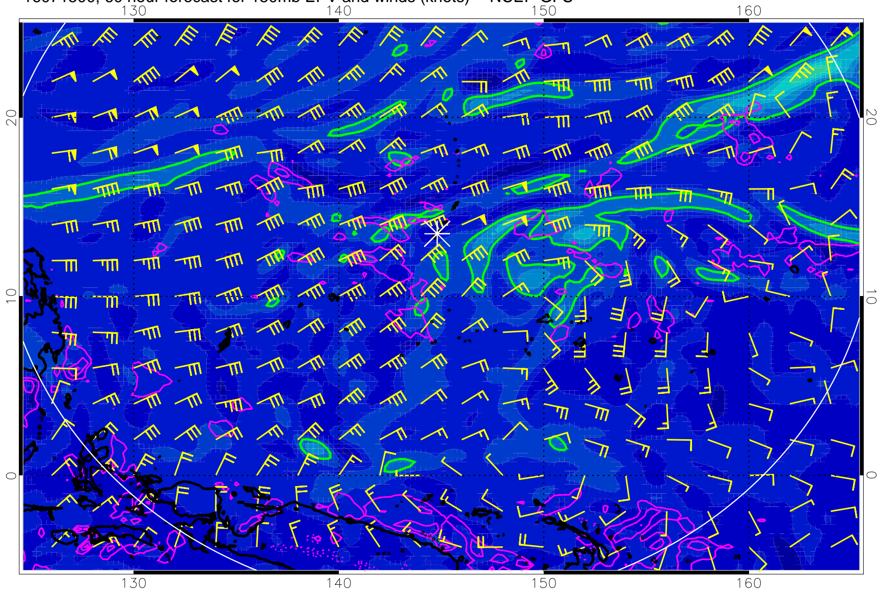
16071500, 60 hour forecast for 150mb EPV and winds (knots) -- NCEP GFS
