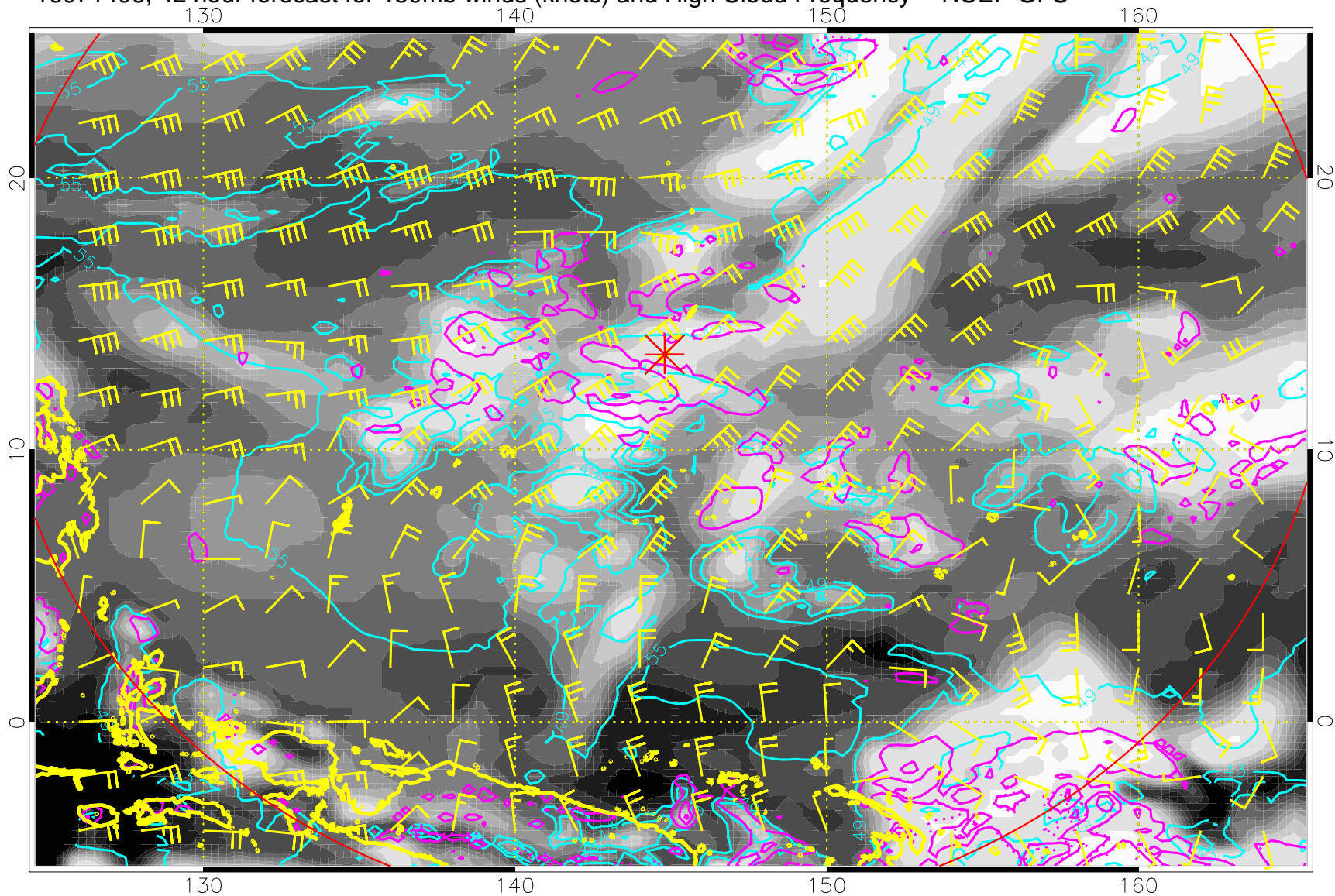
16071406, 42 hour forecast for 150mb winds (knots) and High Cloud Frequency -- NCEP GFS
