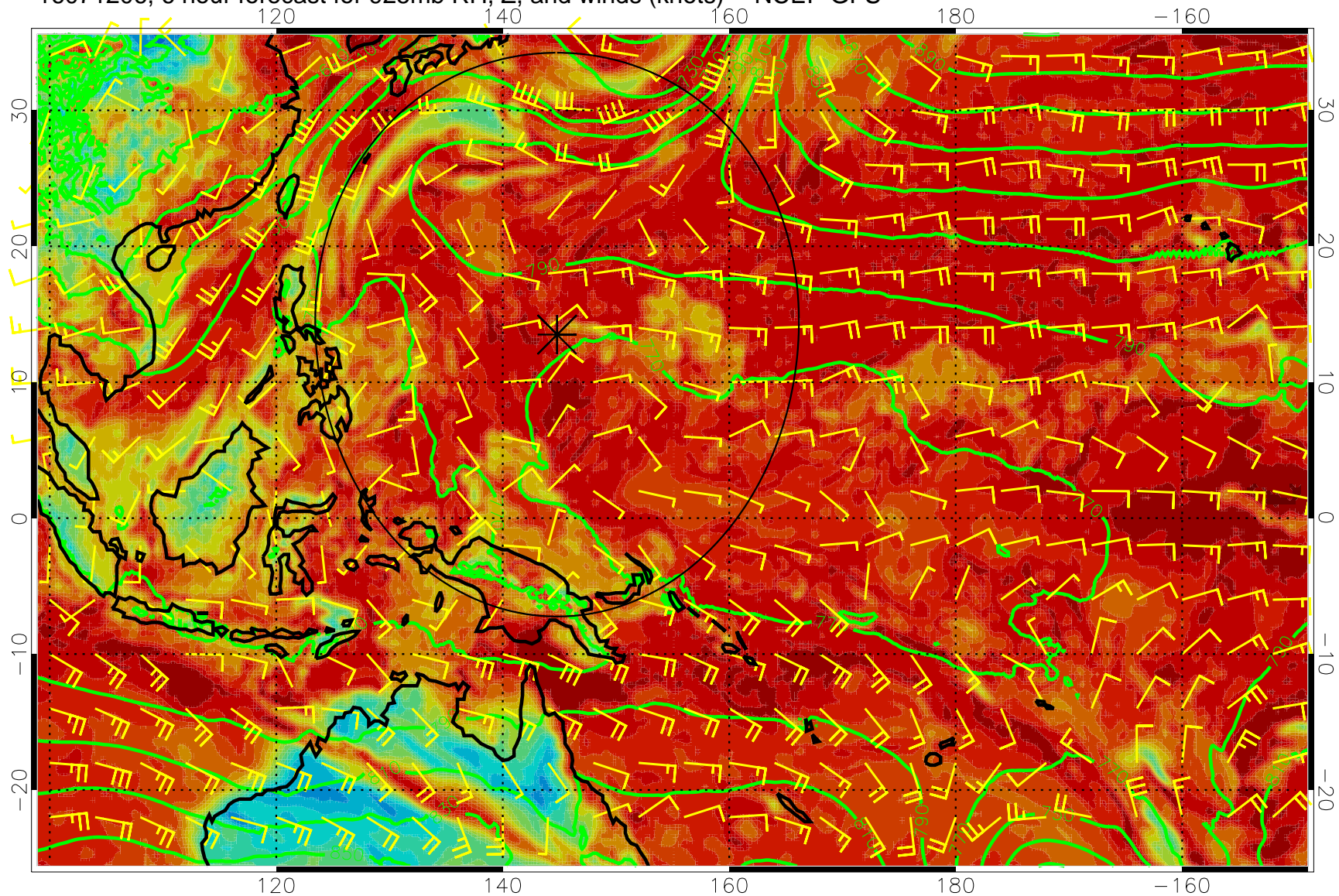
16071206, 6 hour forecast for 925mb RH, Z, and winds (knots) -- NCEP GFS
