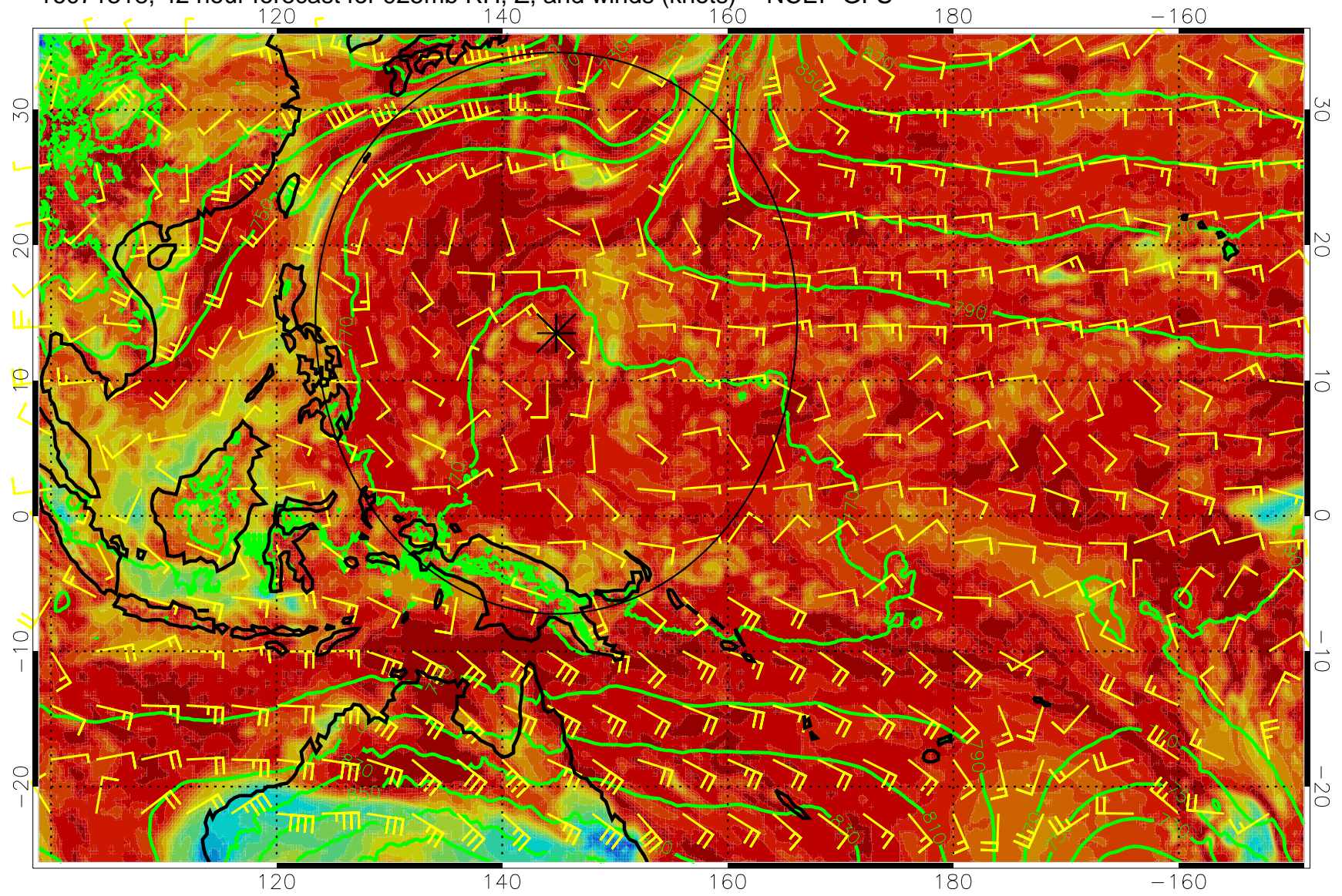
16071318, 42 hour forecast for 925mb RH, Z, and winds (knots) -- NCEP GFS
