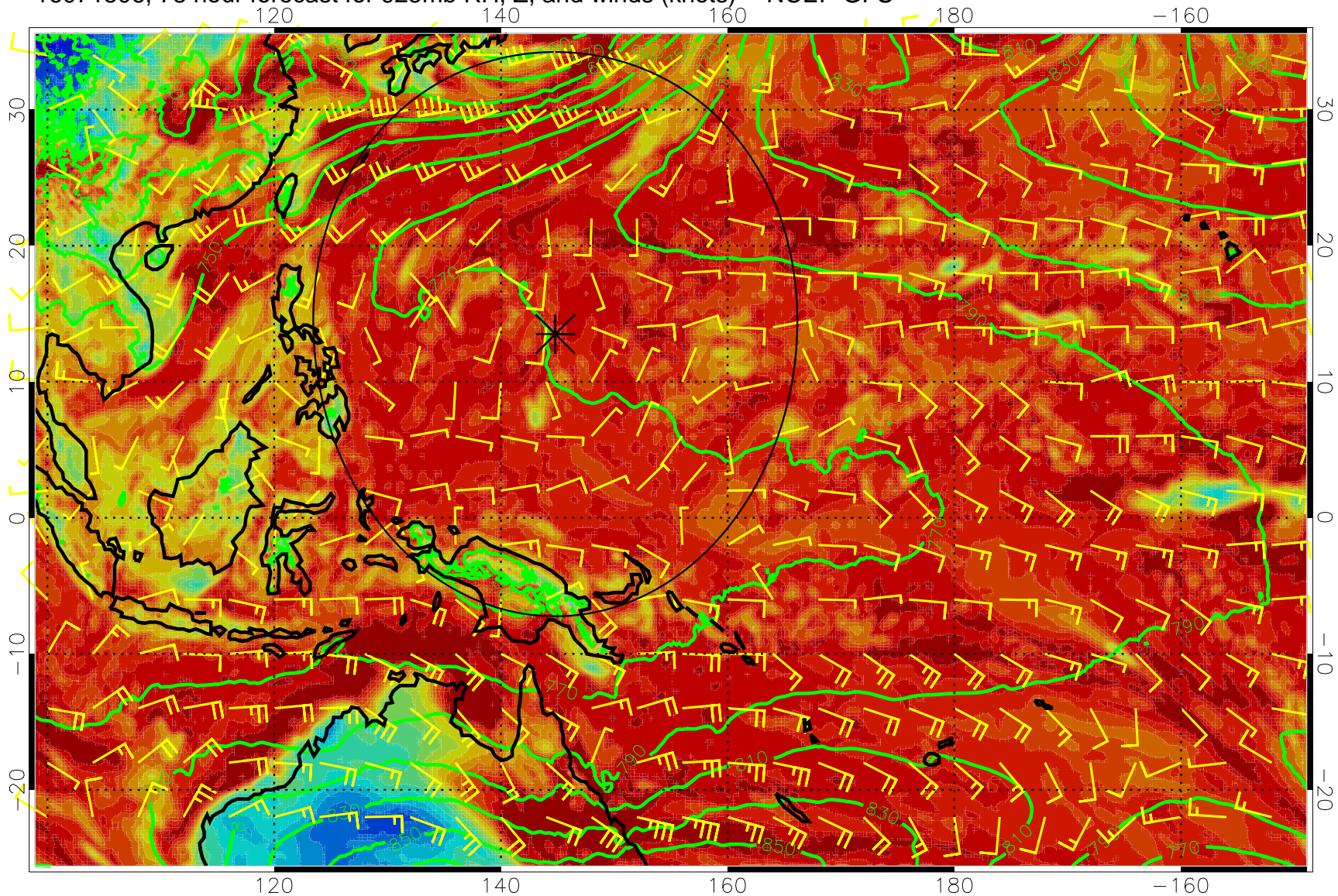
16071506, 78 hour forecast for 925mb RH, Z, and winds (knots) -- NCEP GFS
