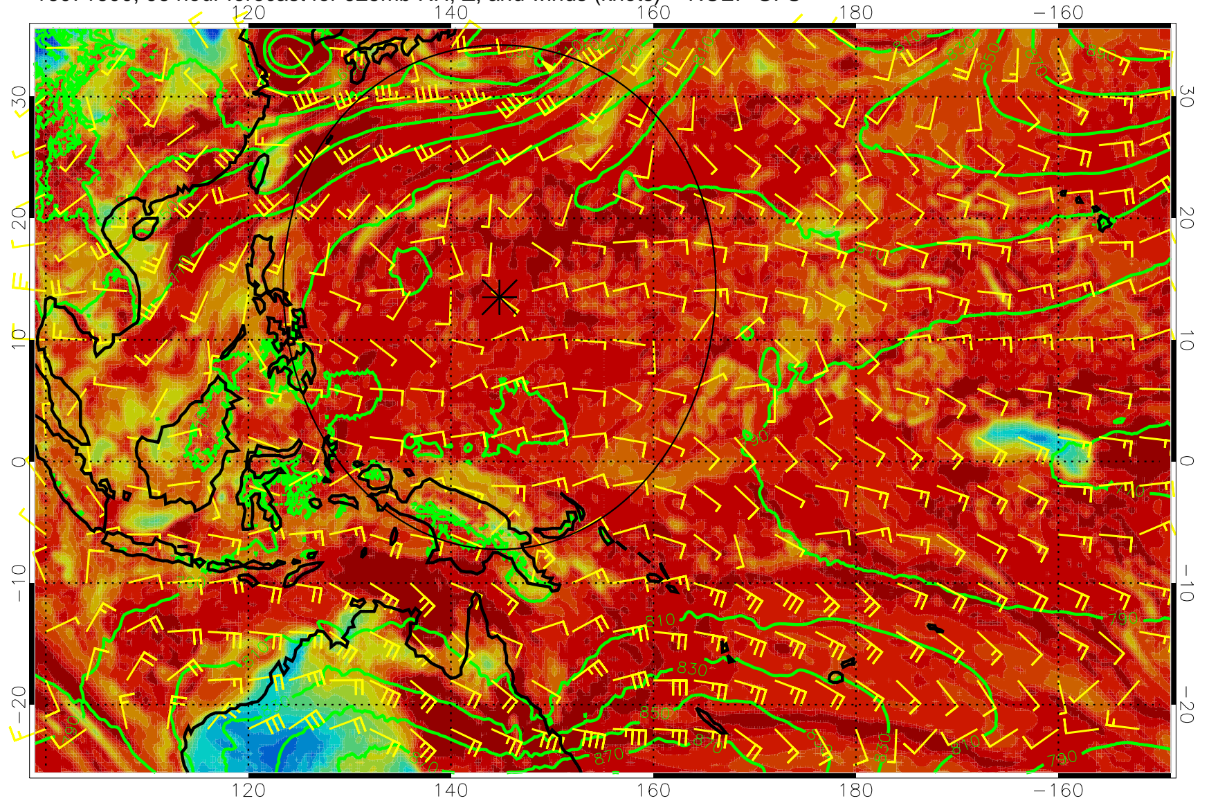
16071600, 96 hour forecast for 925mb RH, Z, and winds (knots) -- NCEP GFS
