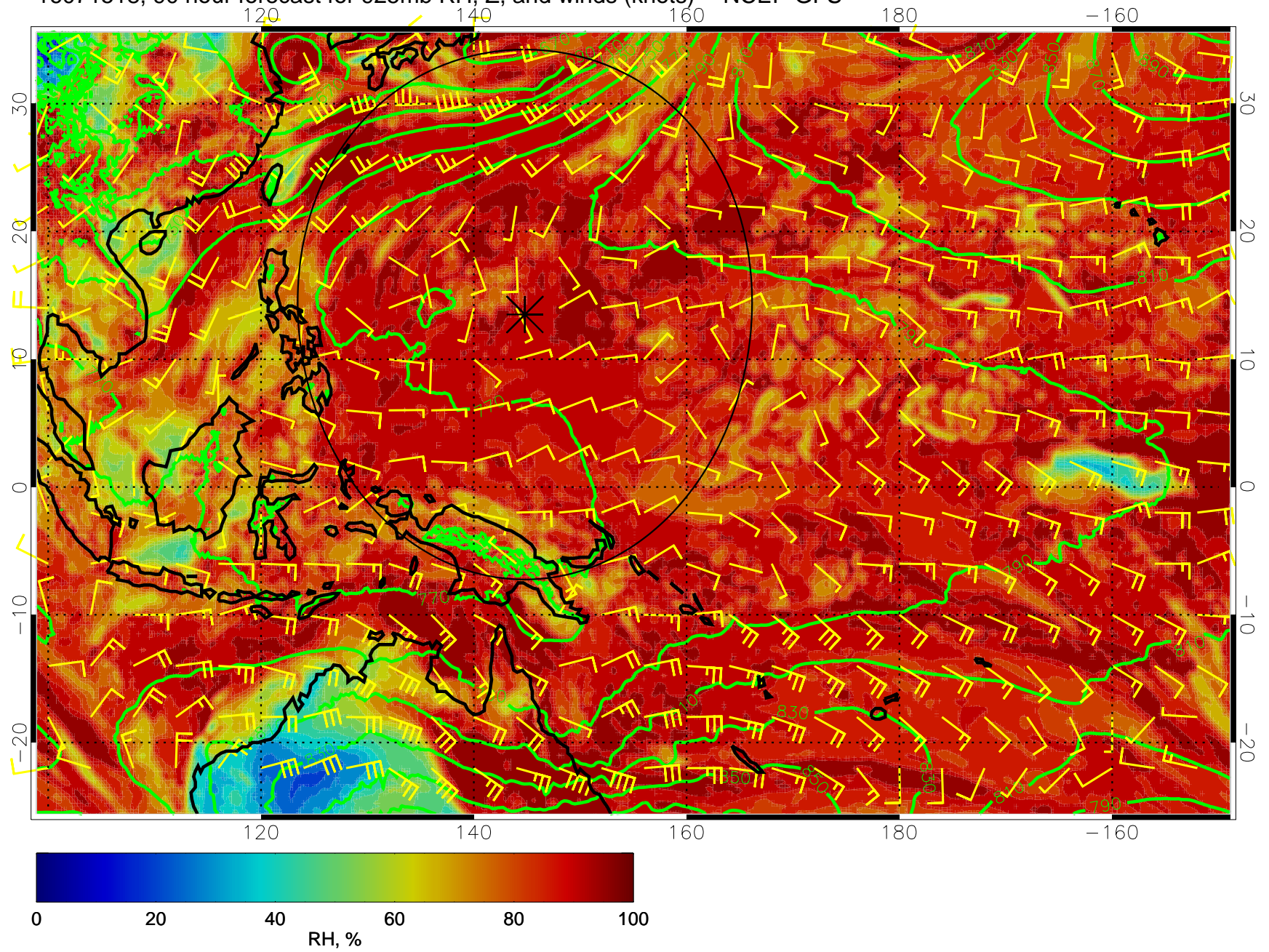
16071518, 90 hour forecast for 925mb RH, Z, and winds (knots) -- NCEP GFS
