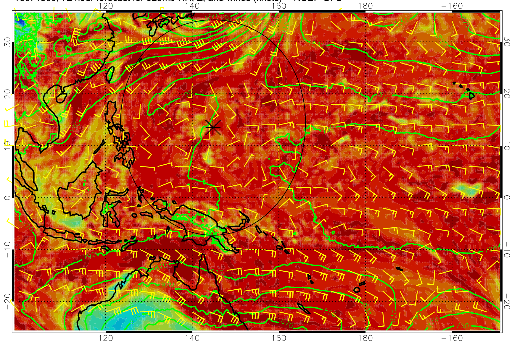
16071500, 72 hour forecast for 925mb RH, Z, and winds (knots) -- NCEP GFS
