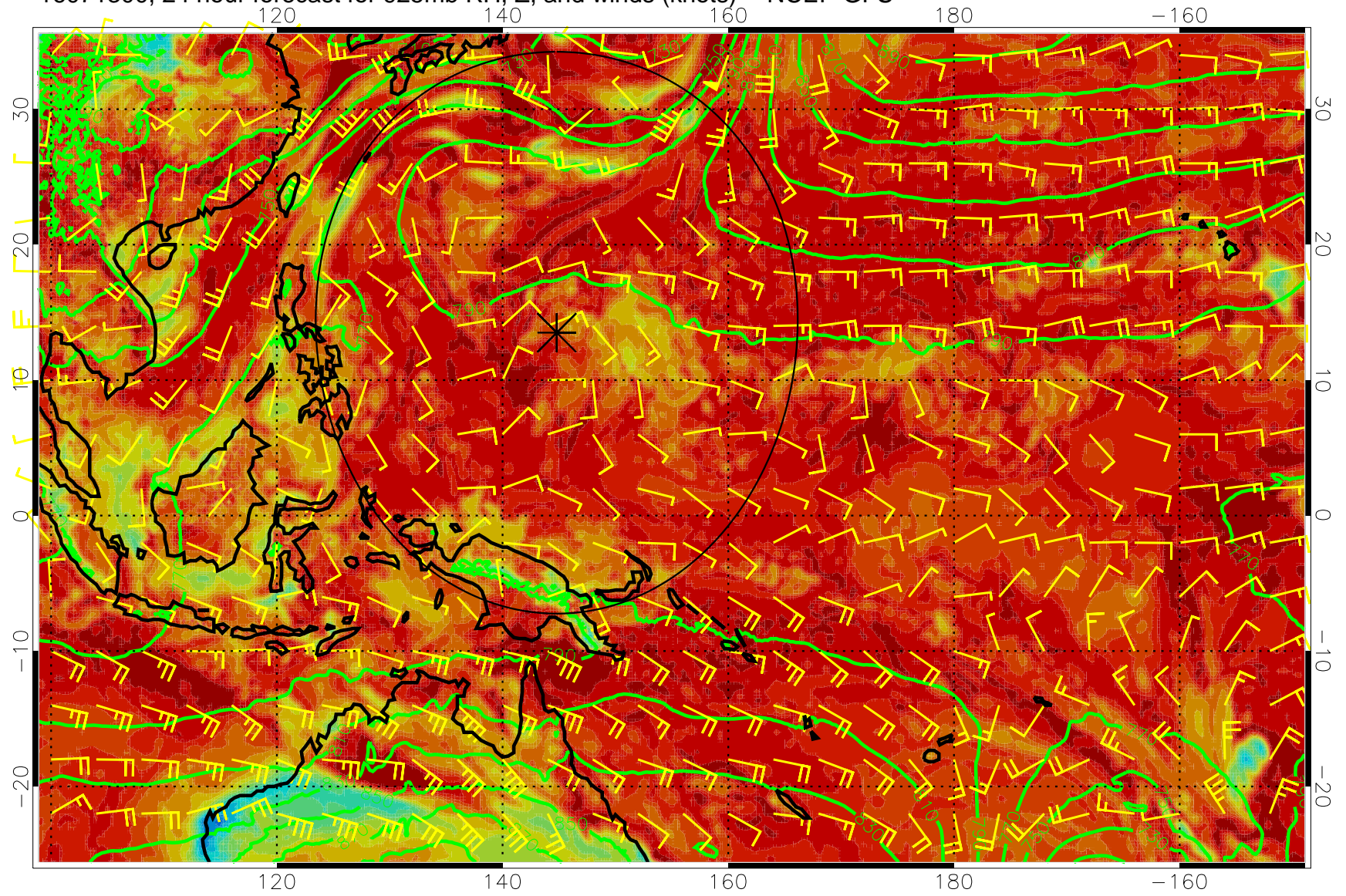
16071300, 24 hour forecast for 925mb RH, Z, and winds (knots) -- NCEP GFS
