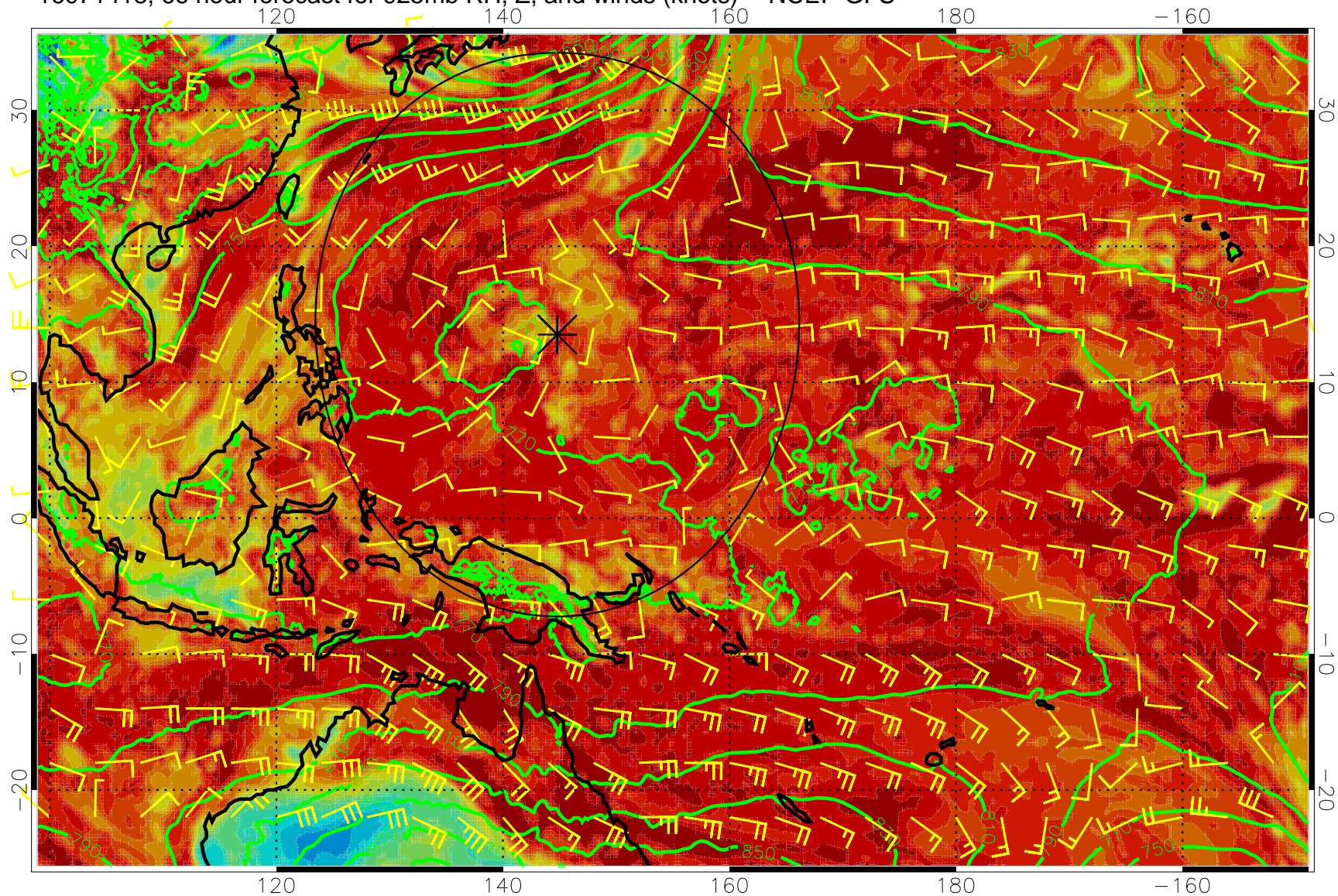
16071418, 66 hour forecast for 925mb RH, Z, and winds (knots) -- NCEP GFS
