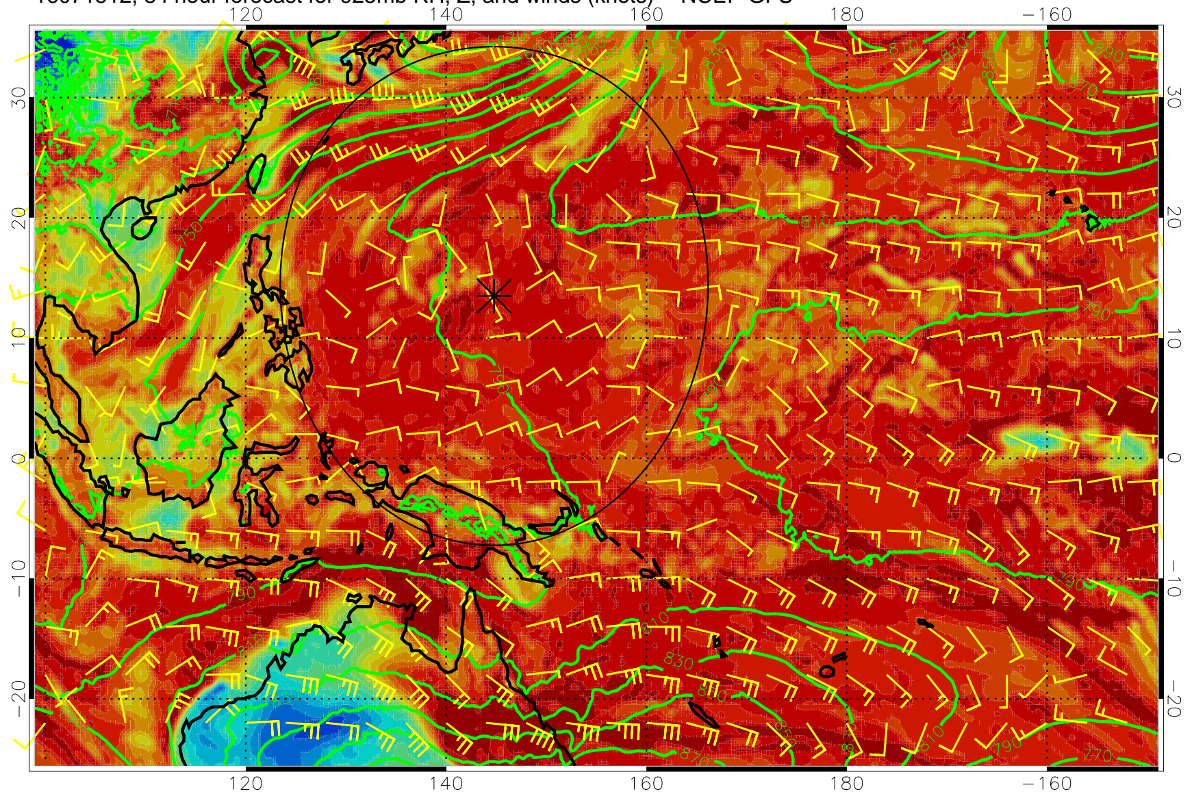
16071512, 84 hour forecast for 925mb RH, Z, and winds (knots) -- NCEP GFS
