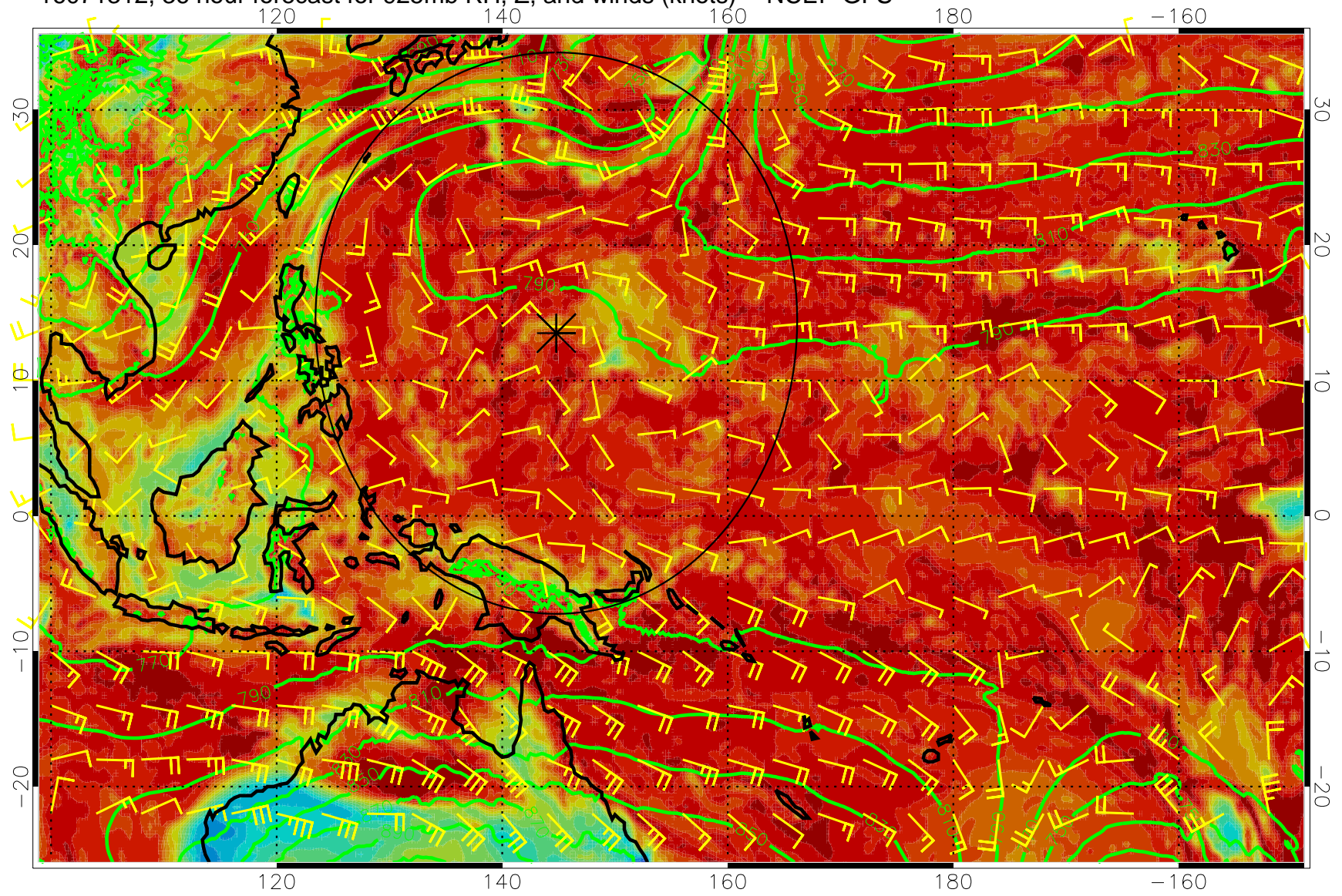
16071312, 36 hour forecast for 925mb RH, Z, and winds (knots) -- NCEP GFS
