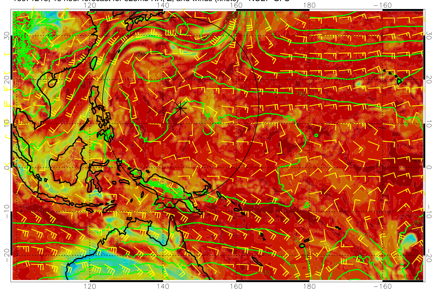
16071218, 18 hour forecast for 925mb RH, Z, and winds (knots) -- NCEP GFS
