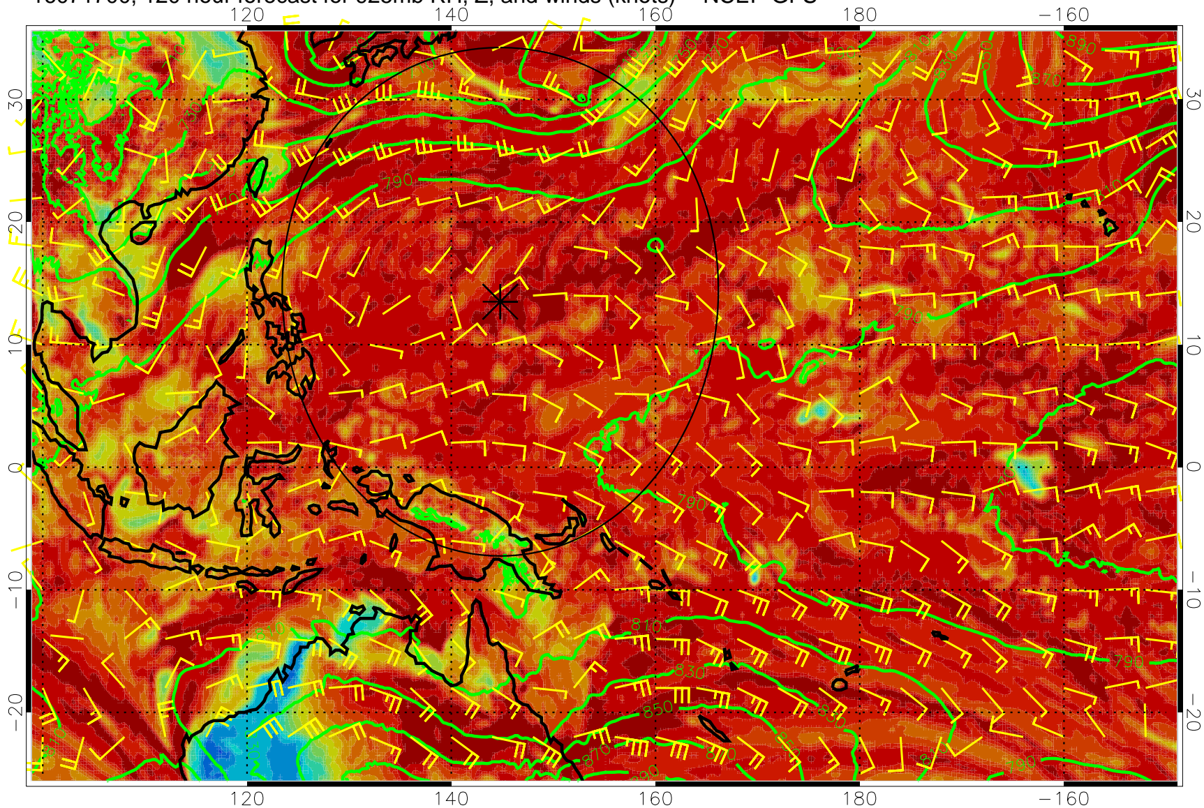
16071700, 120 hour forecast for 925mb RH, Z, and winds (knots) -- NCEP GFS
