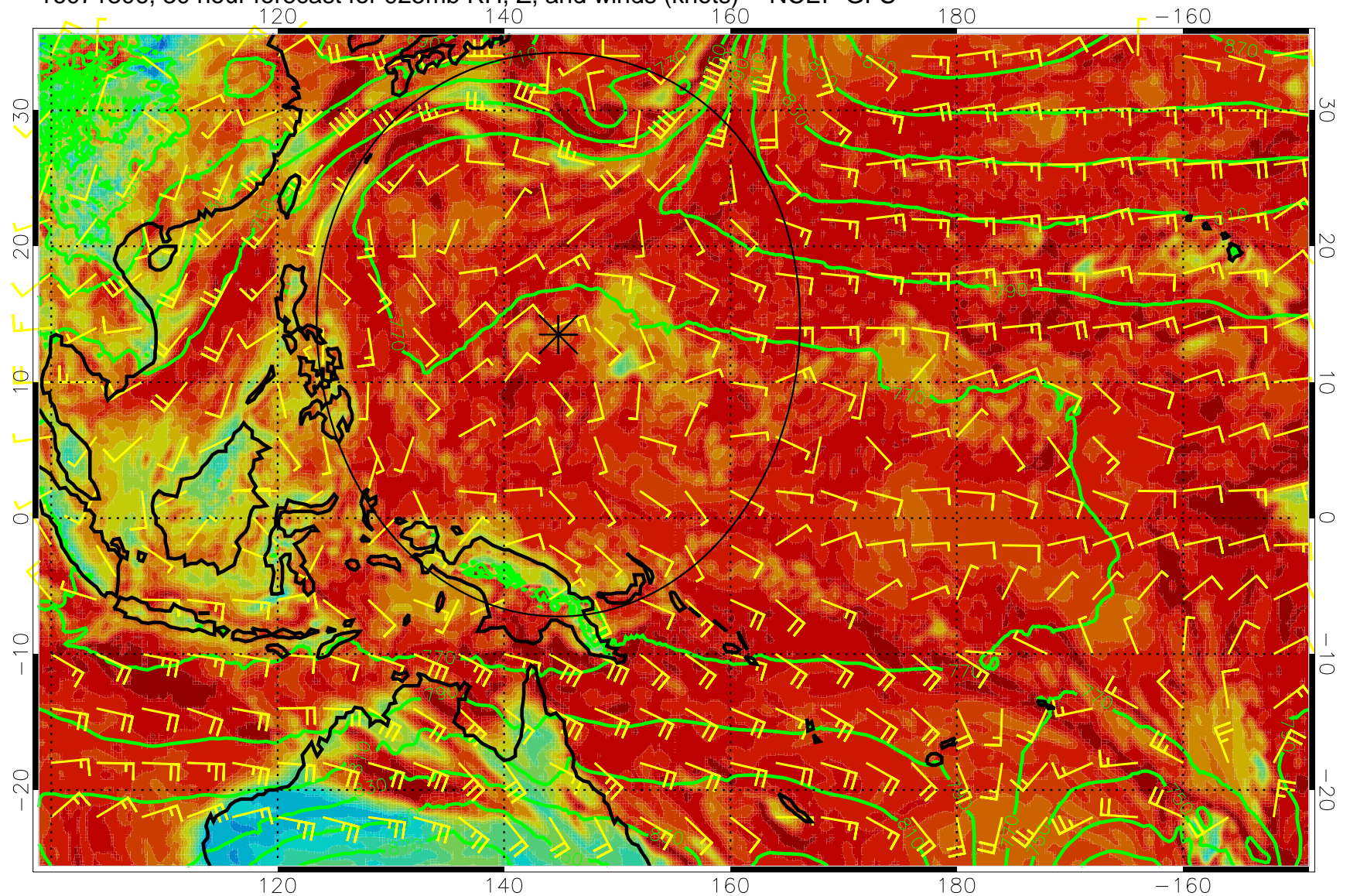
16071306, 30 hour forecast for 925mb RH, Z, and winds (knots) -- NCEP GFS
