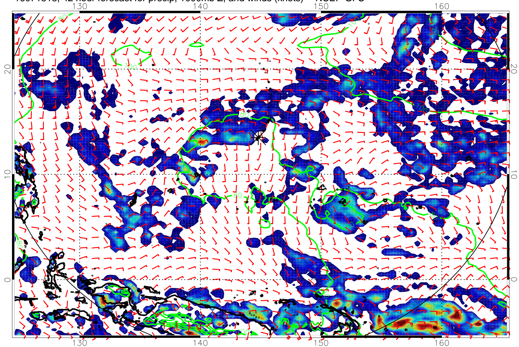
16071318, 42 hour forecast for precip, 1000mb Z, and winds (knots) -- NCEP GFS
