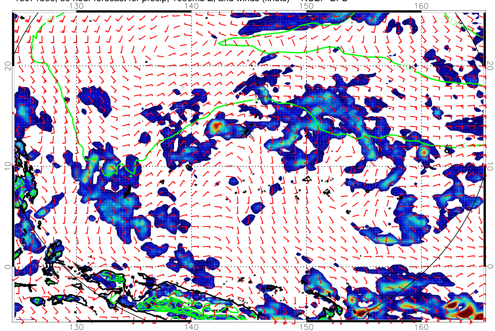
16071306, 30 hour forecast for precip, 1000mb Z, and winds (knots) -- NCEP GFS
