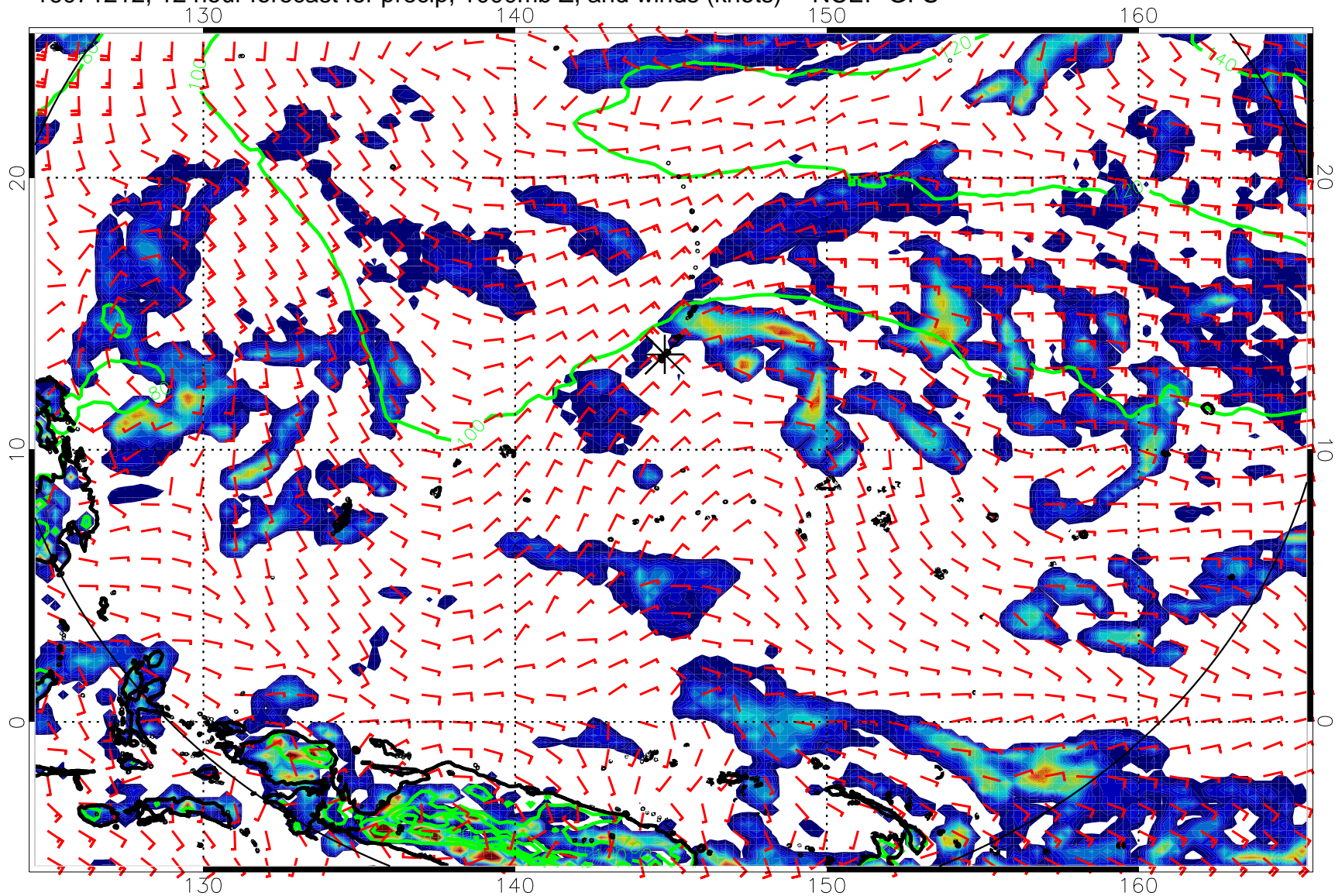
16071212, 12 hour forecast for precip, 1000mb Z, and winds (knots) -- NCEP GFS
