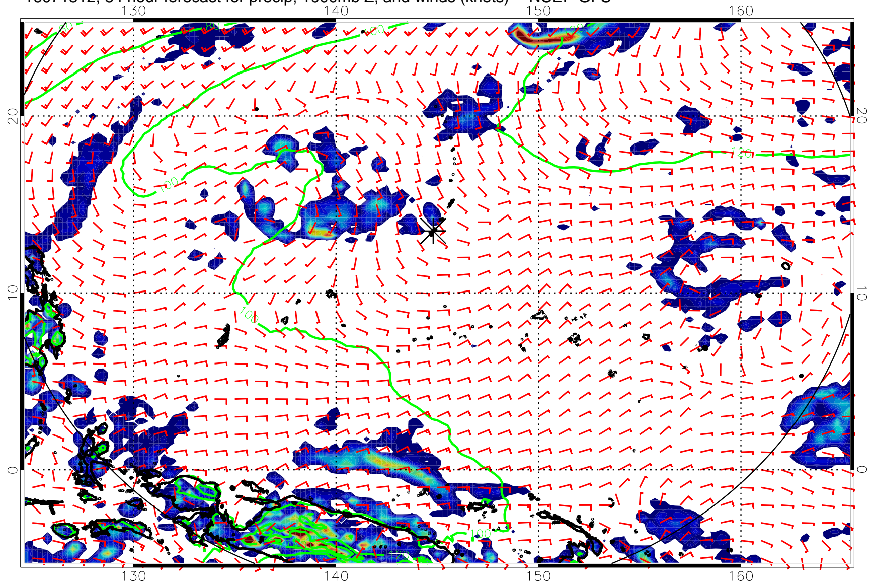
16071512, 84 hour forecast for precip, 1000mb Z, and winds (knots) -- NCEP GFS
