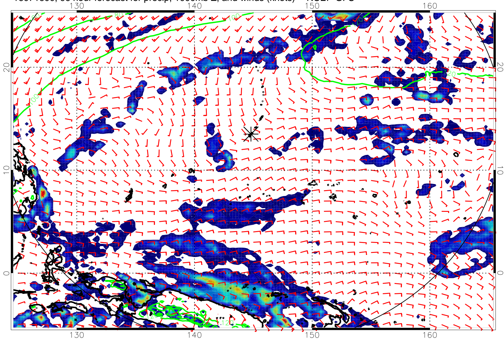
16071600, 96 hour forecast for precip, 1000mb Z, and winds (knots) -- NCEP GFS
