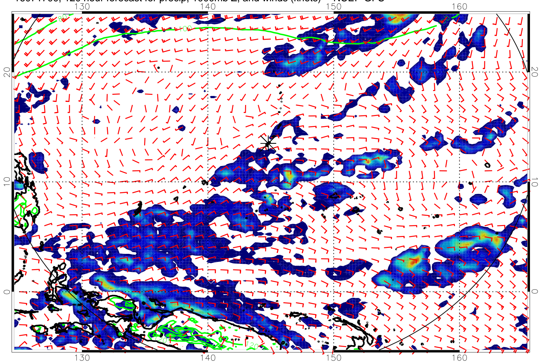
16071700, 120 hour forecast for precip, 1000mb Z, and winds (knots) -- NCEP GFS
