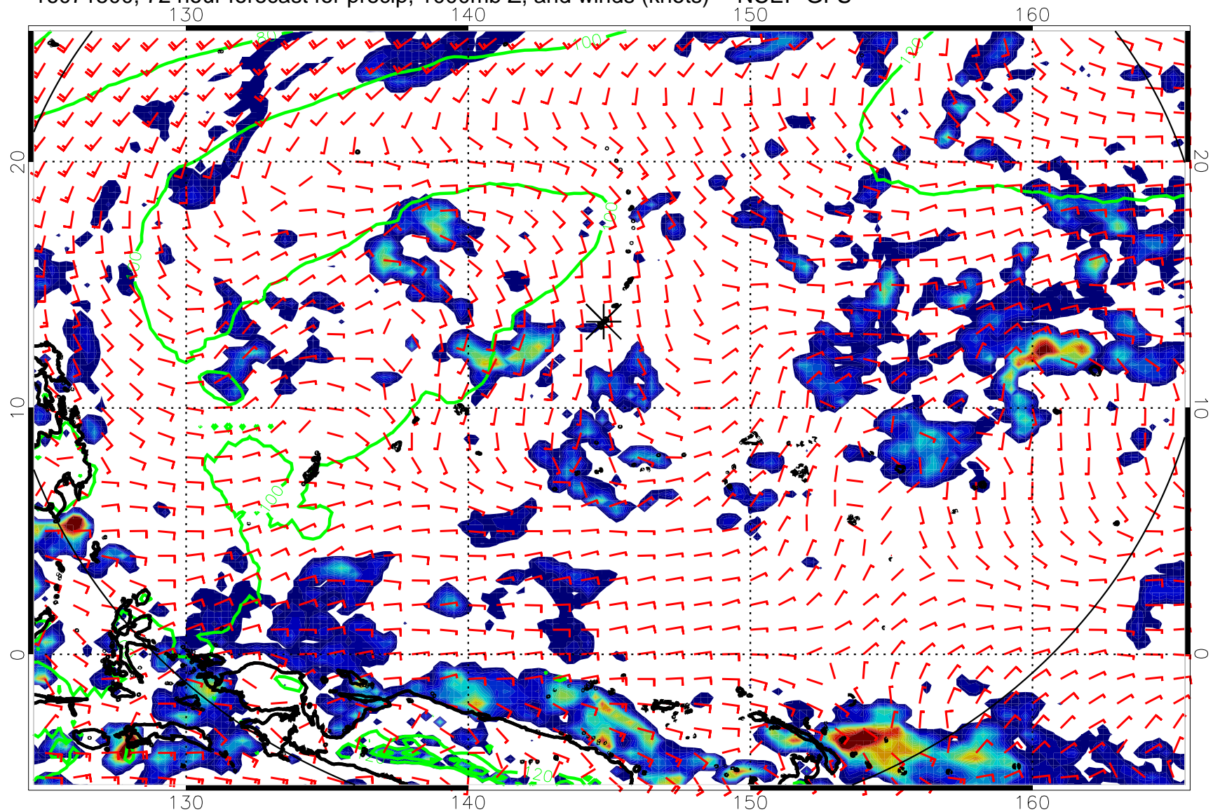
16071500, 72 hour forecast for precip, 1000mb Z, and winds (knots) -- NCEP GFS
