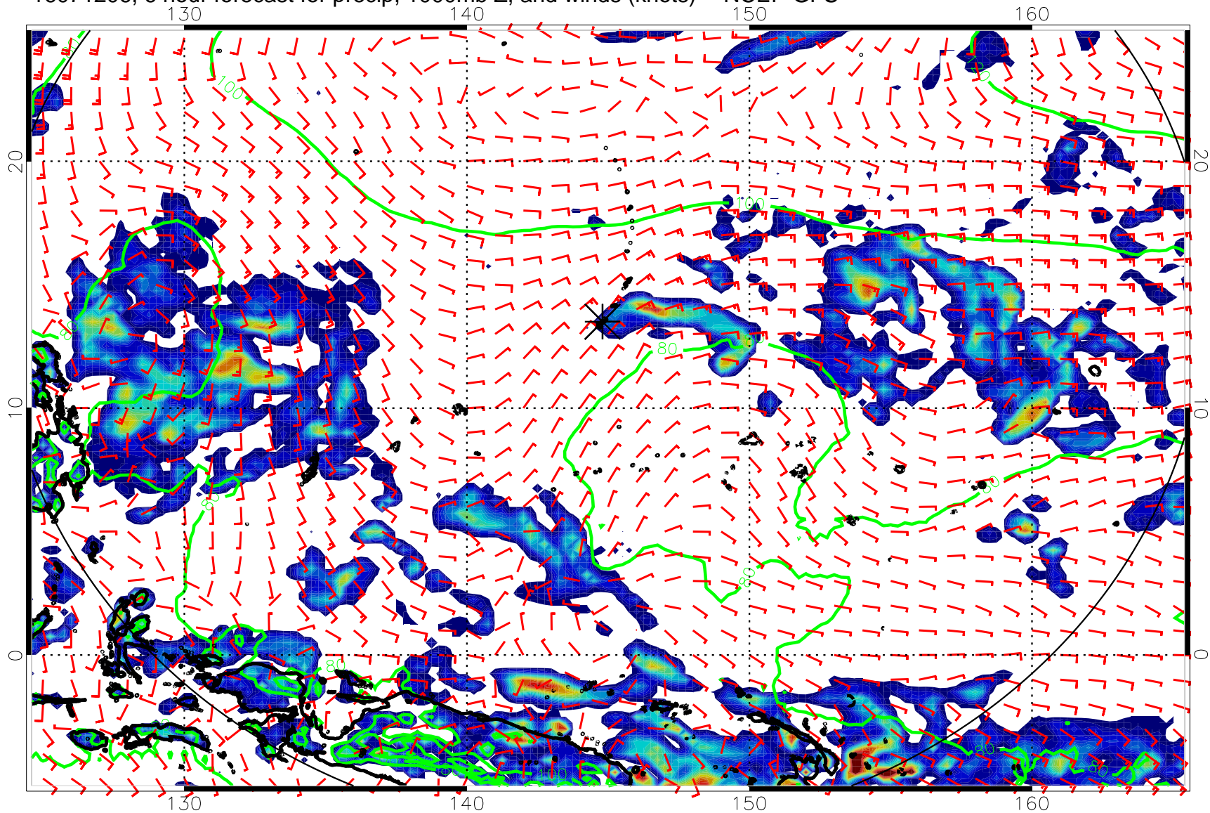
16071206, 6 hour forecast for precip, 1000mb Z, and winds (knots) -- NCEP GFS
