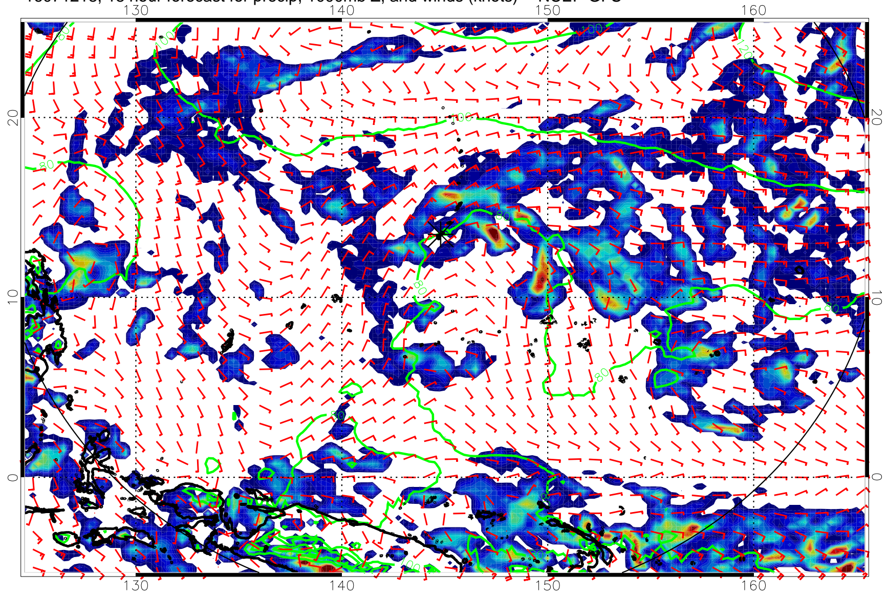
16071218, 18 hour forecast for precip, 1000mb Z, and winds (knots) -- NCEP GFS
