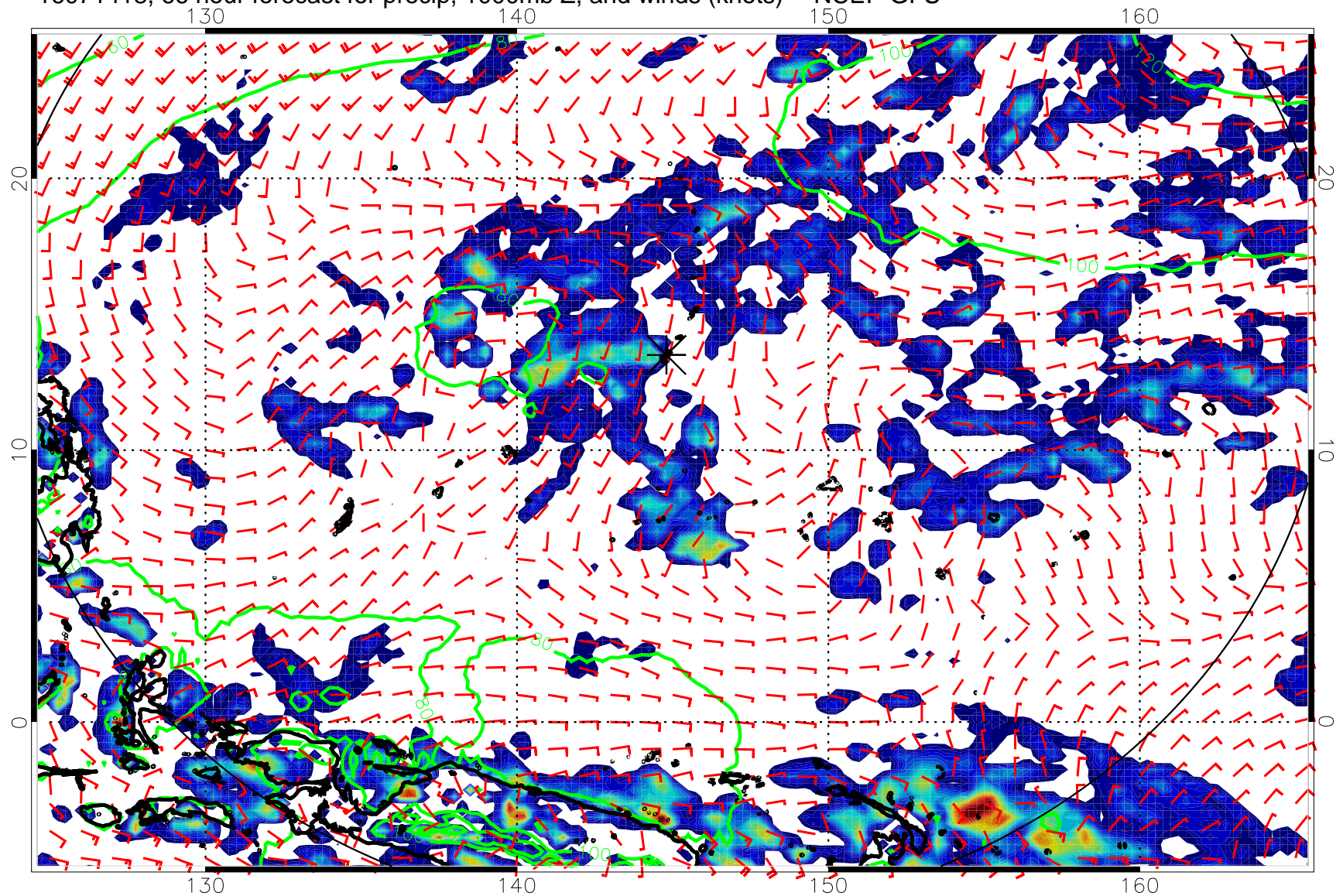
16071418, 66 hour forecast for precip, 1000mb Z, and winds (knots) -- NCEP GFS
