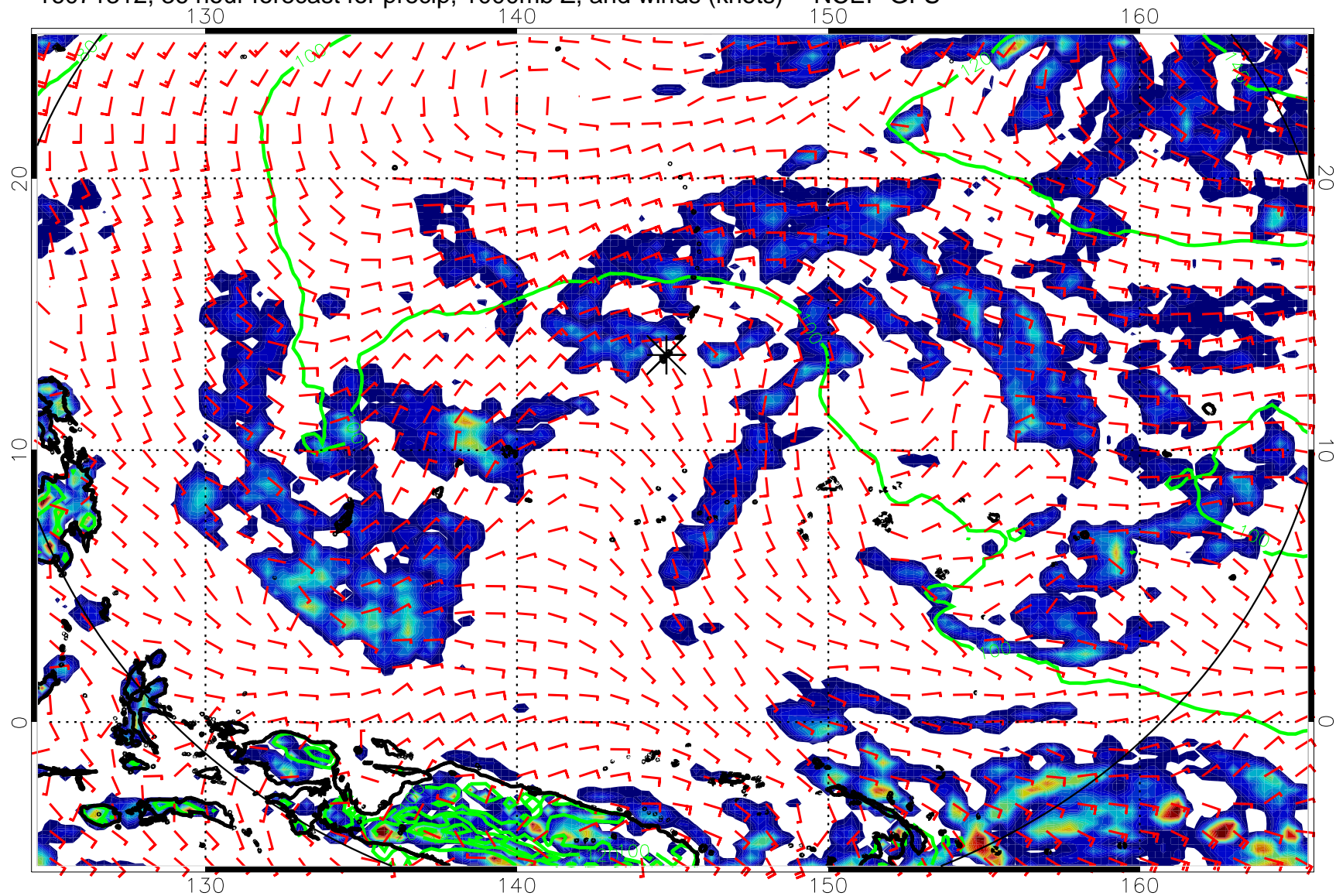
16071312, 36 hour forecast for precip, 1000mb Z, and winds (knots) -- NCEP GFS
