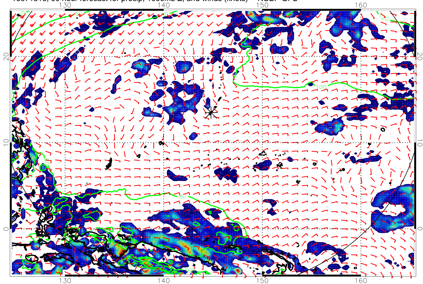
16071518, 90 hour forecast for precip, 1000mb Z, and winds (knots) -- NCEP GFS
