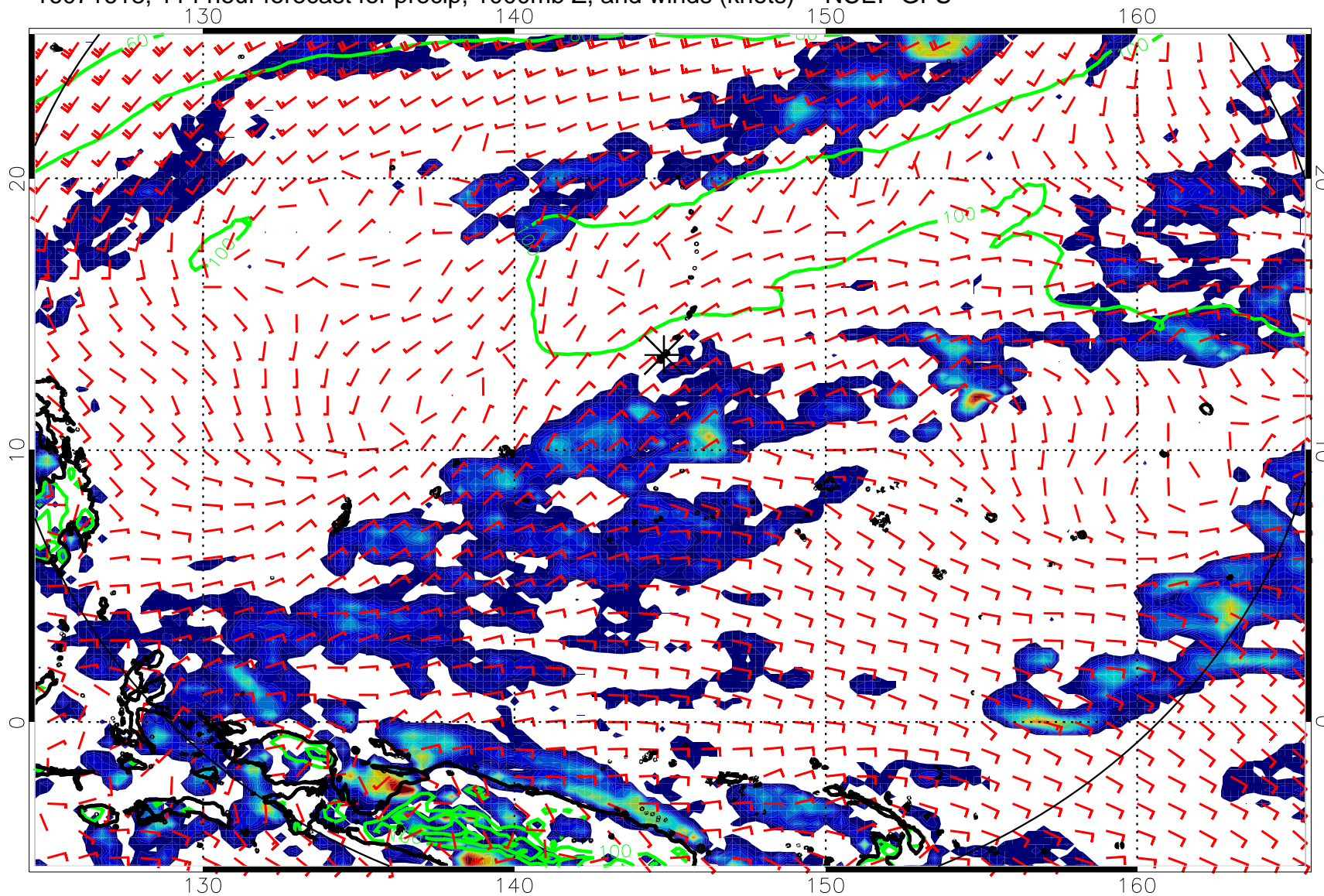
16071618, 114 hour forecast for precip, 1000mb Z, and winds (knots) -- NCEP GFS
