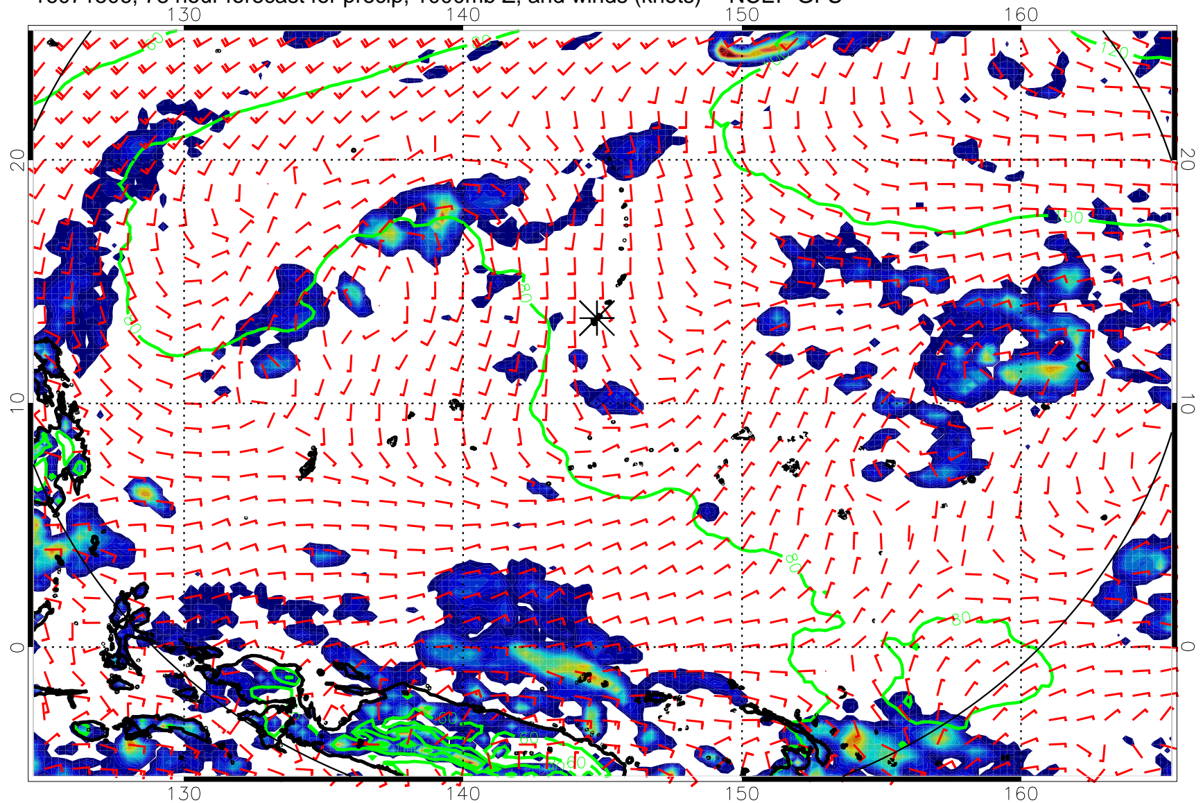
16071506, 78 hour forecast for precip, 1000mb Z, and winds (knots) -- NCEP GFS
