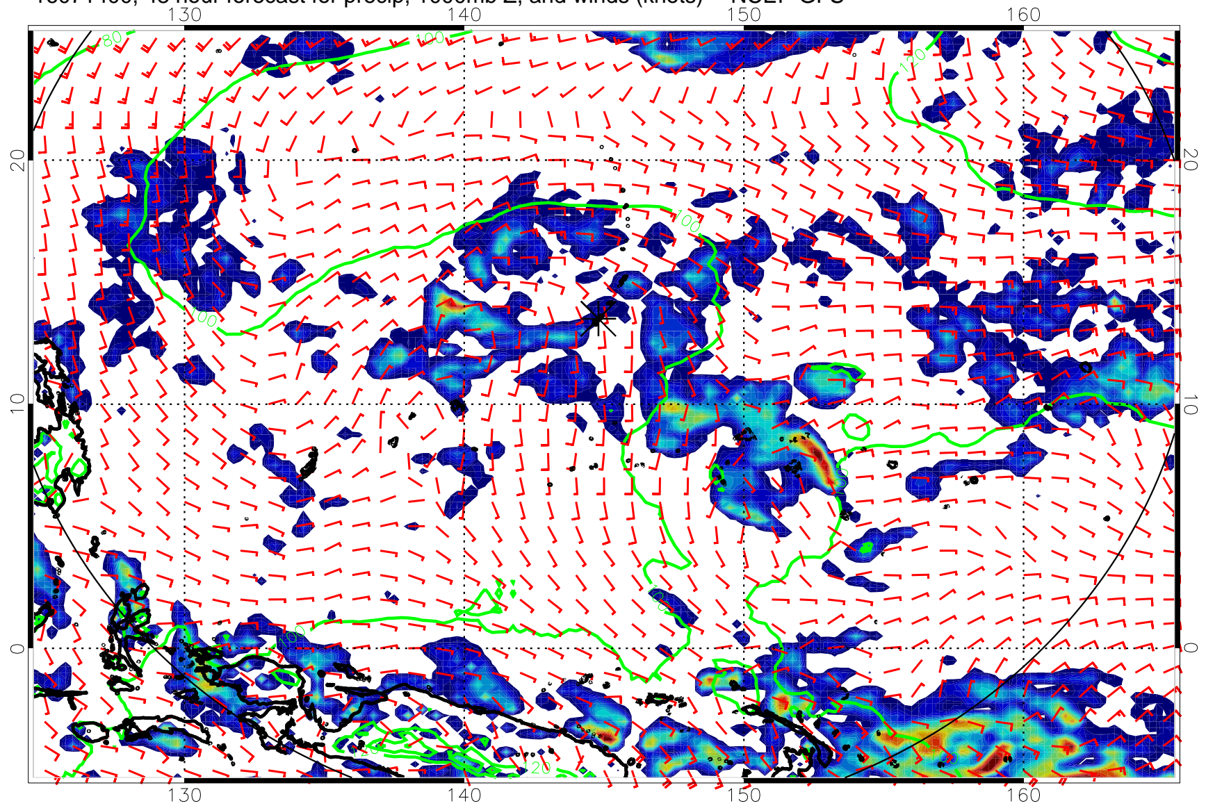
16071400, 48 hour forecast for precip, 1000mb Z, and winds (knots) -- NCEP GFS
