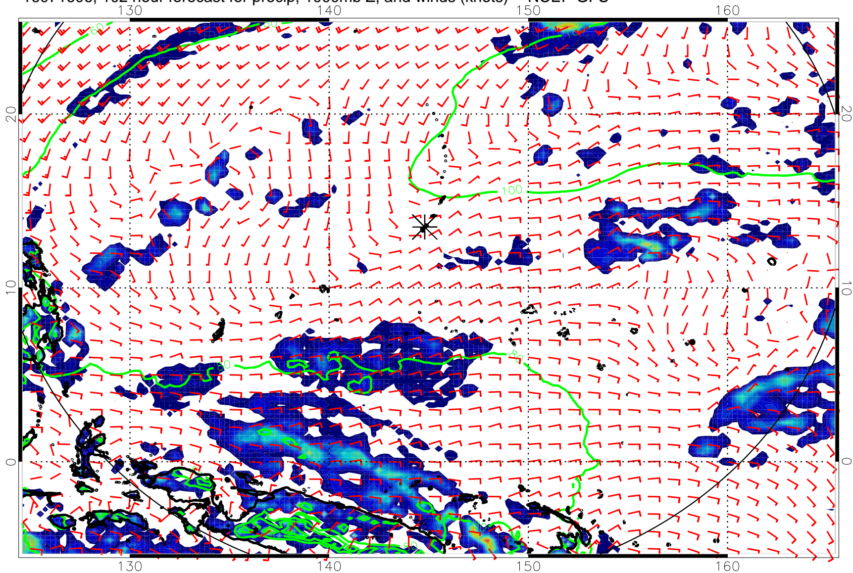
16071606, 102 hour forecast for precip, 1000mb Z, and winds (knots) -- NCEP GFS
