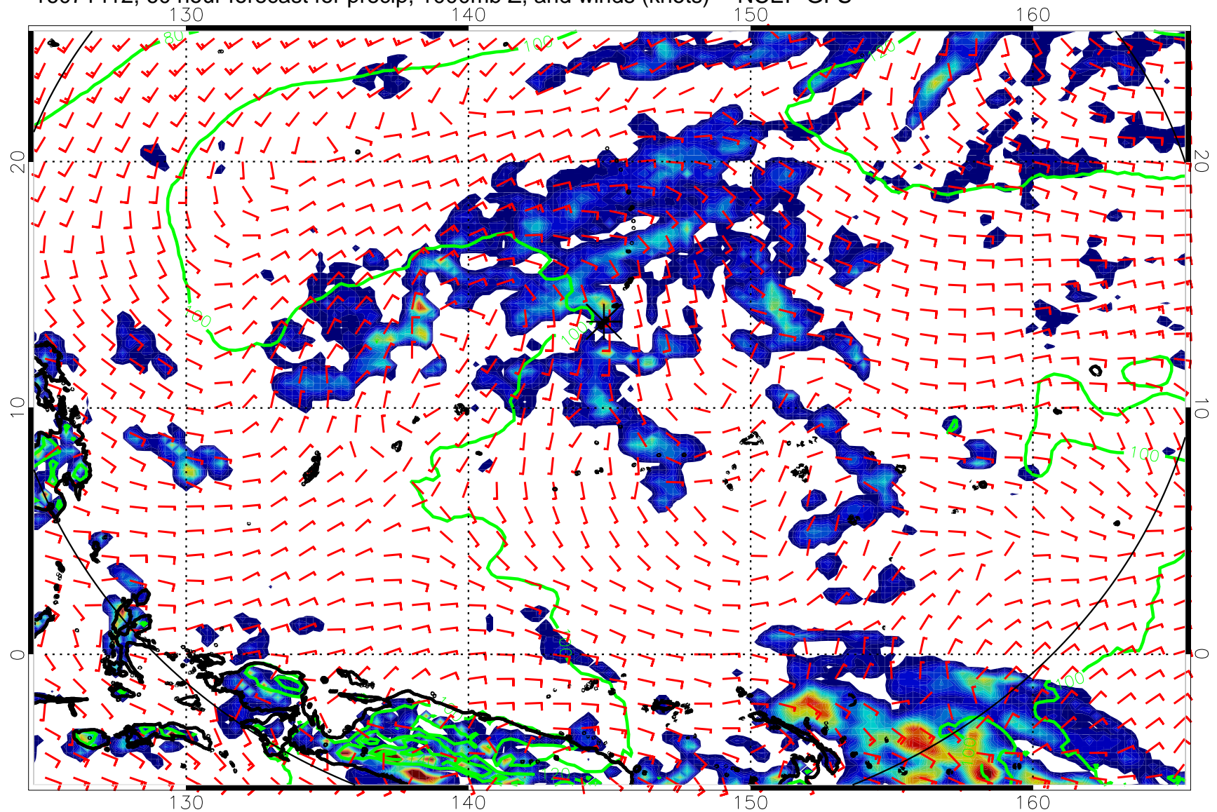
16071412, 60 hour forecast for precip, 1000mb Z, and winds (knots) -- NCEP GFS
