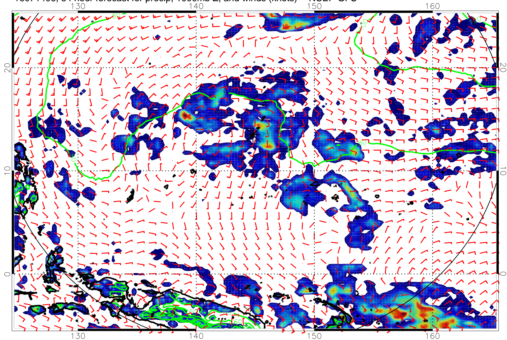
16071406, 54 hour forecast for precip, 1000mb Z, and winds (knots) -- NCEP GFS
