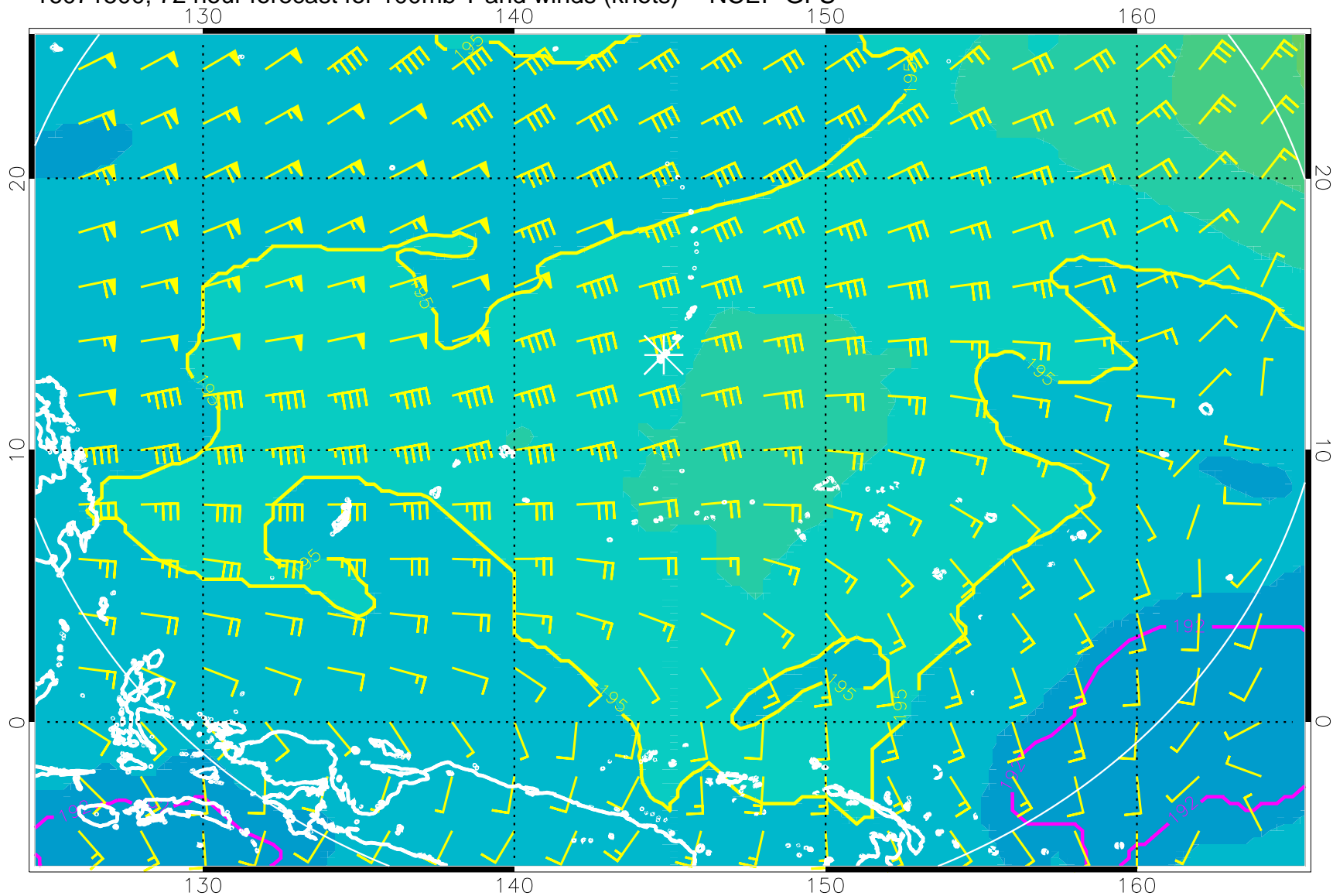
16071500, 72 hour forecast for 100mb T and winds (knots) -- NCEP GFS
