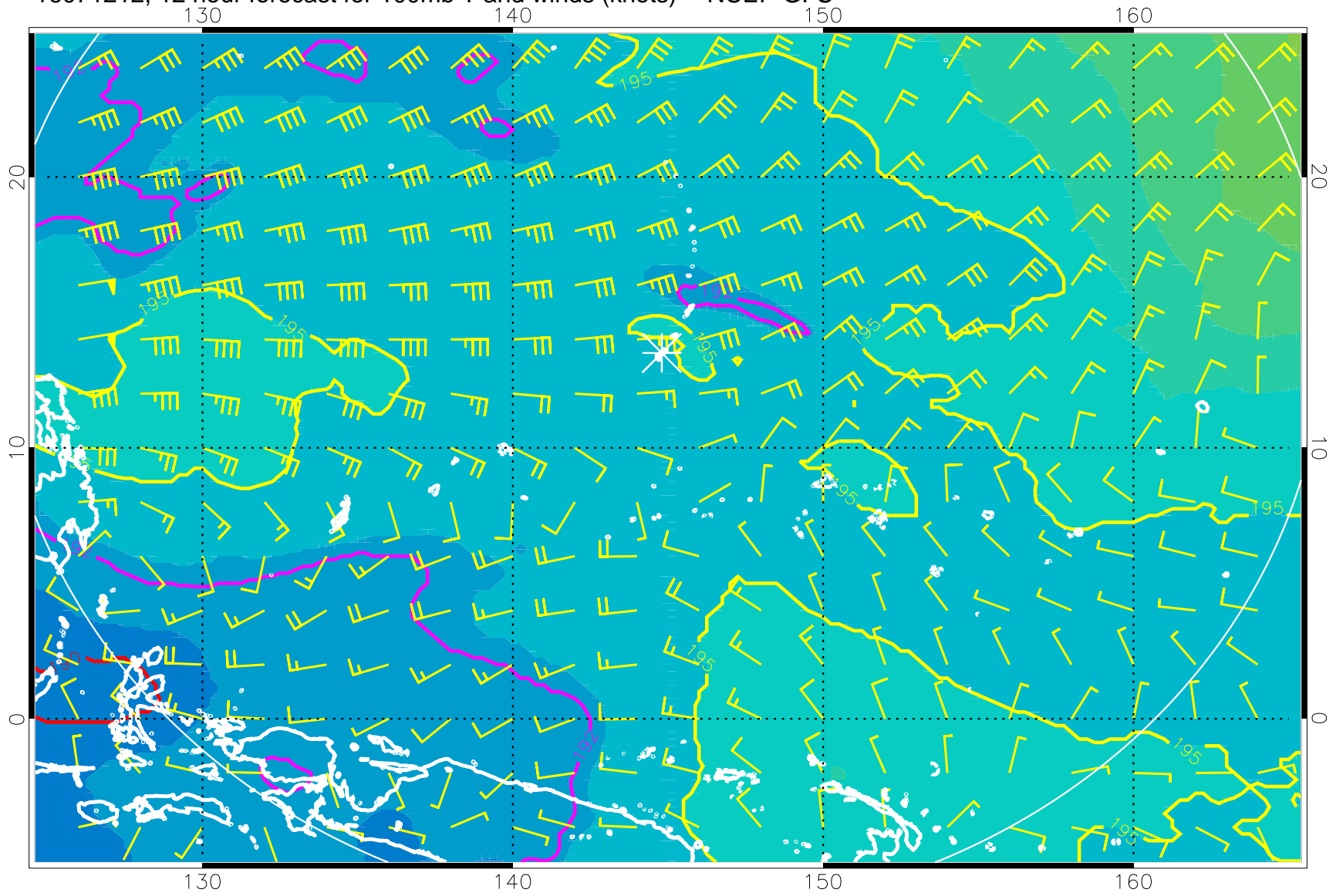
16071212, 12 hour forecast for 100mb T and winds (knots) -- NCEP GFS
