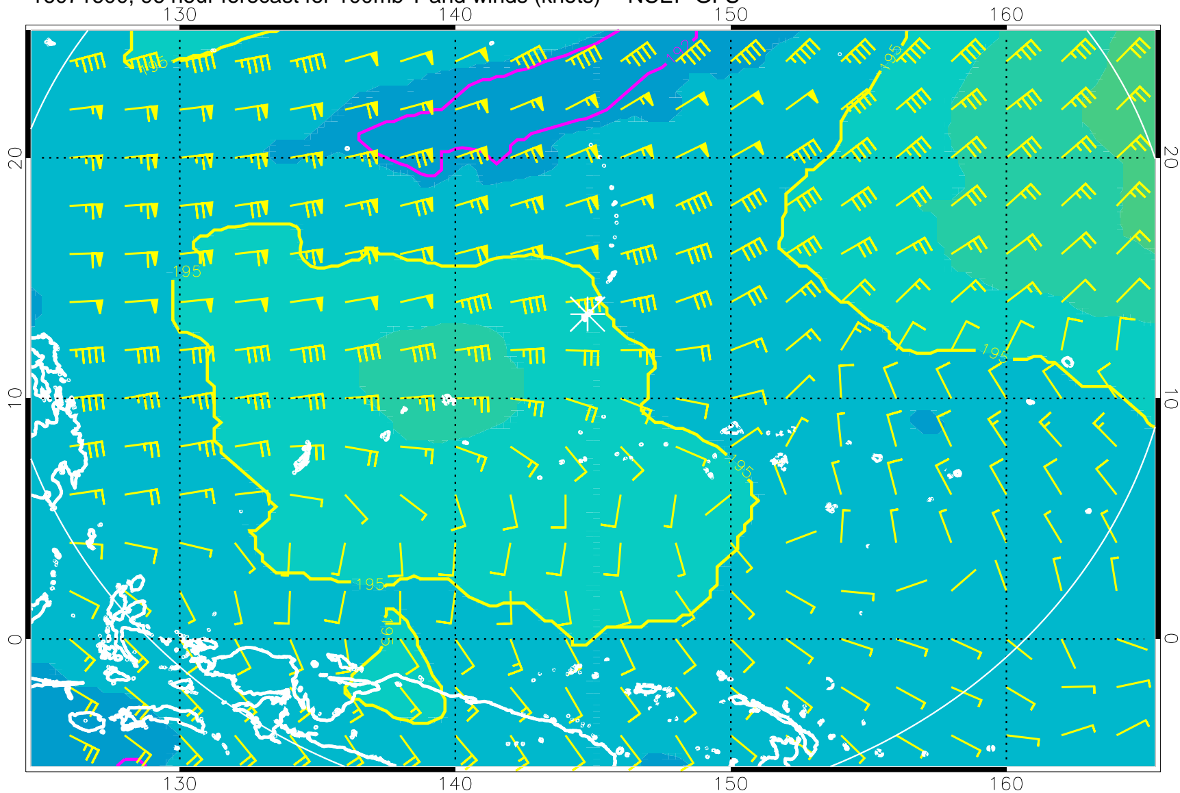
16071600, 96 hour forecast for 100mb T and winds (knots) -- NCEP GFS
