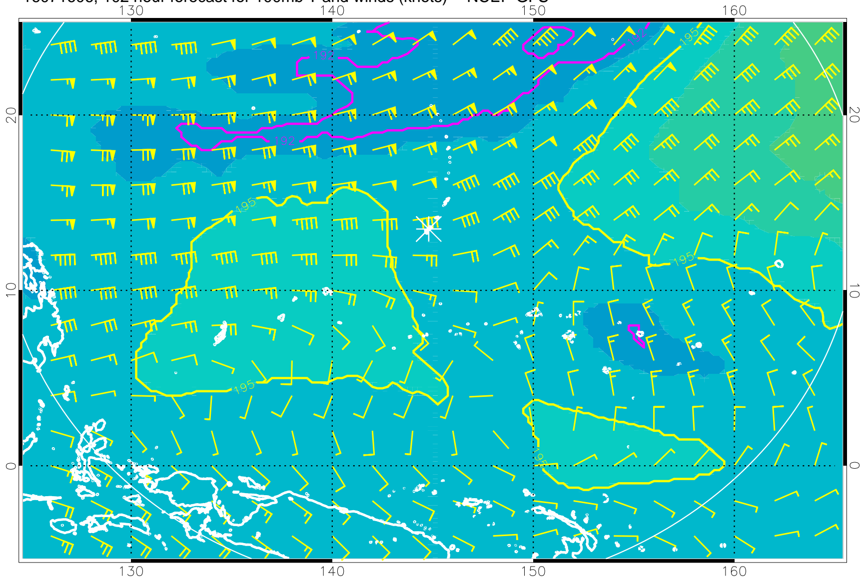
16071606, 102 hour forecast for 100mb T and winds (knots) -- NCEP GFS
