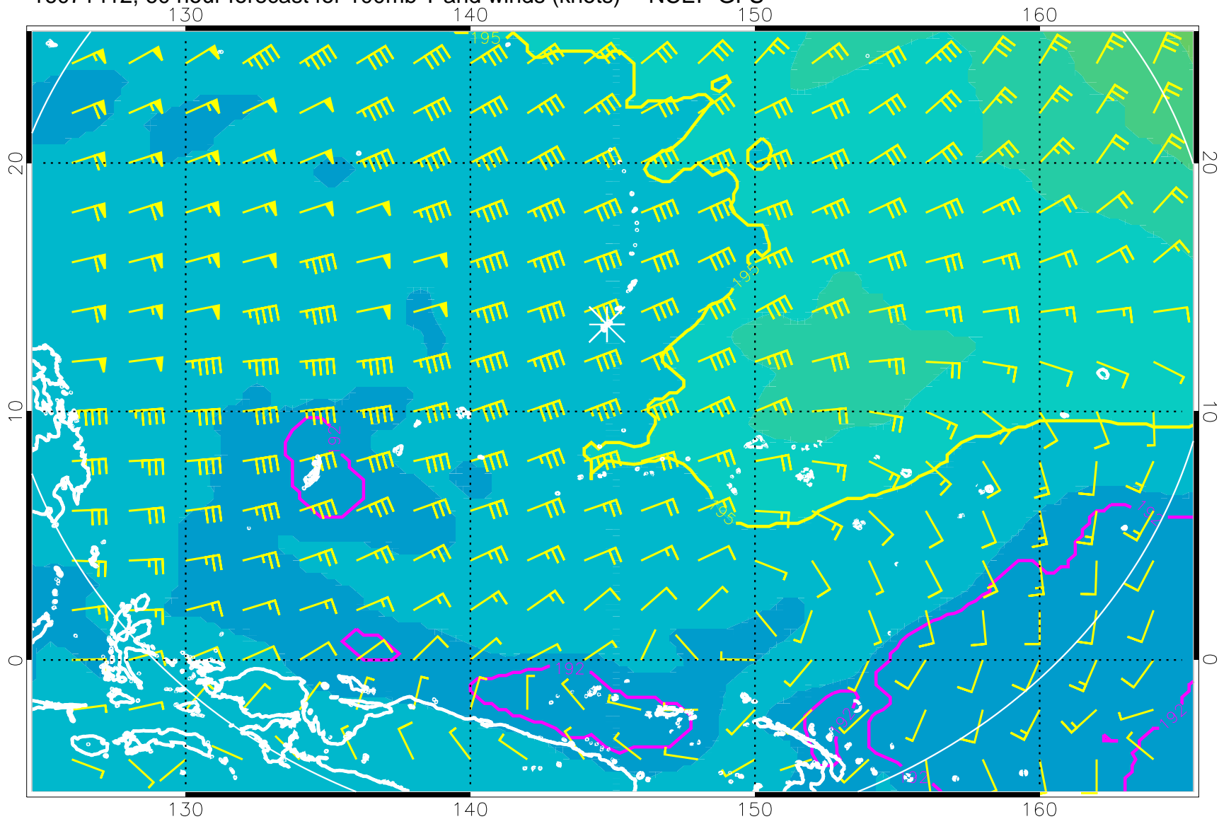
16071412, 60 hour forecast for 100mb T and winds (knots) -- NCEP GFS
