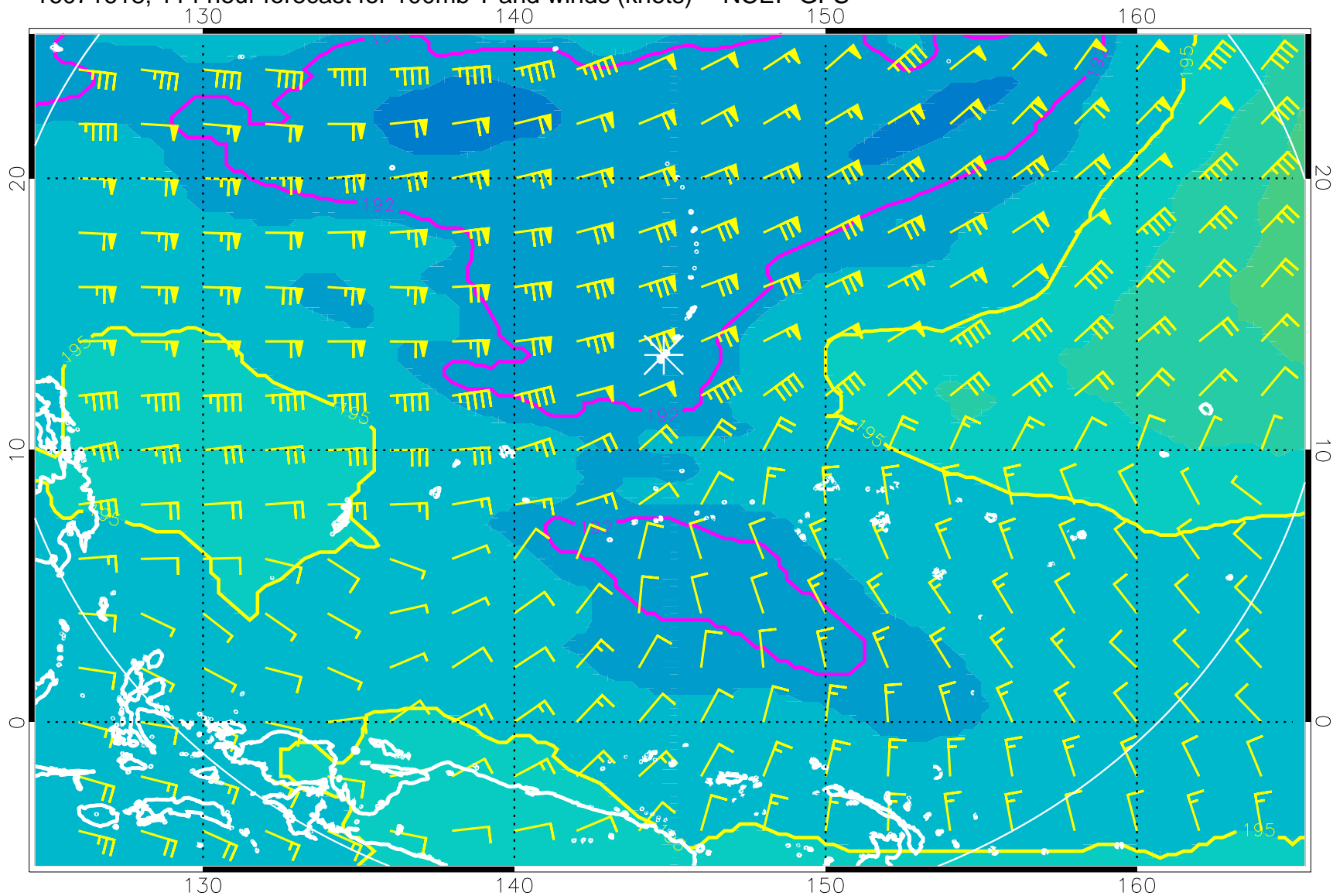
16071618, 114 hour forecast for 100mb T and winds (knots) -- NCEP GFS
