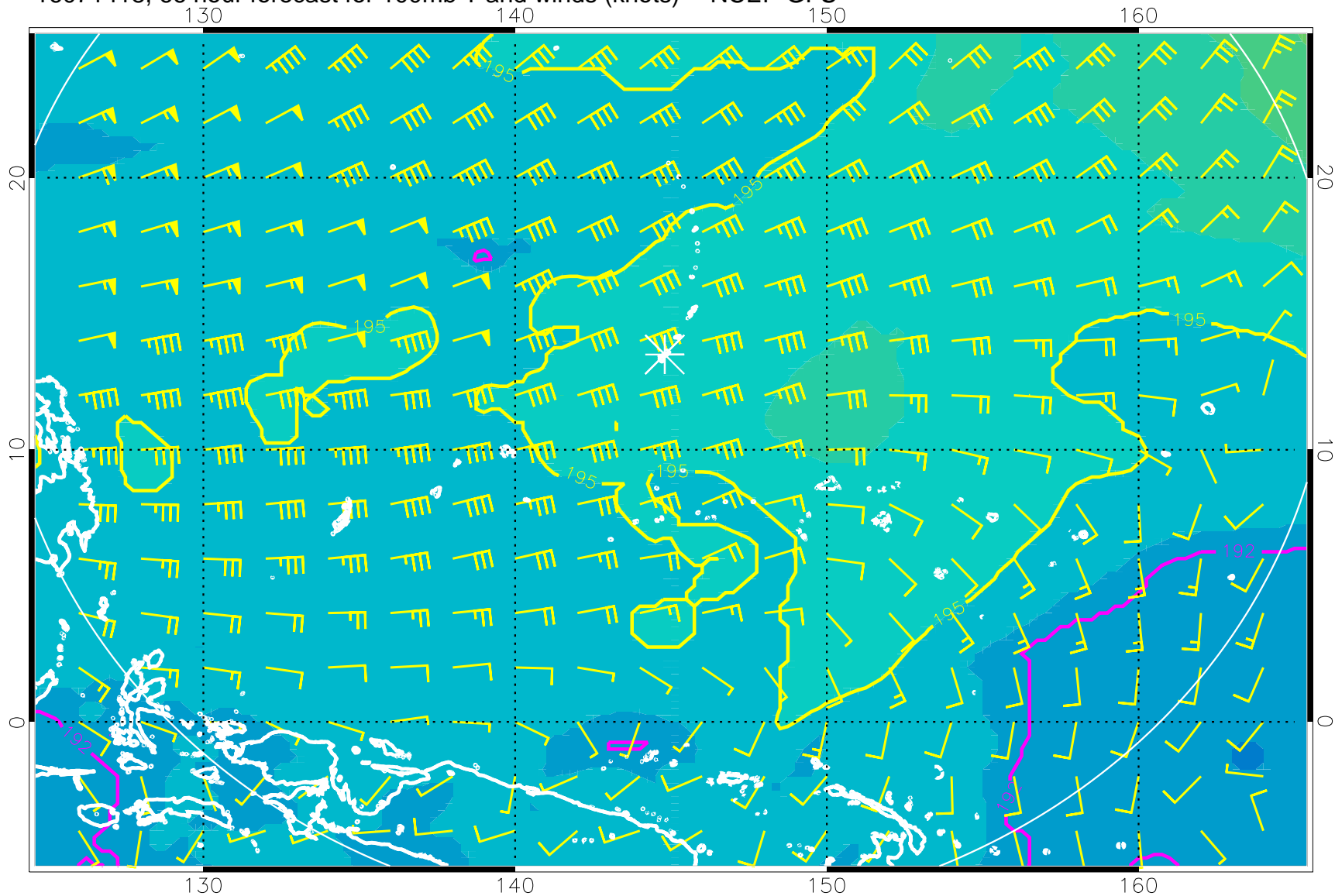
16071418, 66 hour forecast for 100mb T and winds (knots) -- NCEP GFS
