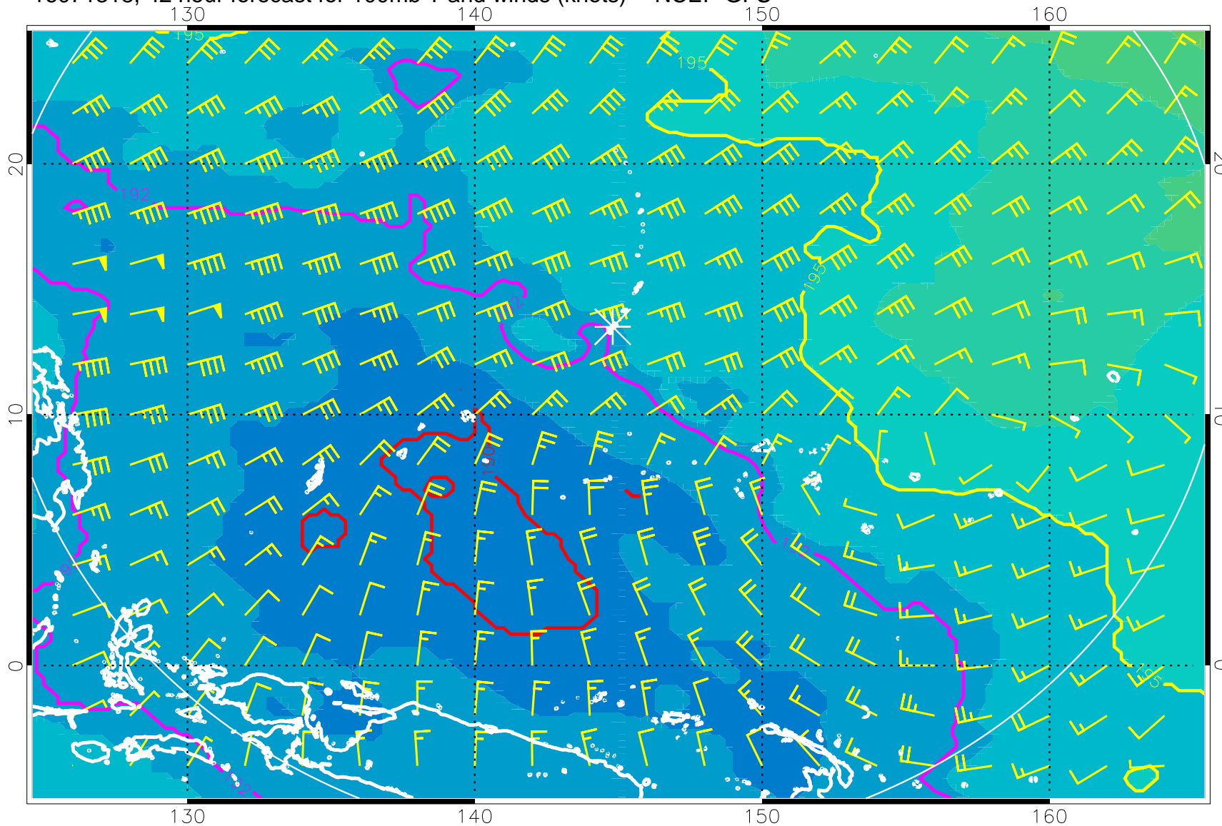
16071318, 42 hour forecast for 100mb T and winds (knots) -- NCEP GFS
