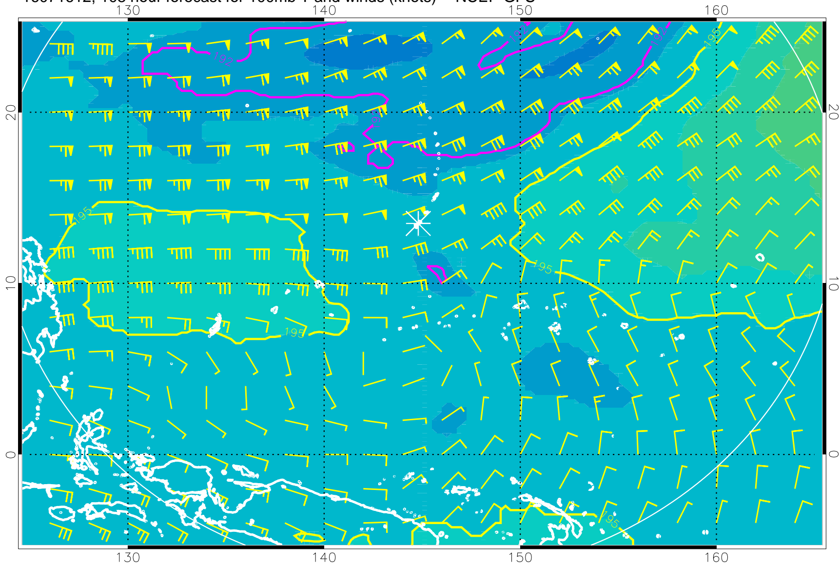
16071612, 108 hour forecast for 100mb T and winds (knots) -- NCEP GFS
