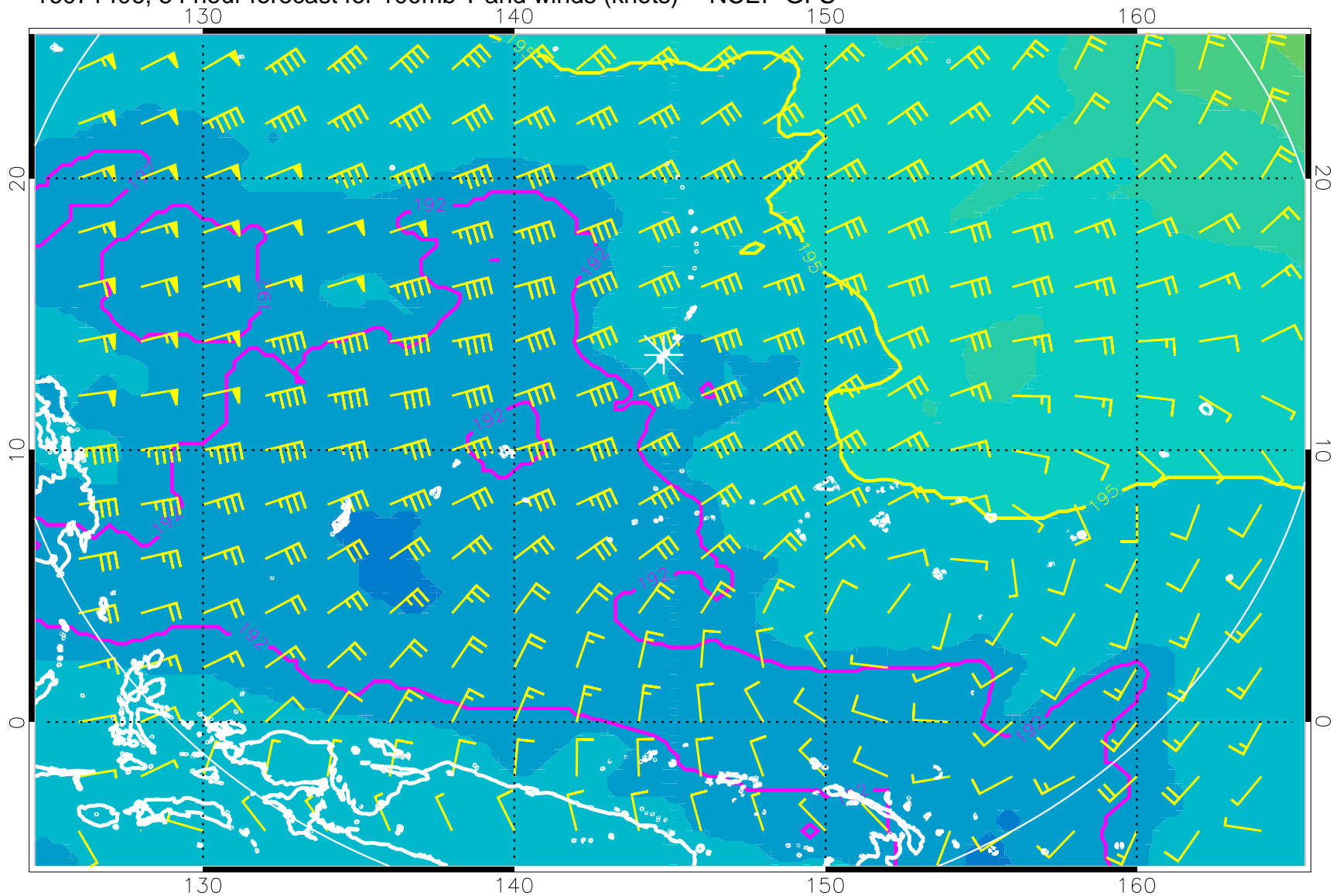
16071406, 54 hour forecast for 100mb T and winds (knots) -- NCEP GFS
