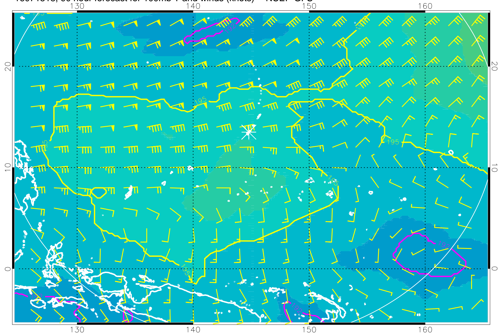
16071518, 90 hour forecast for 100mb T and winds (knots) -- NCEP GFS
