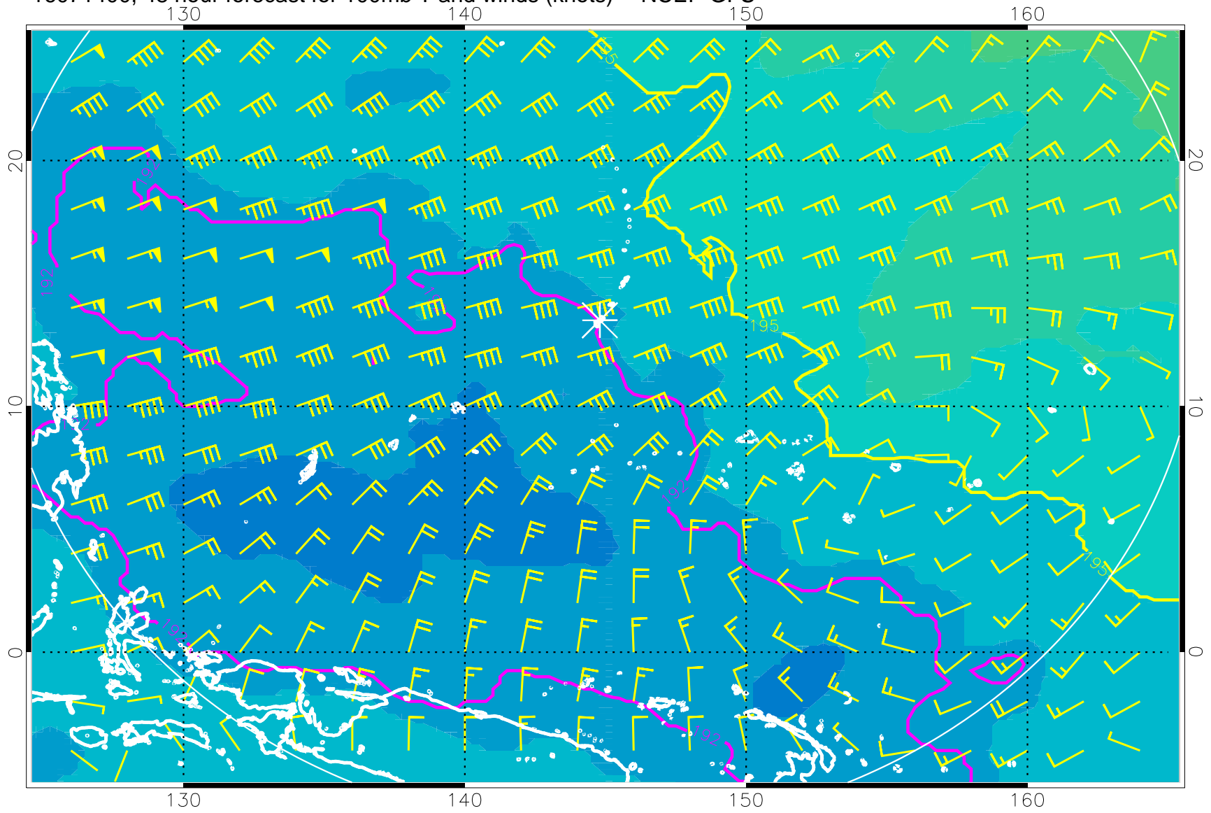
16071400, 48 hour forecast for 100mb T and winds (knots) -- NCEP GFS
