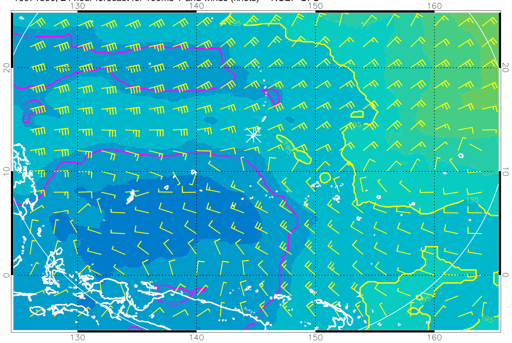
16071300, 24 hour forecast for 100mb T and winds (knots) -- NCEP GFS
