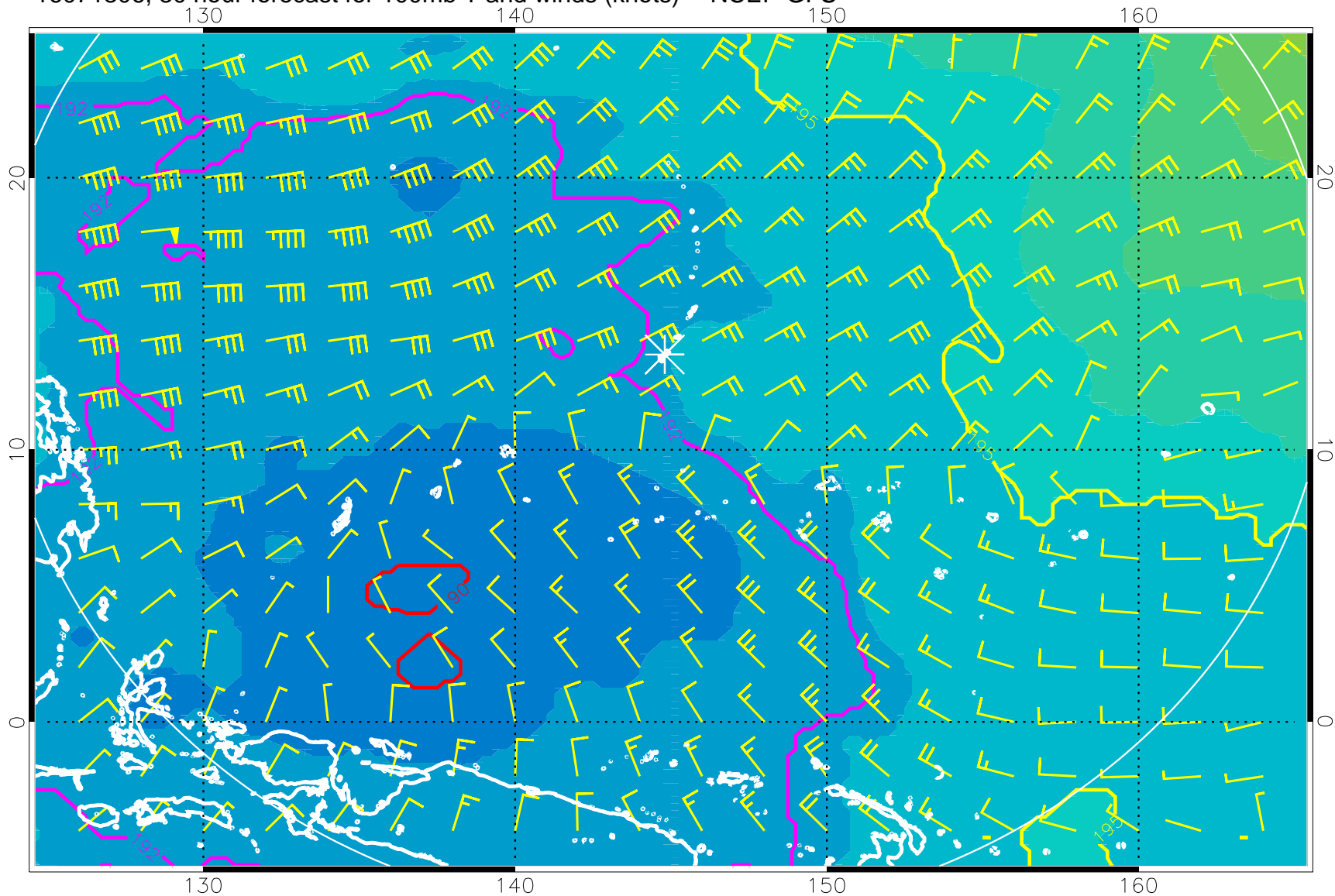
16071306, 30 hour forecast for 100mb T and winds (knots) -- NCEP GFS
