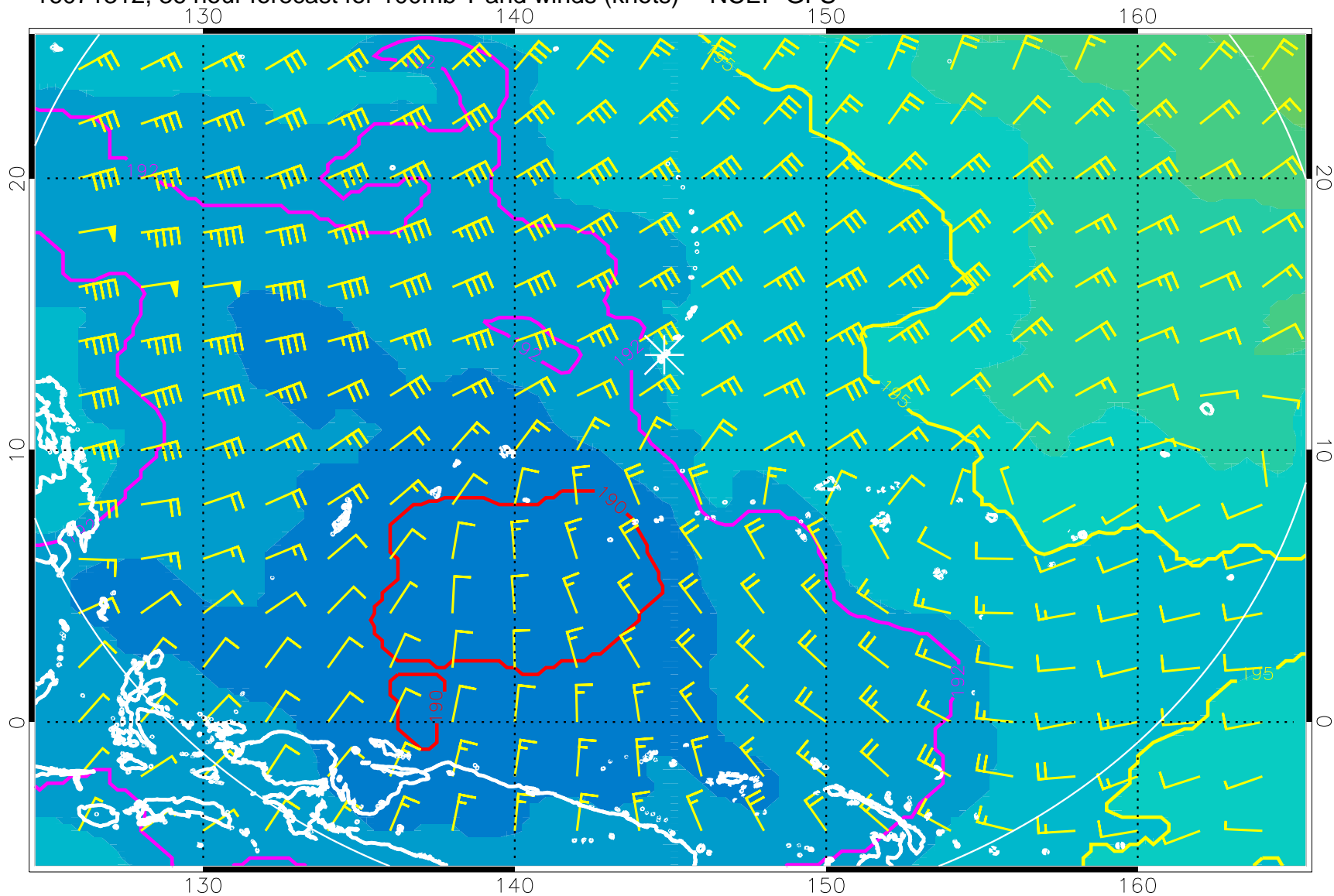
16071312, 36 hour forecast for 100mb T and winds (knots) -- NCEP GFS
