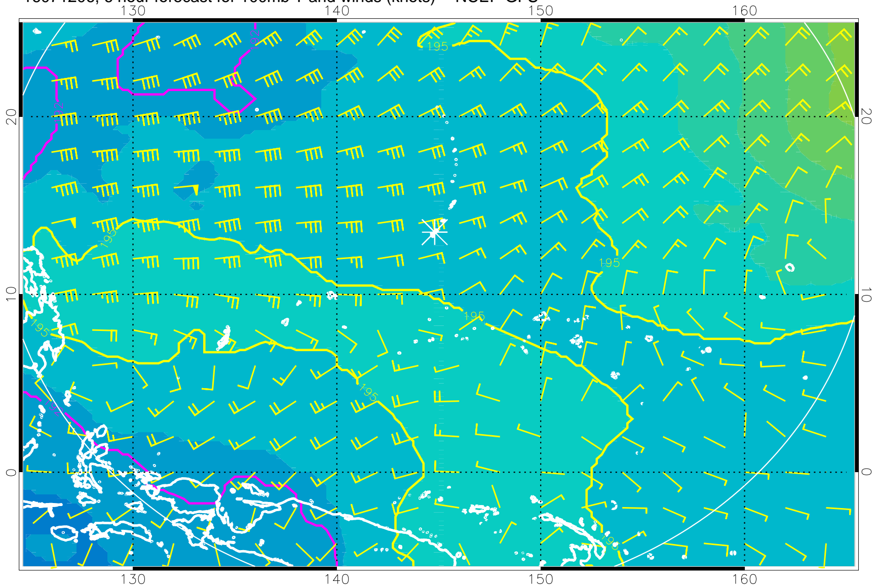
16071206, 6 hour forecast for 100mb T and winds (knots) -- NCEP GFS
