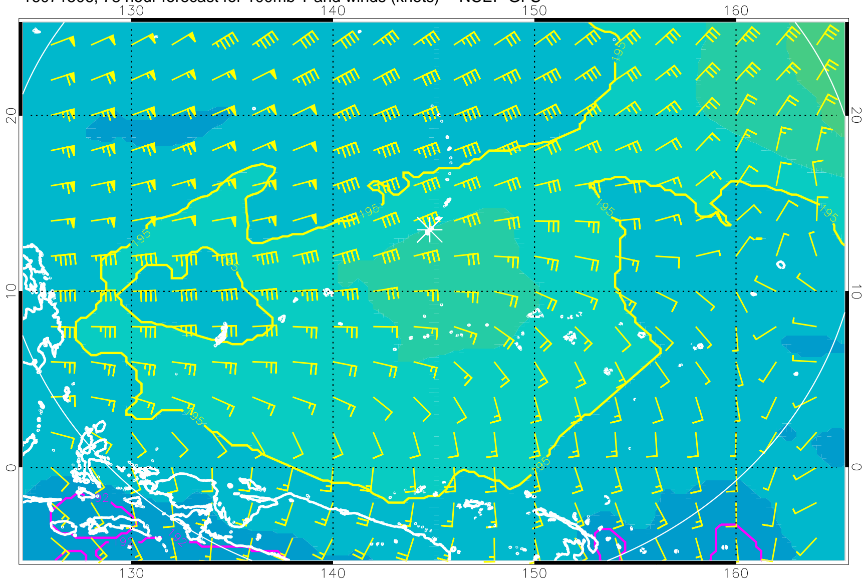
16071506, 78 hour forecast for 100mb T and winds (knots) -- NCEP GFS
