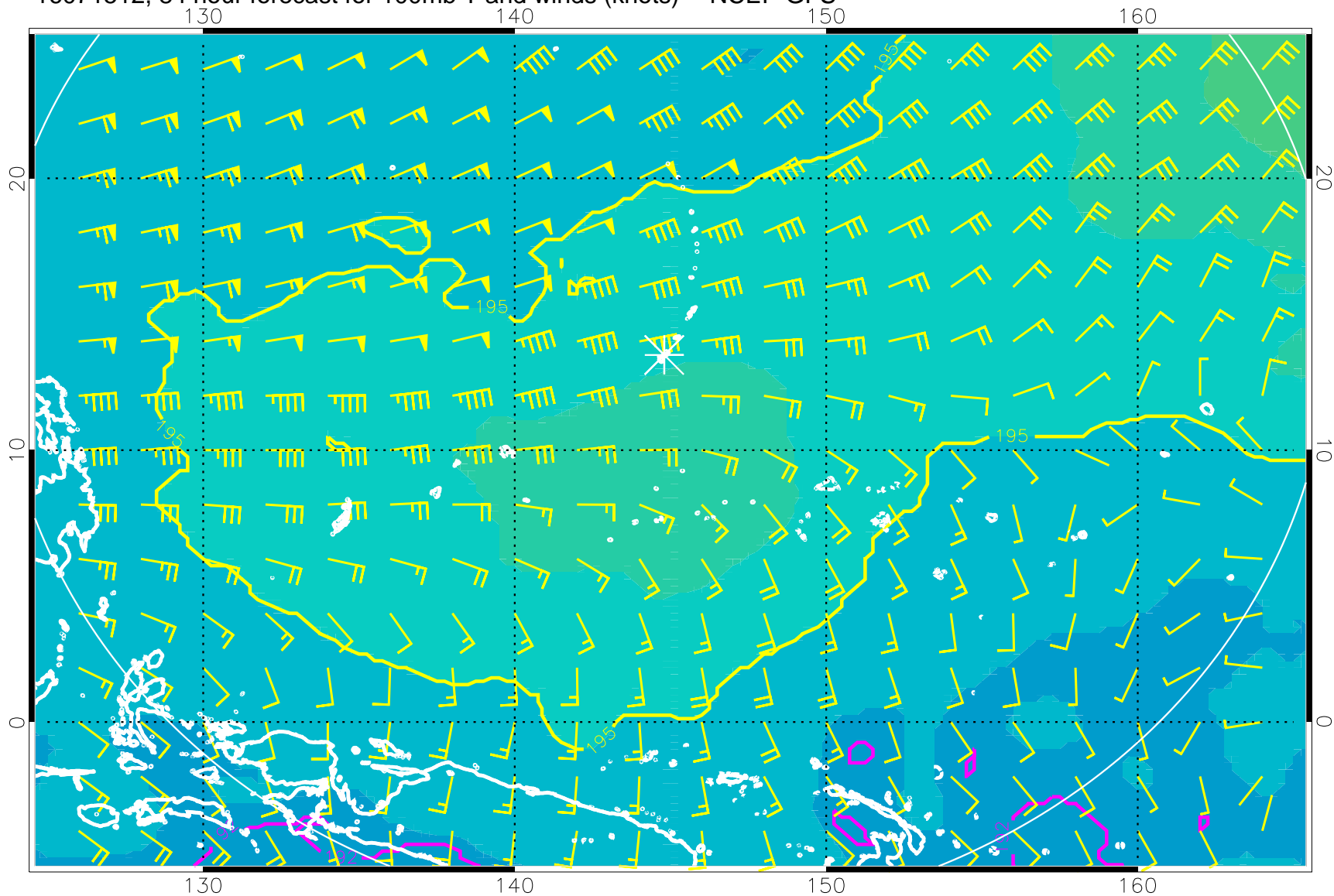
16071512, 84 hour forecast for 100mb T and winds (knots) -- NCEP GFS
