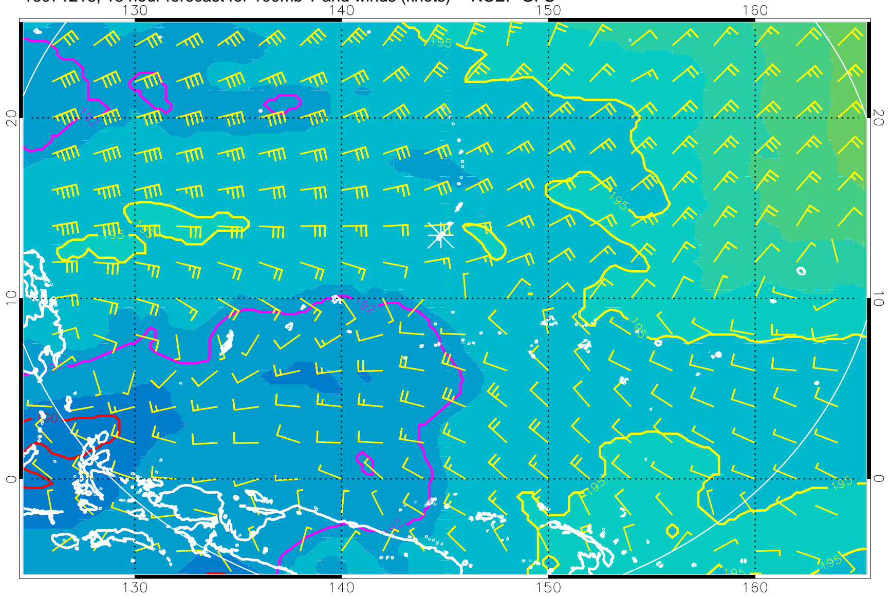
16071218, 18 hour forecast for 100mb T and winds (knots) -- NCEP GFS
