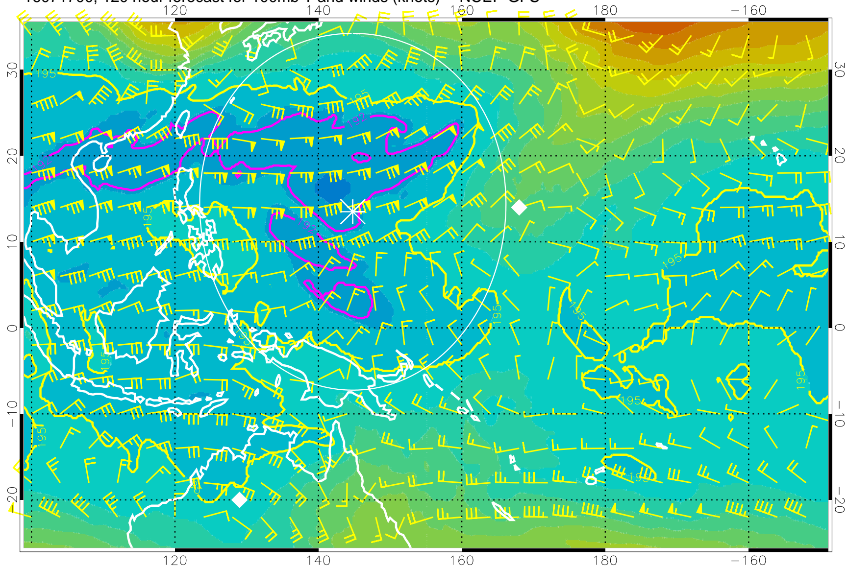
16071700, 120 hour forecast for 100mb T and winds (knots) -- NCEP GFS
