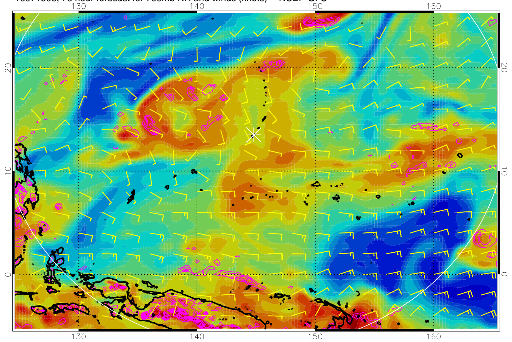
16071506, 78 hour forecast for 700mb RH and winds (knots) -- NCEP GFS
