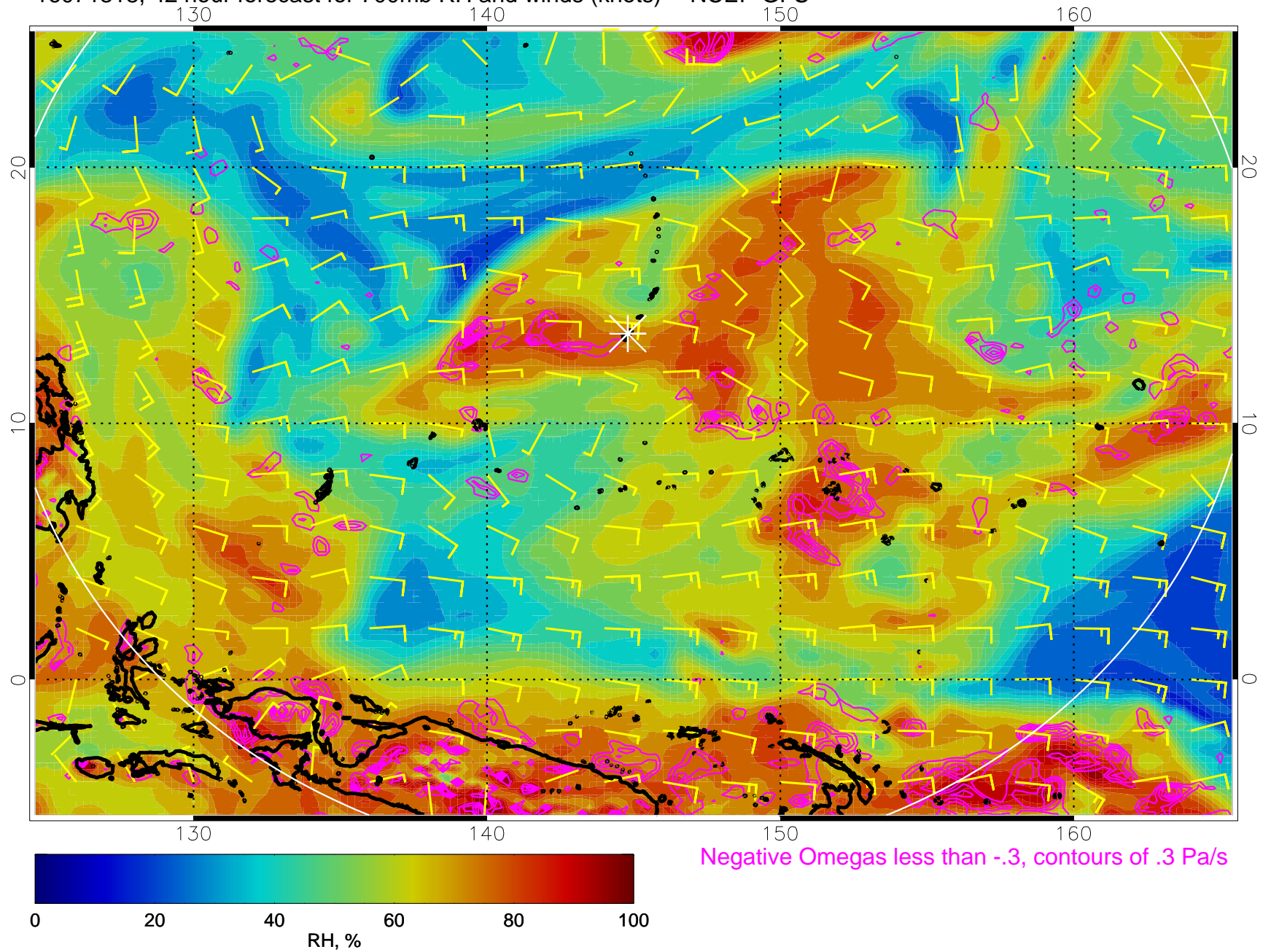
16071318, 42 hour forecast for 700mb RH and winds (knots) -- NCEP GFS
