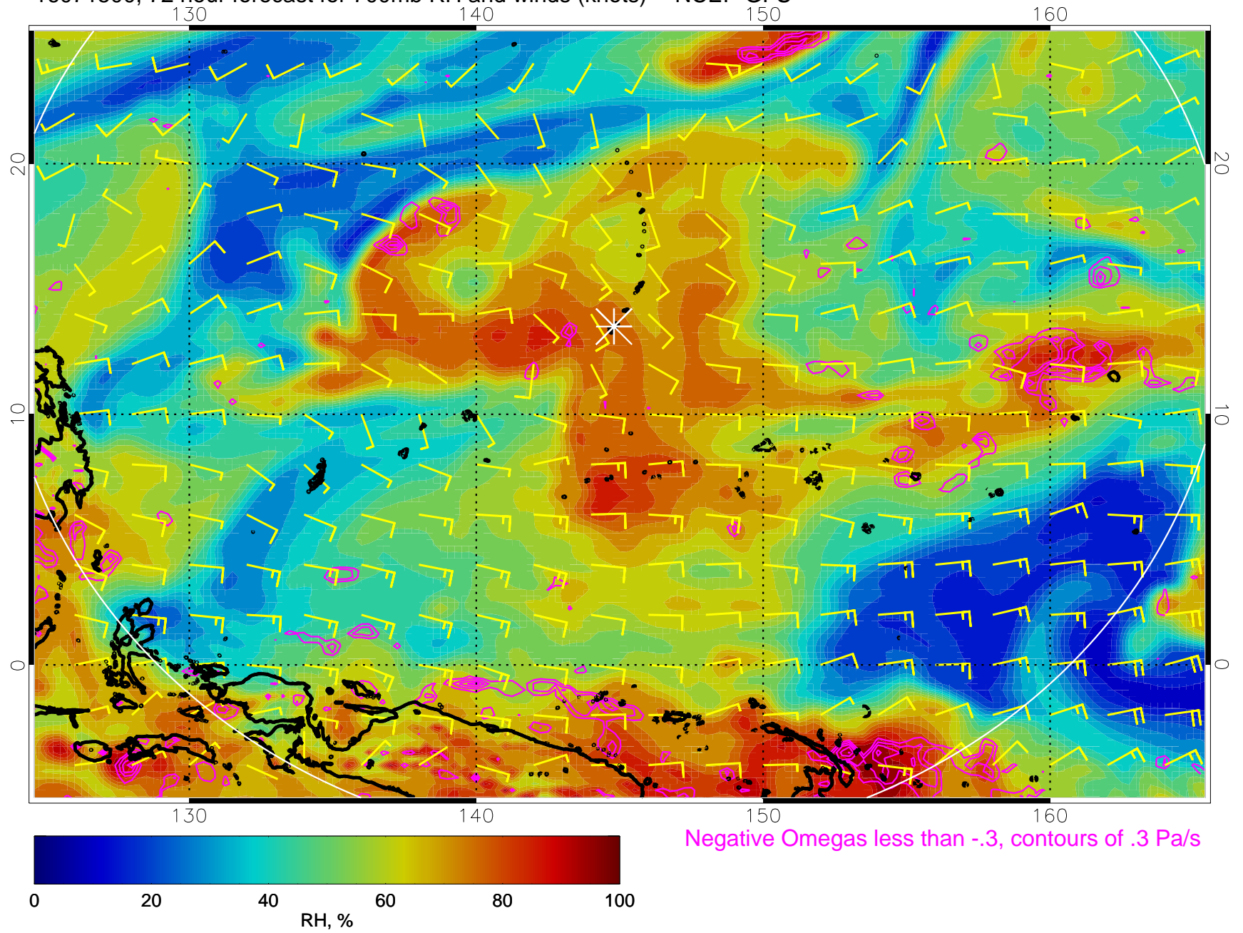
16071500, 72 hour forecast for 700mb RH and winds (knots) -- NCEP GFS
