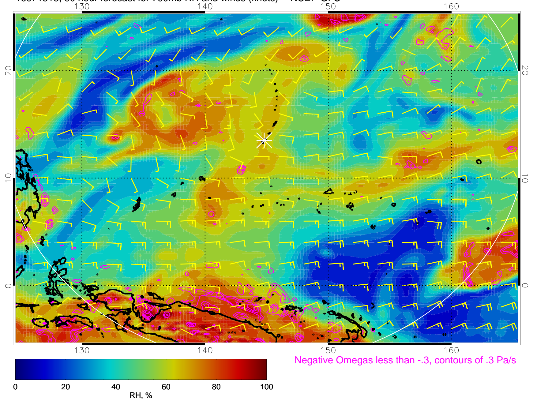
16071518, 90 hour forecast for 700mb RH and winds (knots) -- NCEP GFS
