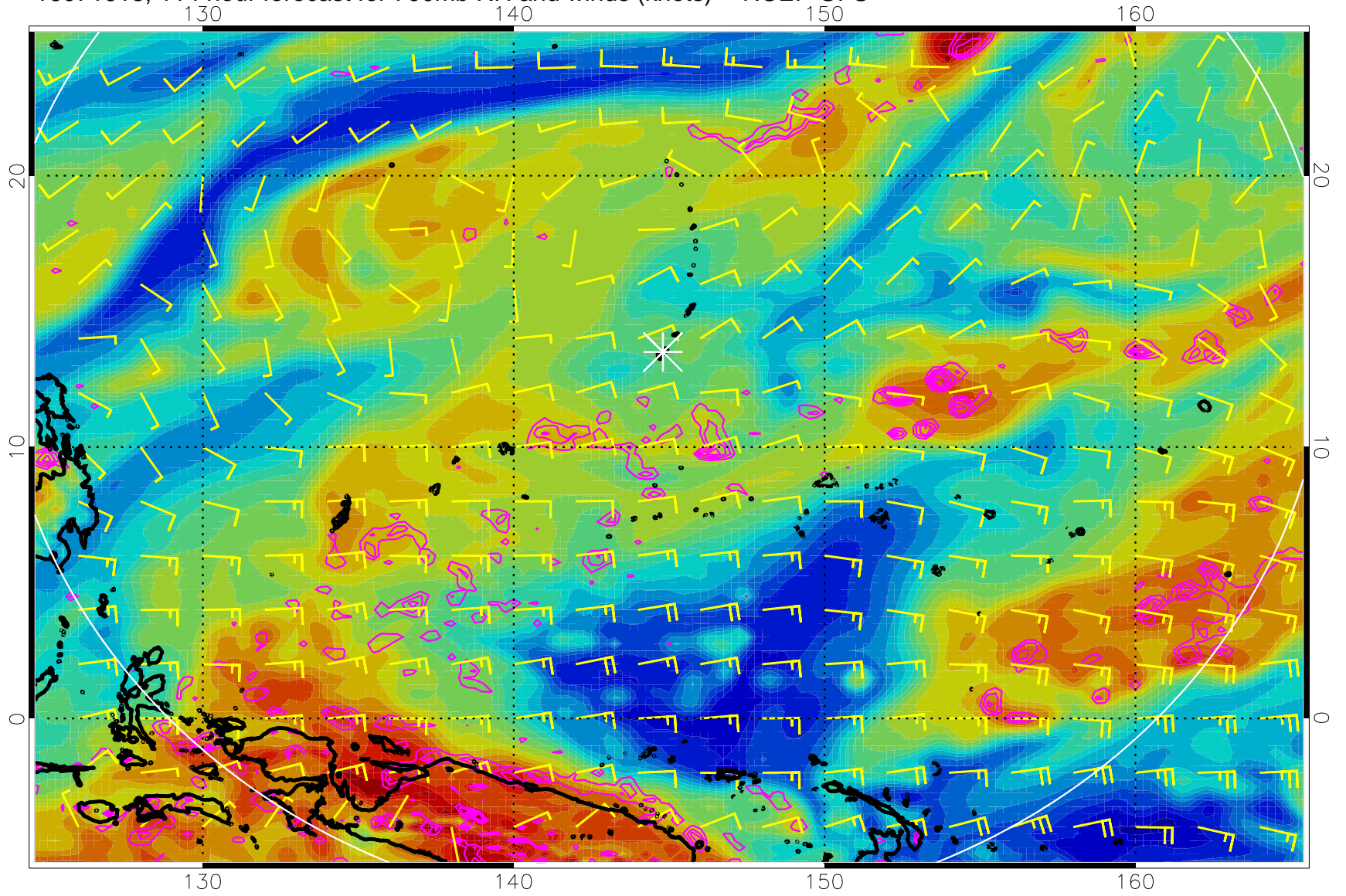
16071618, 114 hour forecast for 700mb RH and winds (knots) -- NCEP GFS
